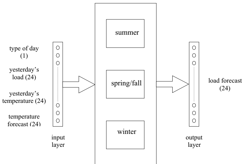
Figure 2.7 Block Diagram
