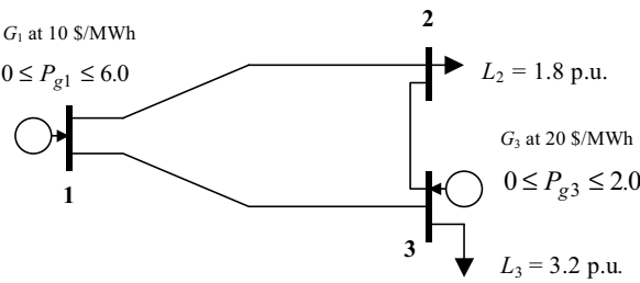
a. System Configuration
