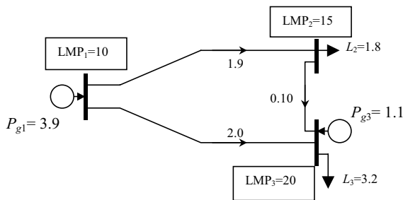
c. Solution When Line Limits are Considered
