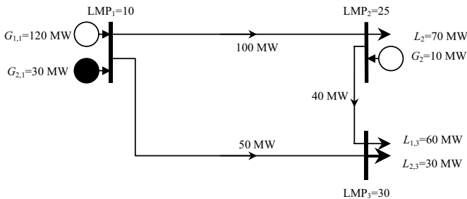
Figure F.1 Example of a 3-Bus System
