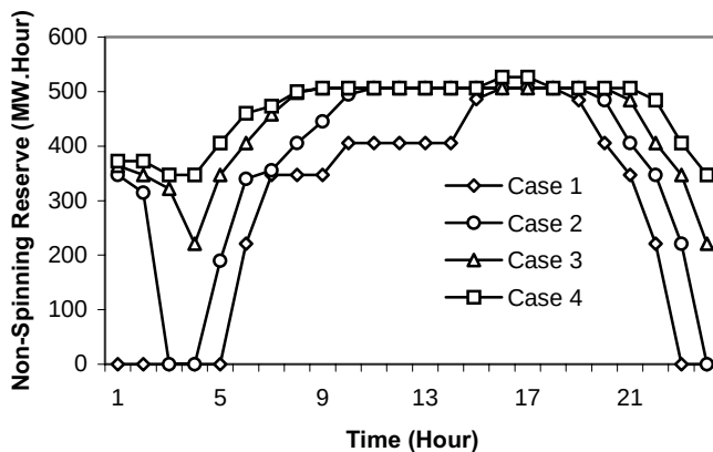
Figure 4.13 Sensitivity Analysis: Non-spinning Reserve Sale
