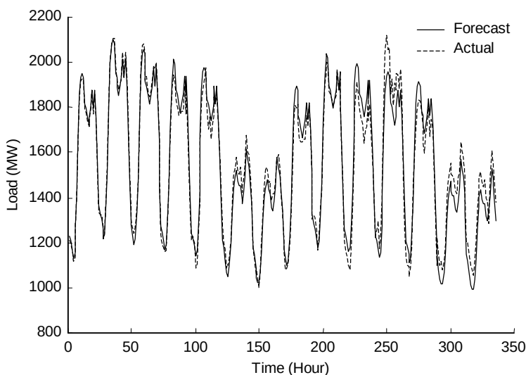
Figure 2.20 Spring Model's 14-Day Forecast
