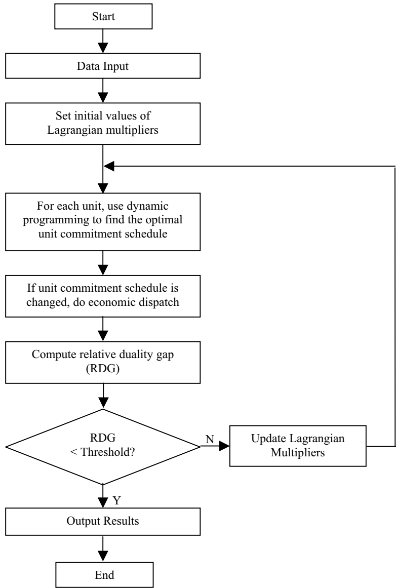
Figure 4.1 PBUC Flowchart
