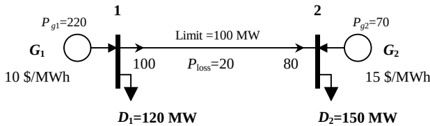
Figure 10.10 Optimal Dispatch
