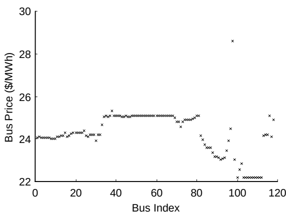
Figure 3.7 Price Profile for 118-Bus System
