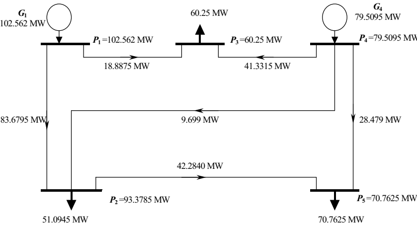
Figure 10.3 Lossless Power Flow
