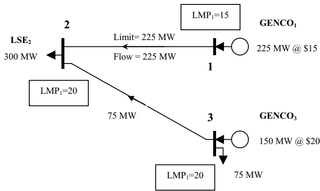
Figure 10.15 Constrained System
