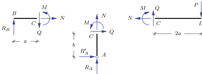
Fig. 3.57: Internal forces by sections in C .
