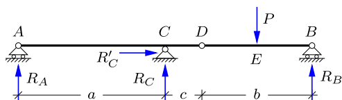
Fig. 3.19: Hinged beams with concentrated force.
