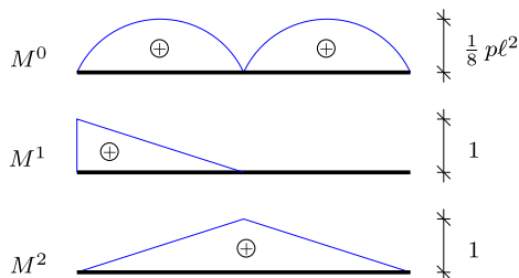
Fig. 6.24: Summary of moment distributions.
