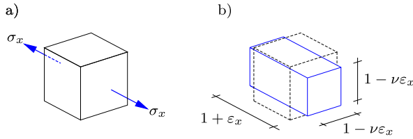
Fig. 9.4: Tension \sigma_x with elongation \varepsilon_x and transverse contraction \nu\varepsilon_x .
