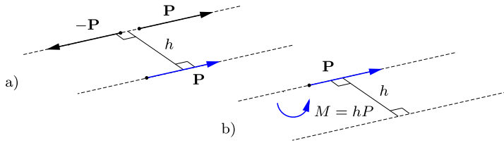
Fig. 1.11: Offset of force by introduction of moment.
