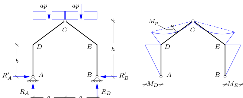
Fig. 3.66: Three-hinge frame with uniformly distributed load.
