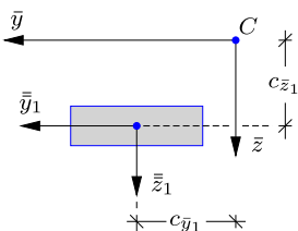
Fig. 10.17: Rectangular flange.
