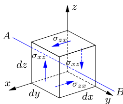
Fig. 8.7: Stress components for moment equilibrium about y -axis.
