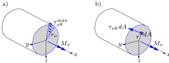
Fig. 11.32: Linear radial dependence of shear stress in cylinder.
