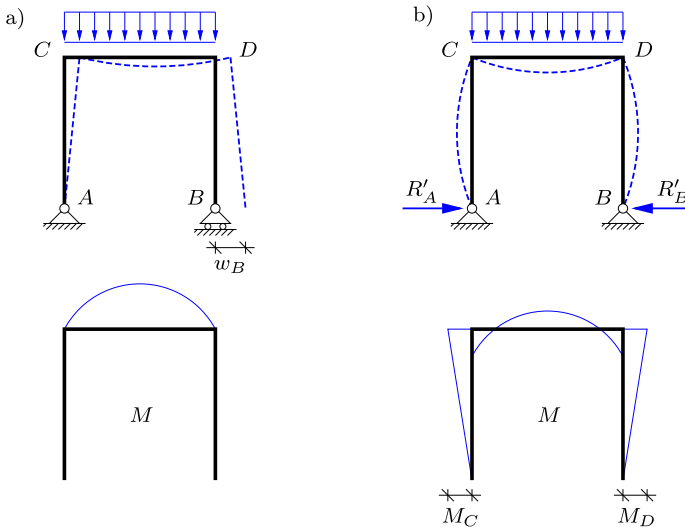
Fig. 6.32: Moment reduction in frame by additional support.
