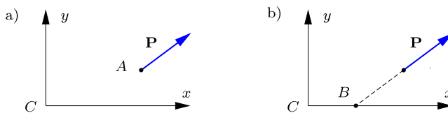
Fig. 1.8: Moment by horizontal and vertical force components.
