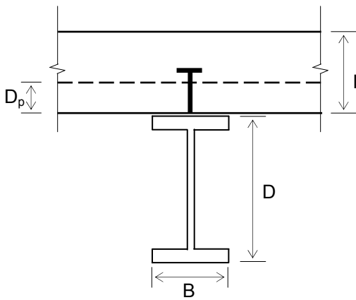
b) Composite beam with composite slab using trapezoidal and re-entrant sheet profiles (Beam span perpendicular to slab span)
