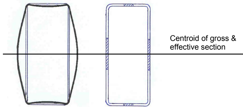
(a) Local buckling (b) Effective section
