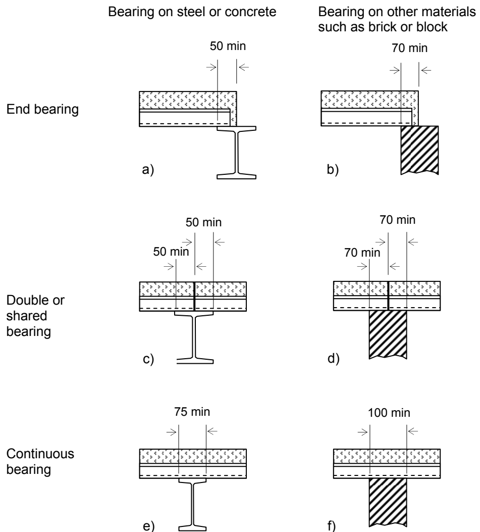
Figure 10.16 - Bearing requirements
