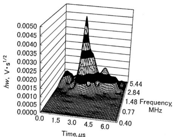
Figure A1-20 Wavelet transform of reflected waves.
