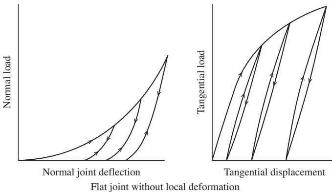
Figure 6-44 Comparison of load-deflection curves for representative flat joints.
