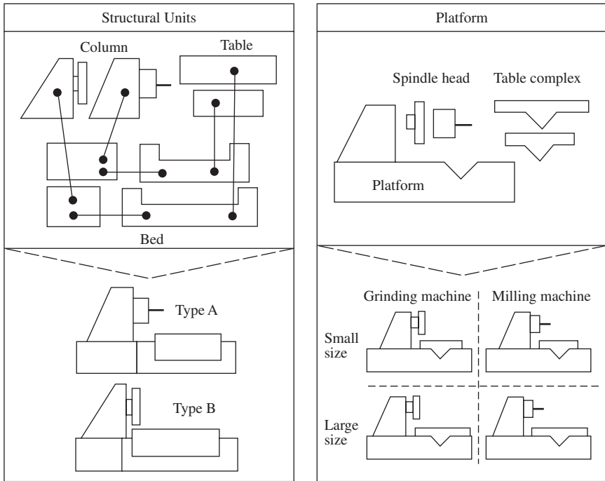
Figure 2-2 Concept of platform to enhance reusability of structural entities—an advanced concept of modular design by Metternich and Würsching (courtesy of Carl Hanser).
