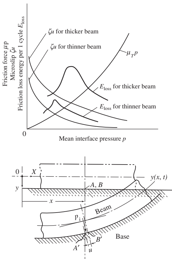
Figure 7-30 Damping mechanism of bolted joint of type A.
