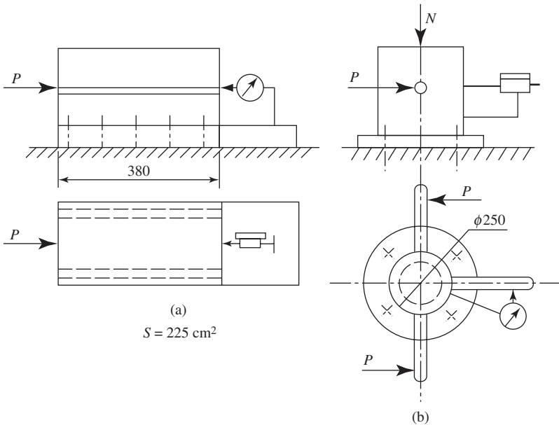
Figure 6-13 Test rigs of Kirsanova: (a) Linear type and (b) circular type.
