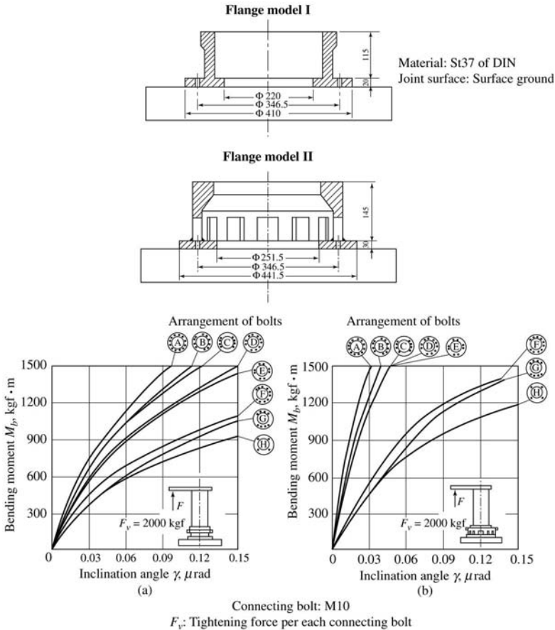
Figure 7-29 Effects of arrangement and number of connecting bolts for a large model: (a) Flange model I and (b) flange model II (by Plock, courtesy of Industrie-Anzeiger).
