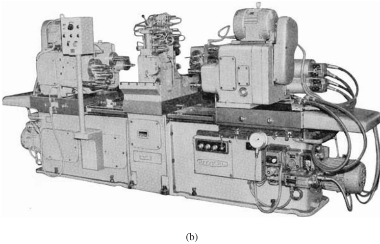
Figure 1-19 Rotary indexing machine and its variant in the 1960s: (a) Rotary indexing machine for large-volume production of precision parts (by Seiko) and (b) three-way drilling machine—a variant of rotary indexing machine (by Hitachi).
