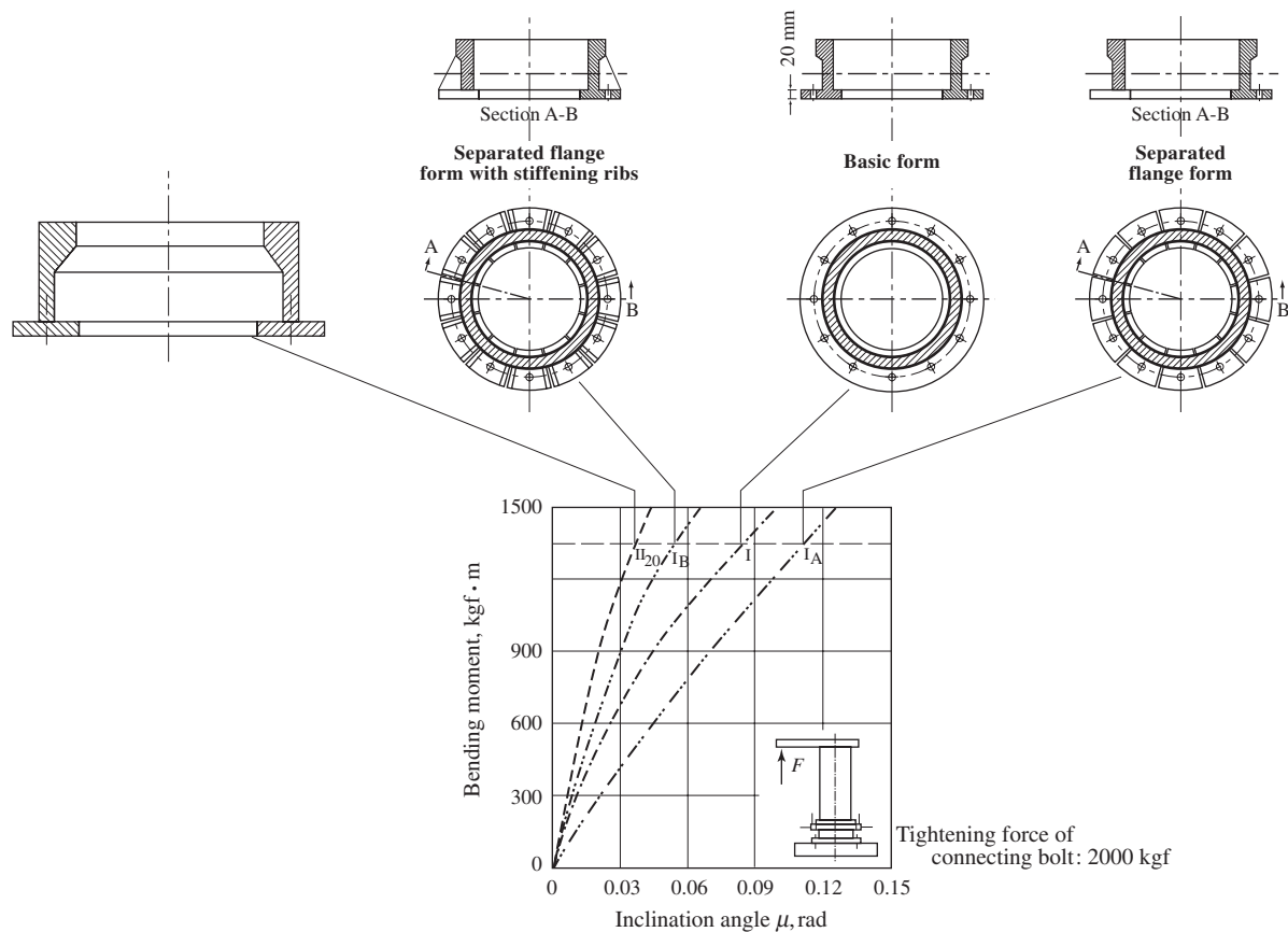
Figure 7-23 Effects of allocation of connecting bolts and flange configurations (by Plock, courtesy of Industrie-Anzeiger).
