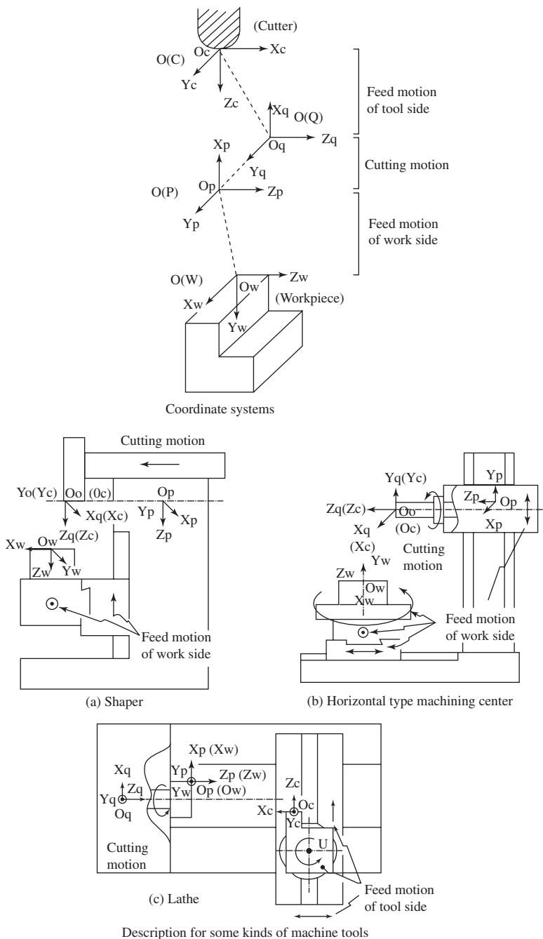
Figure 3-6 A variant of functional description (courtesy of Iwata).
