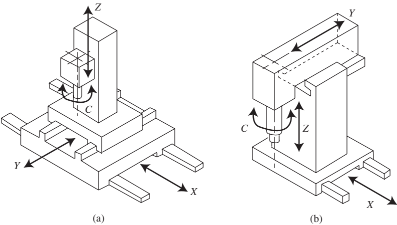
Figure 4-3 Structural configurations corresponding to functional description /XYZC —certain constraint due to description simplicity.
