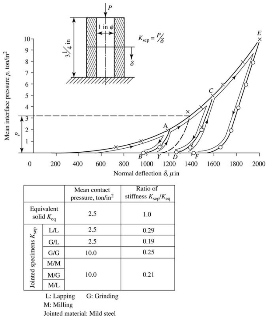
Figure 5-19 Normal deflection in flat joint under higher interface pressure (by Thornley et al. [15]).
