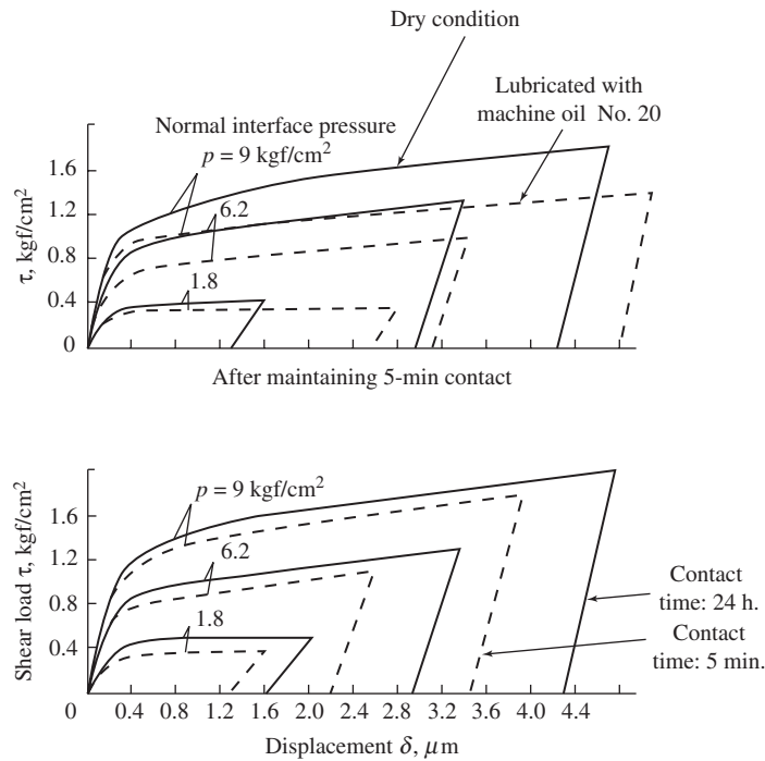
Figure 6-12 Load-deflection curve at first loading cycle (linear type, by Kirsanova).
