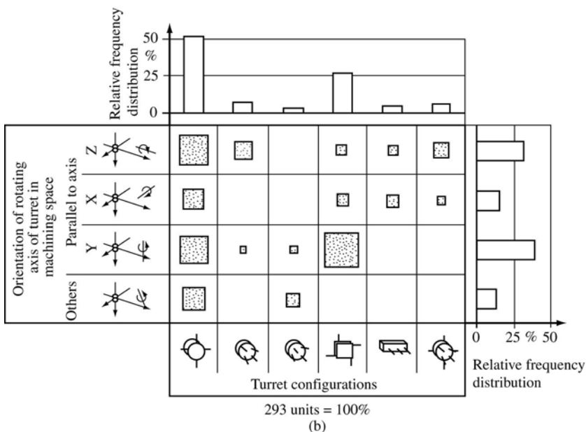
Figure 2-1 Frequency distributions for: (a) Traveling ranges and (b) structural configuration and rotating axis of turret in NC turning machines (by Feldmann).
