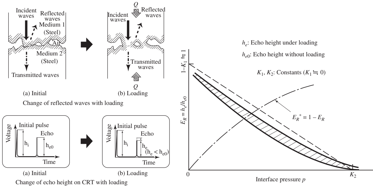
Figure A1-5 Schematic views for measuring principles and fundamental relationships between E_R^* and p .
