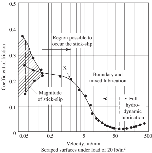
Figure 8-5 General lubrication characteristics of slideway (by PERA).
