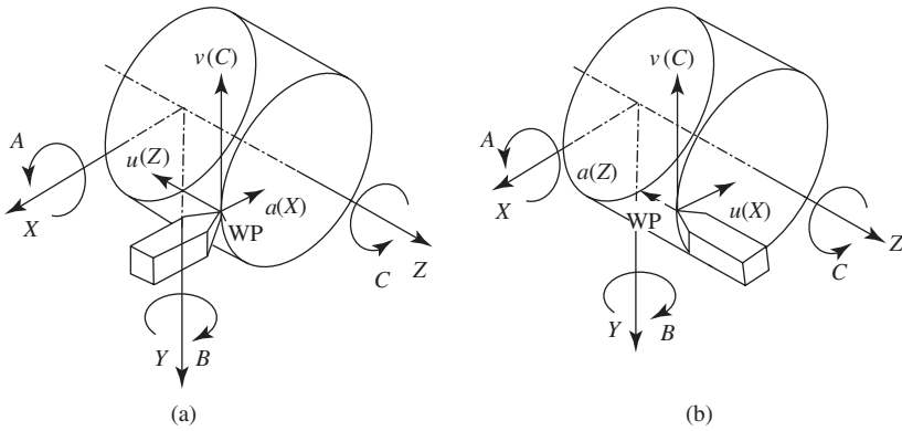
Figure 3-3 Relative movements of cutting tool and work: (a) Cylindrical turning and (b) face turning (courtesy of Saljé).
