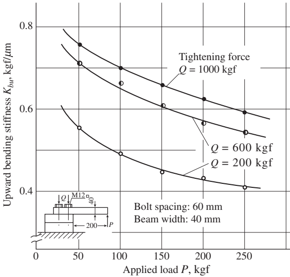
Figure 7-3 Load and tightening force dependence of joint stiffness—separation in joint.
