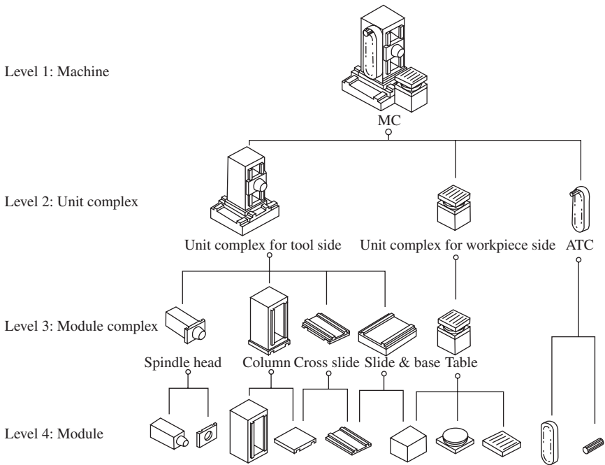
Figure 1-8 Hierarchical structure of MC with modular design.
