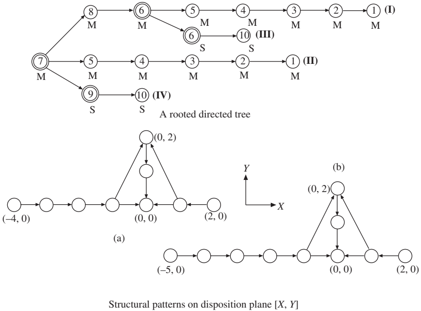
Figure 4-18 Rooted directed tree and disposition plane: (a) Planomiller of double column type and (b) planer of double column type.
