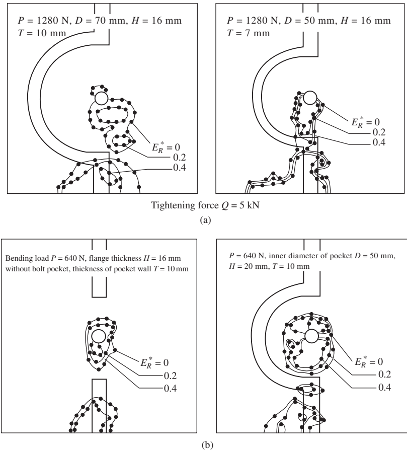
Figure 7-25 Interface pressure distribution in parallel loading: (a) Varying the pocket configuration and (b) effect of the bolt pocket.
