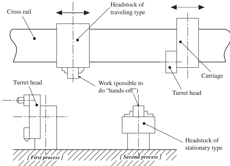
Figure 2-28 NC vertical machine of Hüller Hille make.
