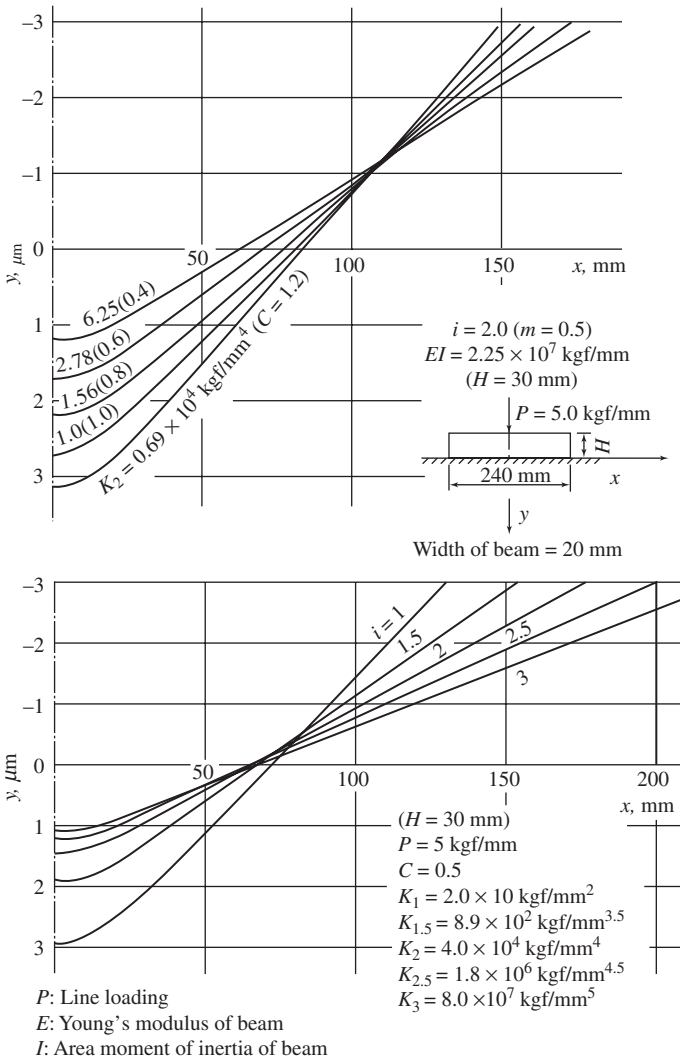
Figure 6-38 Effects of C and m on deformation pattern of cast iron beam.
