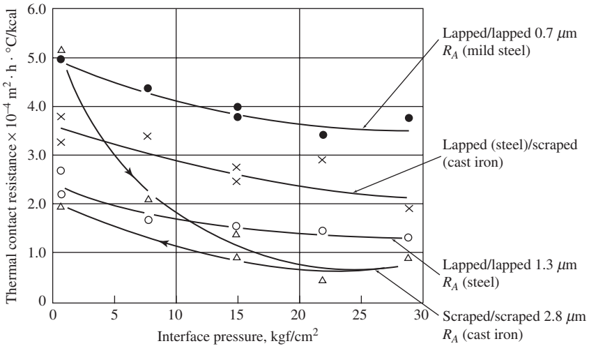
Figure 6-35 Thermal contact resistance in dry joint (courtesy of Yoshida).
