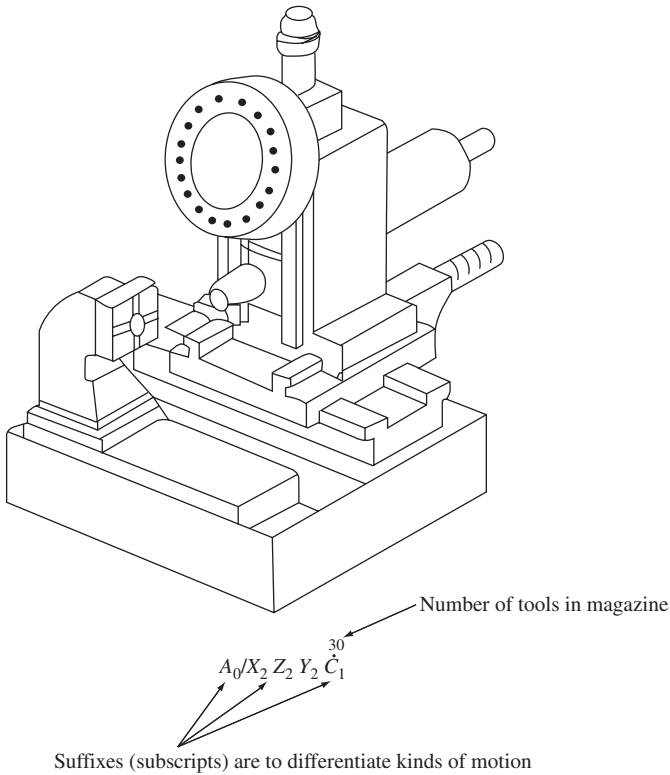
Figure 4-6 Description of MC of column traveling type (MX3, Ikegai Iron Works make, refer to Fig. 1-4).
