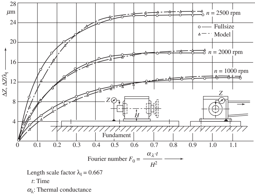
Figure 5-23 Model testing for thermal deformation of main spindle (by Schossig).
