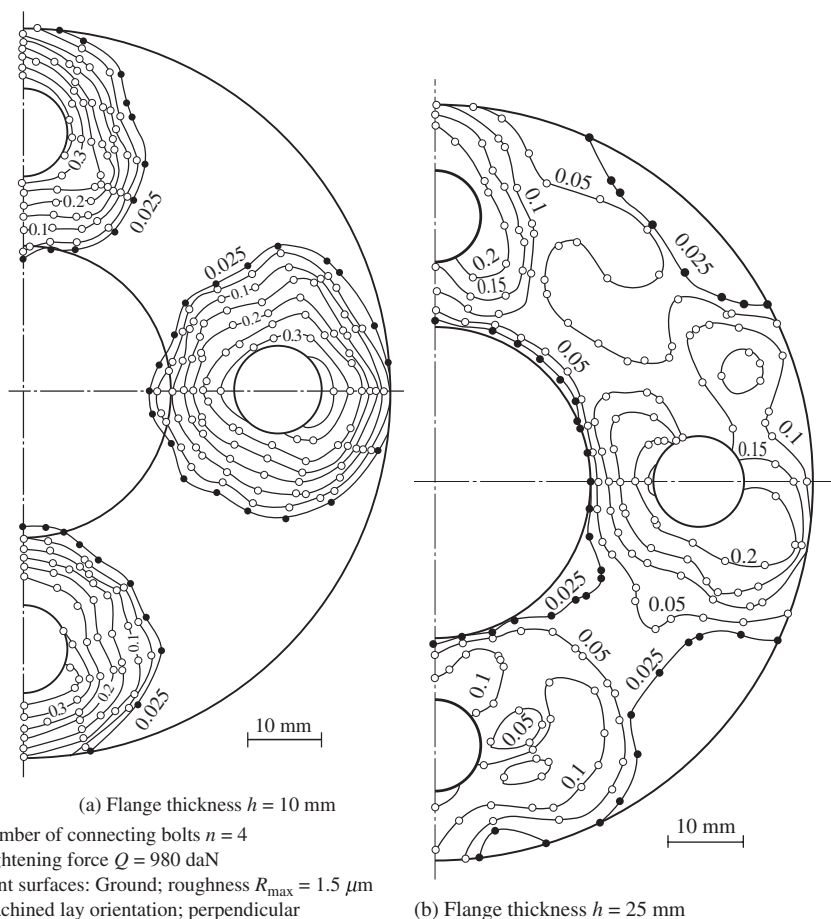
Figure A1-14 Interface pressure distribution in multiple-bolt-flange assembly.
