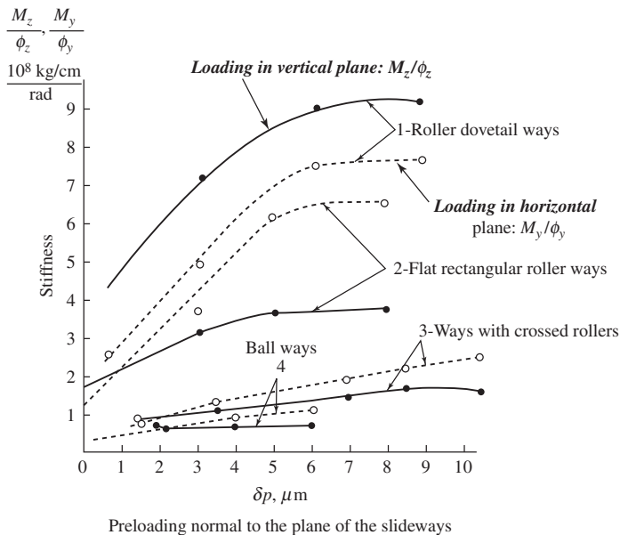
Figure 8-24 Relationships between stiffness of linear rolling guideways and preloading (by Levina).
