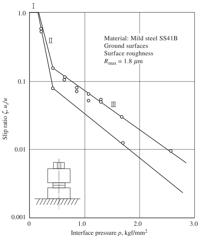
Figure 7-37 Characteristics of microslip in single bolted joint.
