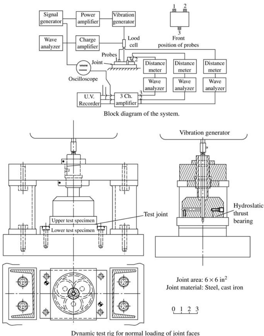
Figure 6-29 Test rig and measuring system for single flat joint (courtesy of Thornley).
