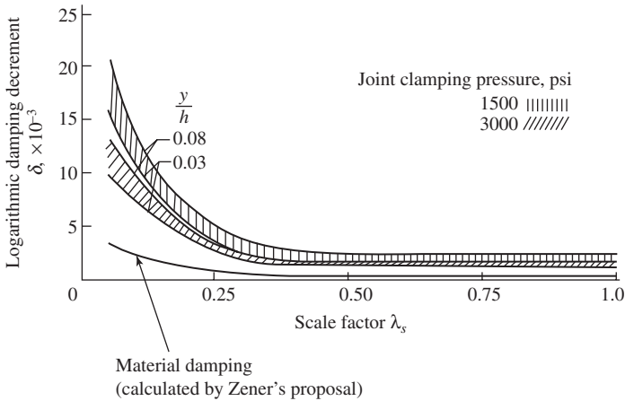
Figure A2-7 Model testing for damping capacity (by Hanks and Stephens).
