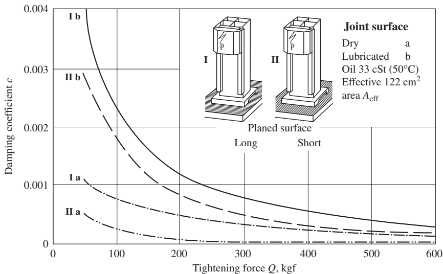
Figure 7-6 Effect of tightening force on damping capacity in consideration of machined lay orientation (courtesy of Groth).
