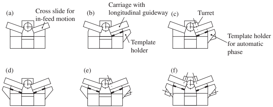
Figure 1-28 Modular design in turning machine of Fronter type (courtesy of Saljé).
