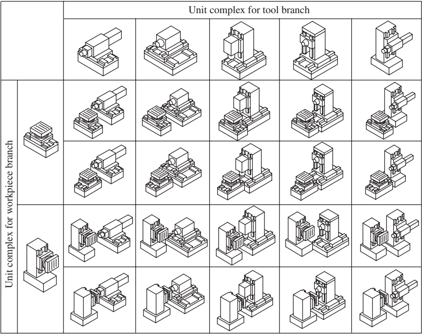
Figure 4-33 Some structural configurations of MC generated from unit complexes.
