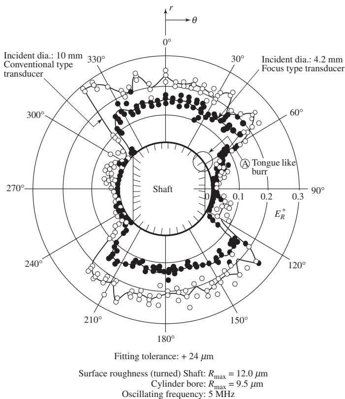
Figure A1-10 Examples of measured contact patterns.
