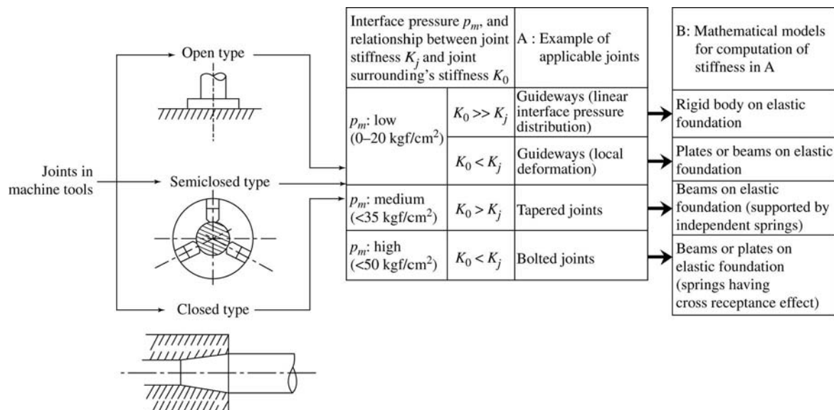
Figure 6-2 Classification of machine tool joints to determine mathematical models.
