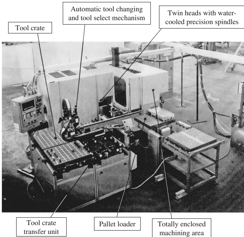
Figure 2-21 A system machine (type AUTOMAX I, courtesy of MPM Co.).
