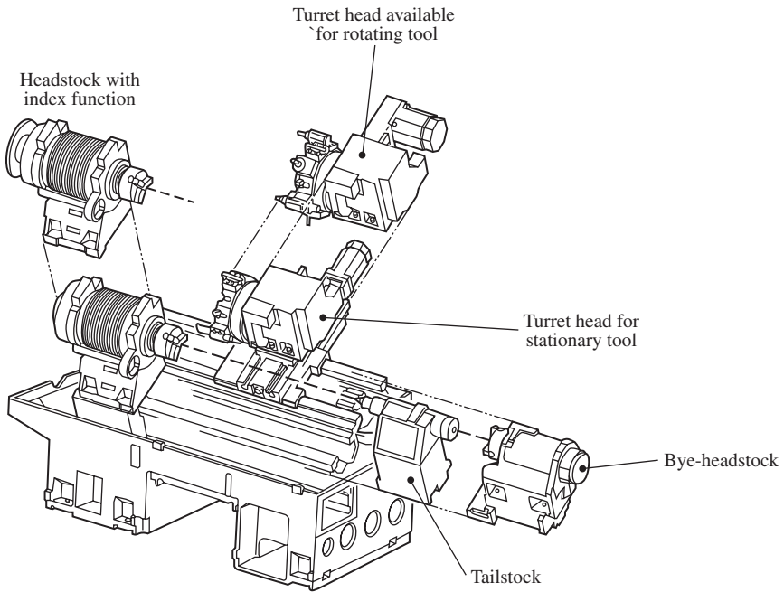
Figure 2-10 A unit construction for TC (type SL, courtesy of Mori Seiki).
