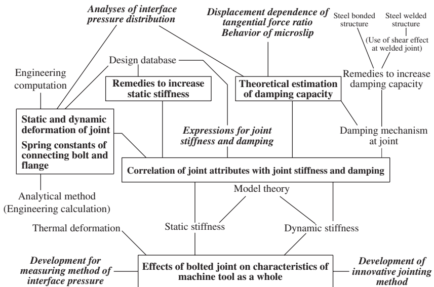
Figure 7-2 Research and engineering development subjects of bolted joint in machine tools.
