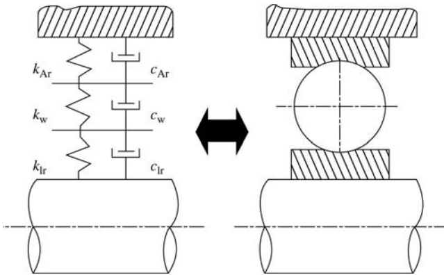
Figure 8-27 A mathematical model of rolling bearing (by Weck, courtesy of Industrie-Anzeiger).
