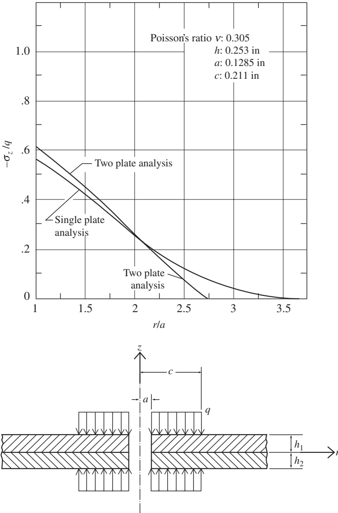
Figure 7-16 Finite element analysis for bolt-flange assembly of 1/4-in plate pair (by Gould and Mikic, courtesy of ASME).
