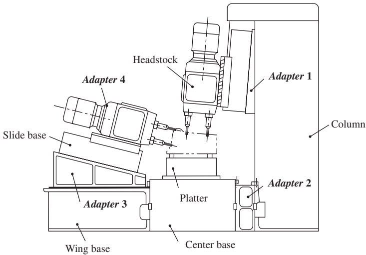
Figure 1-26 Allocation example of adapters.
