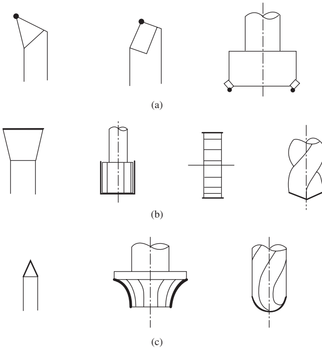
Figure 3-7 Classification of form entities: (a) Pointlike cutting edge; (b) linelike cutting edge; and (c) formed cutting edge (courtesy of Iwata).
