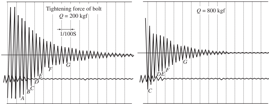
Figure 6-23 Records of stick-slip-like amplitude changes in damped decay-free vibration.
