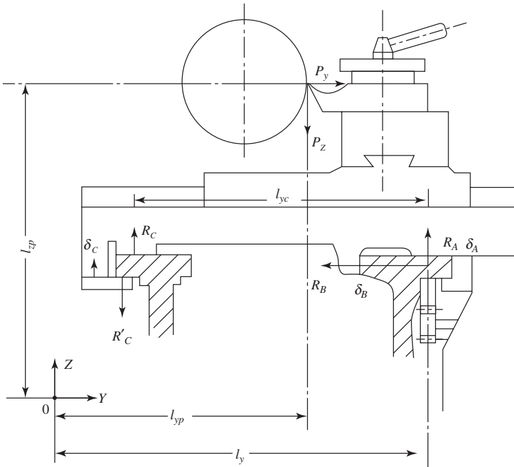
Figure 8-S1 Carriage of engine lathe.
