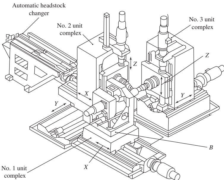
Figure 2-25 Concept of complex machining center developed by Japanese Big National Project in the 1970s.
