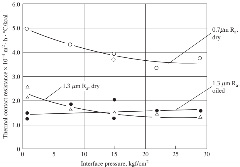
Figure 6-36 Thermal contact resistance in lapped joint with oil (courtesy of Yoshida).
