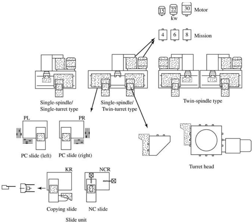
Figure 1-35 Unit construction of NC turning machine in the 1970s (type DP250 of VDF Heidenreich Harbeck make).
