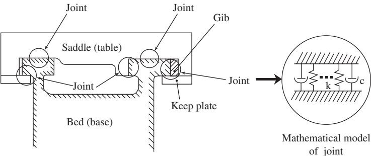
Figure 5-10 Joints in slideway and mathematical model of joint.
