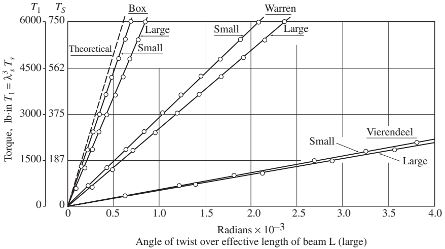
Figure A2-3 Model testing for lathe beds of boxlike type under torsion (by Thornley).
