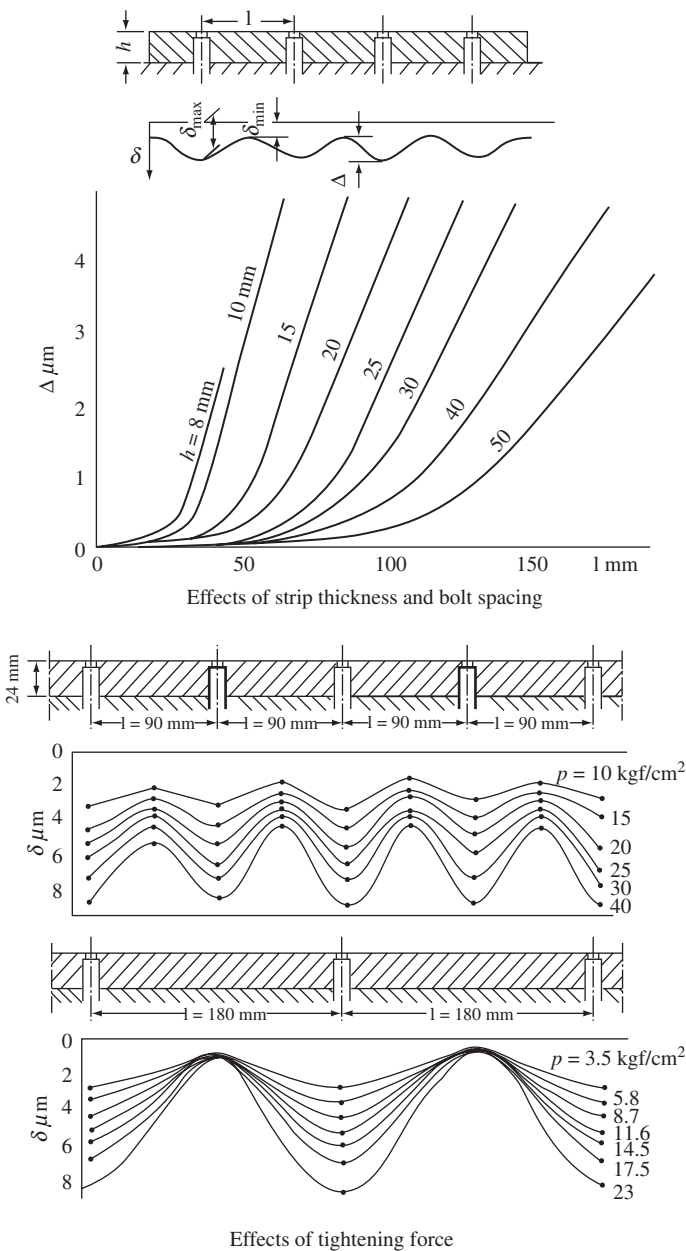
Figure 7-S2 Determination of preferable bolt spacing in hardened strip bolted on bed slideway (by Levina).
