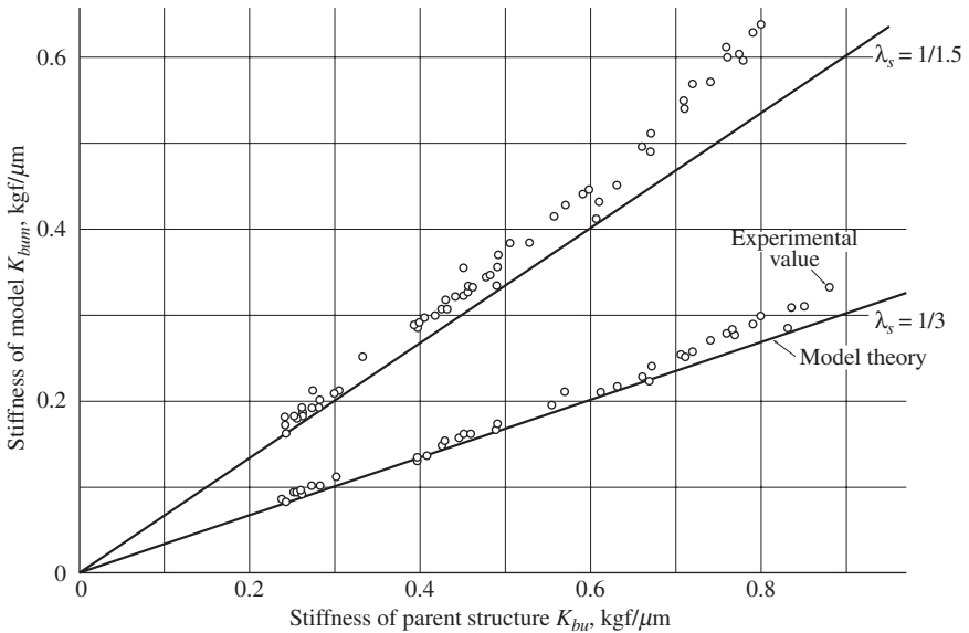
Figure A2-4 Model testing in consideration of joint: upward bending stiffness of bolted cantilever.
