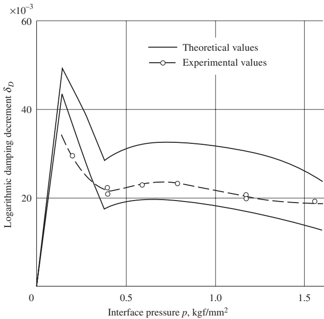
Figure 7-36 Comparison between theoretical and experimental damping capacities.
