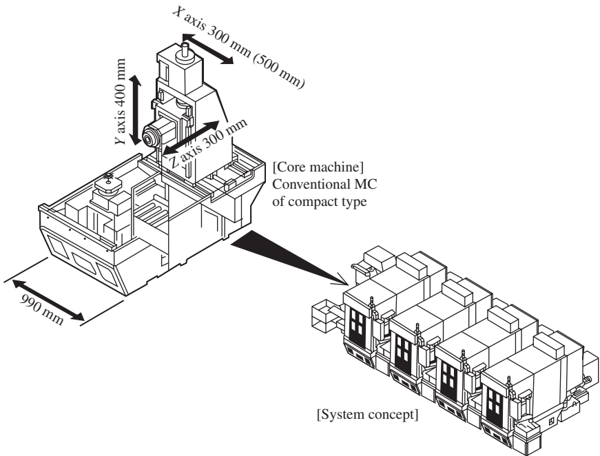
Figure 1-27 Advanced FTL for processing car parts (late 1990s, courtesy of Mori Seiki).
