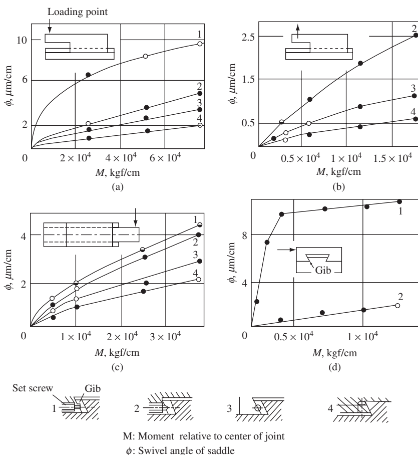
Figure 8-18 Joint stiffness of dovetail slideways with various gib configurations (by Levina and Ostrovskii).
