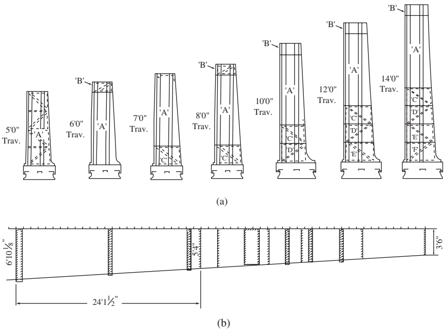
Figure 1-31 Modular design for column in horizontal boring and milling machine using monolithic pattern: (a) Modules of columns and (b) monolithic basic pattern (1960s, by William Asquith Co.).
