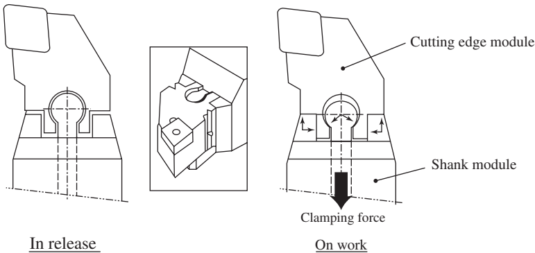
Figure 1-1 Modular tooling system in 1980s—basic ideas (courtesy of Sandvik Co.).
