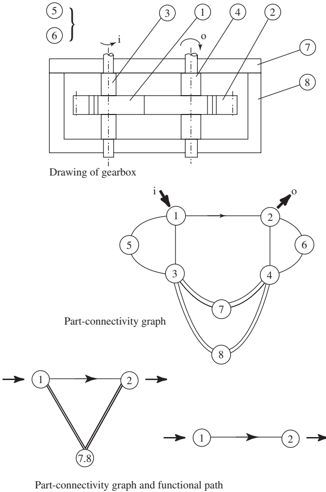
Figure 3-8 Bond graph representation of gearbox (courtesy of Yoshikawa).
