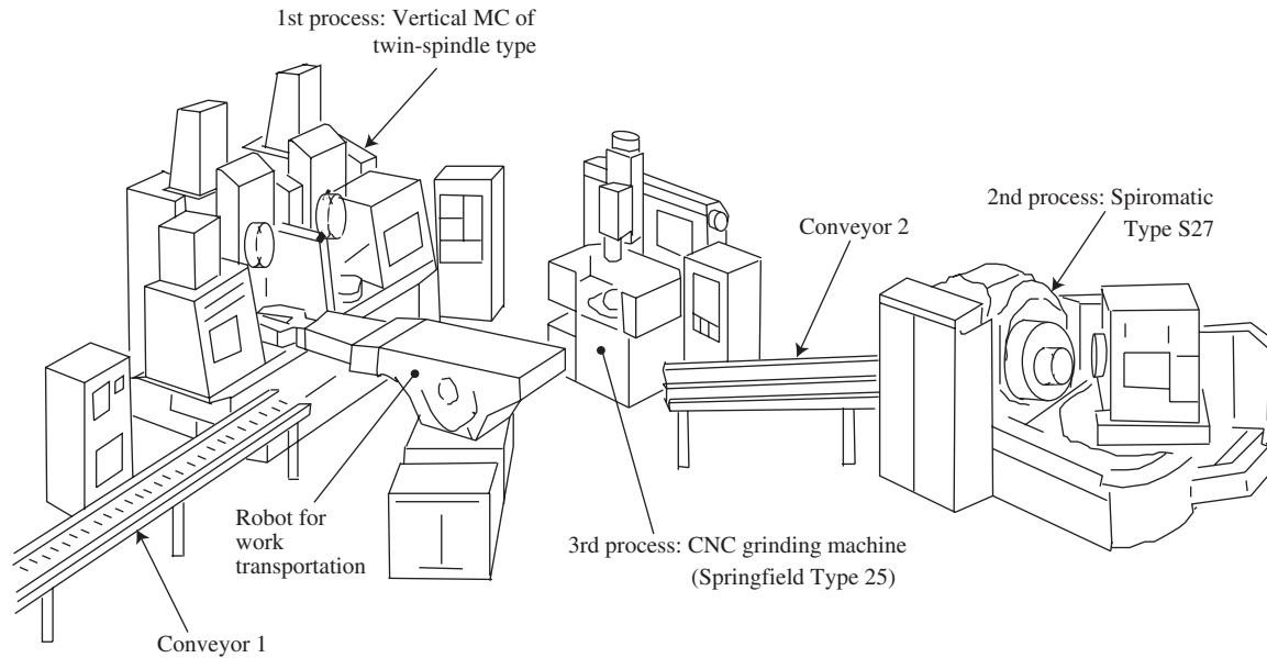
Figure 1-40 FMS for producing spiral bevel gear in 1982 (courtesy of Oerlikon Contraves AG).
