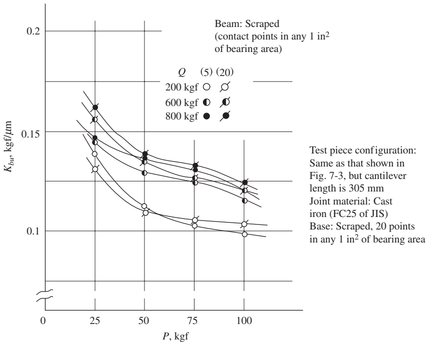
Figure 7-40 Effects of scraping quality on joint stiffness.
