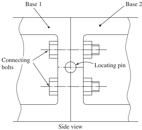
Figure 7-9 Bolted joint for producing long-length base—case of large-size NC horizontal boring and milling machine of Skoda make, 2004.
