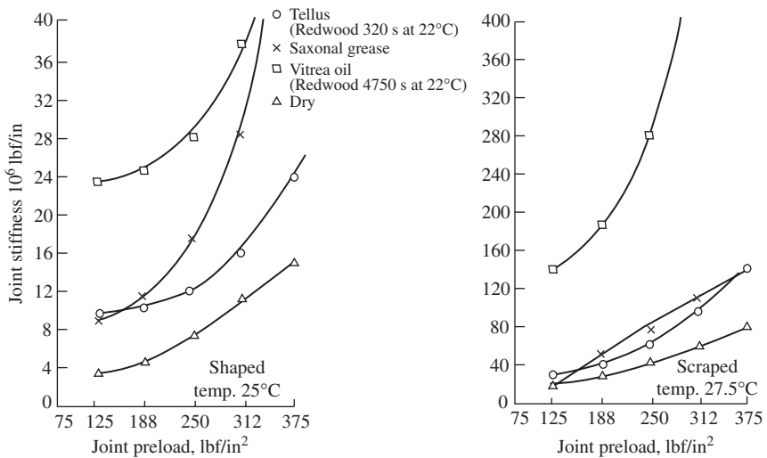
Figure 6-31 Effects of lubricants on joint stiffness (courtesy of Thornley).
