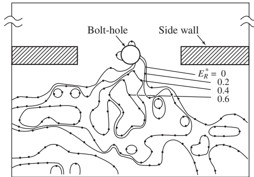
Figure 7-24 Directional orientation effect of bolt pocket—interface pressure distribution of bolted joint under normal loading.
