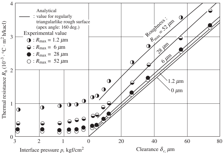
Figure 6-37 Thermal resistance of joints with positive and negative gaps (courtesy of Saito and Nishiwaki).
