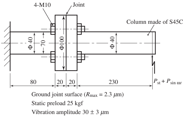
Figure 7-50 Effects of interface layers on damping capacity.
