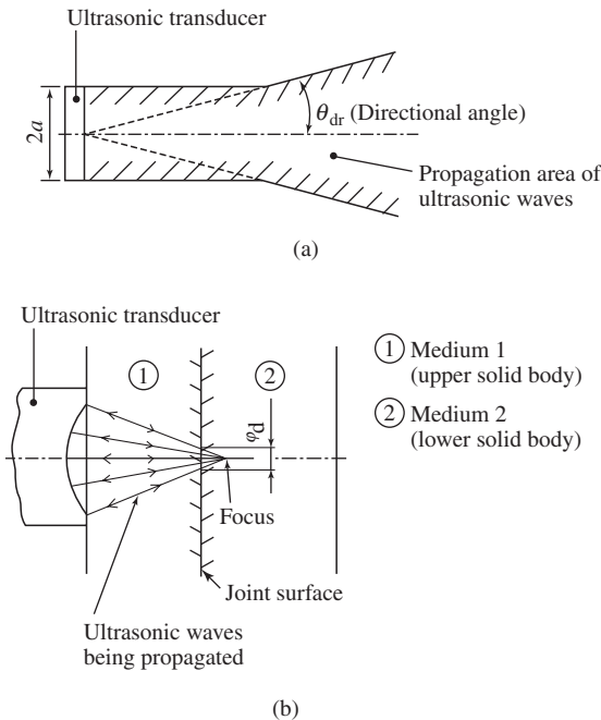
Figure A1-7 Types of ultrasonic transducers and propagation states of ultrasonic waves: (a) Conventional type and (b) focus type.
