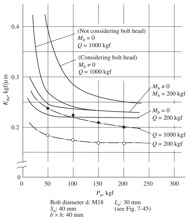
Figure 7-46 Effect of bolt head to increase bending stiffness.
