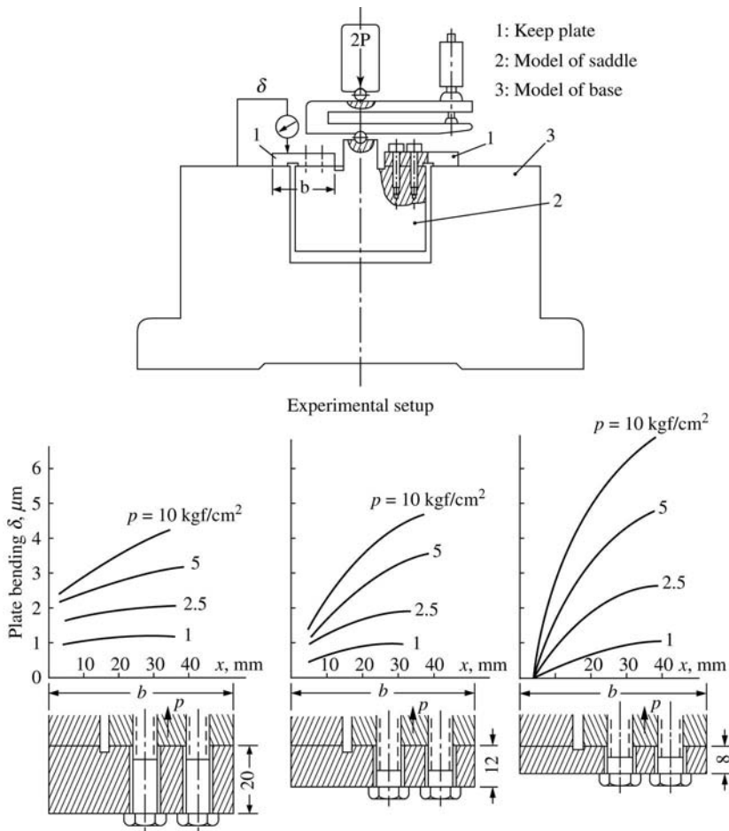
Figure 8-15 Elastic deflections of keep plates (by Levina and Ostrovskii).
