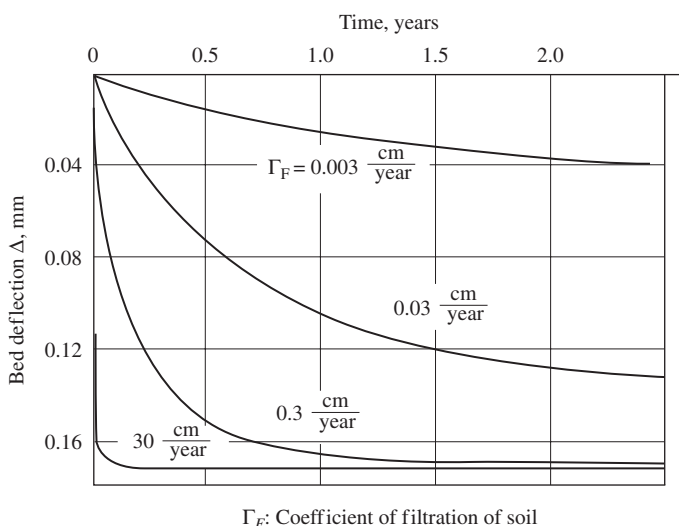
Figure 7-53 Time dependence of machine bed deflection (by Kaminskaya).
