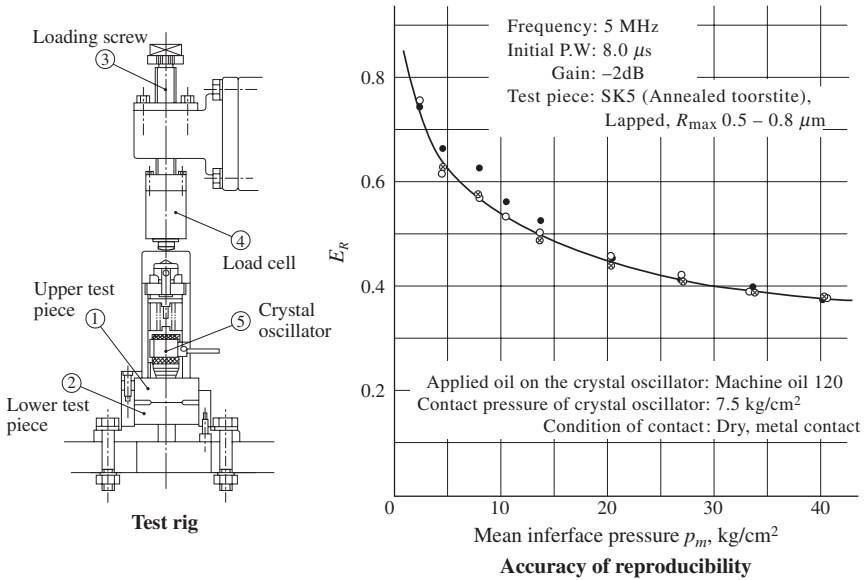
Figure A1-6 Relationships between E_R and mean interface pressure.
