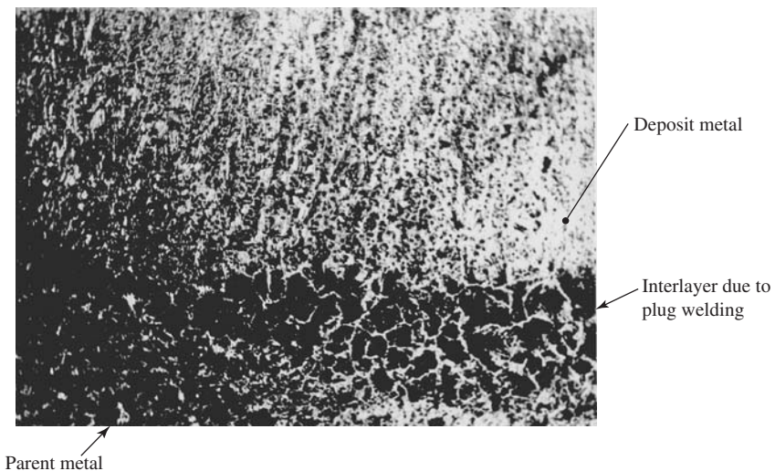
Figure 9-8 Cause of microslip at plug welding.
