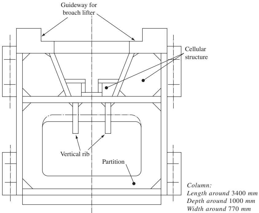
Figure 9-4 Steel welded column of vertical broaching machine (type NUV, from 1960s to 1990s, courtesy of Fujikoshi).
