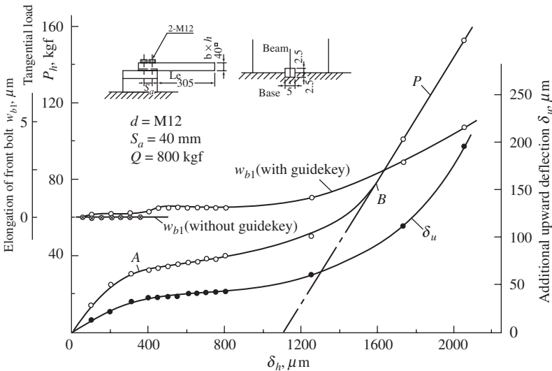
Figure 7-43 Tangential deflection of bolted joint with guidekey.
