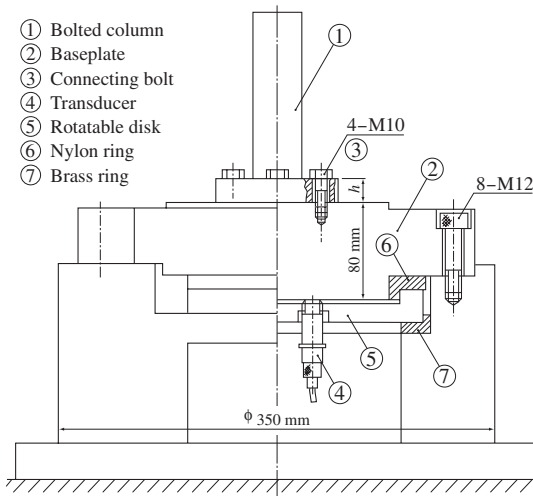
Figure A1-12 Experimental setup to measure three-dimensional contact pattern.
