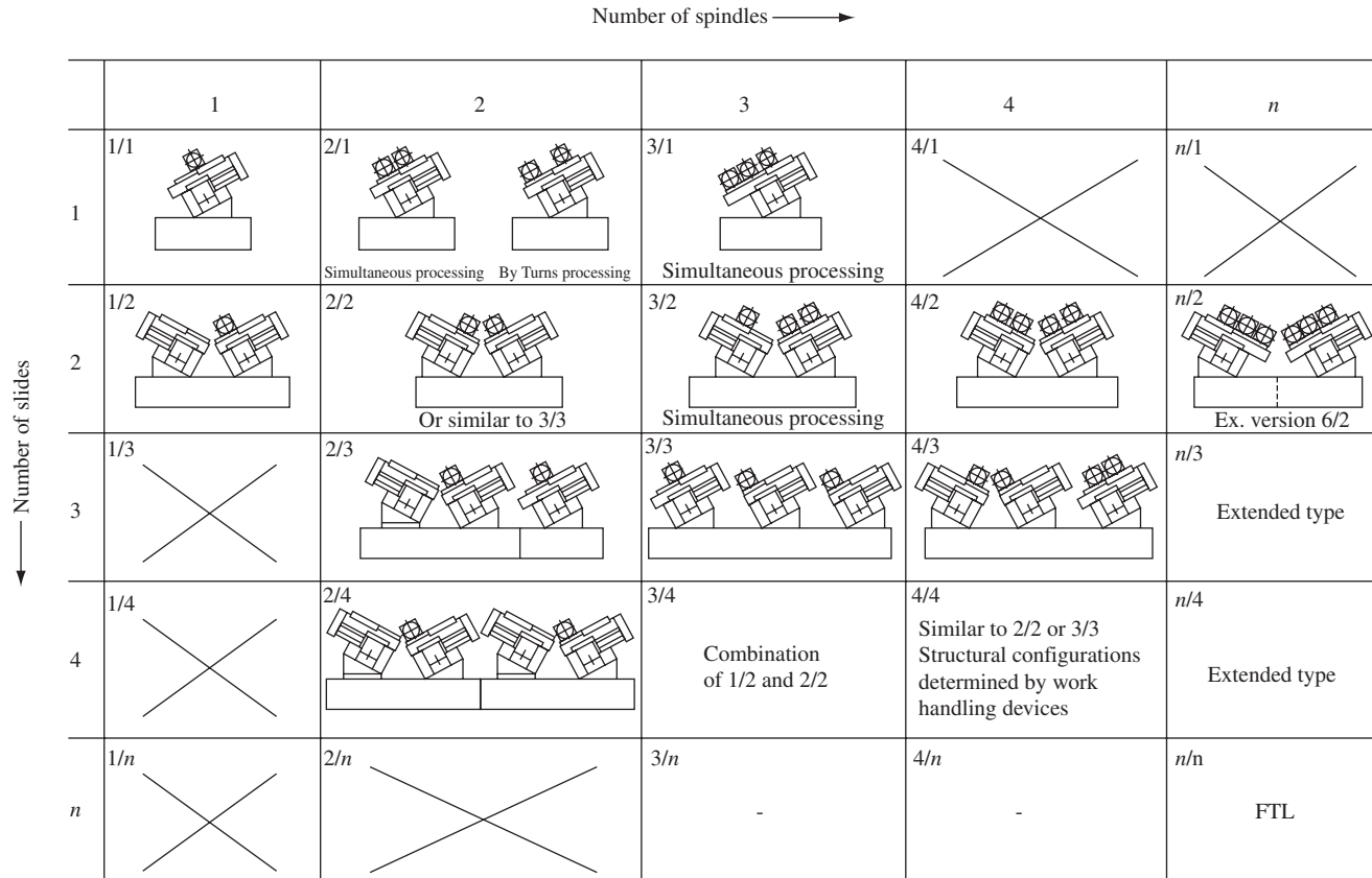
Figure 2-9 Structural master plan to produce chucking machine of Fronter type (by Dietz, courtesy of Industrie-Anzeiger).
