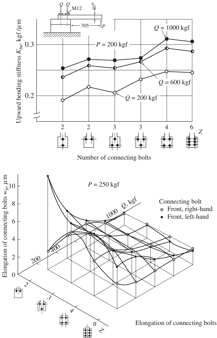
Figure 7-27 Effects of arrangement and number of connecting bolts.
