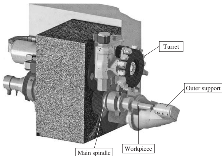
Figure 2-17 A new modular concept with greater accessibility—two-pillar central unit (patented by Accim).
