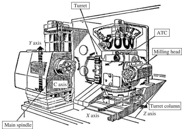
Figure 2-16 ATC of extended type in the late 1970s (courtesy of Okuma Co.).
