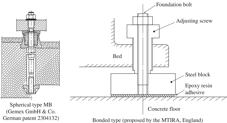
Figure 7-56 Some variants of leveling block.
