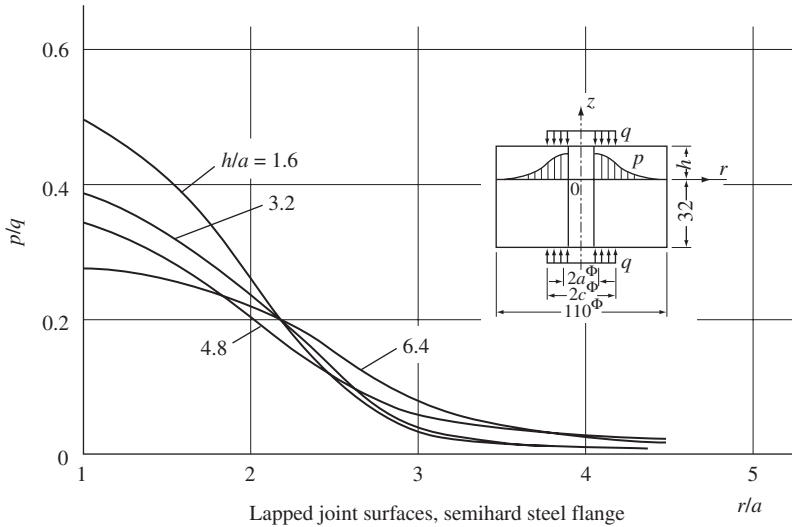
Figure 7-47 Effects of flange thickness on interface pressure distribution.
