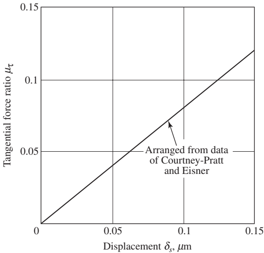
Figure 6-20 Displacement dependence of tangential force ratio in steel joint.
