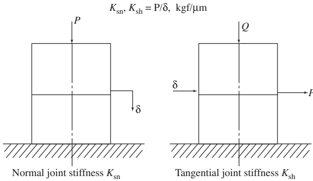
Figure 5-17 Stiffness expressions for flat joints under normal and tangential loading.
