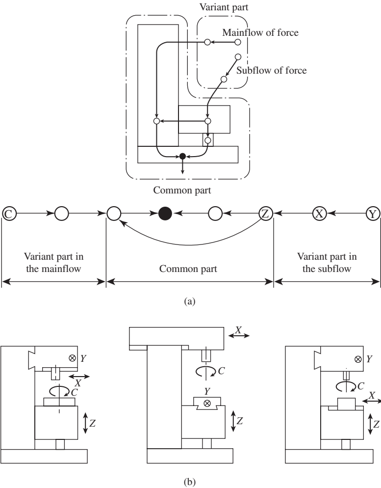
Figure 4-24 Variant design method and its application to milling machine of knee type: (a) Idea of variant design and (b) some examples of variants produced.
