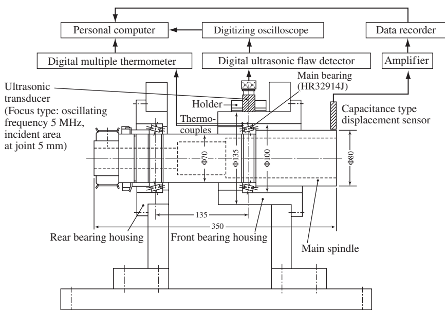
Figure A1-21 Schematic view of spindle model.
