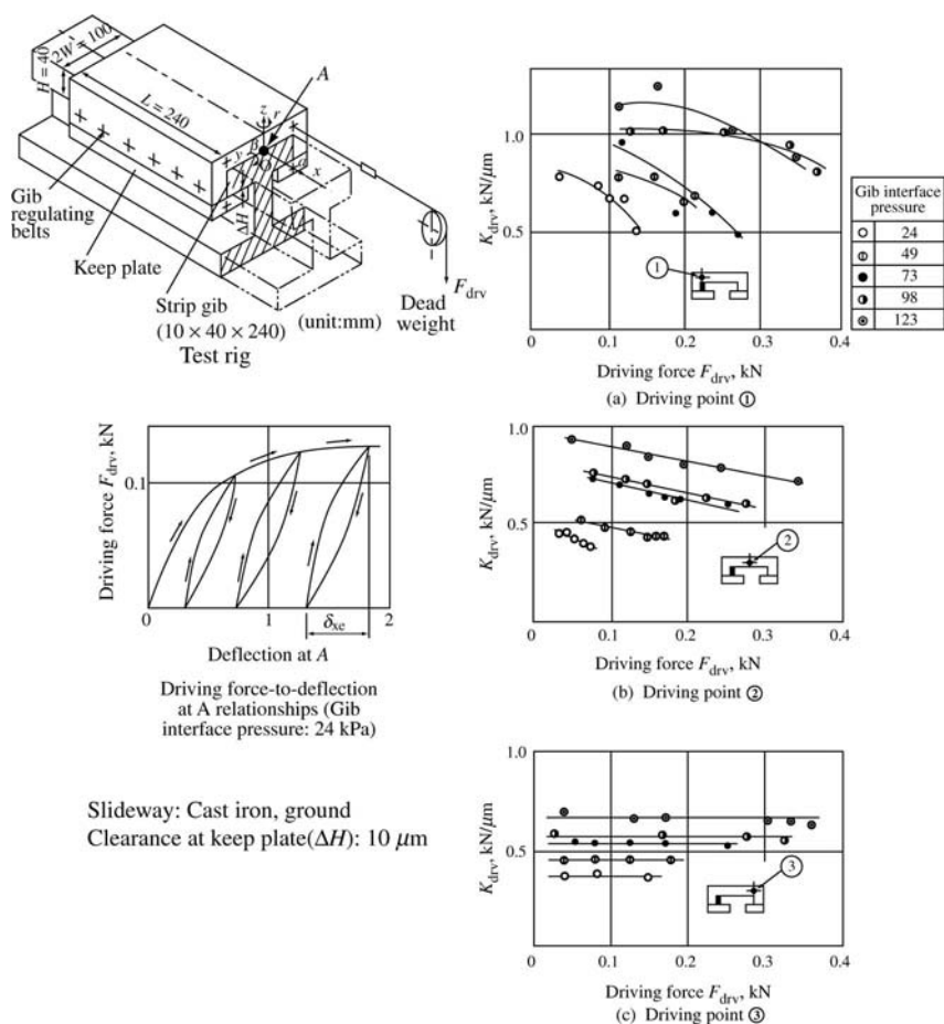
Figure 8-9 Effects of driving point on stiffness of slideway K_{drv} .
