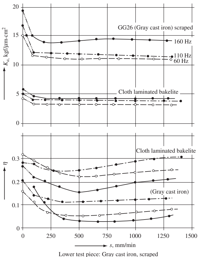
Figure 6-28 Effects of sliding velocity on joint stiffness and damping when excitation frequency is varied (by Corbach).
