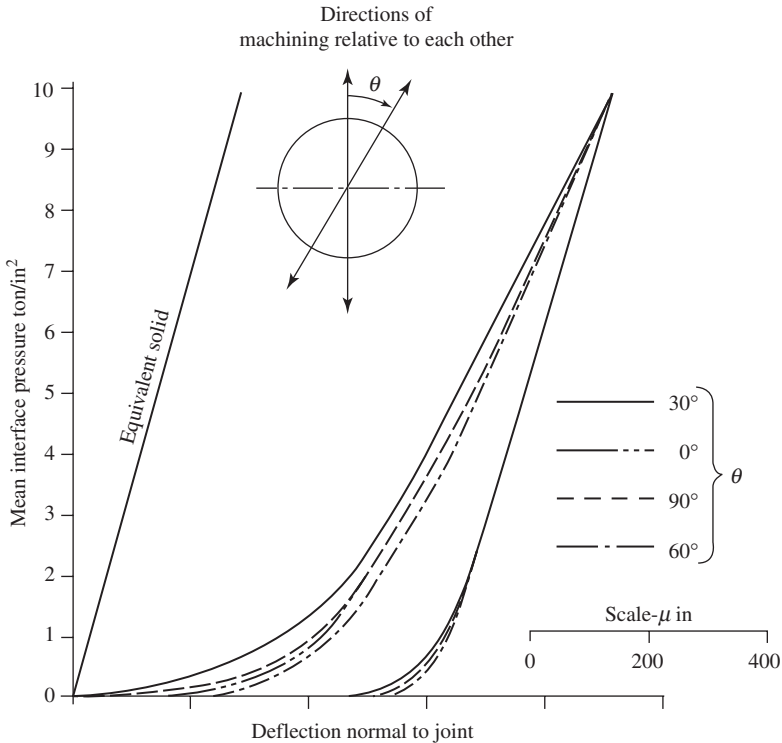
Figure 6-9 Effects of machined lay orientation on joint deflection—shaped mild steel joint (by Thornley and coworkers).
