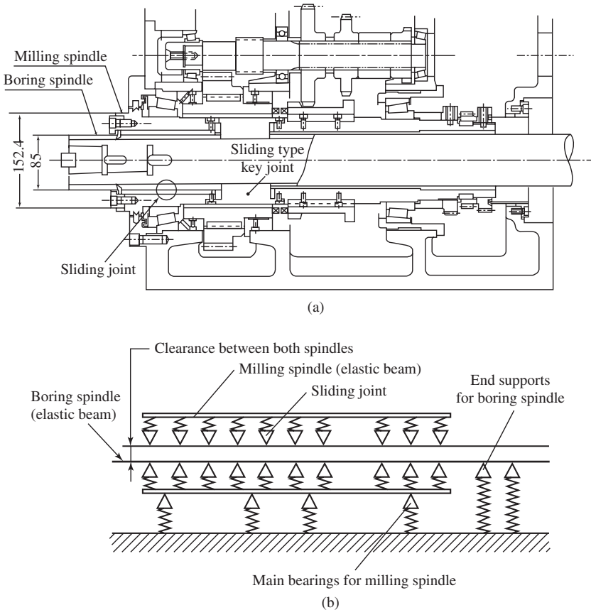
Figure 8-41 Multiple-layered main spindle of traveling type and its mathematical model: (a) Main spindle of boring and milling machine and (b) mathematical model for two-layered spindle (by Bykhovskii).
