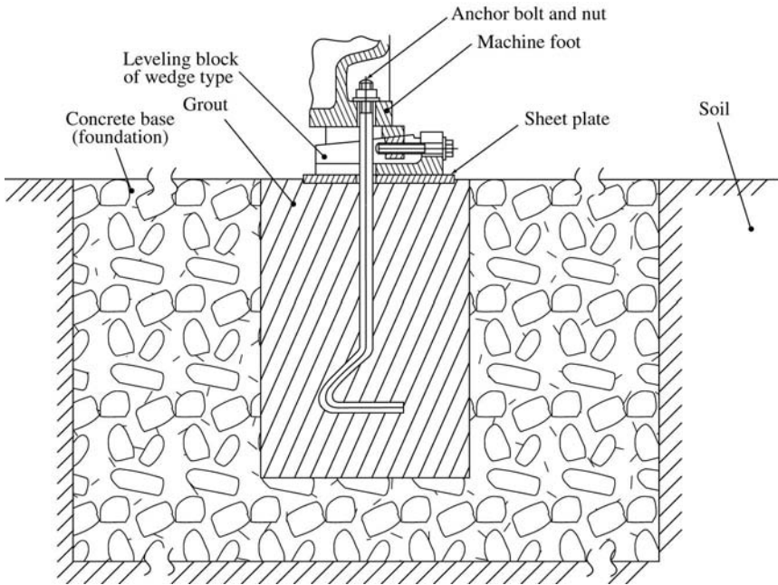
Figure 5-8 Schematic representation of foundation system.
