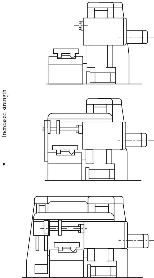
Figure 2-6 Application of one-dimensional decision table (planomiller of TOS make, Czechoslovakia)
