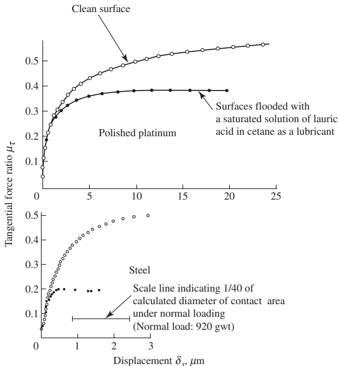
Figure 6-21 Original data for displacement dependence of tangential force ratio (by Courtney-Pratt and Eisner).
