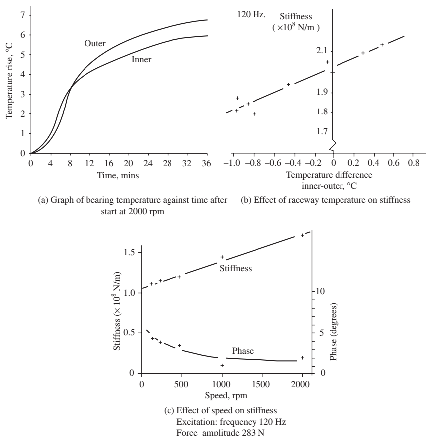
Figure 8-36 Changes for dynamic stiffness of ball bearing with rotational speed and running temperature (by Walford and Stone, courtesy of I MechE).
