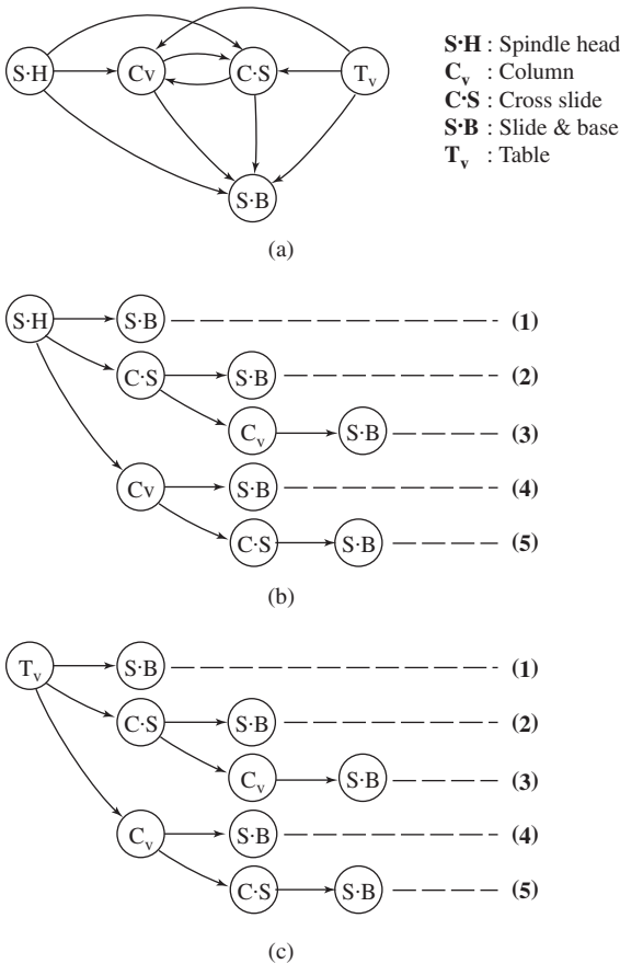
Figure 4-31 Conjunction pattern of module complexes: (a) General conjunction pattern; (b) conjunction pattern for unit complexes in tool branch; and (c) conjunction pattern for unit complexes in workpiece branch.
