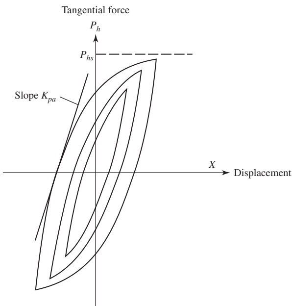
Figure 6-18 Hysteresis loops with increasing tangential loads under constant normal preload (courtesy of Boothroyd).
