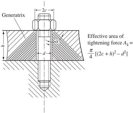
Figure 7-11 Concept of pressure cone proposed by Rötischer.
