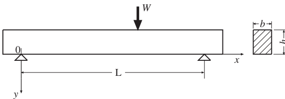
Figure A2-1 Beam simply supported at both its ends.
