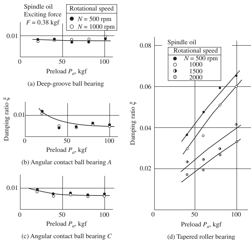
Figure 8-39 Relationships between preload P_A and damping ratio \xi (courtesy of Tsutsumi).
