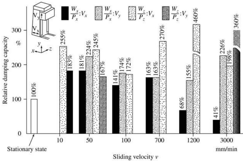
Figure 8-7 Relative damping capacity under bending vibration mode—milling machine of open and column traveling type (courtesy of Groth).
