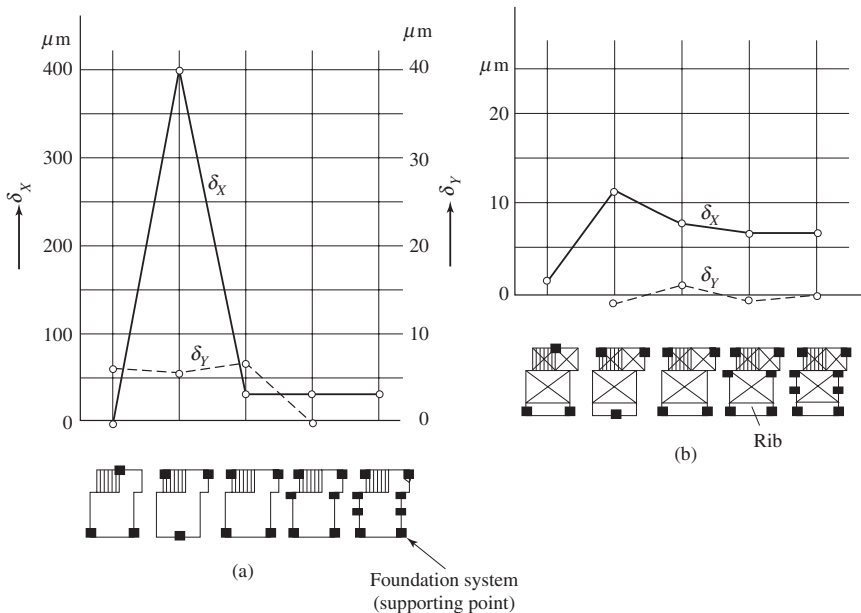
Figure 7-54 Effects of foundation system and bed construction on relative displacements between main spindle and workpiece: (a) Open-type bed and (b) closed-type bed (by Poláček).
