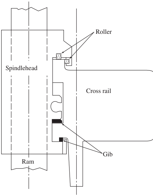
Figure 8-4 Guideway of hybrid type in five-face processing machine (type MCR-B II-HP, 1996, courtesy of Okuma).
