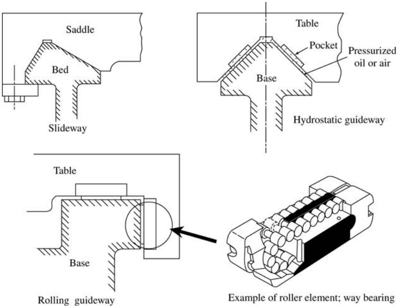
Figure 5-9 Three typical types of guideway.
