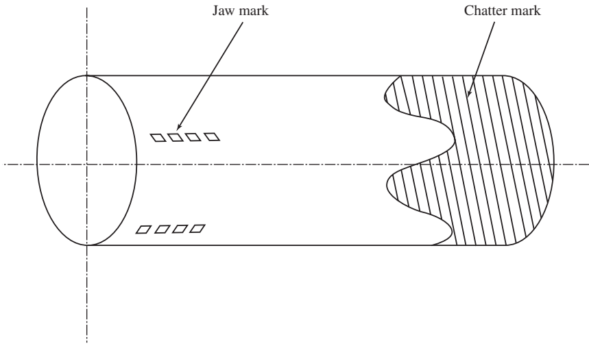
Figure 9-26 Effect of directional orientation on chatter mark.
