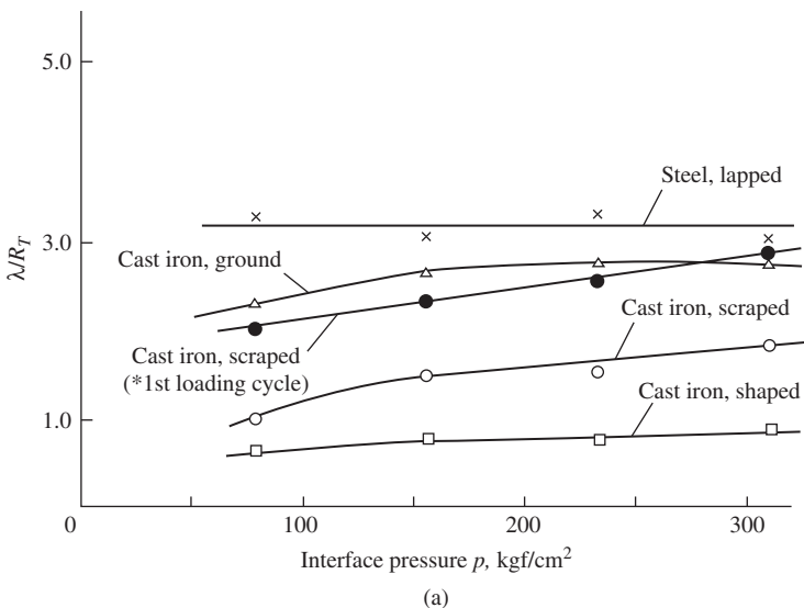
Figure 5-13 Changes of ratio \lambda/R_T with increasing interface pressure: (a) Under higher interface pressure and (b) under lower interface pressure.
