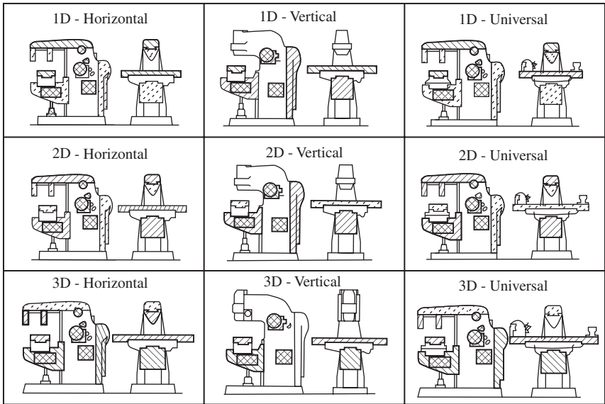
Figure 1-12 Unit construction of milling machines (Wanderer Co., about 1930).
