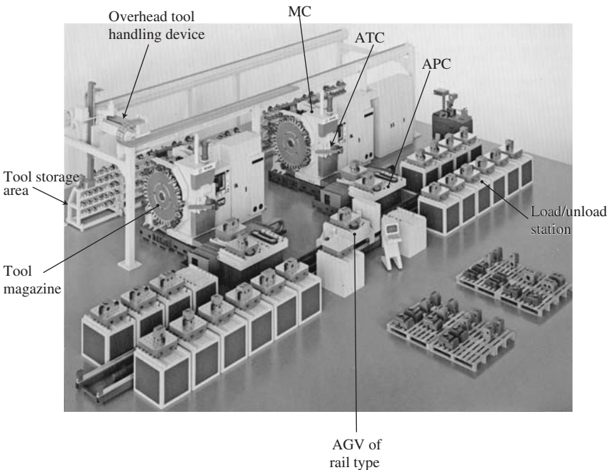
Figure 1-17 FMC of pallet pool type (type DFZ630, courtesy of Hammer of Fritz Werner).
