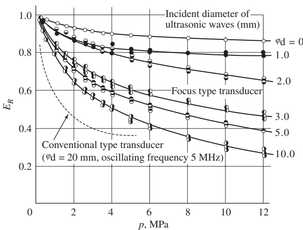
Figure A1-8 Effects of incident diameter d of ultrasonic waves on relationships between mean interface pressure p and value of E_R .
