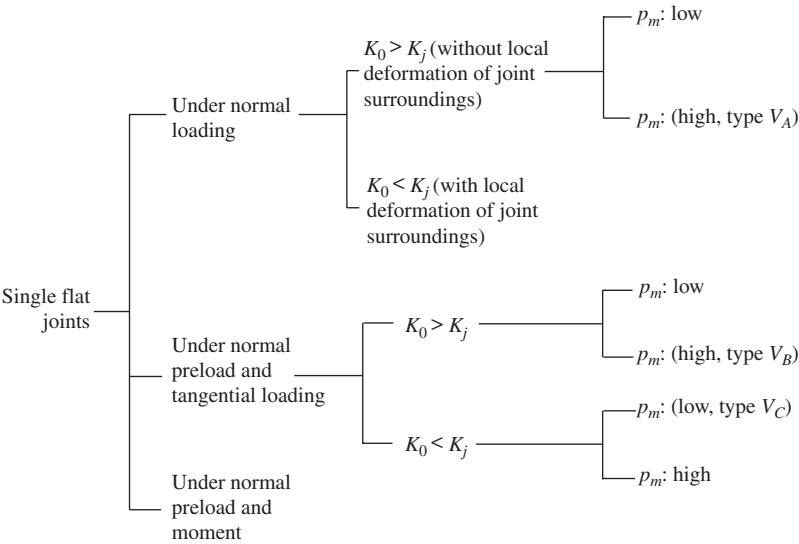
Figure 6-1 Classification of single flat joint.
