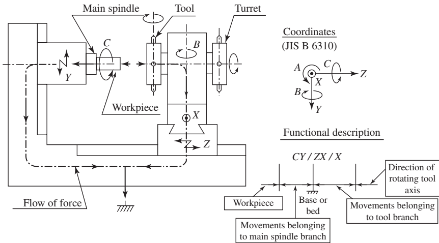
Figure 3-5 Functional description of turning center.
