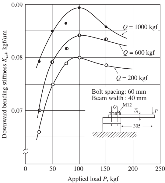
Figure 7-4 Load and tightening force dependence of joint stiffness—nonseparation in joint.
