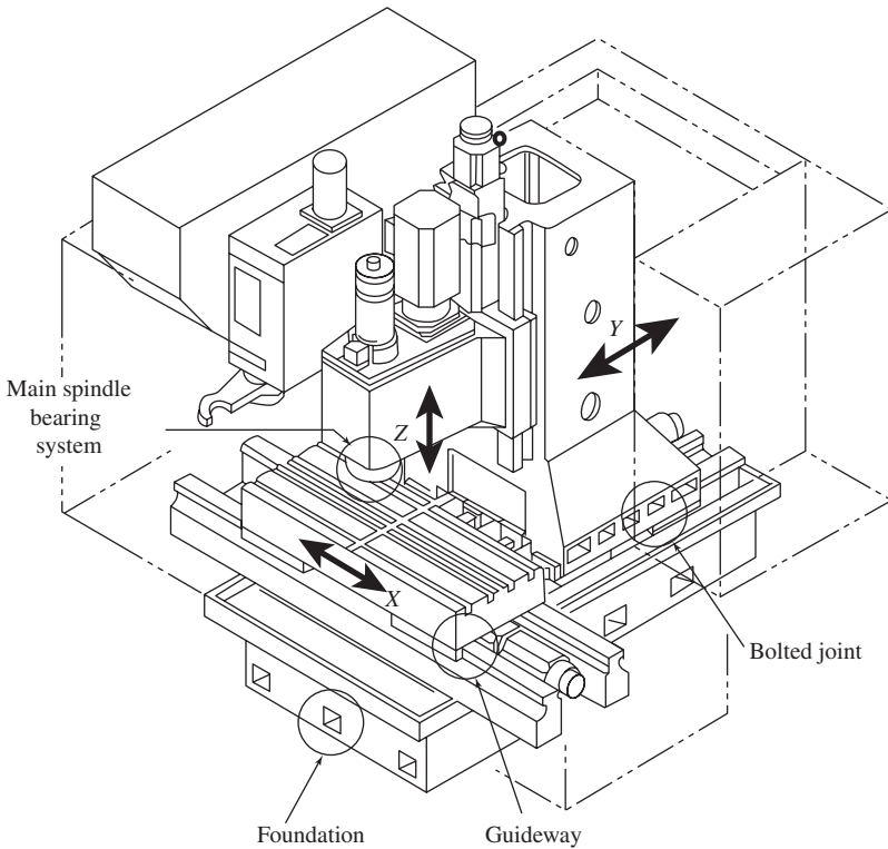
Figure 5-1 Representative joints in a machine tool (courtesy of Okuma).
