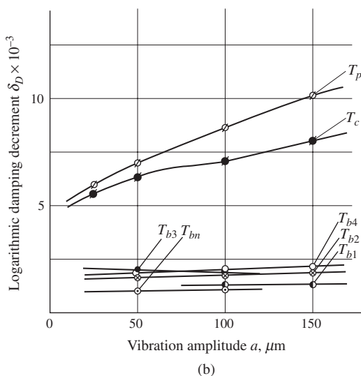
Figure 9-6 Damping capacity for various welded joints: (a) Shapes and dimensions of various welded joints and (b) effects of vibration amplitudes on damping capacity.
