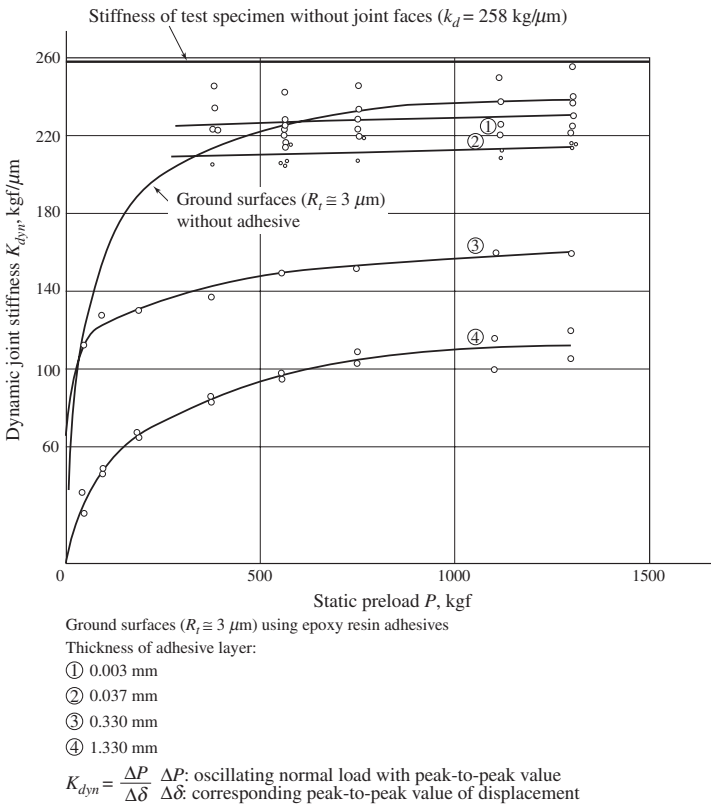
Figure 9-13 Dynamic stiffness of bonded joints under normal loading (by Dekoninck).
