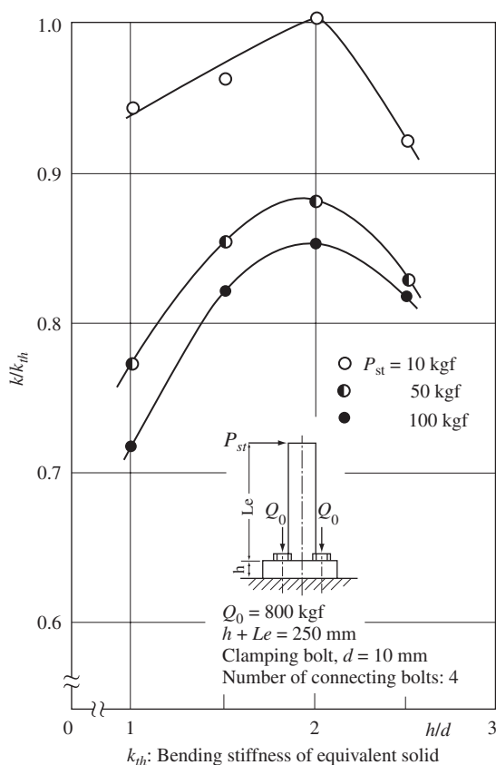
Figure 7-20 Optimum ratio h/d in bolted joint of B type.
