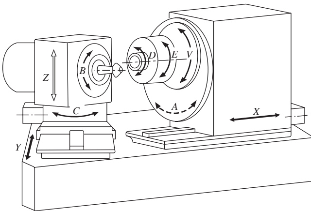
Figure 4-5 A variant of extended functional description—form-generating function in hypoid gear generator.
