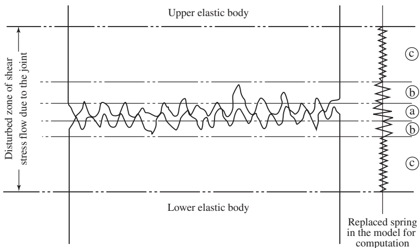
Figure 5-14 The concept of region of joint.
