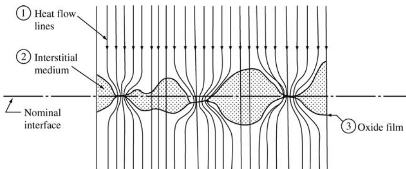
Figure 6-32 Causal sources of thermal contact resistance.
