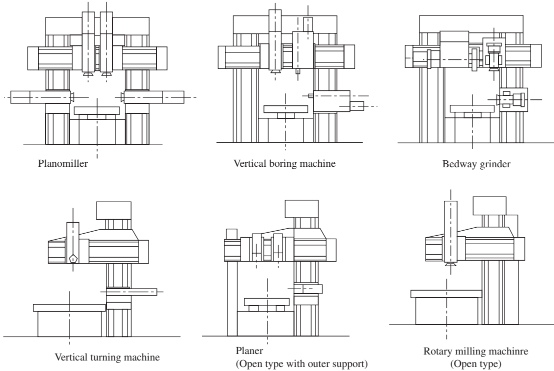
Figure 1-37 Some examples of structural configuration with different-kind generating modular design in 1962–standard combination of common modules (courtesy of Ikegai Iron Works).
