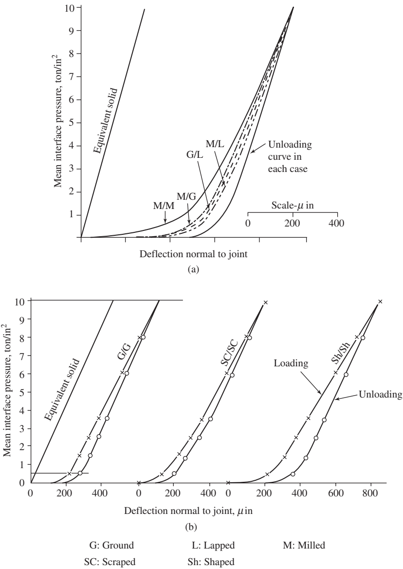
Figure 6-10 Effects of surface finishes on joint deflection: (a) Mild steel joint and (b) cast iron joint (by Thornley and coworkers).
