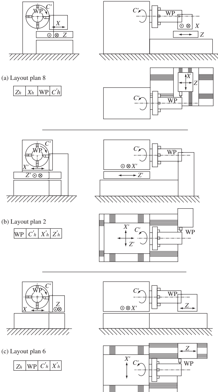
Figure 3-4 Some layout drawings and related functional descriptions for a turning machine (courtesy of Saljé).
