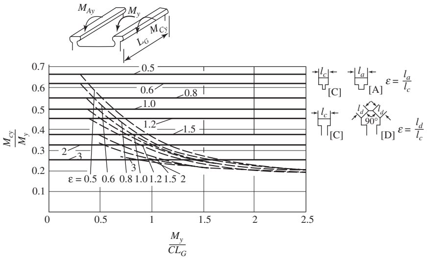
Figure 8-S4 Calculation diagram for M_{Ay} and M_{Cy} .
