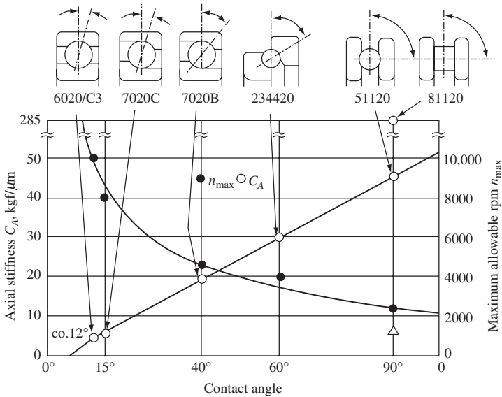
Figure 8-35 Stiffness and maximum allowable speed of ball and roller bearings (by Kunkel).
