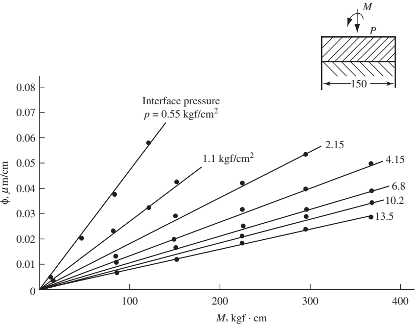
Figure 6-4 Moment–angular deflection relationships of flat joint under complex loading (by Levina).
