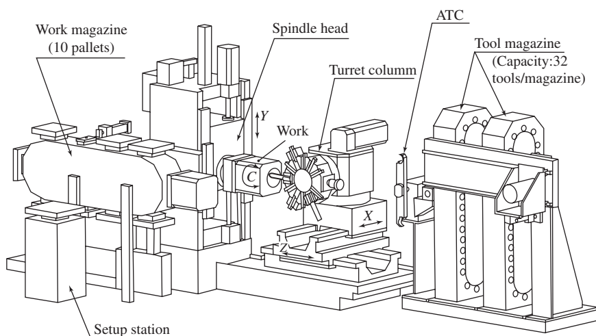
Figure 2-26 Concept of TC—MC Complex (type MMC-30, courtesy of Nihon Kokan).
