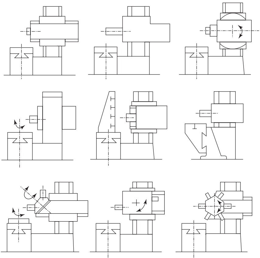
Figure 3-2 Examples of design arrangement of XOYZ (by Vragov).
