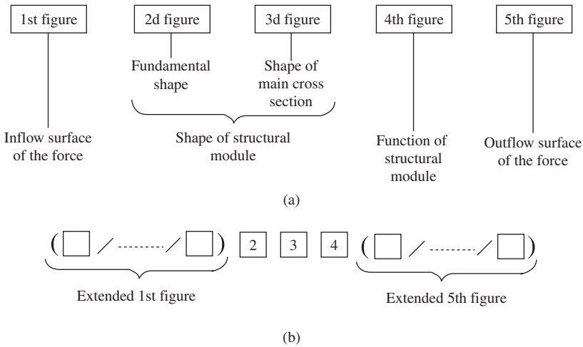
Figure 3-10 Description of structural modules by GT code: (a) Basic coding system for the description of structural module and (b) extended coding system for the description of structural module.
