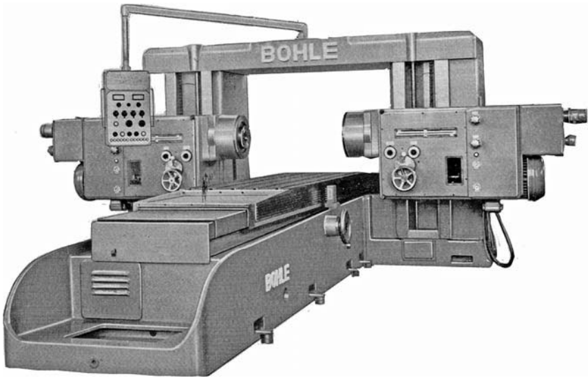
Figure 1-14 Unit construction in milling machine of bed type (type LFD160/3090 of Bohle make).
