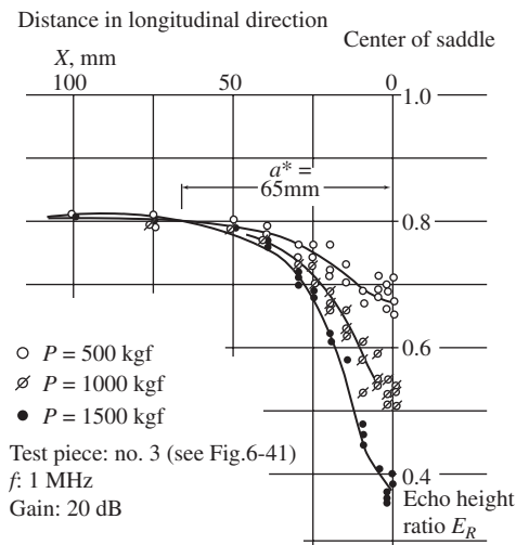
Figure 6-39 Contact pattern of saddle on slideway.
