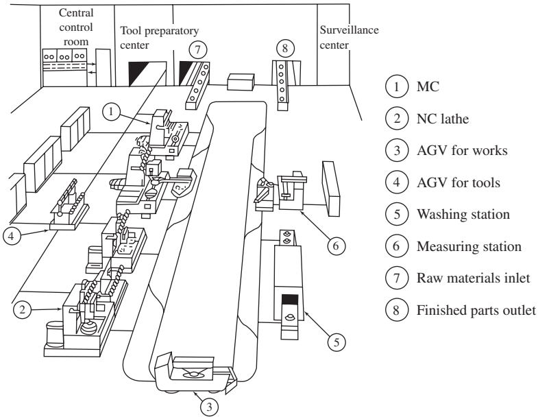
Figure 1-39 FMS consisting of machine tools with modular design of different-kind generating type (Produktionssystem 2000, courtesy of Mauser-Schaerer).
