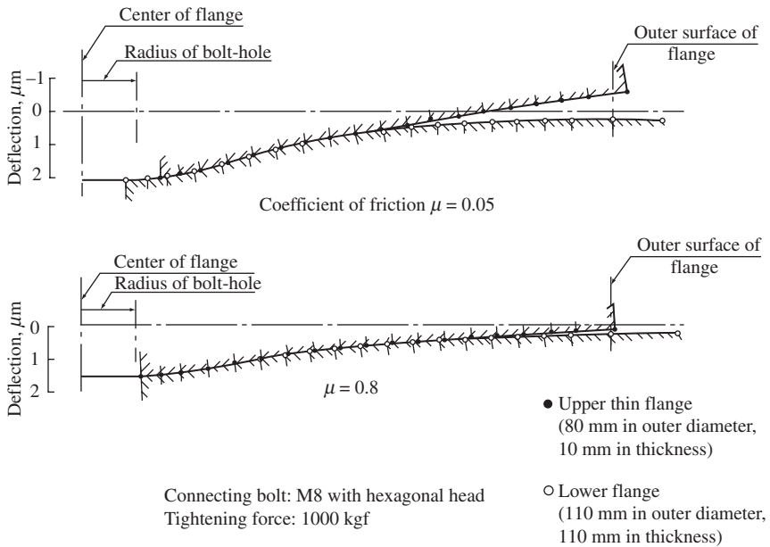
Figure 6-42 Constraint effect of friction on joint deflection (courtesy of Shimizu).
