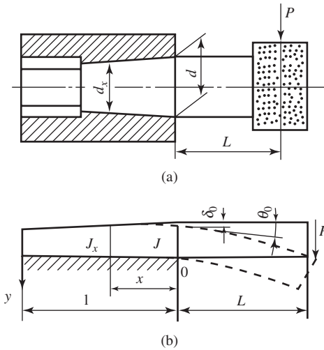
Figure 9-15 A quill-grinding spindle system and its mathematical model: (a) Actual structure and (b) mathematical model (by Levina).
