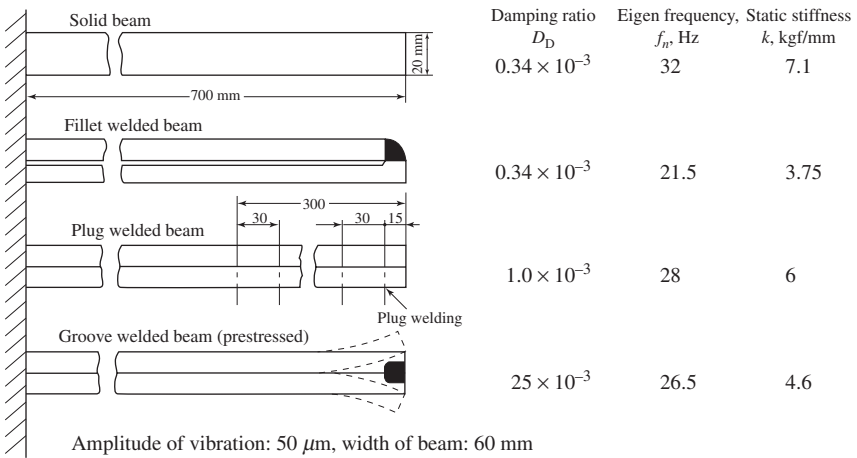
Figure 9-9 Larger damping in laminated and welded beam when using shear effect (by Bobek et al.).
