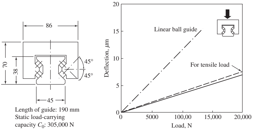
Figure 8-23 Normal stiffness of linear roller guide (courtesy of NSK).
