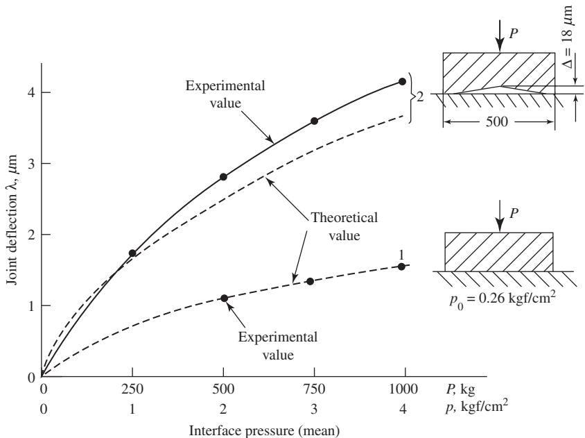
Figure 6-3 Applicability of Ostrovskii's expression to engineering calculation (by Levina).
