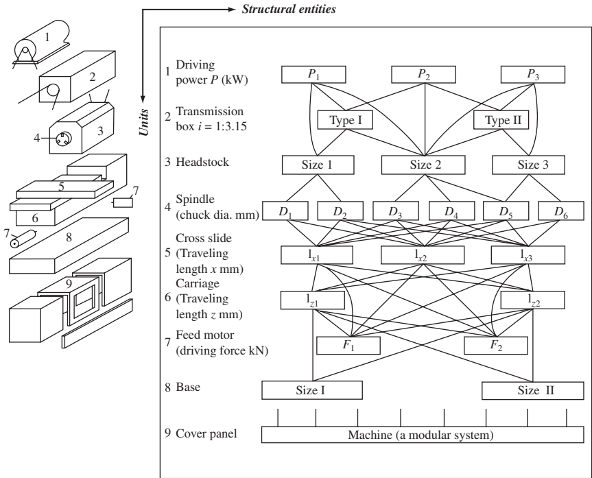
Figure 2-8 Connecting diagram proposed by Dietz in case of chucking machine (courtesy of Carl Hanser).
