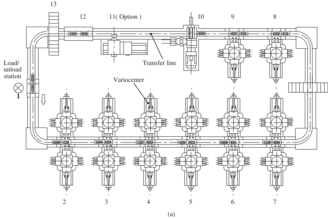
Figure 1-6 FTL for producing automobile parts (1980s, courtesy of Dienesheim): (a) Line flow type and (b) FMC-integrated type.
