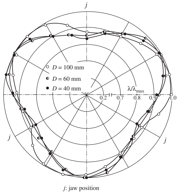
Figure 9-25 Directional orientation in chucking stiffness.
