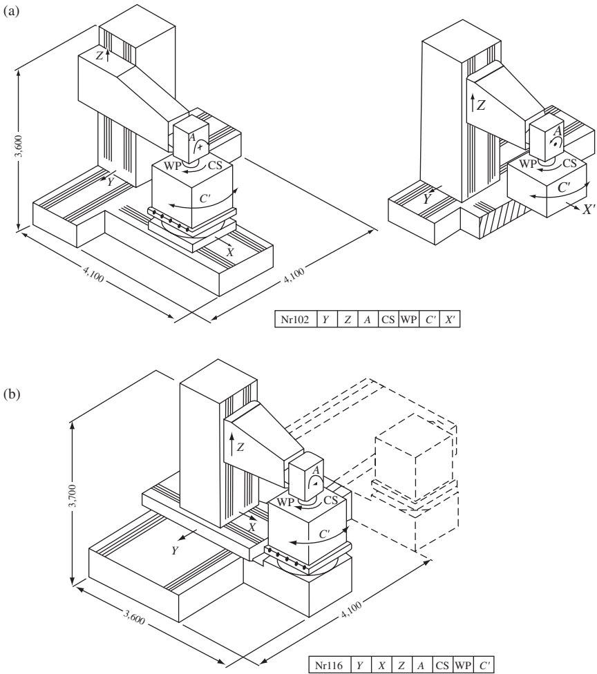
Figure 4-14 Design results of quinaxial controlled milling machines (courtesy of Saljé).
