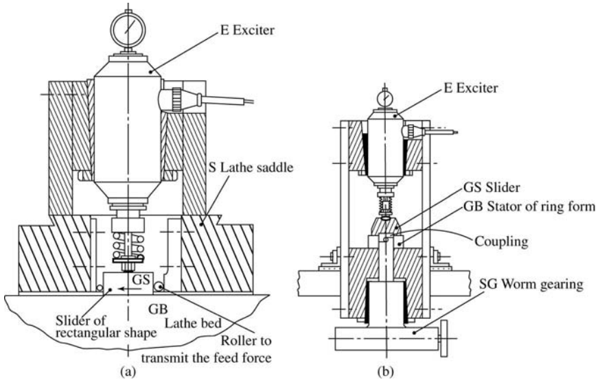
Figure 6-27 Test rigs used by Eisele and Corbach: (a) Linear type and (b) rotary type.
