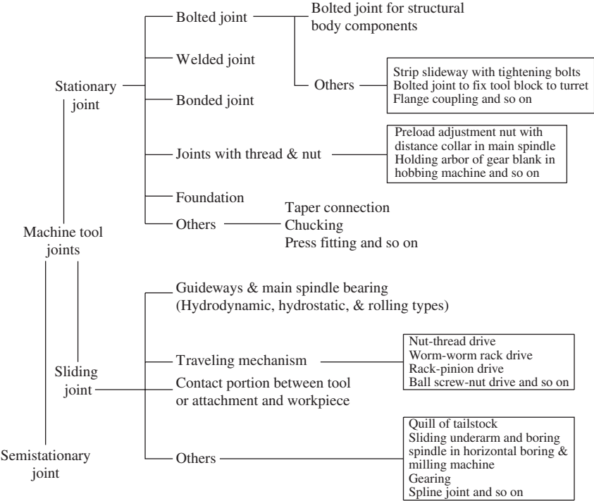
Figure 5-5 Classification of machine tool joints.
