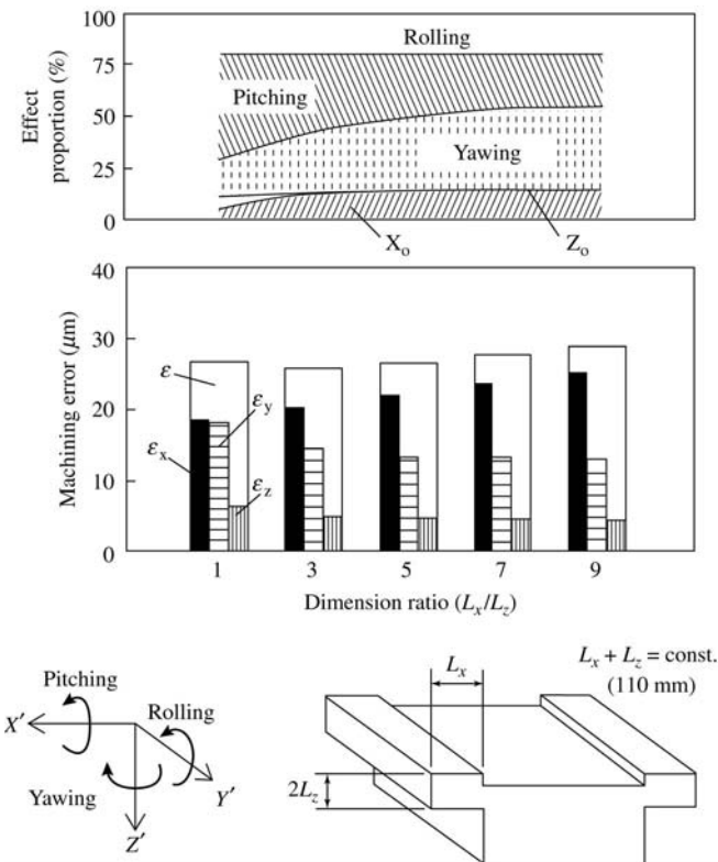
Figure 8-8 Changes of machining error with dimensional ratio, and influencing rate of pitching, yawing, and rolling (courtesy of Furukawa).
