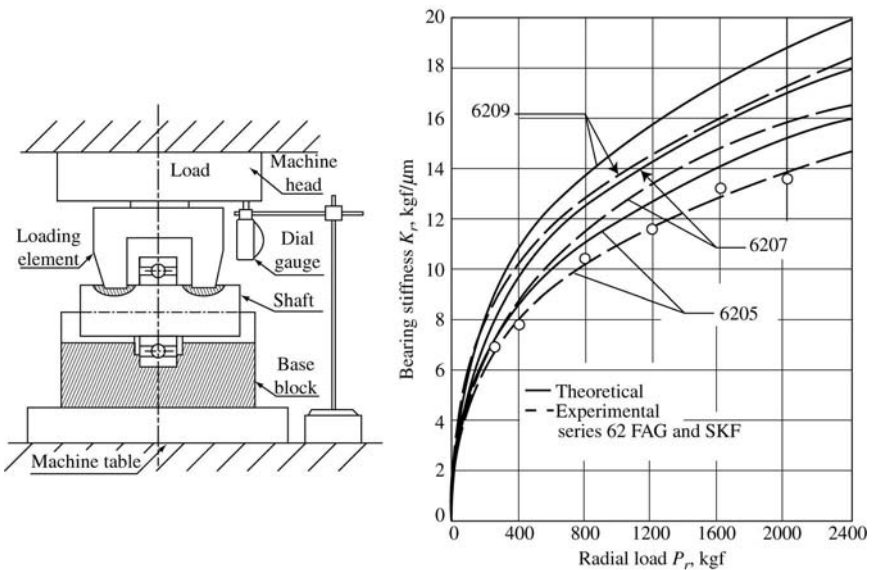
Figure 8-32 Comparison of theoretical and measured bearing stiffness (by El-Sayed).
