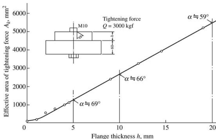
Figure 7-12 Effective area of tightening force (by Plock, courtesy of Industrie-Anzeiger).
