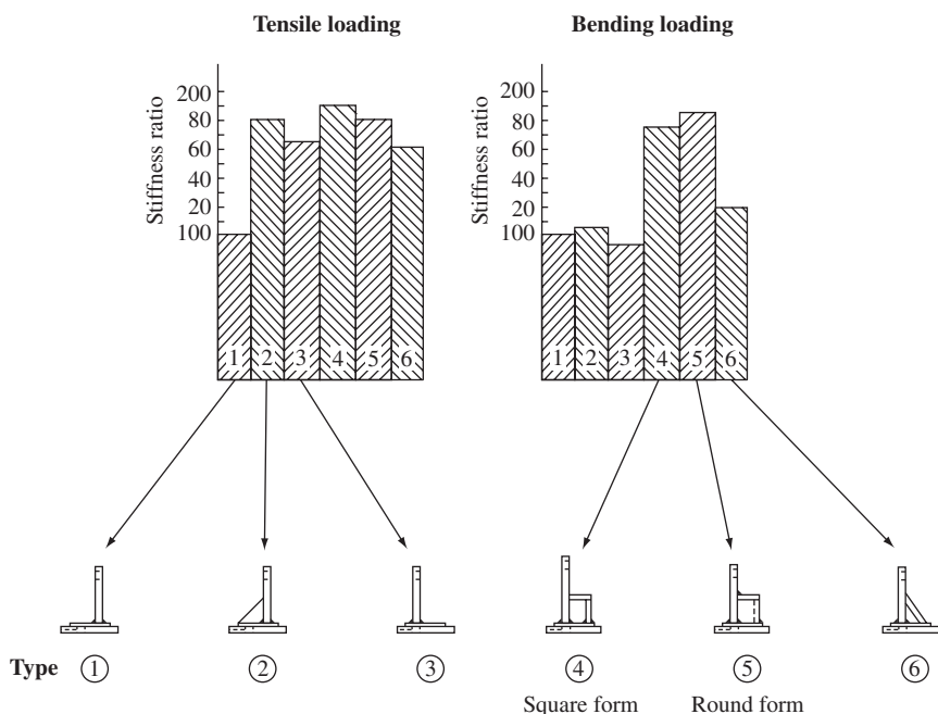
Figure 7-22 Comparison of various remedies for reinforcement (courtesy of Thornley).
