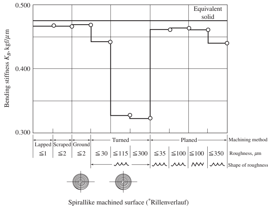
Figure 7-39 Effects of surface roughness on joint stiffness (by Schlosser).
