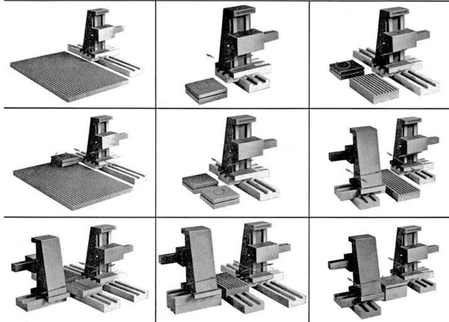
Figure 1-33 Horizontal boring and milling machine with modular design (by Scharmann Co.).
