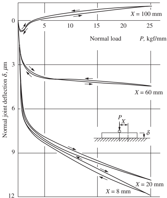
Figure 6-42 Constraint effect of friction on joint deflection (courtesy of Shimizu).
