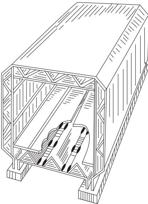
Figure 9-12 A representative welded column using panel structure, U.S. Patent No. 2789480 (Giddings Lewis make).
