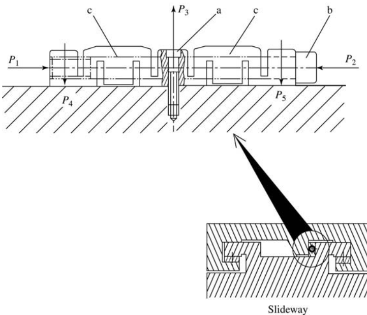
Figure 8-14 A new gib with clearance regulating functionality (by Spieth-Maschinenelemente KG, courtesy of Carl Hanser).
