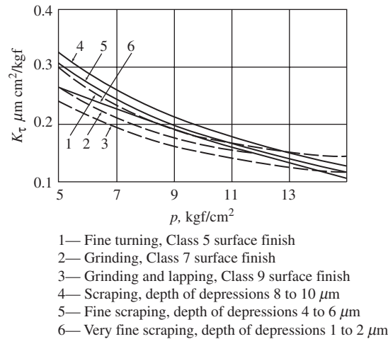
Figure 6-11 Values of K_t in connection with p (by Kirsanova).
