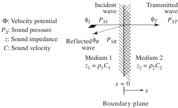
Figure A1-3 Reflection and transmission of plane waves at boundary plane.
