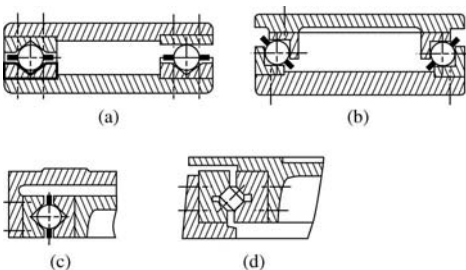
Figure 8-25 Various linear rolling guideways of noncirculating type (by Bankmann, courtesy of Carl Hanser).
