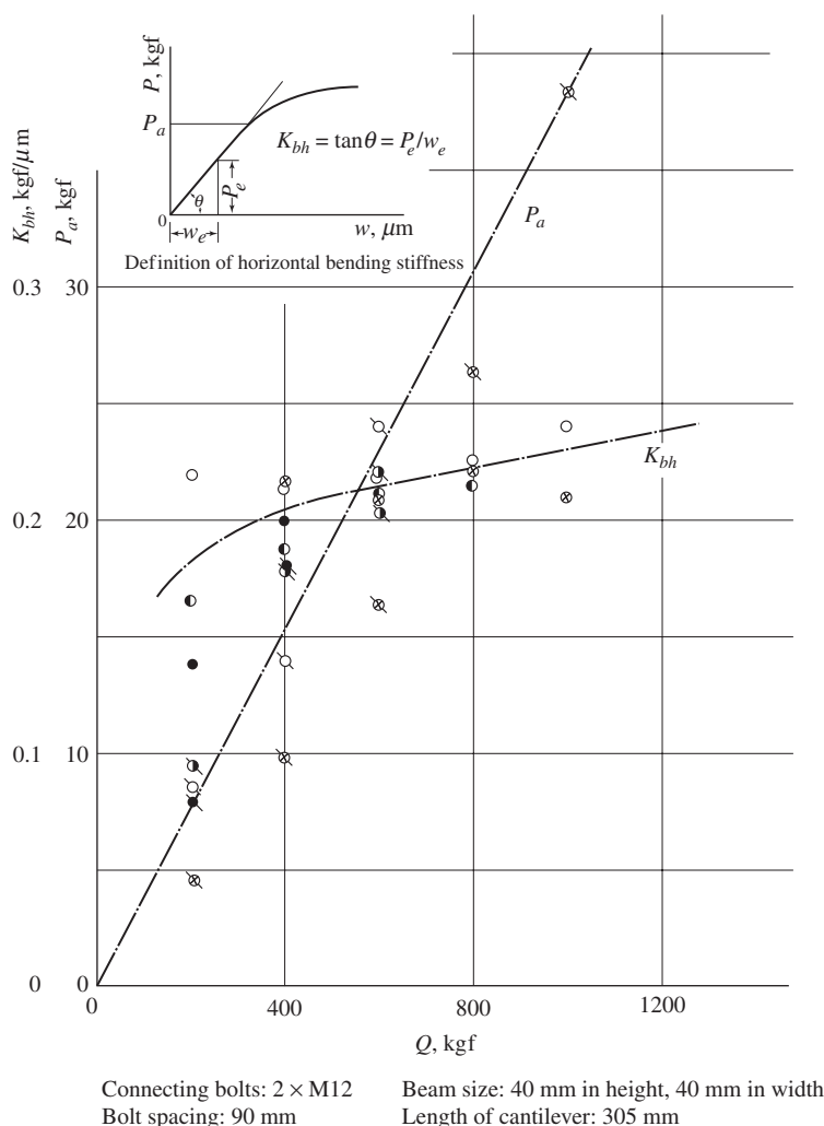
Figure 7-41 Critical bending load and tangential stiffness in bolted joint of A type.
