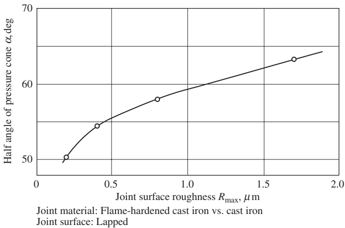
Figure 7-13 Changes of half angle of pressure cone with joint surface roughness.
