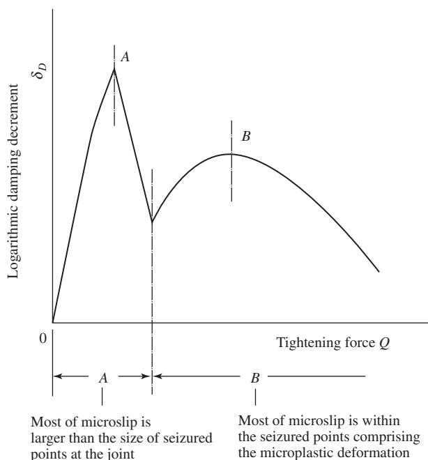
Figure 7-8 Qualitative relationships between damping capacity and tightening force.
