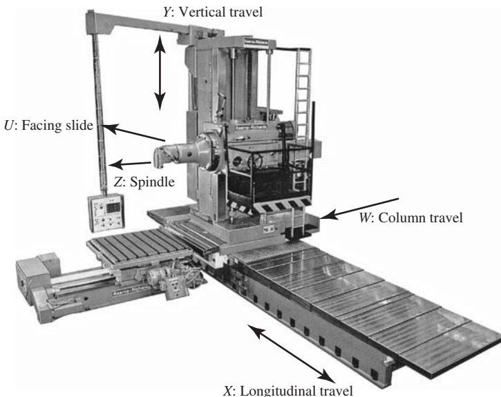
Figure 2-24 System machine originated from traditional horizontal boring and milling machine (type F, around 1990, courtesy of Kearns-Richards).
