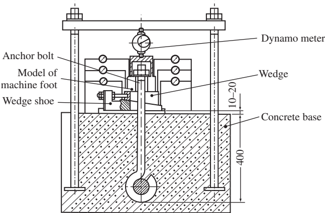
Figure 7-57 Test rig for model of leveling block (by Faingauz).
