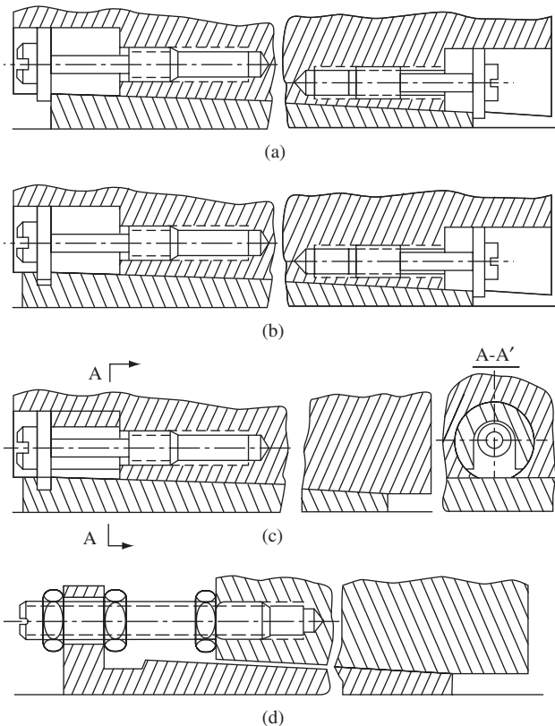
Figure 8-19 Various configurations of taper gib.
