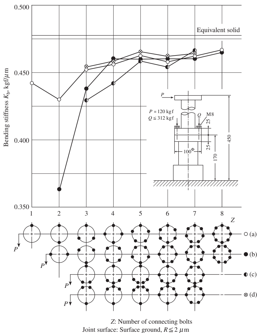
Figure 7-26 Effects of arrangement and number of connecting bolts (by Schlosser).
