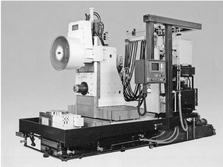
Figure 2-13 MC of line type (type HMC-40LS, 1985, courtesy of Enshu Co.)
