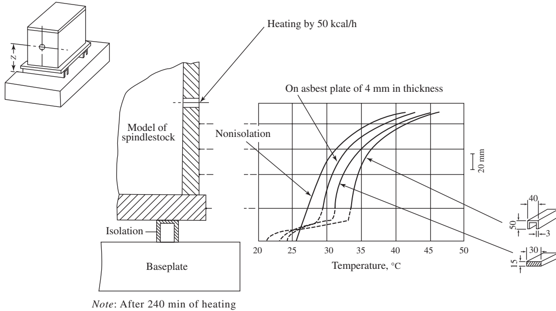
Figure 7-52 Discontinuity in temperature distribution caused by isolation methods (by Opitz and Schunck).
