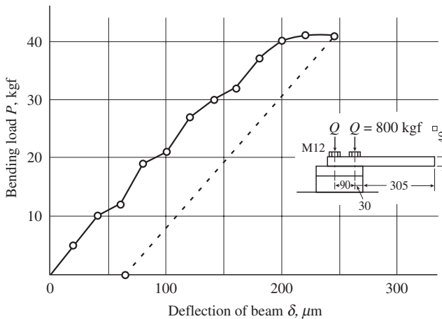
Figure 7-5 Microscopic stick-slip observed at bolted joint under tangential bending load.
