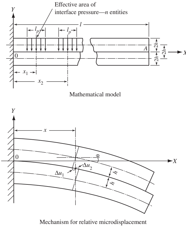
Figure 7-32 Mathematical model of and damping mechanism in two-layered beam in cantilever configuration.
