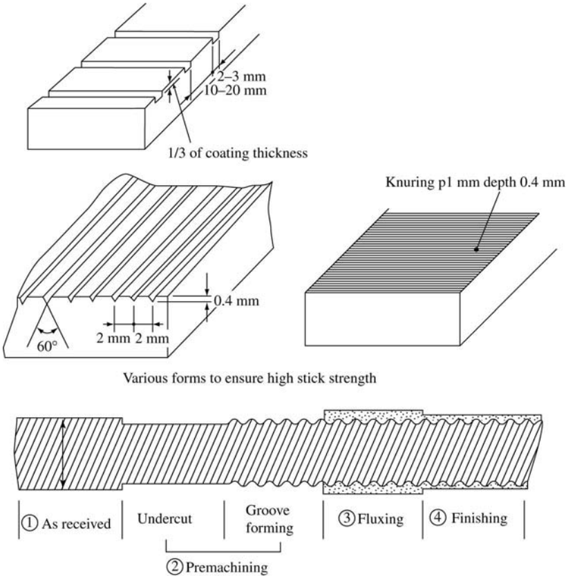
Figures are the process sequence number. Figure 8-11 Producing process of slideway of hard-facing type.
