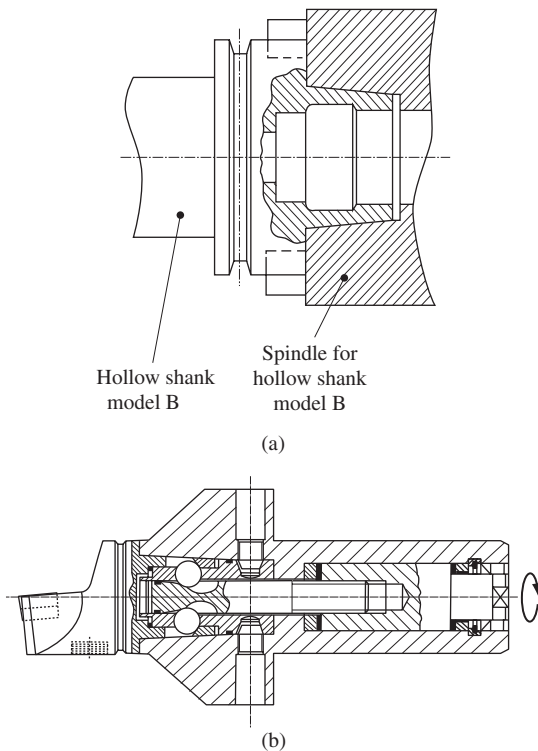
Figure 9-20 HSK-DIN Standard and an application to cutting edge module: (a) Hollow shank model B in DIN 69893 and (b) cutting edge module (by Pegels, courtesy of Carl Hanser).
