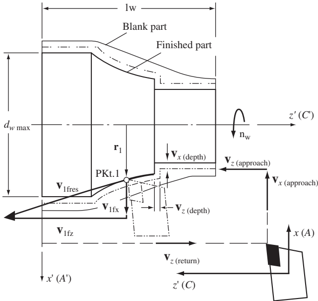
Figure 4-15 Advanced functional description with leading dimensions (courtesy of Saljé).
