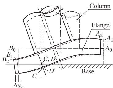
Figure 7-31 Damping mechanism of bolted joint of type B.
