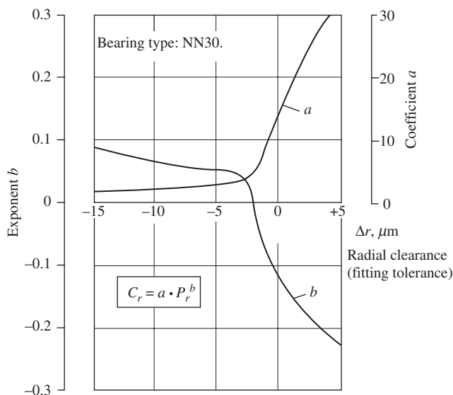
Figure 8-31 Calculation diagram of load distribution factor C_r (by Günther).
