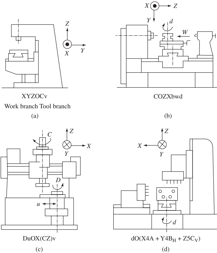
Figure 3-1 Functional description: (a) Vertical milling machine; (b) engine lathe; (c) gear shaper; and (d) rotary indexing machine (by Vragov).
