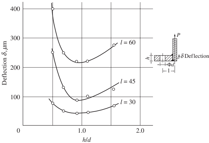
Figure 7-19 Optimum flange thickness of L-shaped bolted flange (by Opitz and Bielefeld).
