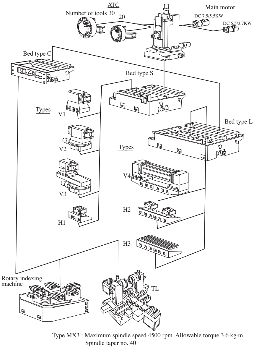
Figure 1-4 Modular design in MC (courtesy of Ikegai Iron Works).
