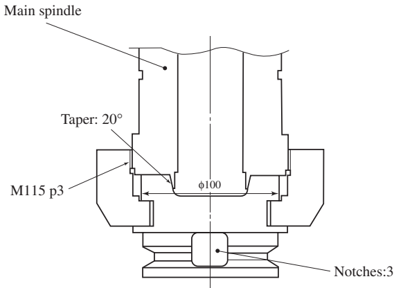
Figure 9-19 Flange mounting tooling developed in the beginning of the 1990s (courtesy of Kuroda Precision Industries).
