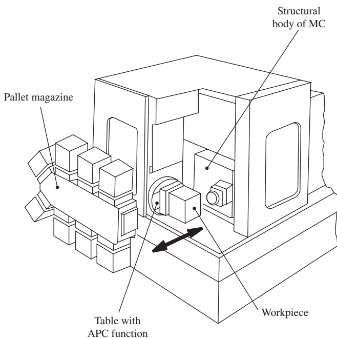
Figure 2-22 Cubiclike FMC of Steinel make (type BZ24FFZ).
