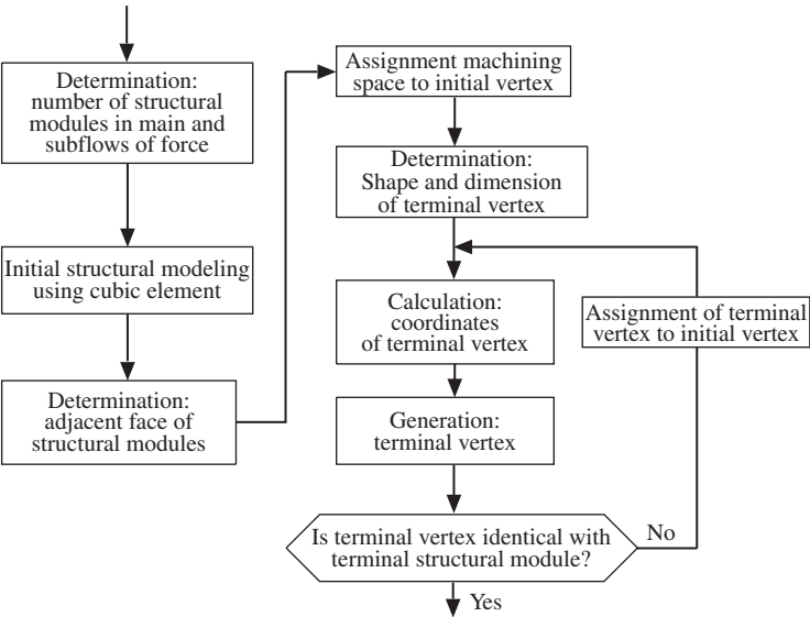
Figure 4-34 Generating procedure for a pair of structural modules.
