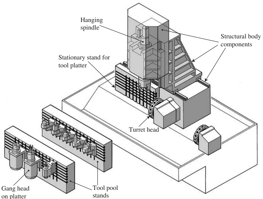
Figure 1-5 An application of modular design to the turning machine (type Vertical Line, 1999, courtesy of Index).
