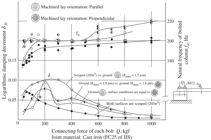
Figure 7-49 Effects of machining methods on damping capacity and natural frequency.
