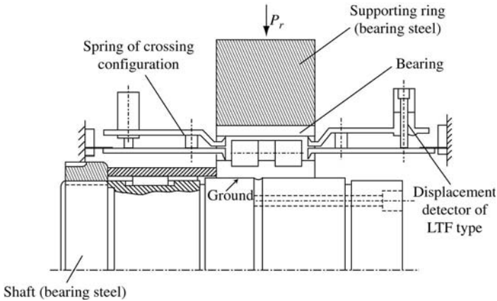
Figure 8-29 Experimental setup for measurement of bearing stiffness (by Günther).
