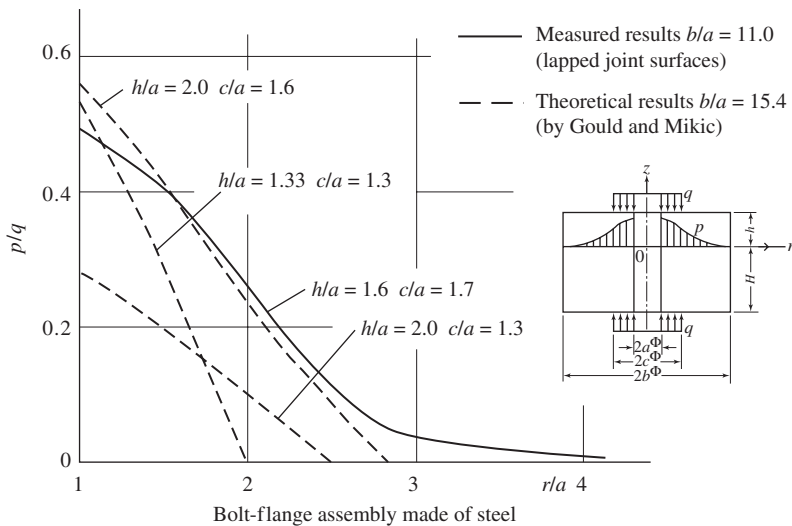
Figure 7-17 Comparison between theoretical and experimental interface pressure distribution.
