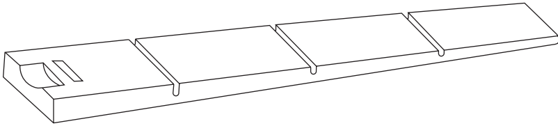
Figure 8-13 Notched gib for cross slide of vertical milling machine.
