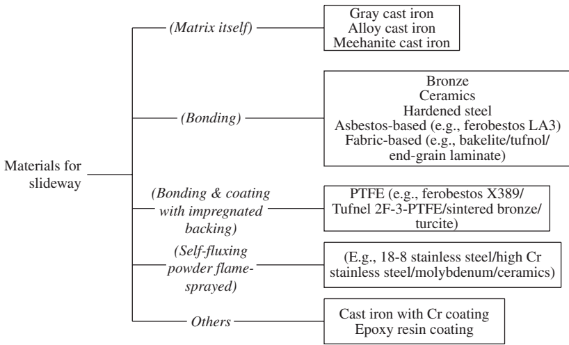
Figure 8-10 Materials applicable to slideway.
