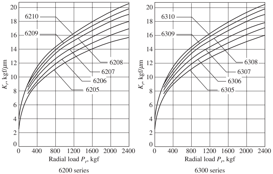
Figure 8-33 Calculation diagram for radial stiffness of ball bearings (by El-Sayed).
