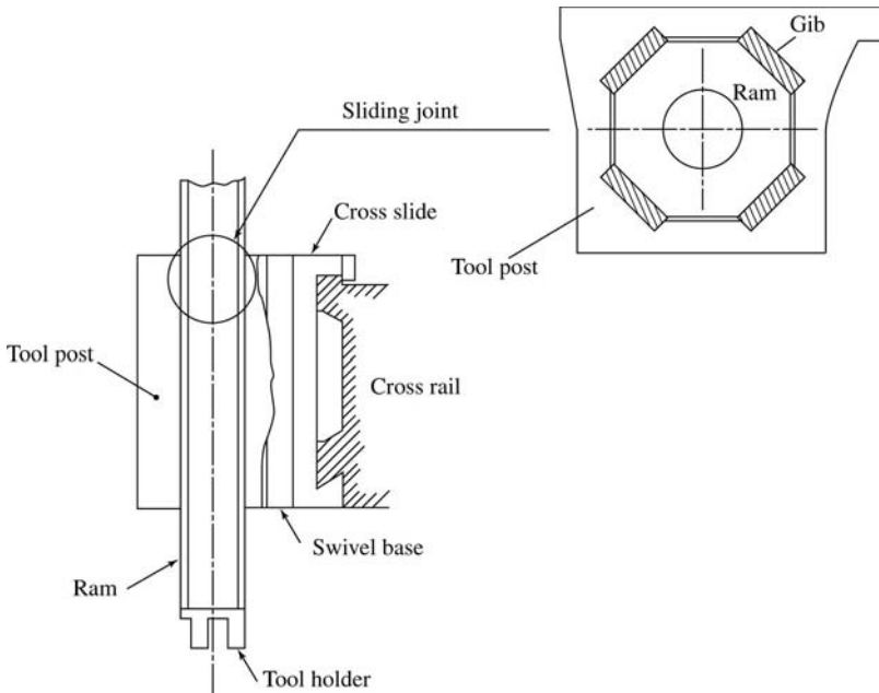
Figure 8-43 Traveling ram of vertical turning machine.
