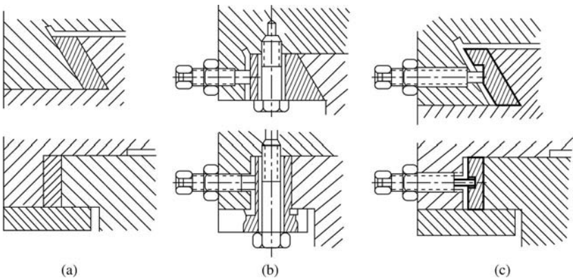
Figure 8-17 Representative gib configurations: (a) Taper gib, (b) strip gib of fixed type, and (c) strip gib.
