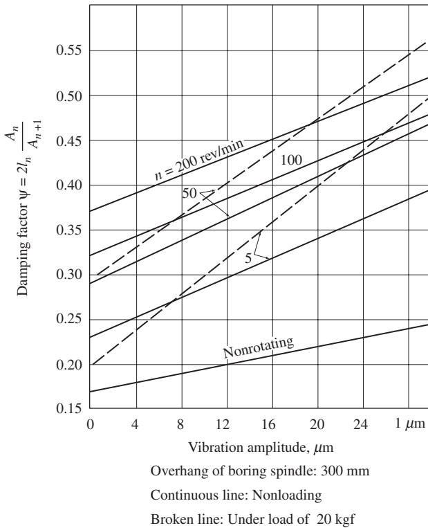
Figure 5-3 Damping capacity of main spindle in horizontal boring machine, measured from decayed free vibration (by Kunin).
