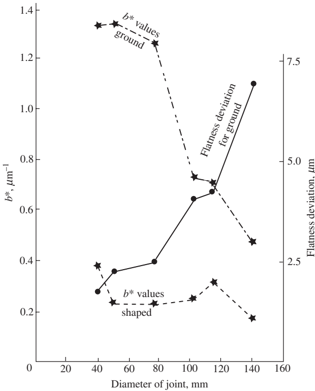
Figure 5-21 Deterioration of joint stiffness by flatness deviation (by Connolly and Thornley).
