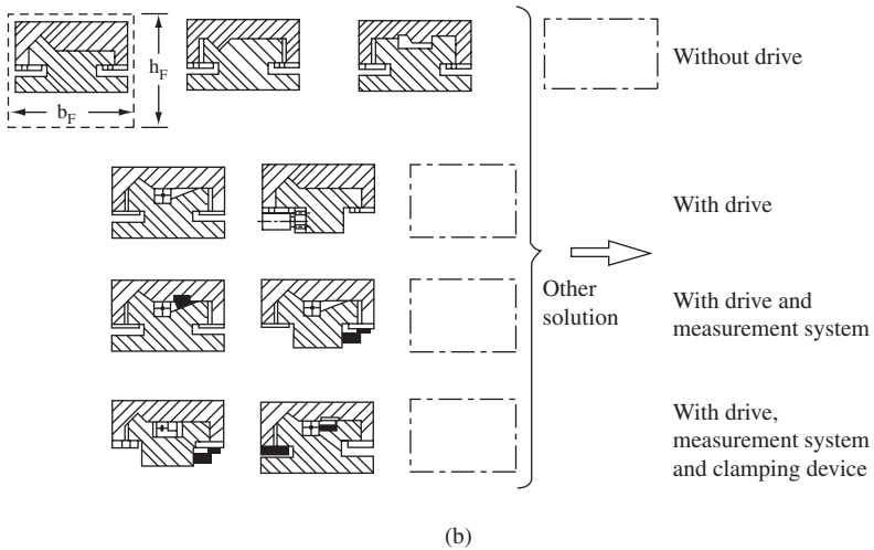
Figure 4-13 Detailed functional description aiming at CAD: (a) General concept representation and (b) catalog of guideways (courtesy of Saljé).
