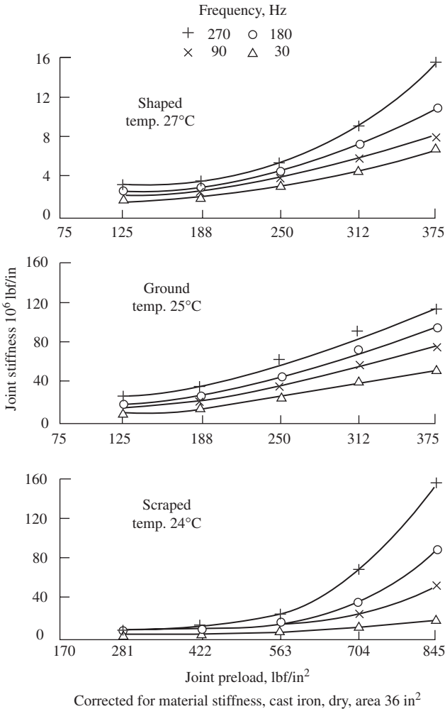
Figure 6-30 Relationships between joint stiffness and static preload when excitation frequency is varied (courtesy of Thornley).
