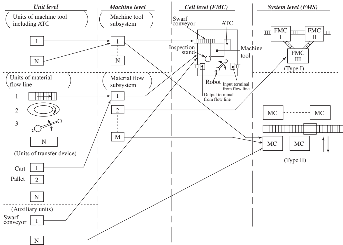
Figure 1-9 Concept of modular design of hierarchical type in FMS design.
