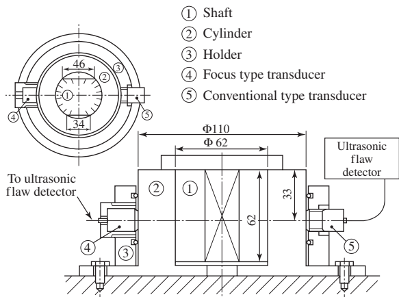
Figure A1-9 Experimental setup to measure contact pattern of press-fitting.
