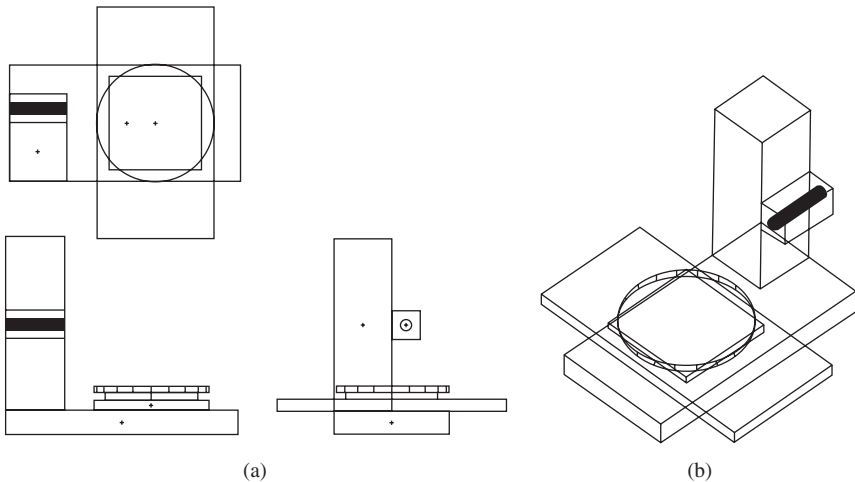
Figure 4-37 Outputs of design results: (a) Plane view and (b) three-dimensional view.
