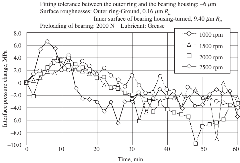
Figure A1-22 Variations of interface pressure with running time.
