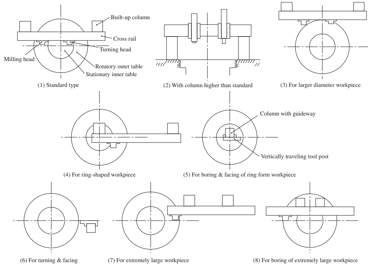
Figure 1-34 Eight variants possible in vertical boring and turning machine of Toshiba Machine make.
