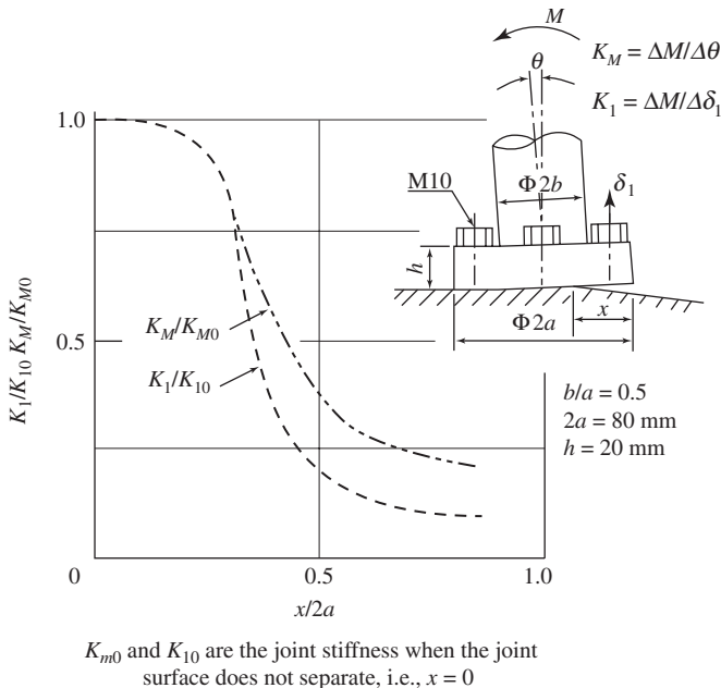
Figure 7-28 Influences of joint separation on deterioration of joint stiffness.
