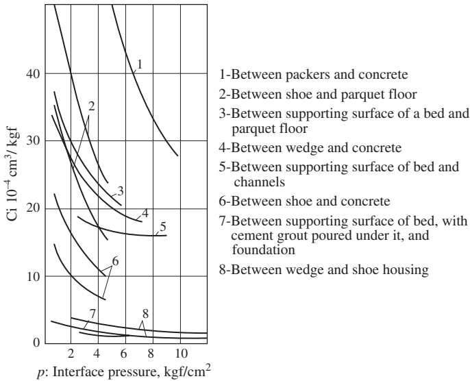
Figure 7-60 Diagram to determine coefficient C_i (by Kaminskaya).
