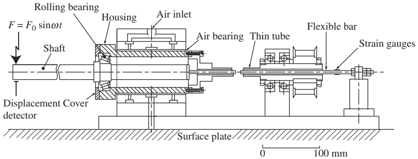
Figure 8-37 Experimental setup to measure damping of bearing while rotating (courtesy of Tsutsumi).
