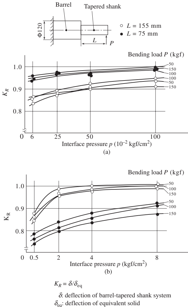
Figure 9-17 Stiffness ratio K_R in taper connection: (a) MT No. 5 and (b) NT No. 40.
