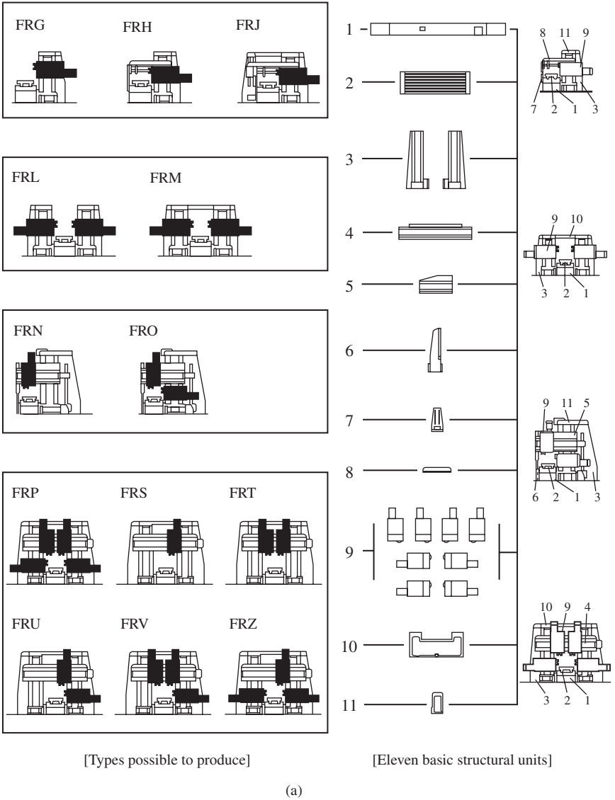
Figure 1-32 Modular design in planomiller: (a) In case of type FR of TOS make and (b) milling heads of quill and ram types (Butler Machine Tool Co.).
