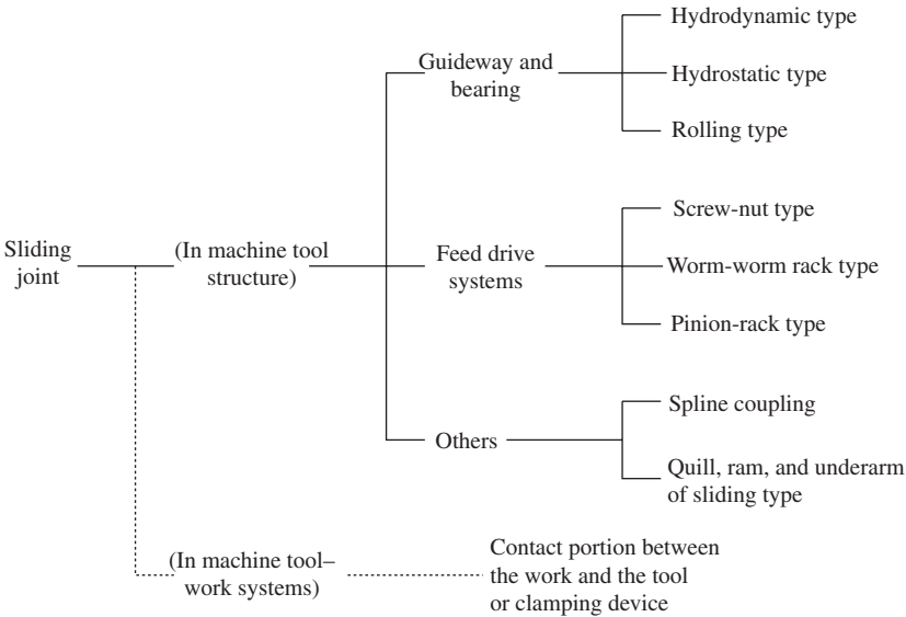
Figure 8-1 Classification of sliding joint.
