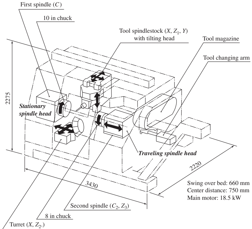
Figure 2-27 Machining complex with modular design—eight-axis control (type TM25YS, courtesy of Ikegai Iron Works).
