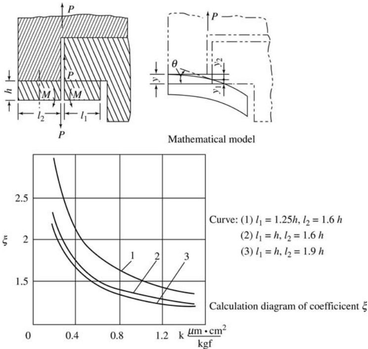
Figure 8-16 Mathematical model of keep plate and calculation diagram of coefficient \xi (by Levina and Ostrovskii).
