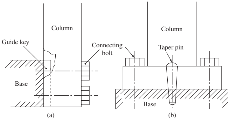
Figure 5-6 Two basic types of bolted joint.
