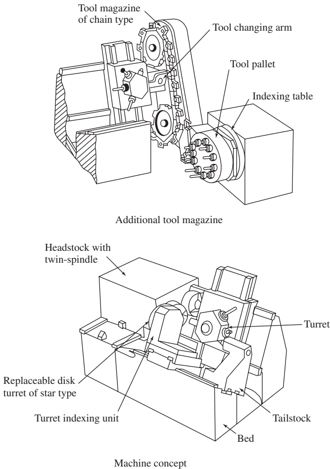
Figure 1-38 Machine tools with modular design in ASP plan (by Astrop, courtesy of Machinery & Prod. Eng. )
