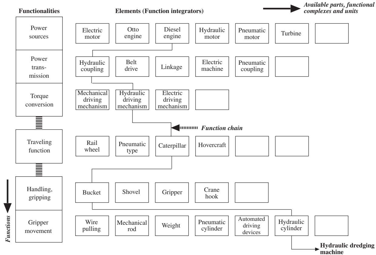
Figure 2-7 Concept of function chain in case of dredging machine (by Brankamp and Herrmann).
