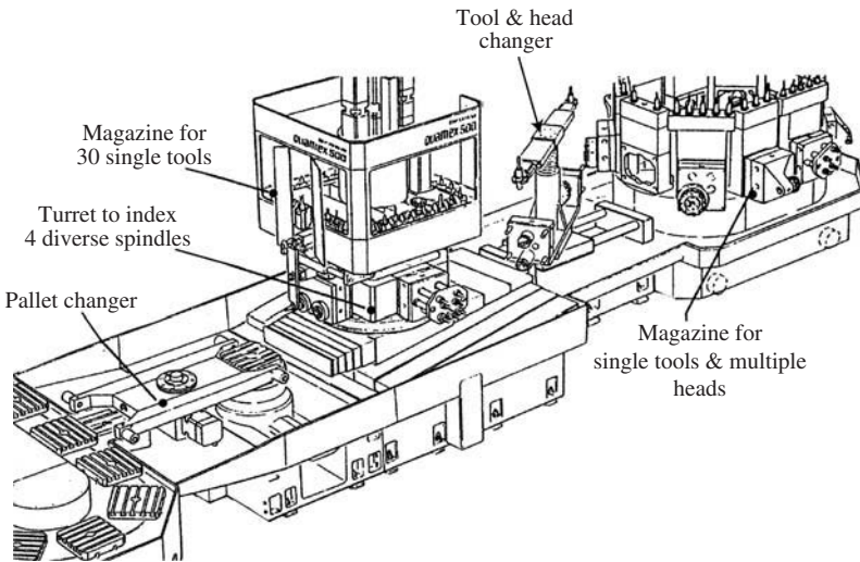
Figure 2-19 CNC station in FTL developed by Ford Co. in mid-1980s (courtesy of Brose Fahrzeugteile GmbH & Co.).
