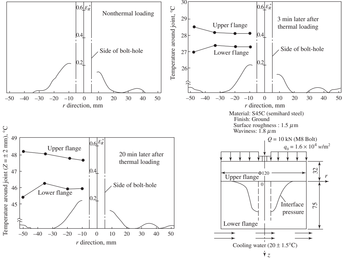
Figure 7-51 Changes of interface pressure distribution when applying steady-state thermal load.
