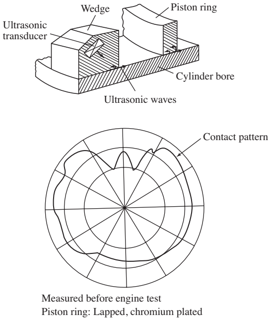
Figure A1-19 Contact pattern of piston ring to cylinder bore (by Rudy).
