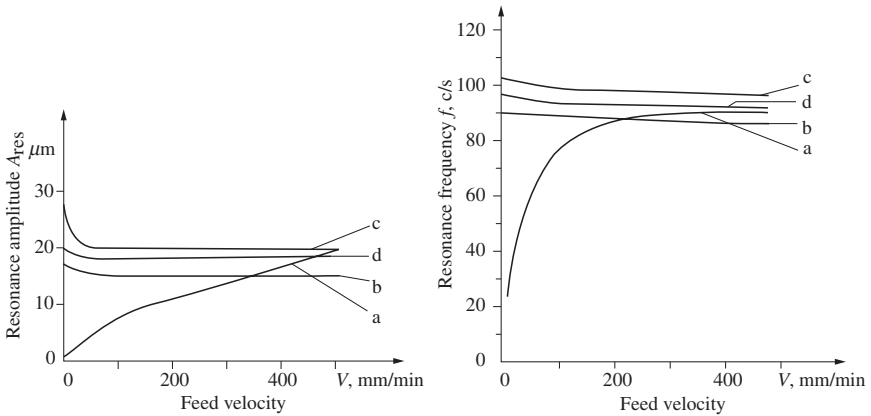
Figure 8-3 Effects of feed velocity on resonance characteristics of various guideways.
