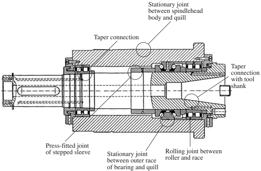
Figure 5-4 Several leading joints in main spindle (modified that of Gebert, courtesy of Carl Hanser).
