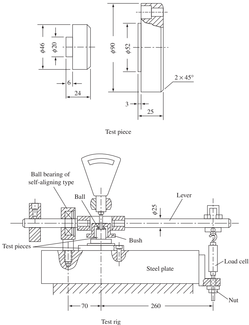
Figure 6-6 Test rig and test pieces used by Ostrovskii.
