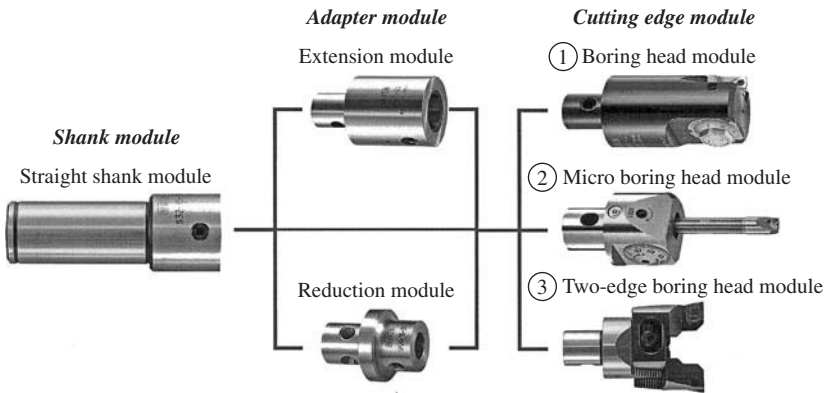
Figure 1-2 Modular boring system (courtesy of Nikken Kosakusho Works).
