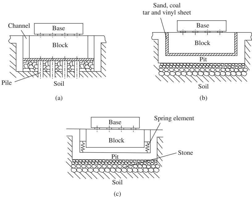
Figure 7-55 Variants of foundation system: (a) Foundation with antivibration channel, (b) two-layered foundation of stationary type, and (c) two-layered foundation of suspension type.
