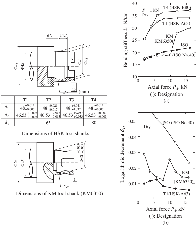
Figure 9-21 Static stiffness and damping capacity of HSK: (a) Comparison of bending stiffness of tools and (b) comparison of damping (courtesy of Tsutsumi).
