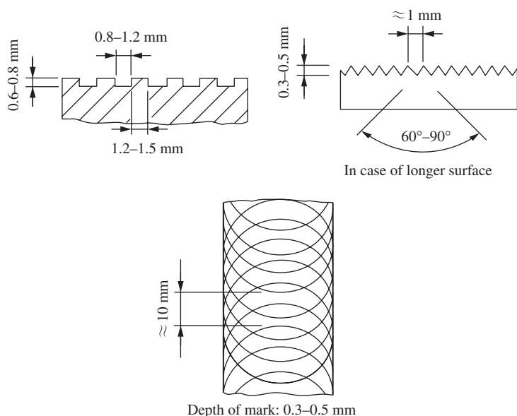
Figure 8-12 Preparatory machining of bed slideway and finished surface with crisscrossed mark (courtesy of Devitt and of SME).
