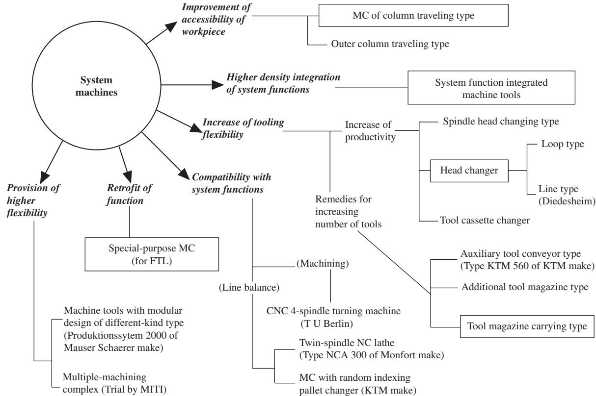
Figure 2-14 Trials for developing system machines.
