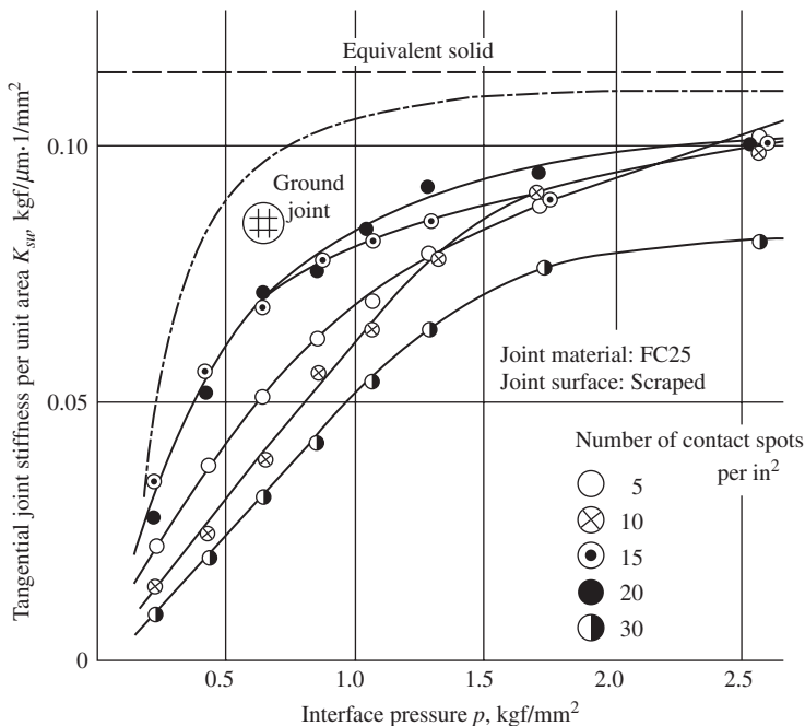
Figure 6-16 Effects of surface finishing quality on joint stiffness.
