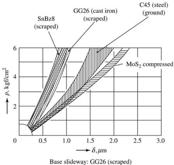
Figure 6-8 Normal joint deflection under lower interface pressure (by Eisele and Corbach).
