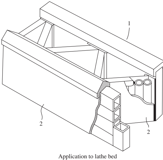
Figure 9-11 A panel structure with temperature control function.
