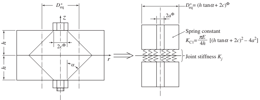
Figure 7-18 Mathematical model for calculating spring constant of clamped component based on pressure cone.
