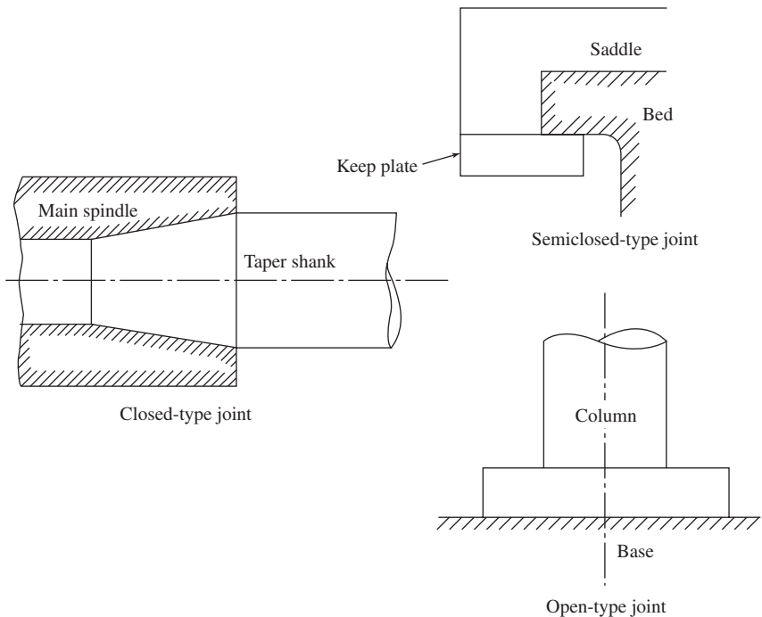
Figure 5-12 Classification of machine tool joints according to configuration aspect.
