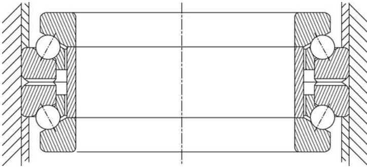
Figure 8-26 Various joints within a rolling bearing—in case of angular contact thrust ball type.
