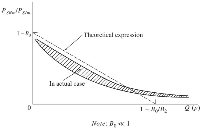
Figure A1-4 Relationships between P_{SRm}/P_{SIIm} and interface pressure p .
