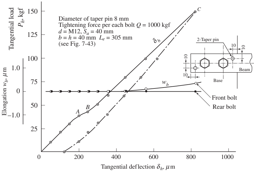
Figure 7-42 Tangential deflection of bolted joint with taper pin.
