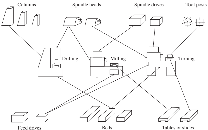
Figure 1-10 Concept of different-kind generating modular design (courtesy of Koenigsberger).
