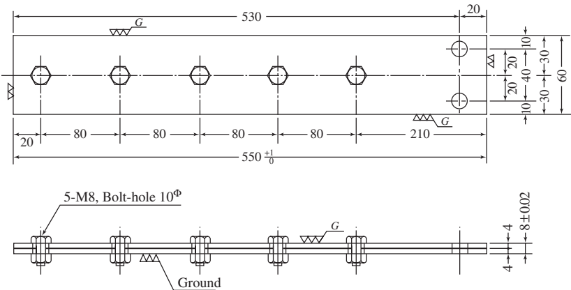
Figure 7-35 Two-layered beam for experiments.
