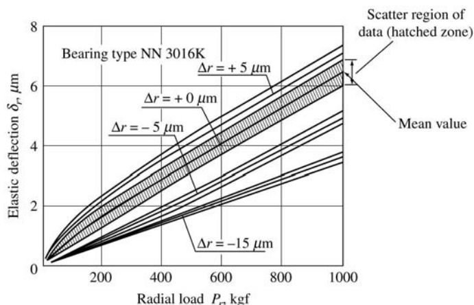
Figure 8-30 Measured values of bearing stiffness (by Günther).
