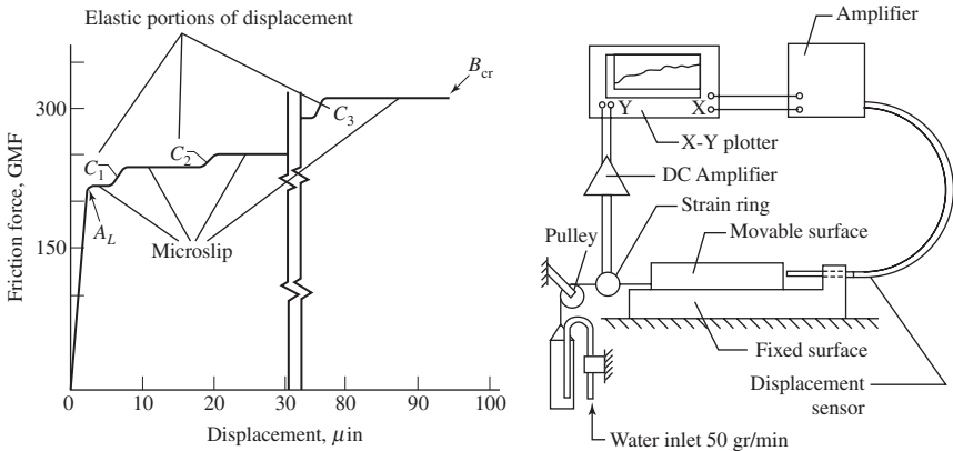
Figure 6-22 Microslips and stick-slip-like movement prior to start of macrosiding (by Simkins).
