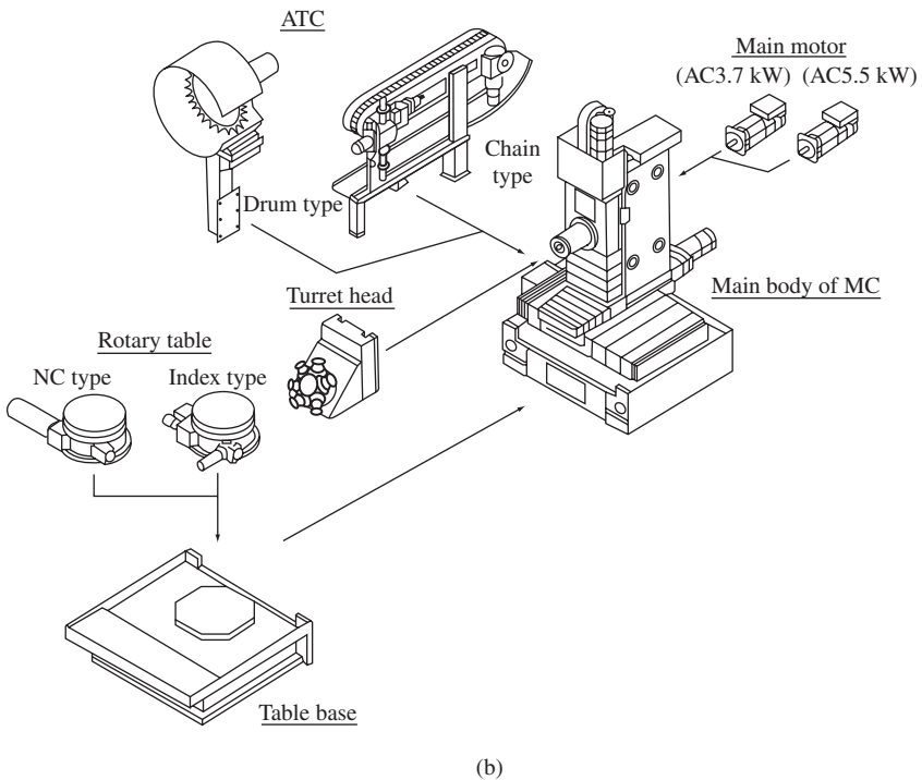
Figure 1-23 Core machines for and concept of FTL: (a) MC of line type and head changer (1989, courtesy of Toyoda Iron Works); (b) modules in MC of line type (type NF1-H, 1990, courtesy of Fujikoshi); and (c) FTL for machining cylinder head, cylinder block, mission case, and so on (1990s, courtesy of Toyama).
