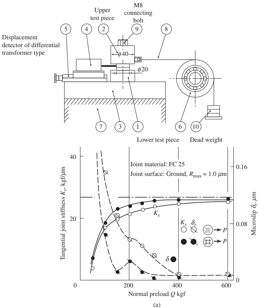
Figure 6-15 Tangential joint stiffness and microslip in varying normal preload: (a) For cast iron joint and (b) for brass joint.
