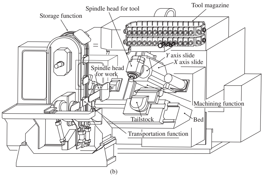
Figure 2-23 System machine of function-integrated type: (a) MA type (on market from 1982) and (b) TA3 type (not on market) (courtesy of Tsugami Co.).
