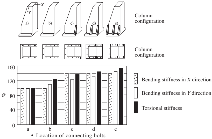
Figure 7-21 Effects of stiffening ribs on stiffness of bolted column with bay-type flange (by Opitz and Bielefeld).
