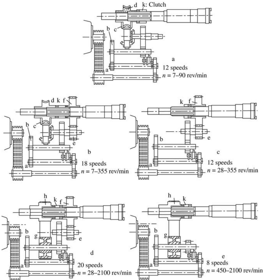
Figure 1-30 Modular design in main spindle driving system (Wanderer Co., 1960s).
