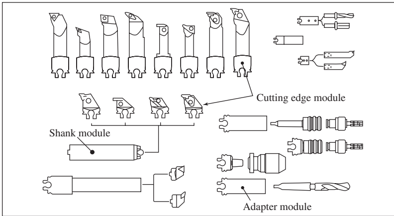
Assembly diagram
