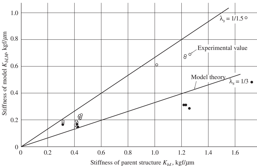
Figure A2-5 Model testing in consideration of joint : tangential stiffness of bolted cantilever.
