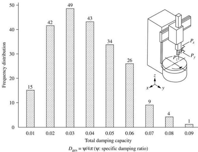
Figure 6A-1 Scatter of measured damping capacity in practical cases (courtesy of Groth).
