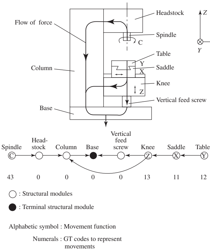
Figure 4-23 Basic structural pattern for milling machine of knee type.
