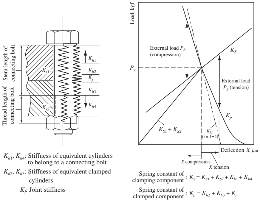
Figure 7-10 Load-deflection diagram of bolt-flange assembly in consideration of nonlinearity in spring constant (by Plock, courtesy of Industrie-Anzeiger).
