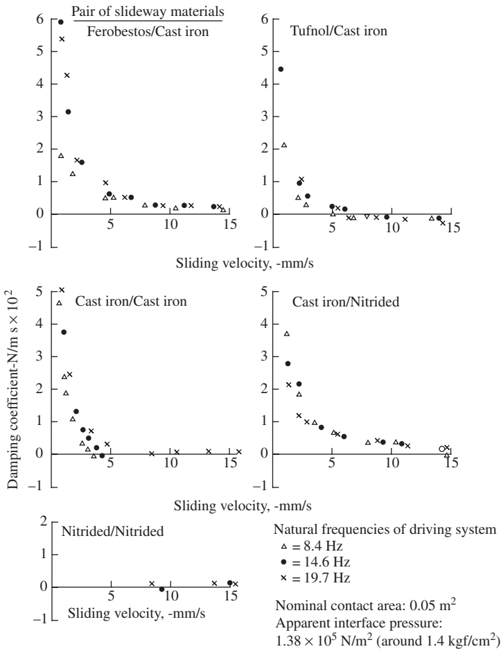
Figure 8-6 Damping characteristics of slideway with polar additive lubricant Tonna (courtesy of Bell).
