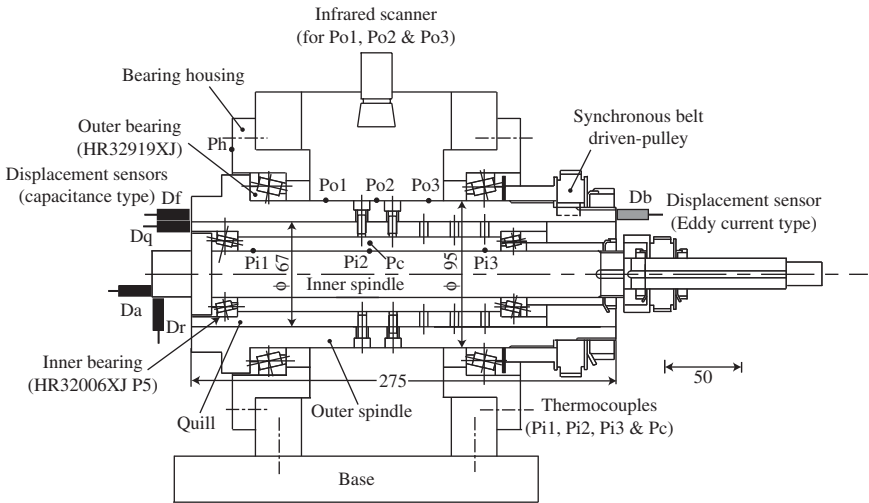
Figure 8-42 Schematic view of experimental setup for an innovative two-layered spindle.
