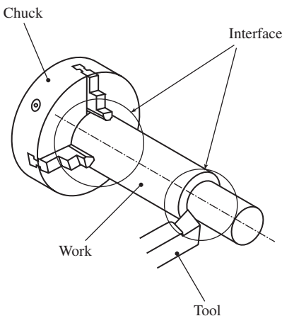
Figure 9-22 A machine-chuck-work-tool system.
