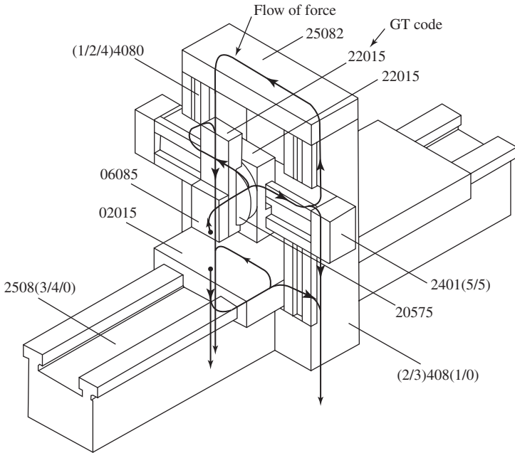
Schematic view of planer
