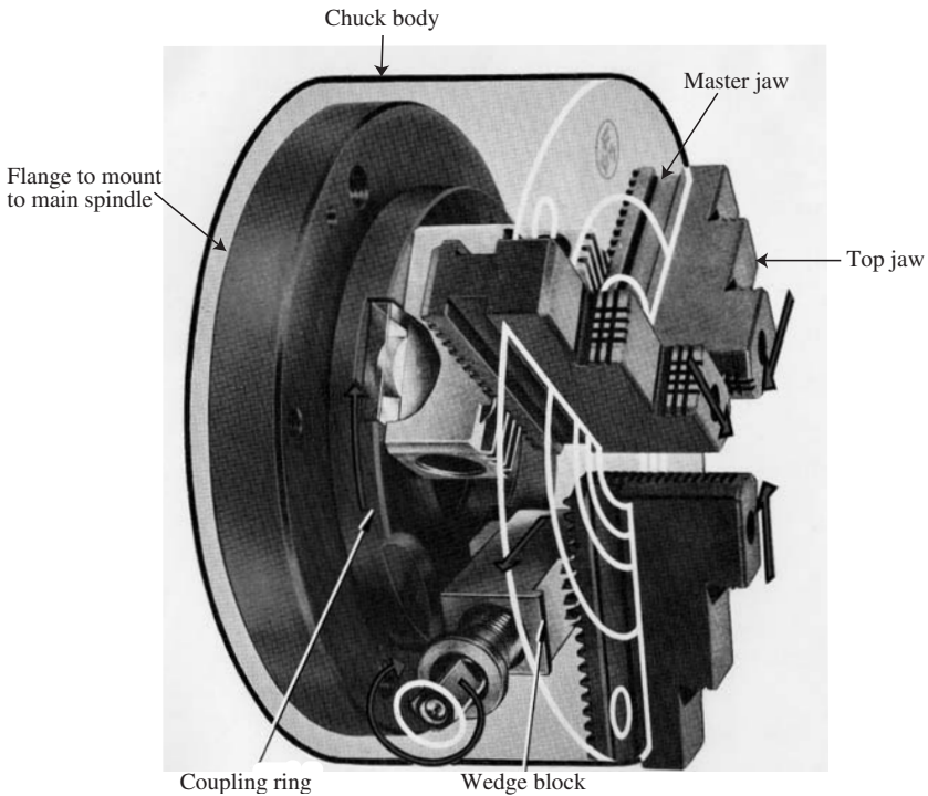
Figure 9-23 A sectional view of three-jaw wedge chuck.
