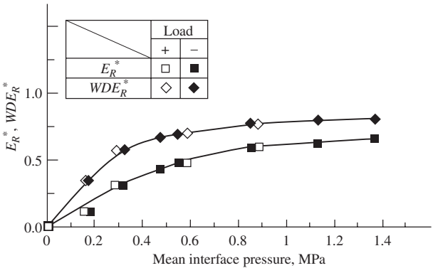
Figure A1-23 Correlation of E_R^* and WDE_R^* to interface pressure (courtesy of Hara).
