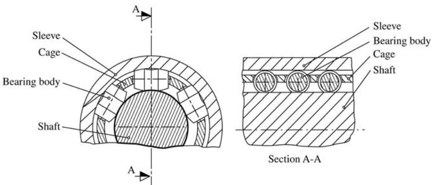
Figure 8-22 Linear roller guide for round way—roller with concave track (by Renker).
