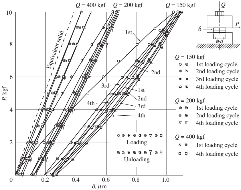
Figure 6-14 Tangential joint deflection under repeated loading cycles—with higher preinterface pressure.
