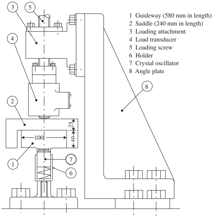
Figure 6-40 Experimental setup for measuring joint stiffness by means of ultrasonic waves.
