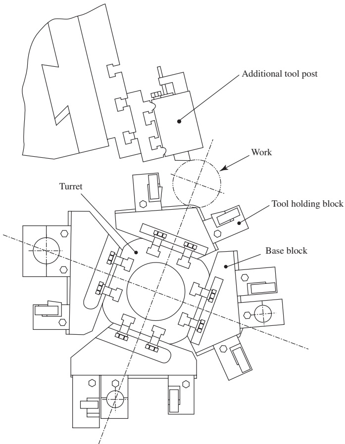
Figure 1-3 Modular principle applied to tool layout on turret (by Dietz, courtesy of Carl Hanser).
