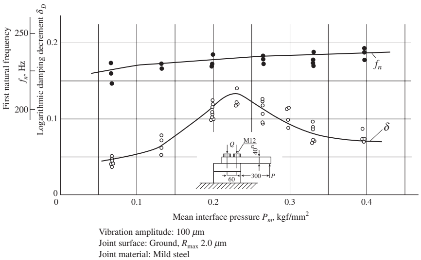
Figure 7-7 Bolted joint showing maximum damping capacity with respect to interface pressure.
