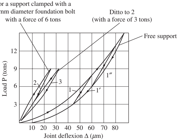
Figure 7-58 Load-joint deflection curves of leveling block (by Faingauz).
