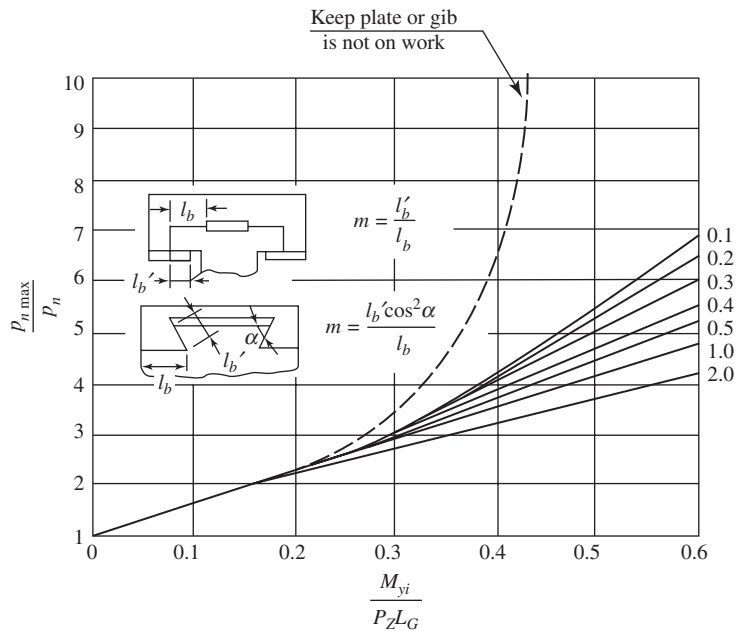
Figure 8-S5 Calculation diagram for maximum interface pressure.
