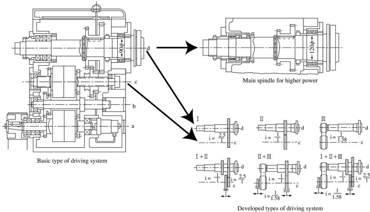
Figure 1-29 Modular design in main spindle and its driving system (type Heycomat of Heyligenstadt make, 1962).
