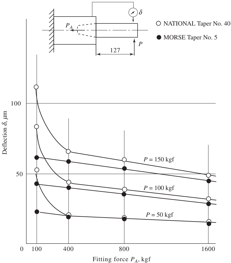
Figure 9-18 Relationships between deflection and fitting force for both types of tapers.
