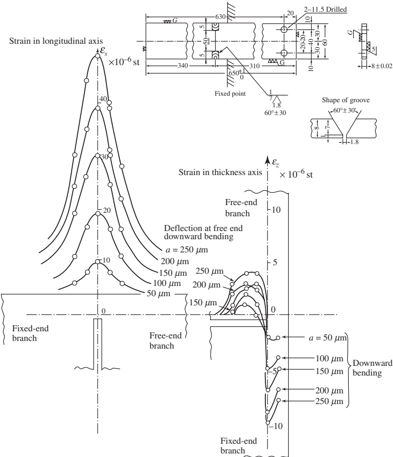
Figure 9-7 Stress concentration at intermittent welded joint.
