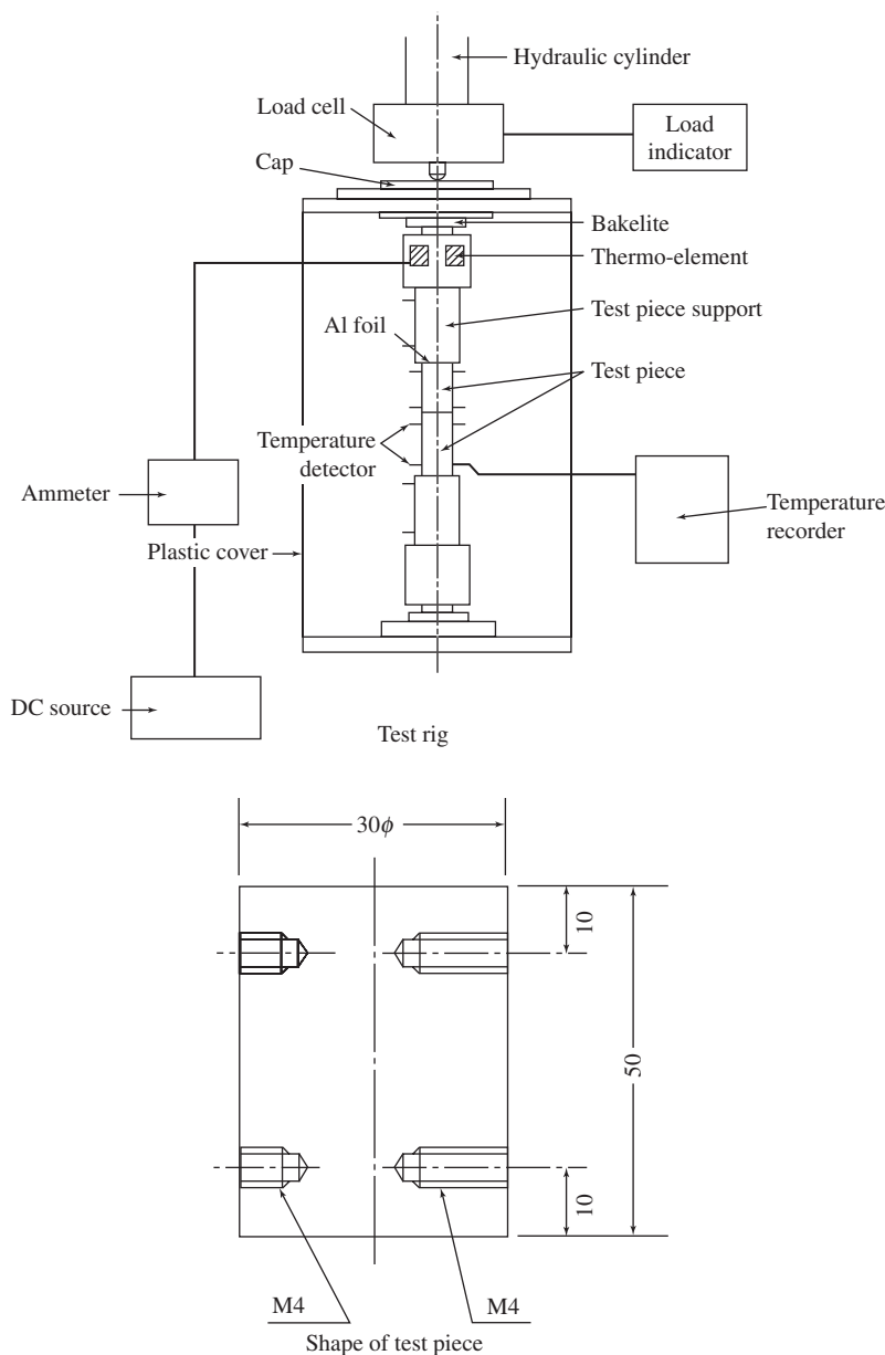
Figure 6-34 Setup to measure thermal contact resistance (courtesy of Yoshida).
