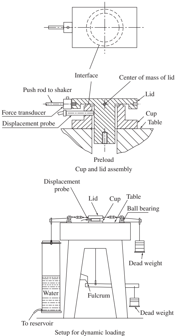
Figure 6-19 Test rig for dynamic tangential behavior of flat joint (courtesy of Boothroyd).
