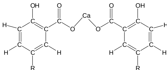
FIGURE 19.4 Calcium salicylate structure.
