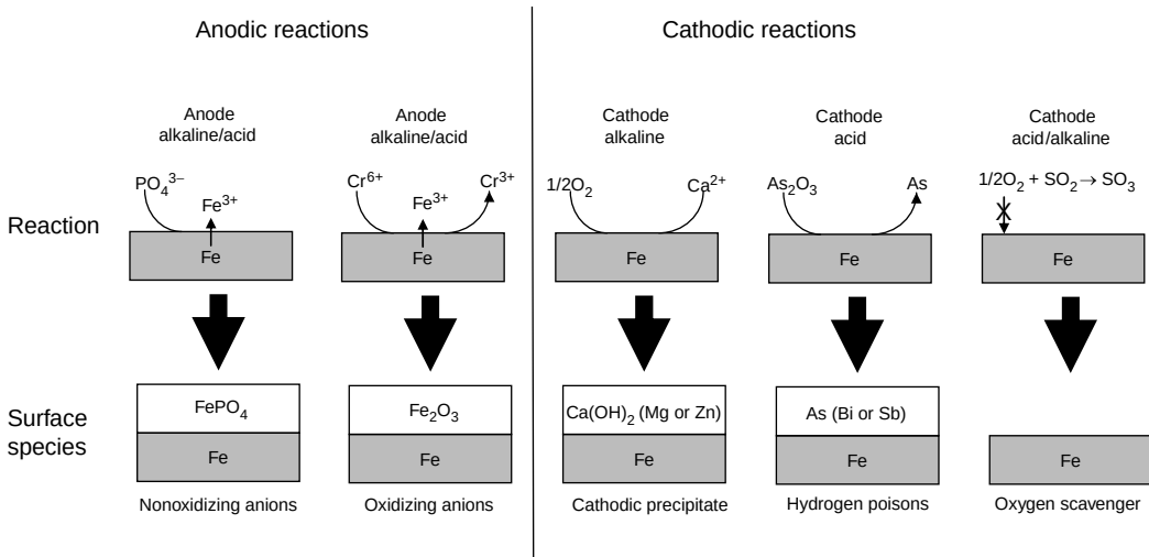
FIGURE 17.3 Schematic mechanism of cathodic and anodic corrosion inhibitors.
