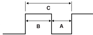
Fig. 1.17 Duty cycle
