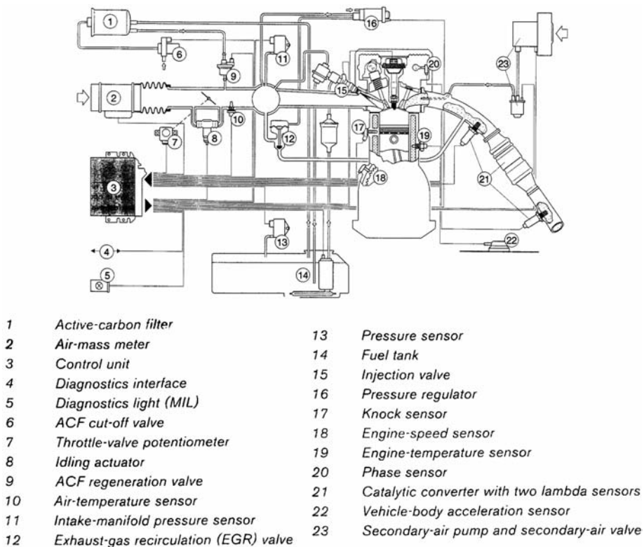
Fig. 8.15 A system that meets OBD II requirements (Bosch)
