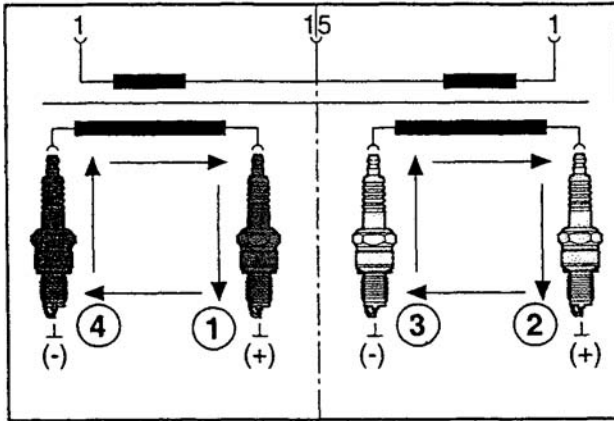
Secondary current : ignition circuit 1-4
