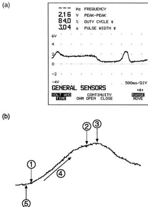
Fig. 7.28 Testing a manifold absolute pressure sensor
