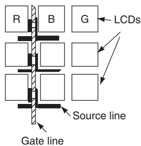
A small part of an LCD screen Each cell is controlled by a mosfet TFT via source and gate lines
