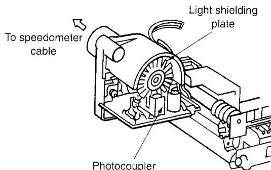
Fig. 5.8 An optoelectronic sensor
