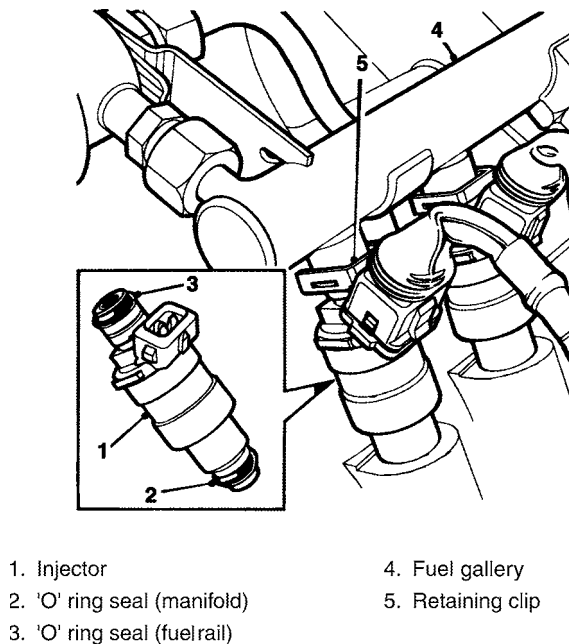
Fig. 1.15 The fuel gallery
