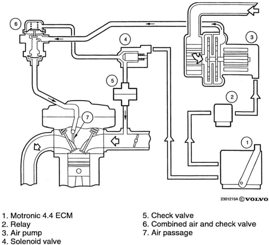
Fig. 8.17 Secondary air injection system
