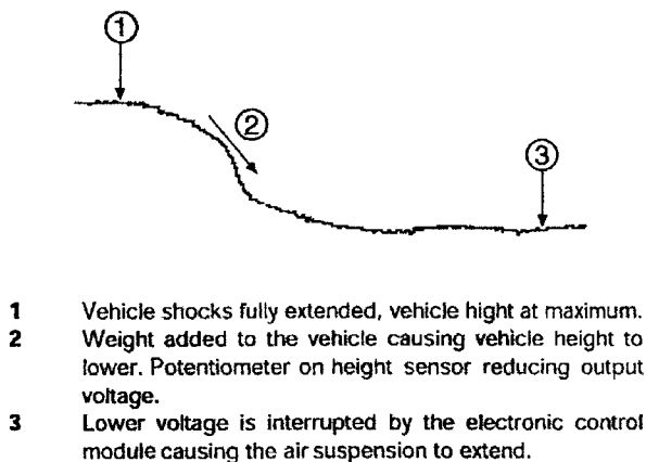
Fig. 5.20 Typical voltage trace for a ride height sensor
