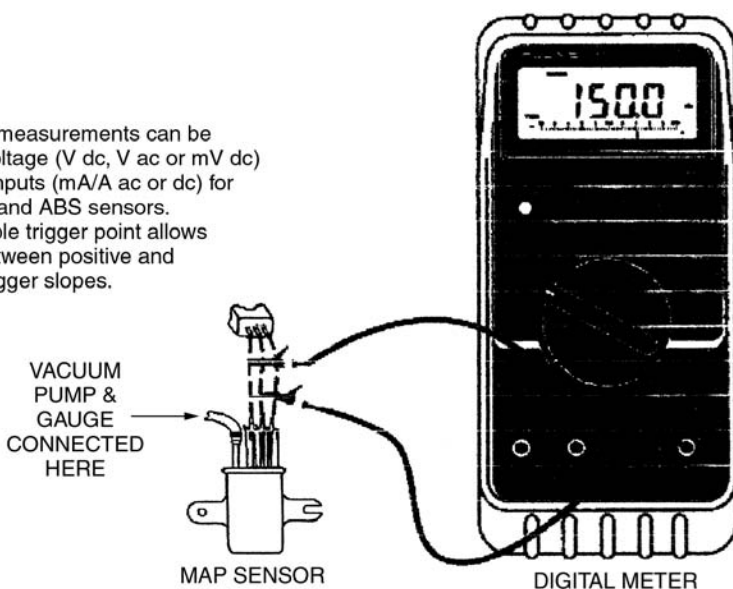
Fig. 4.19 A manifold absolute pressure sensor test
