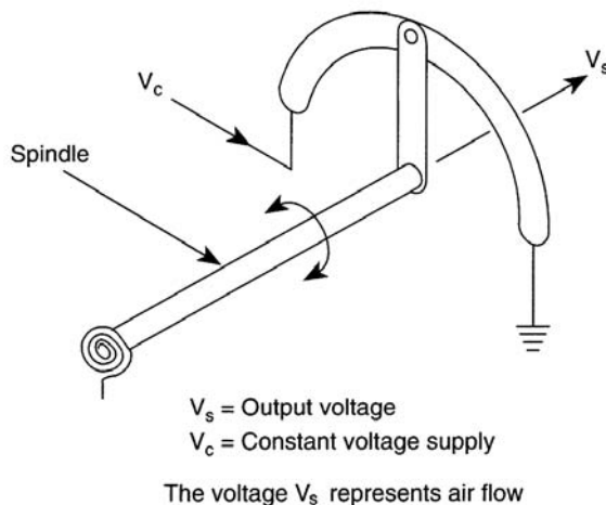
Fig. 5.37 The potential divider applied to an air flow sensor
