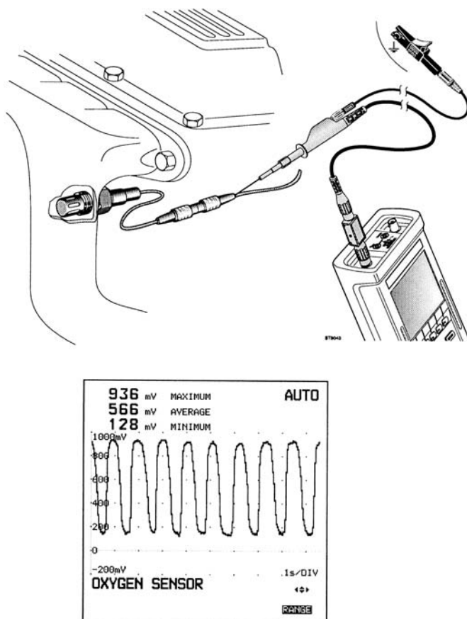
Fig. 7.8 Voltage test at the sensor using the Bosch PMS 100 portable oscilloscope
