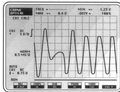
Fig. 5.4 A crank sensor voltage pattern
