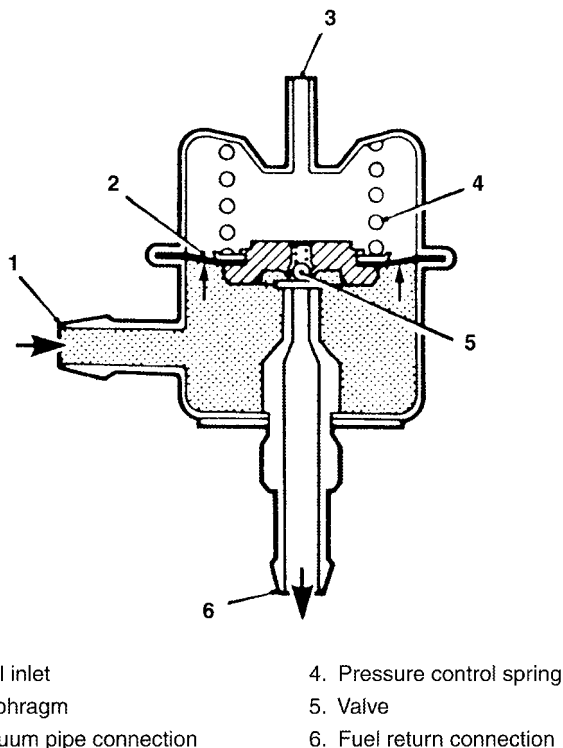
Fig. 1.16 The fuel pressure regulator
