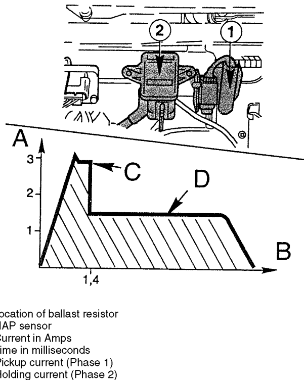
Fig. 6.3 Electric current pattern in injector
