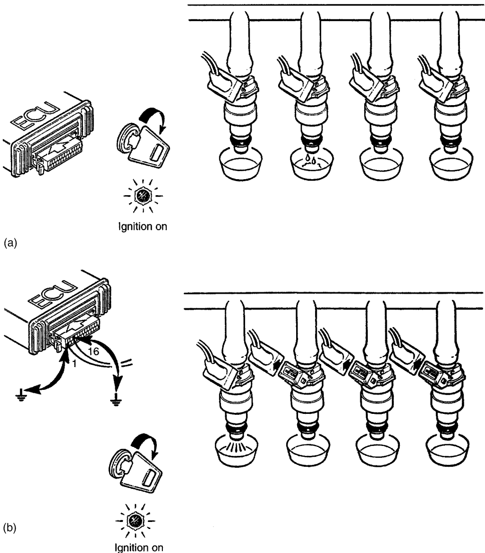
Fig. 6.8 The general principle of a petrol injector test. (a) Testing injectors for leakage. (b) Testing the amount of fuel injector
