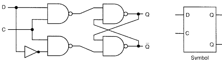
Fig. 2.7 A computer memory element
