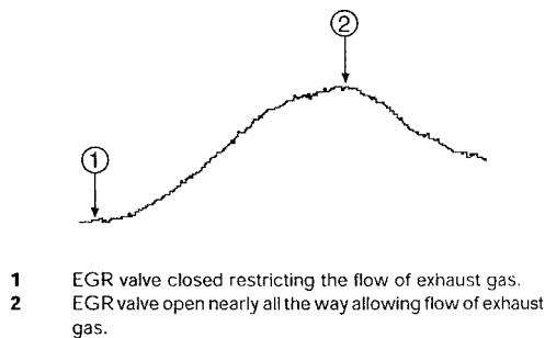
Fig. 6.9 An impression of the voltage trace from an EGR sensor
