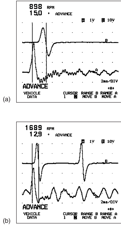
Fig. 7.37 Diesel injection advance
