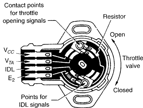
Fig. 5.15 Throttle sensor (Toyota)
