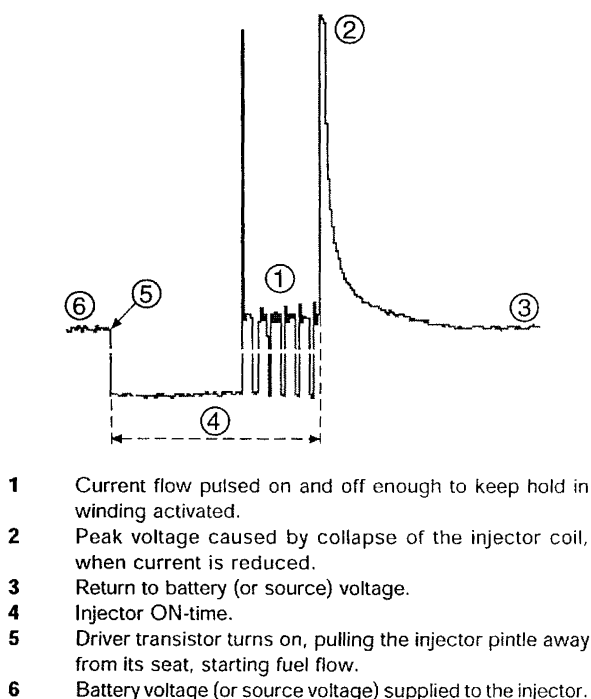
Fig. 6.7 Oscilloscope trace for a pulse width modulated injector
