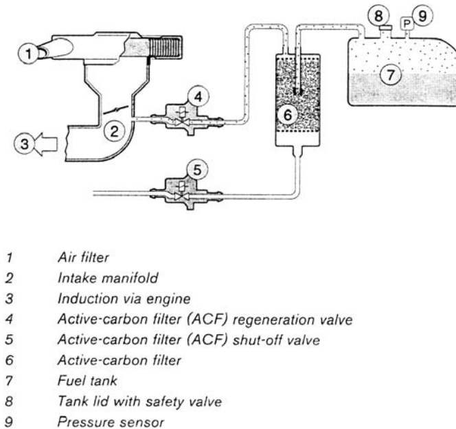
Fig. 8.16 The elements of a leakage detection system
