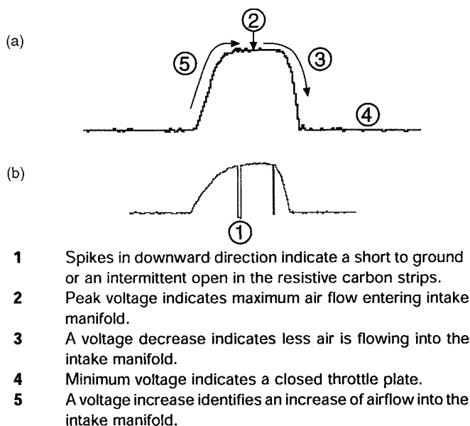
Fig. 7.19 Potentiometer-type air flow sensor voltage signal
