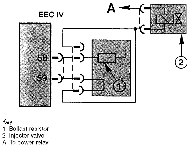
Fig. 6.4 Injector circuit
