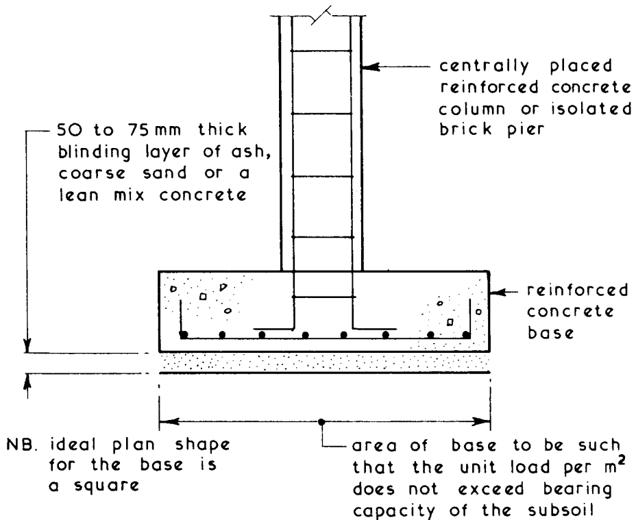
ISOLATED PAD
