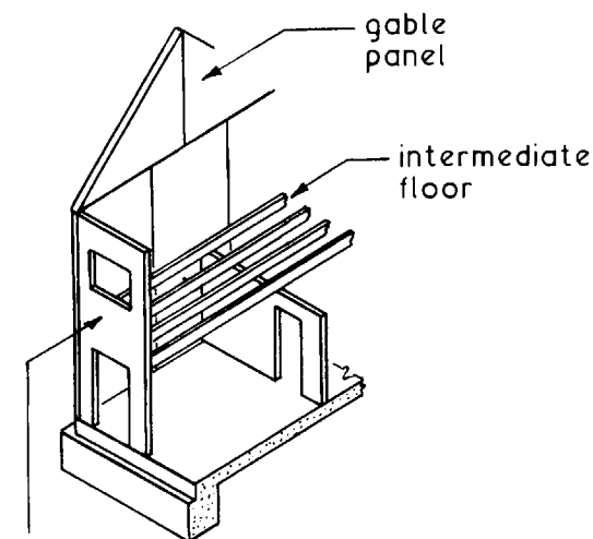
2-storey height panels BALLOON FRAME
