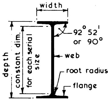
UNIVERSAL BEAMS
