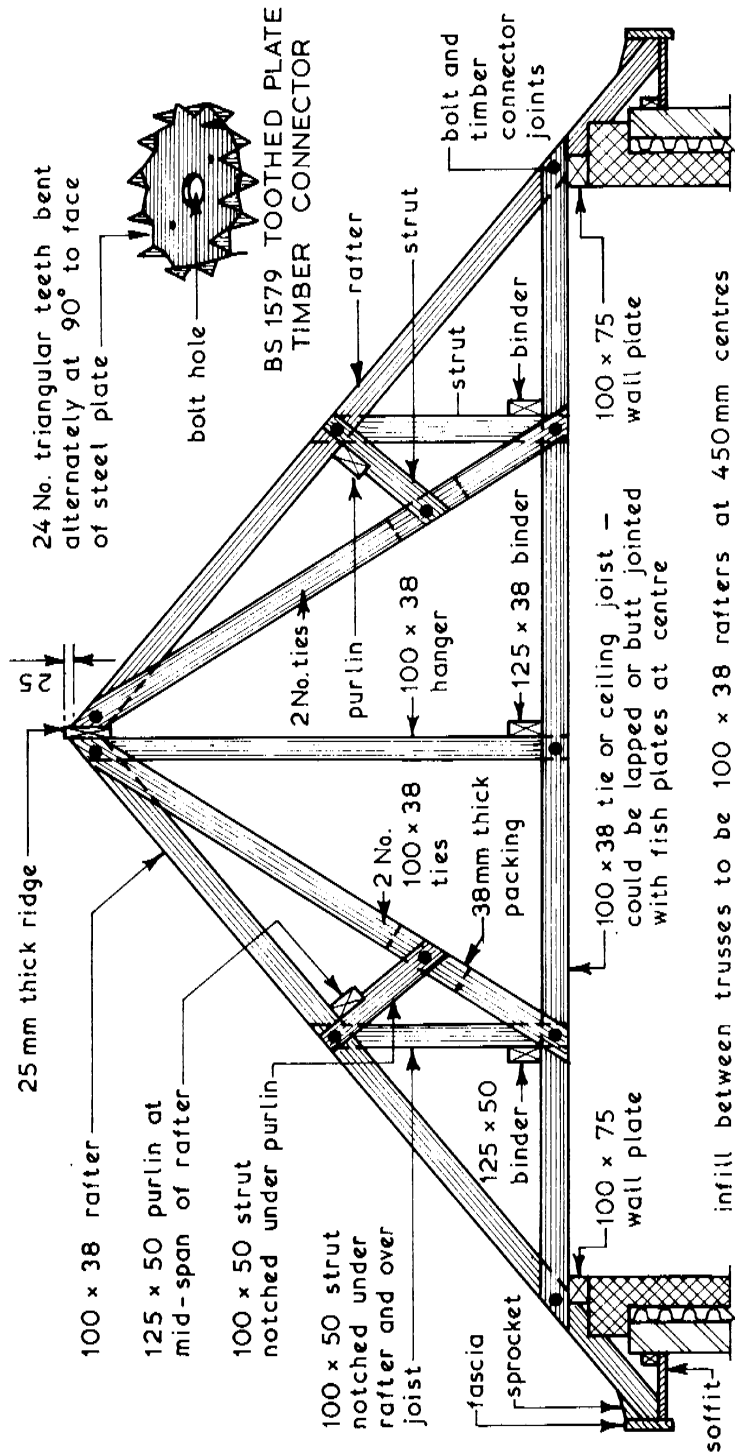
TYPICAL ROOF TRUSS DETAIL
