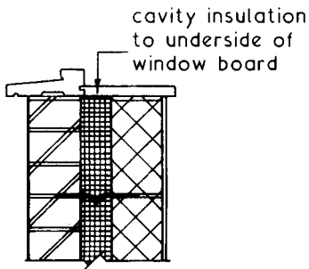
WINDOW SILL
