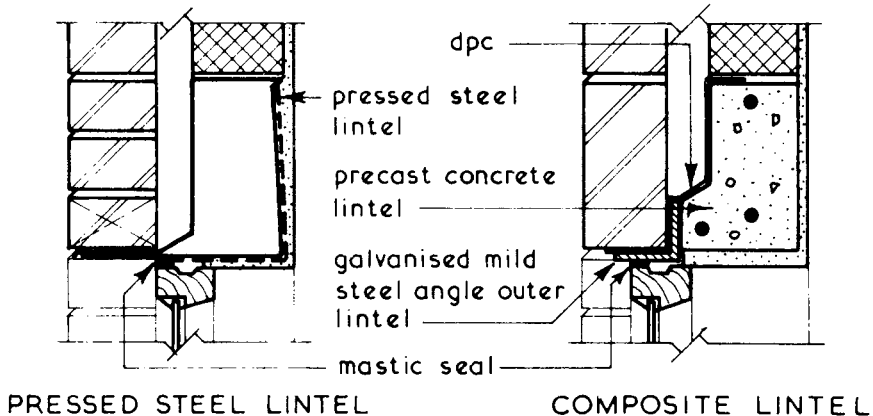
PRESSED STEEL LINTEL
