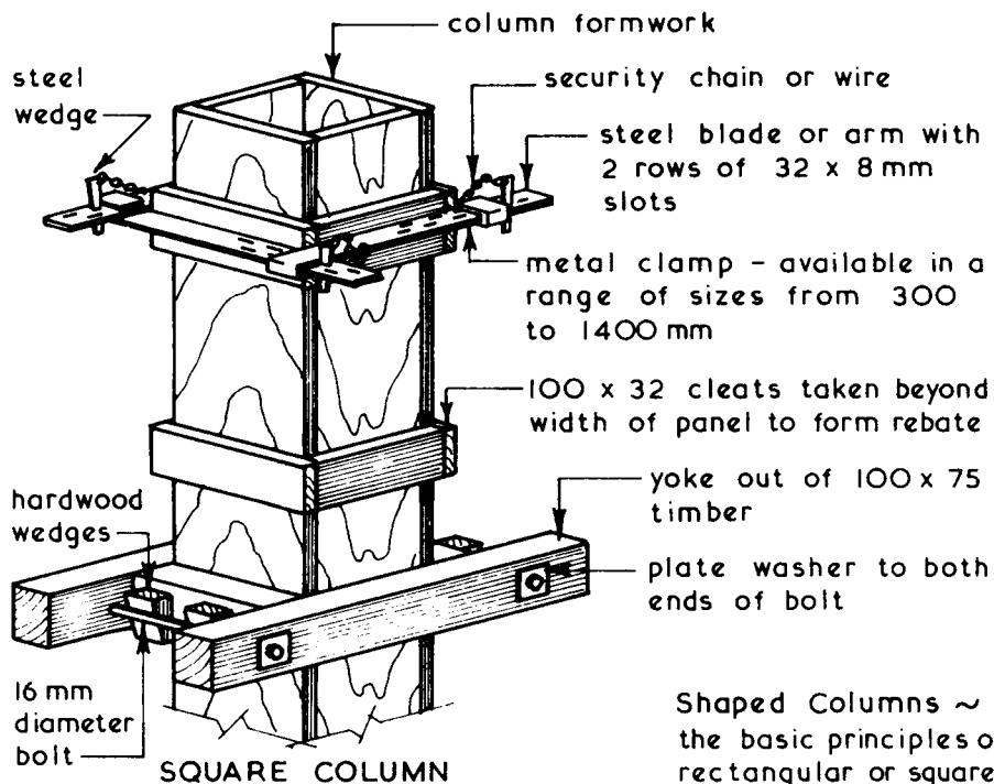
SQUARE COLUMN
