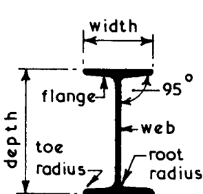
JOISTS
