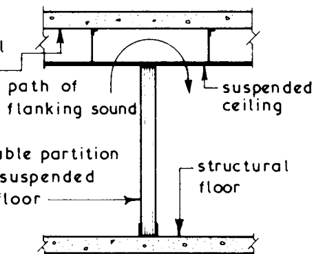
METHOD 2 - easily demounted and re-erected if ceiling can take pressure, flanking sound may be a problem.
