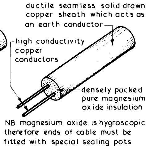
MINERAL INSULATED CABLE
