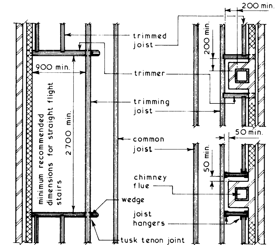
TRIMMING TO STAIRWELL
