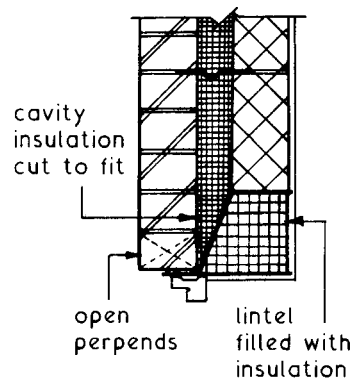
WINDOW/DOOR HEAD
