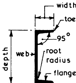
CHANNELS
