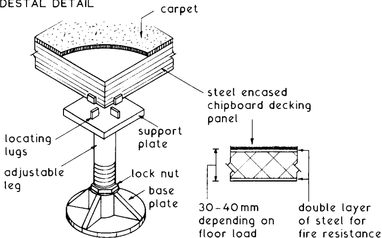
PEDESTAL DETAIL
