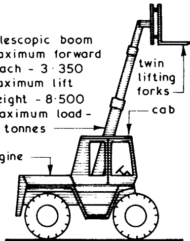
TELESCOPIC BOOM FORKLIFT
