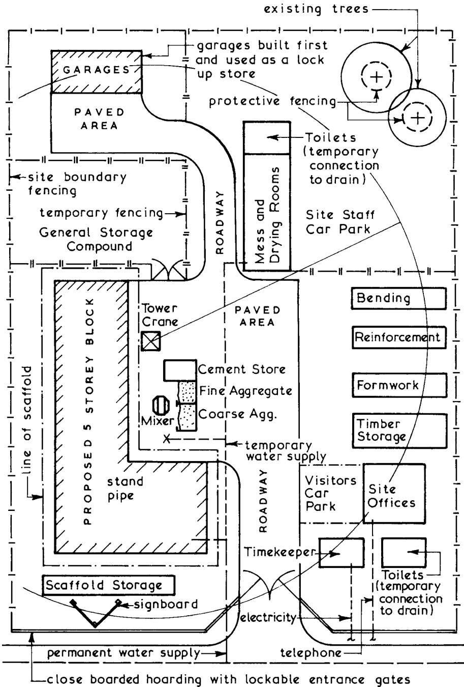
Typical Site Layout Example ~
