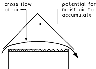
Partial roof void ventilation through the eaves
