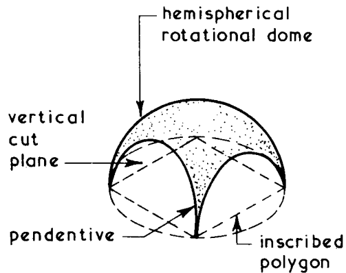
PENDENTIVE DOME
