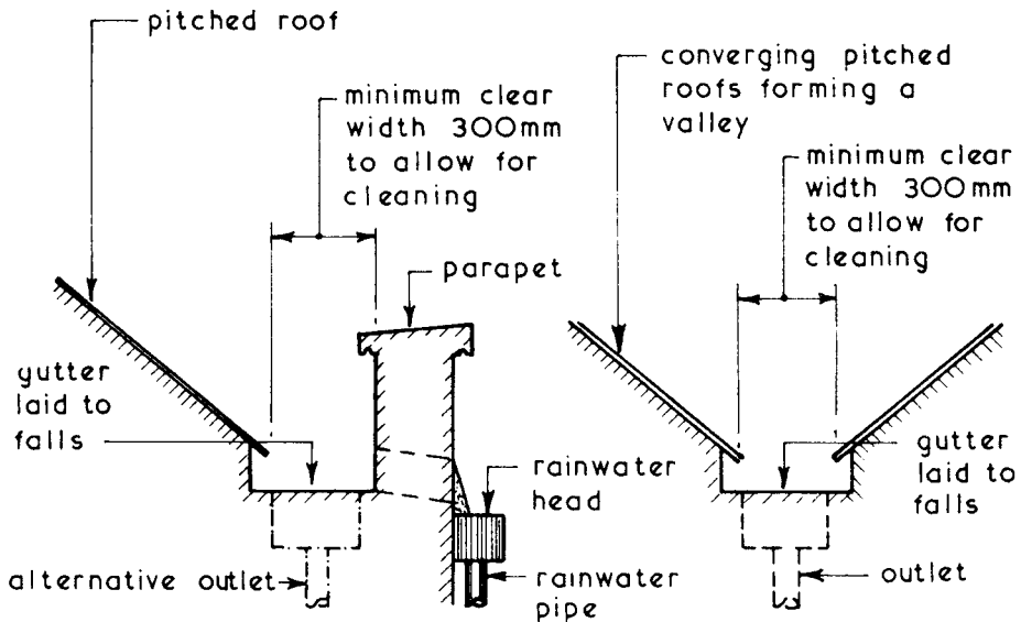
PARAPET GUTTER
