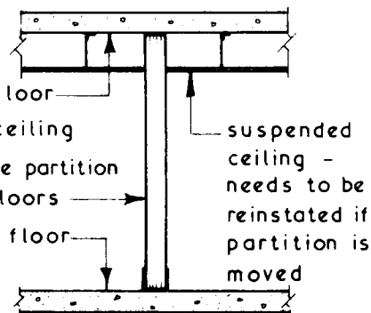
METHOD 4 - alternative to 3
