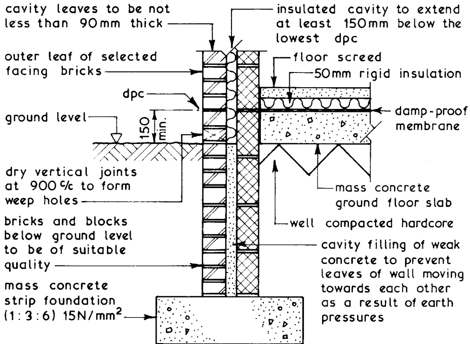
TRADITIONAL CONSTRUCTION
