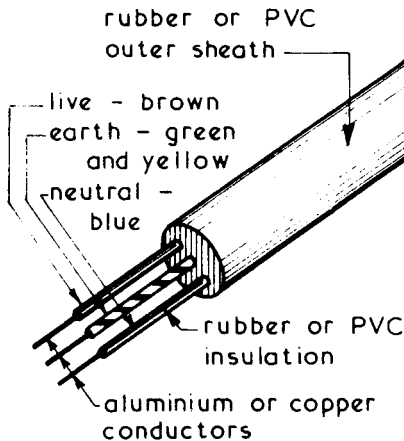
SHEATHED CABLES
