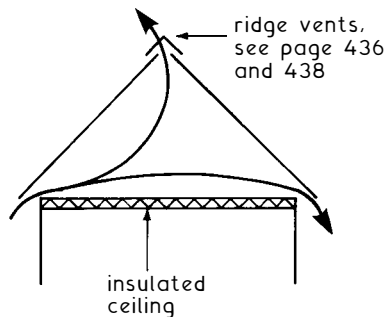
Total roof void ventilation through eaves and high level vents
