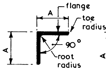
EQUAL ANGLES
