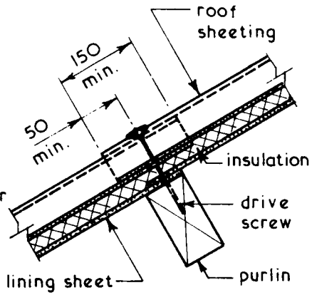
TIMBER PURLIN
