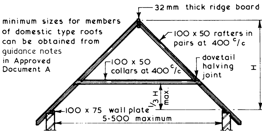
COLLAR ROOF
