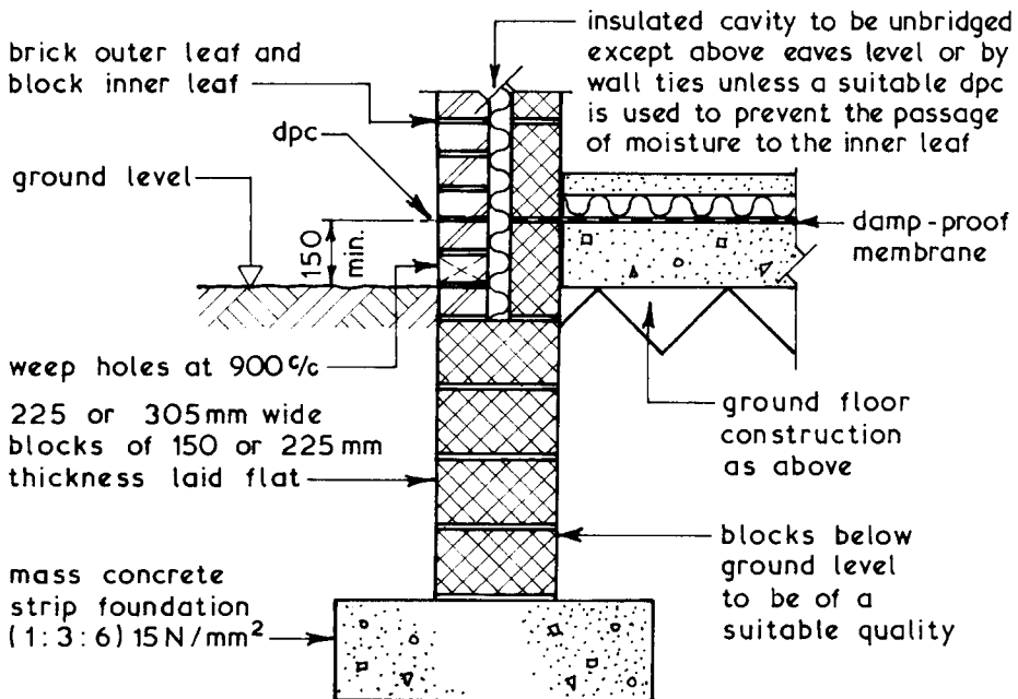
ALTERNATIVE CONSTRUCTION
