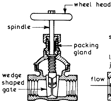
GATE VALVE
