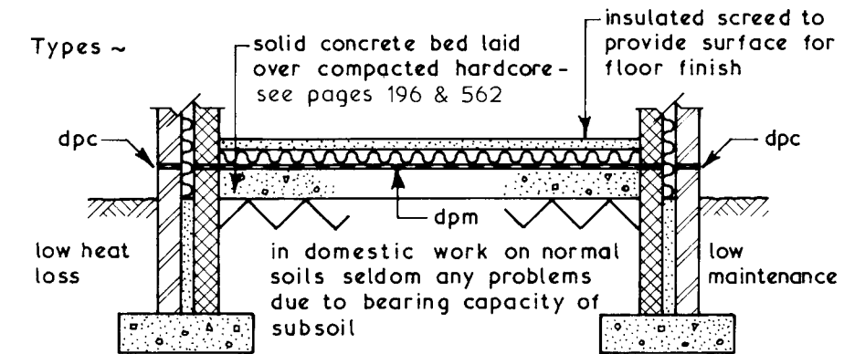
SOLID FLOOR ON LEVEL SITE
