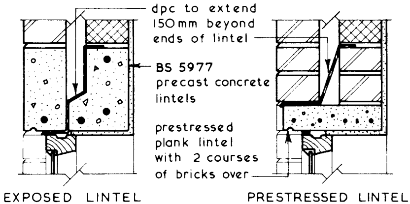
EXPOSED LINTEL
