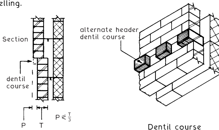
Dentil course
