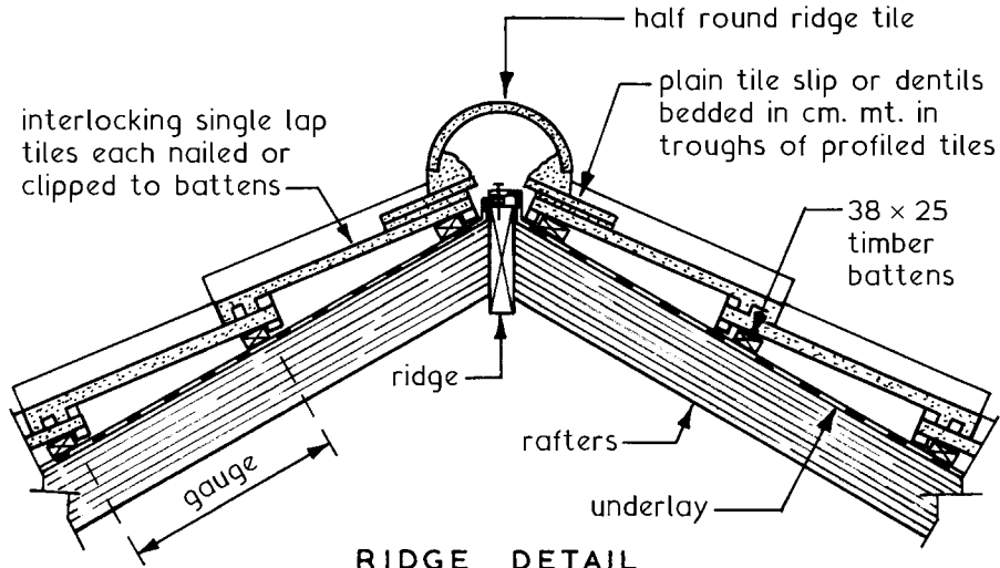
RIDGE DETAIL
