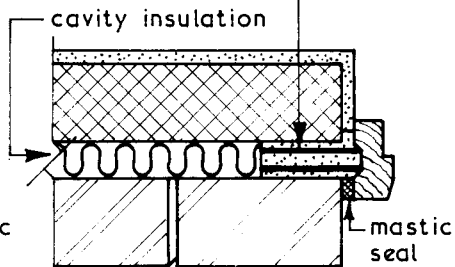
CAVITY WALL 1
