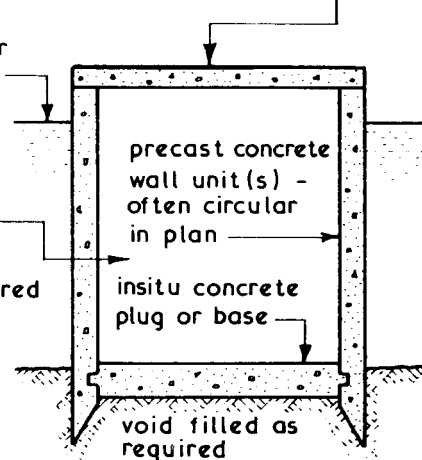
OPEN CAISSON
