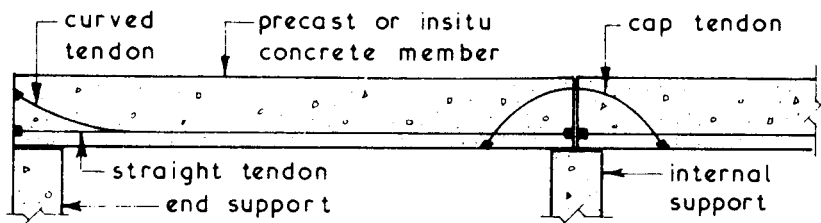
Curved Tendons for Negative Bending Moments~
