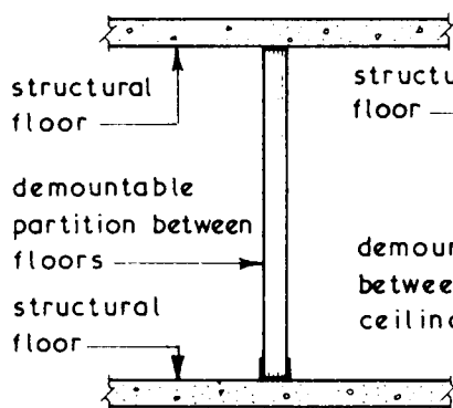
METHOD 1 - easily demounted and re-erected, good sound insulation can be achieved.
