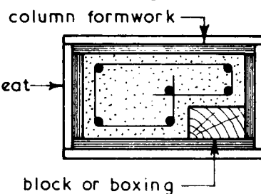
REBATED COLUMN
