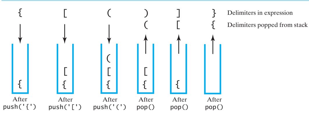
FIGURE 5-3 The contents of a stack during the scan of an expression that contains the balanced delimiters { [ ( ) ] }
