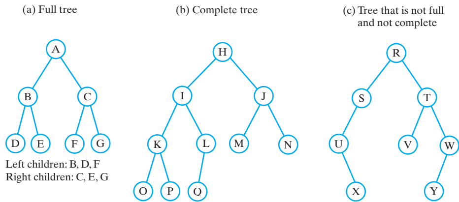
FIGURE 23-6 Three binary trees
