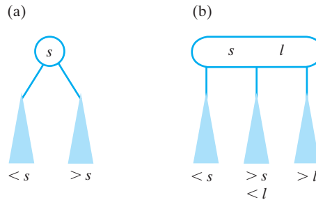
FIGURE 27-11 (a) A 2-node; (b) a 3-node
