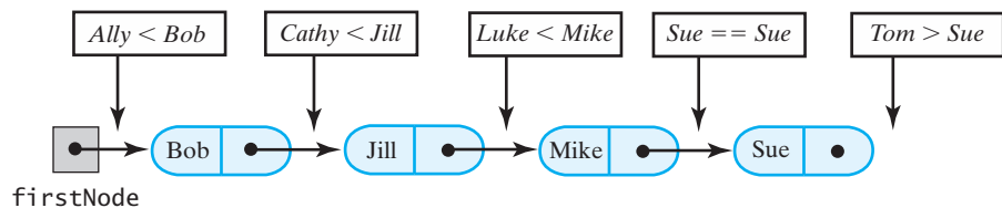
FIGURE 16-1 Places to insert names into a sorted chain of linked nodes
