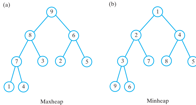
FIGURE 23-20 (a) A maxheap and (b) a minheap that contain the same values
