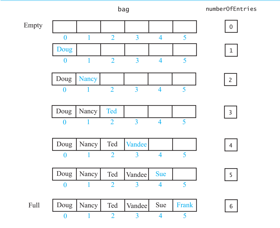
FIGURE 2-3 Adding entries to an array that represents a bag, whose capacity is six, until it becomes full
