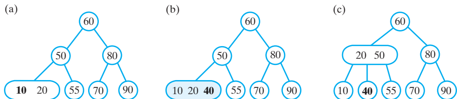
FIGURE 27-16 The 2-3 tree after adding (a) 10; (b), (c) 40
