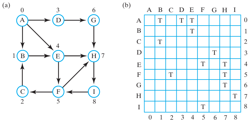
FIGURE 29-1 (a) An unweighted, directed graph and (b) its adjacency matrix
