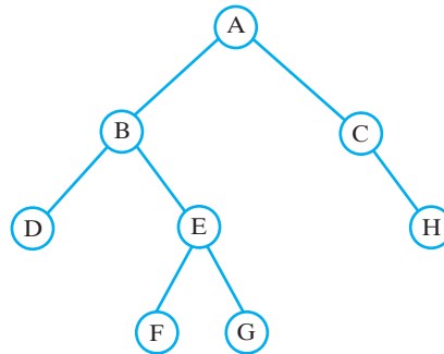
FIGURE 23-13 A binary tree whose nodes contain one-letter strings
