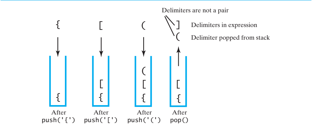
FIGURE 5-4 The contents of a stack during the scan of an expression that contains the unbalanced delimiters { [ ( ) }
