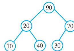
(e) During reheap(1)
