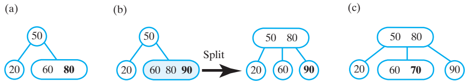
FIGURE 27-14 The 2-3 tree after adding (a) 80; (b) 90; (c) 70
