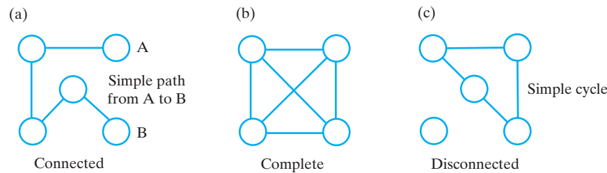
FIGURE 28-4 Undirected graphs
