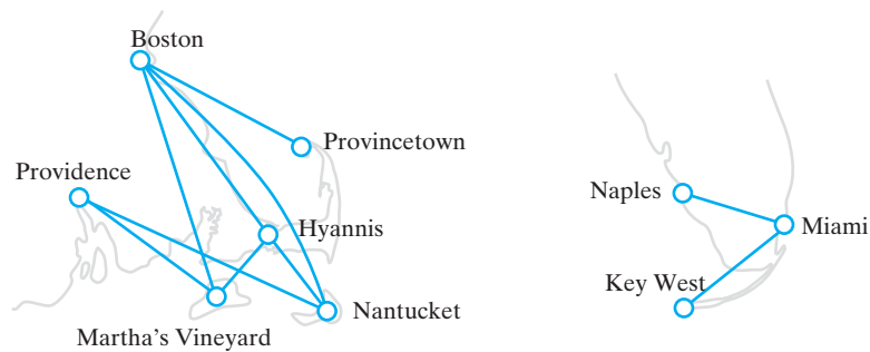
FIGURE 28-6 Airline routes
