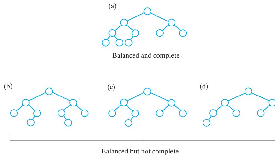
FIGURE 25-14 Some binary trees that are height balanced
