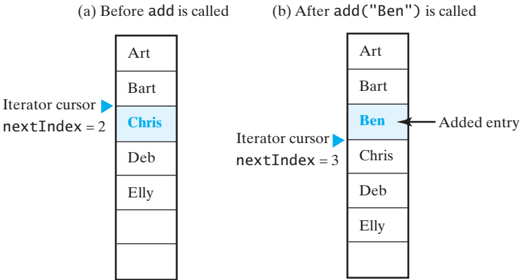
FIGURE 15-12 The array of list entries and nextIndex (a) just before the call to add; (b) just after the call to add
