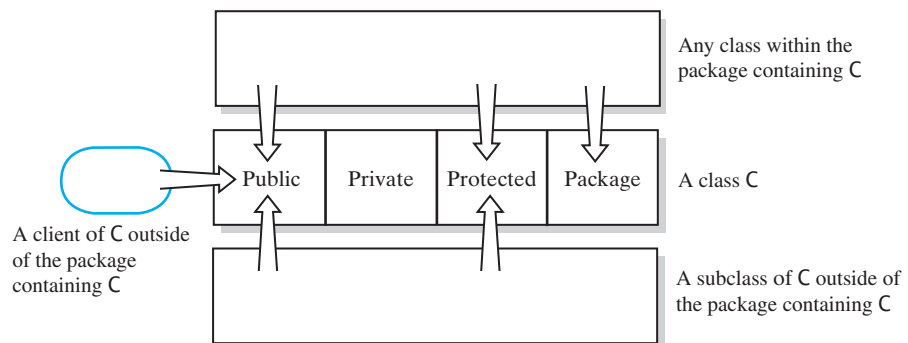
FIGURE C-4 Public, private, protected, and package access of the data fields and methods of class C
