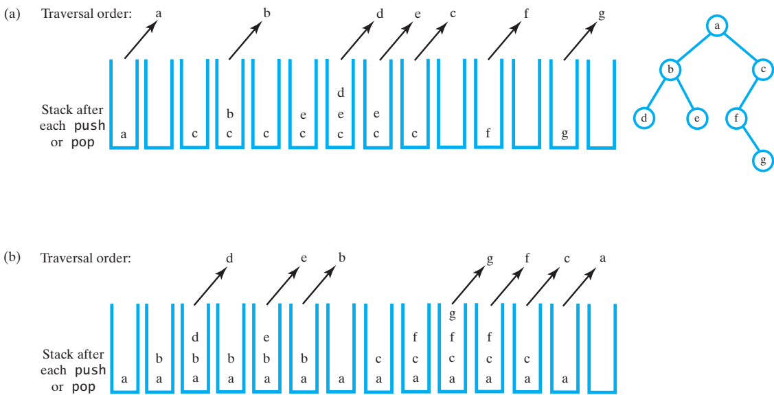
FIGURE 24-6 Using a stack to traverse a binary tree in (a) preorder; (b) postorder
