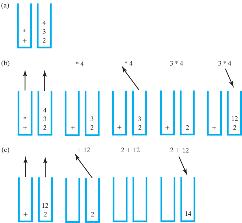
FIGURE 5-12 Two stacks during the evaluation of a + b * c when a is 2, b is 3, and c is 4: (a) after reaching the end of the expression; (b) while performing the multiplication; (c) while performing the addition
