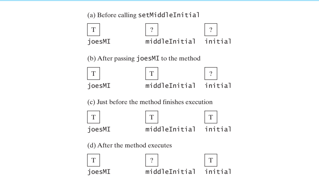
FIGURE B-4 The effect of executing the method setMiddleInitial on its argument joesMI , its parameter middleInitial , and the data field initial
