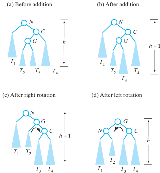
FIGURE 27-7 Before and after an addition to an AVL subtree that requires both a right rotation and a left rotation to maintain its balance
