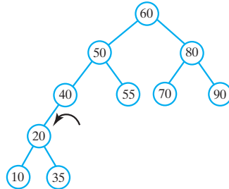
(c) After left rotation about 40
