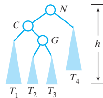
(a) Before addition
