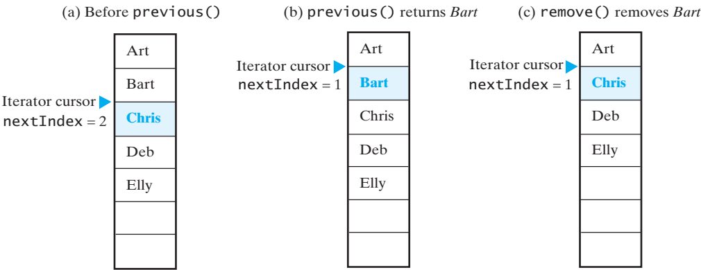
FIGURE 15-13 The array of list entries and nextIndex (a) just before the call to previous; (b) just after the call to previous but before the call to remove; (c) after the call to remove
