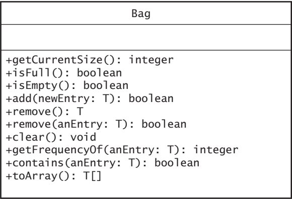
FIGURE 1-2 UML notation for the class Bag
