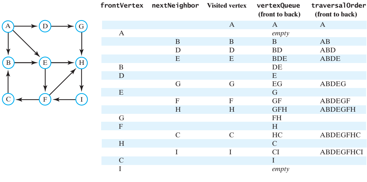
FIGURE 28-10 A trace of a breadth-first traversal beginning at vertex A of a directed graph
