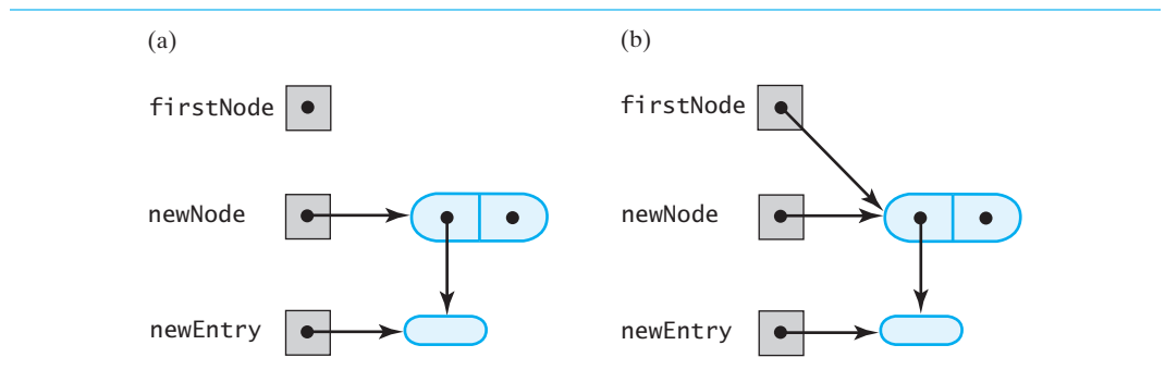
FIGURE 3-6 (a) An empty chain and a new node; (b) after adding a new node to a chain that was empty
