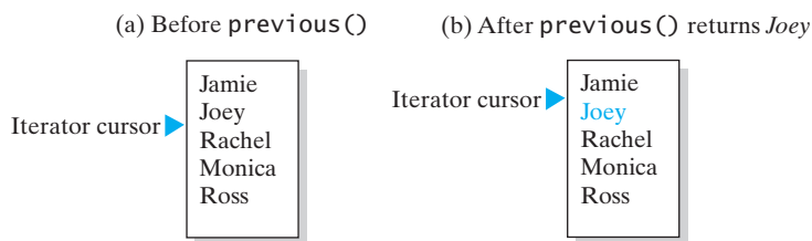
FIGURE 15-9 The effect of a call to previous on a list
