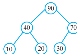
(f) After reheap(1)
