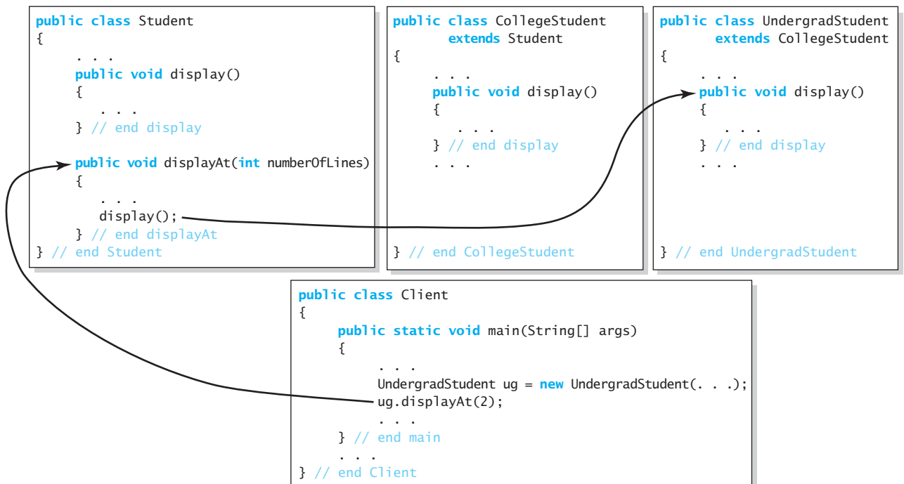
FIGURE C-6 The method displayAt calls the correct version of display
