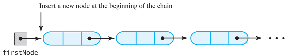
FIGURE 20-7 Adding to an unsorted linked dictionary
