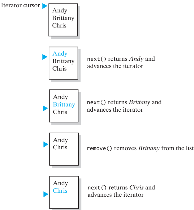
FIGURE 15-3 The effect of the iterator methods next and remove on a list
