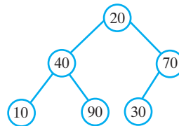
(c) After reheap(3)
