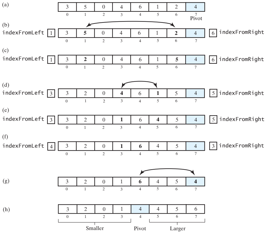
FIGURE 9-6 A partitioning strategy for quick sort
