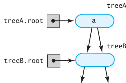
FIGURE 24-3 treeA has identical subtrees
