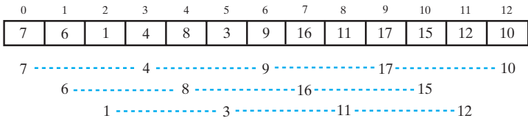
FIGURE 8-14 The subarrays of the array in Figure 8-13 formed by grouping entries whose indices are 3 apart
