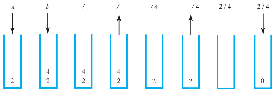
FIGURE 5-10 The stack during the evaluation of the postfix expression a\ b\ /\ when a is 2 and b is 4
