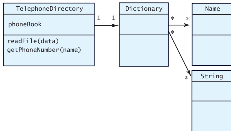
FIGURE 19-4 A class diagram for a telephone directory
