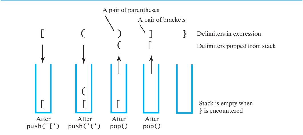
FIGURE 5-5 The contents of a stack during the scan of an expression that contains the unbalanced delimiters [ ( ) }
