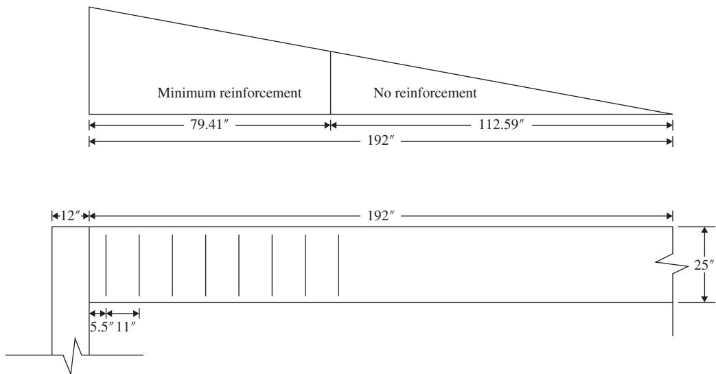
Figure 23.14 Bar distribution for shear reinforcement.
