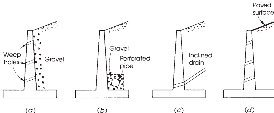
Figure 14.9 Drainage systems.
