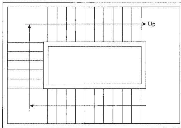
Three-stair flight
