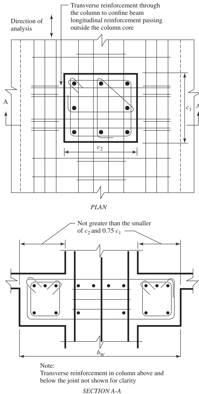
Figure 20.11 Maximum effective width of wide beam and required transverse reinforcement. Courtesy of American Concrete Institute [1]
