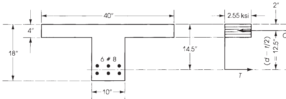
Figure 4.7 Example 4.7: T-section.
