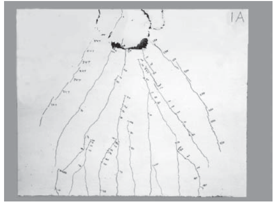
Deep-beam flexural-shear failure.
