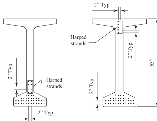
Figure 22.15 Strand pattern.
