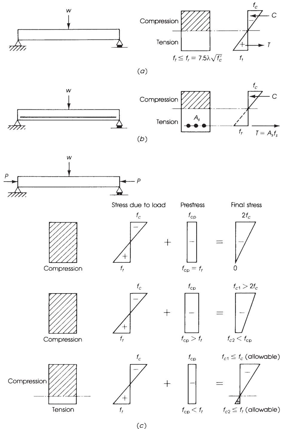
Figure 19.1 Effect of prestressing: (a) plain concrete, (b) reinforced concrete, and (c) prestressed concrete.
