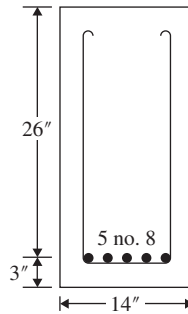
Figure 23.2 Detail of the beam.
