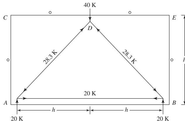
Figure 8.4 Example of steel truss.
