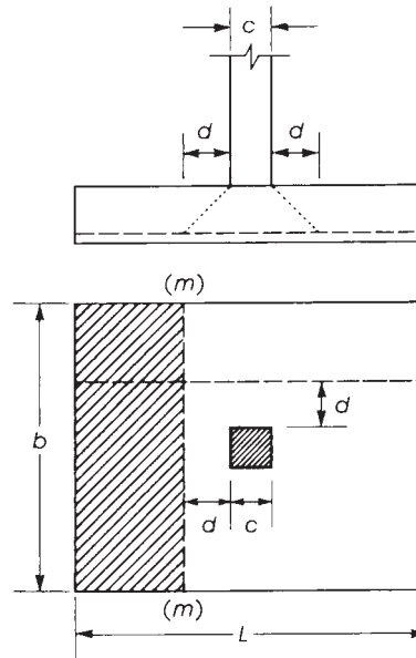
Figure 13.11 One-way shear.
