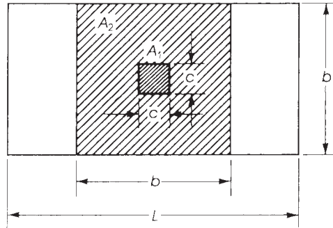
Figure 13.15 Bearing areas on footings. A_1 = c^2 , A_2 = b^2 .
