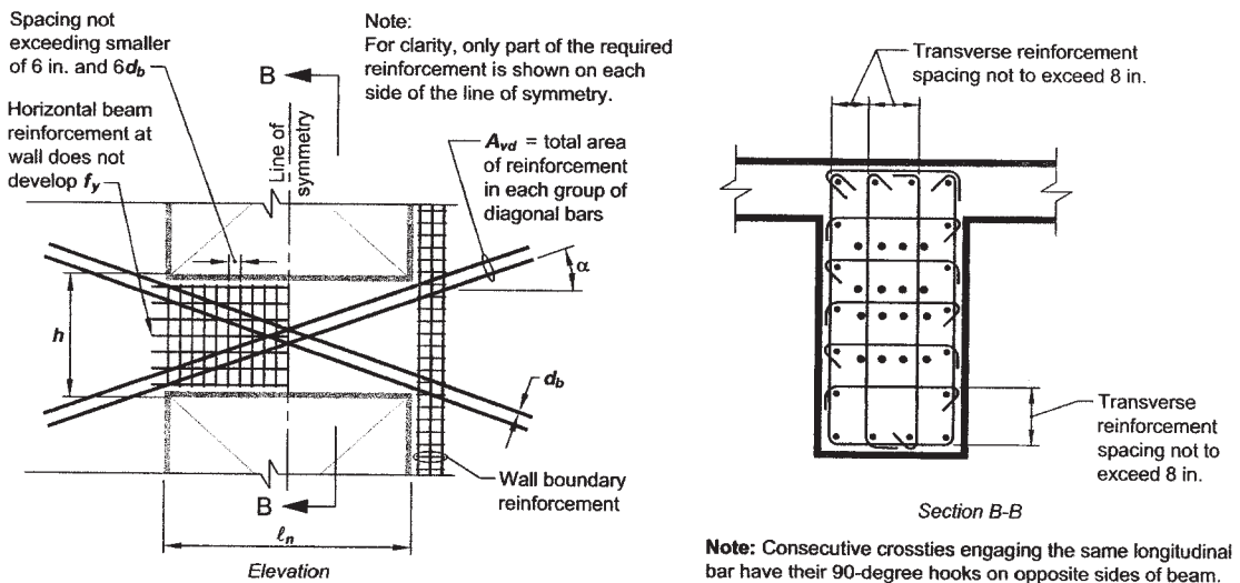
Figure 20.33 Reinforced detailing for coupling beams with diagonally oriented reinforcement. Wall boundary reinforcement is shown on one side only for clarity. Courtesy of American Concrete Institute [1]
