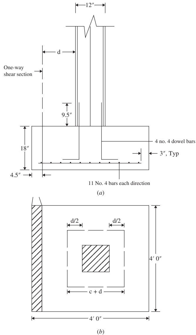
Figure 23.16 Footing details
