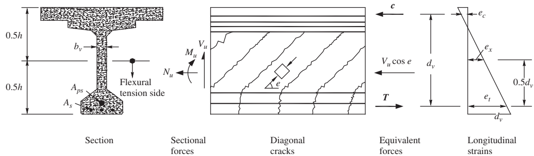
Figure 22.9 Illustration of shear parameters for section containing at least the minimum amount of transverse reinforcement, V_p = 0 . AASHTO LRFD Bridge Design Specifications , 2014. Used by permission
