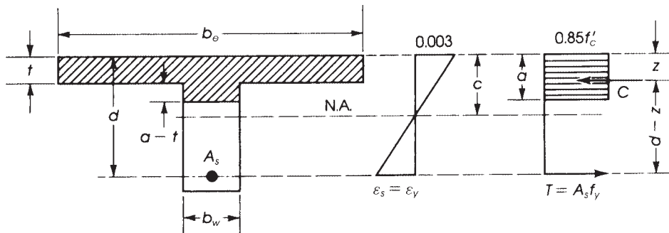
Figure 3.31 T-section behavior.
