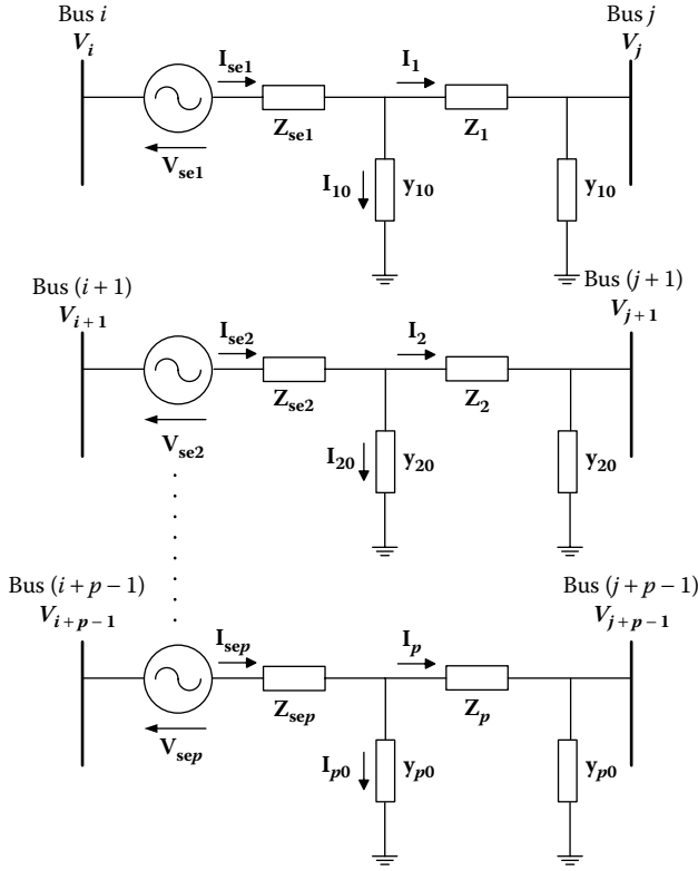
FIGURE 5.2 Equivalent circuit of IPFC-incorporated power system network.
