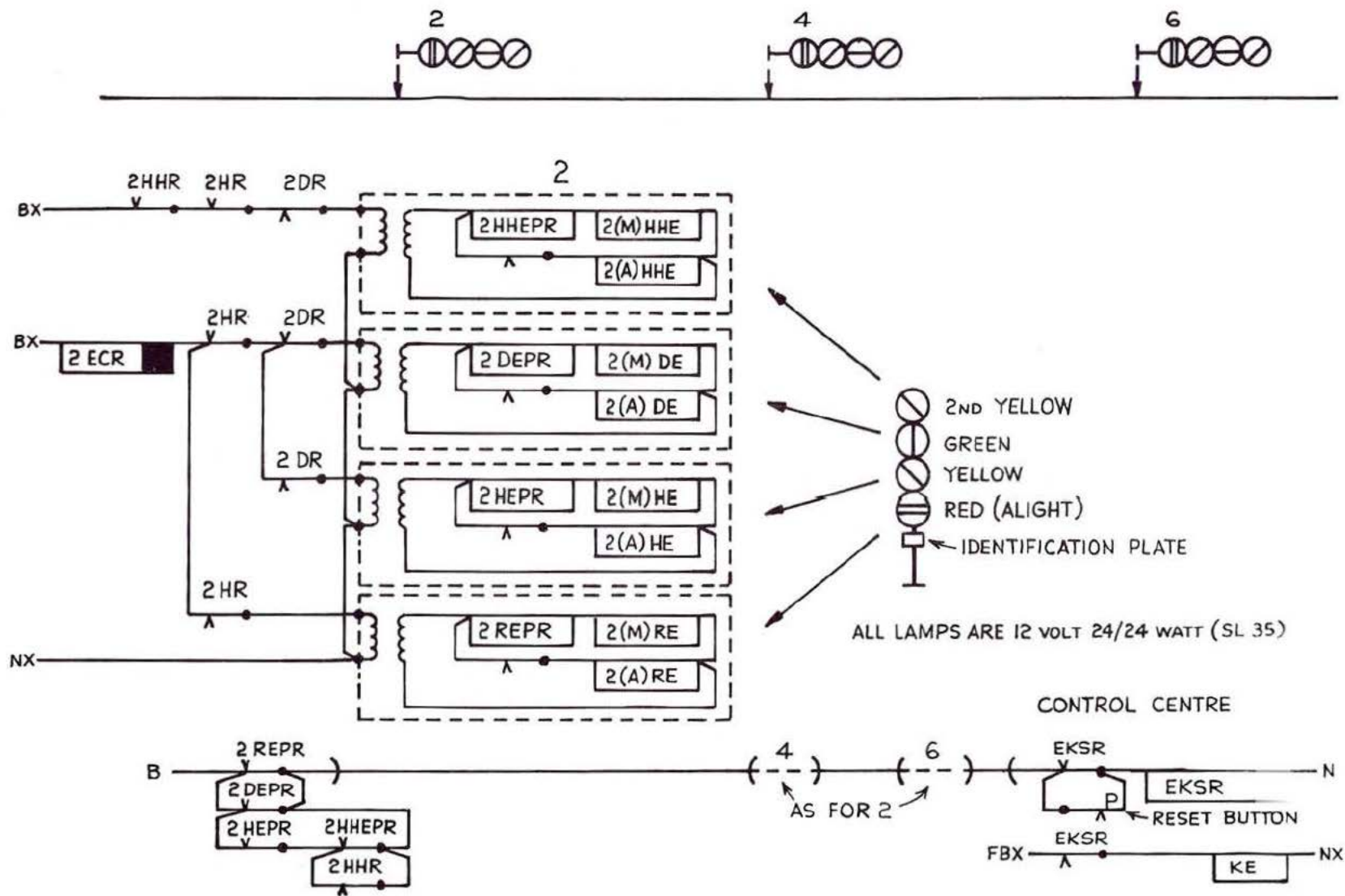
Fig. 4:4 4-aspect multi-unit signal: lighting and main filament lamp indication circuit
