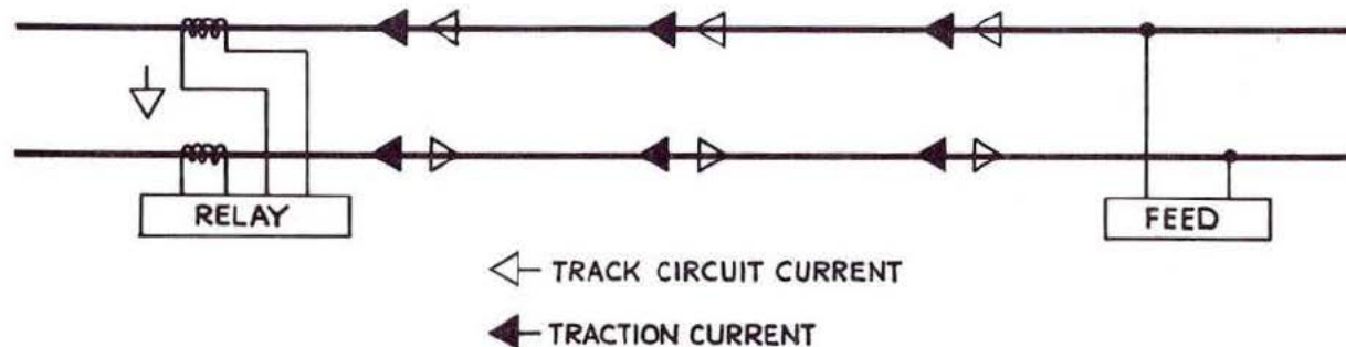
Fig. 7:26 Alsthom current-operated jointless track circuit
