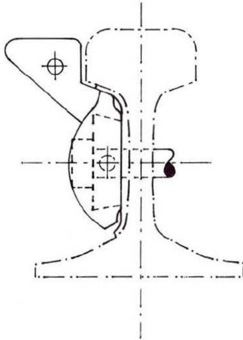
Fig. 7:7 Track circuit interrupter assembly
