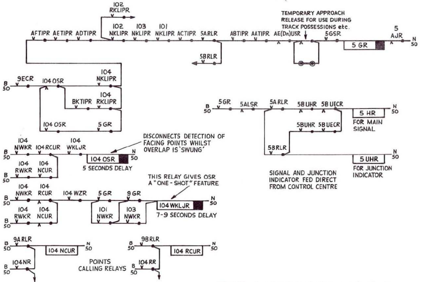
Fig. 4:32 Aspect control and swinging overlap circuits
