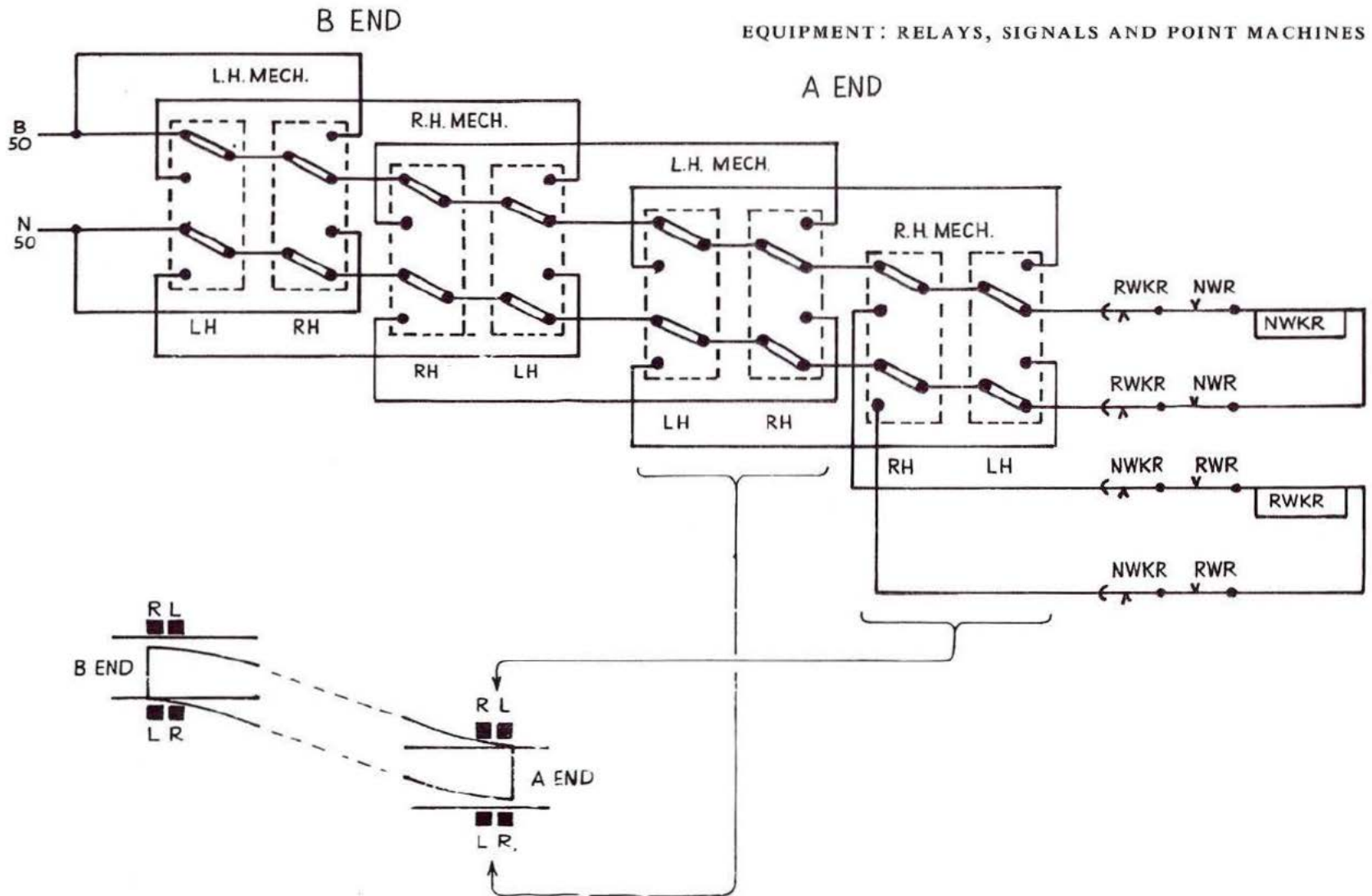
Fig. 4:23 Electro-hydraulic point machine (clamp lock type): detection circuit
