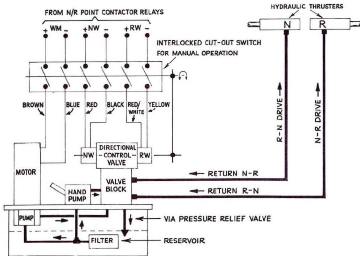
Fig. 4:24 Electro-hydraulic point machine (clamp lock type): hydraulic operation
