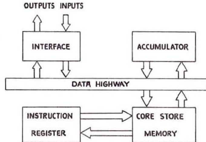
Fig. 9:19 Main components of the computer
