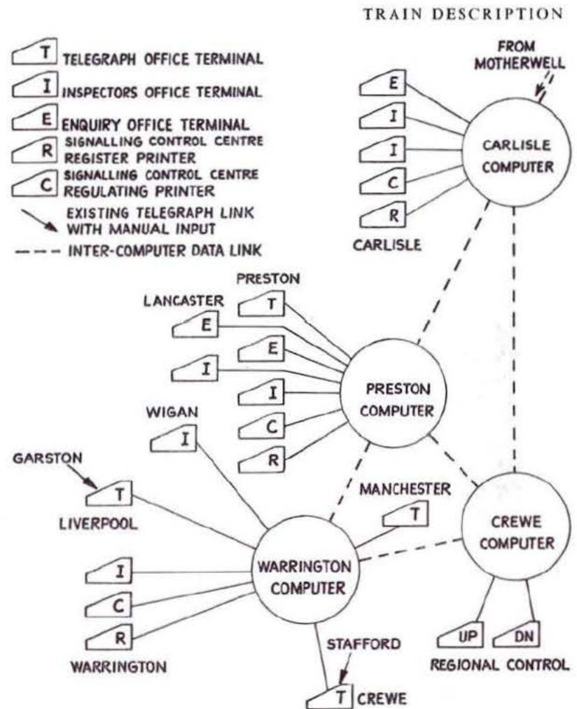
Fig. 9:25 Train reporting system as installed on British Railways (L.M. Region)
