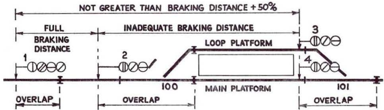
Fig. 2:12 Signalling at an intermediate station with loop platform
