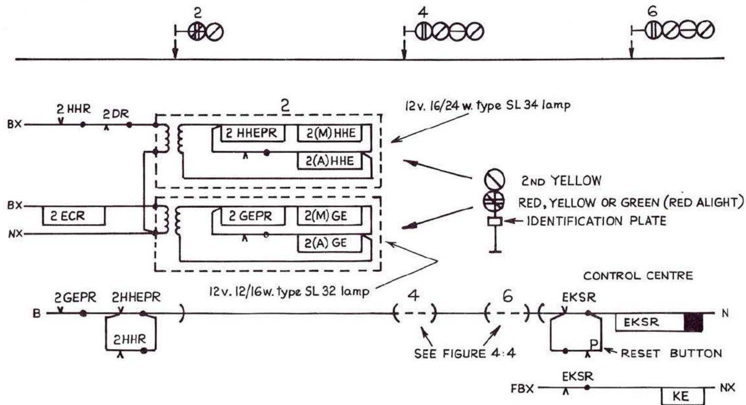
Fig. 4:7 4-aspect searchlight signal: lighting and main filament lamp indication circuit
