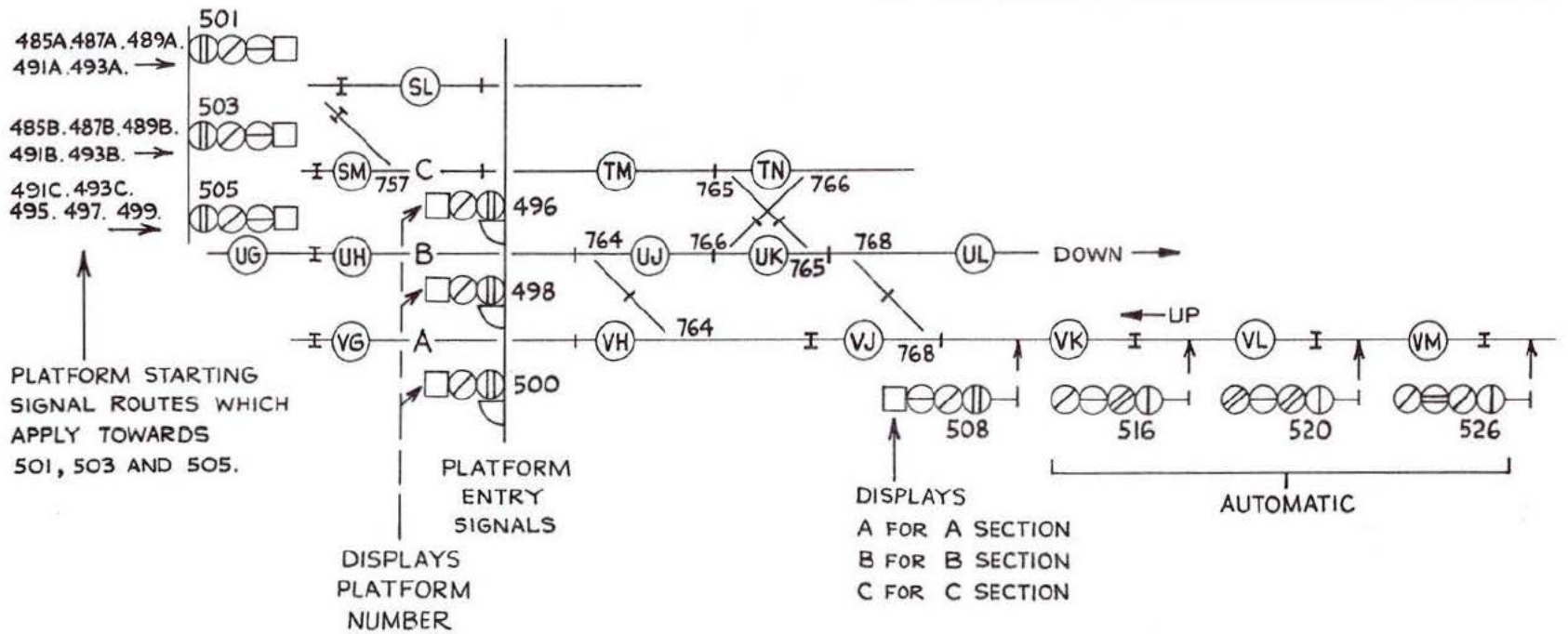
Fig. 3:13 Layout relating to examples of control tables
