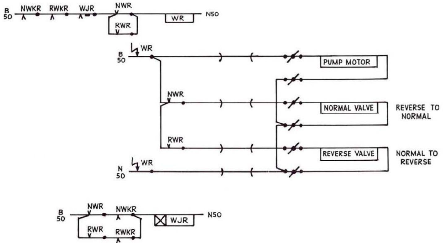
Fig. 4:22 Electro-hydraulic point machine (clamp lock type): control and drive circuit
