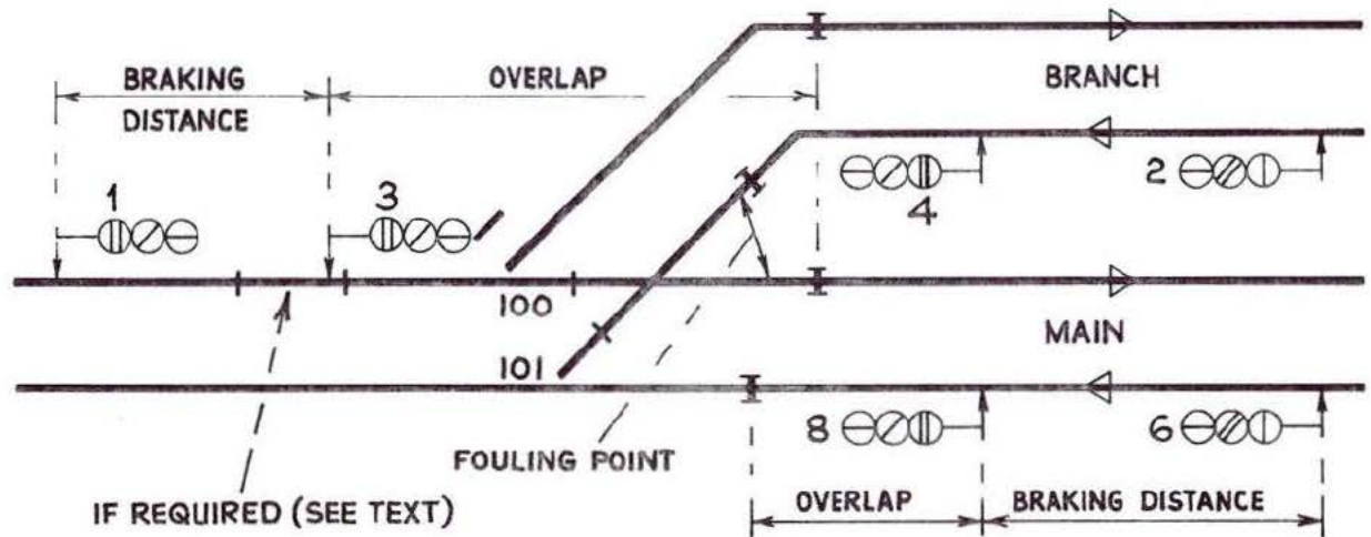
Fig. 2:14 Layout of signals at a double junction
