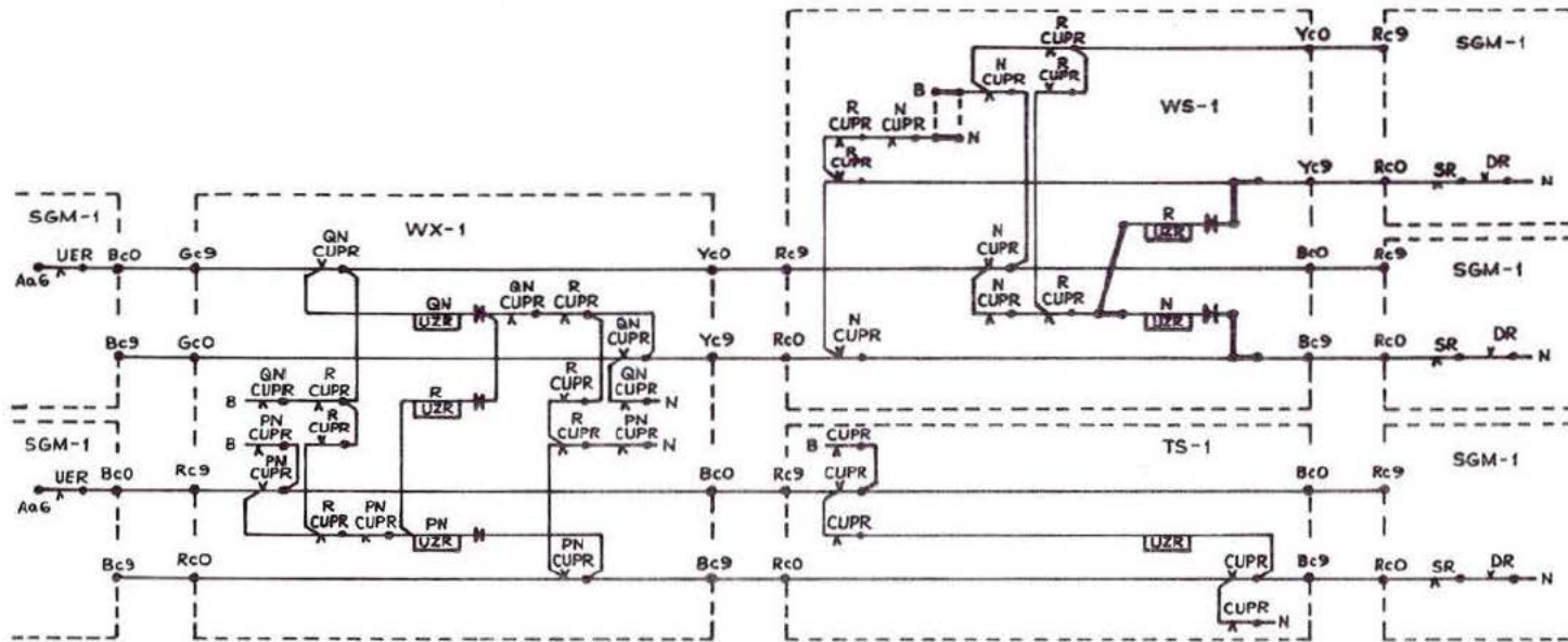
Fig. 6:17 System B: route priming: circuit operation
