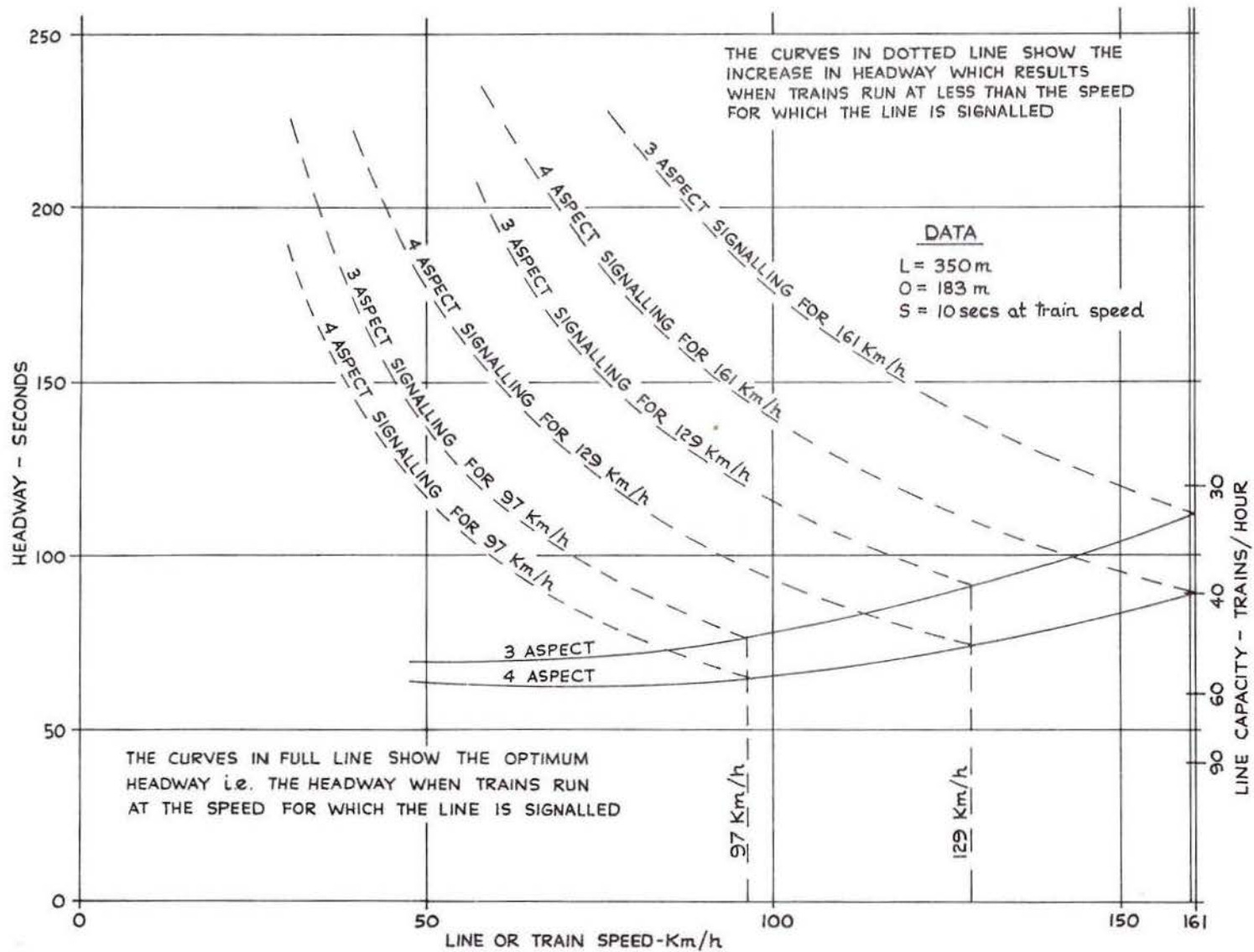
Fig. 2:6 Optimum headway and line capacity and effect of running at a speed less than that for which the line is signalled
