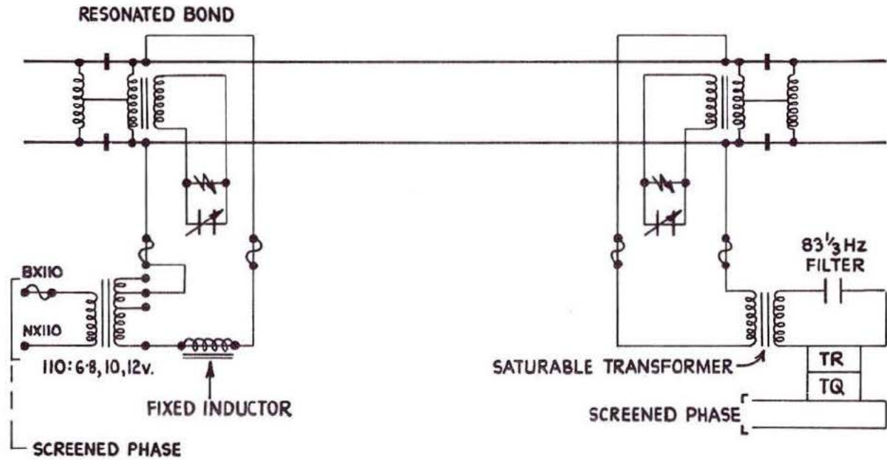
Fig. 7:19 Double rail AC track circuit with inductance feed
