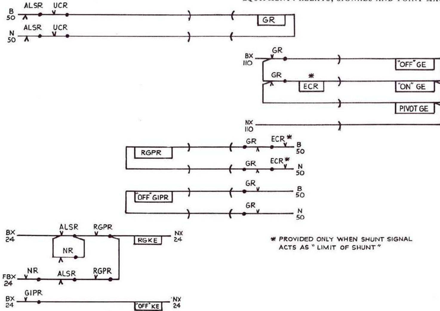
Fig. 4:12 Shunting signal: control, lighting and indication circuit
