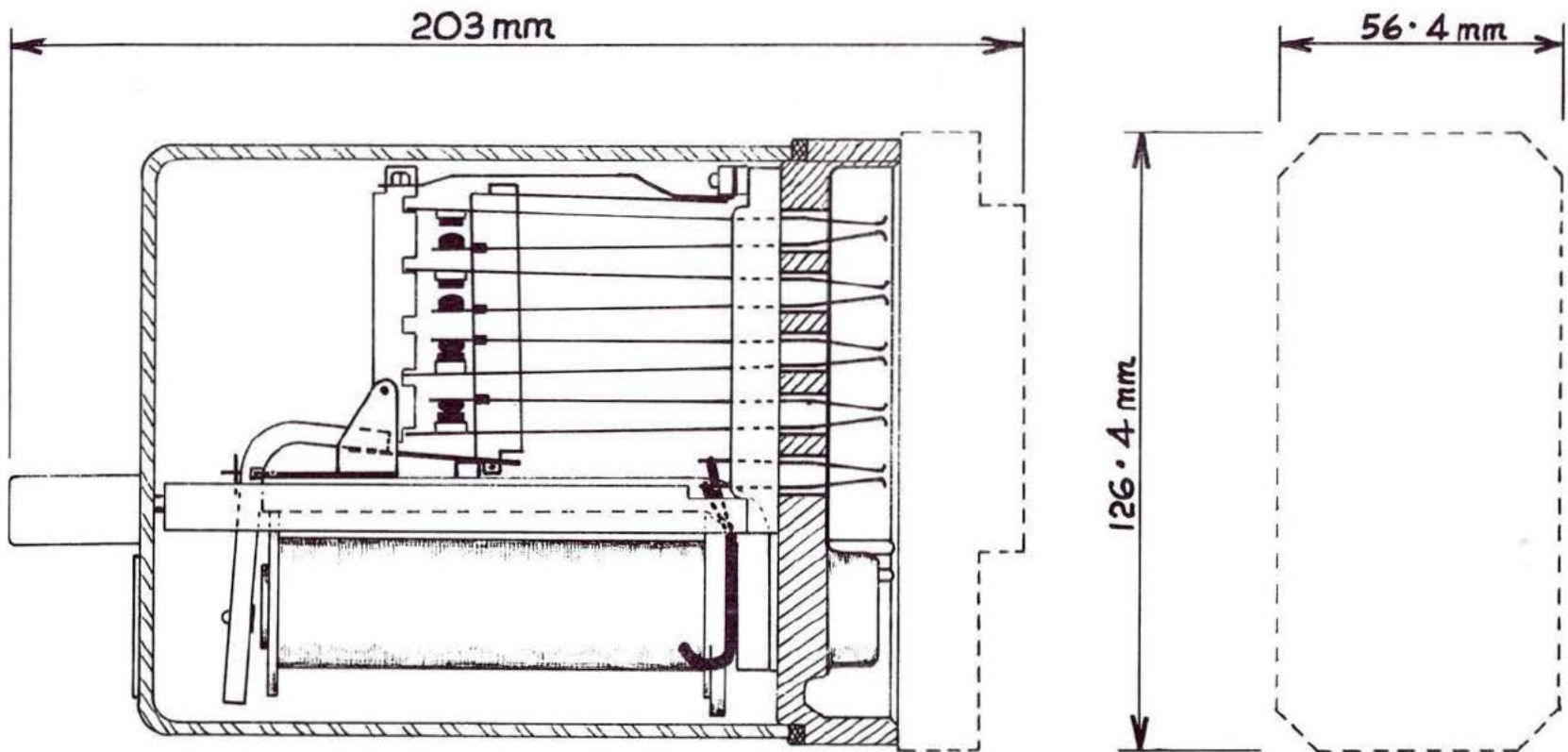
Fig. 4:1 BR 930 series relay
