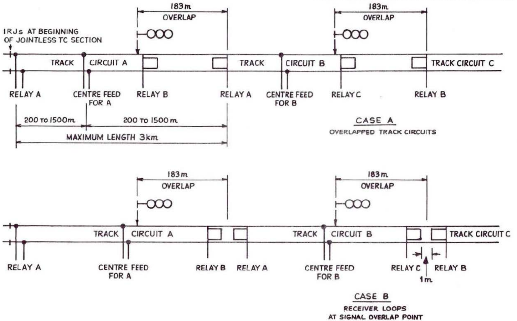
Fig. 7:27 Reed jointless track circuit: typical applications
