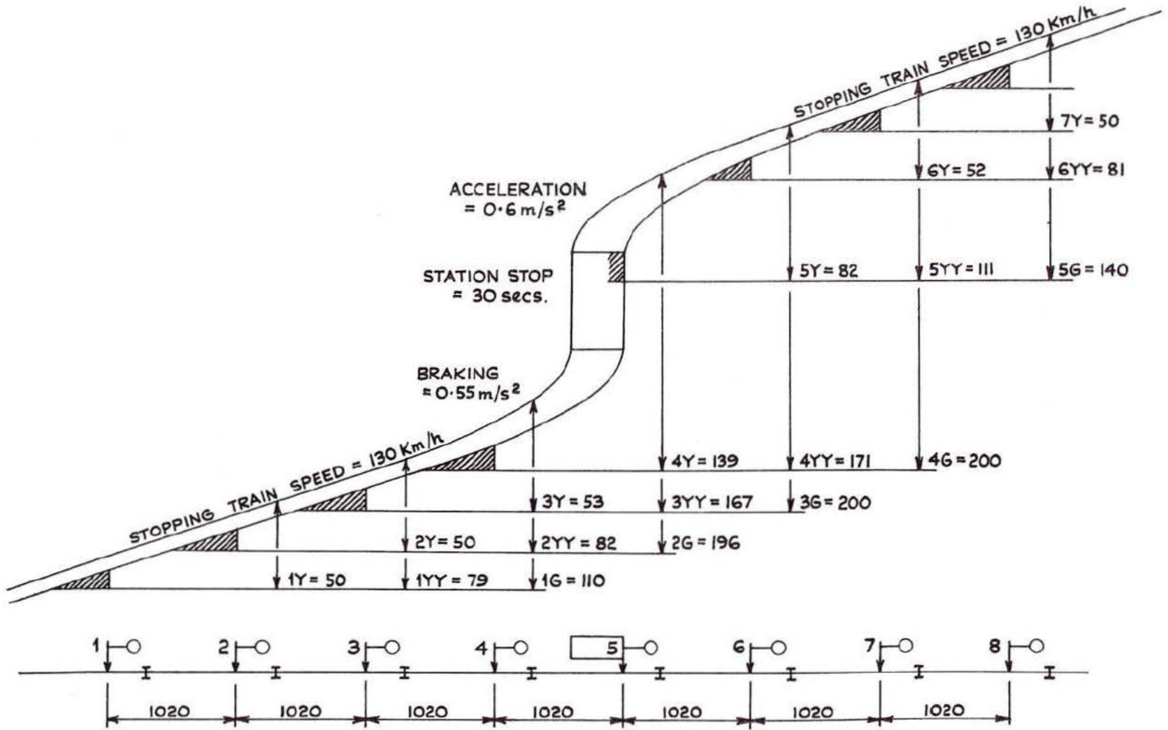
Fig. 2:10 4-aspect stopping train headway calculations for an intermediate station
