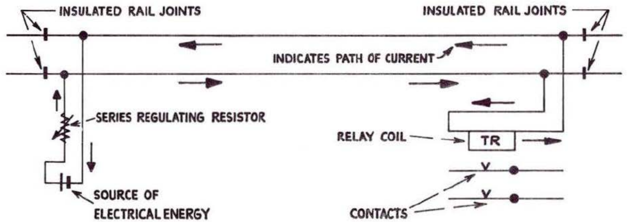
RELAY ENERGISED INDICATING TRACK CLEAR OF VEHICLES
