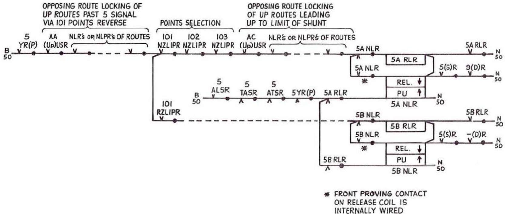
Fig. 4:28 Route LR circuits
