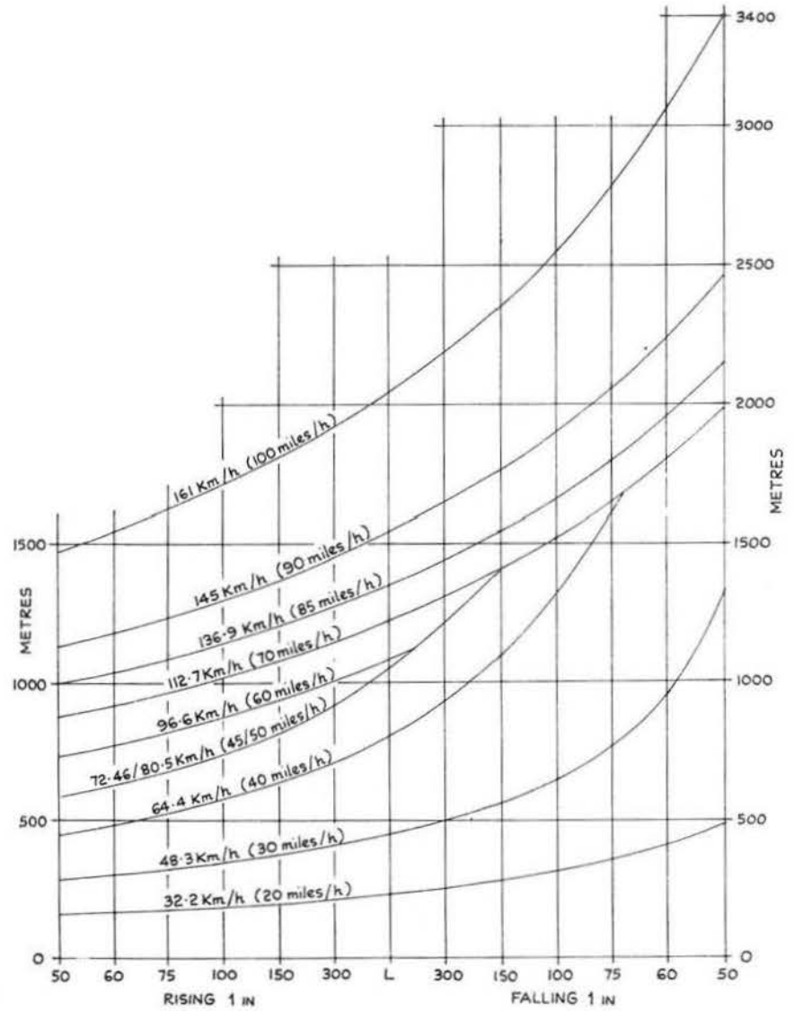
Fig. 2:5 British Railways' standard composite braking curve
