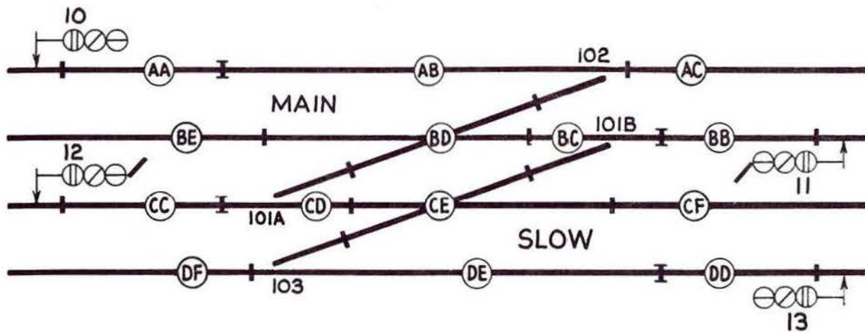
Fig. 3:4 Main signal and point controls at a left-hand running junction
