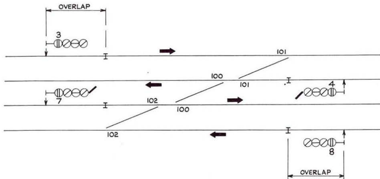
Fig. 2:16 Double running junctions on high speed lines
