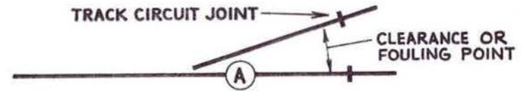
Fig. 2:17 Track circuiting at a divergence of two tracks
