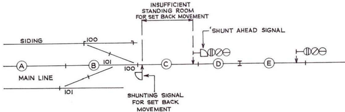
Fig. 2:23 Subsidiary signal as draw-ahead for setting back into siding
