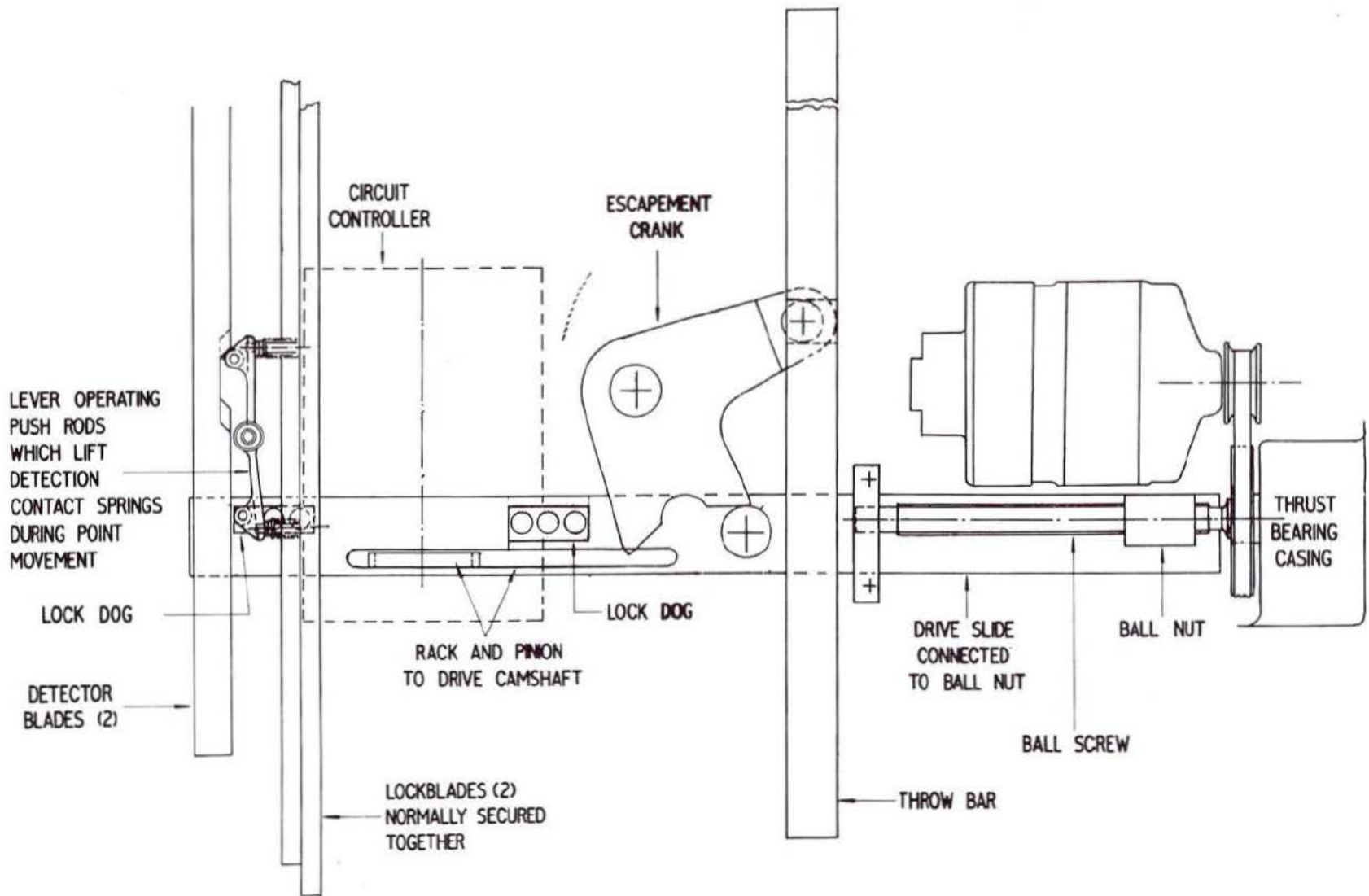
Fig. 4:14 Point machine drive and lock movement: 'straight through'
