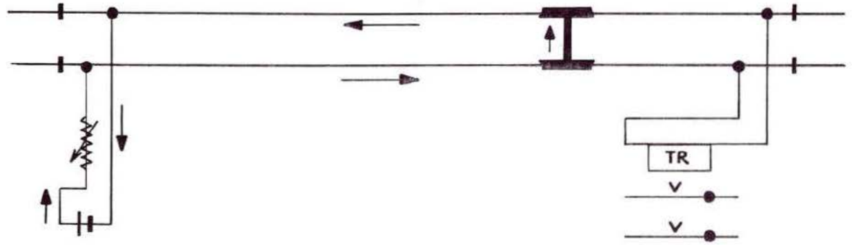
RELAY DE-ENERGISED (CONTACTS BROKEN) INDICATING PRESENCE OF VEHICLE
