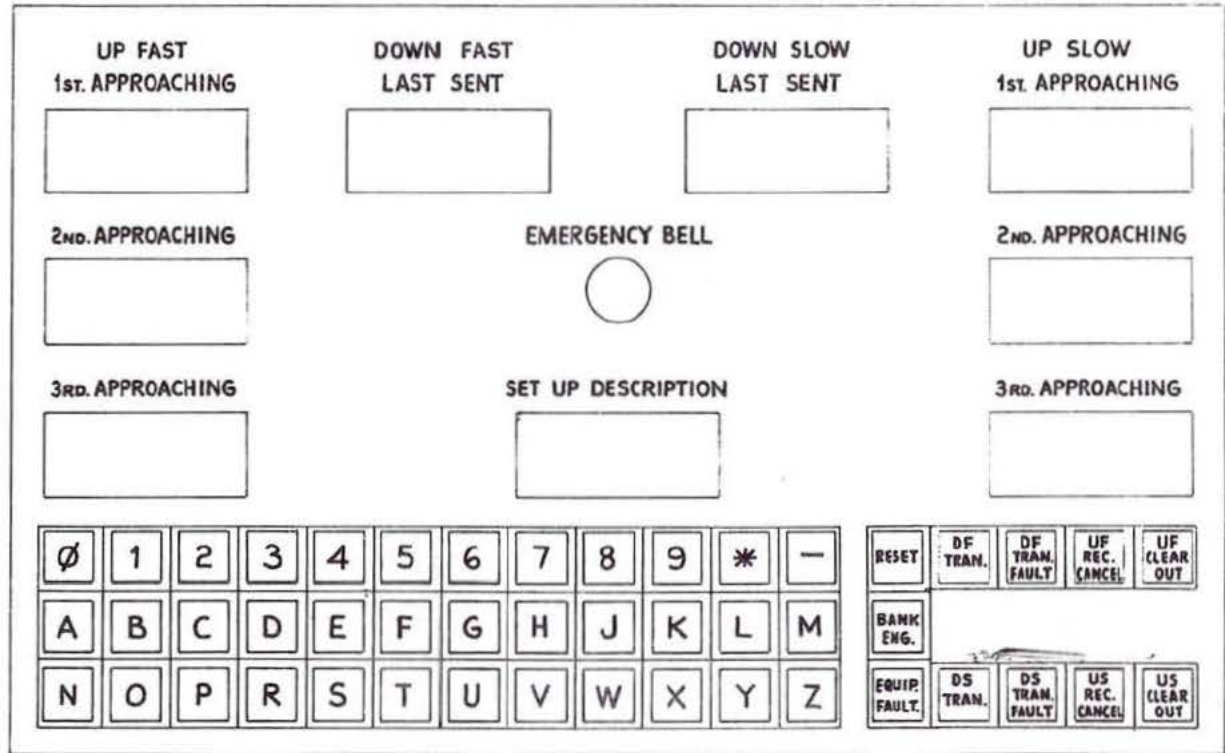
Fig. 9:13 Fringe box signalman's train description panel layout
