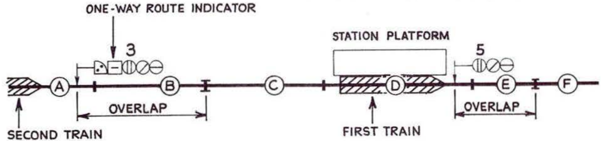
Fig. 2:22 Subsidiary signal at entrance to occupied platform (simple case)
