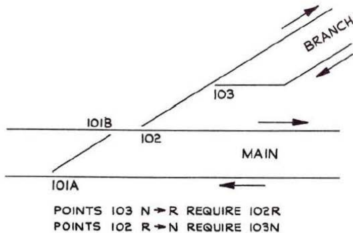
Fig. 3:9 Double junction on high speed line
