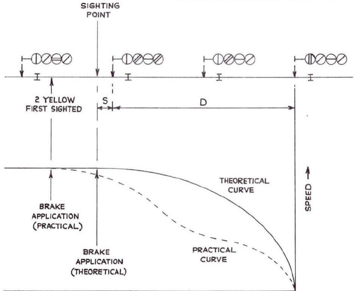
Fig. 2:7 Theoretical and practical braking technique
