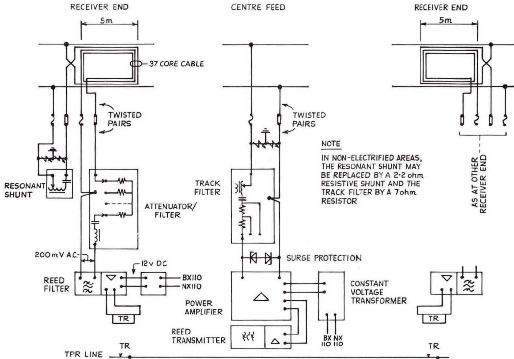
Fig. 7:28 Reed jointless track circuit: details
