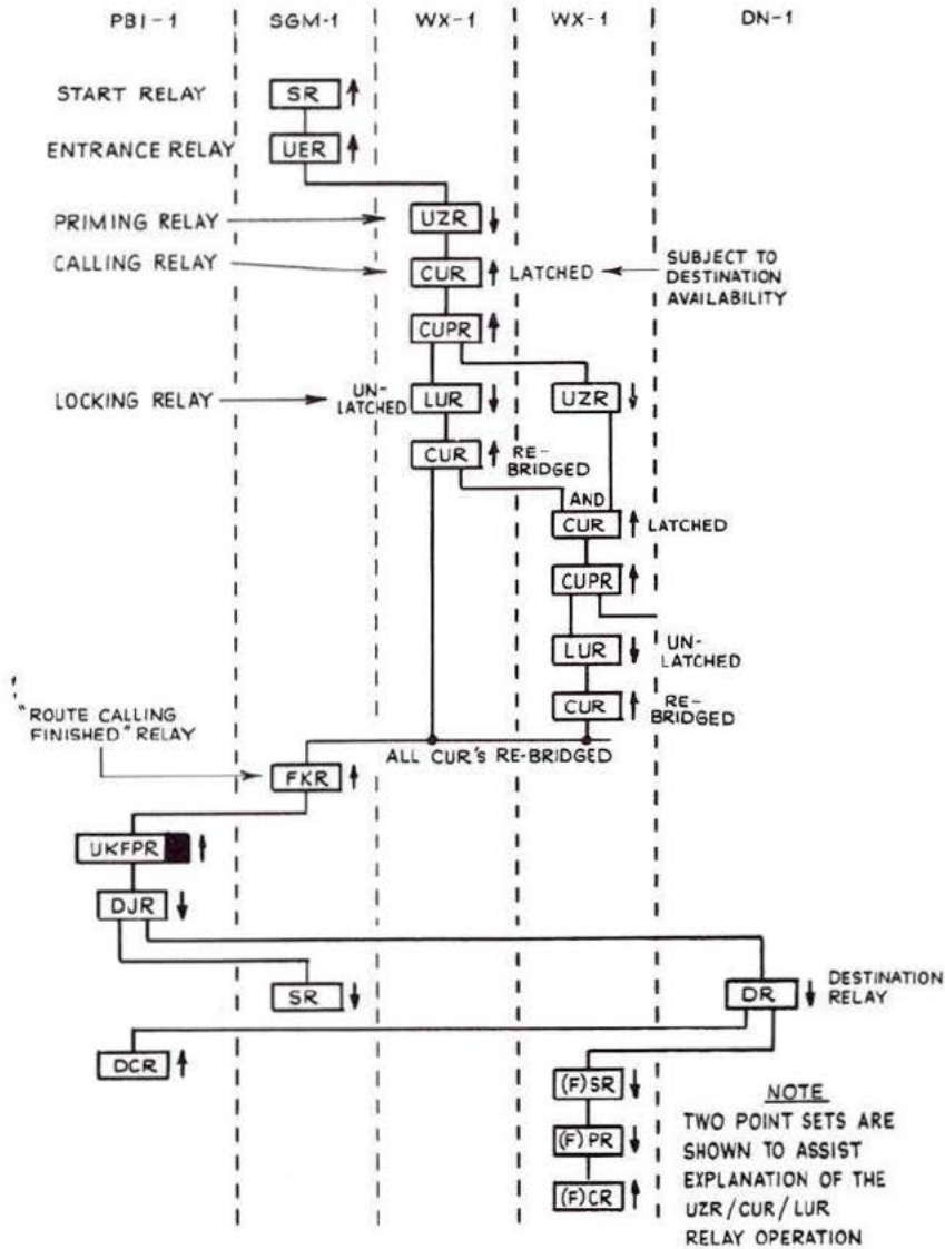
Fig. 6:16 System B: route priming calling and locking: relay operating sequence
