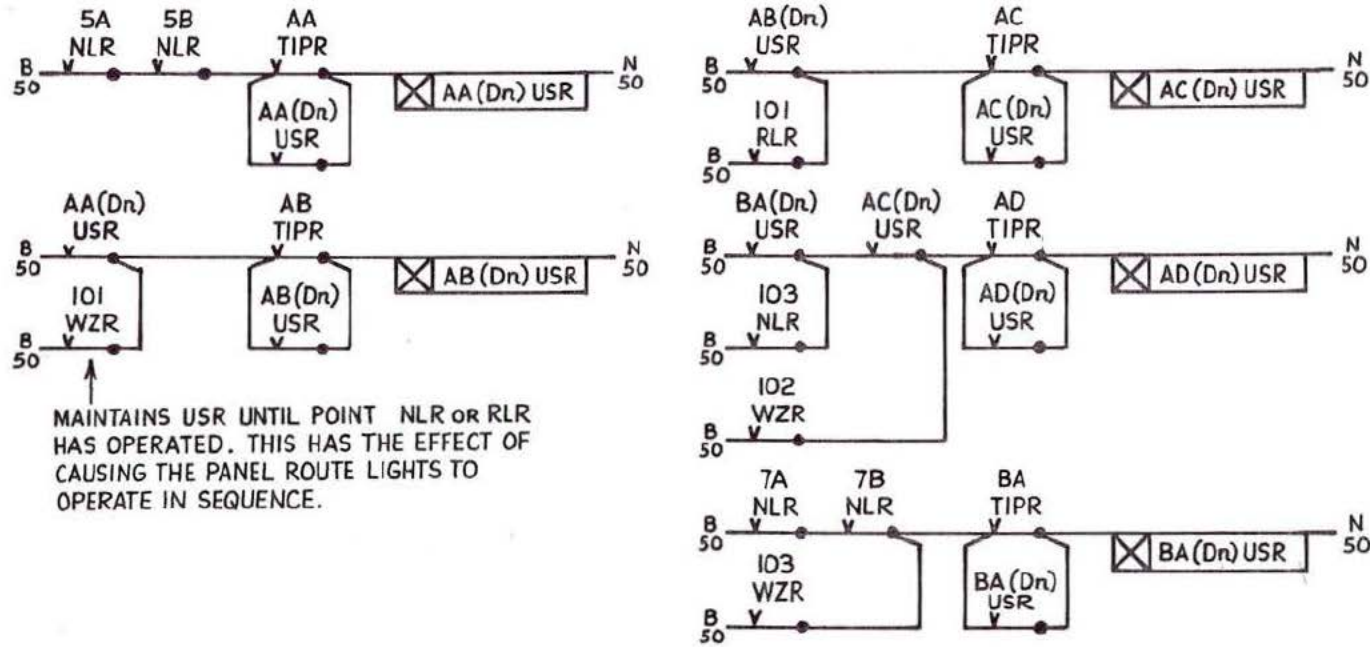
Fig. 4:30 Sectional release route locking circuits
