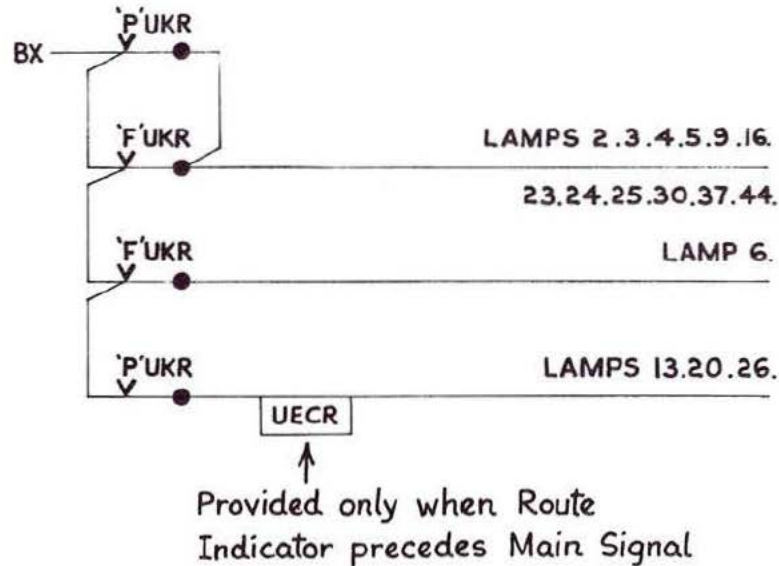
Fig. 4:10 Multi-lamp route indicator
