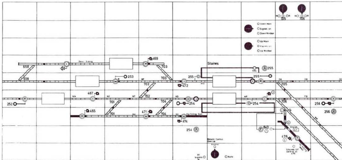
Fig. 5:1 Mosaic diagram: part of a control panel and including an interlocking that is remotely controlled
