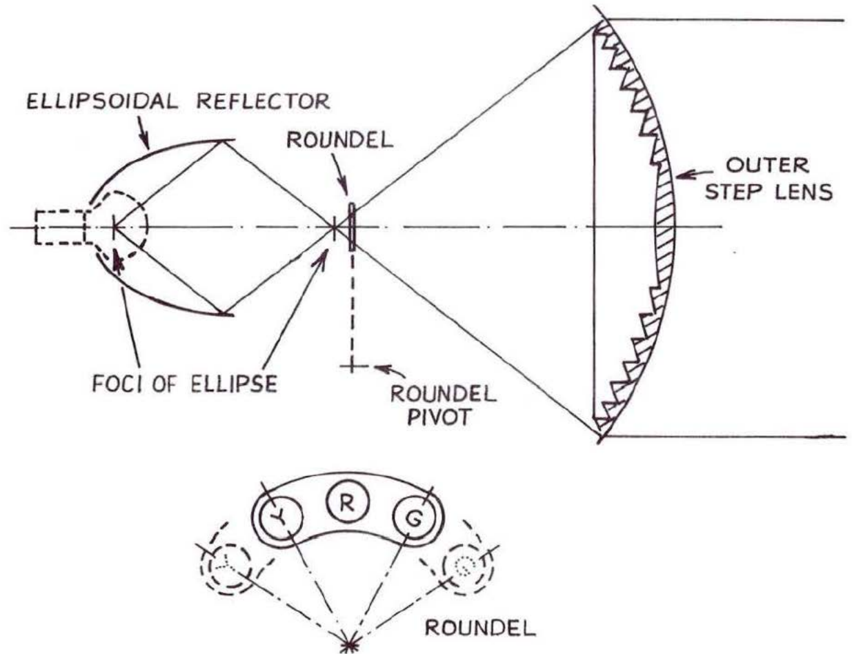
Fig. 4:6 Searchlight signal: optical system
