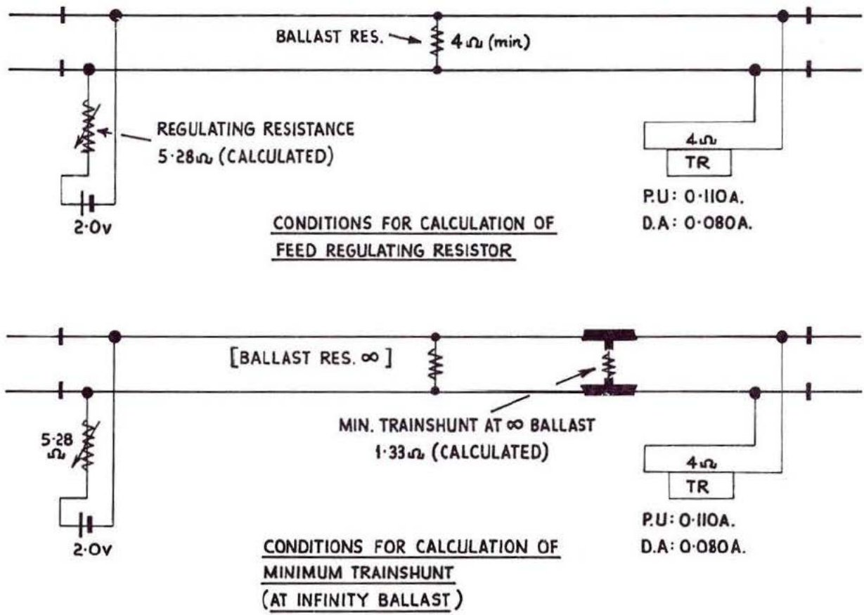
Fig. 7:3 Example of track circuit calculation
