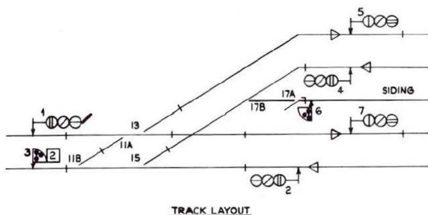
TRACK LAYOUT
