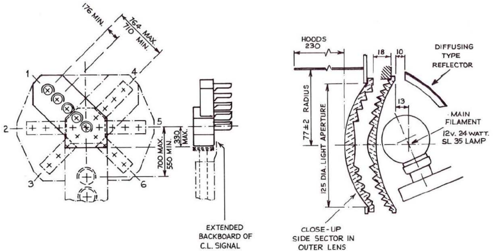
Fig. 4:8 Position light junction indicator and optical system
