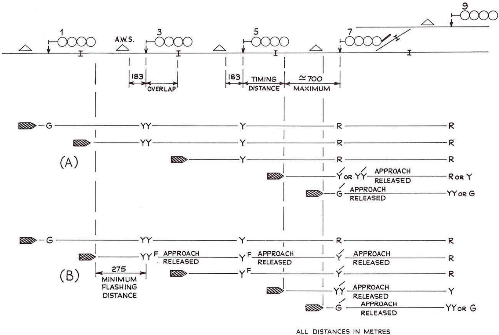
Fig. 2:27 4-aspect junction signalling
