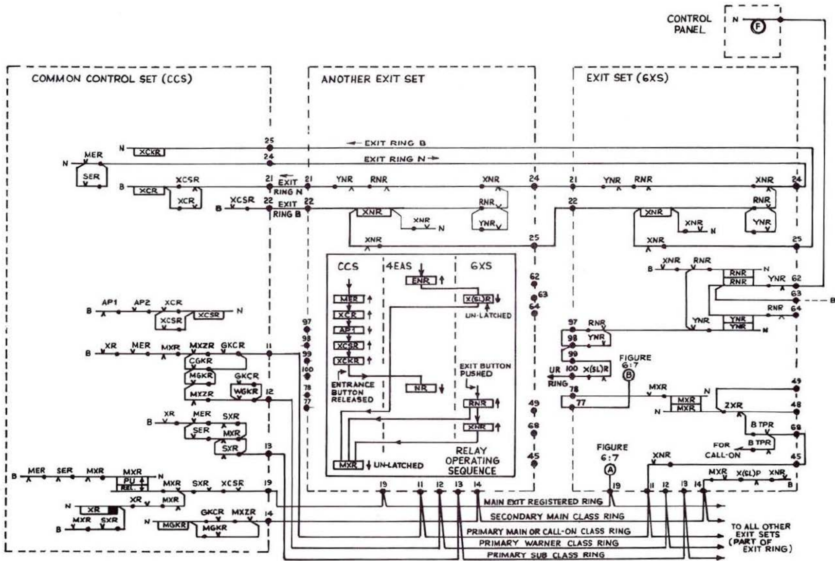
Fig. 6:6 System A: exit registration
