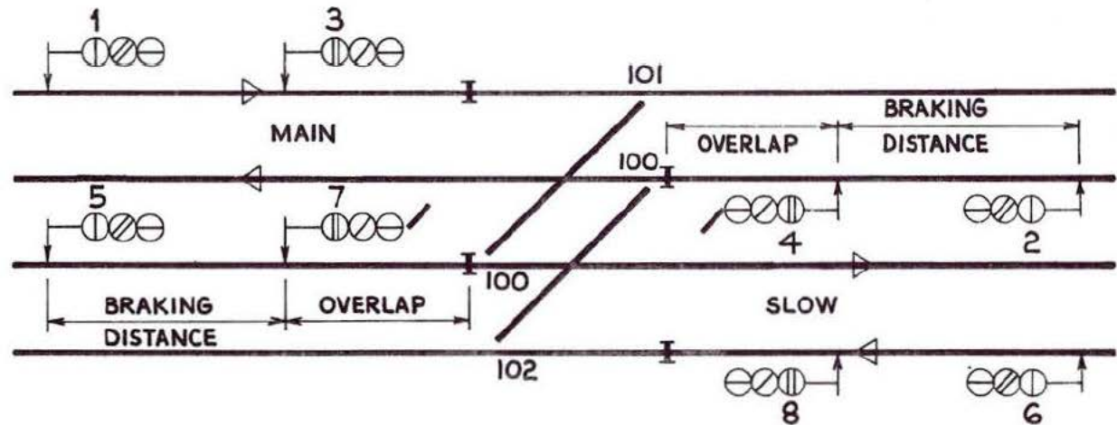
Fig. 2:15 Layout of signals at a left-hand double running junction
