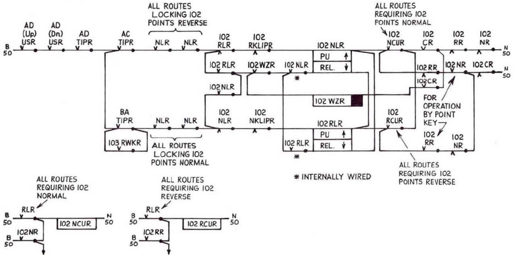
Fig. 4:29 Point setting circuits
