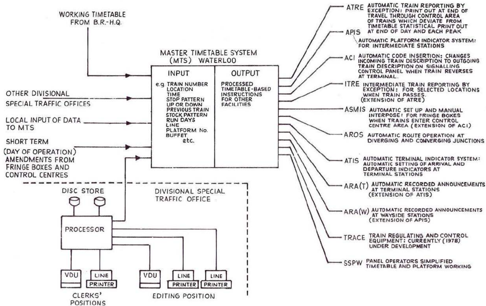
Fig. 9:26 Comprehensive scheme for the automatic compilation of timetables and the provision of other ancillary services using train descriptors currently being installed by British Railways (Southern Region)
