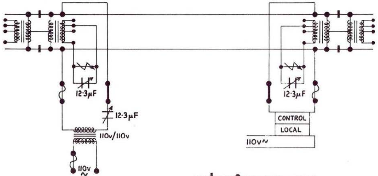
Fig. 7:17 Double rail AC track circuit with resonated impedance bonds
