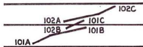
(E) ALTERNATIVE NUMBERING OF DOUBLE COMPOUND POINTS (POINT-TO-POINT INTERLOCKING NOT REQUIRED)
