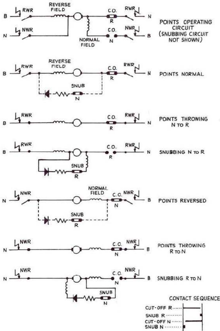
Fig. 4:17 Split field point machine: operating circuit sequence
