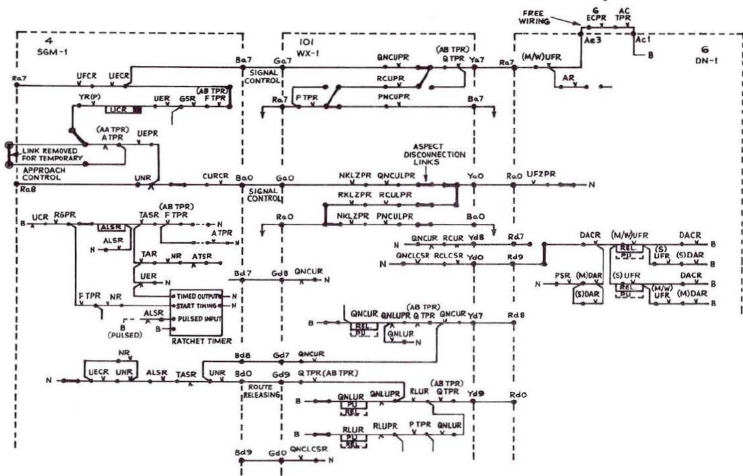
Fig. 6:14 System B: signal control and route releasing
