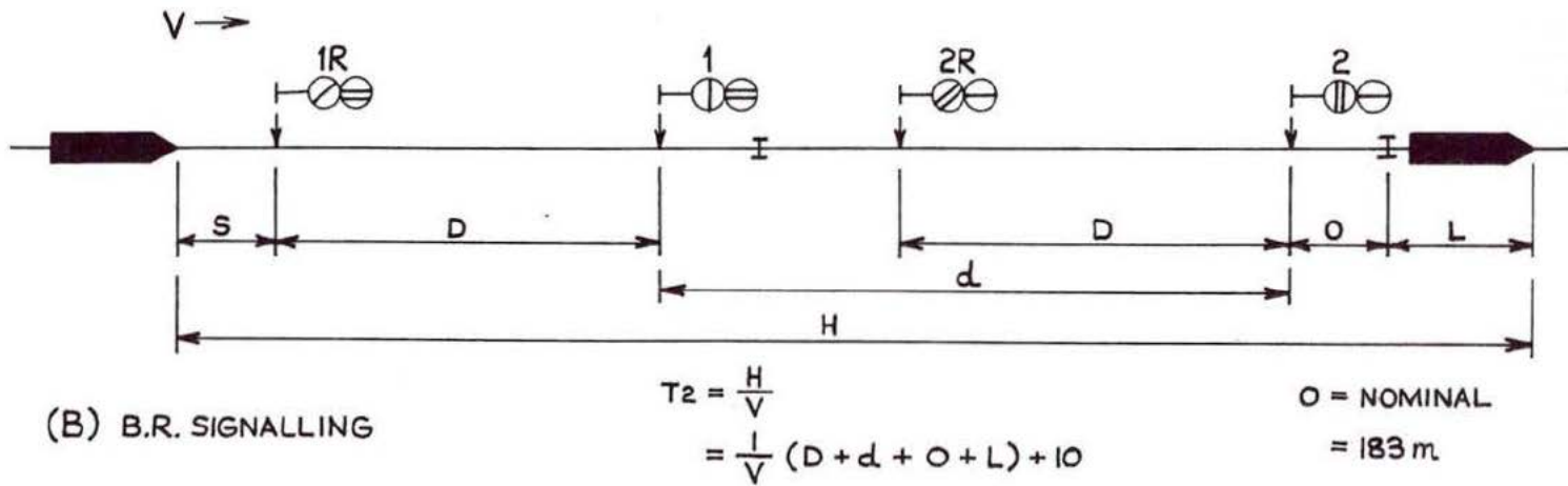
Fig. 2:1 2-aspect signalling: (A) Rapid Transit (B) British Railways
