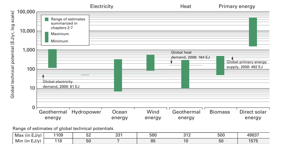
Fig. D1 Estimated global technical potential (EJ per year) of various renewable energy sources. Note the logarithmic scale, used to show the wide range! Source: IPCC SRREN (2011, fig. 1.17).
