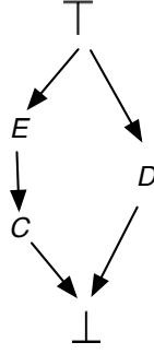
FIGURE 4.7: An \mathcal{EL}^{++} classification example.
