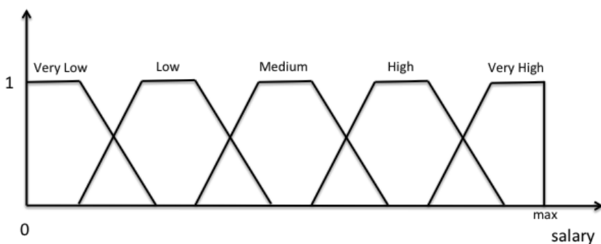
FIGURE 8.2: Fuzzy sets over salaries using trapezoidal functions.
