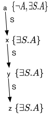
FIGURE C.2: Clash-free complete completion-forest for \mathcal{SHIF} KB.
