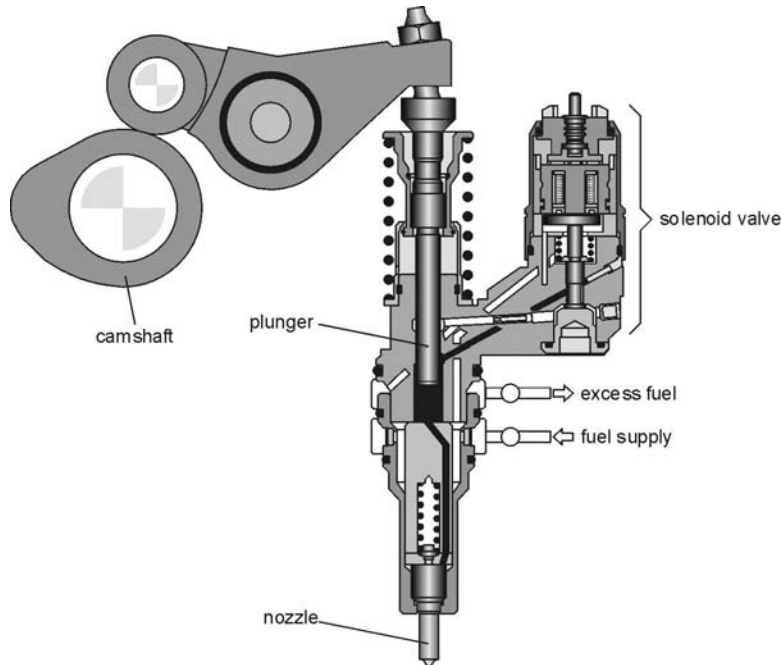
Fig. 2.27. Unit Injector [46]
