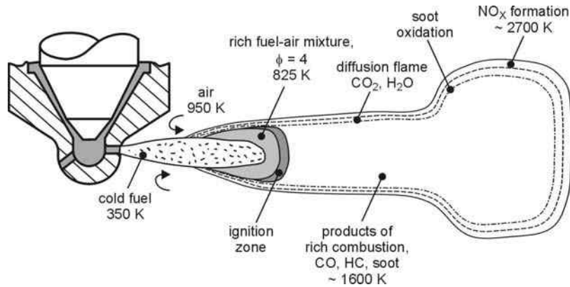
Fig. 6.2. Conventional diesel spray combustion and production of NO x and soot (PM)
