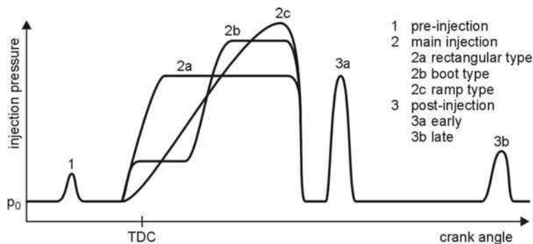
Fig. 6.5. Schematic diagram of a multiple injection
