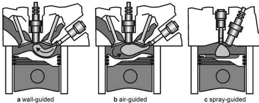
Fig. 6.19. Schematic description of the three possible stratified-charge combustion concepts
