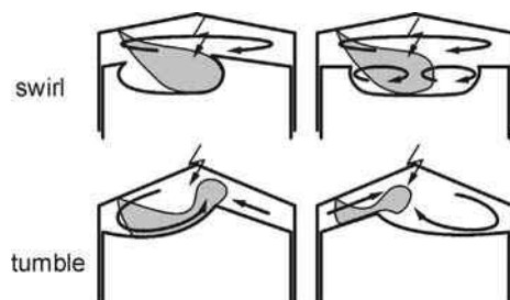
Fig. 6.20. Possible combustion chamber geometries as well as in-cylinder air motions, air-guided technique
