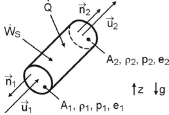
Fig. 3.4. One-dimensional pipe flow with heat and work
