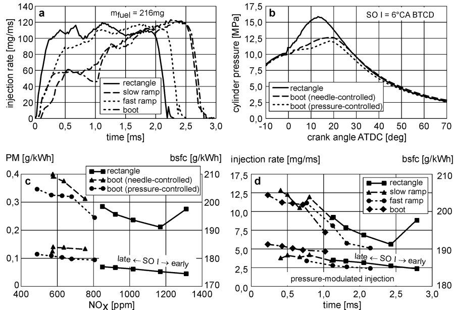
Fig. 6.15. Reduction of soot- \text{NO}_x trade-off: comparison of pressure-modulated and needle lift controlled rate shaping [74]. 2.0 liter single cylinder engine, \varepsilon : 16:1, 1300 rpm, m_{\text{fuel}} = 216 mg (high part load), no EGR
