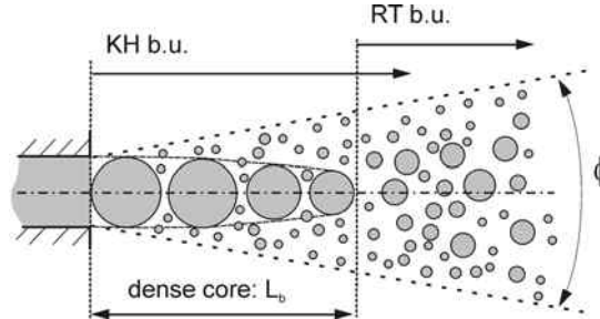
Fig. 4.29. Combined blob-HK/RT model
