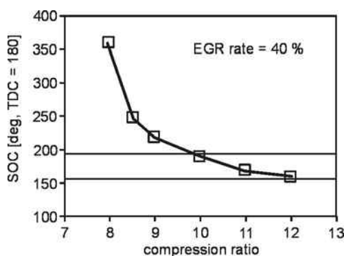
Fig. 6.36. Start of combustion versus compression ratio [71]
