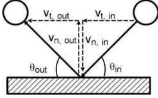
Fig. 4.65. Velocity components and respective angles for an impinging drop
