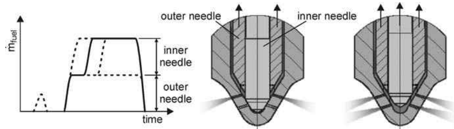
Fig. 6.11. Variable nozzle concept: possibility of rate shaping [9]
