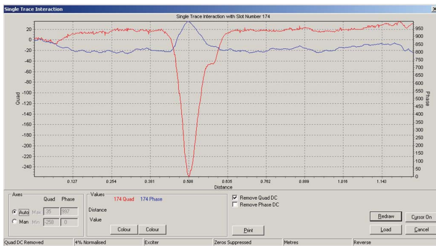
Figure 17.17 Trace of milliampere along the slot length giving indication of localized core insulation defect as indicated by high quadrature current of 258 mA and simultaneous deviation of phase current. (Source: Plot courtesy Iris Power-Qualitrol.)
