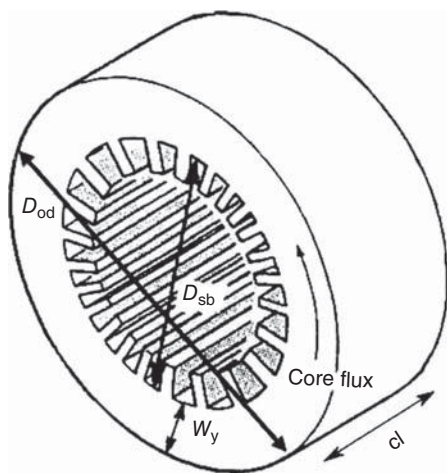
Figure 17.5 Dimensions for calculating core area.
