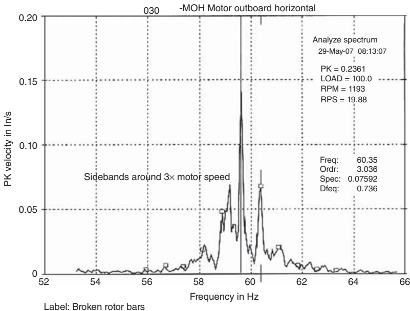
Figure 16.20 Frequency spectrum around 3\times running speed for a six-pole motor with broken bars. (Source: Taken from Reference 46.)
