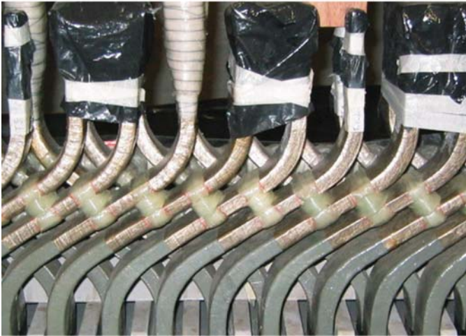
Figure 18.1 Interbar blocks covered with felt.
