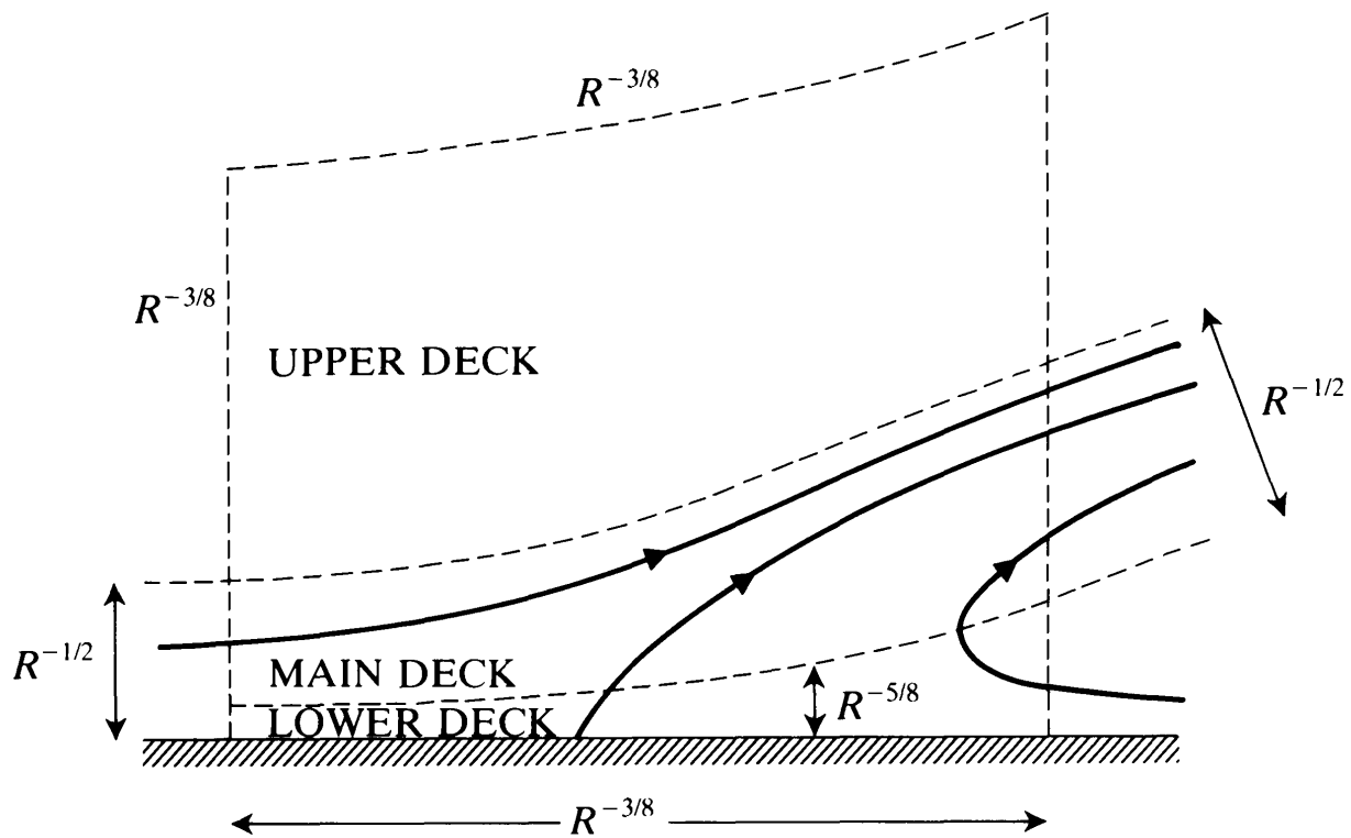
Fig. 8.13. Sketch of the triple-deck structure in the neighbourhood of a separation point on a rigid boundary.
