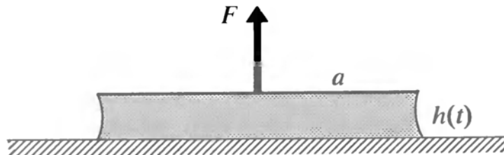
Fig. 7.10. Pulling a circular disc away from a rigid plane.
