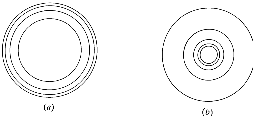
Fig. 3.9. Wave patterns produced by (a) a raindrop and (b) a large stone falling into a pond.
