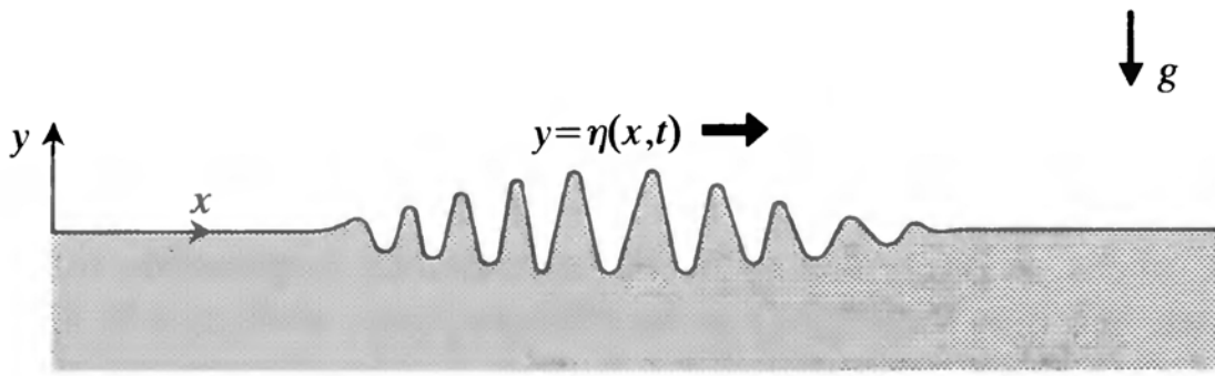
Fig. 3.1. A group of surface waves on deep water.
