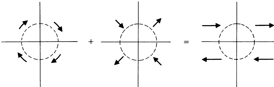
Fig. 6.8. The decomposition of a uniform shear flow.
