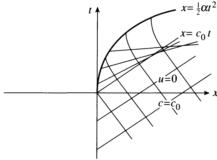
Fig. 3.18. The characteristic diagram.
