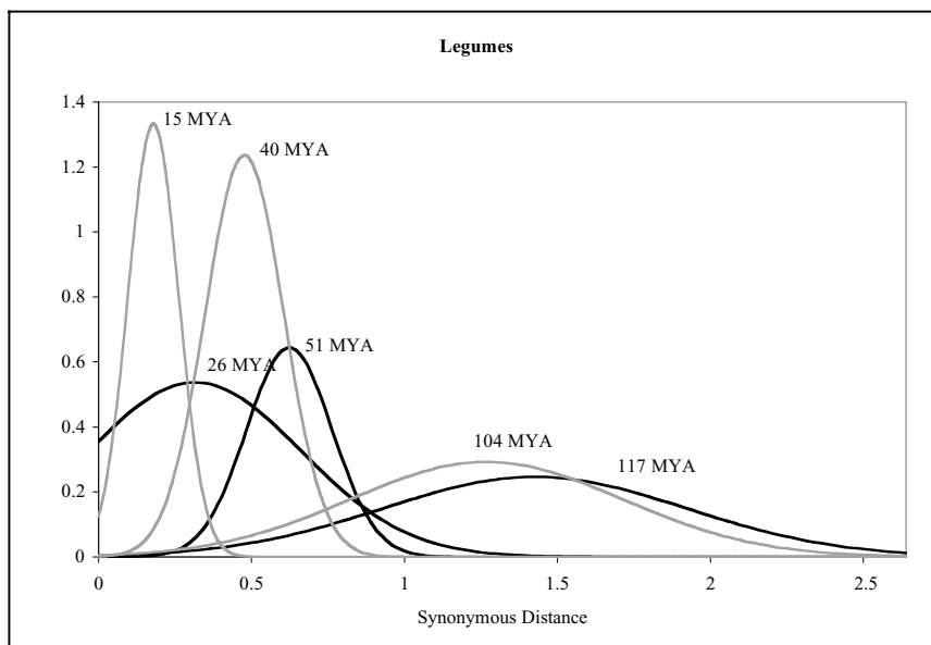
FIGURE 2. Normal distribution densities for both soybean and Medicago. Light grey curves correspond to soybean distributions. Black curves correspond to Medicago distributions. The dates next to each curve are the coalescence estimates in million years ago (MYA).
