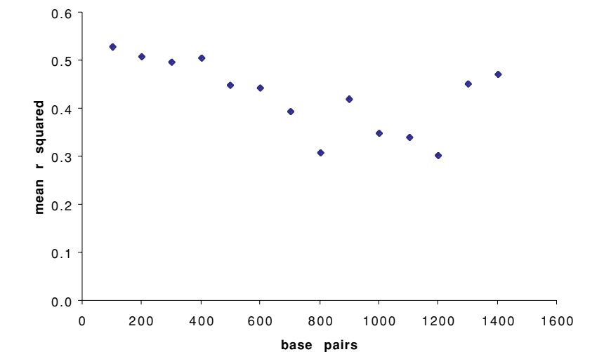
FIGURE 5. Average rate of decay of linkage disequilibrium ( r^2 ) in loblolly pine.
