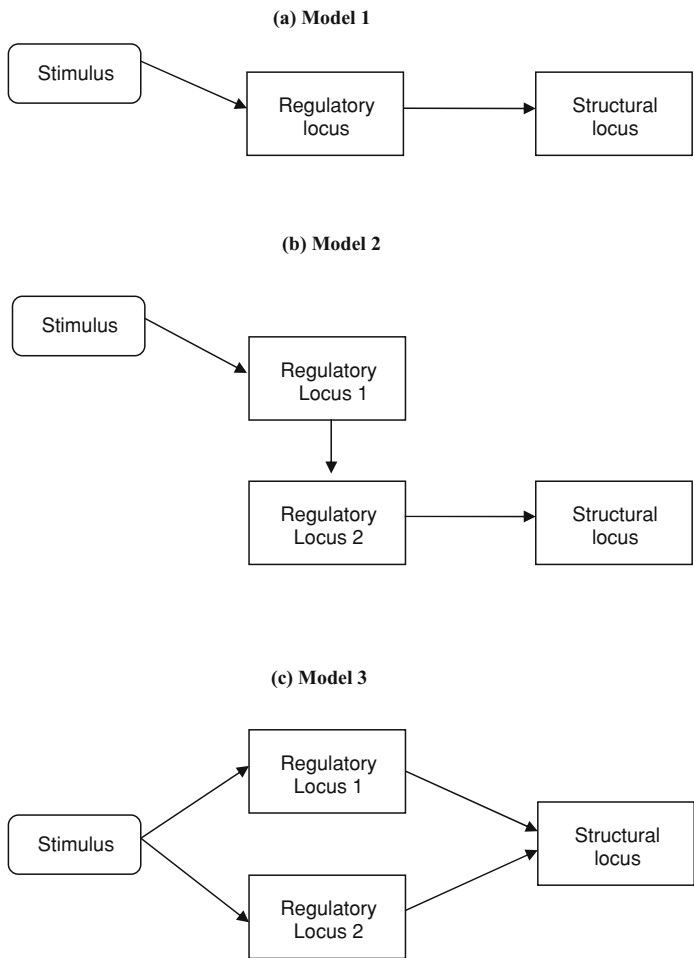
FIGURE 1. Three simple models illustrating a single structural gene with one or two additional determinants of expression level polymorphisms.
