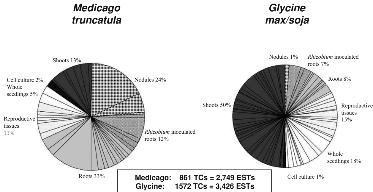
FIGURE 2. EST distribution of legume-specific TCs from Medicago truncatula and Glycine max/soja . Individual pie slices represent unique cDNA libraries from which ESTs were sequenced. Libraries corresponding to similar tissues have been color coded and labeled. In Medicago , 69% of ESTs from the legume-specific TCs correspond to roots; Rhizobium inoculated roots, and nodules. In soybean, 68% of EST from legume-specific TCs correspond to shoots and whole seedlings.
