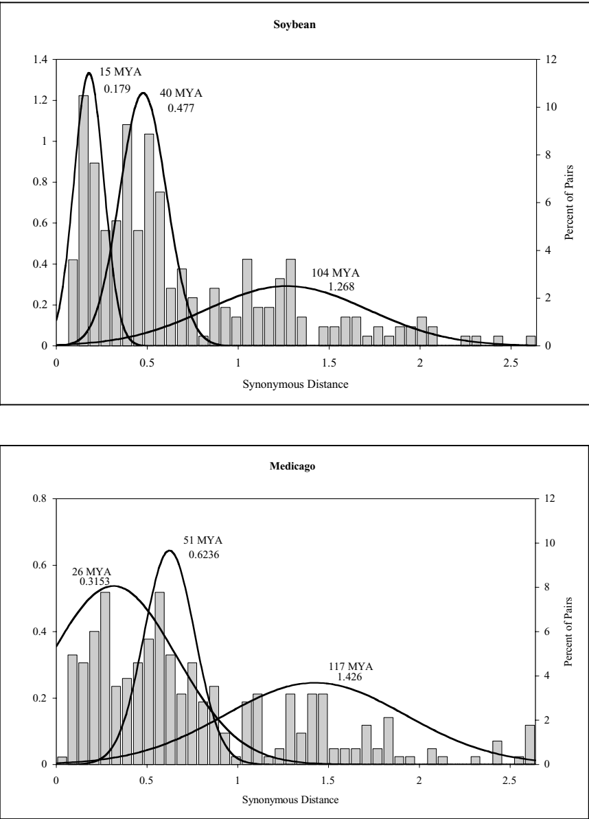
FIGURE 1. Histogram of the percent of identified pairs for both soybean and Medicago (secondary y-axis) based upon estimated synonymous distance measures. The curves are normal distribution densities (y-axis) for the statistically significant number of distributions. Beside each curve are the mean of synonymous distances under that curve as well as the correspondingly calculated coalescence estimates in million years ago (MYA).
