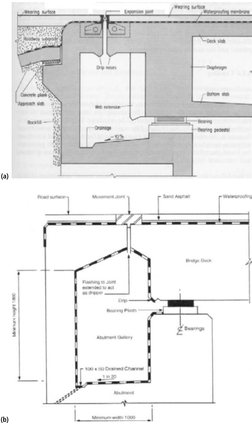
Figure 10.11 Access gallery between deck and abutment: (a) after Menn (1999); and (b) BA57/95.
