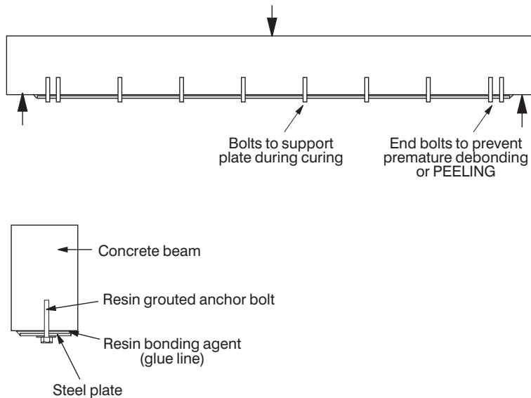
Figure 7.1 Typical plate bonding application.
