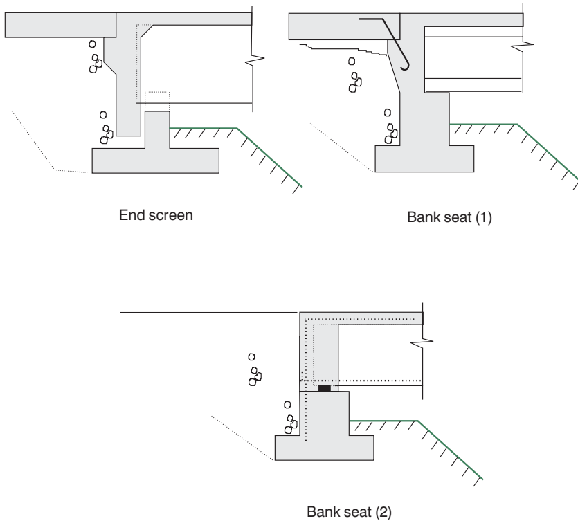
Figure 10.15 Other types of 'sliding' integral abutments.
