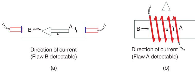
Figure 4.29 Flaw detection using MPI.
