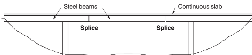
Figure 8.8 Cantilever construction using steel beams.
