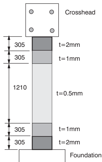
Figure 7.11 Design jacket arrangement for a rectangular column with 2.5% longitudinal reinforcement (after Seible 1997).
