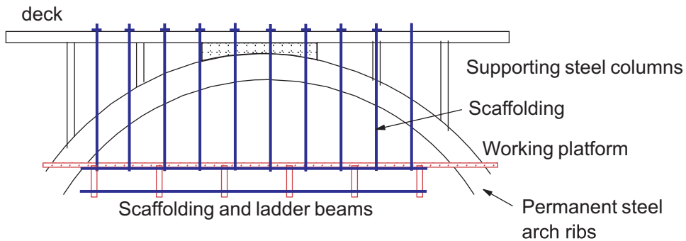
Figure 2.18 Access by hanging platform.
