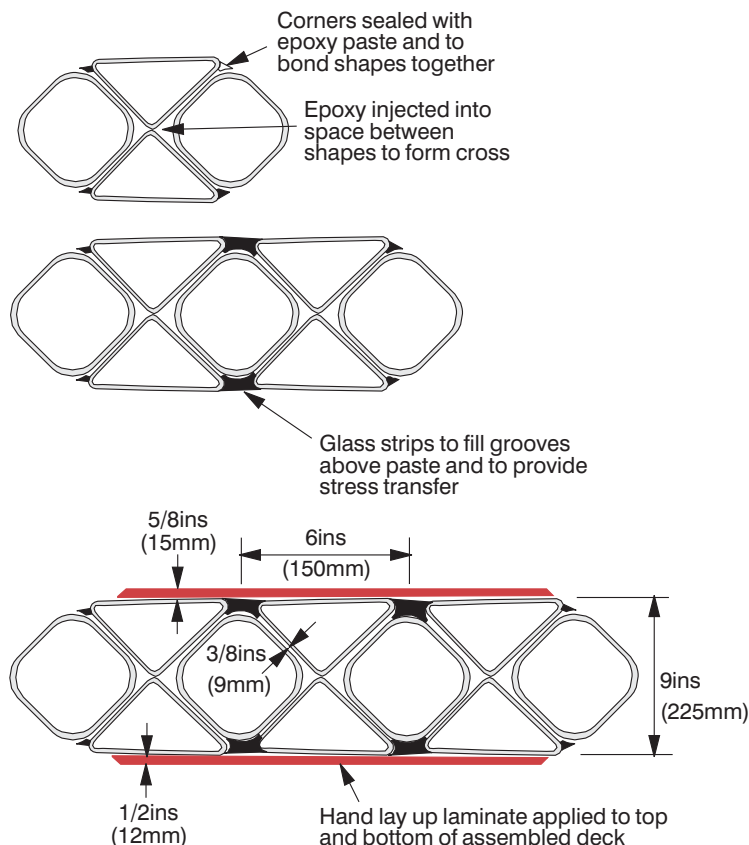
Figure 8.13 Steps in the build-up of the FRP units.
