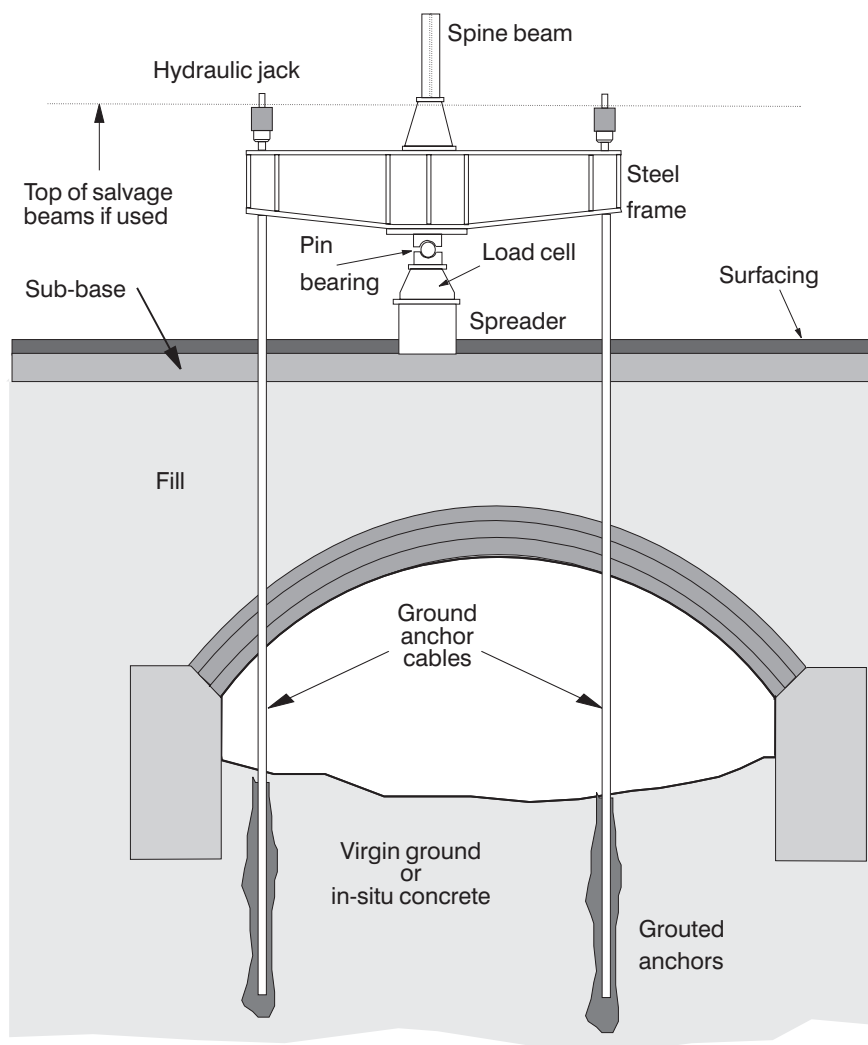
Figure 5.9 Typical jacking arrangement to an arch bridge.
