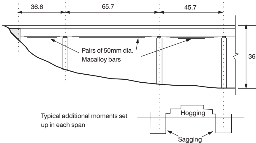
Figure 7.14 Strengthening of Rakewood Viaduct (after Pritchard 1990).
