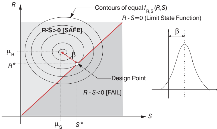
Figure 12.3 Failure zone with respect to joint probability distribution of R and S .
