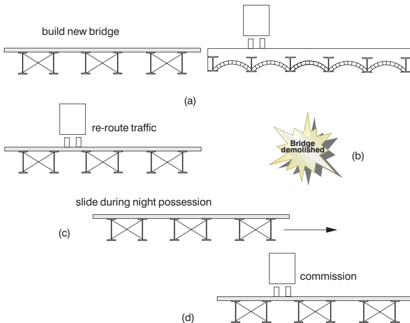
Figure 8.18 Lateral sliding.
