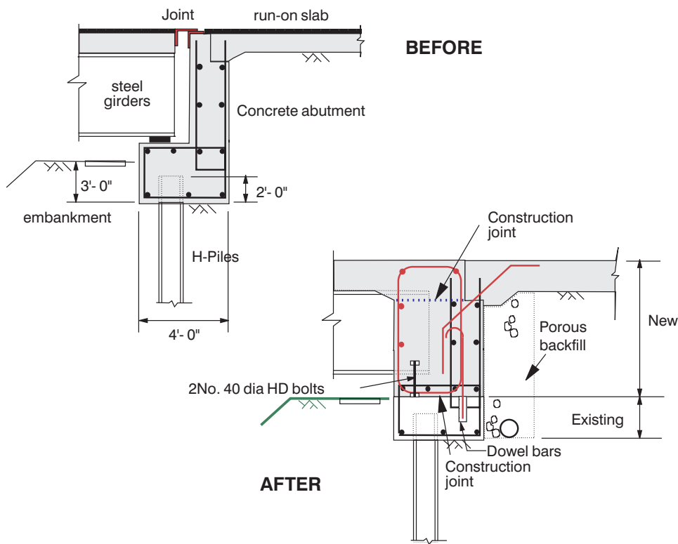
Figure 8.29 Conversion of jointed bridge decks to integral bridge decks.
