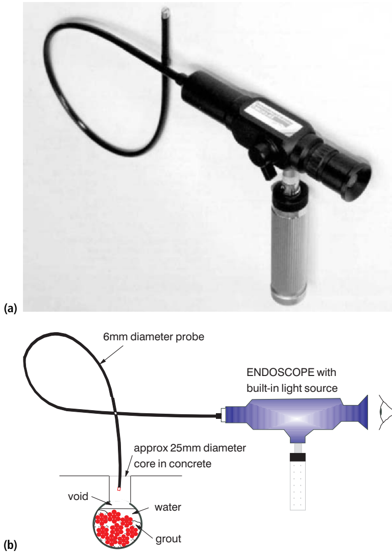
Figure 4.21 (a,b) Typical endoscope and set-up.
