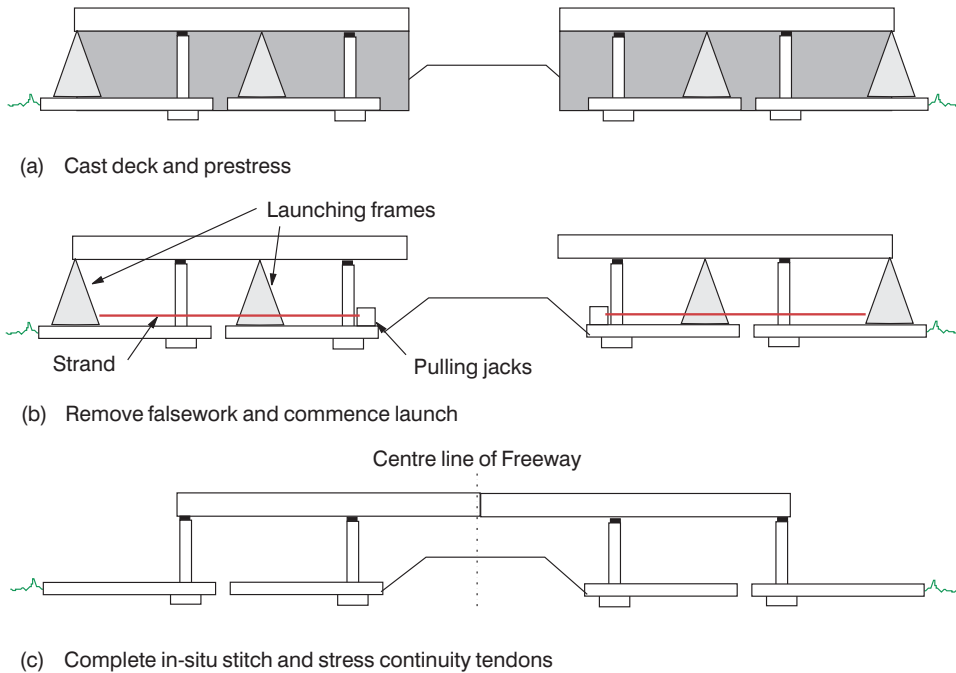
Figure 8.21 Launching method (after Champion, 1994).
