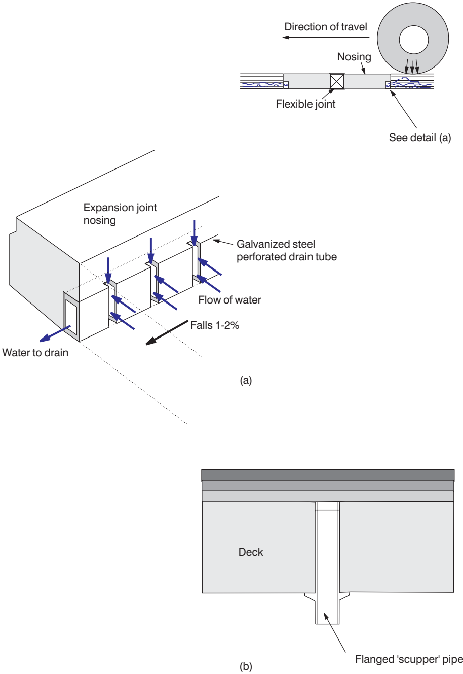
Figure 10.1 Scupper pipe surface drainage and subsurface drainage at expansion joints.
