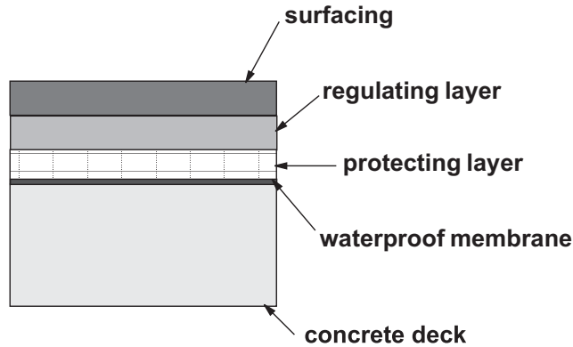
Figure 2.17 Make-up of a typical deck topping.
