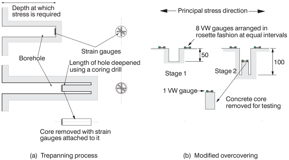
Figure 11.3 Comparison between trepanning process and modified overcore.
