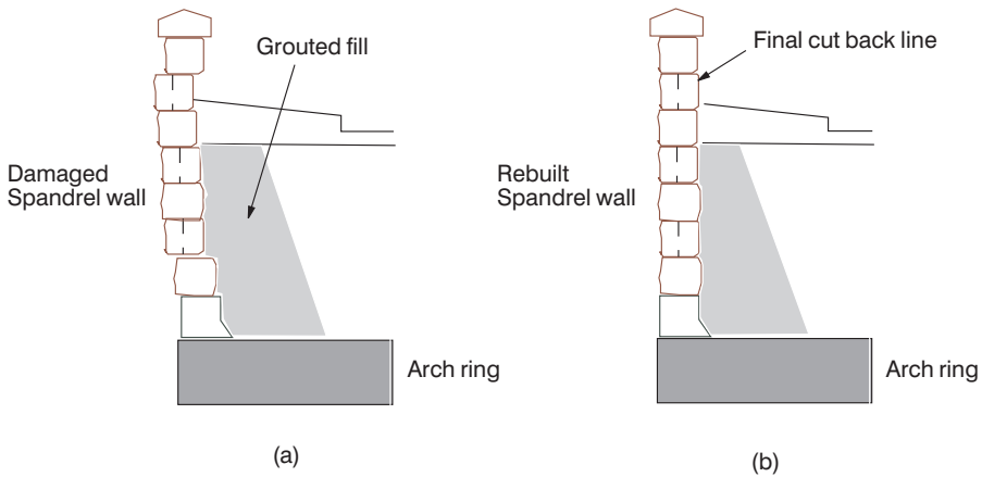
Figure 6.6 Grouted fill repair options for bulging or displaced spandrel walls.
