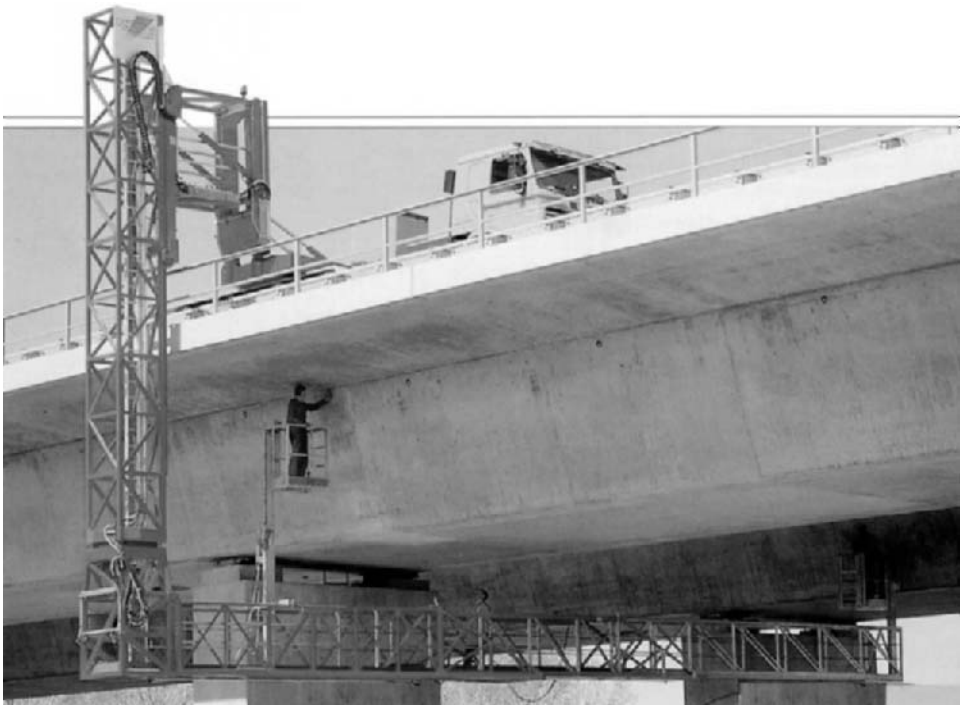
Figure 2.20(a) Lattice platform for inspecting a prestressed concrete box girder bridge.
