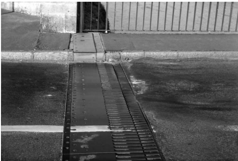
Figure 2.6 Example of deck surfacing damage adjacent to an expansion joint.
