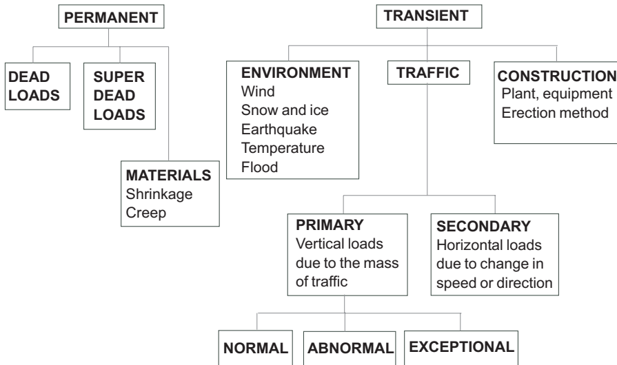
Figure 3.1 Loads on bridges.
