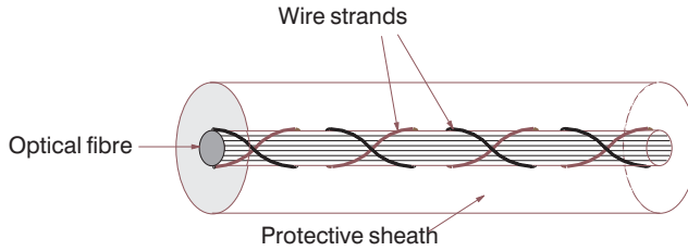
Figure 11.21 Optical fibre sensor (after Wolff and Miesslerer, 1993).
