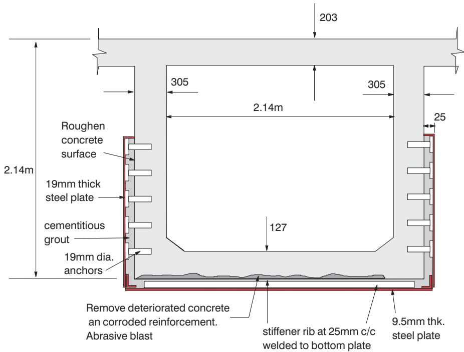
Figure 7.33 Cross-section of strengthened concrete box girder (after Englot, 1996).
