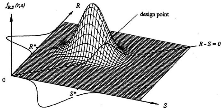
Figure 12.4 Three-dimensional representation of the design point (after Bailey 1996).
