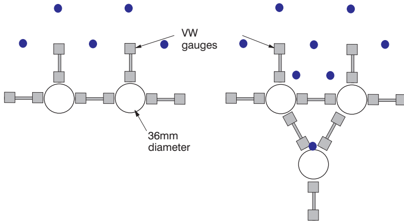
Figure 11.4 Typical gauge layout for multiple holes.
