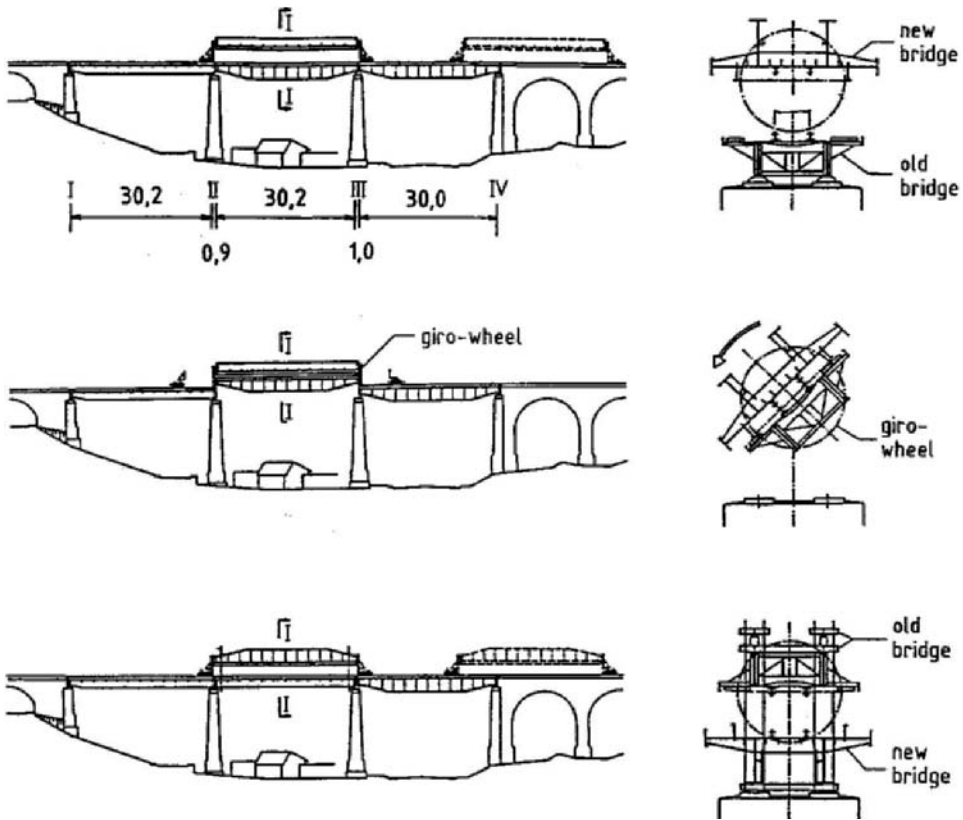
Figure 8.20 Construction procedure for the replacement of the Schwarzbach Valley Bridge at Wuppertal (Saul, 1996).
