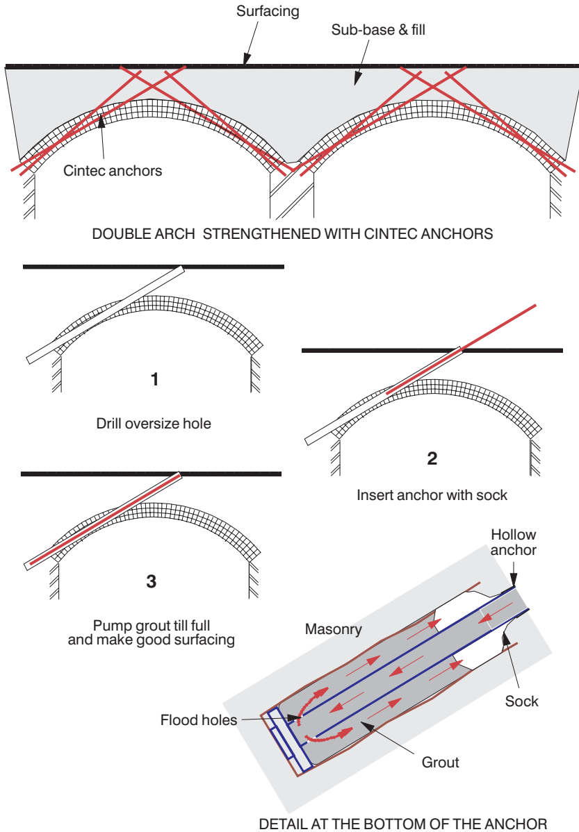
Figure 7.23 Typical stitching application.
