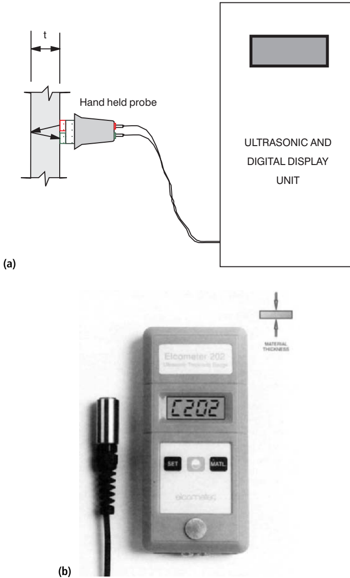
Figure 4.33 (a) Principle and (b) ultrasonic thickness gauge (courtesy of Elcometer Ltd. UK).
