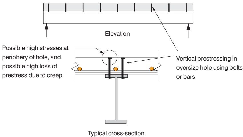
Figure 7.32 Enforced frictional contact using vertical prestressing.
