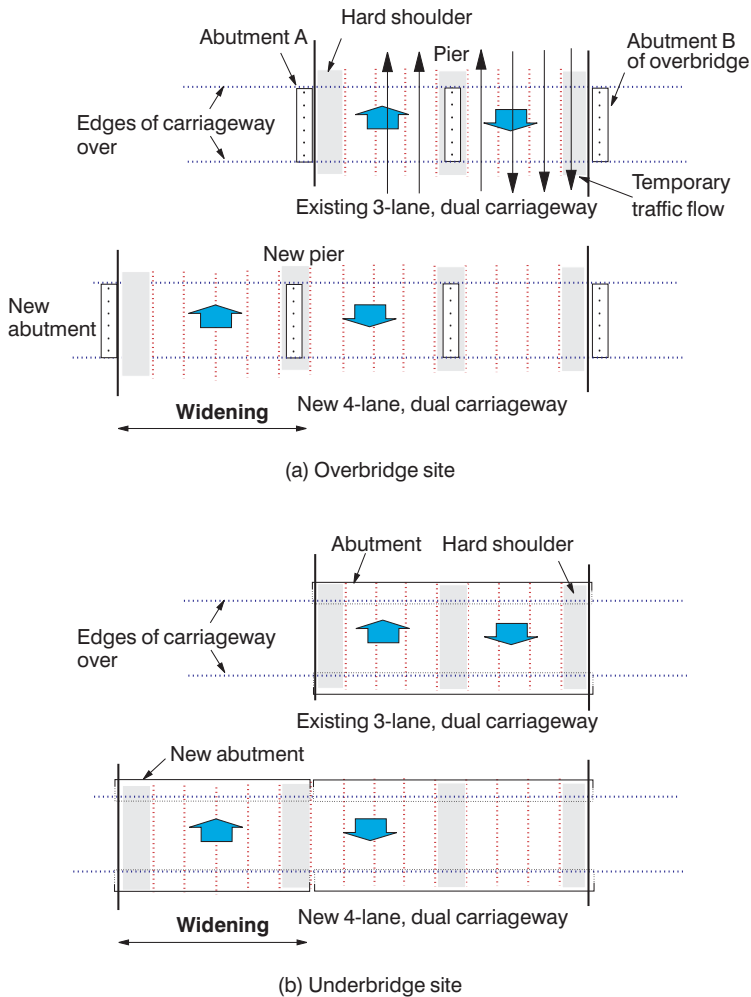
Figure 8.3 Parallel widening.
