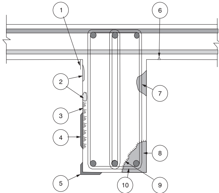
Figure 6.9 Typical hand applied concrete repairs.
