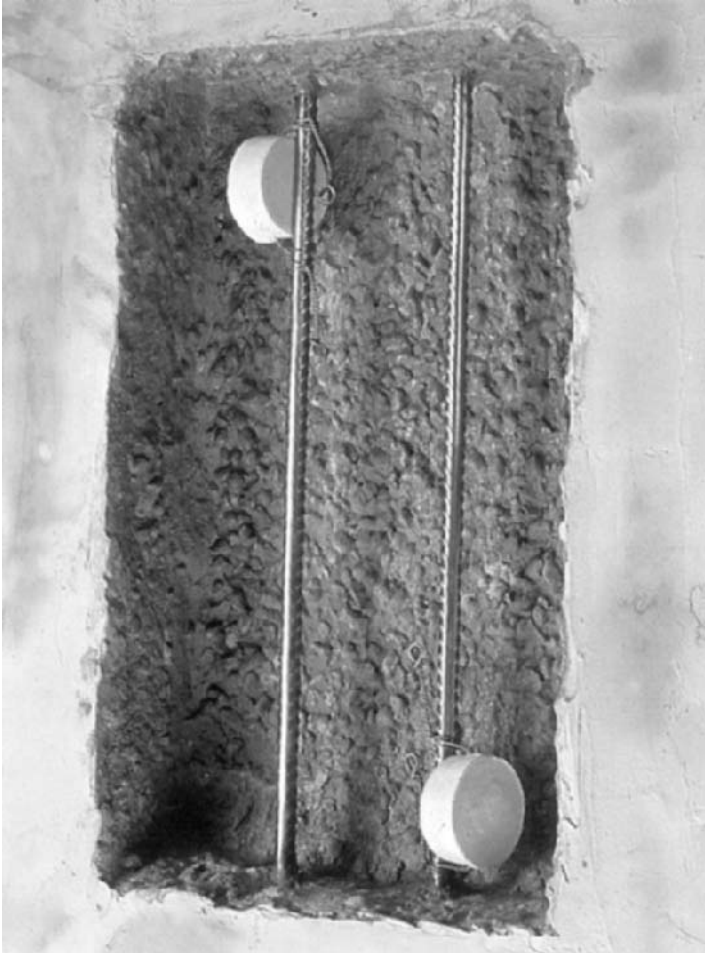
Figure 10.10 Sacrificial anode system in use (Fosroc Systems).
