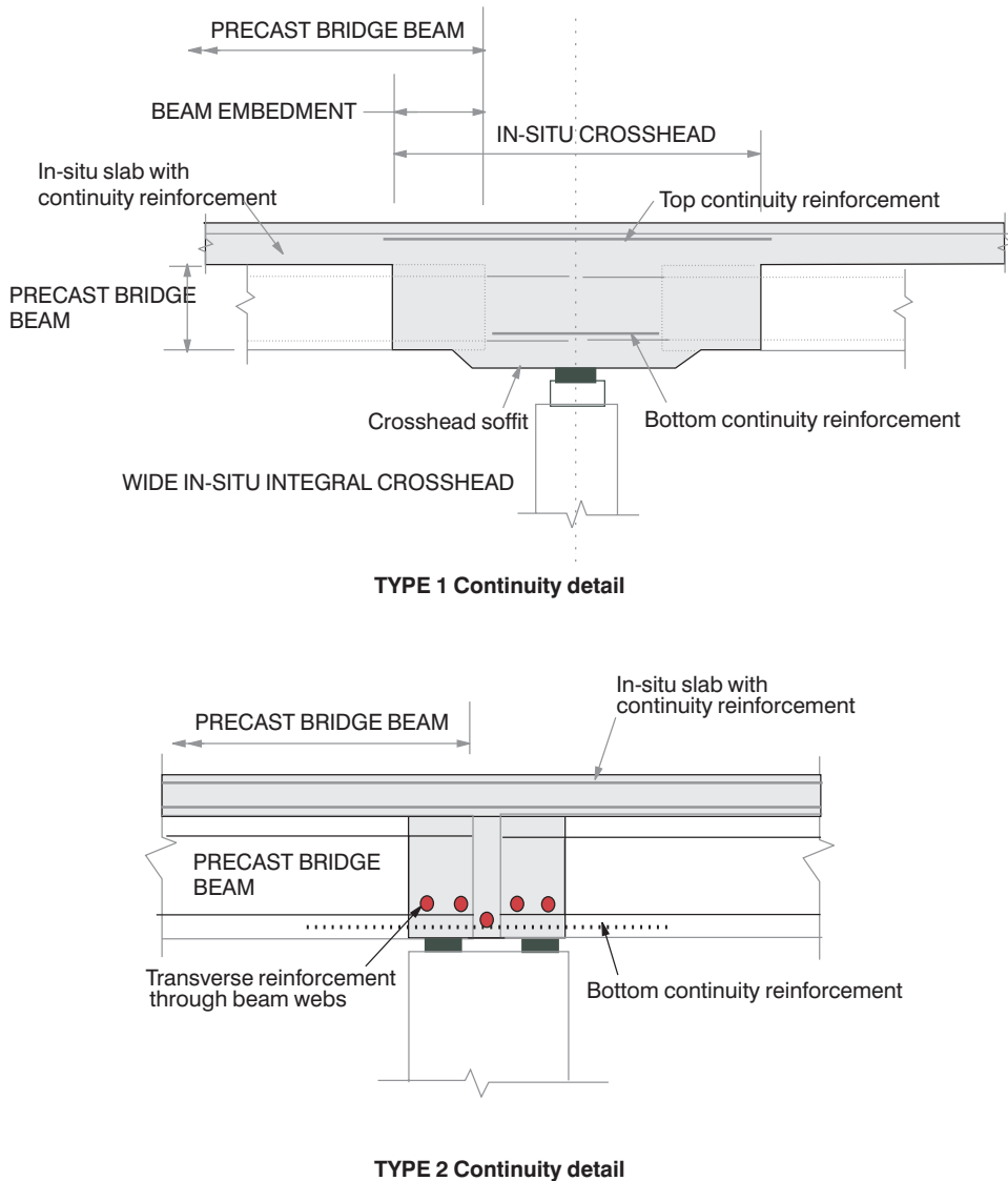
Figure 8.11 Deck continuity.
