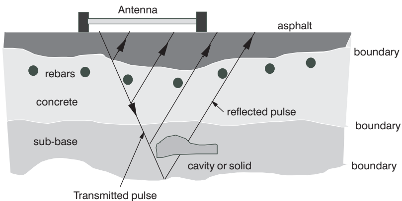
Figure 4.17 Principle of impulse radar.
