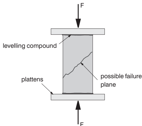
Figure 4.24 Typical set-up for compressive testing of a concrete cylinder.
