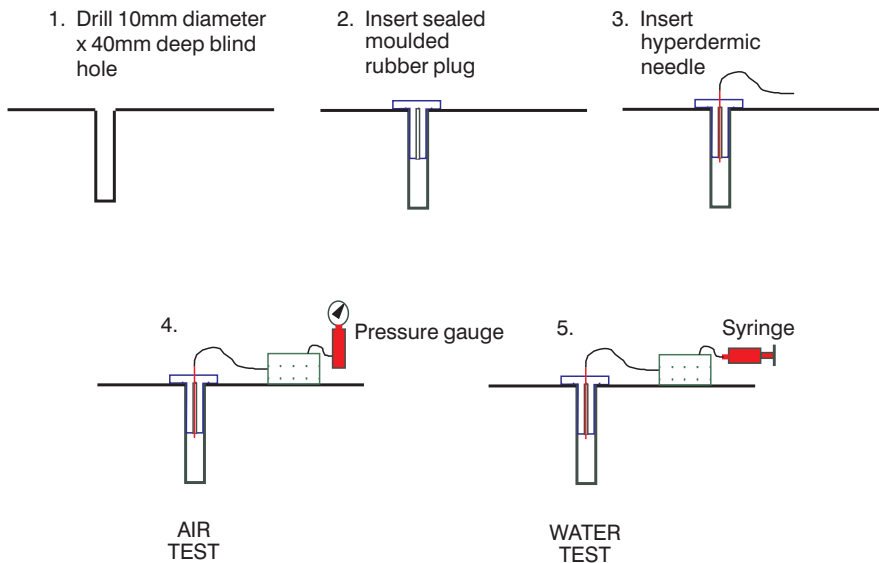
Figure 4.12 Steps in the application of the modified FIGG method.
