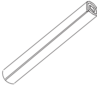
Figure 7.31 Spring pin 'Spirol' shear connectors (Pritchard, 1994).
