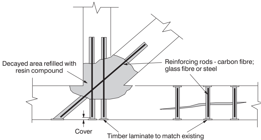
Figure 6.16 Timber repairs using the rod-and-resin technique.
