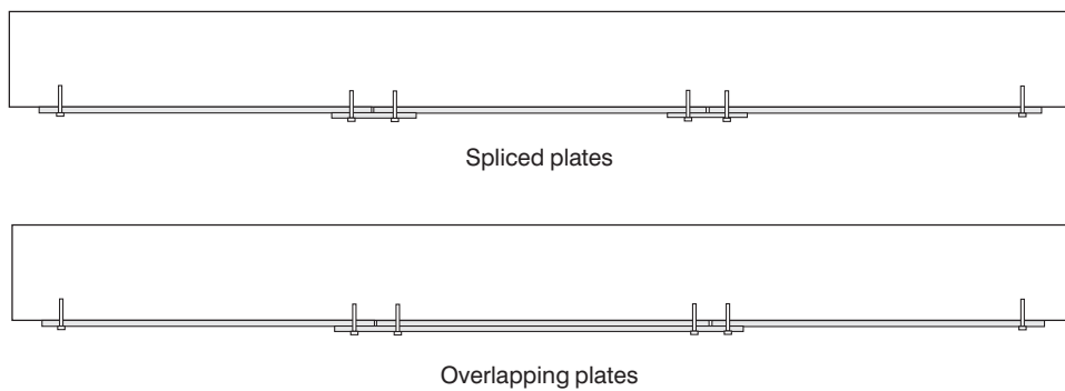
Figure 7.5 Means of providing continuity in plates (for clarity, only anchor bolts shown).
