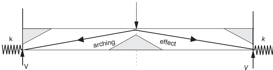
Figure 5.3 Restrained slab (after Jackson, 1995).
