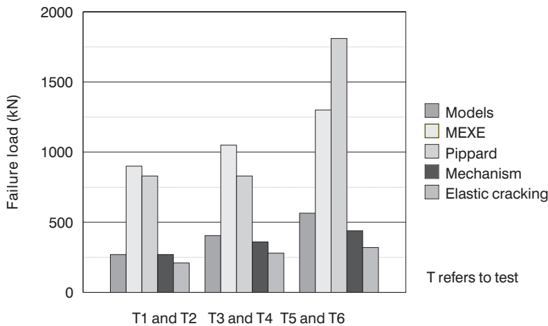
Figure 3.13 Variation of model and predicted assessment loads with masonry and soil type (after Hughes et al. , 1998).
