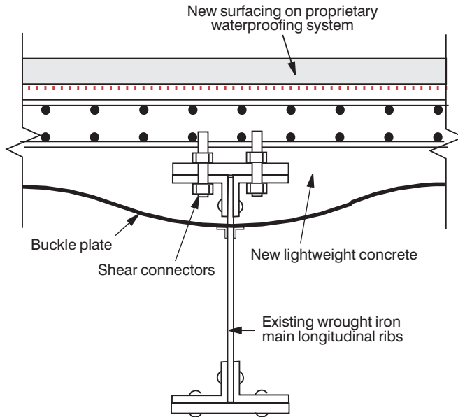
Figure 7.27 Deck reconstruction of the Westminster Bridge (Yeoell and Munson, 1993).
