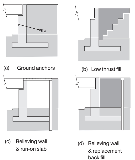
Figure 7.38 Pressure relief methods to abutments.
