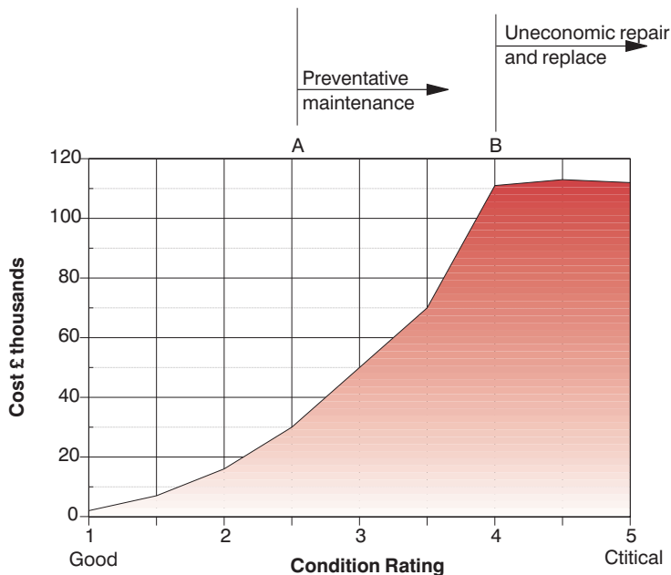
Figure 9.8 Cost of repairs versus condition rating.
