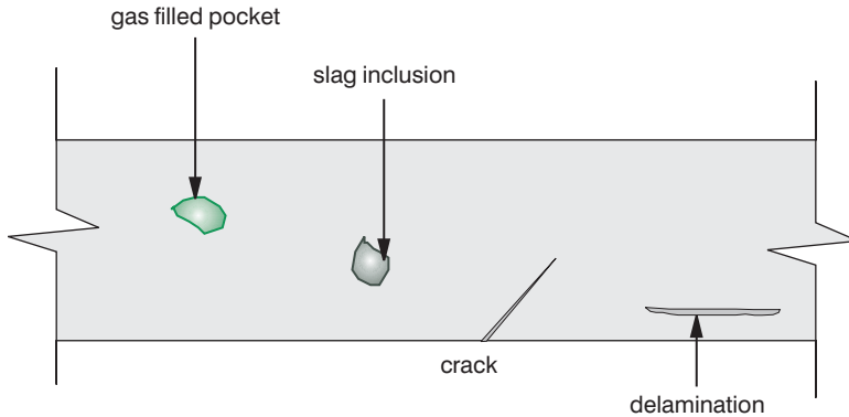
Figure 4.26 Imperfections in steel.
