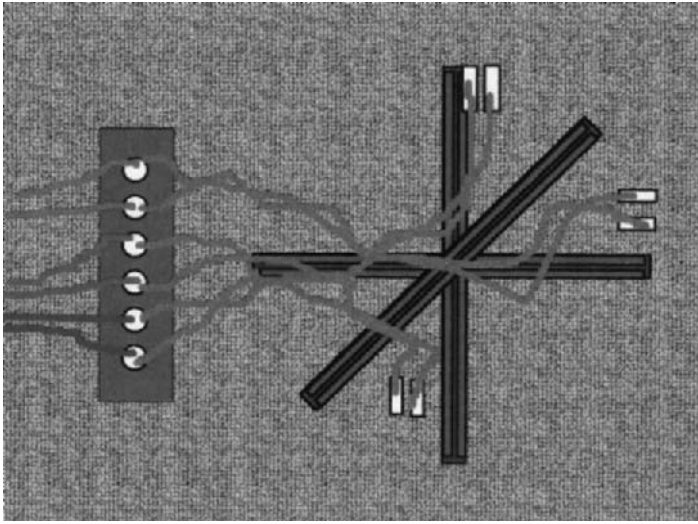
Figure 11.17 Long electrical resistance strain gauges.
