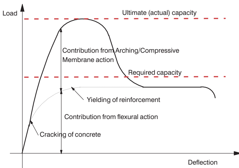
Figure 5.4 Interaction between flexural and compressive membrane action (after Long et al. , 1994).
