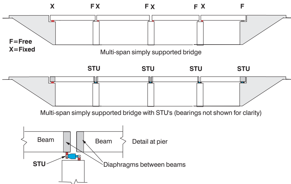
Figure 8.31 Multispan bridge with and without STUs.
