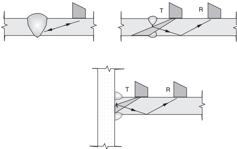
Figure 4.27 Typical probe arrangements when testing welds.
