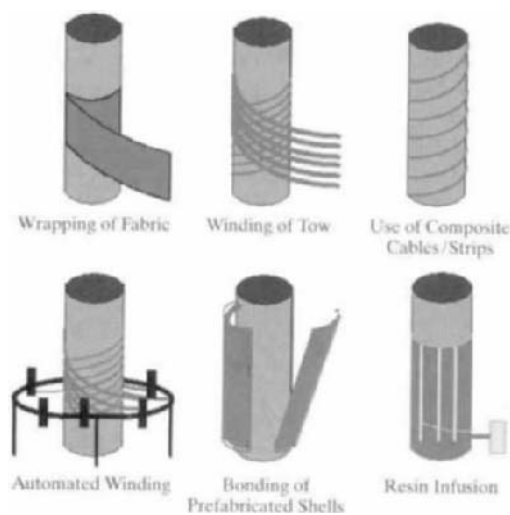
Figure 7.12(a) Application of CFRP wraps to columns (Karbhari and Seible 1999)
