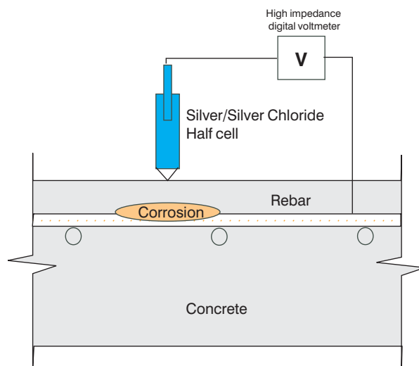
Figure 4.1 Typical half-cell set-up.
