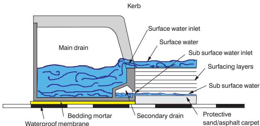
Figure 10.2 Kerb drainage units.
