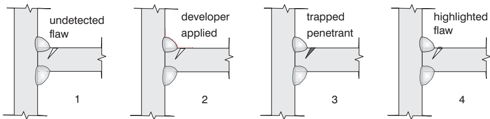
Figure 4.31 The application of LPI.
