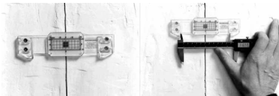
Figure 11.16 (a) Plastic tell-tale in use, and (b) digital caliper (0.1 mm accuracy).
