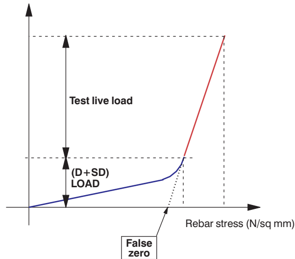
Figure 5.12 Load–Stress plot under applied test load.
