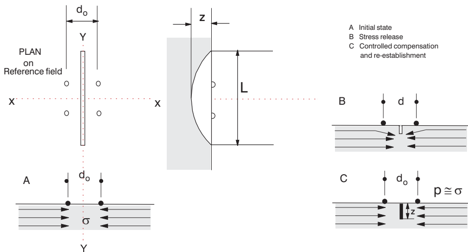
Figure 11.9 Slot cutting method (after Abdunur, 1985).
