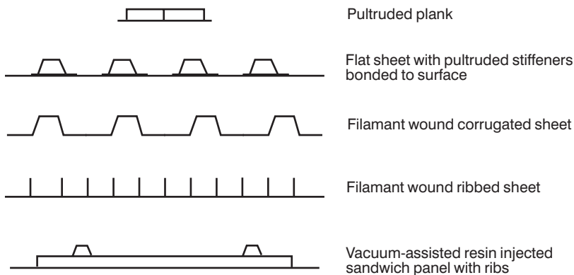
Figure 8.26 Trial GRP profiles.
