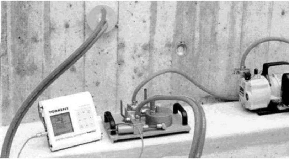
Figure 4.13 Typical FIGG equipment in use.
