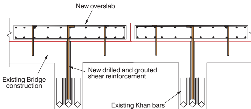
Figure 7.28 New overslab and shear reinforcement to the Woodbridge Old, Guildford.
