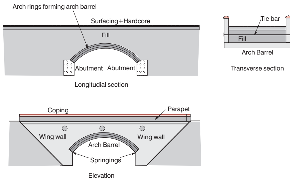
Figure 5.2 Typical arch bridge construction.
