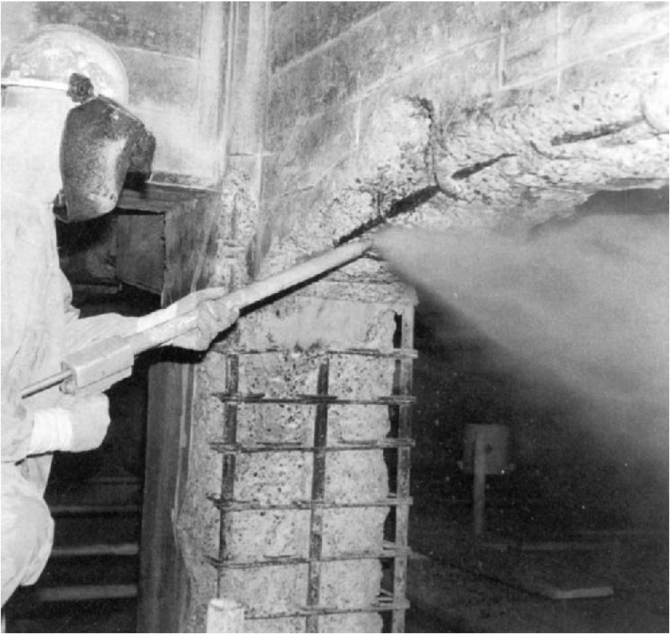
Figure 6.8 Water jetting on the Silverton Viaduct (courtesy Cons. Main & Repair ).
