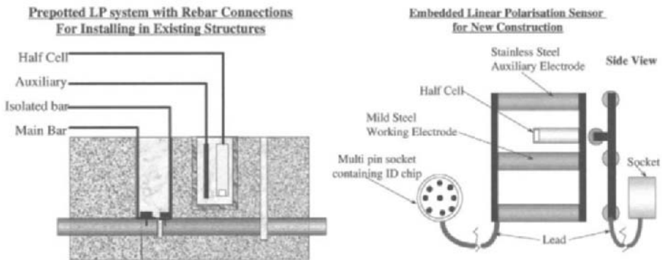
Figure 11.19 Linear polarization sensor in new and existing structures (Broomfield et al. , 1999).
