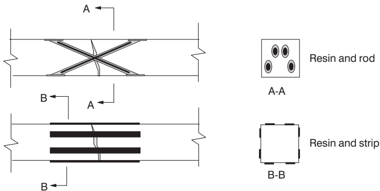
Figure 6.17 Timber repair of a complete fracture.
