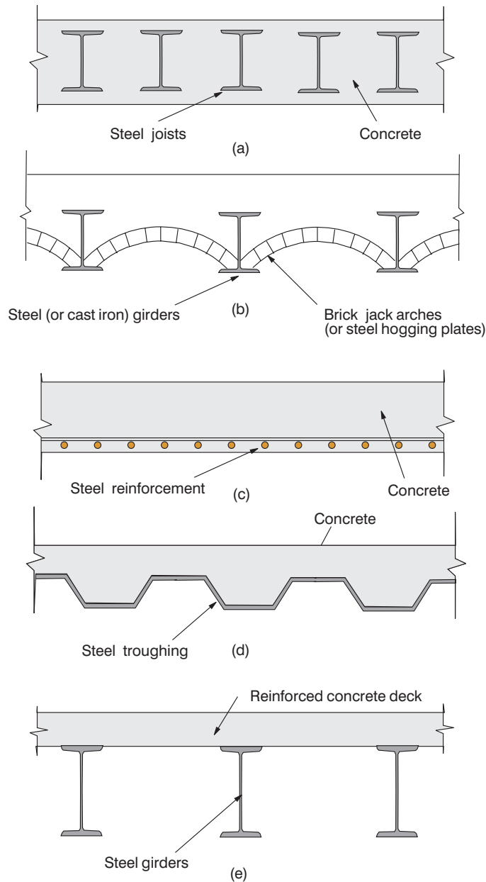
Figure 5.1 Bridges suitable for supplementary testing.
