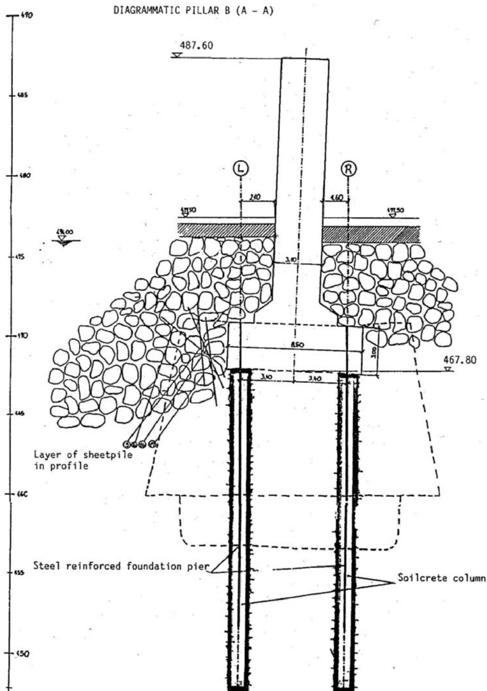
Figure 7.39 Strengthening solution by (Kittinger and Ashaber 1993).
