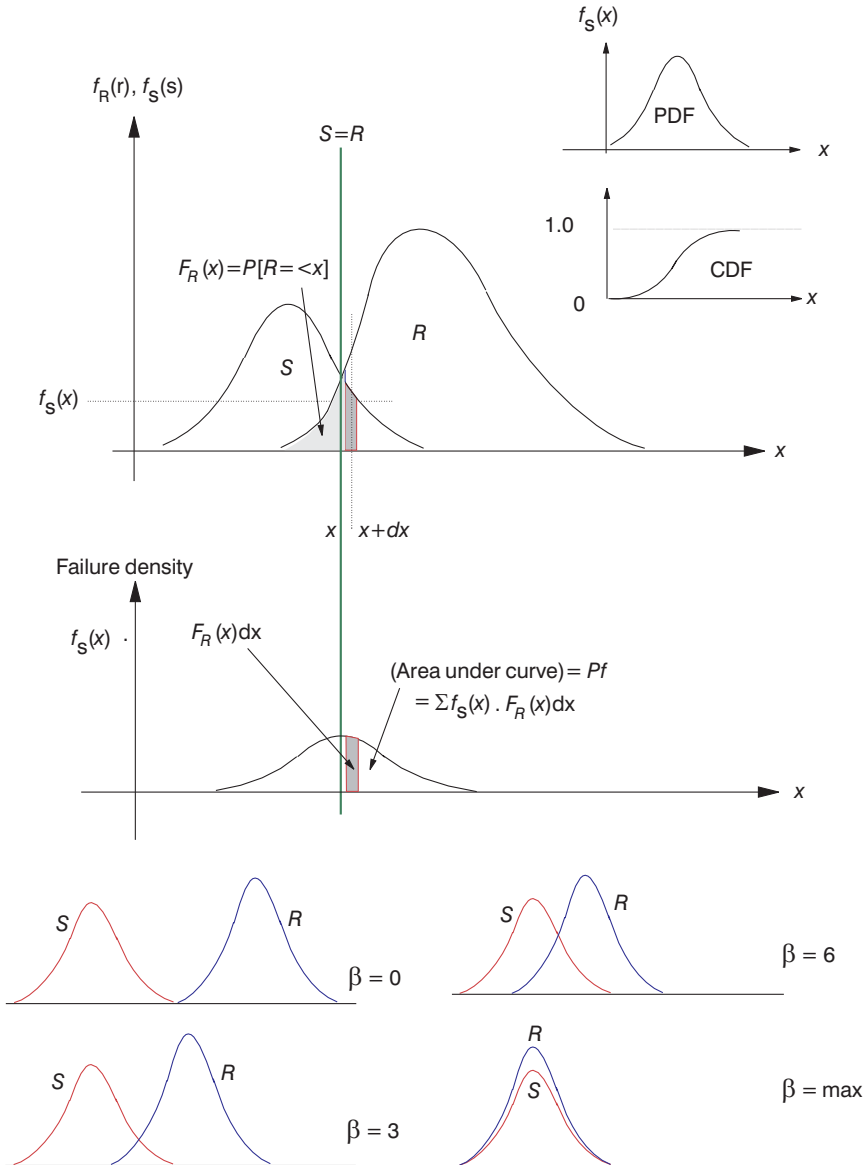
Figure 12.2 Probability distribution of R and S .
