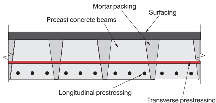
Figure 5.6 Part section of the Cadnum Green Bridge.
