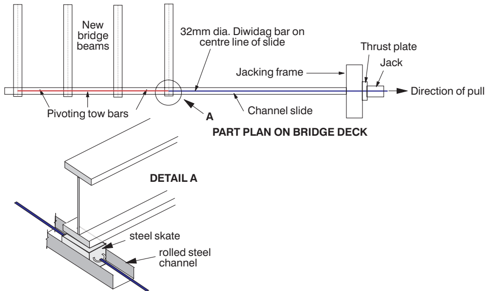
Figure 8.19 Sliding detail on Callender-Hamilton bridge replacement.
