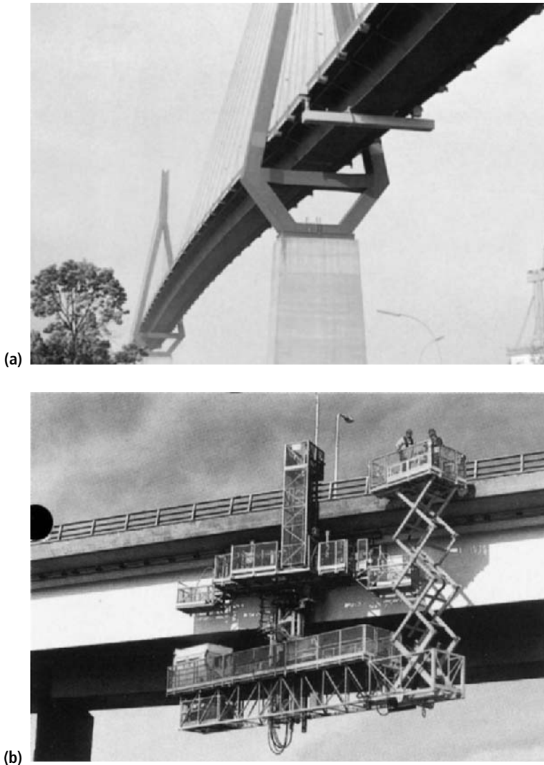
Figure 2.21 Examples of permanent gantries (a) Kohlbrand Bridge near Hamburg; (b) Tay Bridge, Scotland.
