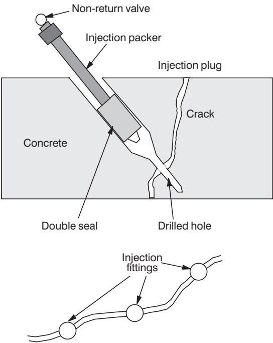
Figure 6.7 Crack injection system.
