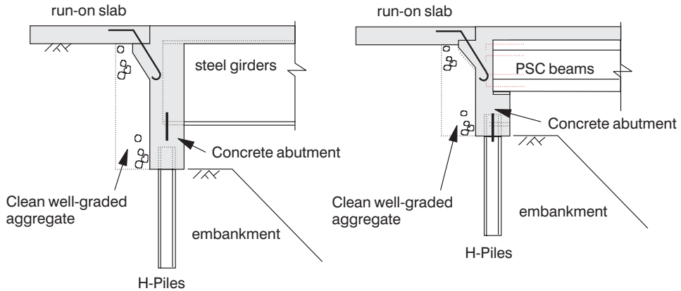
Figure 10.14 Two types of 'flexible' integral abutments.
