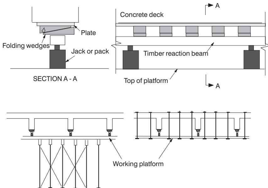
Figure 7.6 Typical working platform and support system for plate bonding.
