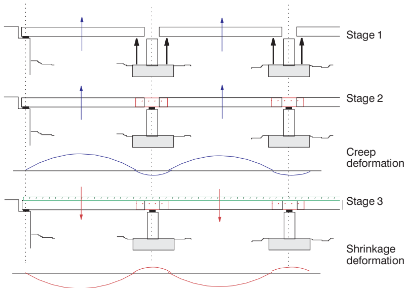
Figure 10.18 Construction stages and effects of creep and shrinkage.
