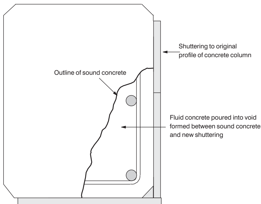
Figure 6.11 Plan on column to be repaired.
