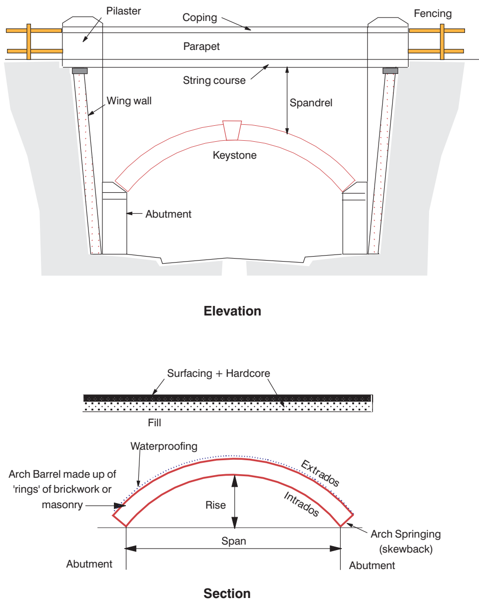
Figure 3.8 General arrangement of a masonry arch bridge.
