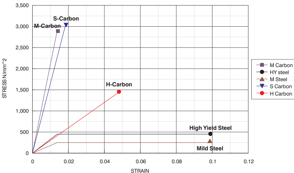
Figure 7.8 Comparison of stress–strain characteristics of steel and carbon.
