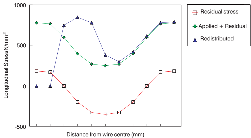
Figure 11.12 Typical stress variations in a steel wire.
