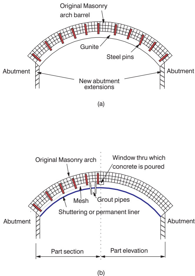
Figure 7.18 Strengthening of the intrados.
