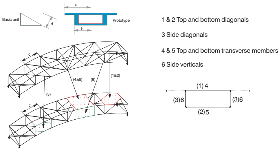
Figure 3.4 Typical space frame representation of a box girder bridge.
