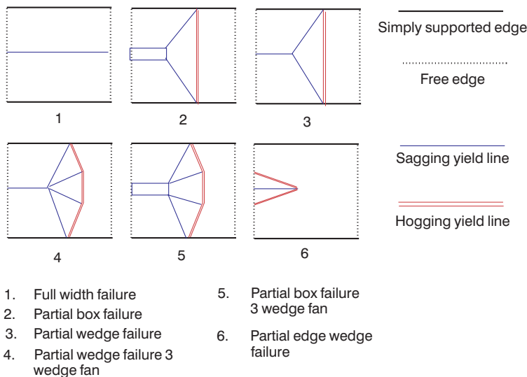
Figure 3.5 Typical failure modes for simply supported slab bridges.
