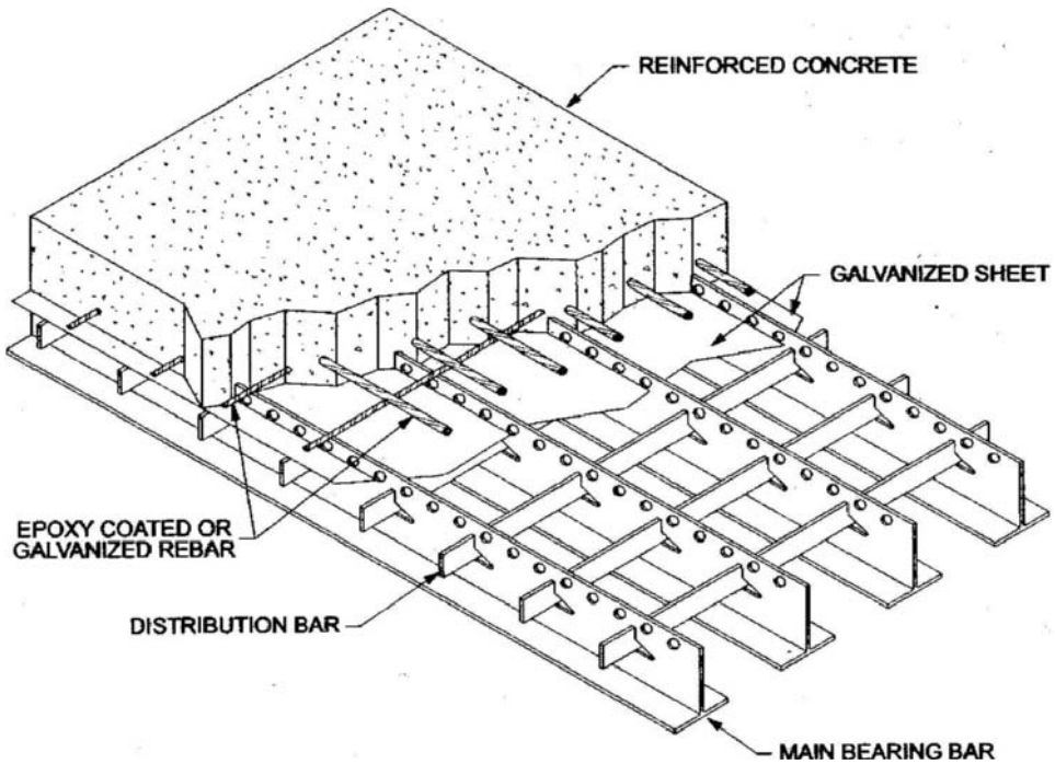
Figure 8.16 Exodermic bridge deck panels.
