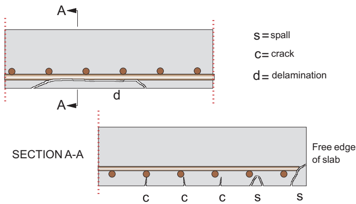
Figure 2A.1 Definitions of damage to concrete (courtesy of Dr Florian Burtescu, Romania).
