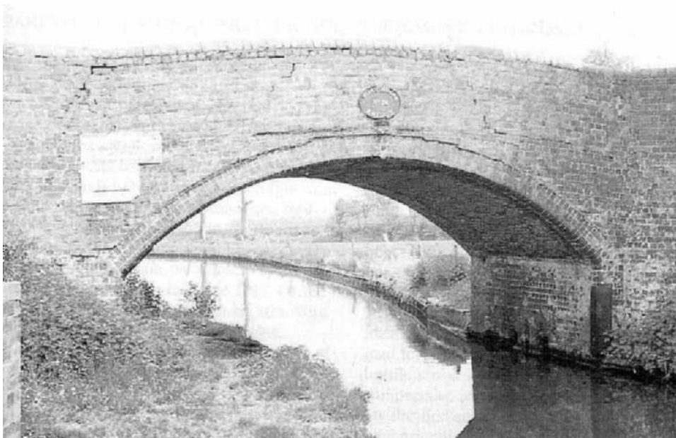
Figure 2.10 Example of cracking between the arch barrel and spandrel wall (cracks highlighted for clarity).
