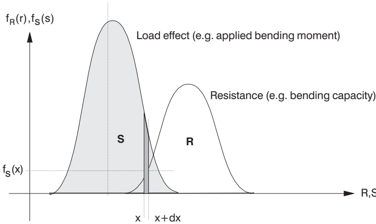
Figure 3.6 Probability distribution of R and S .
