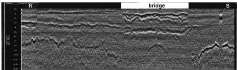
Figure 4.18 Typical impulse radar plot (courtesy EMPA, Switzerland).
