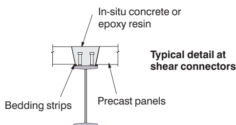
Figure 8.9 Use of precast deck panels in composite construction.
