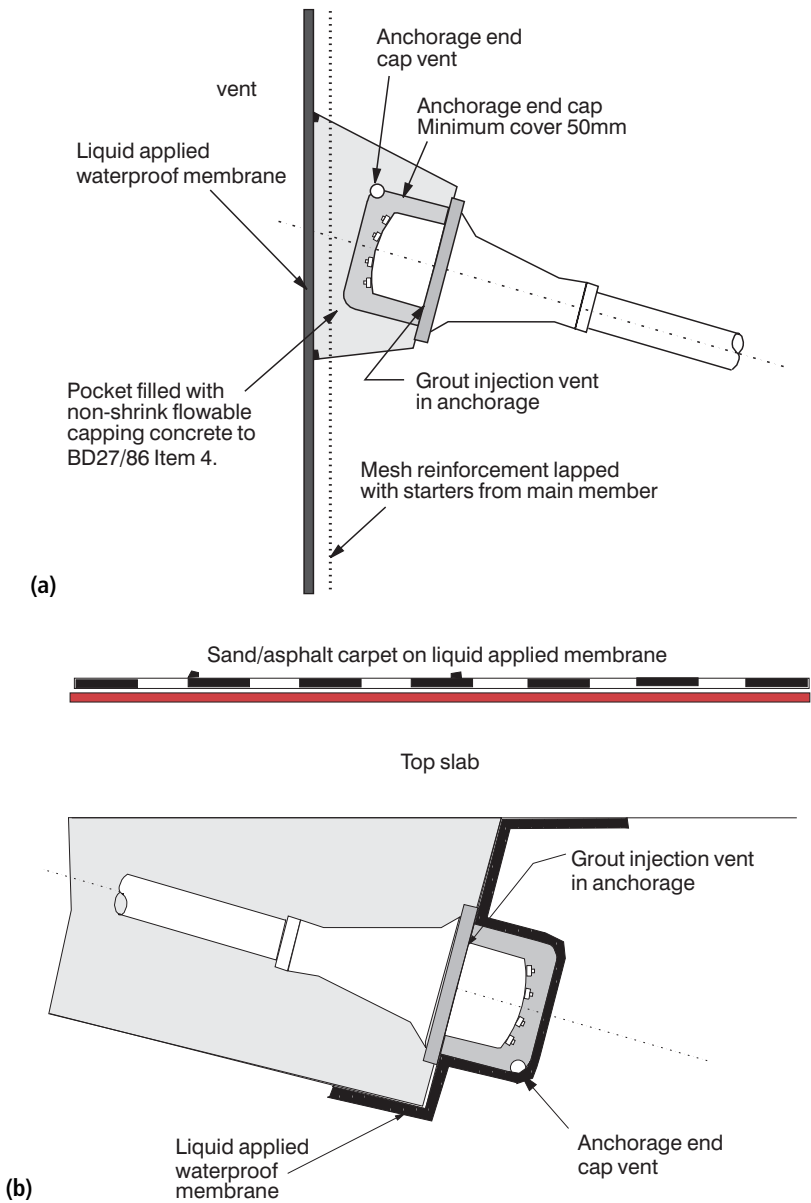
Figure 10.12 Durability details at anchorages.
