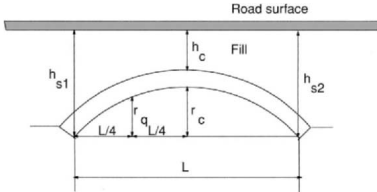
Figure 3B.1 Arch idealization for MEXE method.
