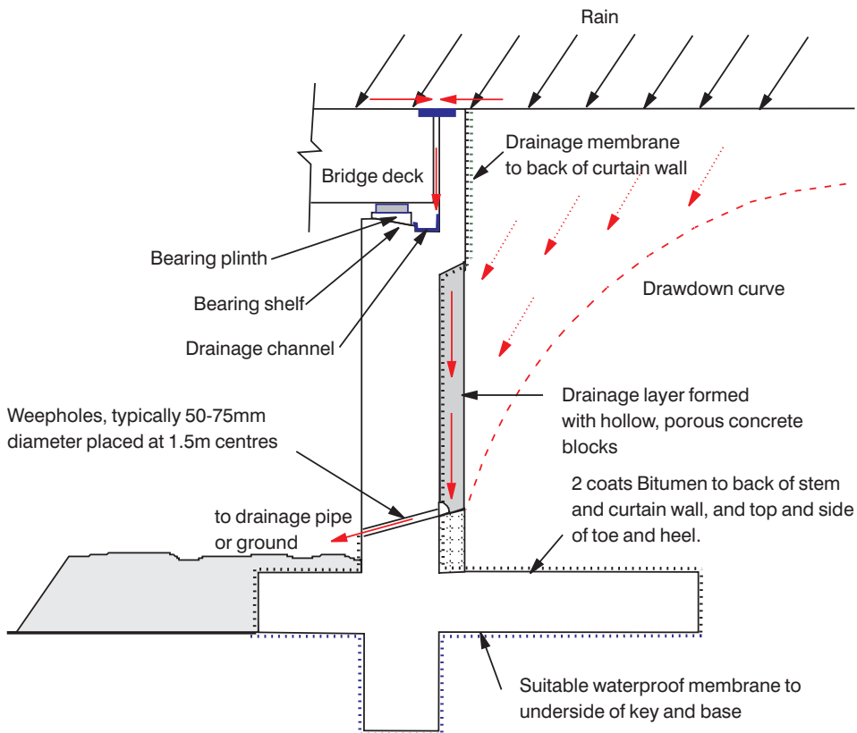
Figure 10.4 Drainage details to abutment.
