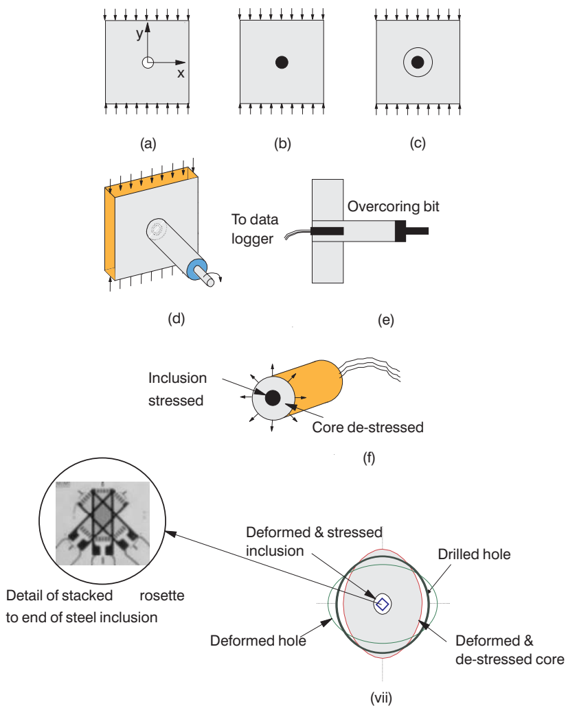
Figure 11.7 Standard inclusion method.
