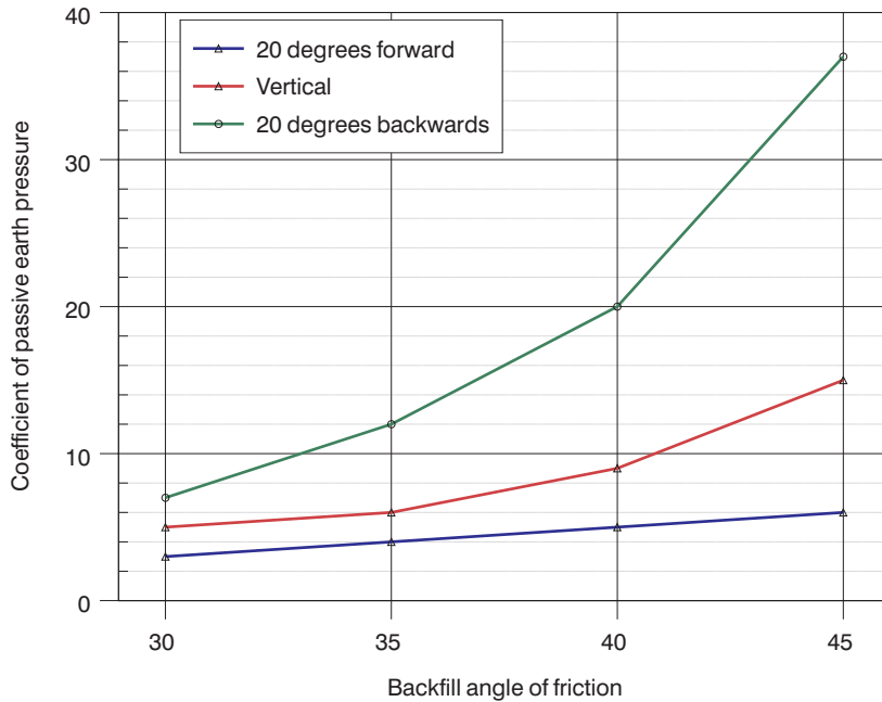
Figure 10.16 Variation of coefficient of passive earth pressure.
