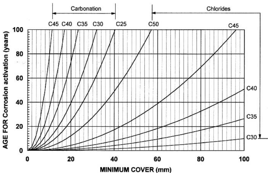
Figure 9.5 Design chart for durability.
