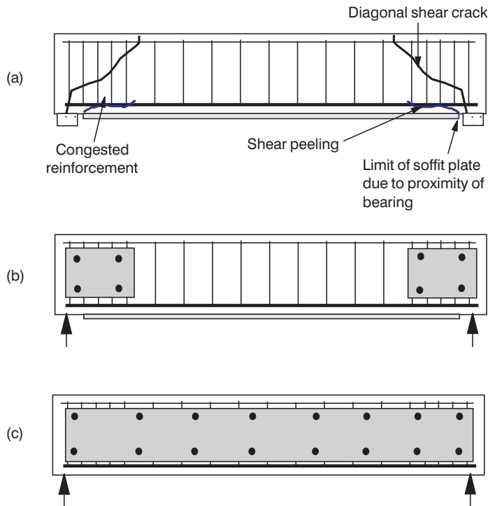
Figure 7.7 Alternative plate bonding solutions.
