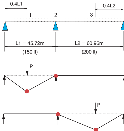
Figure 12.9 Continuous bridge example.
