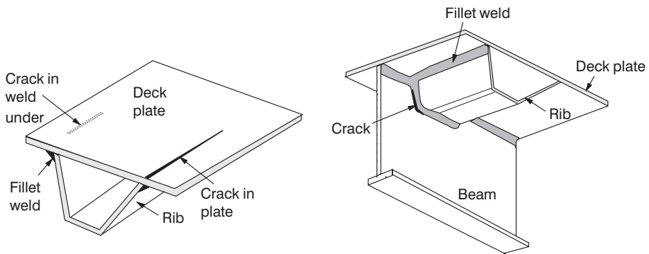
Figure 6.12 Cracking in orthotropic plate decks (after Mehue, 1990).
