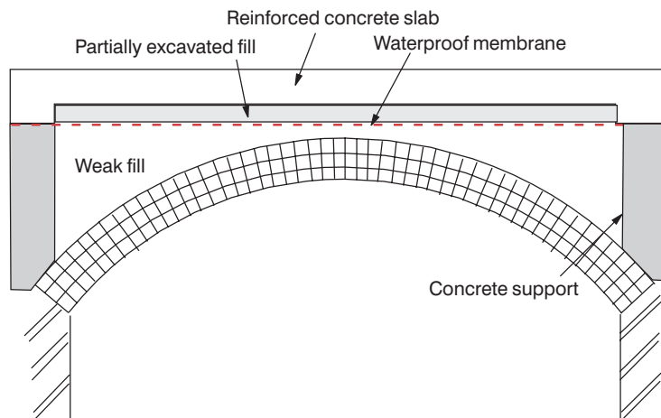
Figure 7.21 Overslabbing.
