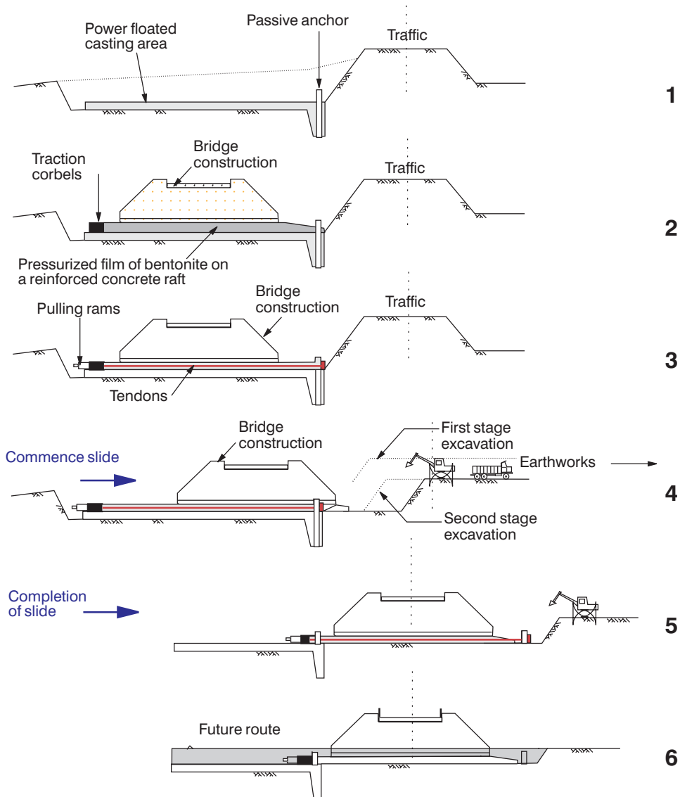
Figure 8.24 Autoripage sliding system (after Hughes, 1999).
