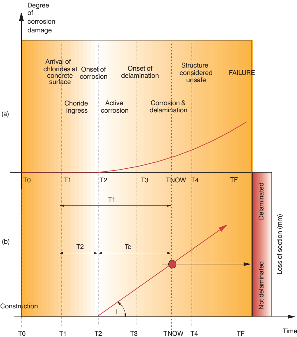
Figure 9.6 Deterioration process for external chloride contamination (top half); and calibration of the deterioration model (bottom half).
