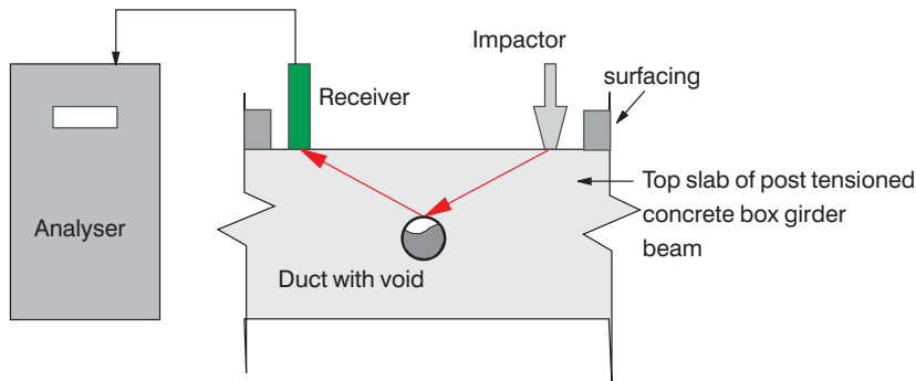
Figure 4.22 Typical impact echo set-up.
