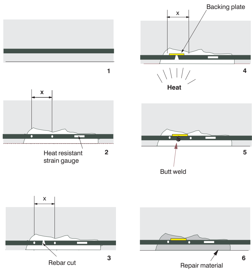
Figure 11.11 Cut bar procedure.
