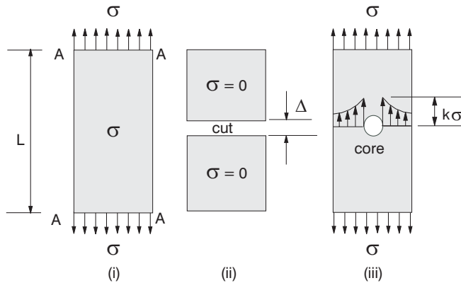
Figure 11.1 Stress relief principle.
