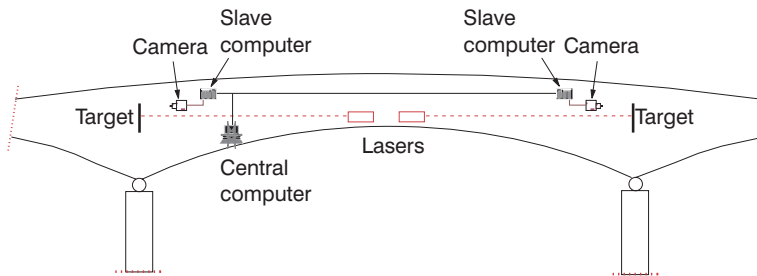
Figure 11.22 Measurement of deflection at the centre of the main span of the Foyle Bridge using lasers (after Sloan et al. , 1990).
