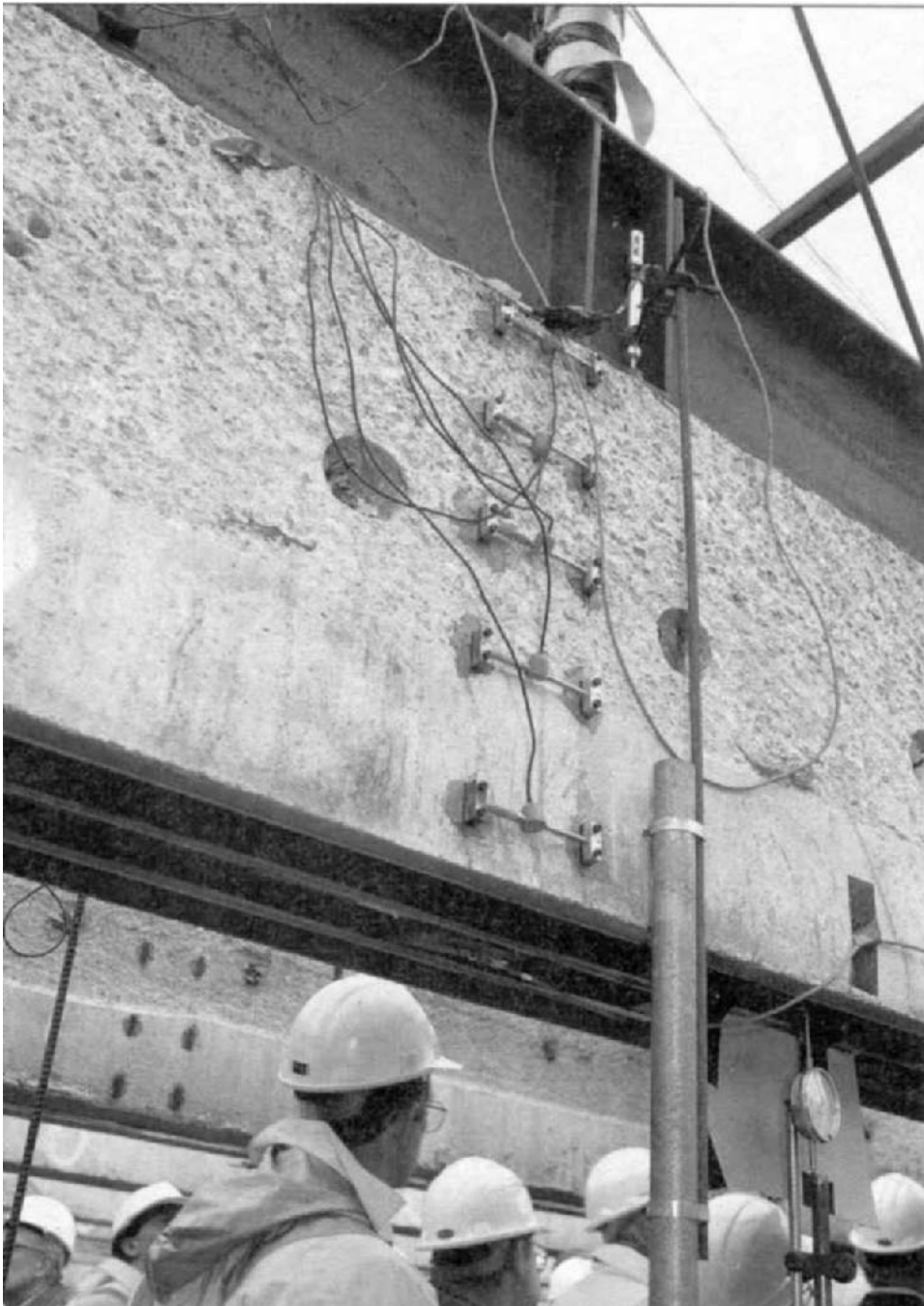
Figure 5.8 Typical VW gauges and displacement transducer in use ( New Civil Engineer , 1996).
