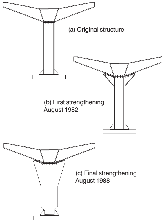
Figure 7.36 Strengthening of a steel pier.
