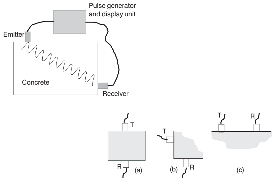
Figure 4.6 Transmission modes (a) direct; (b) semi-direct; (c) indirect.
