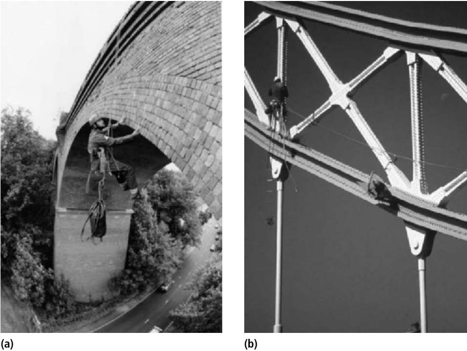
Figure 2.23 (a) Inspection of a brick arch barrel (courtesy of Up and Under) and (b) inspection of Tower Bridge, London (courtesy of Up and Under) (see colour plate section).
