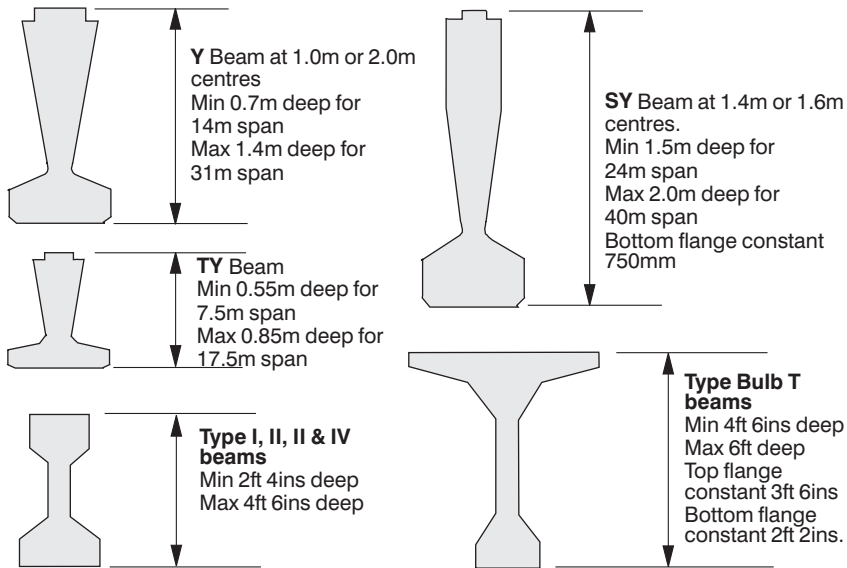
Figure 8.10 Y, SY and TY beams, and types I–IV and bulb T beams.
