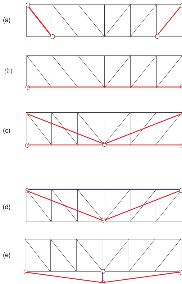
Figure 7.17 Tendon configurations for post-tensioned trusses (after Xanathos 1996).
