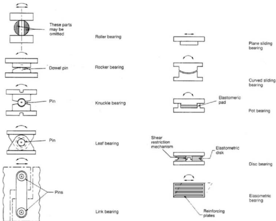
Figure 2.15 Different bearing types (Lee, 1994).
