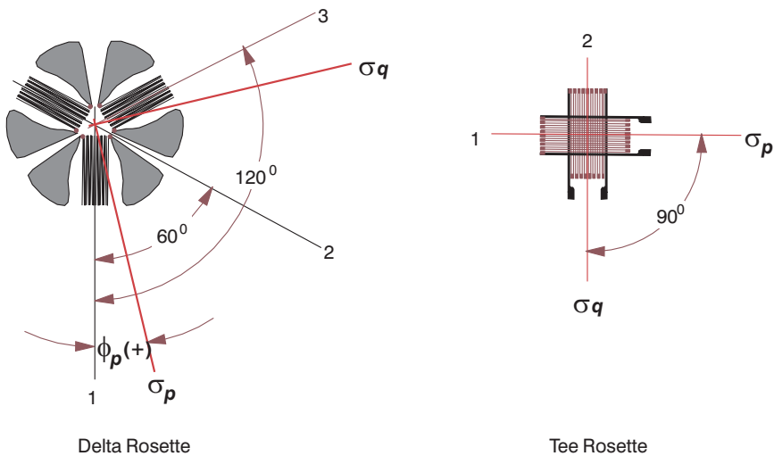
Figure 11.18 Layout of typical rosette gauges.
