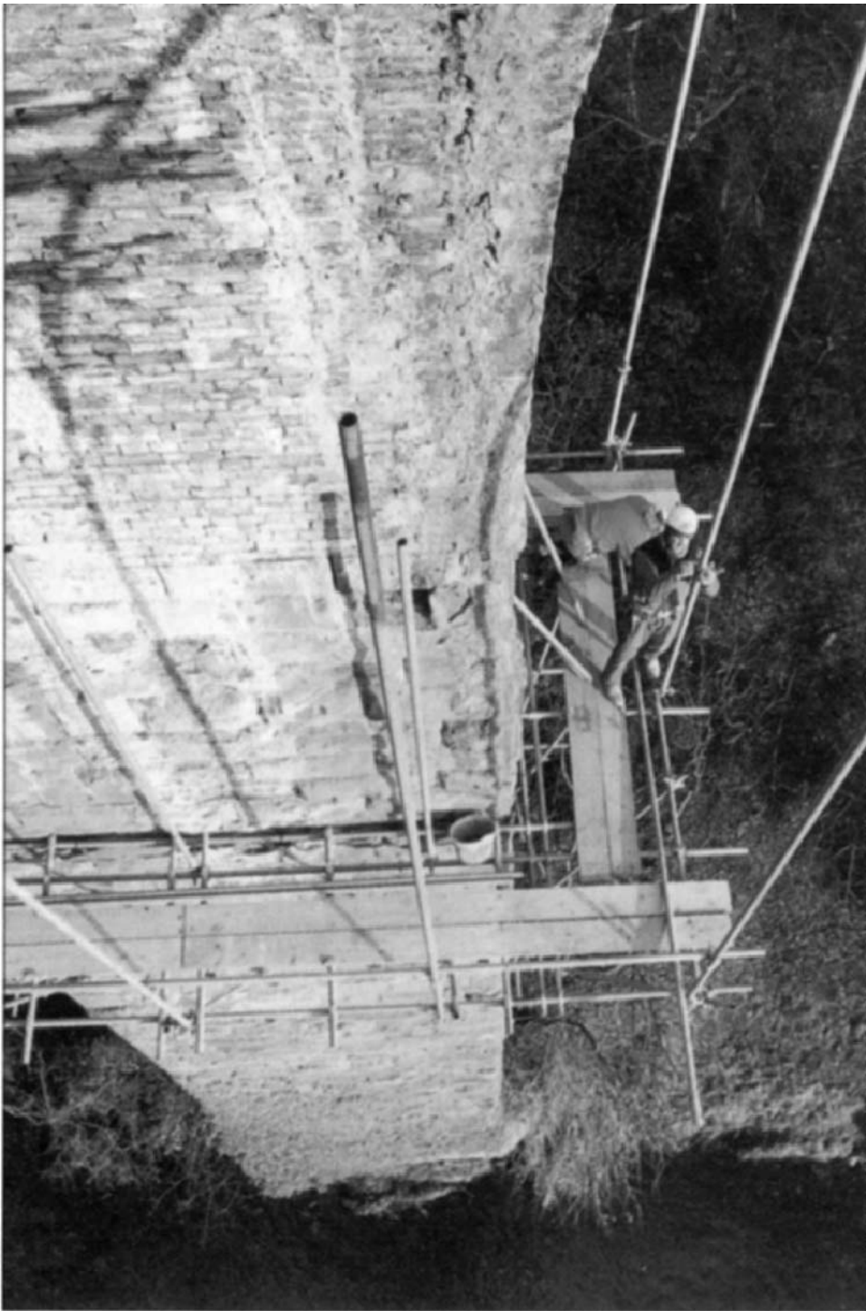
Figure 6.2(a) Suspended scaffolding to viaduct pier.
