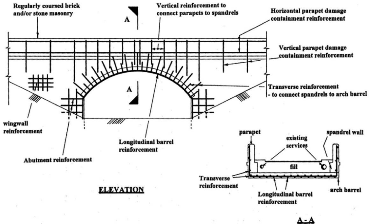
Figure 7.22 Proposed retro-reinforcement for a typical single span masonry arch bridge (after Garrity 1995, p. 561).
