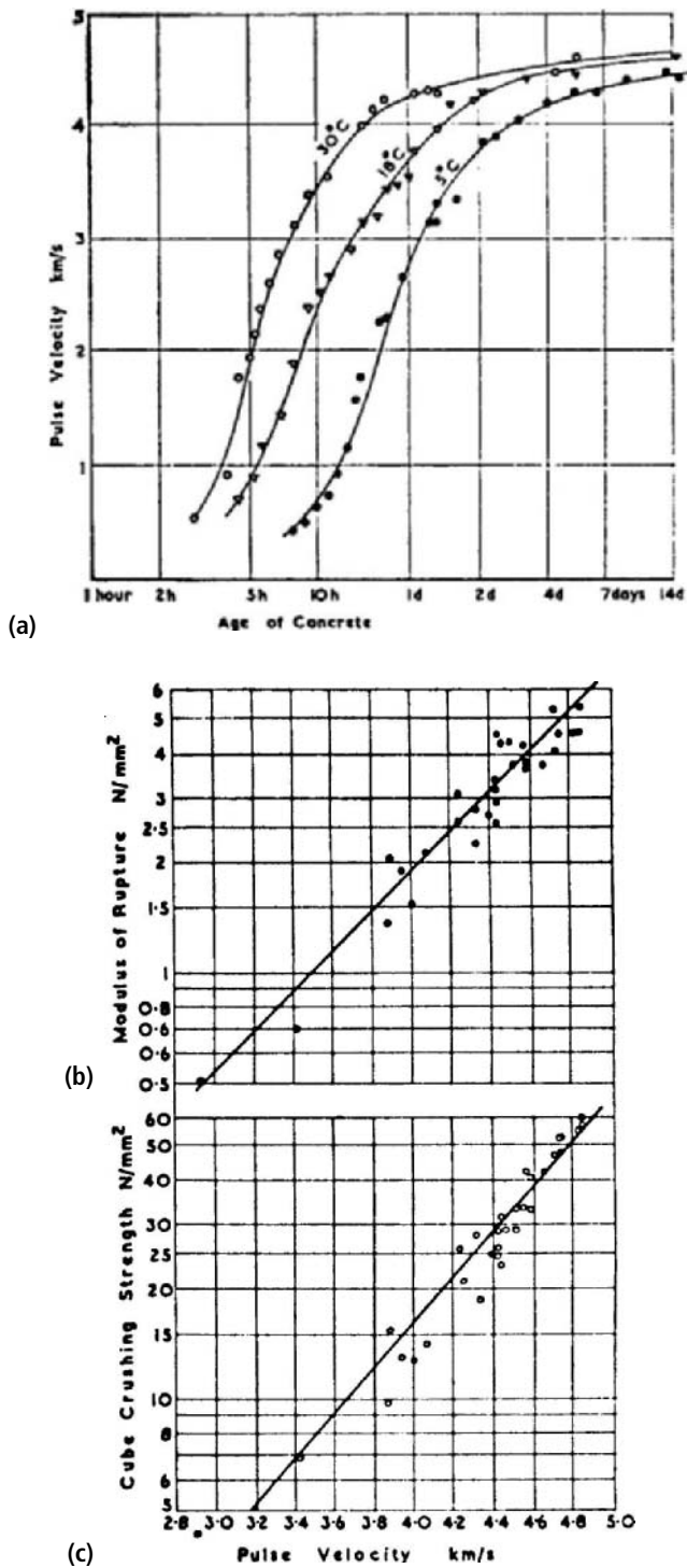
Figure 4.7 (a,b,c) Correlation charts for cube strength; age and Modulus of Rupture.
