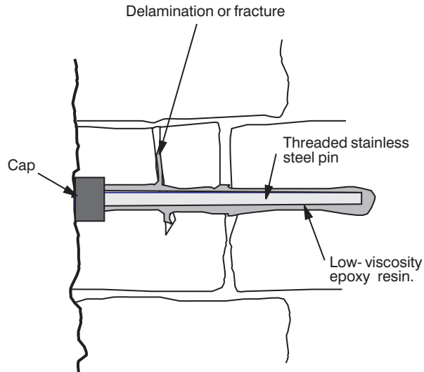
Figure 6.3 Pinning technique.
