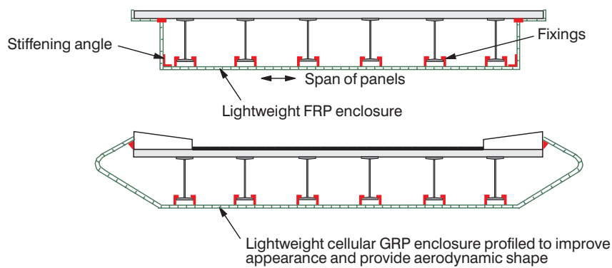
Figure 8.25 Enclosure principle.
