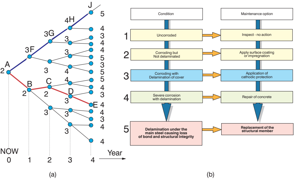
Figure 9.9 Relationship between the Markov Chain and maintenance options.
