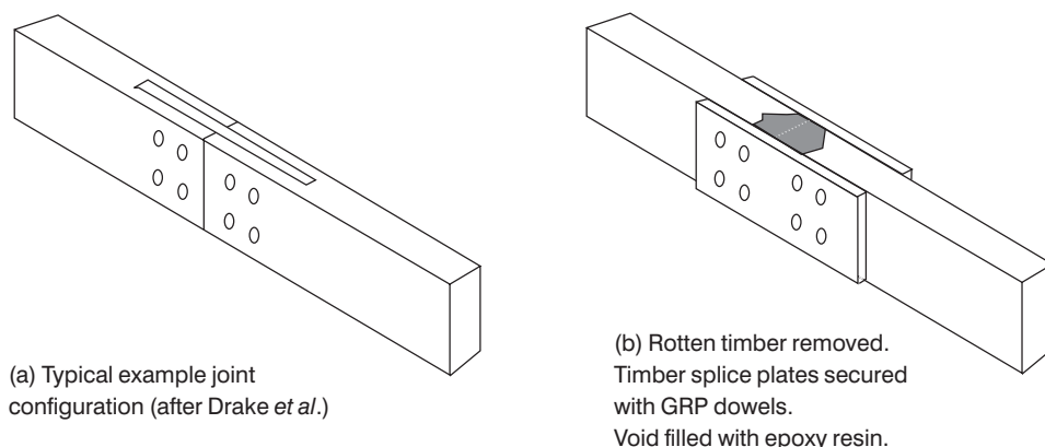
Figure 6.18 (a,b) Typical joint configuration.
