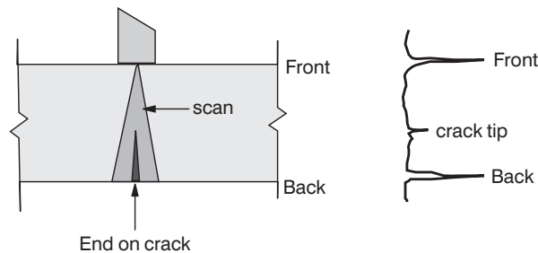
Figure 4.28 Use of a low-noise probe.
