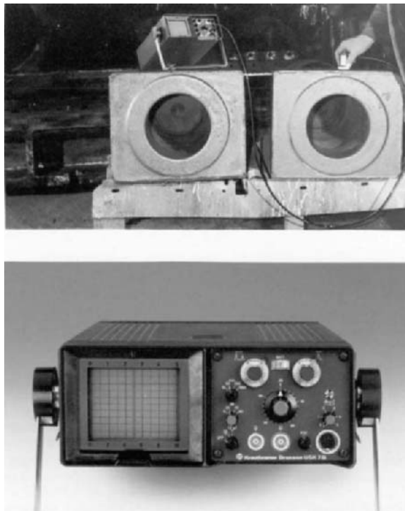
Figure 4.30 Typical MPI set-up on a bridge (courtesy of M. Neave).
