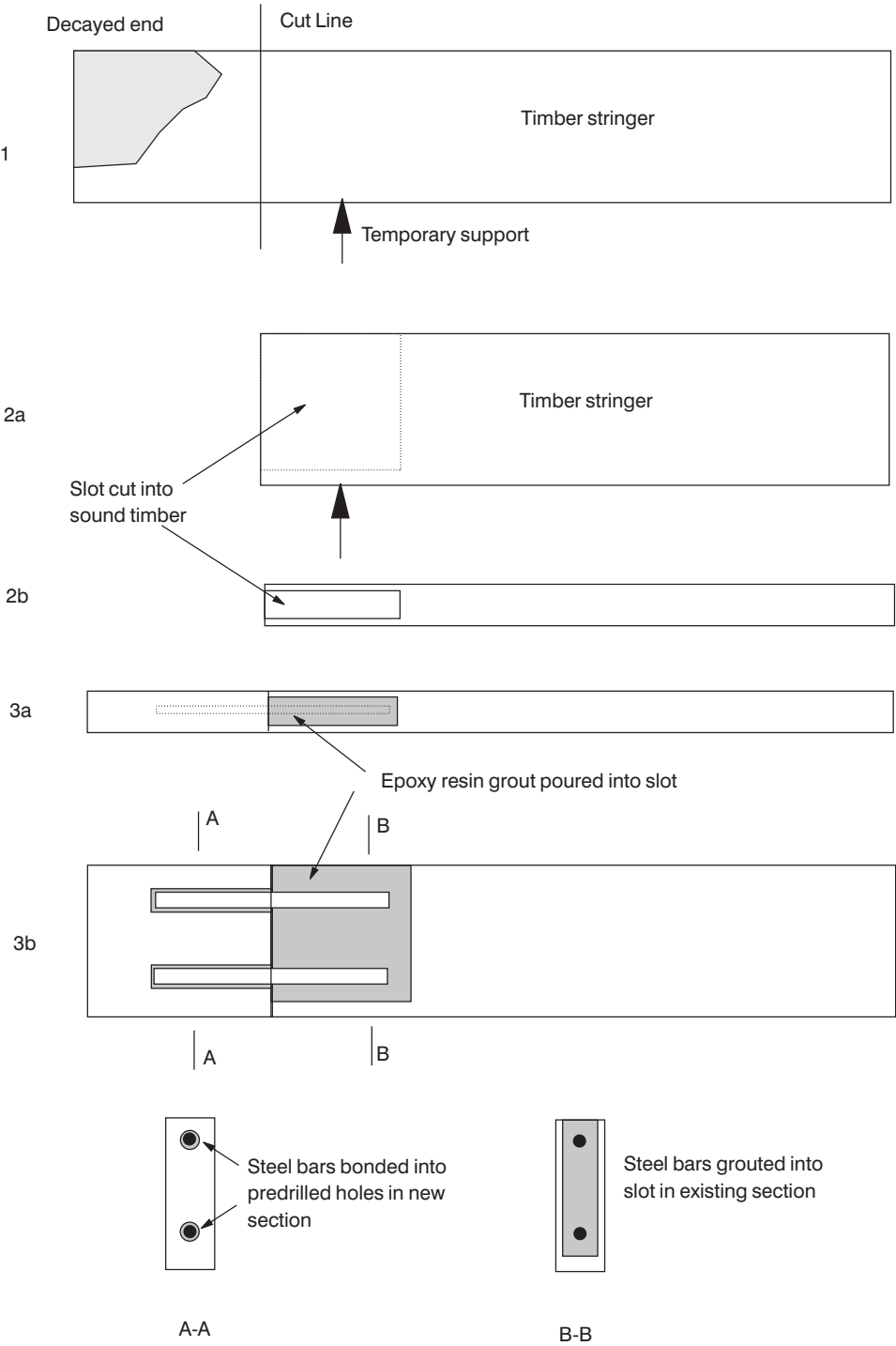
Figure 6.19 General procedure for steel bar/epoxy resin repair.
