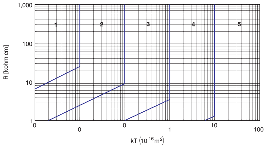
Figure 4.11 Nomogram for determining quality class of moist concrete (after Torrent and Frenzer, 1995).
