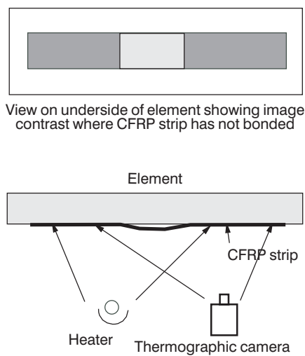
Figure 4.20 Principle of infrared thermography.
