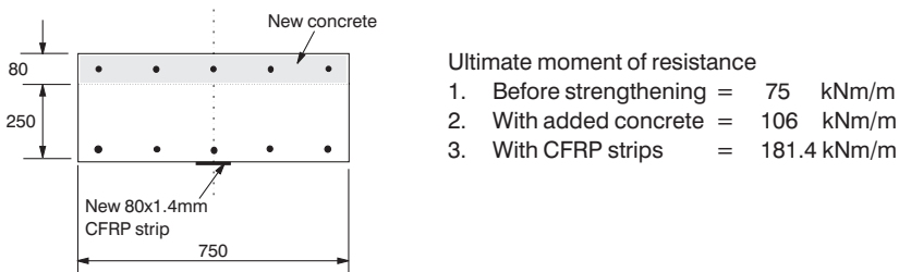
Figure 7.9 Typical section of a strengthened bridge deck using CFRP.
