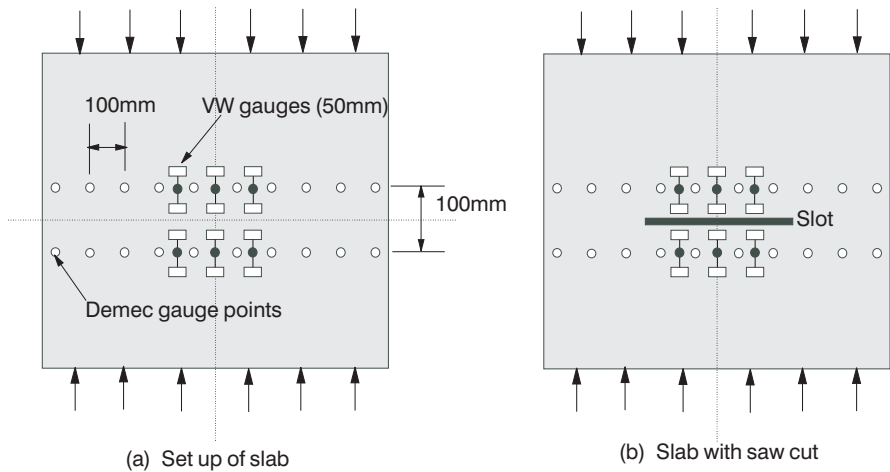
Figure 11.5 Saw cutting method.
