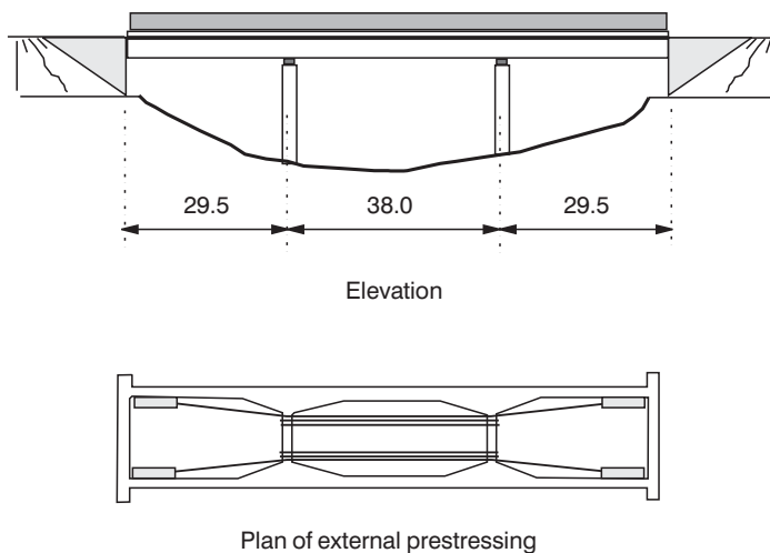
Figure 7.15 Strengthening of Sachsengraben Bridge (after Ivanyi and Buschmeyer 1996).
