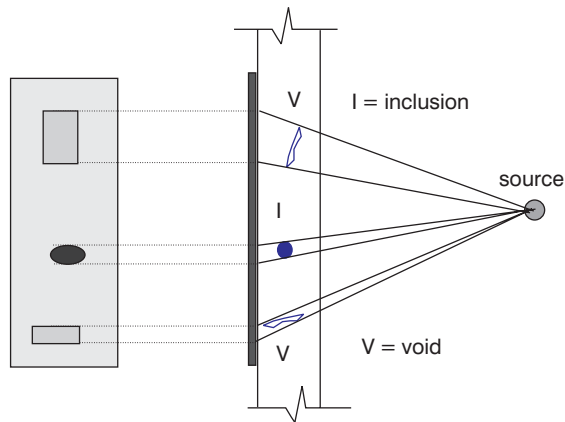
Figure 4.32 Principle of radiography.
