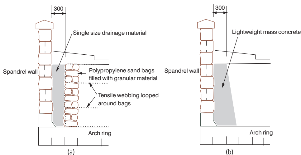
Figure 6.5 Mass concrete fill and reinforced earth repair options for bulging or displaced spandrel walls.
