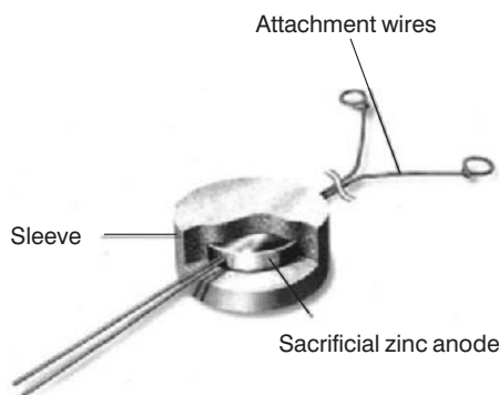
Figure 10.9 Sacrificial anode system for use in patch repairs (Fosroc Systems).
