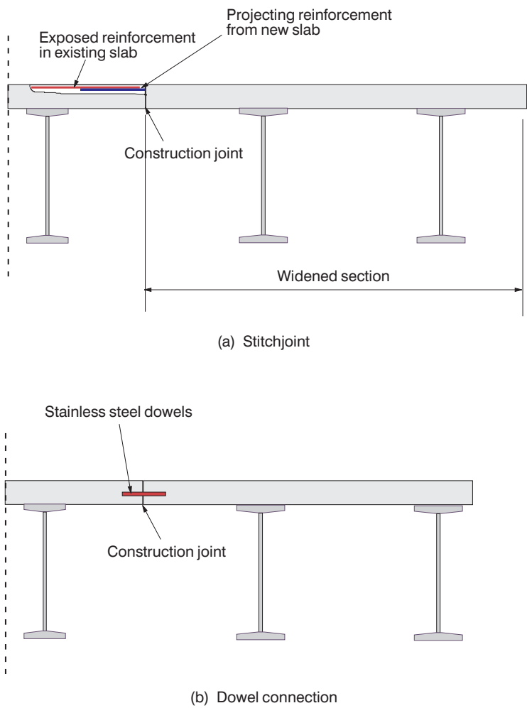
Figure 8.6 Connection of new to old.
