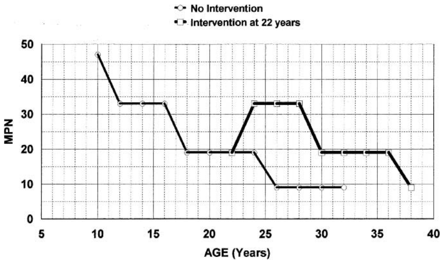
Figure 2.26 Deterioration model (no intervention).
