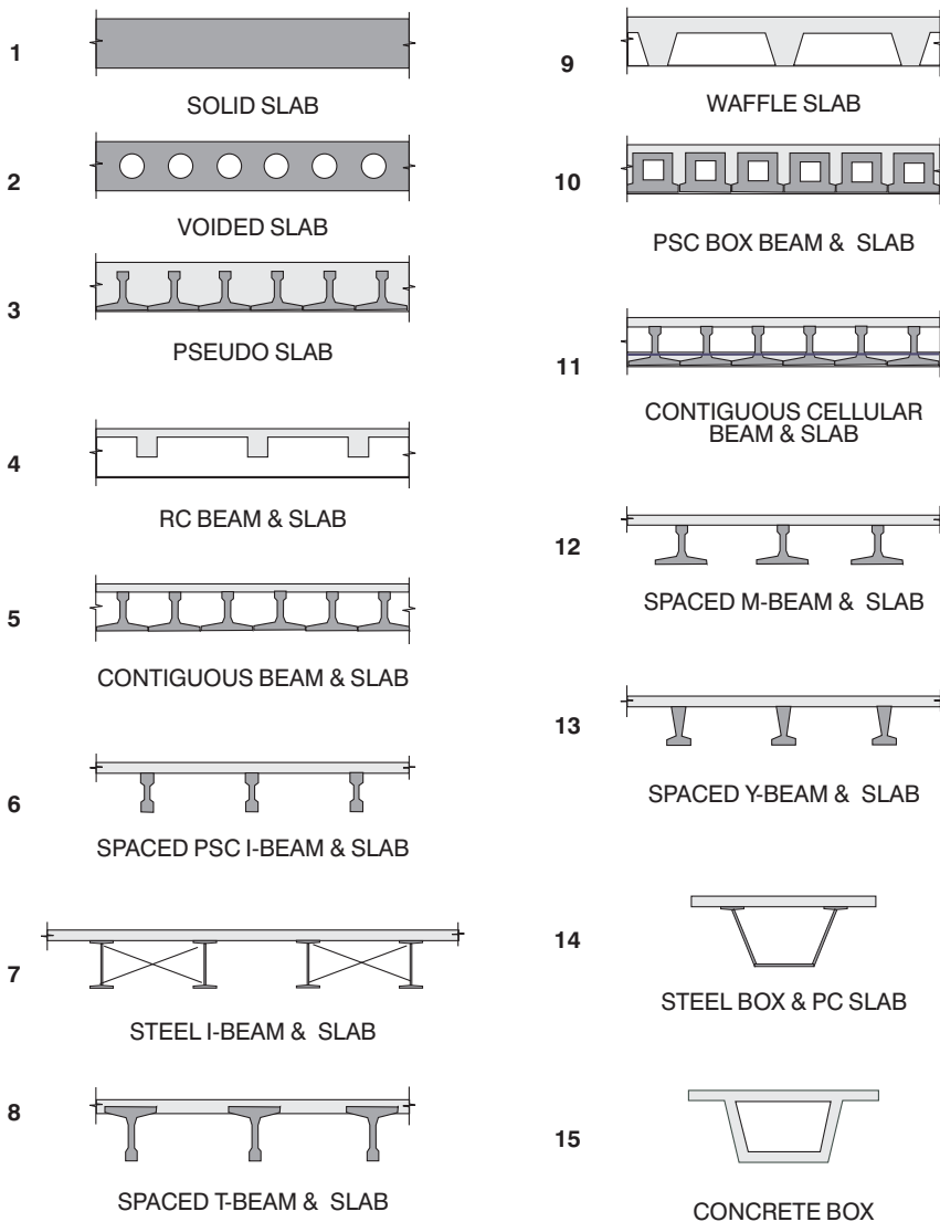
Figure 8.7 Bridge deck types.
