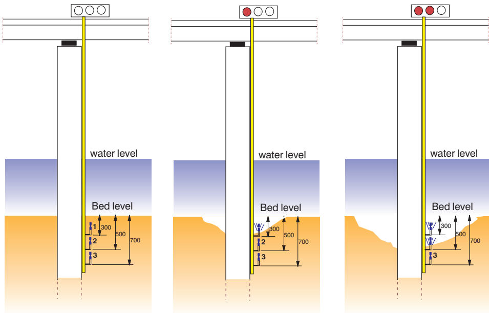
Figure 11.24 Buried motion sensors to monitor scour.
