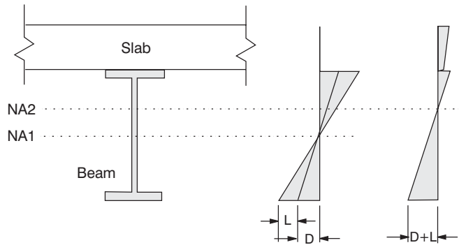
Figure 7.26 Stress distribution in non-composite beam and slab bridges.
