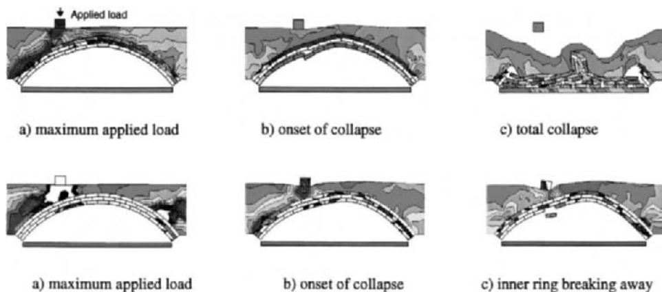
Figure 7.24 Predicted modes of collapse (see colour plate section).
