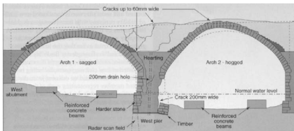
Figure 6.1(c) extent of internal damage (Paxton 1998) (see colour plate section).
