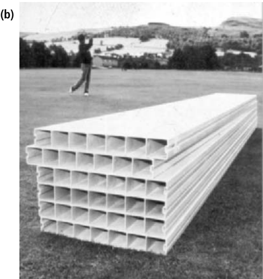
Figure 8.27 (a) ACCS Component data (courtesy of Maunsell Ltd.) and (b) GRP planks.
