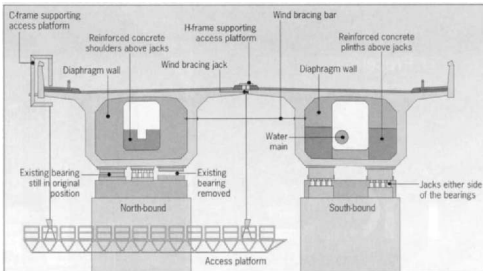
Figure 8.33 Orwell Bridge bearing replacement (Mylius 2000).
