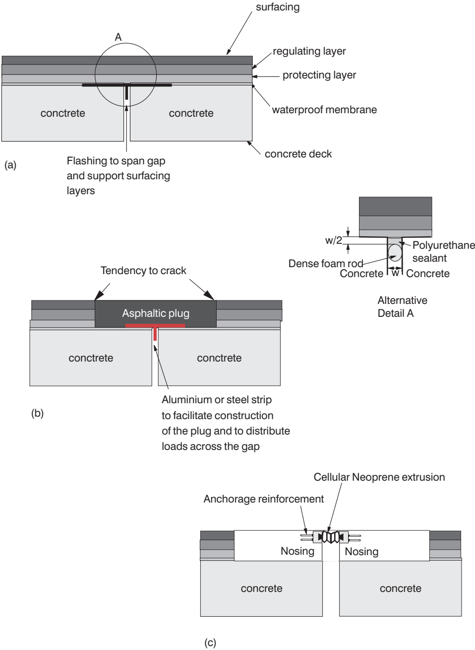
Figure 10.3 (a) Surface; (b) asphaltic plug, and (c) preformed extrusion between nosings.
