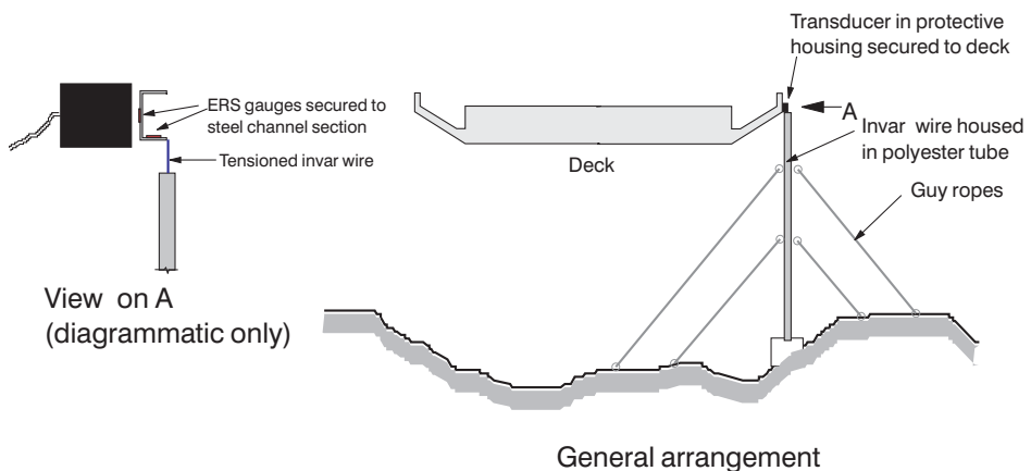
Figure 11.25 Transducer set-up.
