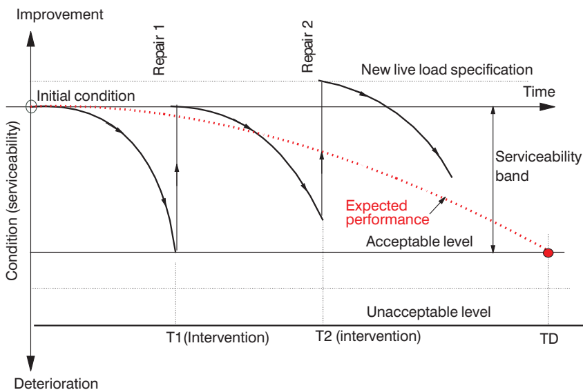
Figure 9.3 Deterioration model.
