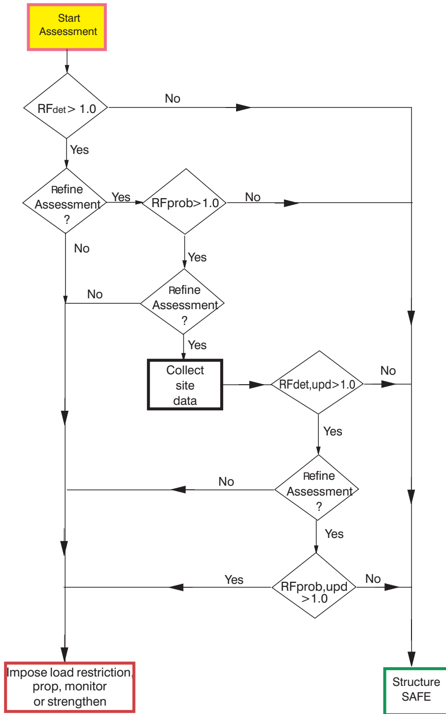
Figure 3.2 Bridge assessment flow diagram (after Bailey, 1996).
