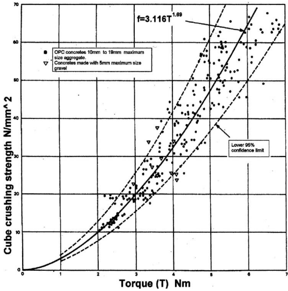
Figure 4.16 Calibration curves for natural aggregates.
