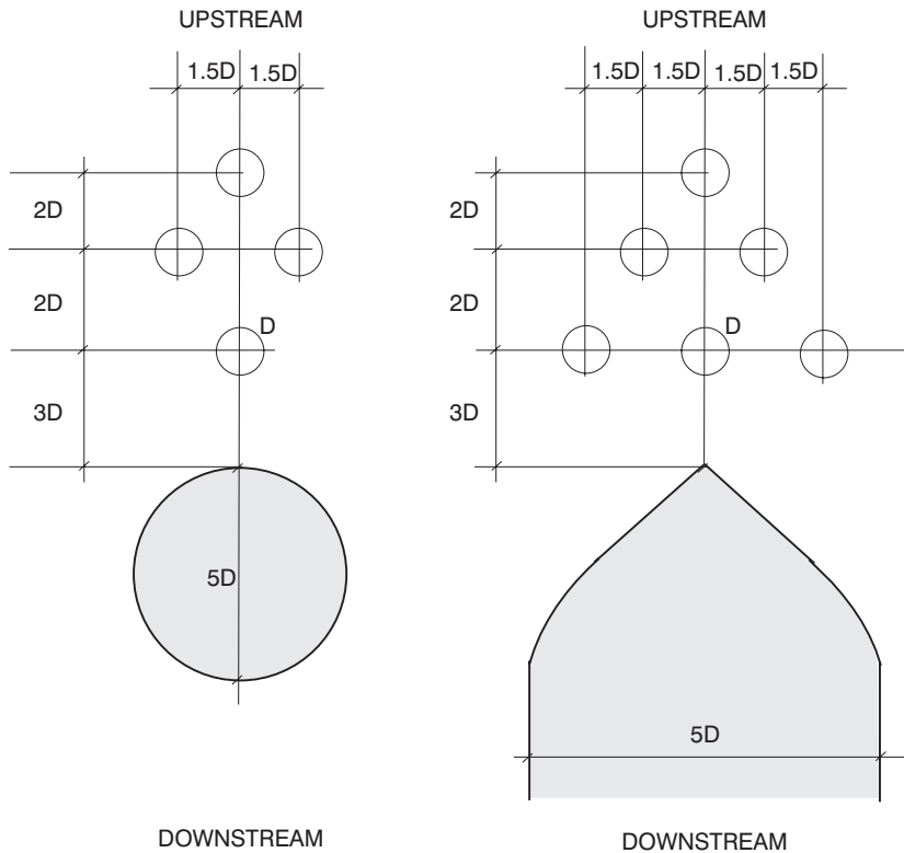
Figure 10.19 Scour protection using circular piles.
