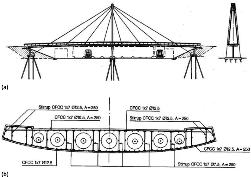
Figure 10.7 Herring footbridge, Denmark: (a) general arrangement; (b) cross-section through deck
