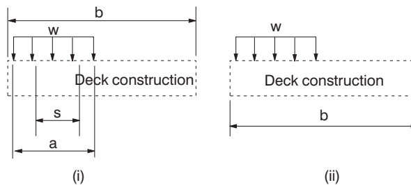
Figure 3.3 Strip analysis – upper and lower bound solutions.
