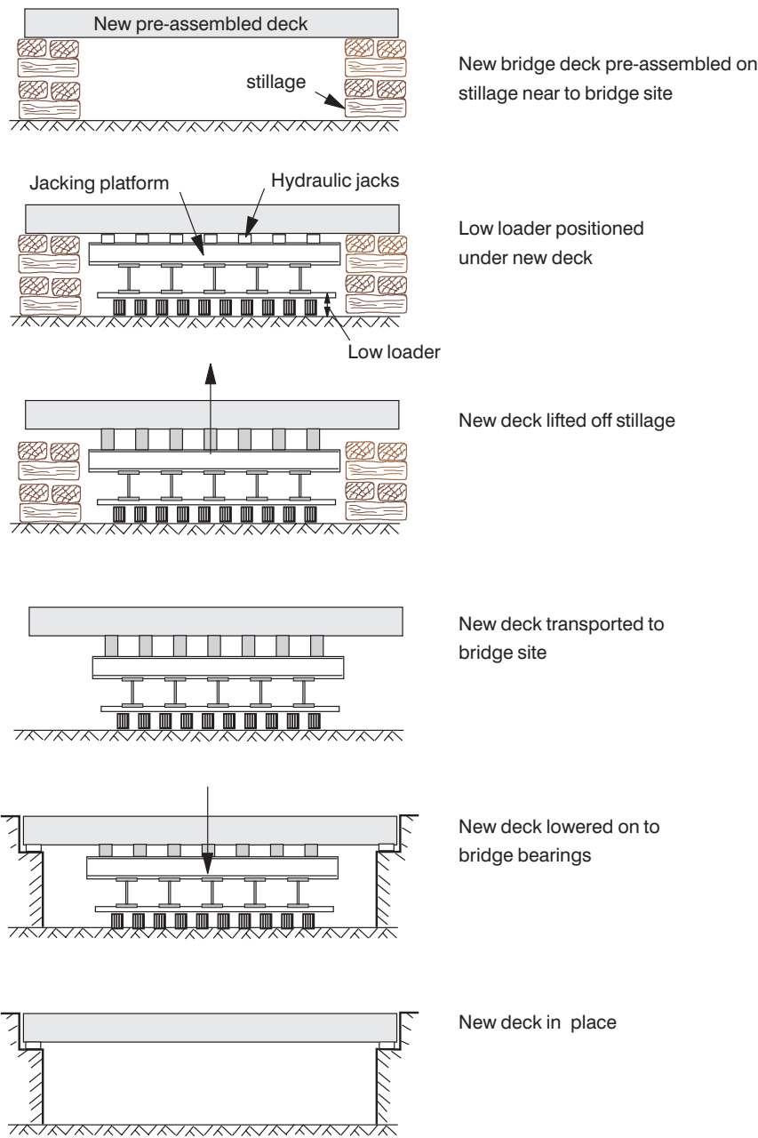
Figure 8.22 Low loader method.
