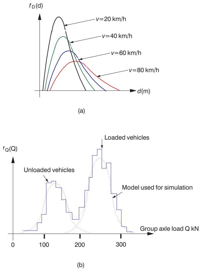
Figure 12.6 (a) Distance between vehicles in congested traffic, and (b) distribution of axle group weight.
