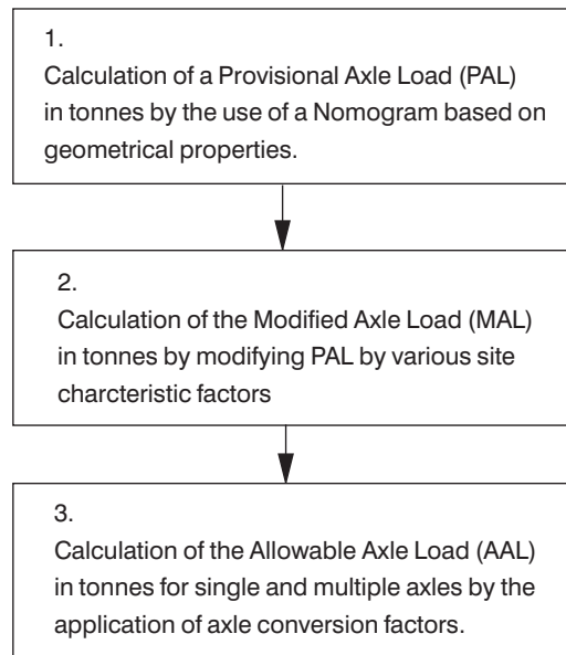
Figure 3.10 Steps in the MEXE method.
