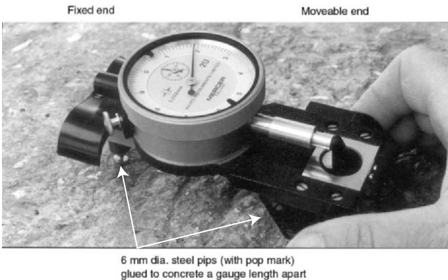
Figure 11.15 Mechanical (Demec) gauge.
