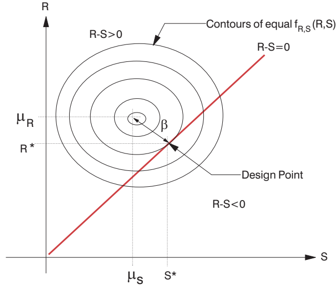
Figure 3.7 Failure zone with respect to joint probability distribution of R and S .
