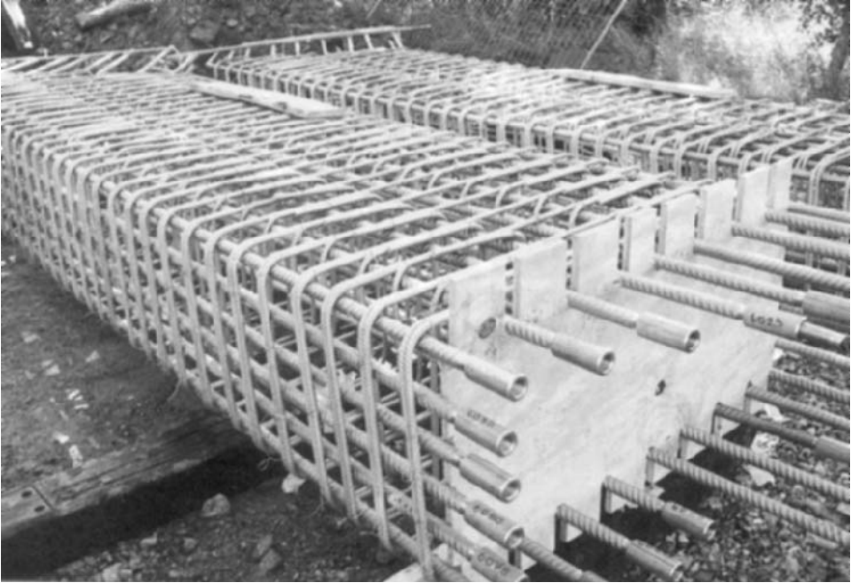
Figure 10.6 Stainless steel reinforcement cage for a bridge foundation (Abbott, 1999) (see colour plate section).
