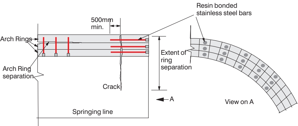
Figure 6.4 Tying of longitudinal cracks in arch ring.
