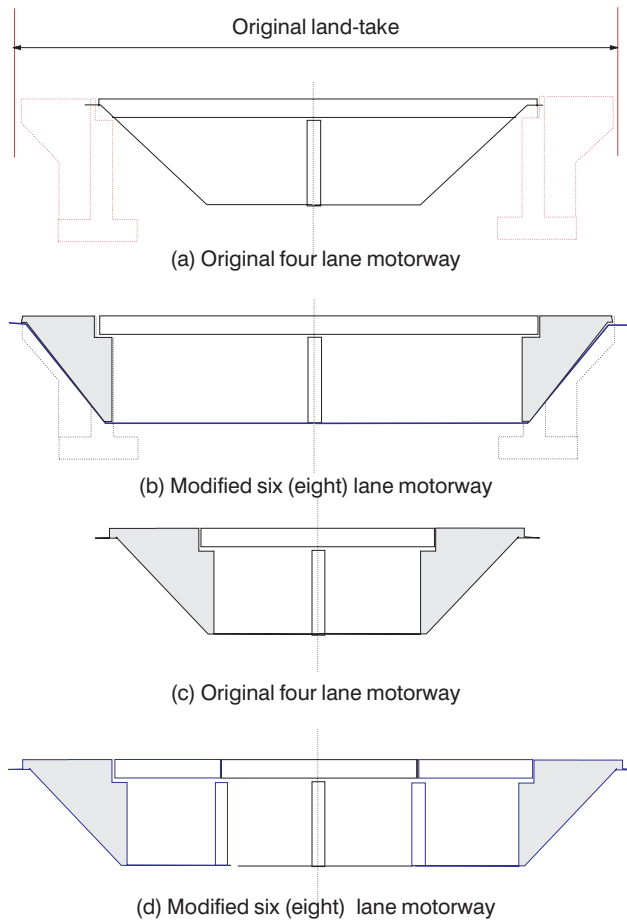
Figure 8.5 Widening at overbridge locations with open and closed abutments.
