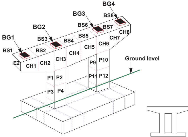
Figure 2.24 Example of segmental referencing.
