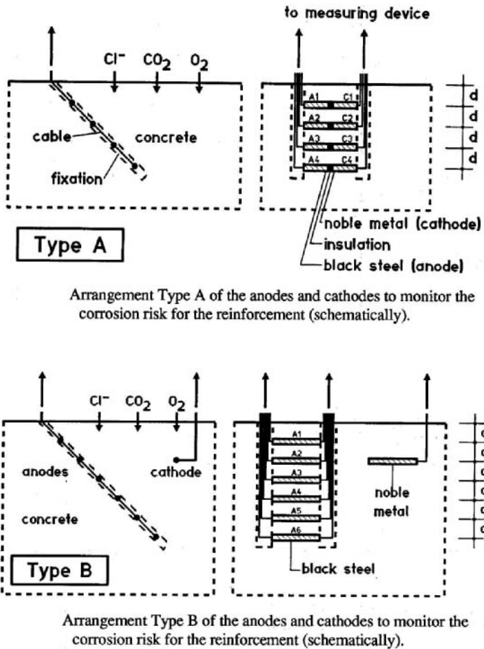
Figure 11.20 Type A and Type B arrangements (Schießl and Raupach, 1993).
