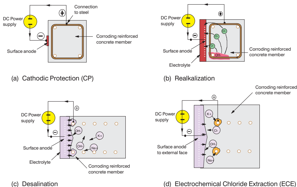
Figure 10.8 Principle of cathodic protection, desalination and realkalization.
