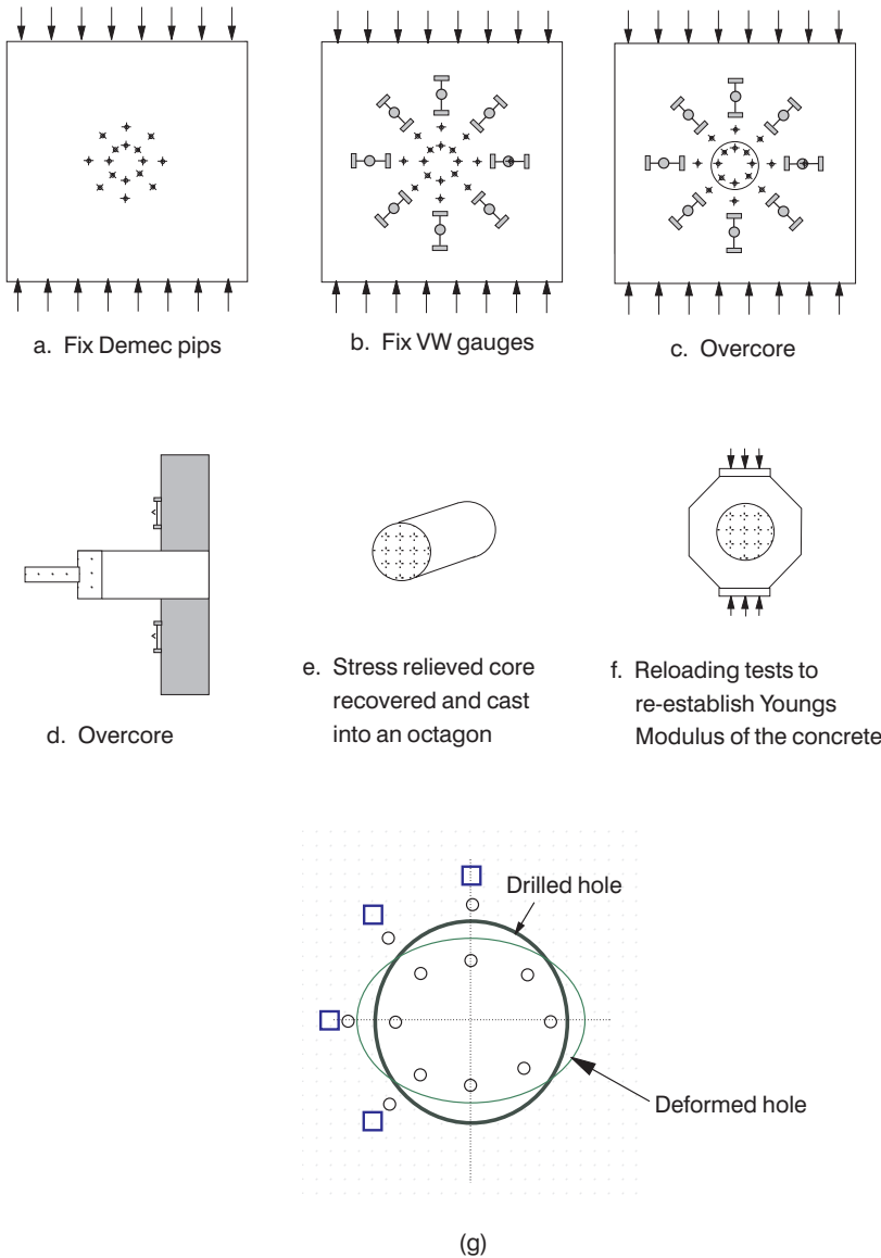
Figure 11.2 Standard overcoring method.
