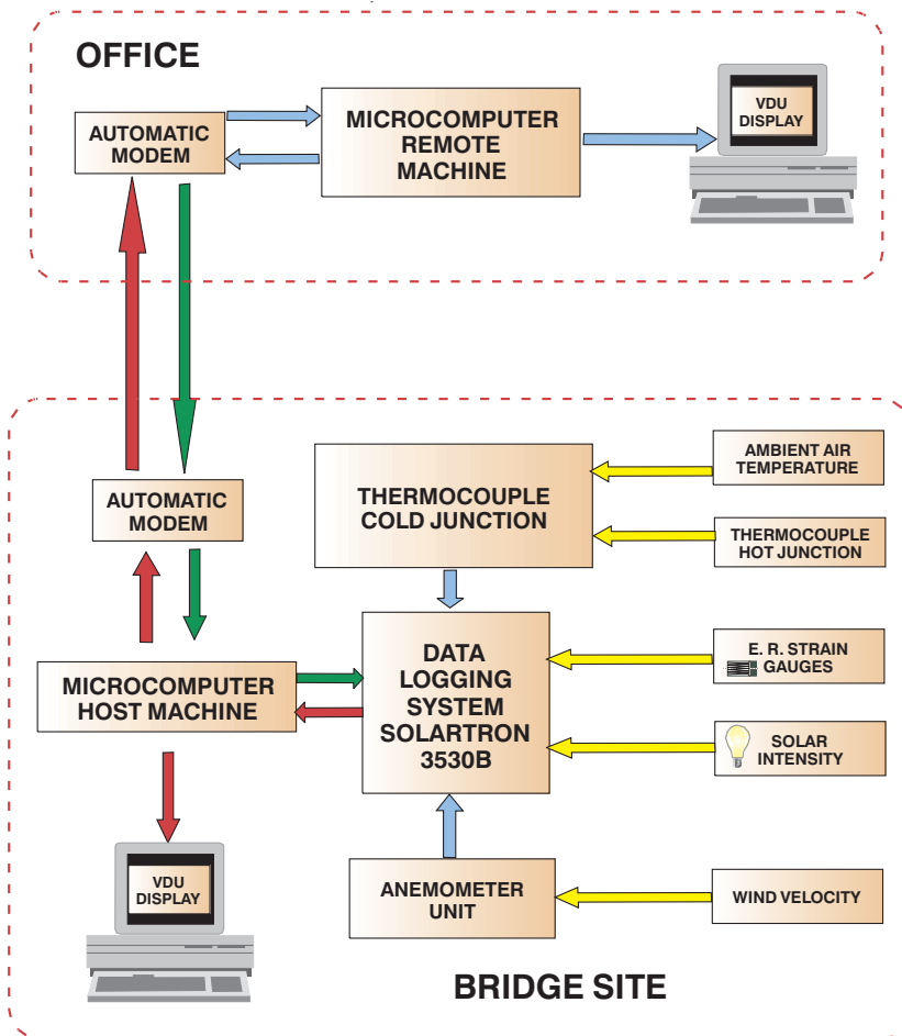
Figure 11.23 Data acquisition and telemetry system (after Sloan et al. , 1990).
