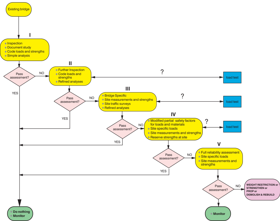
Figure 3C.1 Flow chart for utilizing assessment levels I–V.
