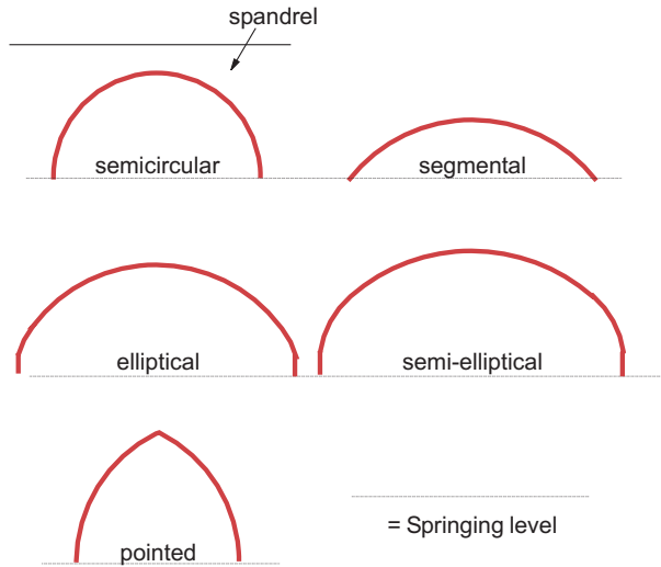
Figure 3.9 Different arch profiles.
