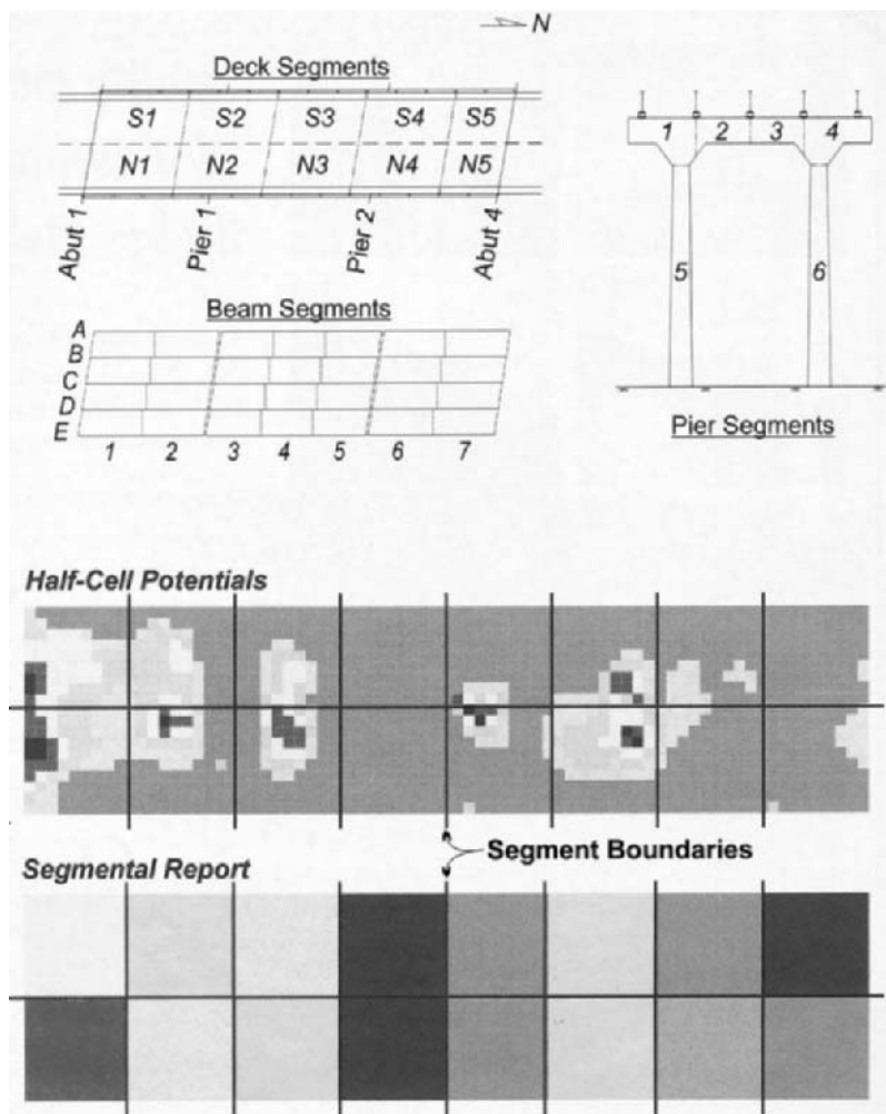
Figure 2.25 Segmental inspection of bridge elements (after Hearn, 1998).
