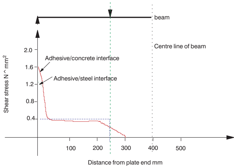
Figure 7.2 Shear stress distribution in a steel plated beam (Mays 1993, p. 674).
