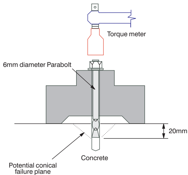
Figure 4.15 Fracture test arrangement.
