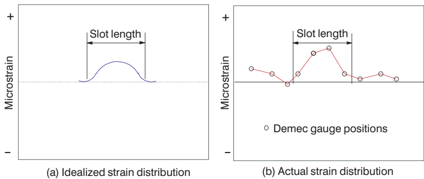
Figure 11.6 Comparison of ideal and actual strain distribution across a saw cut.
