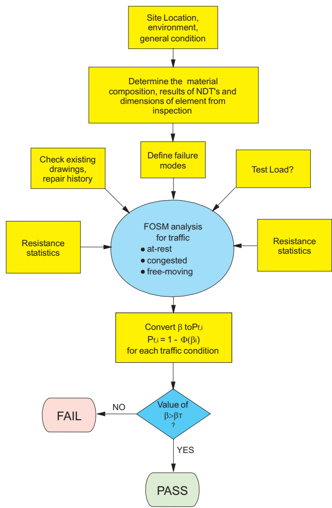
Figure 12.8 Typical reliability process.
