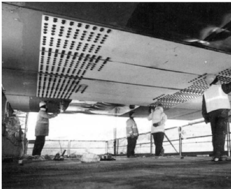
Figure 6.14 Fitting of doubler plates to the bottom flange ( Construction Repair , 1997).
