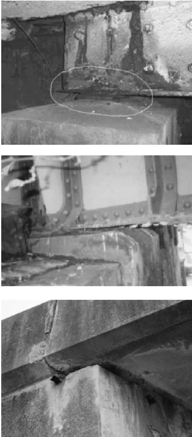
Figure 2.16 'Failing' bearings.
