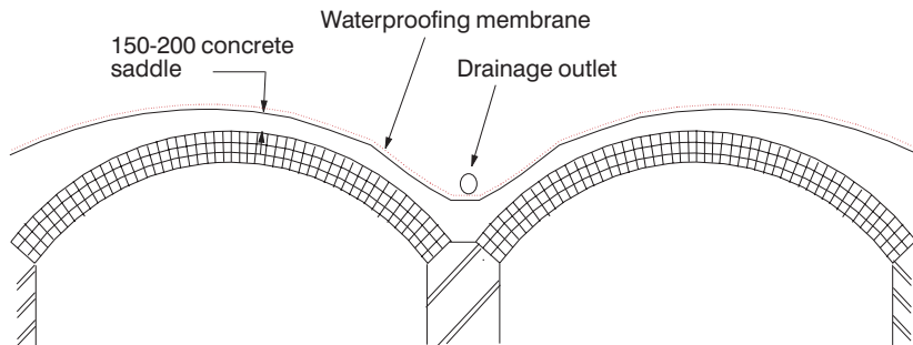
Figure 7.19 Typical saddle strengthening.
