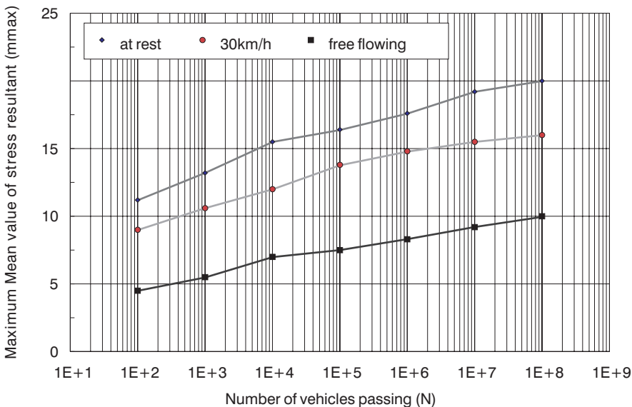
Figure 12.7 Mean maximum effect for different traffic conditions.
