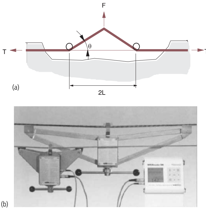
Figure 11.14 (a) Crossbow principle, and (b) crossbow instrument.
