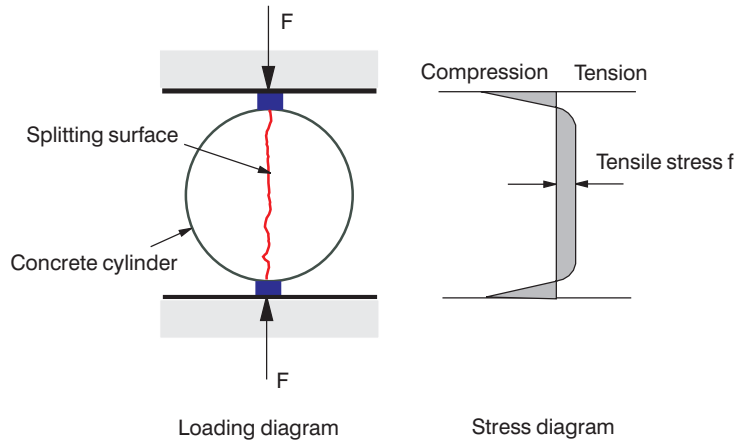
Figure 4.25 Typical set-up for tensile testing of a concrete cylinder.
