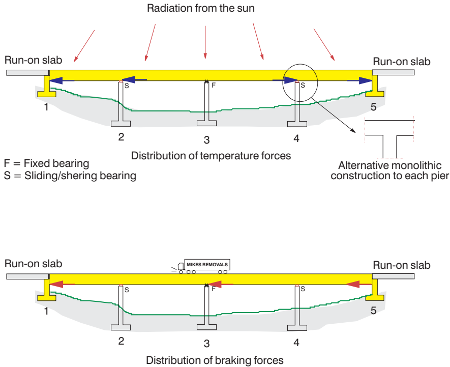
Figure 10.13 Principle of integral bridges (based on Hambly, 1992).
