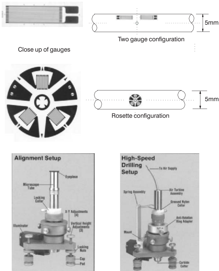
Figure 11.13 Gauge configurations and milling guide (courtesy of Measurements Group UK, Ltd.).
