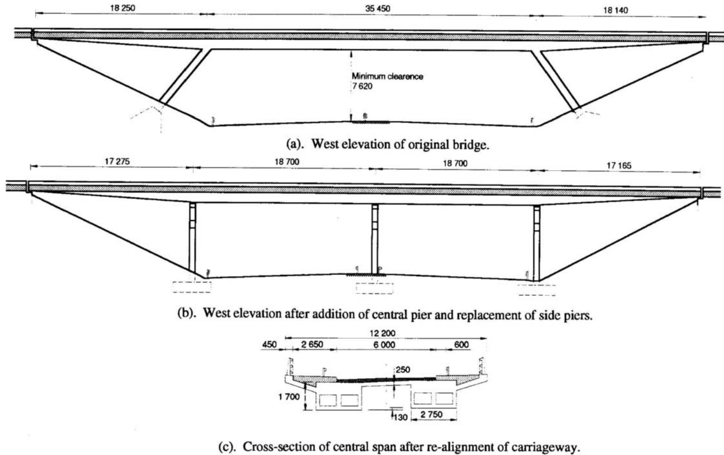
Figure 7.30 (a) West elevation of original bridge (b) west elevation after addition of a central pier and replacement of side piers and, (c) cross-section of central span after re-alignment of carriageway (Wall et al. , 1996).
