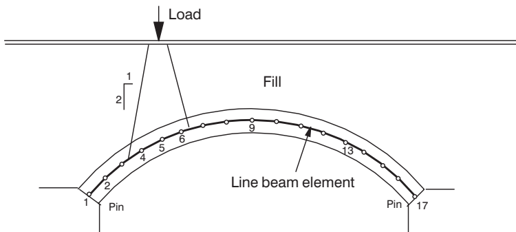
Figure 3.12 Typical line representation of arch barrel.
