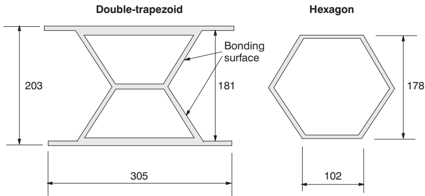
Figure 8.14 Modular FRP system.
