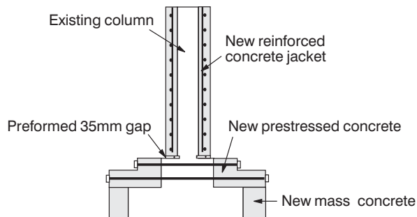
Figure 7.35 Strengthening of the columns to the Horsham Road Bridge.
