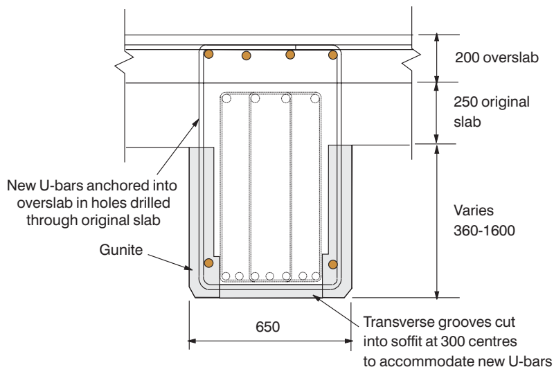
Figure 7.29 New shear reinforcement to the deck beams.
