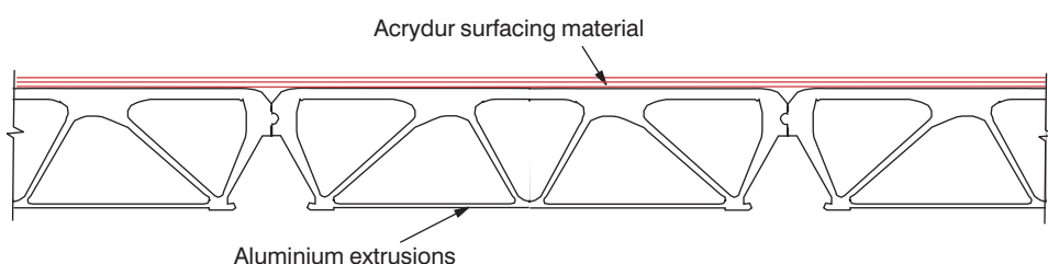
Figure 8.12 Section through aluminium bridge deck extrusion (after Svensson and Pettersson, 1990).
