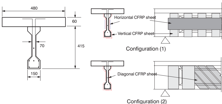
Figure 7.13 Details of CFRP shear reinforcement.
