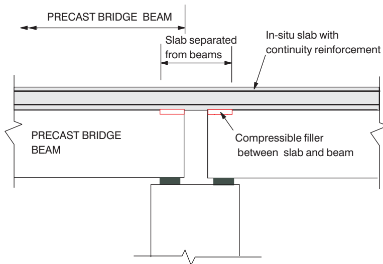
Figure 10.17 Type 4 – Continuous separated deck slab.
