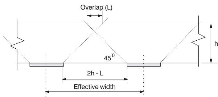
Figure 7.4 Effective width of slabs strengthened with steel plates.
