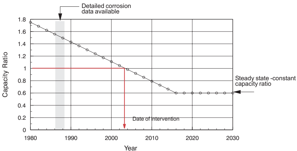
Figure 12.10 Deterioration model.
