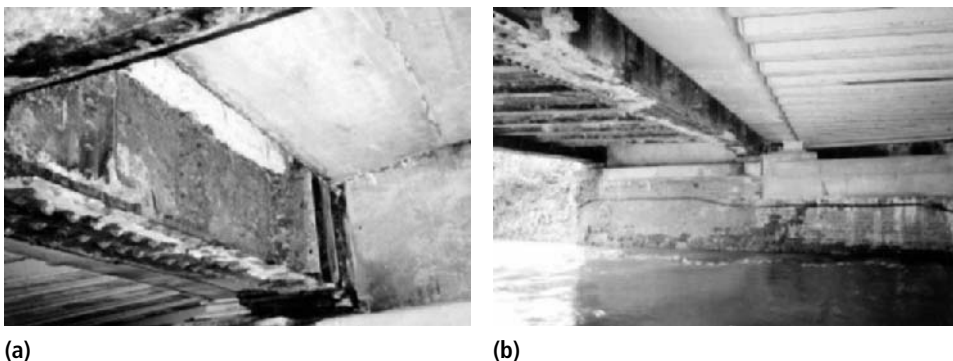
Figure 2.9 Severe rusting of steel superstructure (a) at a support, (b) main superstructure.
