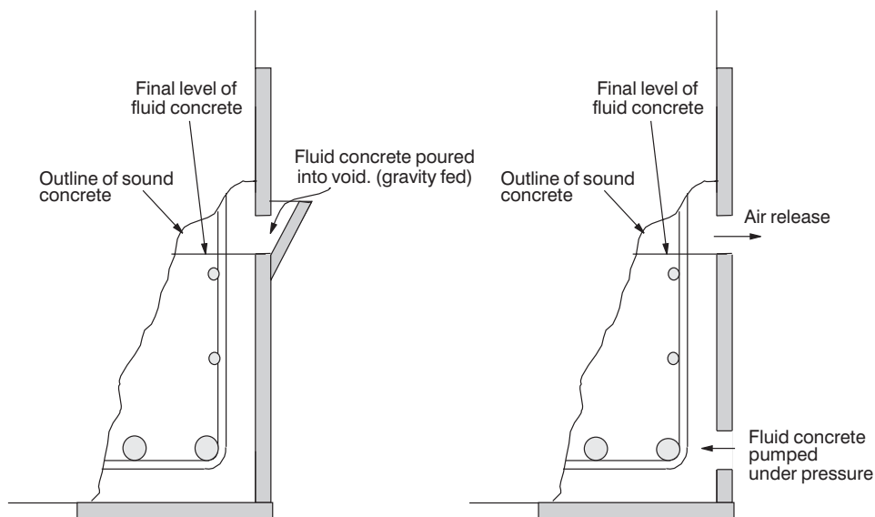
Figure 6.10 Traditional 'letter-box' arrangements for the application of fluid concrete to a beam element.
