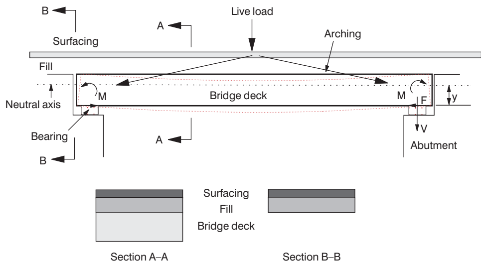
Figure 5.5 Effect of end restraint.
