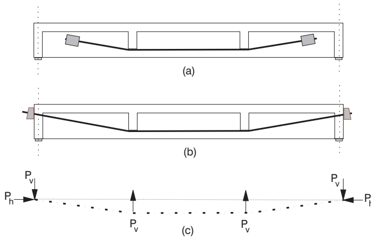
Figure 7.16 Bridge strengthening using externally applied inclined tendons.
