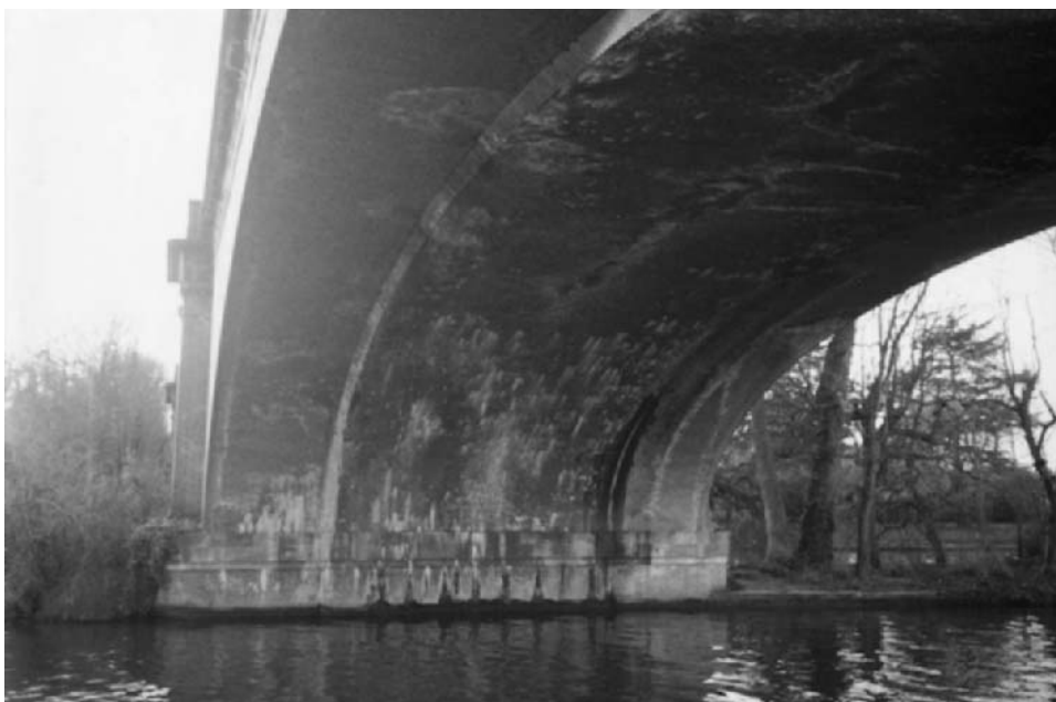
Figure 2.11 Leakage deposits on the barrel of an arch bridge (courtesy A.S. Glover).
