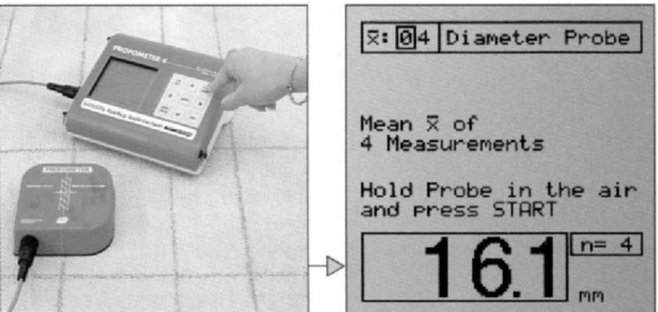
Figure 4.4 Typical rebar locator and visual display.
