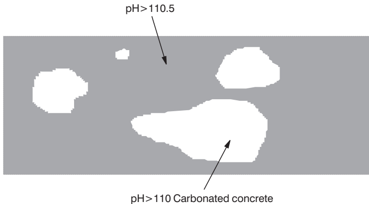
Figure 4.10 Results of a carbonation test.
