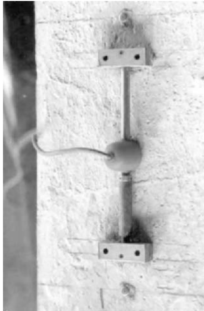
Figure 5.7 Typical vibrating wire gauges in use.
