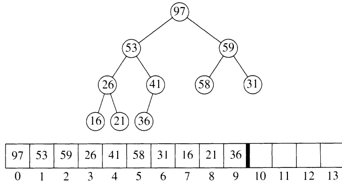
Figure 21.28 Max heap after the buildHeap phase.
