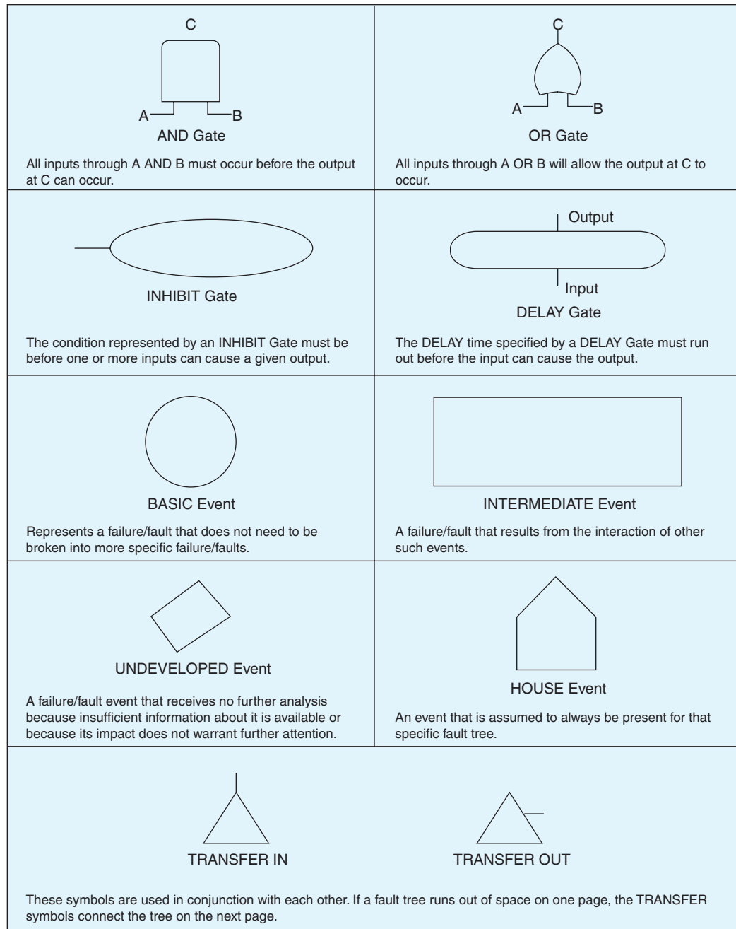
FIGURE 27-7 Symbols used in fault tree analysis.
