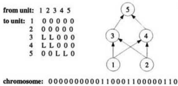
Figure 2.21: An illustration of Miller, Todd, and Hegde's representation scheme. Each entry in the matrix represents the type of connection on the link between the "from unit" (column) and the "to unit" (row). The rows of the matrix are strung together to make the bit-string encoding of the network, given at the bottom of the figure. The resulting network is shown at the right. (Adapted from Miller, Todd, and Hegde 1989.)
