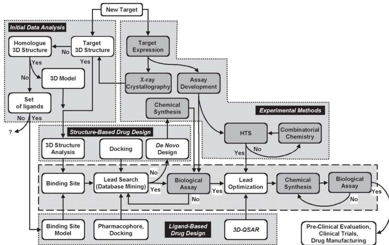
Fig. 10. General strategy of computer-assisted drug discovery.
