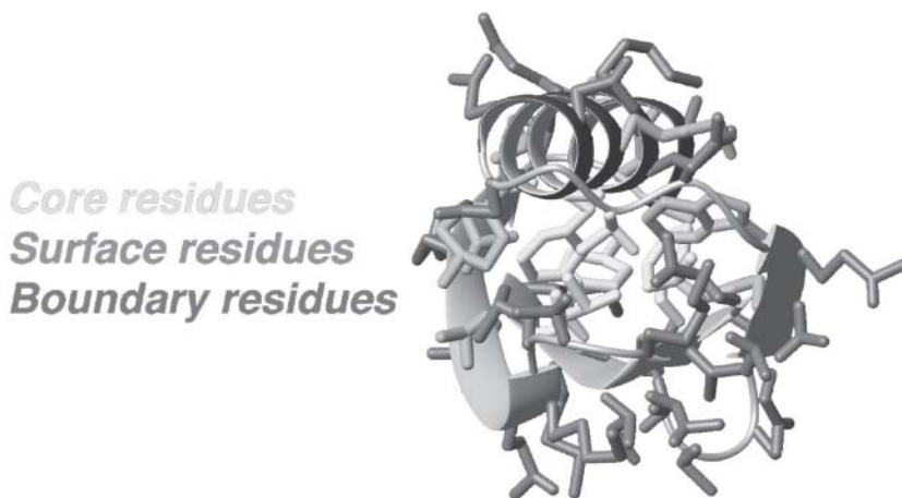
Fig. 2. Core (light gray), boundary (dark gray), and surface (medium gray) residues in protein G \beta 1 (Protein Data Bank identifier 1gb1). Region classification was by buried surface area calculations.
