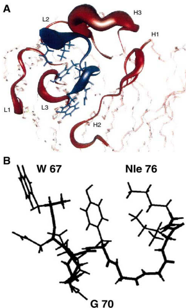
Fig. 12. (A) Fit of peptide into recognition site of antibody Fv198; the width of the backbone drawing is proportional to the root mean square deviation. (B) Conformation of main immunogenic region peptide (WNPDDYGGVK) from \alpha -subunit of acetylcholine receptor with antiacetylcholine receptor autoantibodies (Fv198). (Adapted from ref. 40.)
