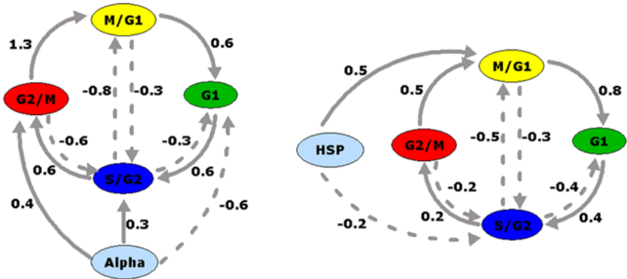
Fig. 4. Interaction of expression levels among cell-cycle phases: (A) \alpha -Data set; (B) cdc-15 data set. Cell-cycle genes for different phases are shown, as well as \alpha -pheromone-activated genes ( \alpha ) and heat-shock-activated genes (HSP). Solid lines indicate positive influence or induction, and dotted lines indicate negative influence or inhibition. Numbers along the edges are the mean value of transition matrix entries of each clustered block and correspond to the influence between cell-cycle phases. (Reprinted with permission from ref. 9.)
