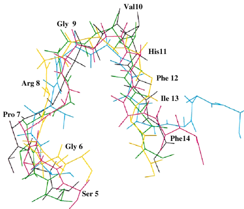
Fig. 11. Structure of SGPRGVHFIF region of gp91 phox C-terminal peptide bound to p47 phox . Shown are the five lowest energy structures having the best agreement with the transferred nuclear Overhauser effect spectroscopy data (Adapted from ref. 38 .)
