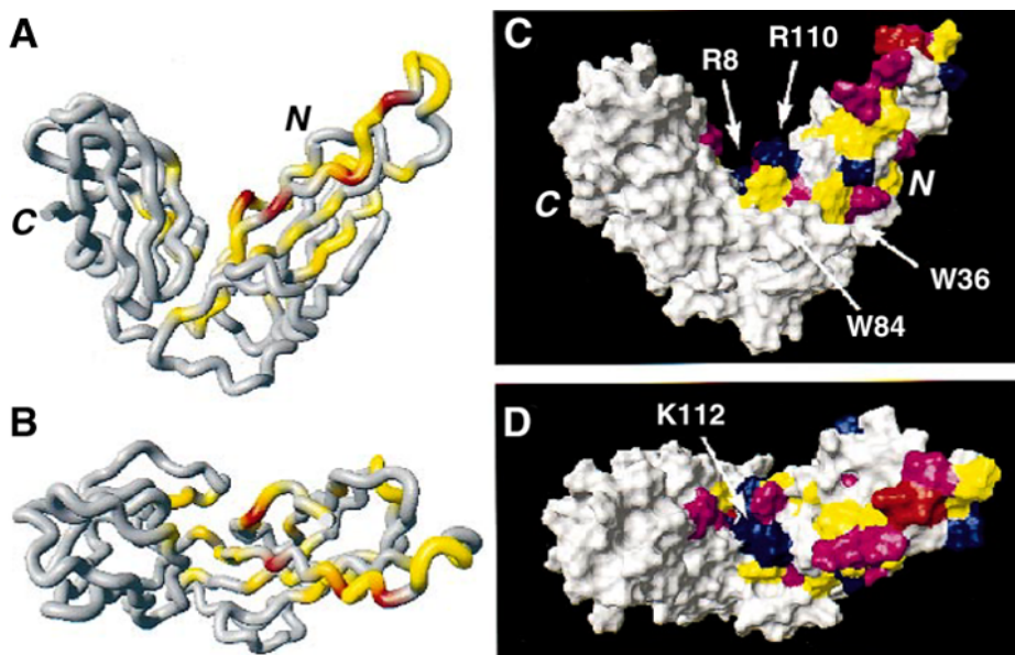
Fig. 28. (A) Mapping of ^{15}\text{N} and ^1\text{H} chemical shift differences for FimC–FimH complex onto 3D structure of FimC. Part (B) is the same as (A) after rotation by 90^\circ about a horizontal axis so that the two wings of the structure point toward the viewer. (From ref. 77. Copyright by Nature Publishing Group. Used with permission.) Molecular surface of nuclear magnetic resonance structure of FimC 3 showing binding surface for FimH. The residues with \delta\Delta > 0.1 ppm are dark. Part (D) is the same as (C) after a 90^\circ rotation of the molecule.
