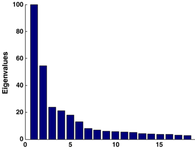
Fig. 1. Bar plot showing eigenvalues from \alpha -factor synchronized cell-cycle data set (1). Singular value decomposition was conducted in Matlab. Note how the first two eigenvalues dominate.
