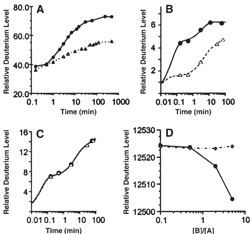
Fig. 5. Protein-protein interactions by hydrogen exchange (HX) and determination of K_d . Plots of deuterium incorporation with time (as in Fig. 4, lower right) were prepared for a protein when incubated with a binding partner. (A) Relative deuterium uptake of protein A alone (●) and in presence of protein B (△). Although not shown, HX into protein B was unaffected by the presence of protein A. (B) Representative deuterium uptake of region of protein A where deuterium exchange was altered on binding (symbols same as in [A]). (C) Peptic fragment from protein B that showed no difference in deuterium uptake as a result of interaction with protein A (protein B alone [●] and in presence of protein A [△]). (D) Relative deuterium uptake of protein A plotted against different mixtures of proteins A and B ([B]/[A]): (—●—) wild-type protein A and (— —) mutant form of protein A (35) that cannot bind to protein B.
