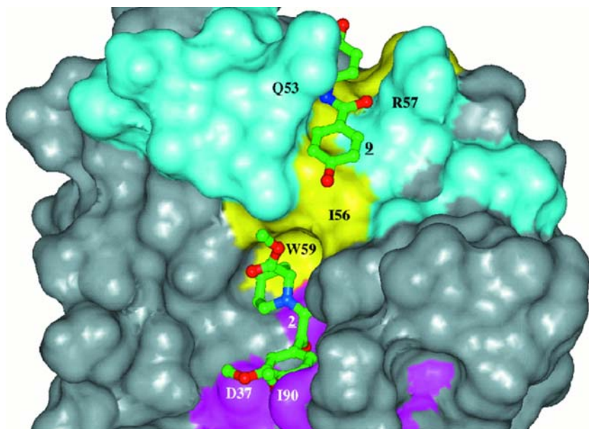
Fig. 24. Surface of FK506-binding protein showing binding sites of compounds 2 and 9 (Fig. 23), as determined from ^{15}\text{N} - ^{13}\text{C} -filtered nuclear Overhauser effect data (see Note 2). Residues that exhibited the largest chemical shift changes on the binding of 2 , 9 , or both 2 and 9 are D37, I90, Q53, R57, W59, I56, respectively. Chemical shift changes for 9 are those observed on the addition of 9 to FKBP in the presence of saturating amounts of 2 (2.0 mM). Weighted averaged chemical shifts were used ( \Delta(^1\text{H}, ^{15}\text{N}) = |\Delta(^1\text{H})| + 0.2 \cdot |\Delta(^{15}\text{N})| ), and indicated residues are those for which \Delta(^1\text{H}, ^{15}\text{N}) exceeded 0.15 and 0.05 ppm for 2 and 9 , respectively. (From ref. 19 with permission.)
