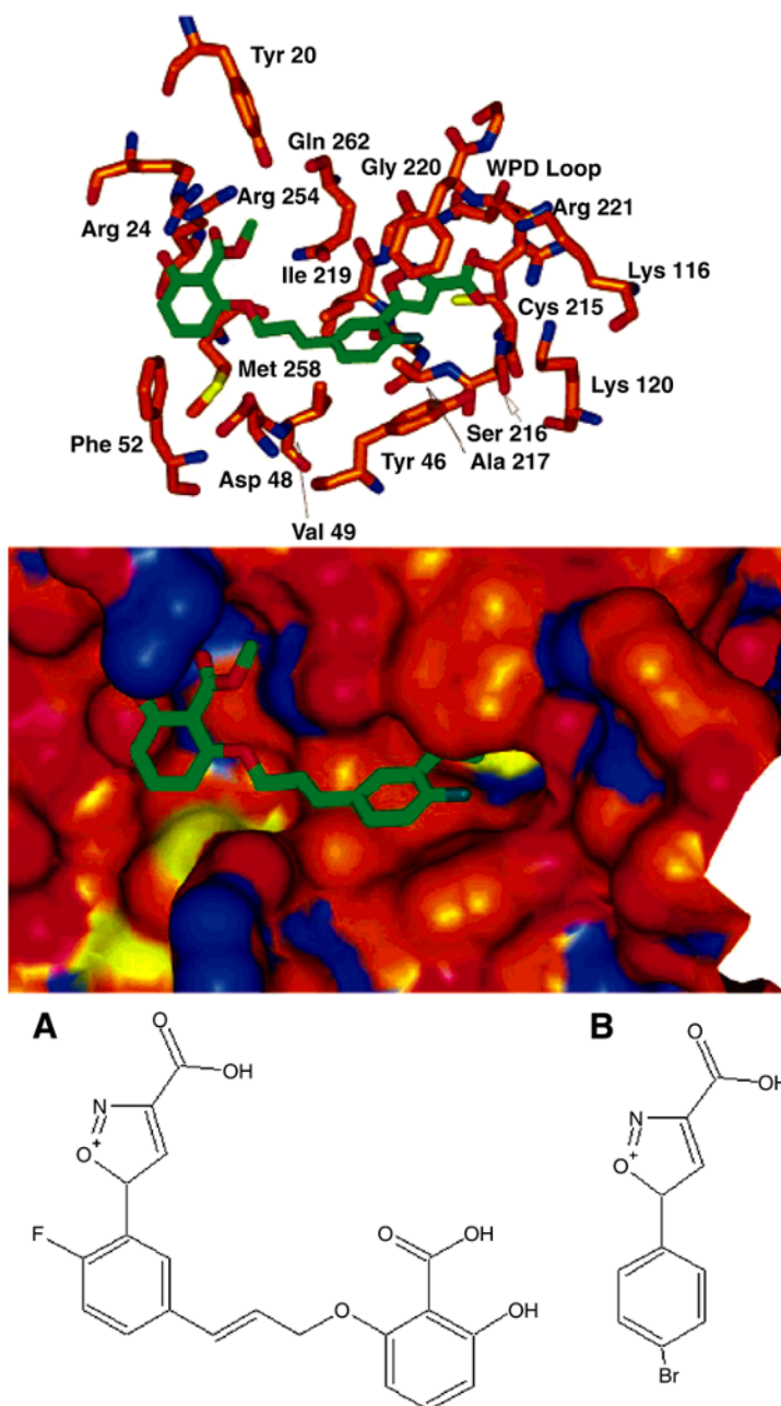
Fig. 27. ( Top ) Stick drawing and X-ray structure of protein tyrosine phosphatase 1B complexed with 3-carboxy-5-{5-[(1 E )-3-(2-carboxy-3-hydroxyphenoxy)prop-1-enyl]-2-fluorophenyl}-5 H -isoxazol-1-ium ( A ). ( B ) Structure of 5-(4-bromophenyl)-3-carboxy-5 H -isoxazol-1-ium, a weak binder to site 2 of protein tyrosine phosphatase 1B ( K_D = 0.8 mM). (Adapted from ref. 65. )
