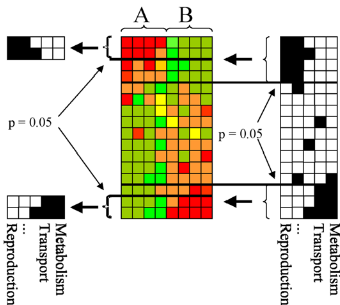
Fig. 7. Two forms of using biological information to describe a list of genes ranked by differential expression between experimental conditions A and B (highly expressed in A on the top and highly expressed in B on the bottom). (Left) Gene expression profiles are examined and, using an appropriate statistical model, only those genes that show significant differences (conventional levels, e.g., type I error rate of 0.05, are used for establishing a threshold) between A and B are selected. The information associated with genes over the threshold is then analyzed using, e.g., FatiGO. (Right) The arrangement of genes is used to study the distribution of gene ontology terms that reflect the biological processes that account for the differences between classes A and B.
