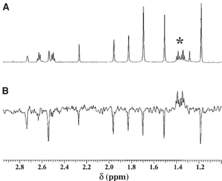
Fig. 18. (A) Reference proton nuclear magnetic resonance spectrum of mixture of 10 compounds in presence of 10 mM cdk2; (B) spectrum showing magnetization transfer from water to the drugs. The methyl group resonances from the cdk2 binder ethyl- \alpha -(ethoxycarbonyl)-3-indoleacrylate are denoted by an asterisk. (Adapted from ref. 48 .)
