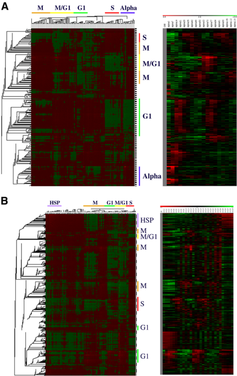
Fig. 3. Hierarchical clustering of transition matrix: (A) \alpha -data set; (B) cdc-15 data set. The clustering result of the \lambda -matrix is shown on the left. Influencing genes are across the top and responding genes are along the side. Expression profiles of genes in the same order as in clustering are shown on the right. Genes with similar expression profiles are grouped together and are labeled with the cell-cycle phases. \alpha -Labels \alpha -pheromone-regulated genes, and HSP labels genes from heat-shock-activated proteins. (Reprinted with permission from ref. 9.)
