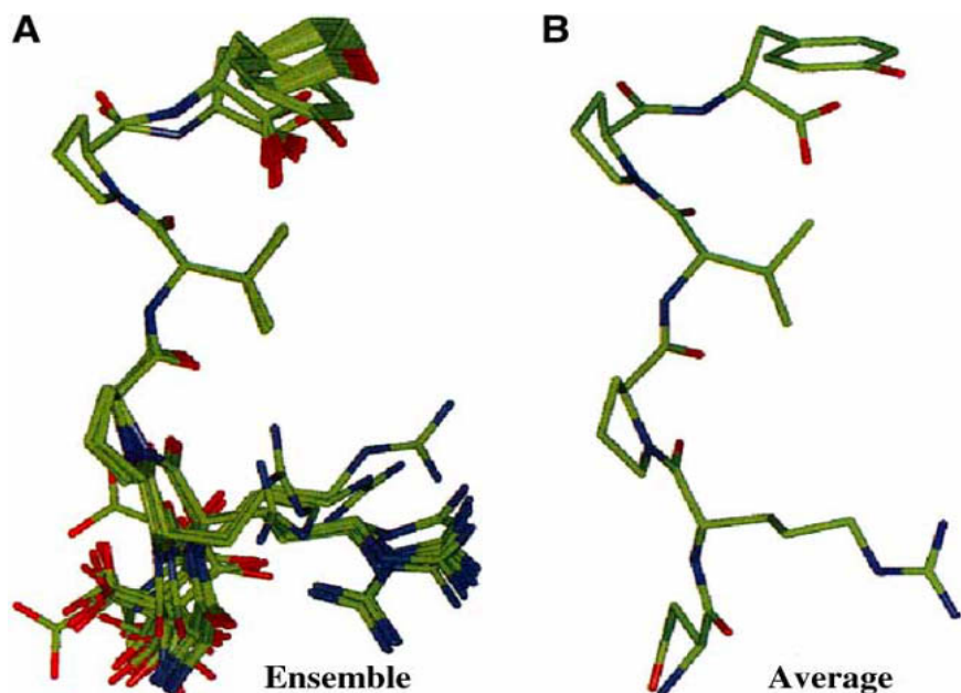
Fig. 15. QUIET-trNOESY of DRPVYPY hexapeptide mimic of trisaccharide repeating unit, L-rhamnose- \alpha -(1 \blacklozenge 2)-(D- N -acetylglucosamine- \beta -(1 \blacklozenge 3))- \alpha -L-rhamnose, of Streptococcus group A cell-wall polysaccharide bound to SA-3 monoclonal antibody: (A) ensemble of 27 lowest-energy structures; (B) average of structures shown in (A). (Adapted from ref. 47 .)
