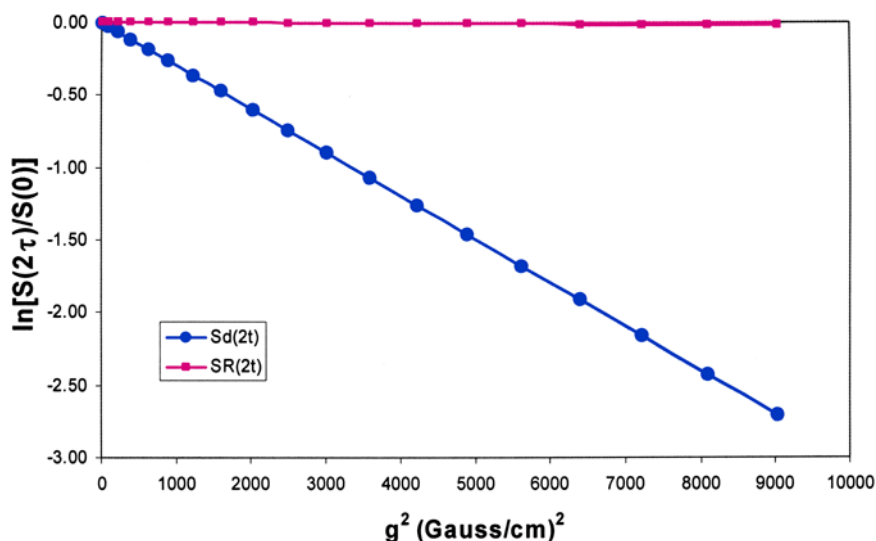
Fig. 1. Example of decay of nuclear magnetic resonance (NMR) signals from two molecules with differing molecular masses of 113 (solid circles = drug) and 30,000 Daltons (solid squares = receptor) in a pulsed-field gradient of strength up to 95 G/cm. Note that at the highest gradient strength, the NMR signal from the smaller molecule has decayed by a factor of 15 with respect to the macromolecule.
