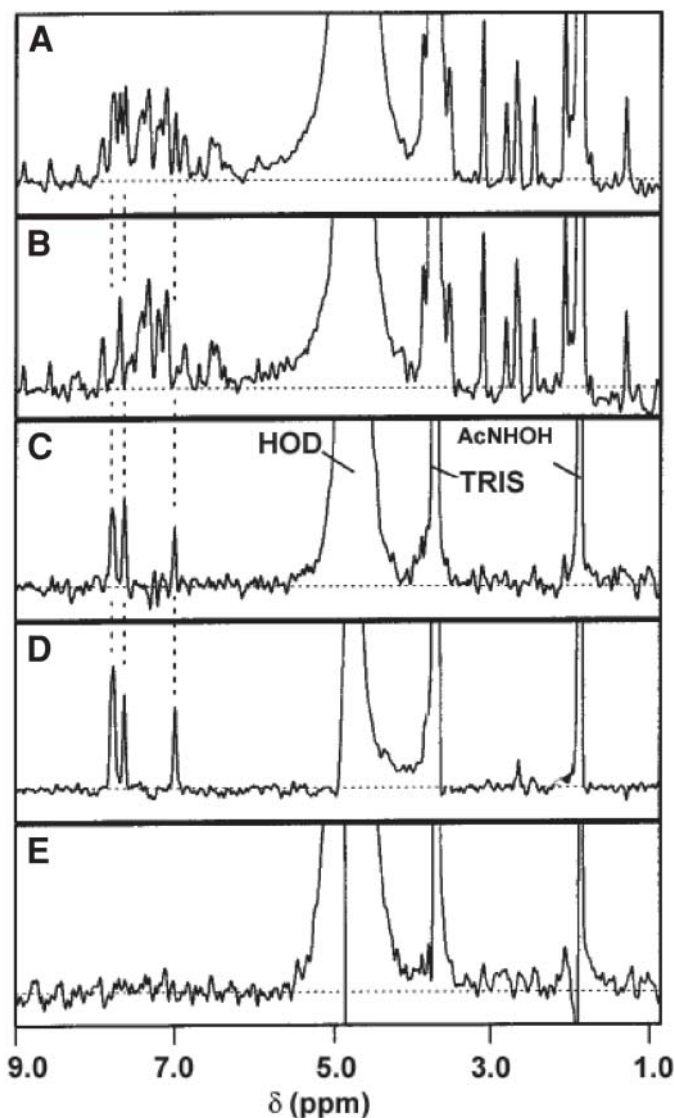
Fig. 5. Diffusion editing of a mixture of molecules to discover compounds that bind to stromelysin. (A) Nuclear magnetic resonance (NMR) spectrum of mix without protein; (B) spectrum of mix in presence of stromelysin taken with gradients; (C) difference spectrum ( [A] - [B] ) showing signals from single binding molecule, 2-phenylimidazole; (D) NMR spectrum of only 2-phenylimidazole; (E) control difference spectrum like in (C) but without 2-phenylimidazole. (Adapted from ref. 20.)
