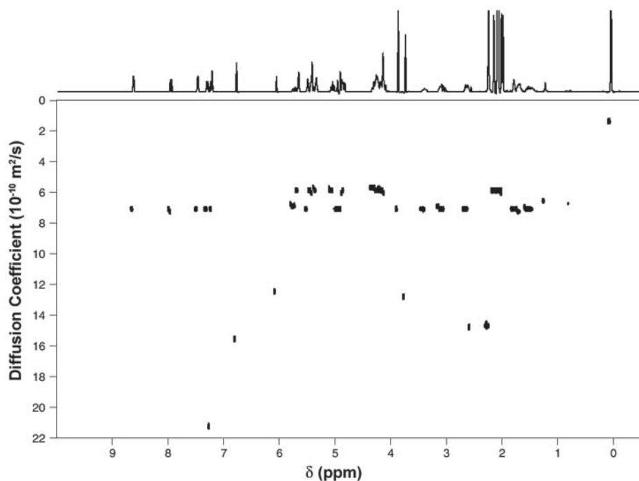
Fig. 7. Diffusion-ordered spectrum of a mixture of polydimethylsiloxane, mesitylene, trimethoxybenzene, sucrose octaacetate, and quinine. Sixteen transients were acquired for each of 20 gradient values ranging from 5 to 25 G/cm in a total time of 32 min. (Adapted from ref. 25 .)
