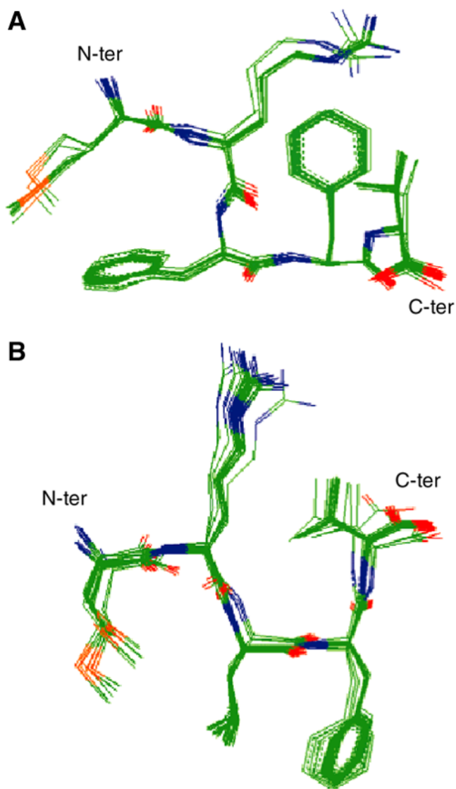
Fig. 16. Structures of ribosome-bound (A) K-peptide and (B) E-peptide, determined by means of transferred NOESY data. These are superpositions of the 20 lowest energy structures determined by simulated annealing. (Adapted from ref. 37 .)
