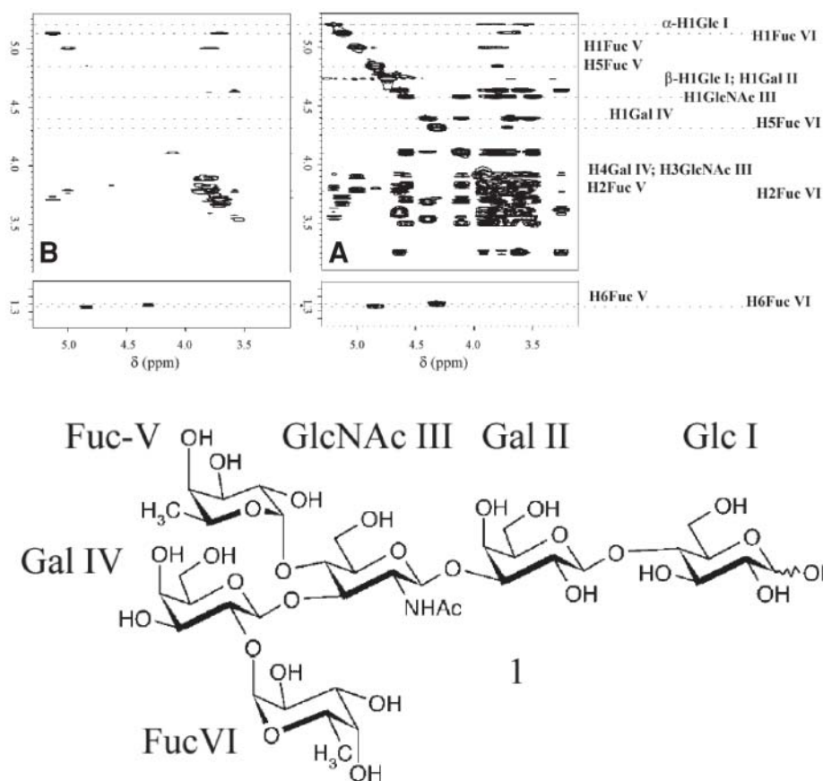
Fig. 19. Saturation transfer TOCSY nuclear magnetic resonance spectra of Lewis-B hexasaccharide ( 1 ) in (A) absence and (B) presence of agglutinin from A. aurantia . In (B) only the fucosyl residues of 1 are seen to acquire saturation from the protein. The on-resonance ( \delta = 10 ppm) and off-resonance ( \delta = 30 ppm) TOCSY spectra were taken at 300 K from 1 mmol of hexasaccharide and 10 nmol of protein. (Adapted from ref. 50.)
