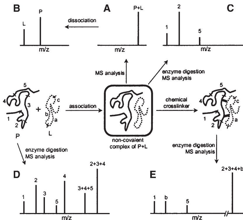
Fig. 2. Noncovalent complex analysis, crosslinking studies, and proteolysis investigations with MS. Two proteins (P and L) may associate and form a noncovalent complex (center). Direct analysis of this noncovalent complex can be accomplished with electrospray methods (see Sub-heading 3.1. ). (A) Peaks corresponding to the combined mass (P + L) indicate formation of the complex. (B) Subsequent dissociation into the individual components verifies that the peak of P + L was indeed composed solely of P and L. In more complicated complexes involving multiple partners, dissociation can help sort out the stoichiometry. (C, D) Binding may alter the enzymatic digestion pattern. P can be digested into peptides 1–5 and L into peptides a, b, and c (enzyme cutting sites indicated by short, perpendicular lines). Analysis of P peptides after complex formation (C) is compared with the peptides produced when P was alone before complex formation (D). Changes to the digestion pattern can indicate which enzyme sites are occluded by complex formation. After complex formation, a chemical crosslinker may also be utilized to link covalently the two proteins together. The resulting mass spectrum (E) will contain peptides with m/z values of the combination of peptide(s) from P that were crosslinked to peptide(s) from L. In this example, the diagnostic peak is 2 + 3 + 4 + b . With spectra of the peptides from each protein without crosslinking, simple addition calculations of peptide masses indicates which peptides have been linked together.
