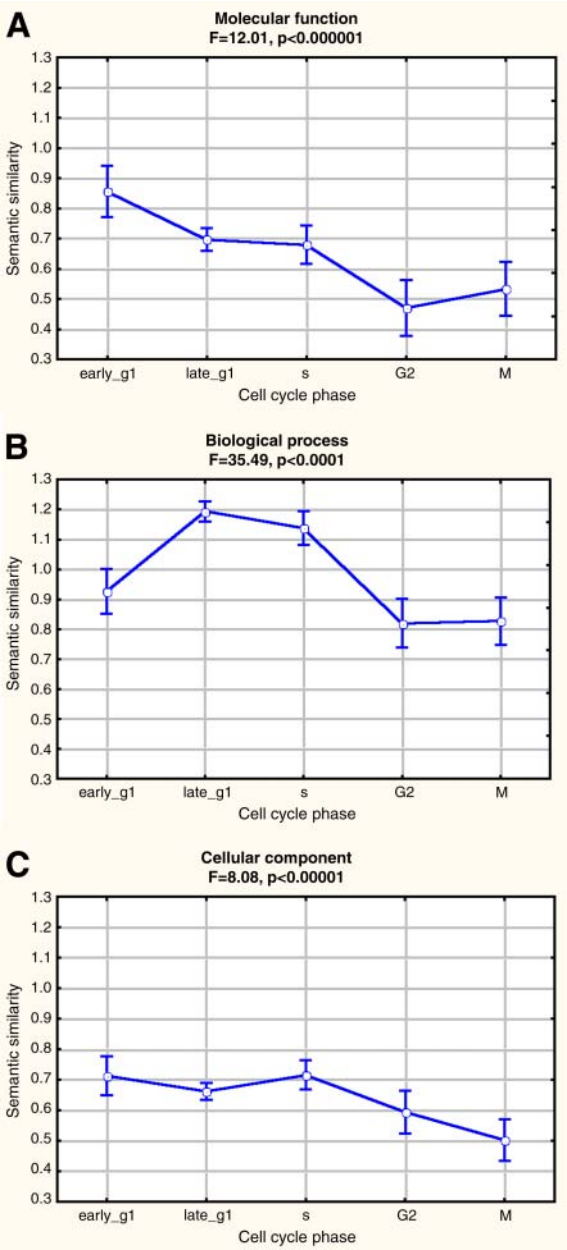
Fig. 4. Linking expression correlation and semantic similarity based on gene ontology. One-way analysis of variance using Resnik’s semantic similarity as the dependent variable and cell-cycle phase as categorical predictor (factor). (A) Results generated by molecular function taxonomy; (B) results generated by biological process taxonomy; (C) results generated by cellular component taxonomy.
