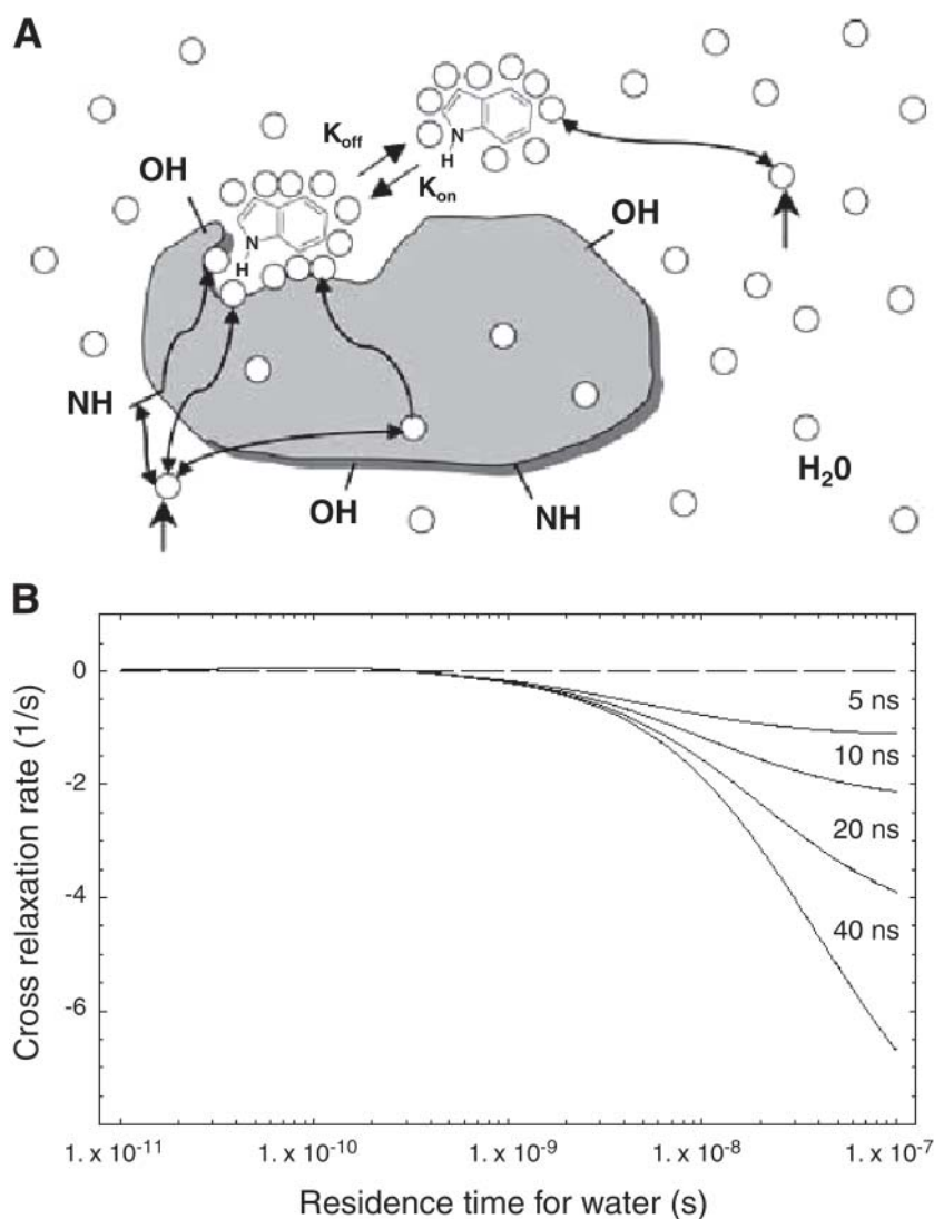
Fig. 17. (A) Mechanisms for nuclear Overhauser effect magnetization transfer from water (circles) bound with ligand at binding site of a macromolecule. Spin diffusion and exchange with bulk water brings magnetization into the binding cavity. (B) Cross-relaxation rate for water molecules at 600 MHz, 2.5 Å from protein proton as function of water residence time in binding site and for values of protein correlation time. (Adapted from ref. 48.)
