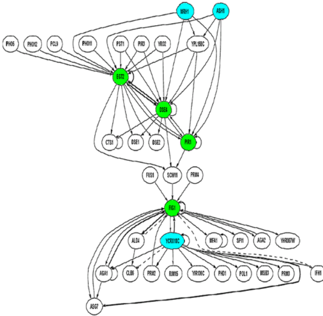
Fig. 2. Network generated from yeast cell-cycle data set. The nodes are genes labeled with standard gene names, and the edges indicate the phenological influence of one gene on another. Solid lines indicate positive influence (induction). Dashed lines indicate negative influence (inhibition). Bold solid lines indicate a strong influence (absolute value of entry of \oplus 0.08 ). Dark gray nodes are genes with more than four edges coming into and going out from them. Light gray nodes are genes with more than four edges going out from them. (Reprinted with permission from ref. 9.)
