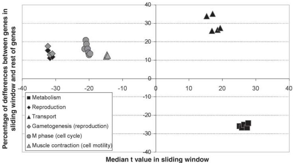
Fig. 8. Over- and underrepresented gene ontology (GO) terms in genes differently expressed when comparing testis and kidney in mice. The left side of the x -axis corresponds to higher levels of expression in testis, and the right side to the kidney, as measured by the statistics. The y -axis represents the percentage of over- or underrepresentation of GO terms with respect to the remaining genes. Terms in black correspond to the third GO level and those in gray to the fourth level.
