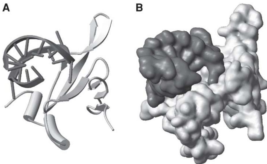
Fig. 8. Complex of capsid protein (in white) from Bacteriophage MS2 with RNA aptamer (in gray), available from Protein Data Bank (PDB) (PDB index 5MSF) ( 125 ). (A) Schematic representation of complex; (B) solvent surface representation.
