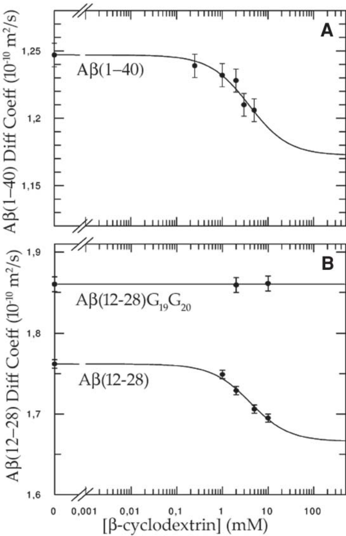
Fig. 6. Measurement of dissociation constant for A \beta peptides for \beta -cyclodextrin by diffusion-filtered nuclear magnetic resonance: (A) A \beta (1-40) and (B) A \beta (12-28) and A \beta (12-28) Gly 19 Gly 20 . (Adapted from ref. 24 .)
