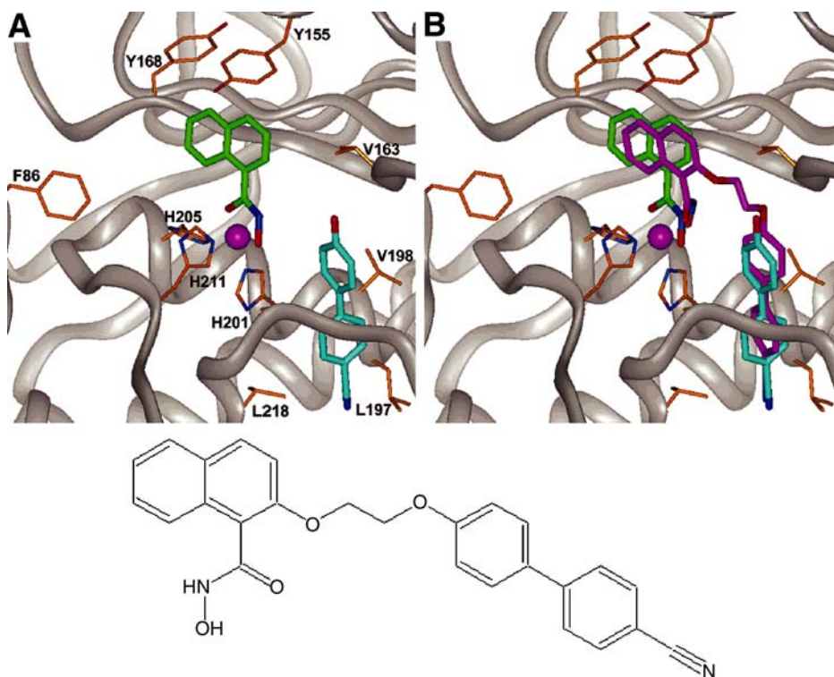
2-[2-[(4'-Cyano[1,1'-biphenyl]-4-yl)oxy]-ethoxy]-N-hydroxy-1-naphthalenecarboxamide
