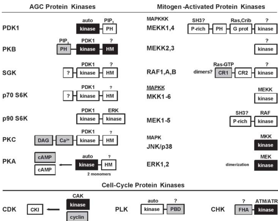
Fig. 1. Domain organization of well-characterized serine–threonine protein kinases of pharmaceutical interest. The isolated kinase domain constructs for which X-ray 3D structures have been reported are indicated in black: phosphoinositide-dependent protein kinase-1 (PDK1); protein kinase B/Akt (PKB); cyclic adenosine monophosphate (cAMP)-dependent protein kinases (PKA); c-JUN NH 2 -terminal protein and 38-kDa protein kinases (JNK/p38); extracellular signal-regulated protein kinases (ERK1,2); cyclin-dependent protein kinases (CDK); and checkpoint kinases (CHK). The active kinase domains of each family member must be phosphorylated, and the upstream protein kinase activator is indicated above each domain. Interestingly, PDK1 serves as the upstream activator of serum- and glucocorticoid-induced protein kinase (SGK), 40- and 90-kDa 40S ribosomal protein S6 kinase (p70 and p90 S6K), and Ca 2+ -activated protein kinase (PKC). No upstream activator has been clearly identified for phosphorylation of the C-terminal hydrophobic motif (HM) domains of PKB, SGK, p70 S6K, PKC, and PKA. The regulatory domain constructs for which X-ray or NMR structures have been reported are indicated in gray: pleckstrin homology (PH) domain of PKB; diacylglycerol (DAG) and Ca 2+ domains of PKC; cAMP-regulatory subunit of PKA; cyclin-regulatory subunit of CDK; the conserved region 1 (CR1) domain of the first identified downstream effector kinases (RAF1,A,B) of the mitogen-activated G protein (RAS); the polo box domain (PBD) of polo-like kinase (PLK) and the forkhead-associated (FHA) domain of CHK. Regulatory domains that bind either small-molecule second messengers or regulatory proteins are indicated. PIP 3 , phosphatidylinositol 3,4,5-triphosphate; CAK, CDK-activating kinase; MEK, MAPK/ERK kinase; SH3, Src-homology 3 domain; ATM/ATR, ataxia telangiectasia mutated kinase/ataxia- and Rad-related kinase; MAPK, mitogen-activated protein kinase.
