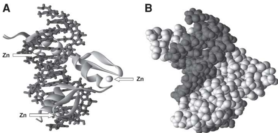
Fig. 4. Zinc-finger protein–DNA recognition. A designed consensus zinc-finger protein (in white) bound to DNA (in gray), available from Protein Data Bank (PDB) (PDB index 1MEY), is shown (73). (A) Schematic representation of complex; (B) Van der Waals representation.
