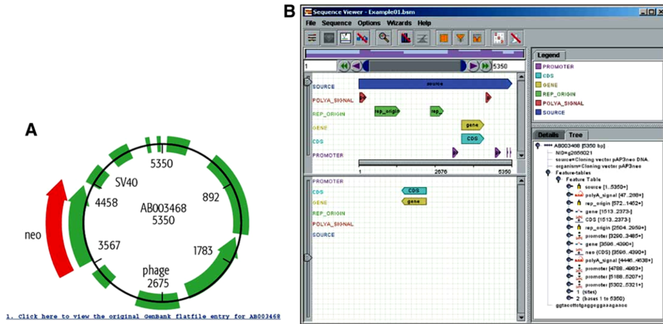
Fig. 10. Browser visualization of (A) genomic XML widgets, and (B) exploration of sequence information from BSM source data.
