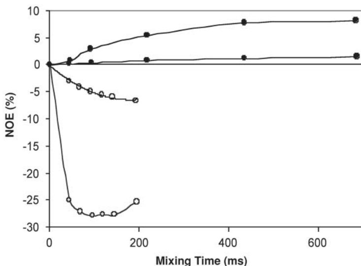
Fig. 10. Nuclear Overhauser effect (NOEs) for two proton pairs of \alpha -L-Fuc(1 \leftrightarrow 6)- \beta -D-GlcNAc-OMe in absence (closed symbols) and presence (open symbols) of Aleuria aurantia agglutinin. The transferred NOEs (open symbols) are larger, build up faster, and are negative with respect to the NOEs for the disaccharide free in solution (closed symbols). (Based on data from ref. 34.)
