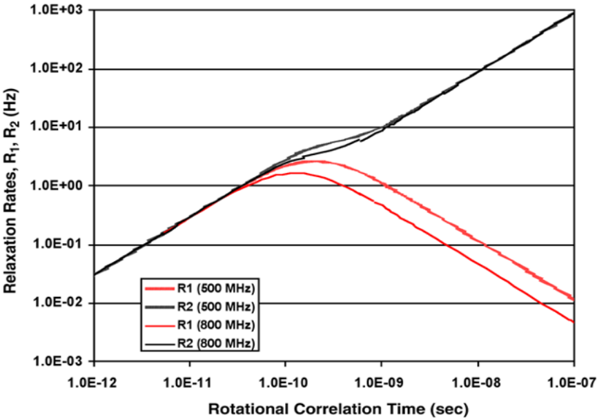
Fig. 2. Relationship between the proton relaxation rates R_1 and R_2 and rotational correlation time for two different nuclear magnetic resonance frequencies, 500 and 800 MHz.
