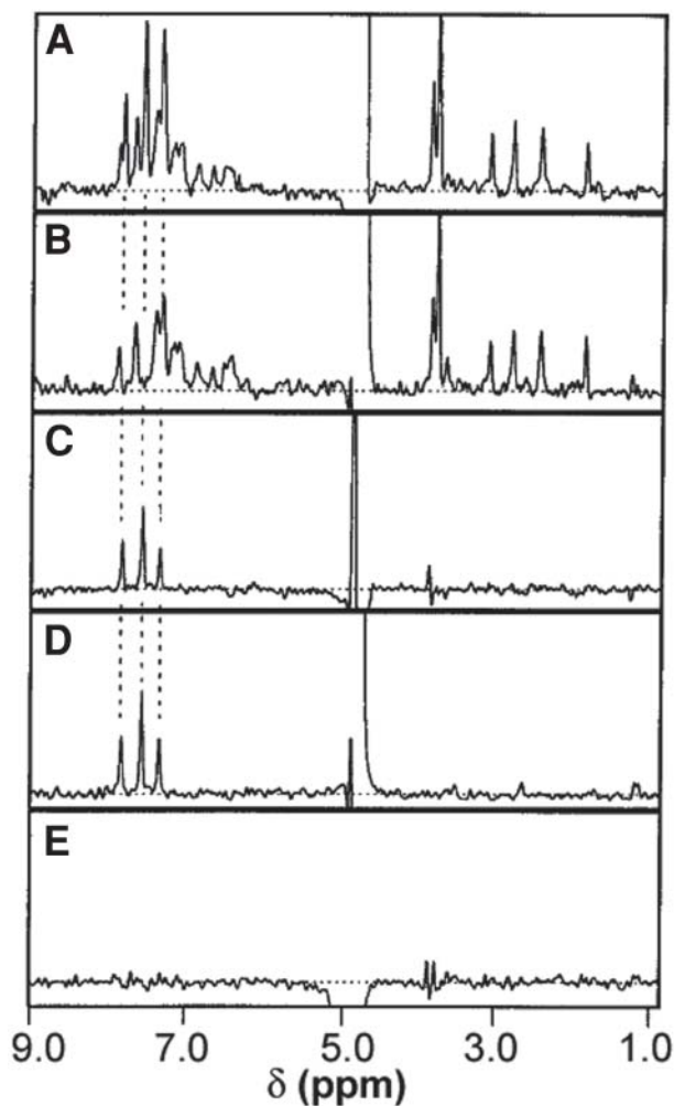
Fig. 9. Transverse relaxation editing of ligand binding to FK506 binding protein: (A) T_2 -edited ^1\text{H} spectrum of a mix of nine compounds, one of which was the FKBP ligand, 2-phenylimidazole; (B) T_2 -edited spectrum of same mix in presence of FKBP; (C) difference spectrum (A – B); (D) reference spectrum of 2-phenylimidazole alone; (E) difference spectrum as in (C) but without 2-phenylimidazole. (Adapted from ref. 21 .)
