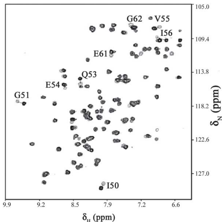
Fig. 22. Superposition of ^{15}\text{N} heteronuclear single quantum coherence nuclear magnetic resonance spectra of FK506-binding protein without (gray) and with (black) compound 3 (Fig. 23). The labeled amide signals display significant chemical shift changes on binding 3 . Each spectrum was taken in the presence of saturating amounts of compound 2 , which bound to a site on the protein adjacent to that occupied by 3 . (Adapted from ref. 19.)
