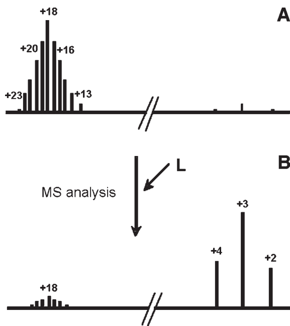
Fig. 6. Complexation and charge-state distributions in electrospray spectra. (A) A protein exhibits a bimodal distribution of charge states, indicating the presence of two distinct conformational forms in solution. The unfolded or higher charge-state distribution centered around +18 is the predominant form in the absence of “L” (where “L” is a ligand that could be a metal ion/drug molecule/peptide or another protein), and so on. (B) Ligand complexation causes a conformational change in the protein leading to a more compact conformation that accommodates relatively fewer charge states (+2 to +4) compared to uncomplexed form.
