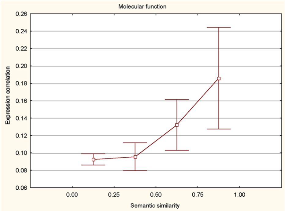
Fig. 3. Linking expression correlation and semantic similarity using gene ontology molecular function taxonomy. Semantic similarity is based on Lin’s measure (Eq. 2).
