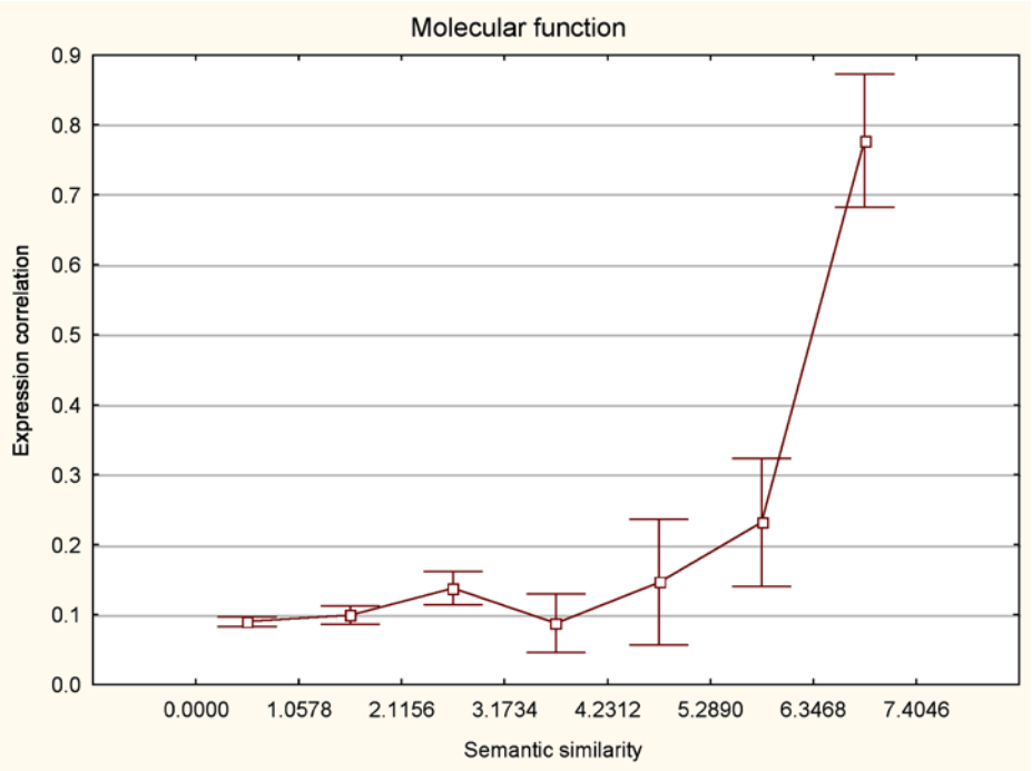
Fig. 2. Relationship between expression correlation and semantic similarity using gene ontology molecular function taxonomy. The axis of abscissas is divided into similarity intervals. The axis of ordinates shows the mean expression correlation values for each similarity interval and their \pm 0.95 confidence intervals. Semantic similarity is based on Resnik’s measure (Eq. 1).
