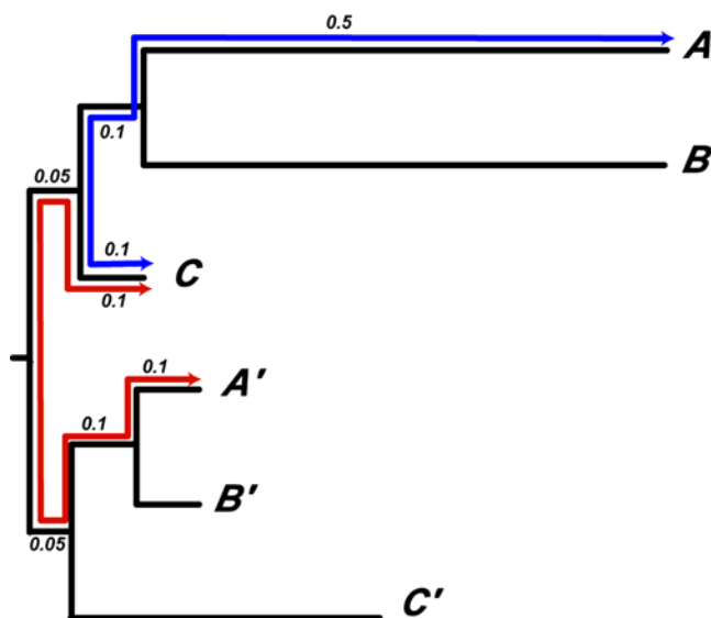
Fig. 2. Phylogenetic tree uniting a number of sequences that display evolutionary rate heterogeneity. In this case, the similarity between sequence C and its true ortholog, sequence A, is much less than the similarity between sequences C and its paralog in species A, the sequence denoted as A'.
