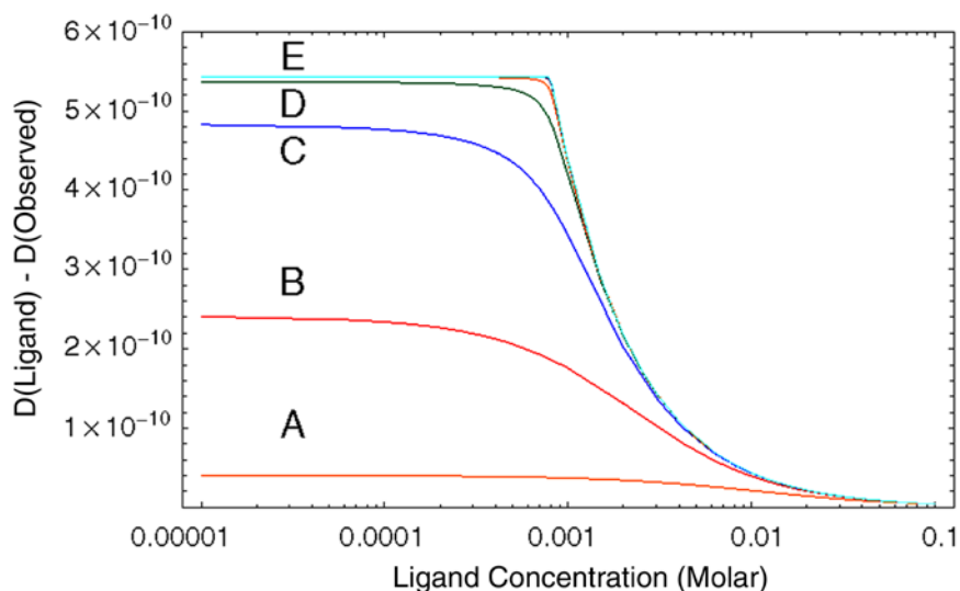
Fig. 8. Difference between free and bound diffusion coefficients for mixture of human serum albumin and tryptophan (see text for parameters) for various dissociation constants, K_d , as function of ligand concentration. K_d = 0.01\text{ M} , 0.001\text{ M} , 0.1\text{ mM} , 10\text{ }\mu\text{M} , and 10\text{ nM} , for curves A, B, C, D, and E, respectively.
