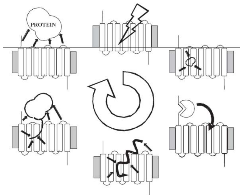
Fig. 1. Diversity in G protein-coupled receptor (GPCR) ligand-binding. Beveled cylinders linked by loops drawn as lines represent transmembrane helices. The membrane is shaded. Solid arrows indicate specific contacts between receptor and ligand. Starting at 12 o'clock and working clockwise, one sees a gradual increase in the size of bound ligands and the complexity of ligand-receptor interactions: first, light interacting with a rhodopsin molecule; second, a small molecule binding to an aminergic GPCR; third, a self-activating GPCR cleaved by a protease; fourth, a peptide binding GPCR; fifth, a small protein, such as a chemokine, binding to a GPCR, exhibiting a mixed binding mode, with interactions from both the transmembrane region and external loops, which is intermediate between that of a peptide and a large protein; sixth, a large protein binding to a GPCR.
