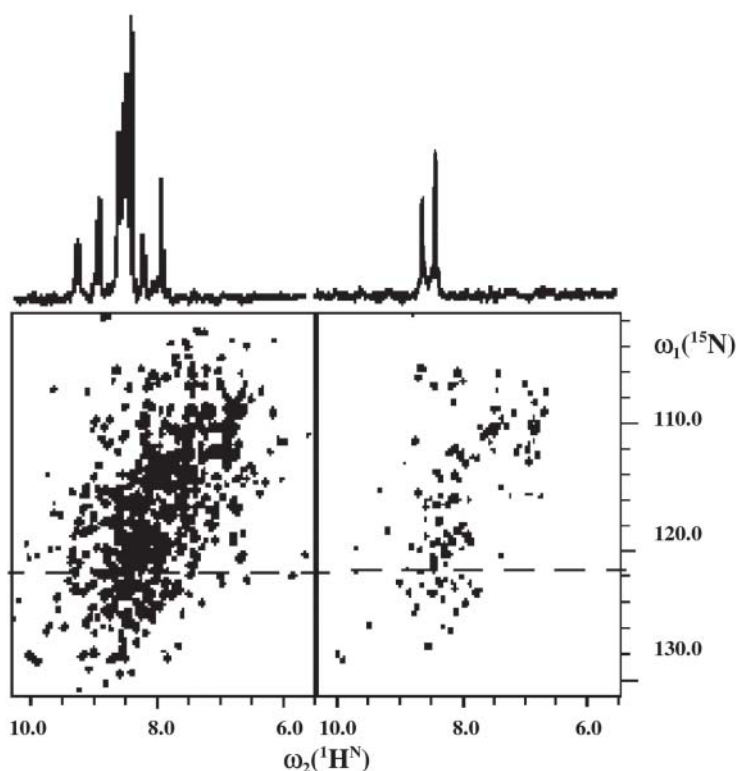
Fig. 4. Transverse relaxation optimized spectroscopy (TROSY) of P450 reductase ( see Note 1 ) from rat liver ( left ) compared with solvent-exposed amide (SEA)-TROSY ( right ). The SEA-TROSY spectrum is much simpler than the TROSY spectrum because the SEA element only picks up resonances from amides exposed to the solvent water protons. (Adapted from ref. 12 .)
