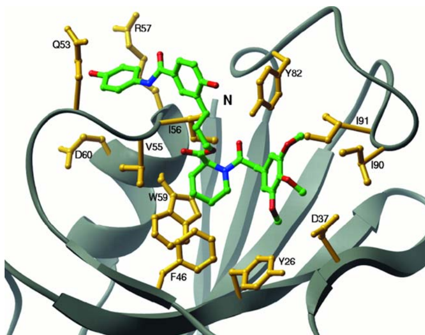
Fig. 25. Ribbon depiction of structure of FKBP (gray) when complexed to 14 (Fig. 23; unlabeled carbon atoms). Labeled FKBP residues are those residues that have nuclear Overhauser effects to the ligand. (From ref. 19 with permission.)
