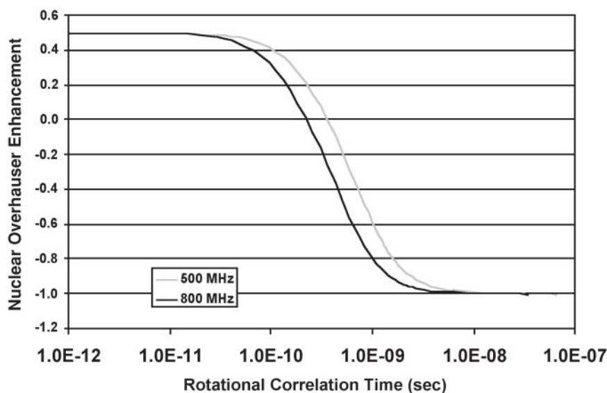
Fig. 3. Relationship between rotational correlation time of a molecule and maximum nuclear Overhauser enhancement (NOE) for a proton relaxed by a neighboring proton for two different proton resonance frequencies, 500 and 800 MHz. Note that there is also a 1/r^6 distance dependence of the NOE that attenuates this maximal interaction.
