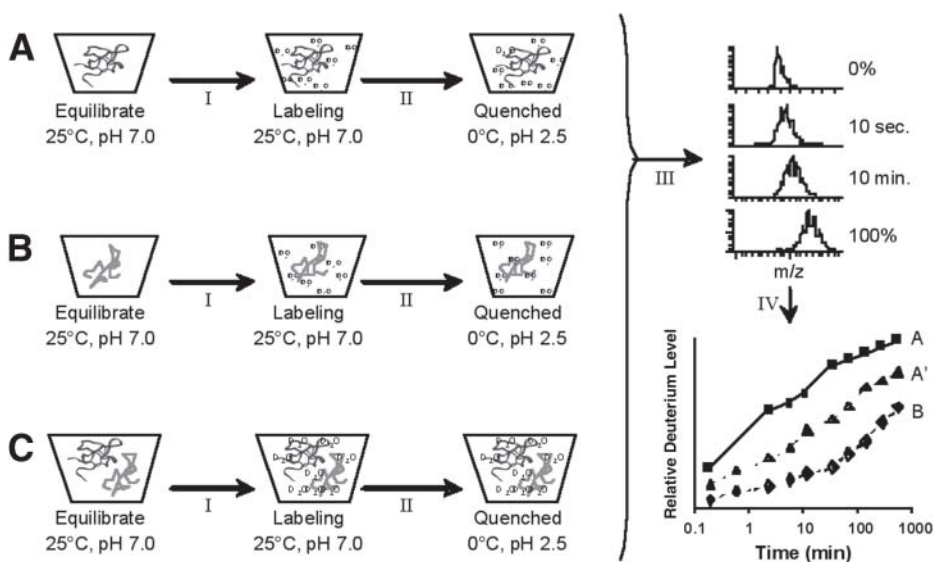
Fig. 4. General hydrogen exchange (HX) mass spectrometry (MS) methodology for protein interaction studies. Two proteins are analyzed separately ( A,B ) to provide baseline information and then together as a complex ( C ). In each case, the protein or protein mixture is incubated in an equilibrium buffer at 25°C, pH 7.0 in H 2 O. D 2 O is then added (I) to initiate the HX reaction. At various times after the introduction of D 2 O HX of an aliquot of the labeling sample is quenched (II) by adjusting the pH to 2.5 and the temperature to 0°C. The quenched samples are then analyzed individually by MS (III) either as whole proteins or after pepsin digestion (not shown). The resulting mass spectra indicate the amount of deuterium incorporation at each exchange time point. These results are plotted (IV) as deuterium level vs. time. In this example, the deuterium uptake of protein A when by itself and protein B when by itself were plotted. When protein A was in the presence of protein B (indicated as A'), its deuterium uptake was less than when it was alone. The deuterium level of protein B in the presence of protein A is not shown. See Subheadings 3.2. and 3.4. for more details.
