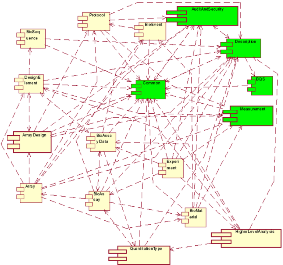
Fig. 11. Relationships among the 17 packages in MAGE-OM. (See color image in ebook.) (Adapted from ref. 68a. )
