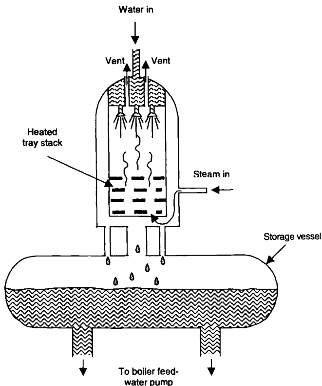
Figure 2.5 Principle of a deaerator
