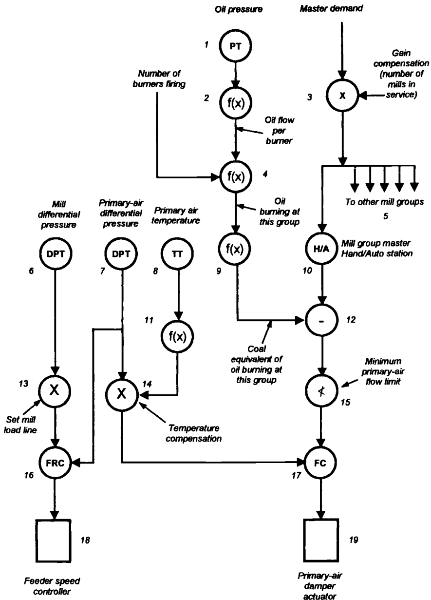
Figure 5.18 A comprehensive mill control system (one mill group shown, excluding temperature control)
