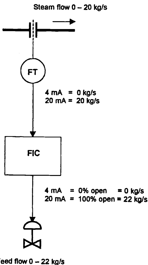
Figure 6.1 Feed-water control based on feed-flow measurement only
