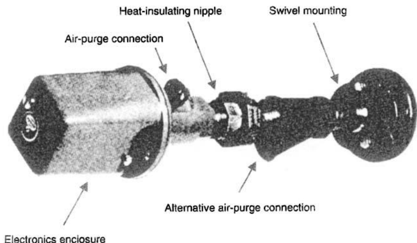
Figure 5.21 Typical flame scanner
