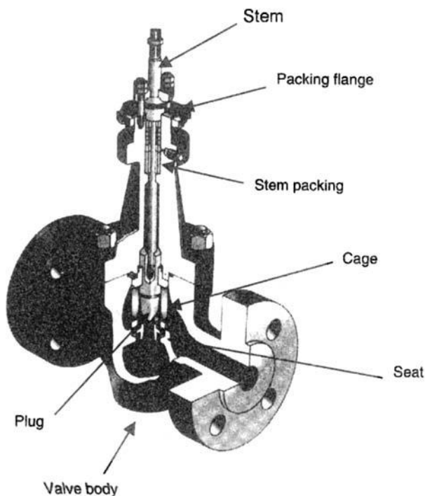
Figure 6.9 A typical feed-water control valve body
