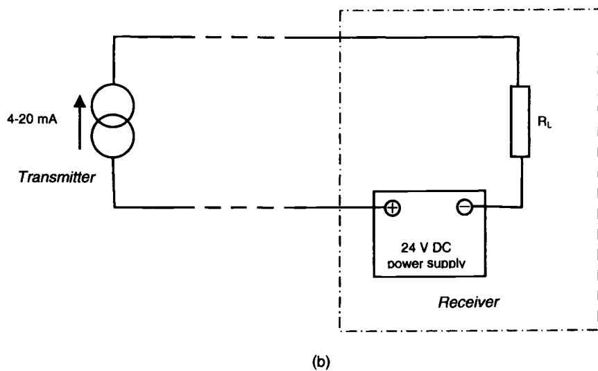
Figure 8.9 The advantages of two-wire transmission a Transmission without 'live zero' b Two-wire transmission (with 'live zero')
