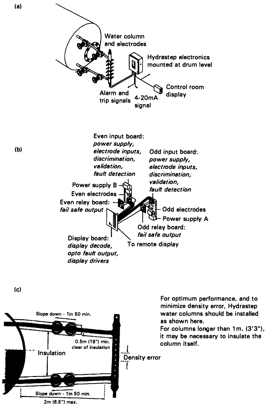
Figure 6.6 The 'Hydrastep' level-indicating system © Solotron Ltd. Reproduced by permission
