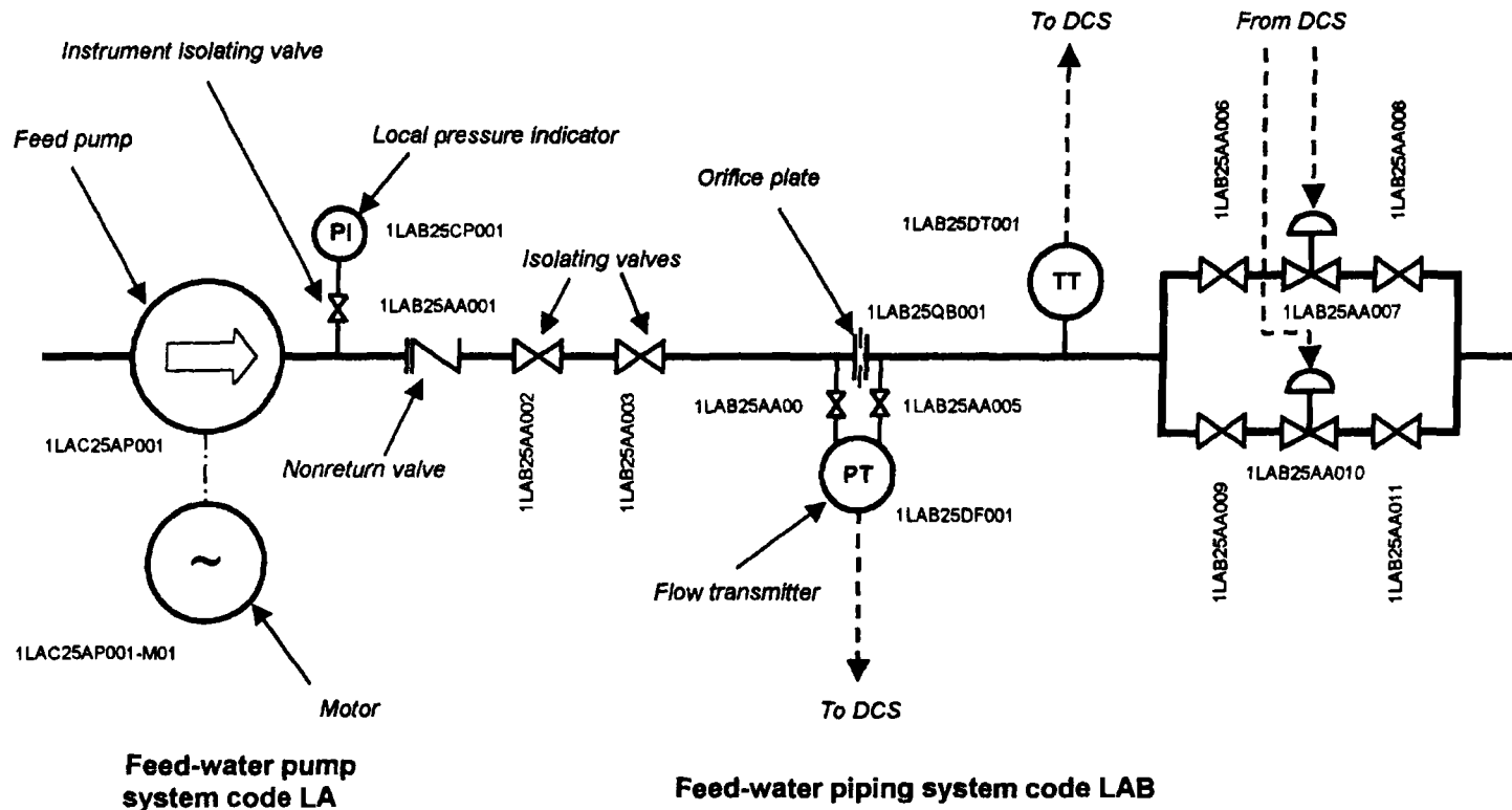
Figure 9.4 KKS coding applied to a feed-water pump system
