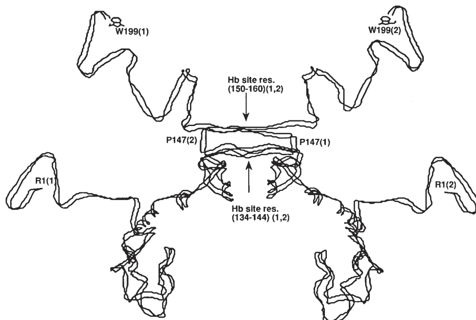
Fig. 12. \alpha -Carbon chain trace of backbone without side chains of hydrophobic stabilized (Hb) antiparallel sheet dimer of \alpha_{sI} -casein B; the large sheets centering on proline 147 are docked. (R) represents the N-terminal residues of molecules (1) and (2), while (W) represents the C-terminal residues of molecules (1) and (2).
