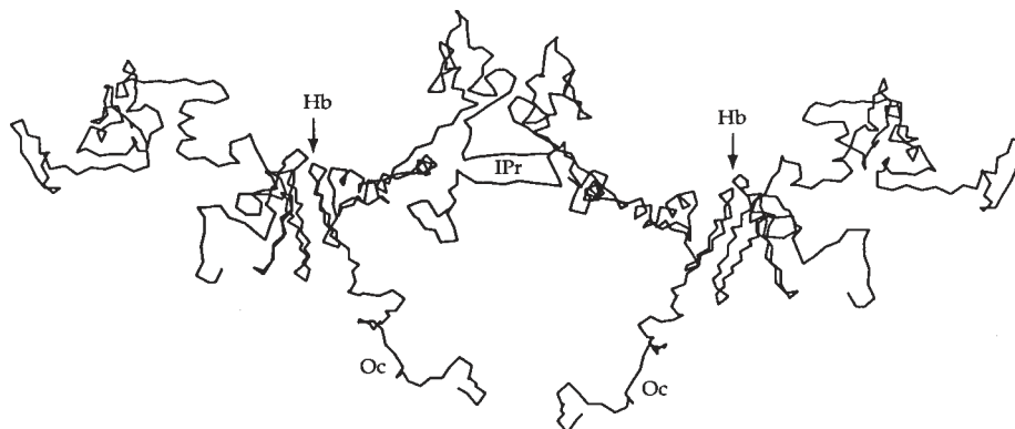
Fig. 17. \alpha -Carbon chain trace of \alpha_{sI} -casein B tetramer resulting from the docking of two molecules (left and right sides of the figure) of \alpha_{sI} -B through the hydrophobic (Hb) scheme shown in Fig. 12 with the (IPr) ion pair dimer given in Fig. 16 . Sites for octamer formation (Oc) are noted.
