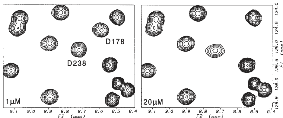
Fig. 3. \text{Mn}^{2+} -induced broadening effects in ^1\text{H} - ^{15}\text{N} HSQC spectra of the \text{C}_2\text{A} -domain. Expansions of ^1\text{H} - ^{15}\text{N} HSQC spectra of the \text{C}_2\text{A} -domain acquired in the absence of \text{Ca}^{2+} and presence of 1\ \mu\text{M} or 20\ \mu\text{M} \text{Mn}^{2+} are shown on the left and right panels, respectively. Note that only the cross-peaks from D238 and D178 NH are significantly broadened with 20\ \mu\text{M} \text{Mn}^{2+} , whereas no broadening is observed for all other cross-peaks, which correspond to NH groups that are far from the metal-binding sites. The D178 NH cross-peak is broadened more severely than that of D238 NH, in agreement with the fact that D178 NH is closer to site Ca1 than D238 NH (Ca1 is the only site being significantly populated by \text{Mn}^{2+} under these conditions).
