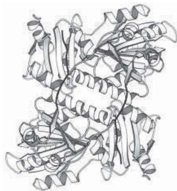
Fig. 2. Ribbon representation of the front-to-front interaction. Two molecules are related by a crystallographic twofold axis. The extended N-terminal residues ( ^3\text{GLDFPEYDGVDRV}^{15} ) of one monomer, depicted with black, become inserted into the other monomer.
