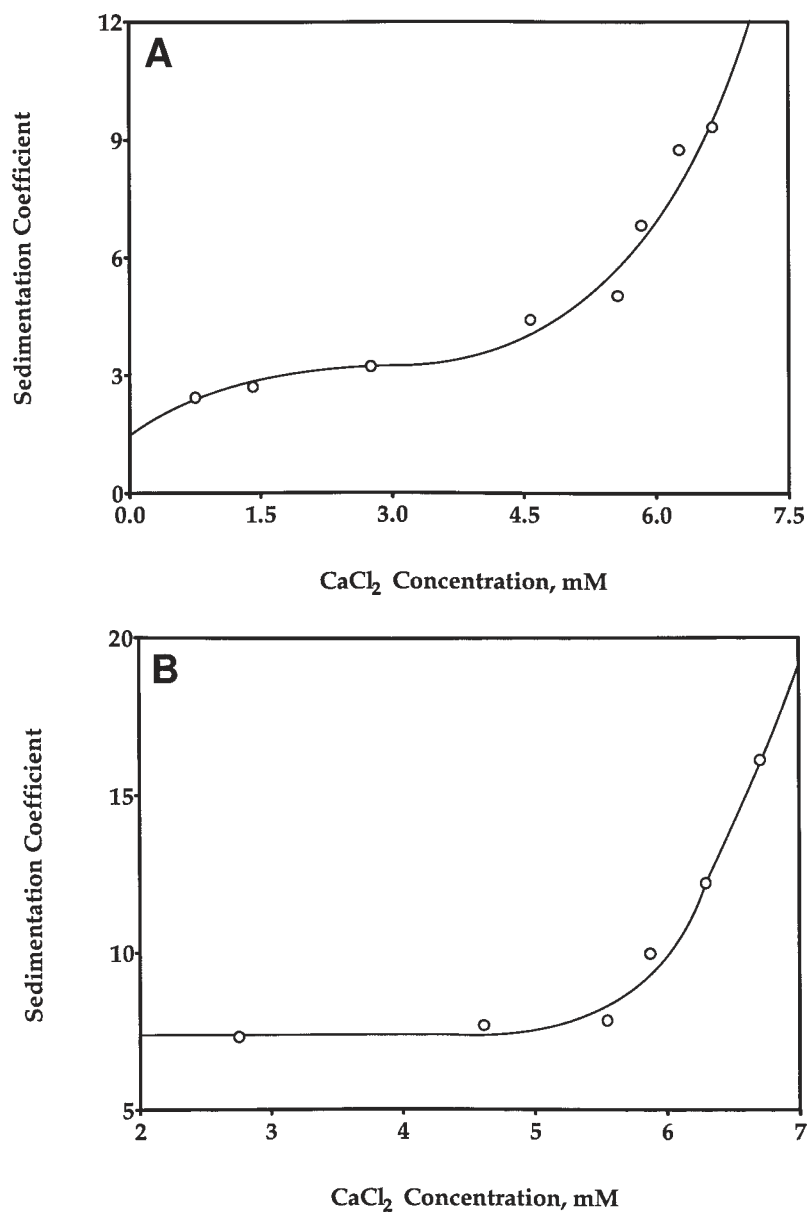
Fig. 7. Sedimentation velocity of \alpha_{SI} -B at 10 mg/mL as a function of added \text{CaCl}_2 . Two peaks were observed a slow one (A) and a fast one (B); analysis was by use of Eq. 4 and given in Table 5; data are replotted from Waugh et al. (1971) (35).
