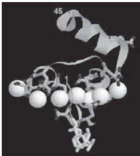
Fig. 2. The structure of the \text{Ca}^{2+} -loaded Gla domain of factor VIIa. Residues 1–45 are shown with the seven \text{Ca}^{2+} ions (white balls) in one plane. The Gla residues are shown in stick representation and all but one (Gla 35 ) are directly involved in \text{Ca}^{2+} binding. It is also striking how the Gla residues form two carboxylate surfaces, a minor surface below the plane of the \text{Ca}^{2+} ions comprising residues Gla 6 and Gla 7 and a major surface on top of the metal ions. The three residues postulated to be in contact with the phospholipid surface are shown in yellow at the bottom. For details of picture generation, see Fig. 1.
