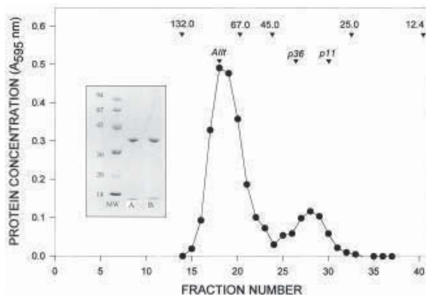
Fig. 2. Formation of recombinant annexin II tetramer. Recombinant annexin II (0.260 \mu mol) and recombinant p11 (0.258 \mu mol) were mixed and incubated overnight on ice in 40 mM Tris-HCl, pH 7.5, 1 mM DTT, 0.15 M NaCl, and 0.1 mM EGTA. The mixture was applied to a Sephacryl S-100 gel-filtration column equilibrated with the same buffer and fractions were analyzed for protein concentration. The position in the elution profile of several globular proteins of known molecular weight is provided. For comparison, the position in the elution profile of bovine lung AII t (AII t ), recombinant annexin II (p36), and recombinant p11 (p11) is also indicated. Inset: SDS-PAGE analysis of pooled recombinant AII t (fractions 18–21), (A) and bovine lung AII t , (B).
