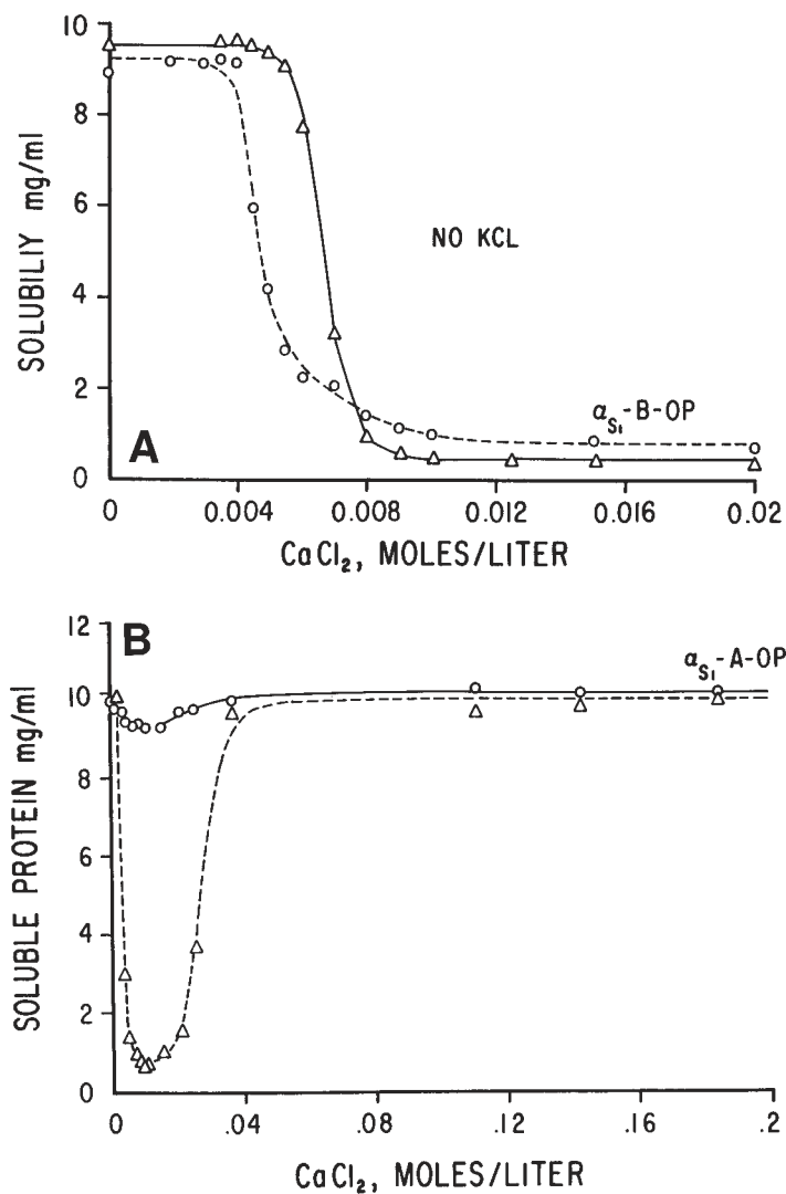
Fig. 6. (A) Solubility at 37°C of native and dephosphorylated \alpha_{sI} -B ( \alpha_{sI} -B-OP) as a function of \text{CaCl}_2 concentrations at 10 mg/mL. (B) Solubility of \alpha_{sI} -A O-P as a function of calcium ion concentrations at 1°C (—) and at 36°C (---). Data were fitted by Eq. 4. Results of analyses are given in Table 4.
