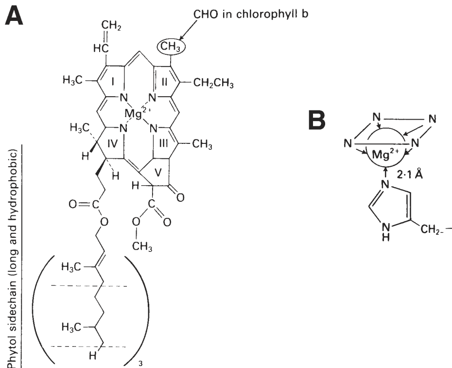
Fig. 5. The formula of chlorophyll and an illustration of how \text{Mg}^{2+} nearly fits the central cavity. N- and 5-coordination is forced upon the \text{Mg}^{2+} ion.
