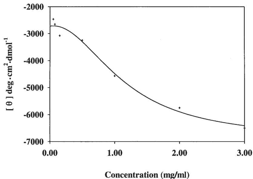
Fig. 14. Plot of change in [\theta] at 283 nm as a function of protein concentration for \alpha_{SI} -casein. The data were derived from Fig. 13 and fitted with Eq. 4 ; the calculated apparent constants are given in Table 8 .
