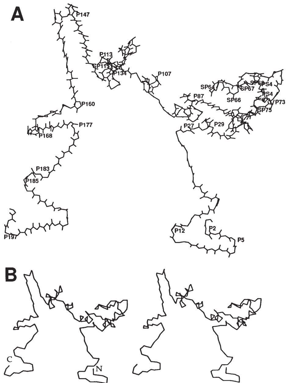
Fig. 8. (A) Backbone of the refined model of \alpha_{S1} -casein B, without side chains, prolines (P) and serine phosphates (SP) indicated. (B) Stereo view of the refined three-dimensional molecular model of \alpha_{S1} -casein; the N- and C-terminal ends of the molecule are labeled.
