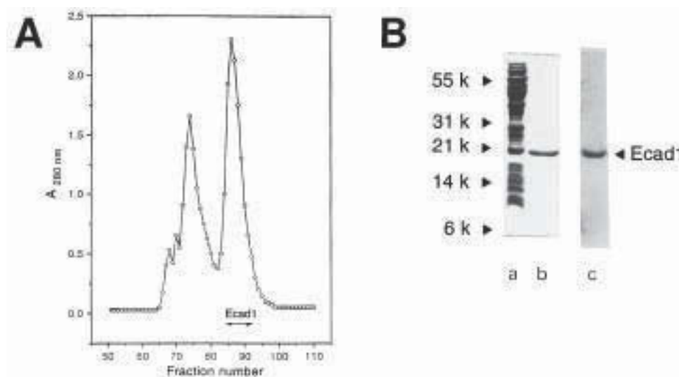
Fig. 1. (A) Gel filtration chromatography of Ecad1 (residues 1–145). (B) SDS-PAGE of ECAD1. Lanes a–c contain, respectively, the total soluble extract from E. coli , purified Ecad1, and an autoradiogram obtained from a ^{45}\text{Ca} blot of Ecad1.
