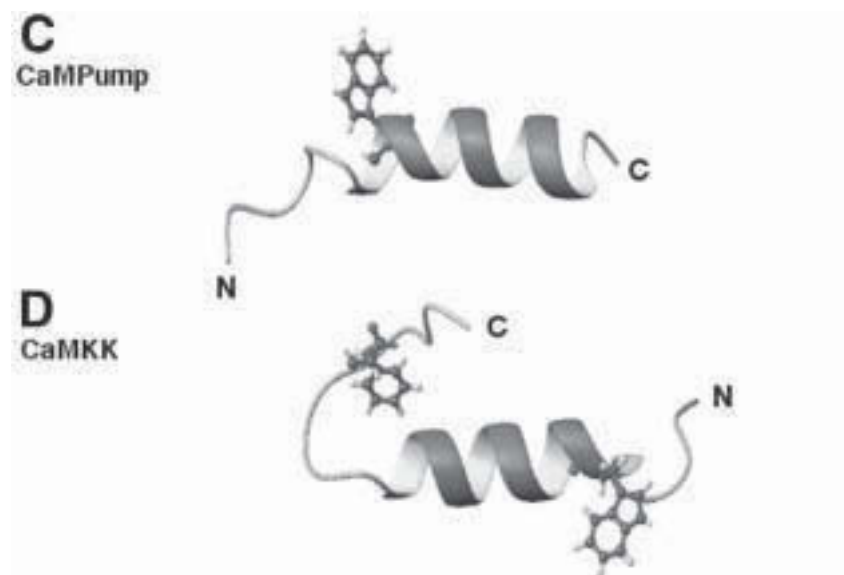
Fig. 4. ( continued ) (D) CaM-dependent protein kinase kinase (Osawa et al., 1999), with the two major hydrophobic “anchor” residues shown in ball-and-stick format. The first two peptides (skMLCK, CaMKII) bind CaM (shown schematically above the structures) in an antiparallel fashion, with the N-terminal anchor residue burying in the C-terminal hydrophobic patch of CaM. The pump peptide, which only binds to the C-terminal lobe of CaM, only has one hydrophobic anchor residue. The CaMKK peptide binds to CaM in a parallel fashion, with its tryptophan residue buried in the N-terminal lobe of CaM. This figure was generated with the MOLMOL molecular rendering program (70).
