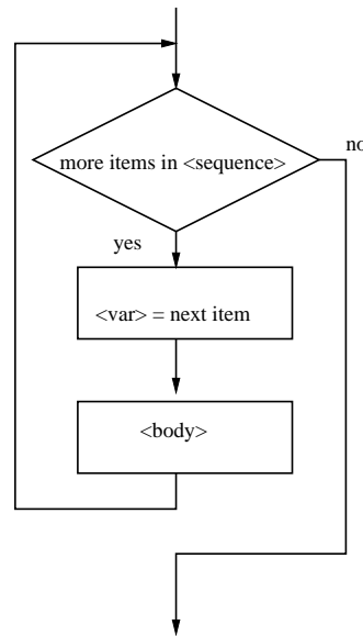
Figure 2.1: Flowchart of a for loop.
