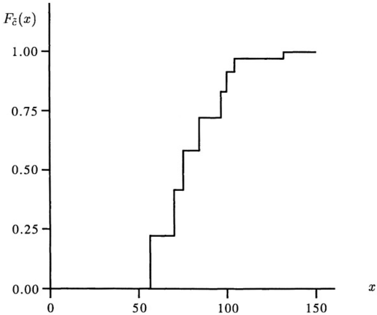
Figure 2.1. Distribution function for the random variable \tilde{c} defined in Example 2.4.
