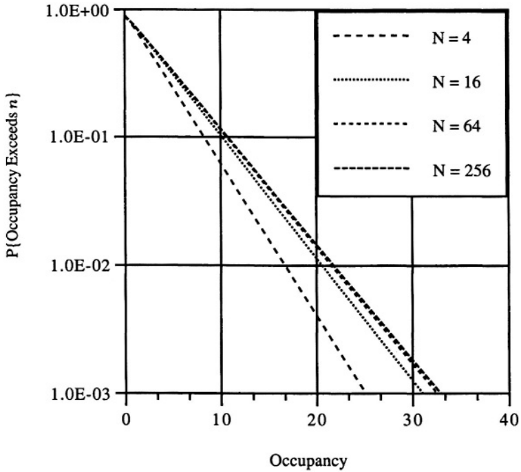
Figure 5.4. Survivor functions with unit deterministic service and binomially distributed arrivals with N as a parameter at \rho = 0.9 .
