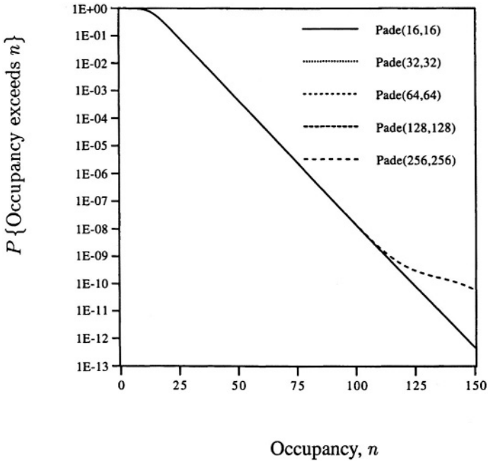
Figure 5.8. Survivor functions for deterministic (16) batch sizes with Pade(n, ℓ)-approximated deterministic service and Poisson arrivals at a traffic load of 0.9 for various choices of n = ℓ .
