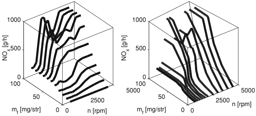
Fig. 6.10 \text{NO}_x map plotted in the n and m_f directions. Left plot represents the \text{NO}_x emissions at iso- m_f values, while right plot shows the \text{NO}_x emissions at iso- n
