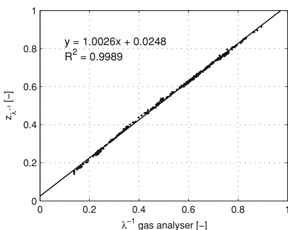
Fig. 3.15 \lambda^{-1} from \text{ZrO}_2 sensor ( z_{\lambda^{-1}} ) and the gas analyser under different steady operating conditions; the linear fit and correlation coefficient are represented
