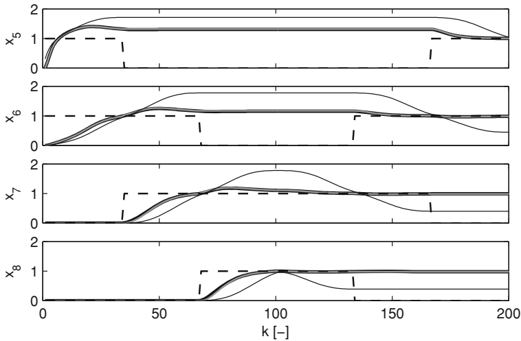
Fig. 5.10 States evolution for a monotonically varied inputs sequence. Black thick line is KF, gray line is SKF, thin black is SSKF and dashed line shows when the element is observable (1 is active; 0 is not active)
