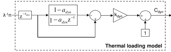
Fig. 4.10 Block diagram of the thermal loading factor C_{dyn}
