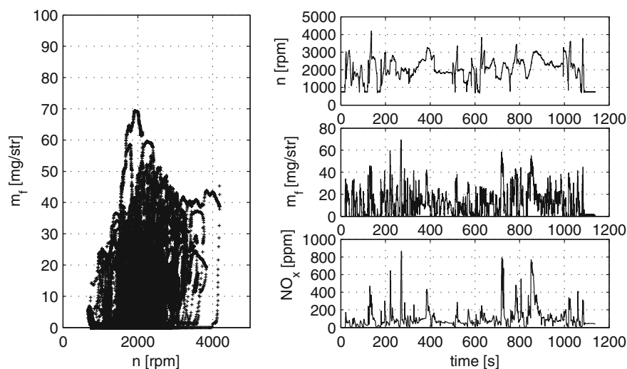
Fig. 3.11 Rural CADC cycle performed on the engine
