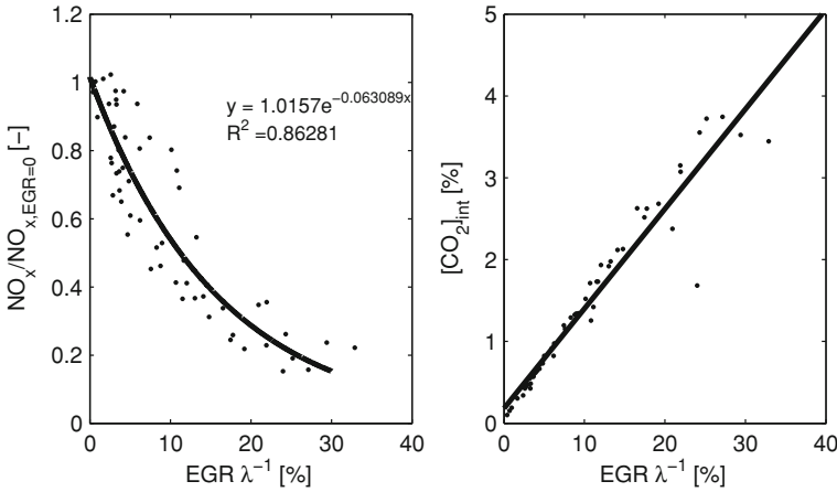
Fig. 4.5 Left plot shows normalised \text{NO}_x emissions as function of EGR\lambda^{-1} for different operating points in the diesel engine explained in Chap. 3. Right plot shows the fitting of [\text{CO}_2]_{\text{int}} and EGR\lambda^{-1}
