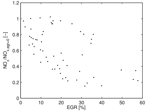
Fig. 4.6 Normalised NO x emissions as function of EGR for different nominal operating points of the DW12B engine
