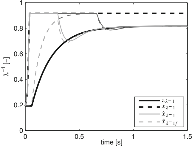
Fig. 6.4 \hat{x}_{\lambda^{-1}} for two different conditions of freezing for an injection step from 15 to 30 mg/str at 2,250 rpm. Thin solid lines represents \hat{x}_{\lambda^{-1}} , lighter to darker gray is less to more severe freezing condition. \hat{x}_{\lambda^{-1}f} models linked with the estimate \hat{x}_{\lambda^{-1}} are also included with dashed lines
