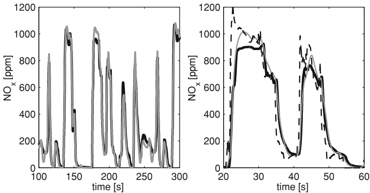
Fig. 4.17 Left y_{NO_x} (gray) and z_{NO_x} (black) in the TRAN A ( T_{cool} = 75^\circ\text{C} , \Delta u_{egr} = 5\% , \Delta p_{boost} = 0 ). Right x_{NO_x} (dashed black), y_{NO_x} (thin gray) and z_{NO_x} (black) in the same test. x_{NO_x} is the actual NO x , no delay nor filtering are expected
