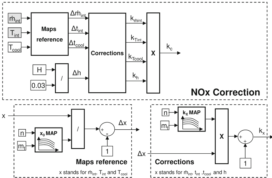
Fig. 4.9 Structure of the factor C_{NO_x} calculation for correcting NO x output
