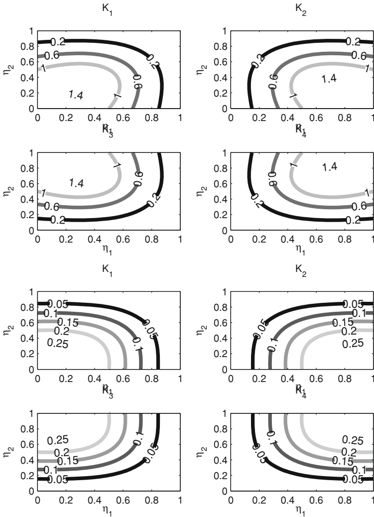
Fig. 5.5 Membership functions for Kalman gain correction for the 2D case for \sigma_v^2/\sigma_w^2 = 0 (top) and \sigma_v^2/\sigma_w^2 = 0.1 (bottom)
