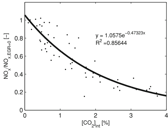
Fig. 4.4 Normalised NO x emissions as function of [CO 2 ] int for different nominal operating points in the diesel engine explained in Chap. 3 and coming from the steady-state campaign. Engine calibration is the standard given by the manufacturer
