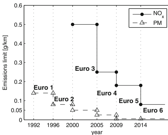
Fig. 1.2 NO x and PM emission limits for diesel passenger cars and light-duty vehicles (M1) from Euro 1 to Euro 6 standards. NO x limits were first imposed in Euro 3 . Euro 6 is to be applied in 2014
