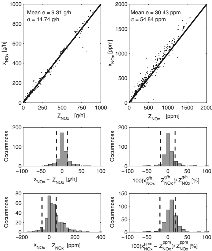
Fig. 4.14 RT NO x model results with steady tests. Top plots Model fitting with respect to the NO x sensor output. Medium plots Absolute and relative error in percentage with respect to the NO x sensor output and for g/h output ( x_{NO_x}^{g/h} ) of the model. Bottom plots Absolute and relative error in percentage with respect to the NO x sensor output and for ppm output ( x_{NO_x}^{ppm} ) of the model
