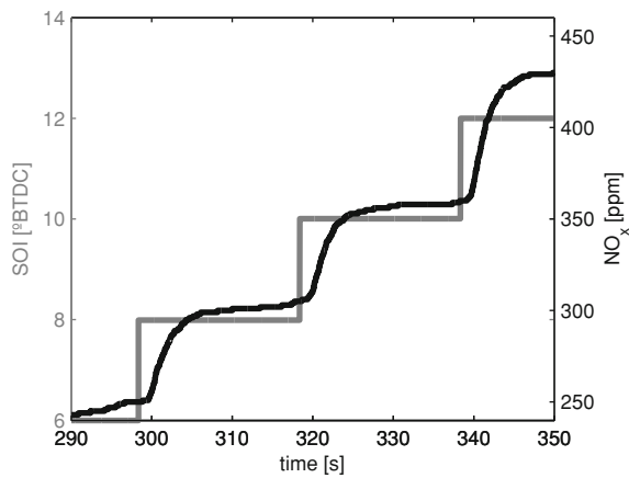
Fig. 2.6 NO x sensor response to SOI steps ( black-right axis ). NO x presents a clear delay and filtering with respect to the SOI signal ( gray-left axis ). The dynamic response could be fitted with a first order delayed discrete filter. SOI units are crank angle degrees before the top dead centre (°BTDC), while NO x is measured in ppm. The delay is in the order of 1 s while the response time is around 0.75 s
