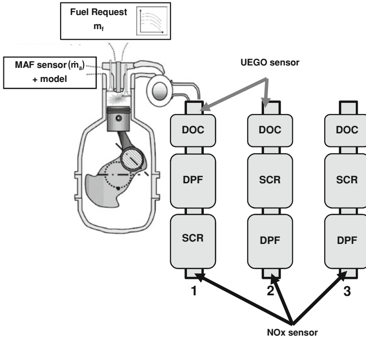
Fig. 5.1 Possible UEGO and NO x sensors configuration setup for a turbocharged diesel engine
