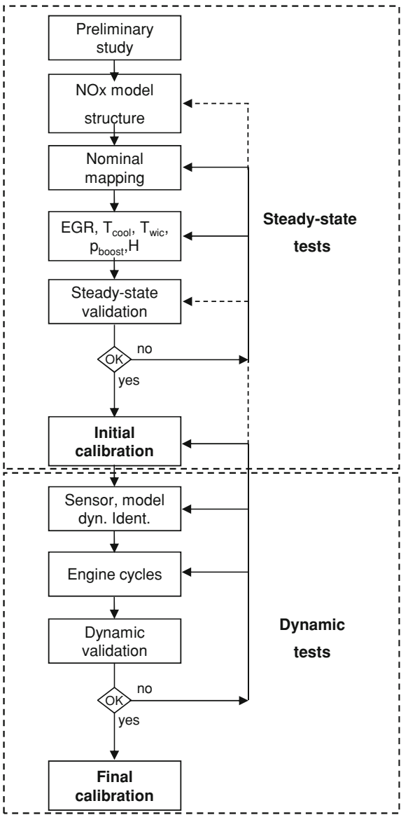
Fig. 4.13 Scheme of the calibration and validation procedure for the NO x model
