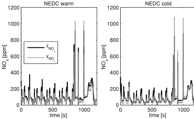
Fig. 4.19 y_{NO_x} model output and z_{NO_x} measured by the sensor in the NEDC. Left NEDC warm cycle A1. Right cold cycle A2
