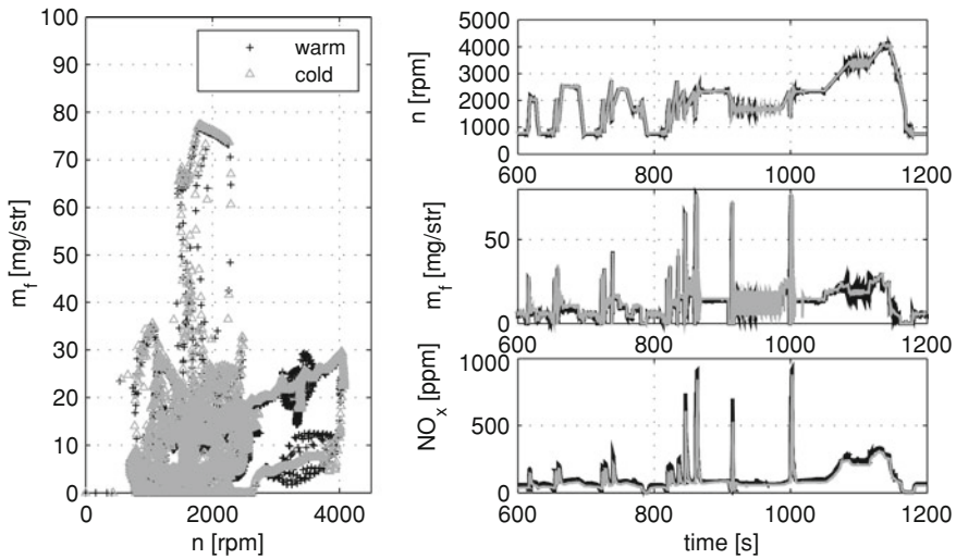
Fig. 3.9 NEDC cycle performed on the engine
