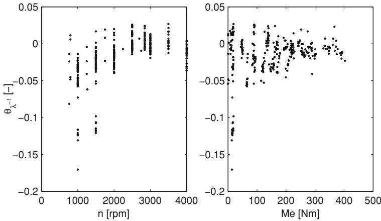
Fig. 4.2 Model bias for the steady-state tests
