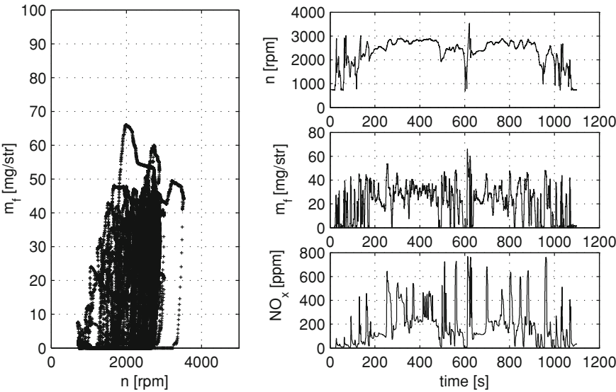
Fig. 3.12 Highway CADC cycle performed on the engine
