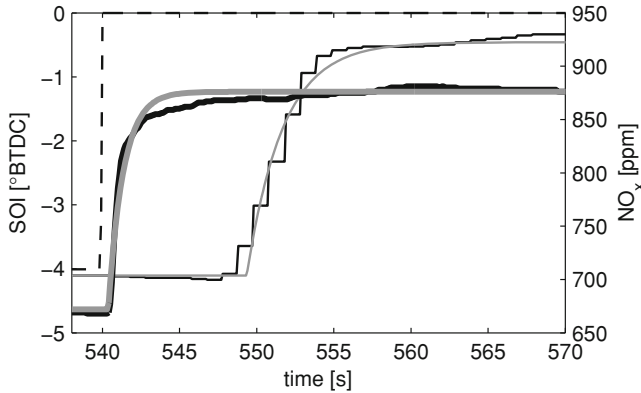
Fig. 3.18 Identified models ( solid gray ) and measured evolution ( solid black ) for both sensors: thin lines correspond to the gas analyser while thick ones to the NO x sensor. SOI step is reproduced with a black dashed line. The delay of the gas analyser is clear with respect to NO x sensor
