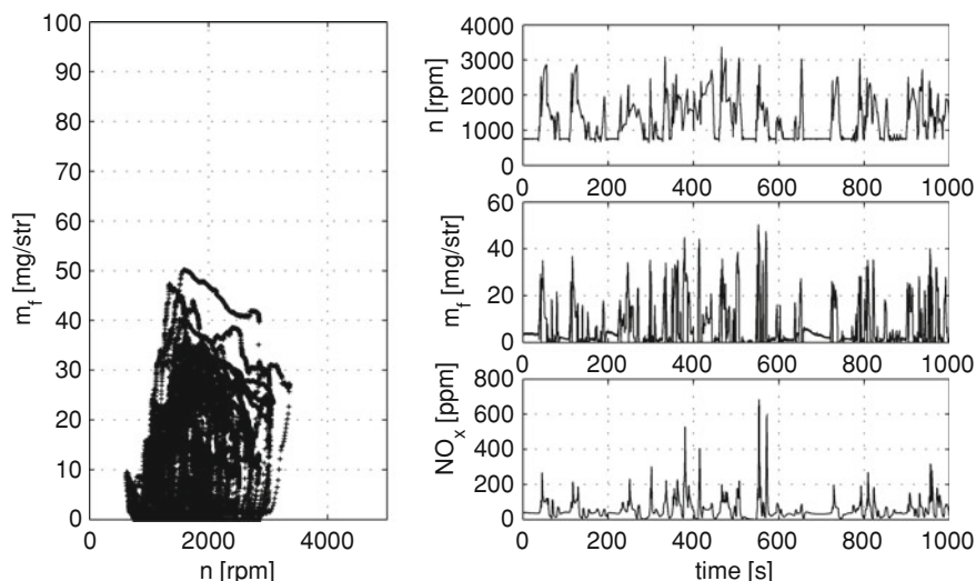
Fig. 3.10 Urban CADC cycle performed on the engine.
