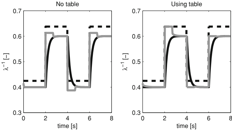
Fig. 6.5 \hat{x}_{\lambda^{-1}} without table ( left ) and using an adaptive table ( right ) changing the operating point condition of the engine repeating two times a cycle by simulating. Black line is z_{\lambda^{-1}} , dashed black line is x_{\lambda^{-1}} and gray line is \hat{x}_{\lambda^{-1}} . Deactivation freezing rules are applied
