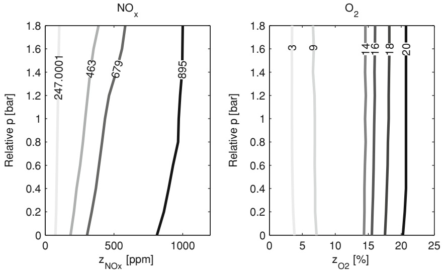
Fig. 3.13 Effect of the pressure over the NO x sensor for the NO x output z_{\text{NO}_x} (left) and oxygen estimation z_{\text{O}_2} from \lambda^{-1} output (right). It seems that the manufacturer has compensated the oxygen output but not the NO x output
