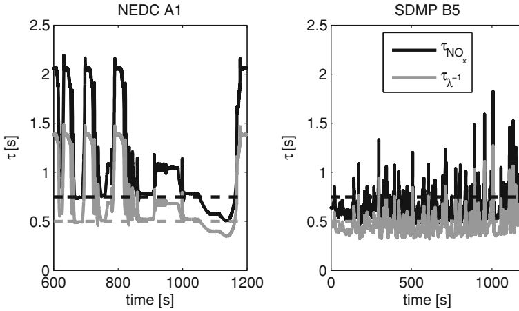
Fig. 3.23 Variable sensor delay modelled for z_{NO_x} and z_{\lambda^{-1}} outputs from the NO_x sensor during the second half of the NEDC A01 ( left ) and SDMP B5 ( right ). Higher peaks correspond to the idling operating conditions, which are overestimated. In general, the bigger m_f and n , the lower the delay
