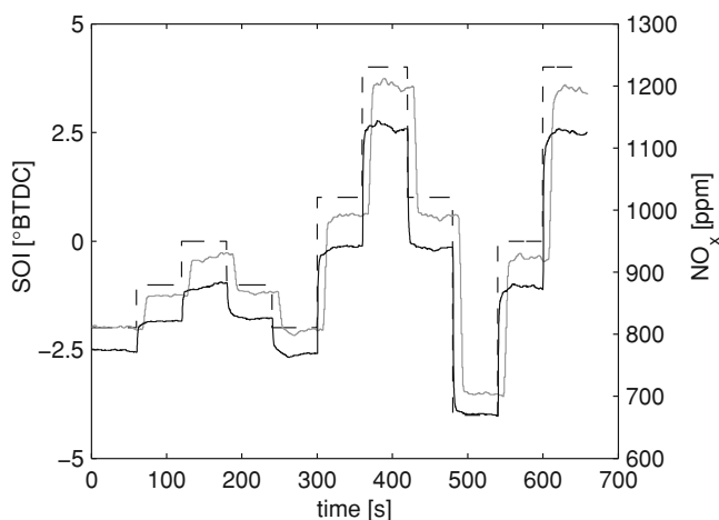
Fig. 3.16 \text{NO}_x concentration during a SOI step-like test at 2,000 rpm and 50 mg/stroke. Legend: dashed line is SOI, black line is the \text{NO}_x sensor ( z_{\text{NO}_x} ) before the steady-state calibration and gray line is the gas analyser. The difference in terms of delay, dynamics and steady-state values between both sensors is clearly noticed in the Figure
