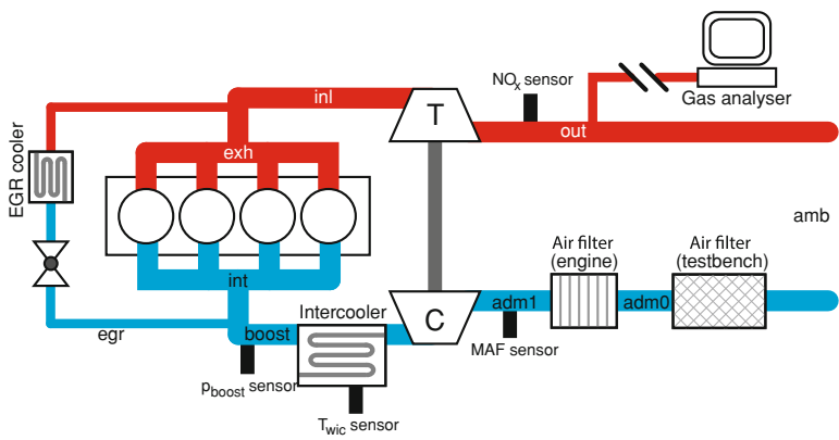
Fig. 3.1 Engine layout with the main sensors used in this work (pressures, temperatures in different positions are also measured but are not shown for clarity)
