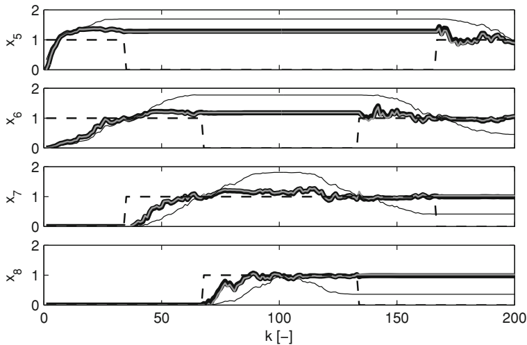
Fig. 5.14 States evolution for noisy measurements. Black thick line is KF, gray line is SKF, thin black is SSKF and dashed line shows when the element is active (1 is active; 0 is not active)
