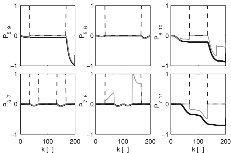
Fig. 5.12 P_{ij} analysis for a monotonically varied inputs sequence. Values are normalised by 100. Black line is KF, gray line is SKF and dashed line shows when the element is active (1 active; 0 is not active)
