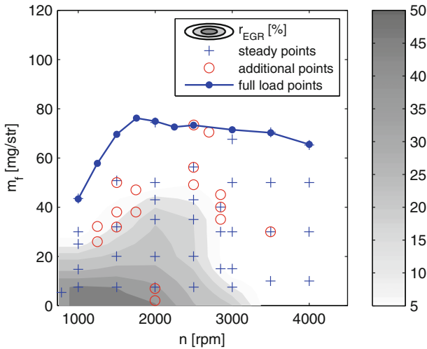
Fig. 3.5 [n, m_f] set of values run for testing the engine in steady-state. In each set, different variations of u_{egr} , T_{cool} , p_{boost} and T_{int} are made for characterizing the engine. Some additional points are measured for completing the engine characterization. Nominal EGR map EGR_0 (white area corresponds to EGR valve closed, EGR = 0 ) and full load line are also plotted
