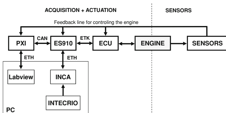
Fig. 3.2 System layout for rapid prototyping (fast acquisition, bypass and control) and integration of new sensors for testing the engine
