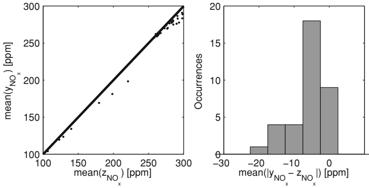
Fig. 4.18 Left mean value of NO x emissions, comparing the sensor z_{NO_x} against the model y_{NO_x} by simulating the NO x model in all the TRAN cycles. Right absolute error bar distribution of the model against the sensor \text{mean}(|y_{NO_x} - z_{NO_x}|) . The mean absolute error is less than 10 %
