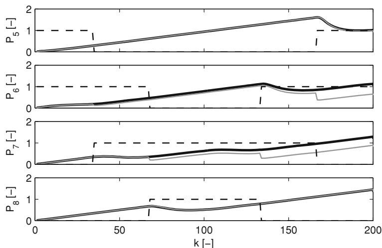
Fig. 5.11 P_{ii} analysis for a monotonically varied inputs sequence. Values are normalised by 100. Variances of elements 9–12 are equal to those of 5–9 because of symmetric properties. Black line is KF, gray line is SKF and dashed line shows when the element is active (1 active; 0 is not active)
