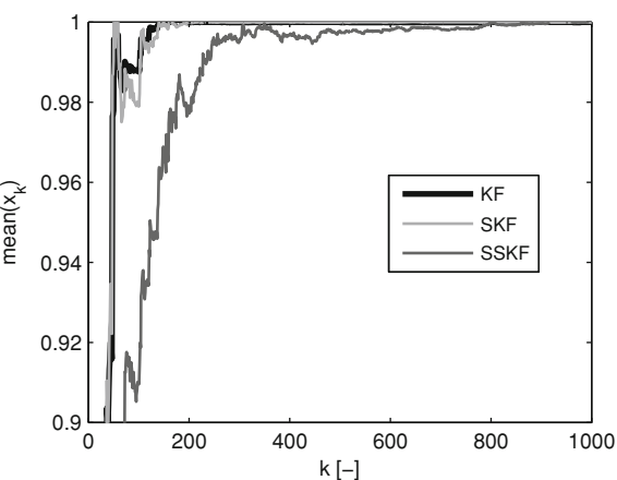
Fig. 5.8 Averaged value of table parameters for the three updating methods when considering an uniform distributed inputs sequence. The correct value is 1
