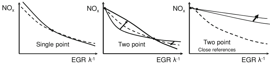
Fig. 4.7 Single point reference model ( left plot ) versus two-point reference models ( center and right plots )
