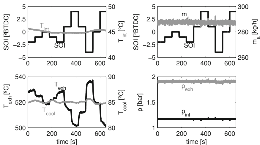
Fig. 3.17 Evolution of different engine variables during a SOI step-like test at 2,000 rpm and 50 mg/str
