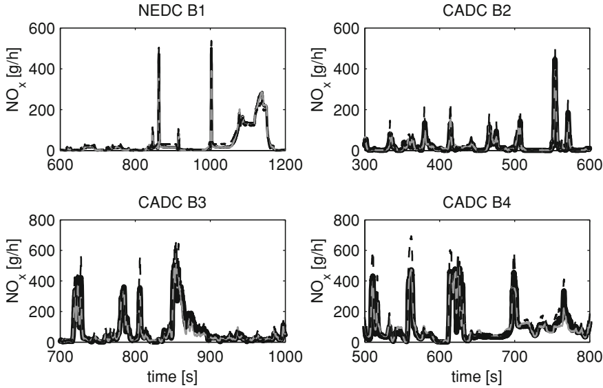
Fig. 6.18 Comparison of the NO x estimation by three different sources in 4 different cycles: sensor signal z_{NO_x} (black), y_{NO_x} by using the RT NO x model (dashed thin black) and y_{NO_x} computed by updating the NO_{x,0} table with the SKF method (gray). Left to right and top to bottom NEDC B1, CADC B2, CADC B3 and CADC B4 cycles
