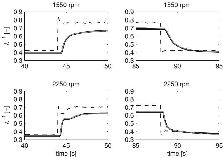
Fig. 3.21 Two sensor responses ( z_{\lambda^{-1}} in solid lines) for injection steps from 15 to 30 mg/str (left plots) and the opposite (right plots) at 1,550 rpm (top plots) and 2,250 rpm (bottom plots). The model x_{\lambda^{-1}} is provided for comparison (dashed black)
