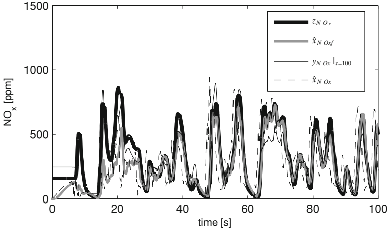
Fig. 6.19 \text{NO}_x estimation by three ways: z_{\text{NO}_x} sensor measurement, online observation of the sensor signal by the SKF method \hat{x}_{\text{NO}_xf} , offline prediction y_{\text{NO}_x} by using the map \Theta_{\text{NO}_x,100} and online actual estimation \hat{x}_{\text{NO}_x}
