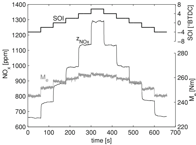
Fig. 3.20 \text{NO}_x concentration measured by the \text{NO}_x sensor ( z_{\text{NO}_x} ) and torque evolution ( M_e ) at 2,000 rpm and 50 mg/stroke when varying SOI
