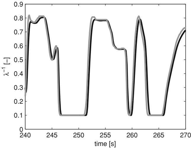
Fig. 6.3 z_{\lambda^{-1}} measurements from two \text{NO}_x sensors, the first located downstream of the turbine (gray) and the second downstream of the AT line (black) in an engine equipped with DOC, SCR and DPF (see the third configuration of Fig. 5.1). Both sensors are the same commercial model and present a saturation in approximately \lambda^{-1} = 0.1
