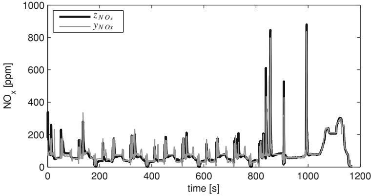
Fig. 6.14 Adaptive \text{NO}_x estimation in the NEDC A01, where it is estimated with a table that is updated during the whole cycle and then used for simulating y_{\text{NO}_x} . z_{\text{NO}_x} is provided for comparison. The estimation keeps the dynamic properties of z_{\text{NO}_x} but after updating, the drift in Fig. 4.19 is cancelled
