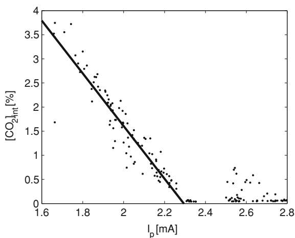
Fig. 3.4 Equivalency between [\text{CO}_2]_{\text{int}} and the pressure corrected signal I_p from the UEGO sensor. The saturation of the intake probe is evident for values of I_p around 2.3, i.e. equivalent to a low [\text{CO}_2]_{\text{int}} concentration
