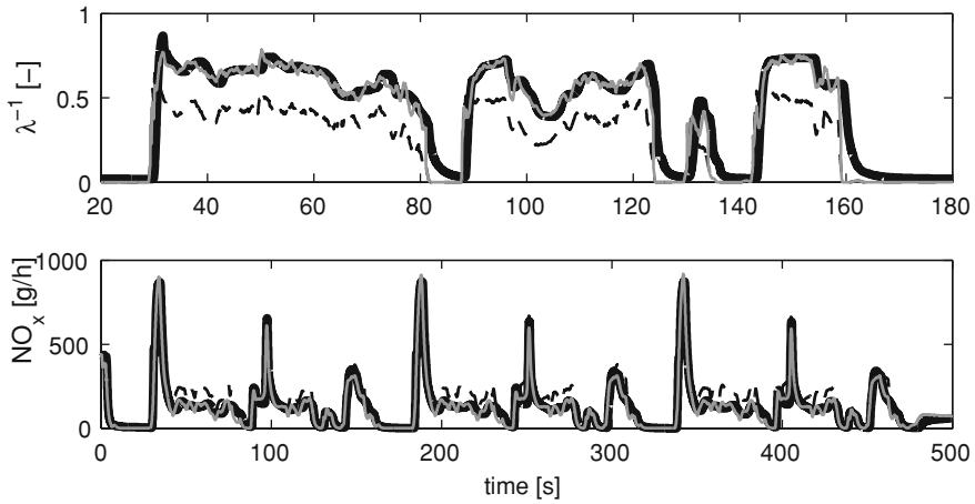
Fig. 6.17 \lambda^{-1} and NO x estimations in a TRAN B ( T_{cool} = nom , \Delta u_{egr} = 0\% , \Delta p_{boost} = 0 ). Top plot z_{\lambda^{-1}} sensor signal (black), x_{\lambda^{-1}} calculated by the model (dashed thin black) and \hat{x}_{\lambda^{-1}} observed by a drift augmented model (gray). Bottom plot NO x estimation by three ways, z_{NO_x} sensor signal (black), y_{NO_x} by the NO x model using x_{\lambda^{-1}} as input (dashed thin black) and y_{NO_x} by using an adaptive model with \hat{x}_{\lambda^{-1}} as \lambda^{-1} input
