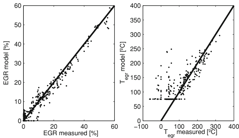
Fig. 4.15 Relevant results from the EGR flow model. Left plot EGR calculated by the model and from the gas analyser measurements. Right plot T_{egr} calculated by the model and measured by a sensor
