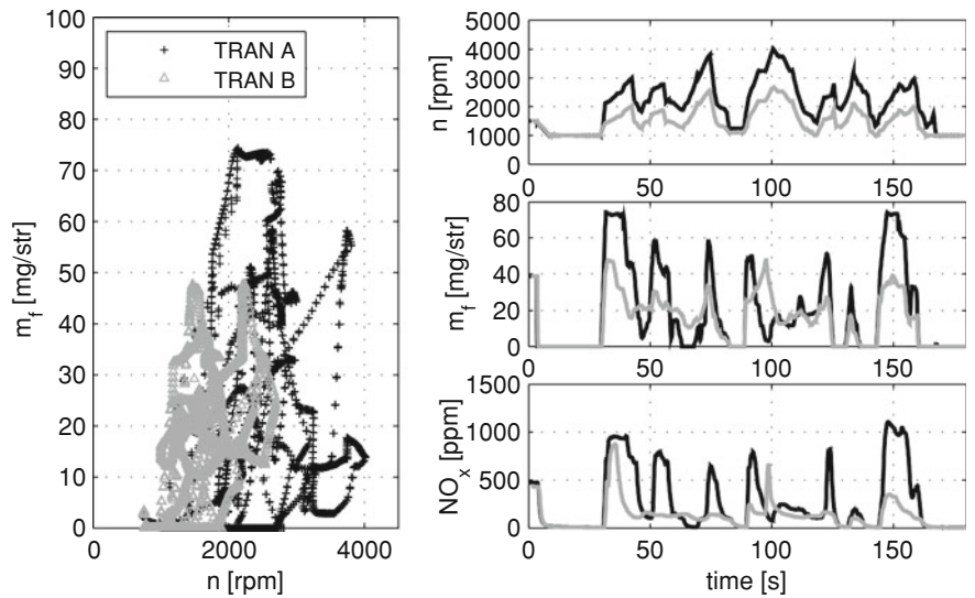
Fig. 3.6 TRAN nominal cycles designed for the model validation. TRAN A is the black line, while TRAN B is the grey line
