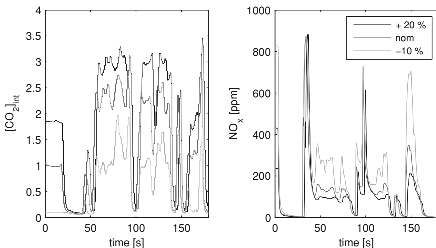
Fig. 3.7 [\text{CO}_2]_{\text{int}} at intake and \text{NO}_x emissions for TRAN B after varying the EGR set-point. The legend in the right plot shows the values of u_{\text{egr}} . Note that the higher u_{\text{egr}} the lower \dot{m}_{\text{egr}}
