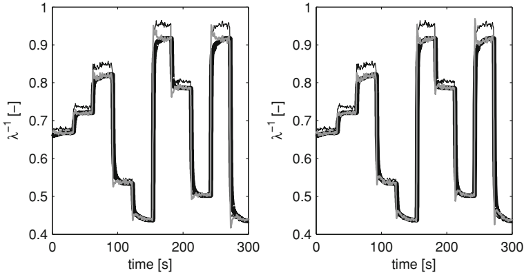
Fig. 6.6 \hat{x}_{\lambda-1} performing injection steps at 1,500 rpm without using a look-up table. Left plot Slow correction, with \sigma_w^2/\sigma_v^2 = 10^{-5} . Right plot Fast correction, with \sigma_w^2/\sigma_v^2 = 10^{-4} . Legend: Thick black is z_{\lambda-1} , thin black is x_{\lambda-1} and gray is \hat{x}_{\lambda-1}
