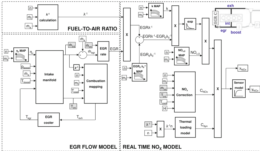
Fig. 4.8 Structure of the RT NO x model, where the main blocks are depicted: the EGR flow model (or air path model), the fuel-to-air ratio calculation and the proper NO x model calculation. The model inputs (coming from ECU signals) are marked with squares with white front , while the squares with gray front are used as short-cuts for linking intermediate variables in the model. At the top right , the legend for the engine positions is shown
