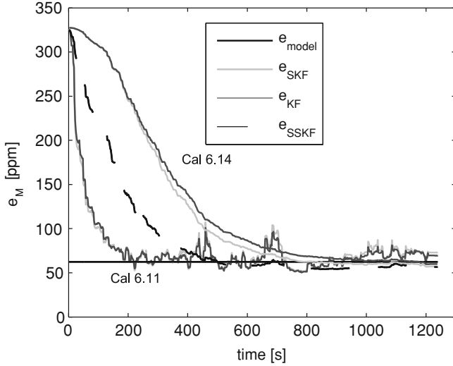
Fig. 6.12 Evolution of the mean of the absolute error e_M for the different methods in the SDMP B5 cycle and for two different filter calibrations. SSKF dashed line is calculated by using the filter calibration (6.11). Lines left to the SSKF one using calibration (6.11). During first iterations, the error is high, as far as the table has no initial knowledge, but once that the time is around 400 s, the error is minimum, although the noise transmission is evident. Lines right to the SSKF one using calibration (6.14), noise transmission is reduced but the convergence speed as well. The chosen filter tuning must be a trade-off between the robustness and convergence speed
