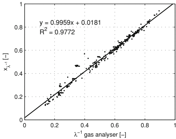
Fig. 4.1 x_\lambda^{-1} and \lambda^{-1} from the gas analyser for different steady operating conditions; the linear fit and correlation coefficient are represented
