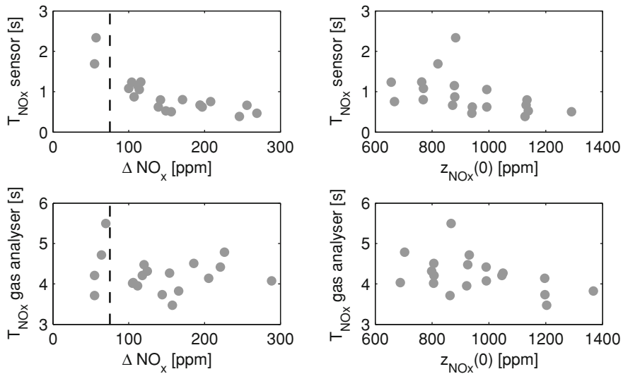
Fig. 3.19 Response time T_{\text{NO}_x} for the NO x sensor as function of the concentration step \Delta \text{NO}_x and the initial concentration z_{\text{NO}_x}(0)
