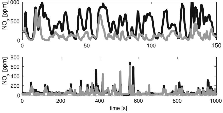
Fig. 6.16 Offline \text{NO}_x prediction y_{\text{NO}_x} (gray) against \text{NO}_x sensor (black) by using a table \Theta_{\text{NO}_x} updated online in the NEDC B1 cycle. Top plot results in the SDMP B6 cycle. Bottom plot results in the CADC B2 cycle
