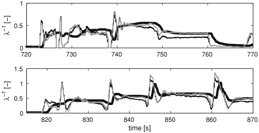
Fig. 6.9 Top and bottom \hat{x}_{\lambda^{-1}} using the table and applying freezing conditions to the NEDC B01 cycle. z_{\lambda^{-1}} is the sensor output ( thick black ), x_{\lambda^{-1}} is the model output ( thin black ) and \hat{x}_{\lambda^{-1}} is the observation ( gray ). The drift is corrected while the dynamics of the observation \hat{x}_{\lambda^{-1}} are maintained
