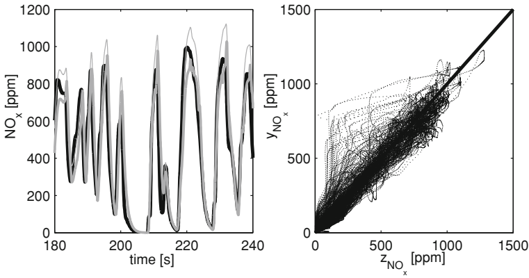
Fig. 4.16 Left y_{NO_x} calculated normally (thick gray) and cancelling thermal dynamic factor; i.e. C_{dyn} = 1 (thin gray), and z_{NO_x} (black) during a part of the SDMP B5. Right y_{NO_x} against z_{NO_x}
