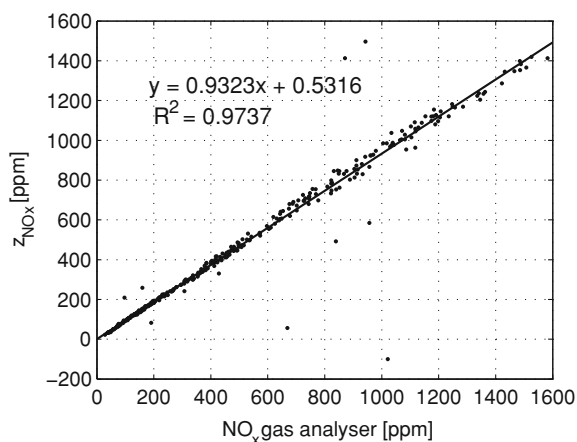
Fig. 3.14 \text{NO}_x from \text{ZrO}_2 sensor ( z_{\text{NO}_x} ) and the gas analyser under different steady operating conditions; the linear fit and correlation coefficient are represented
