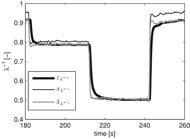
Fig. 6.8 \hat{x}_{\lambda^{-1}} using table and freezing conditions performing different injection steps at 1,500 rpm
