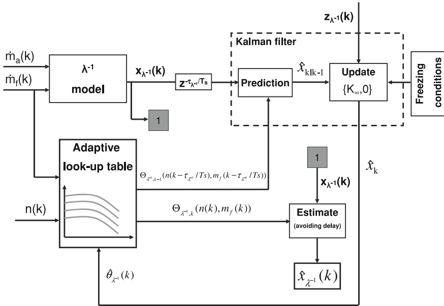
Fig. 6.2 Schematic view of the proposed procedure for \lambda^{-1} estimation
