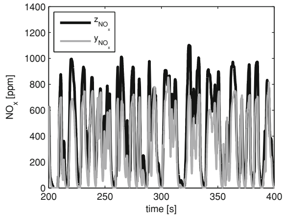
Fig. 5.2 Model output y_{\text{NO}_x} and \text{NO}_x sensor signal z_{\text{NO}_x} in the SDMP B6 test with a non-optimized calibration data set. Even though the dynamics are well caught, y_{\text{NO}_x} is biased with respect to z_{\text{NO}_x}
