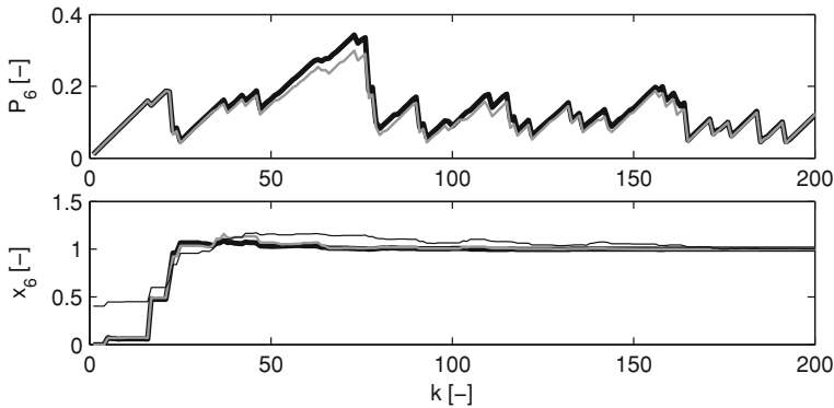
Fig. 5.9 Variance analysis for an uniform distributed inputs sequence. Top Variance evolution of the 6th element P_6 where black thick line is the KF and gray line is the SKF ( P_6 is normalised by 100 in both cases). Bottom x_6 value where black thick line is the KF, gray line is the SKF, thin black is the SSKF
