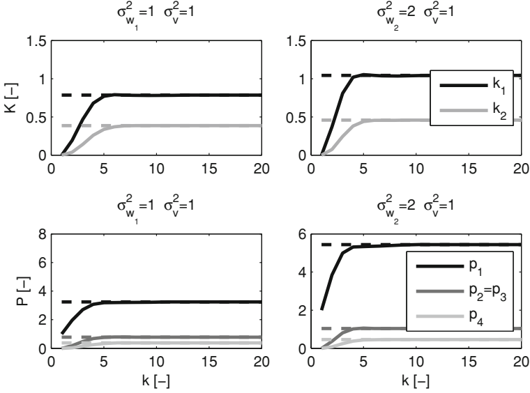
Fig. A.1 Kalman gain K and covariance matrix P calculation for two noise sets with a = 0.8 . Solid lines corresponds to the standard Kalman formulation by the iterative Riccati equation (2.13a, b, c), while dashed lines correspond to the proposed analytical formulation ((A.19) for K and (A.20) for P )
