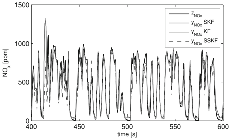
Fig. 6.11 NO x prediction for the three methods by performing the SDMP B5 cycle. The maps are updated during 400 s, i.e. a subset of 20,000 measurements of z_{\text{NO}_x} . y_{\text{NO}_x} is simulated with the updated tables at 400 s \Theta_{\text{NO}_x,400} . The sensor measurement z_{\text{NO}_x} is provided for comparison
