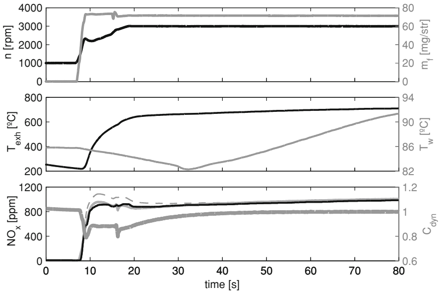
Fig. 4.11 \text{NO}_x and thermal response during a sharp transient. Top plot n and m_f evolution. Middle plot exhaust temperature ( T_{\text{exh}} ) and coolant temperature ( T_{\text{cool}} ) during the transient. Dynamics of both signals, especially for T_{\text{cool}} , are slow, which affects final \text{NO}_x . Bottom plot and left axis : black line z_{\text{NO}_x} by sensor, gray dashed line y_{\text{NO}_x} with C_{\text{dyn}} = 1 , thin gray line y_{\text{NO}_x} using C_{\text{dyn}} . Bottom plot and right axis : thick gray line C_{\text{dyn}} factor calculated by the thermal model
