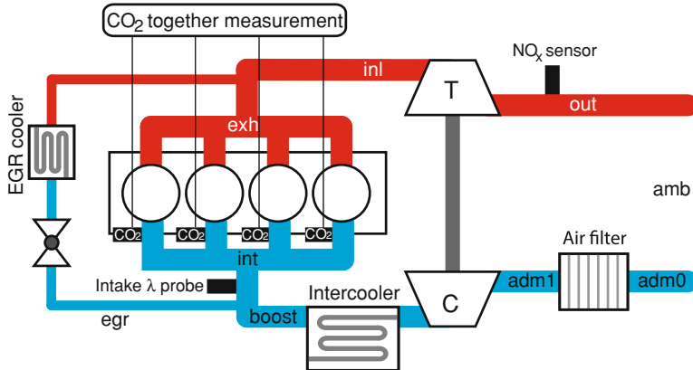
Fig. 3.3 Engine layout showing the main sensors used for measuring [O_2]_{int} or equivalently [CO_2]_{int}
