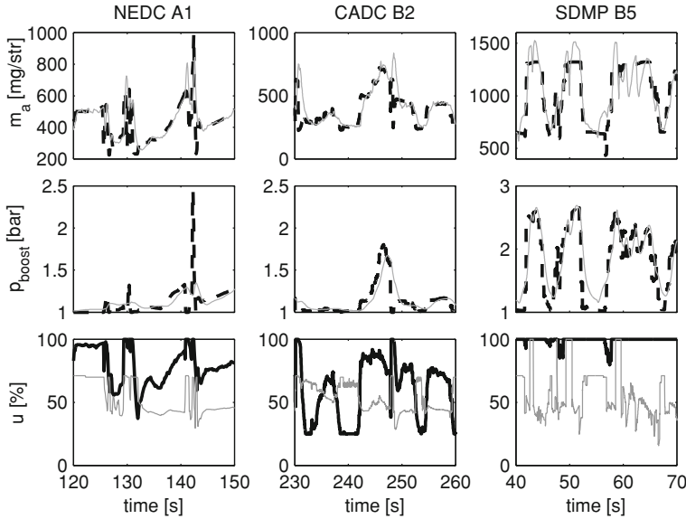
Fig. 4.3 Air and fuel path response to variations in the driver's command ( u_\alpha ) for different cycles. First and second row plots: dashed line is set-point \dot{m}_a^* and p_{boost}^* , and gray line is measured value of \dot{m}_a and p_{boost} . Last row plots: gray line u_{wg} [mg/str], black line u_{egr} [mg/str] is the smoke limit for injection. Note that 100 % in u_{egr} corresponds to the EGR valve fully closed and around 25 % the EGR mass flow is maximum (the relation between u_{egr} command and the effective area is not linear). For the case of u_{wg} , 100 % corresponds to WG fully closed and the two turbo shafts working
