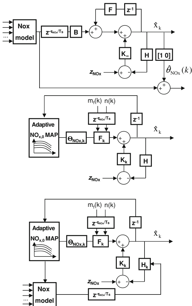
Fig. 6.1 From top to bottom , algorithms 1 to 3: drift correction model, adaptive table for \text{NO}_x estimation and adaptive \text{NO}_x model
