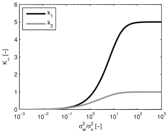
Fig. 5.3 Evolution of the elements of K_\infty gain vector when varying \sigma_w^2/\sigma_v^2 . Coordinate axis is in logarithmic scale and a = 0.8
