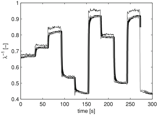
Fig. 6.7 \hat{x}_{\lambda-1} performing injection steps at 1,500 rpm and using an adaptive look-up table for modelling \theta_{\lambda-1} . Legend: Thick black is the sensor z_{\lambda-1} , thin black is the model x_{\lambda-1} and gray is \hat{x}_{\lambda-1} . Values for tuning the KF are \sigma_w^2/\sigma_v^2 = 1/80
