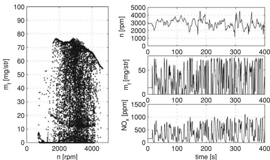
Fig. 3.8 SDMP cycle performed on the engine
