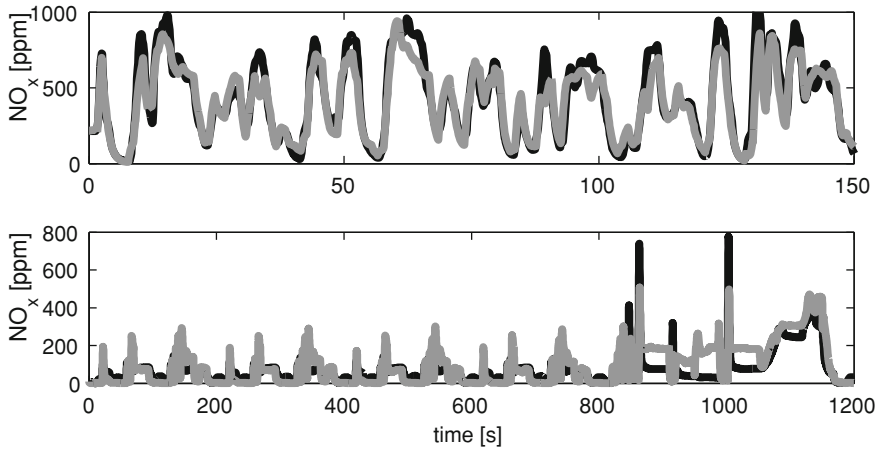
Fig. 6.15 Offline NO x prediction y_{\text{NO}_x} (gray) against NO x sensor (black) by using a table \Theta_{\text{NO}_x} updated online in the SDMP B5 cycle. Top plot results in the SDMP B6 cycle. Bottom plot results in the NEDC B1 cycle
