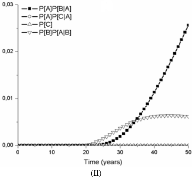
Figure 11. Failure modes due to the carbonation corrosion – Application 1: (I) individual probabilities; (II) failure paths.
