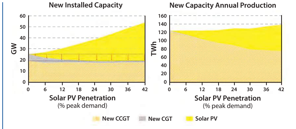
Figure 8.14 Evolution of Installed Capacity and Corresponding Annual Energy Production (California-Like System)
