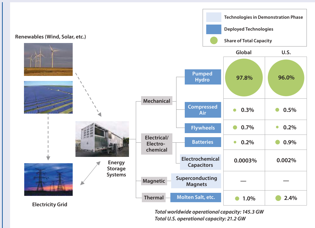
Figure C.1 Grid-Related Energy Storage Technologies Deployed or in the Demonstration Phase ii
