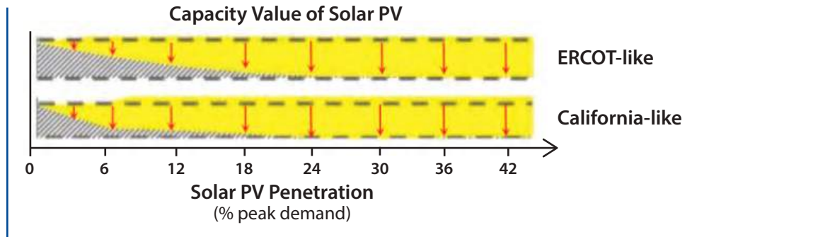
Figure 8.15 Capacity Value of Solar PV in the ERCOT and California Systems
