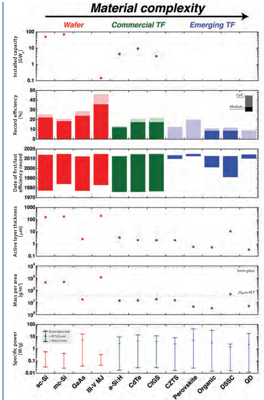
Figure 2.8 Key Metrics for Photovoltaic Technologies Ordered by Material Complexity
