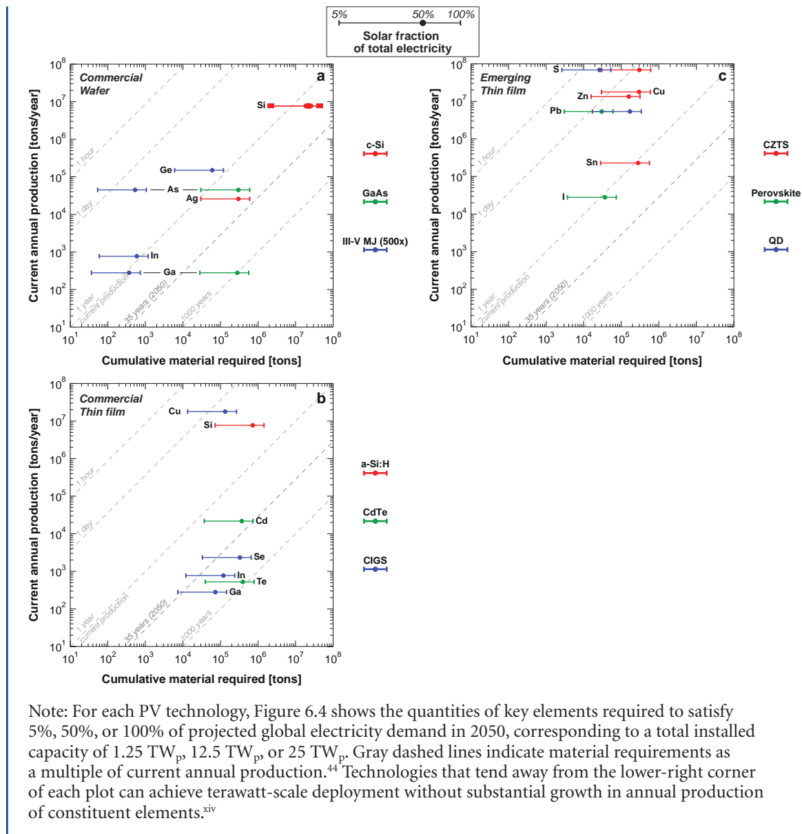
Figure 6.4 Critical Materials Requirements for Large-Scale Deployment of Different PV Technologies
