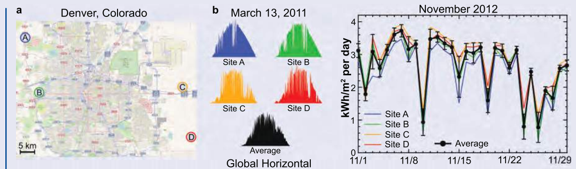
Figure A.7 Irradiance Profiles at Four Sites in the Denver Area
