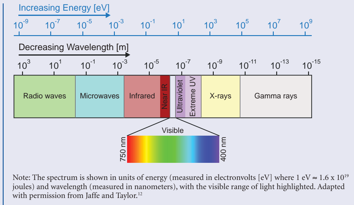
Figure B.2 The Electromagnetic Spectrum
