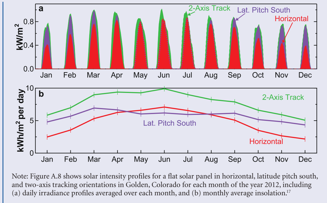
Figure A.8 Daily Irradiance and Monthly Insolation Profiles for Different Solar Panel Arrangements
