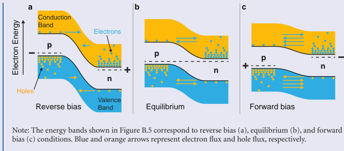
Figure B.5 Energy Bands during Operation of a pn-Junction Diode
