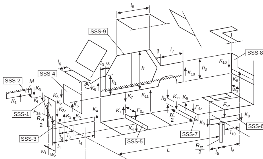
Figure 6.23 SSS model, saloon car – bending
