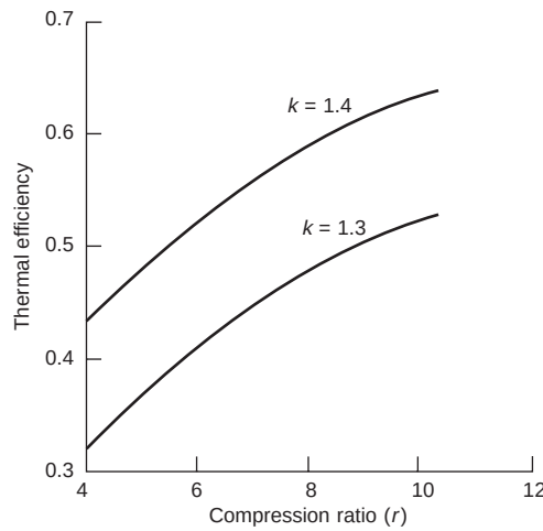
Figure 12.2 The influence of compression ratio r on the ideal cycle thermal efficiency for different values of the polytropic exponent
