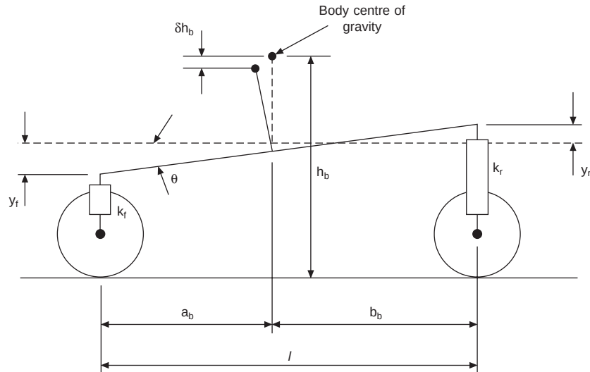
Figure 14.16 Determination of vehicle body pitch angle
