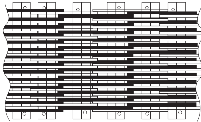
Figure 13.29 The LuK-PIV chain construction
