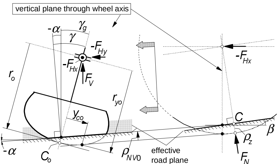
Fig. 9.71 . Situation with wheel camber \gamma and road camber \alpha at a forward slope \beta .
