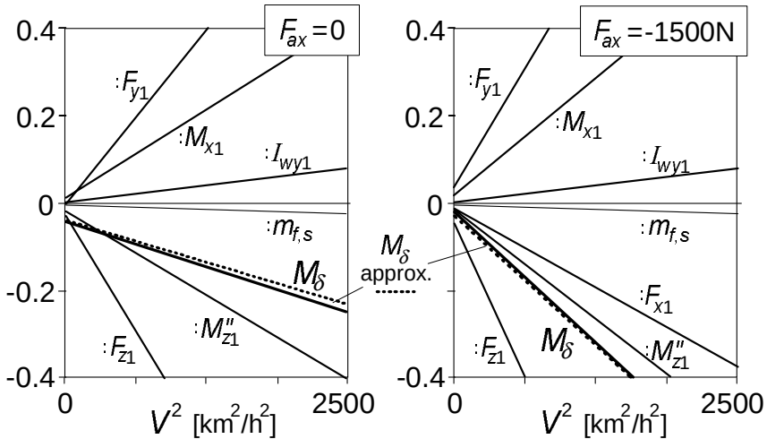
Fig. 10.20. The non-dimensional steer torque ( M_\delta/(F_{z1}l) ) and its components (cf. Eq.(10.147)) per unit non-dimensional path curvature 1/R . In M''_{z1} the F_{x1} contribution is omitted.
