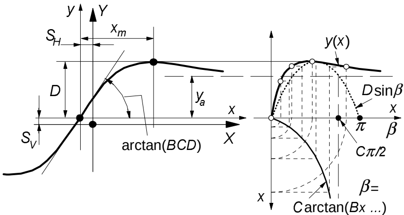
Fig. 4.9. Curve produced by the original sine version of the Magic Formula, Eqs.(4.49). The meaning of curve parameters have been indicated.
