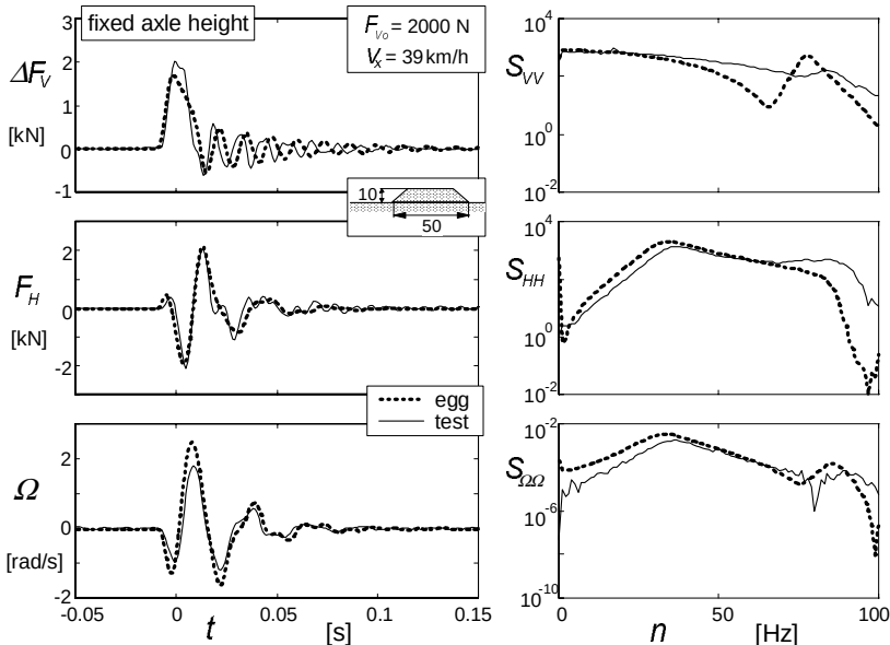
Fig. 9.64. Time traces and power spectra of vertical force, horizontal longitudinal force and angular velocity for wheel running at given speed of 39 km/h and initial vertical load of 2000 N over trapezium cleat at constant axle height using SWIFT tyre parameters and obstacle parameters of Table 9.6. (Schmeitz).
