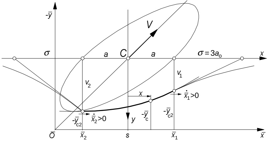
Fig. 5.47. On the development of the contact line of the bare string model.
