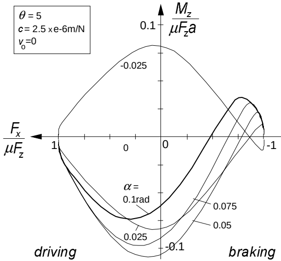
Fig. 3.20. The influence of lateral carcass compliance on the aligning torque for a braked or driven wheel according to the extended brush model.
