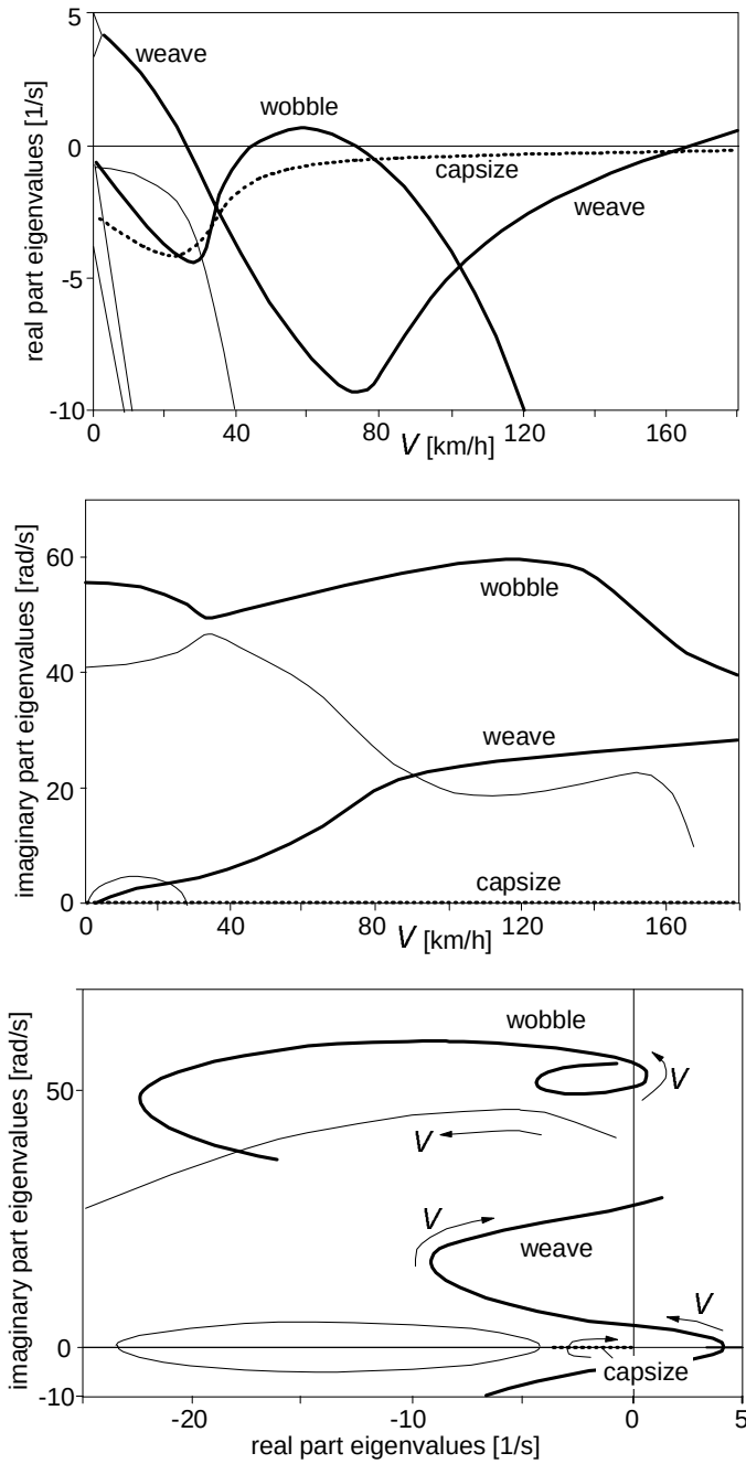
Fig. 10.7. Baseline configuration (rigid rider, with air drag, zero forward acceleration, no control). Real and imaginary parts of eigenvalues versus speed of travel V .
