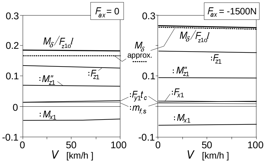
Fig. 10.21. The non-dimensional steer torque ( M_\delta/(F_{z1}l) ) and its components (cf. Eq.(10.147)) per m.c.g. lateral offset y_{mv} . In M''_{z1} the F_{x1} contribution is removed.
