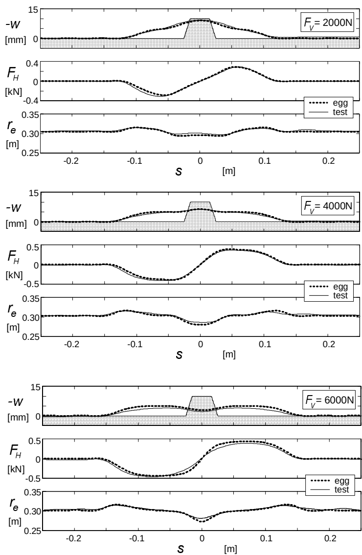
Fig. 9.63. Rolling over a trapezium cleat (length:50mm, height: 10mm). Measured and calculated variation of vertical axle displacement, horizontal longitudinal force and effective rolling radius at three different constant vertical loads. Measurements carried out on the Delft flat plank machine (very low speed) and calculations conducted with the use of the tandem egg technique (Fig.9.56) and Eq.(9.258). Tandem egg parameters according to Table 9.6.
