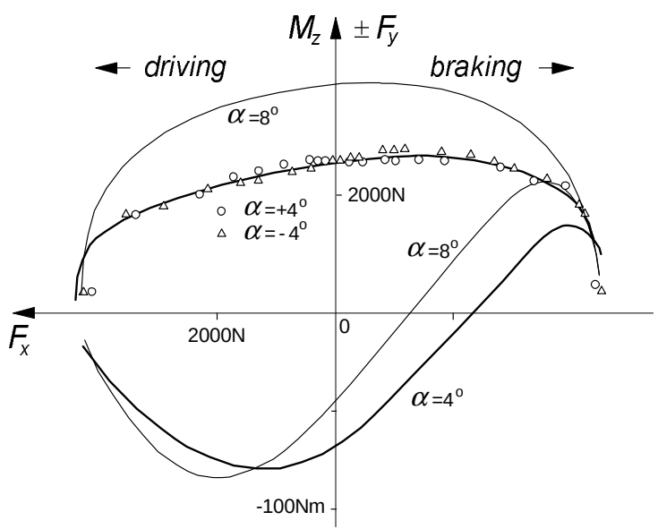
Fig. 3.17. F_y - F_x characteristics for 6.00-13 tyre measured on dry internal drum with diameter of 3.8m (from Henker 1968).
