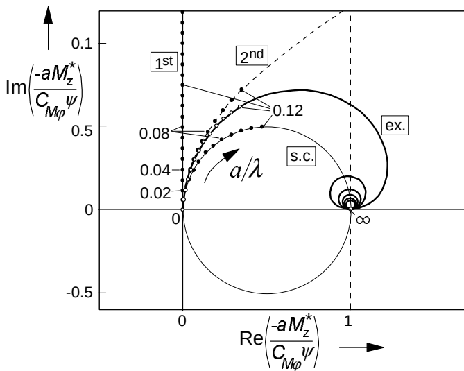
Fig.5.26. Nyquist plot of the frequency response function of the torque due to tread width -M_z^* with respect to the wheel yaw angle \psi . ex.: exact (brush); s.c.: straight connection (linear interpolation); 2nd: second-order app.; 1st: first-order approx.
