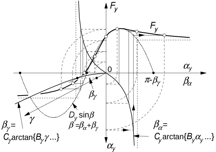
Fig. 10.30. The structure of the for motorcycle tyres adapted Magic Formula rendering the side force versus slip angle characteristic for a given camber angle.
