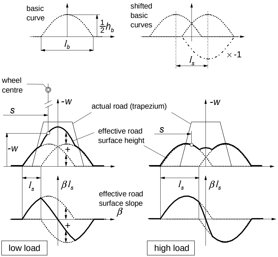
Fig. 9.49. The construction of the curves representing the effective height end effective slope of the local road plane from the basic function associated with the trapezium cleat.
