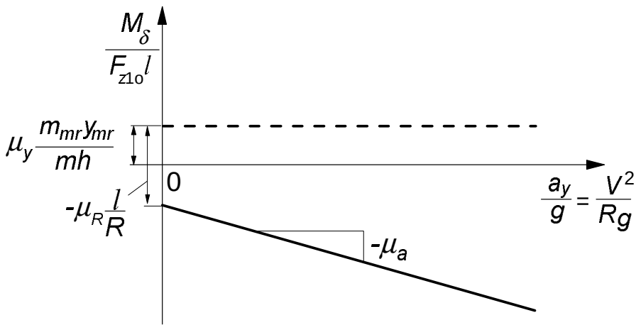
Fig. 10.19. The non-dimensional steer torque due to path curvature 1/R and c.g.lateral offset y_{mr} and the variation with lateral acceleration a_y or speed V .
