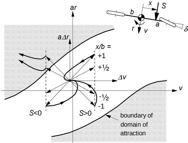
Fig. 1.25. Large disturbance in a curve. New initial state vector ( \Delta v, \Delta r ) after the action of a lateral impulse S . Once outside the domain of attraction the motion becomes unstable and may get out of control.
