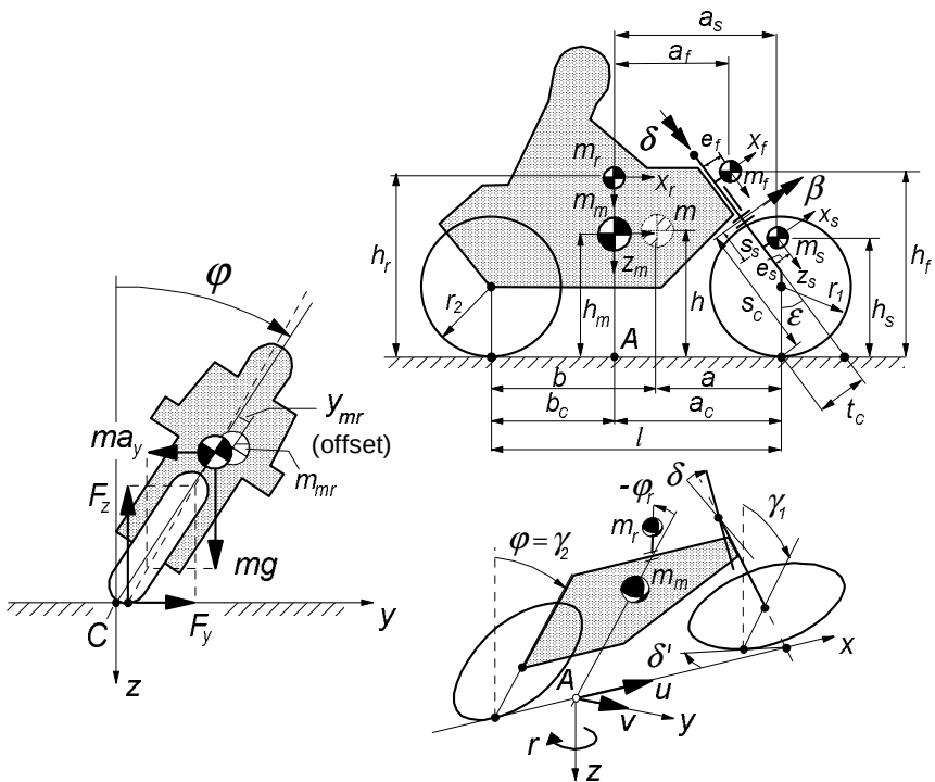
Fig. 10.1. Motorcycle model configuration.
