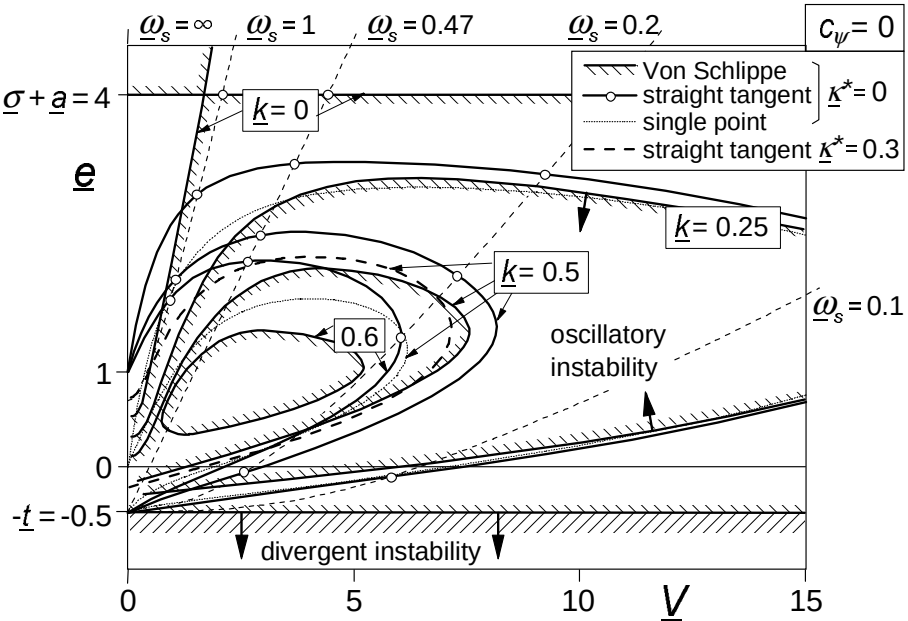
Fig. 6.2. Areas of instability for the trailing wheel system of Fig. 6.1 without steer stiffness at different levels of viscous steer damping. Consequences of using different tyre models can be observed.
