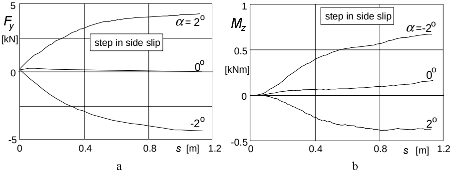
Fig. 5.11. Step response of side force F_y and aligning torque M_z to slip angle \alpha as measured on an aircraft tyre with vertical load F_z = 35\text{ kN} . (From Besselink, 2000; test data is provided by Michelin Aircraft Tire Corporation).
