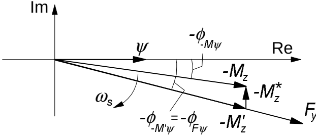
Fig.5.16. Complex representation of side force and moment response to yaw oscillations \psi .
