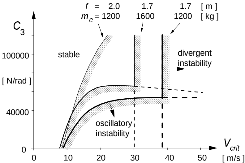
Fig. 1.30. Stability boundaries for the car caravan combination in the caravan cornering stiffness versus critical speed diagram. Vehicle parameters according to Table 1.1, in addition: h = 2 m, g = 2 m, k_c = 1.5 m ( I_c = m_c k_c^2 ), cf. Fig. 1.29.
