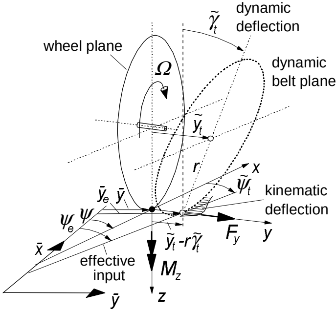
Fig. 5.39. 'Dynamic' average plane deflection of belt and associated effective input.
