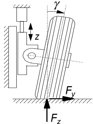
Fig. 7.14. Cambered wheel moved up and down (Exercise 7.1).
