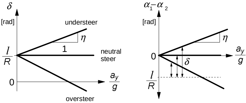
Fig. 1.10. The steer angle versus lateral acceleration at constant path curvature (left graph). The difference in slip angle versus lateral acceleration and the required steer angle at a given path curvature (right graph). The understeer gradient \eta .
