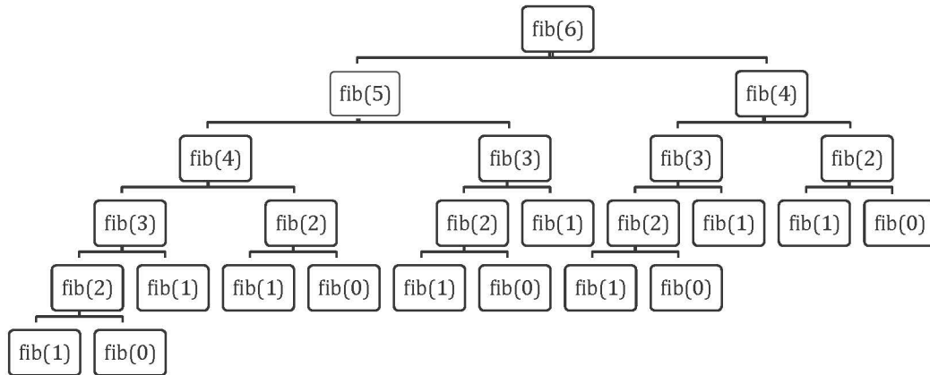
Figure 18.1 Tree of calls for recursive Fibonacci
