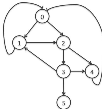
Figure 17.8 Depth-first-search shortest path algorithm
