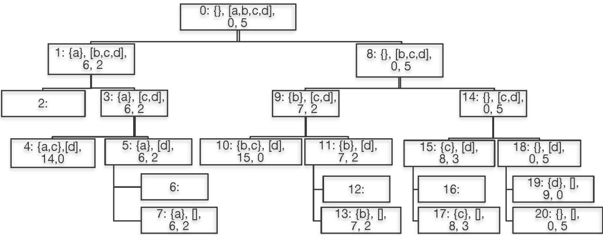
Figure 18.4 Decision tree for knapsack problem
