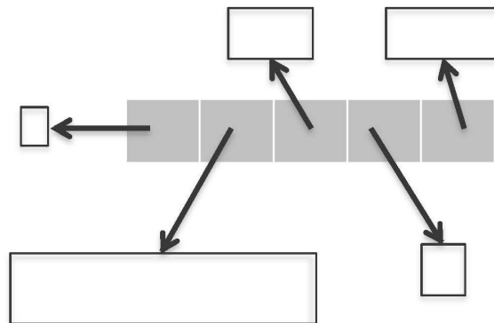
Figure 10.1 Implementing lists
