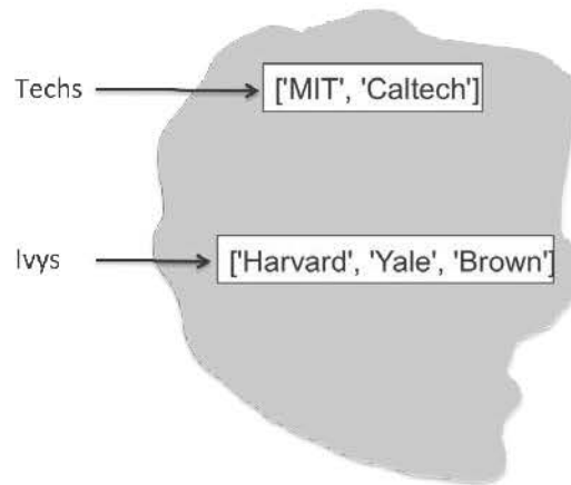
Figure 5.1 Two lists
