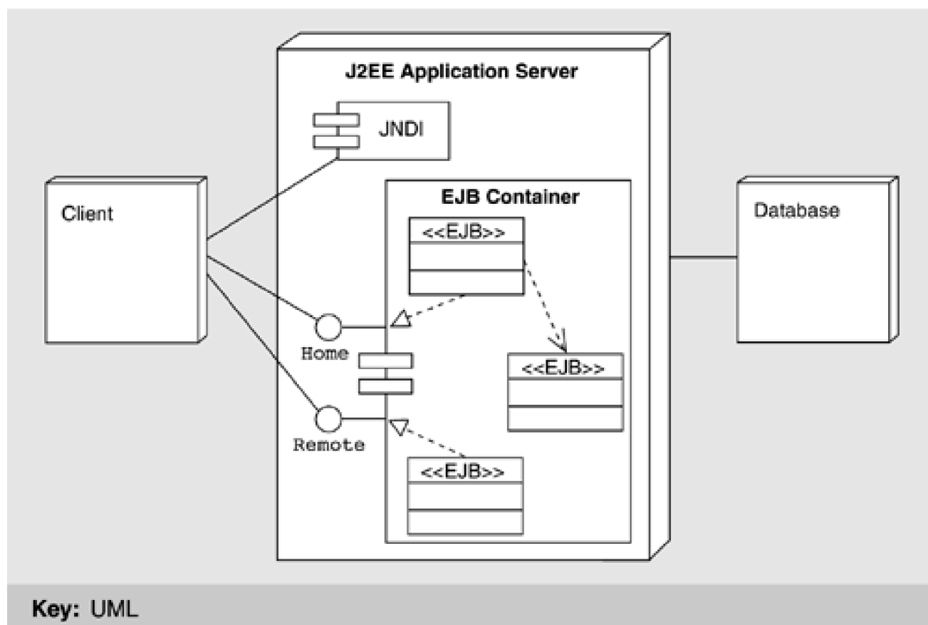
Figure 16.3. Example deployment view of the EJB architecture
