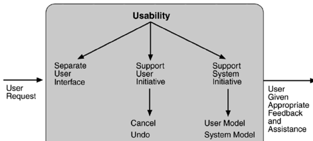
Figure 5.13. Summary of runtime usability tactics
