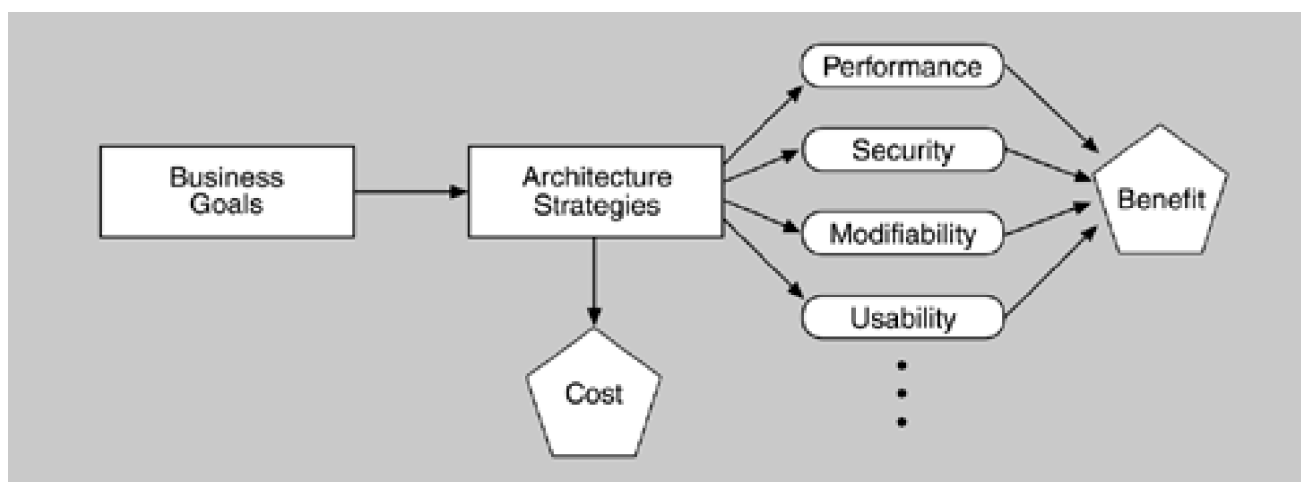
Figure 12.1. Context for the CBAM
