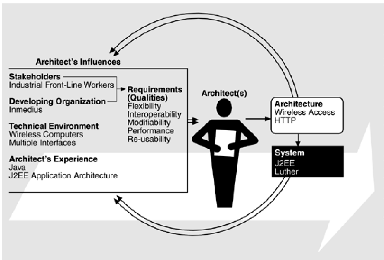
Figure 17.1. The ABC as it pertains to Inmedius and Luther
