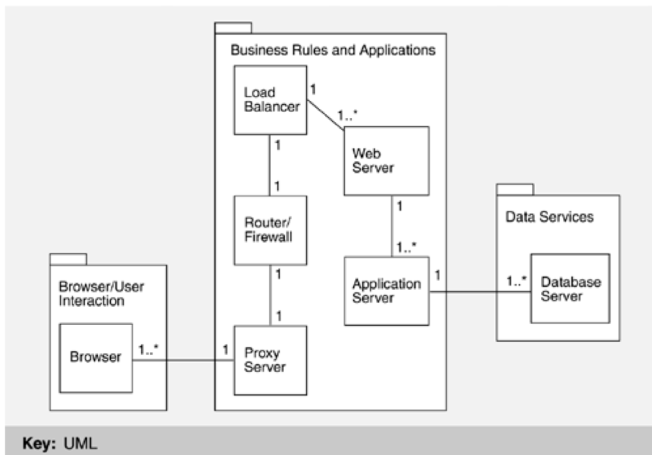
Figure 13.7. A typical e-commerce system
