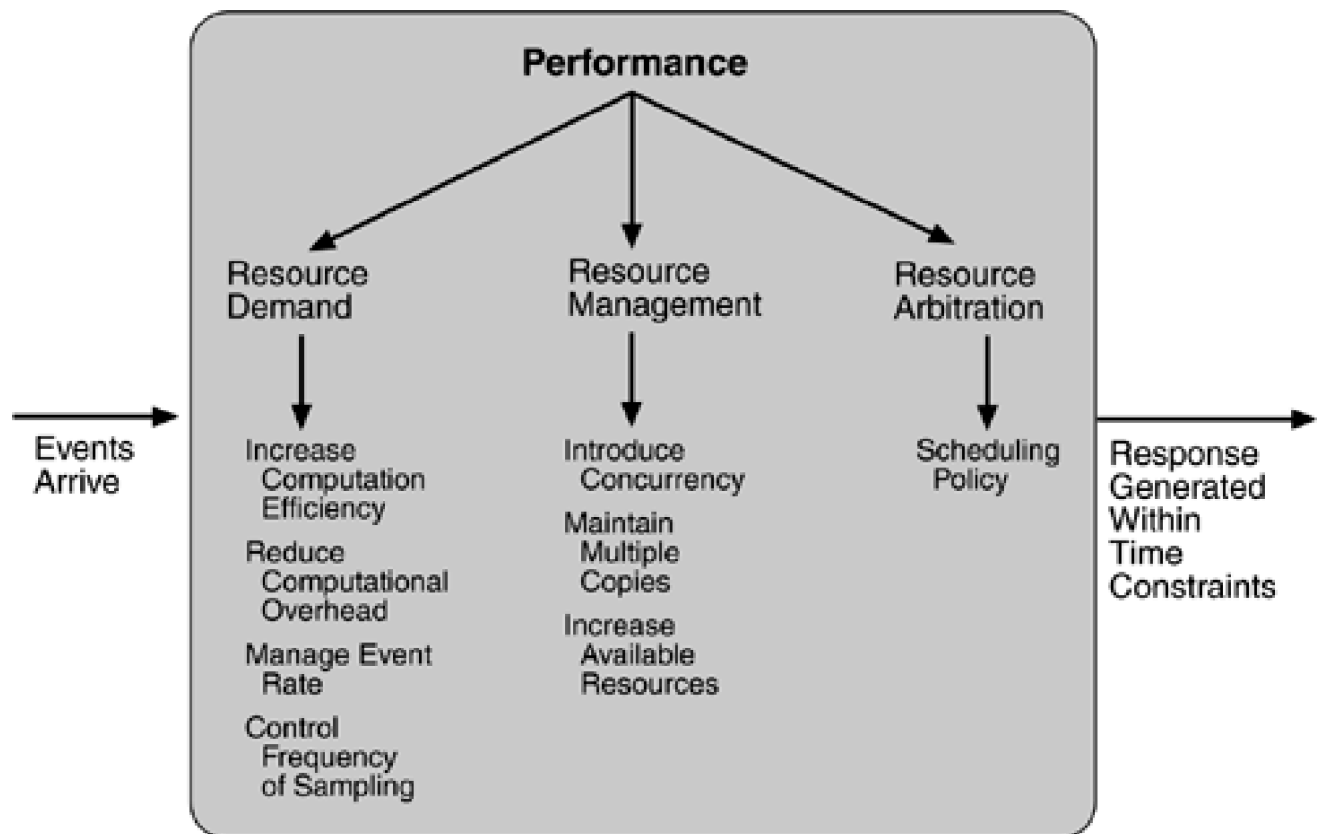
Figure 5.7. Summary of performance tactics
