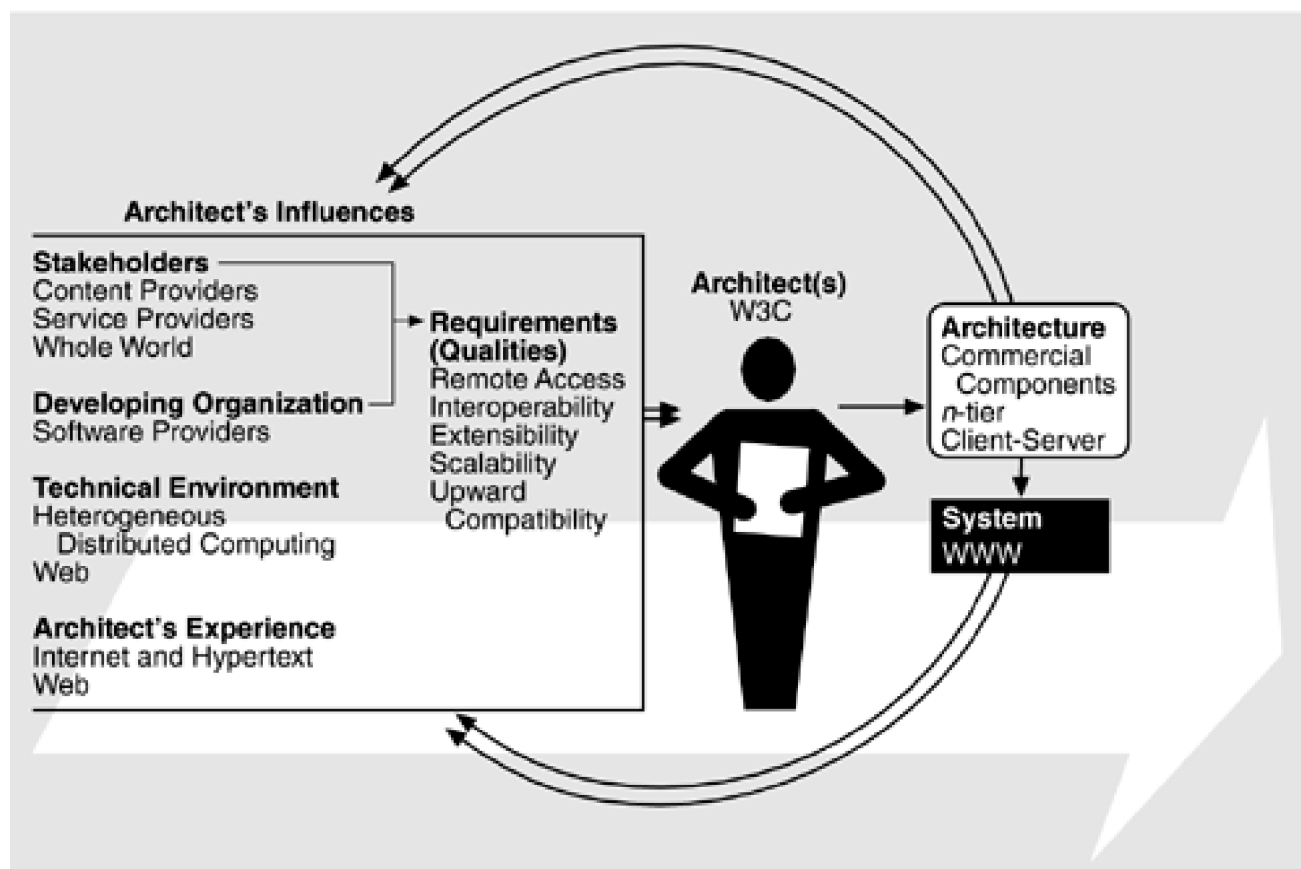
Figure 13.8. The current ABC for the Web
