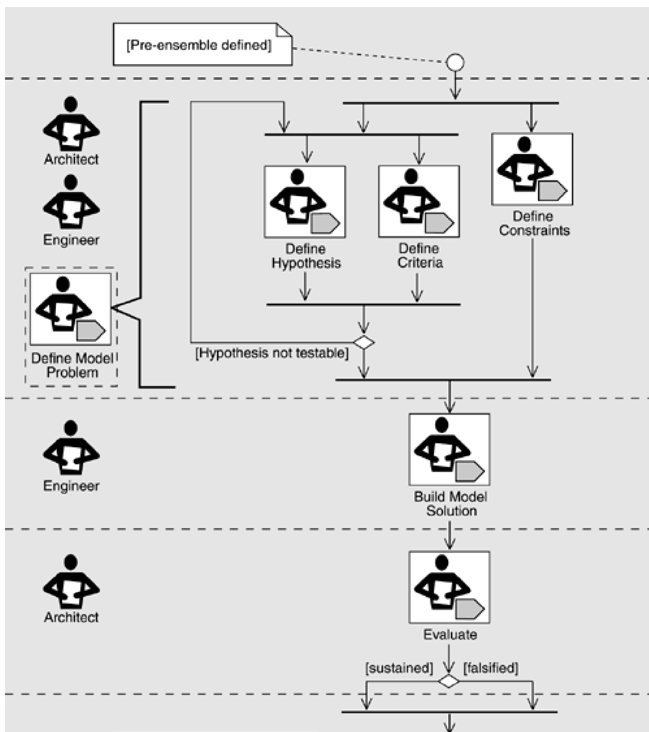
Figure 18.1. Model problem work flow
