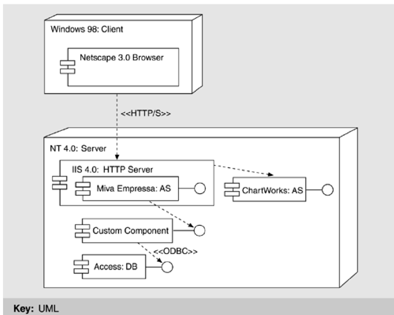
Figure 18.2. Miva Empressa ensemble
