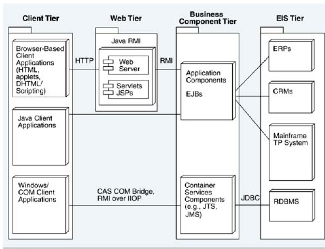
Figure 16.2. Deployment view of the J2EE multi-tier architecture
