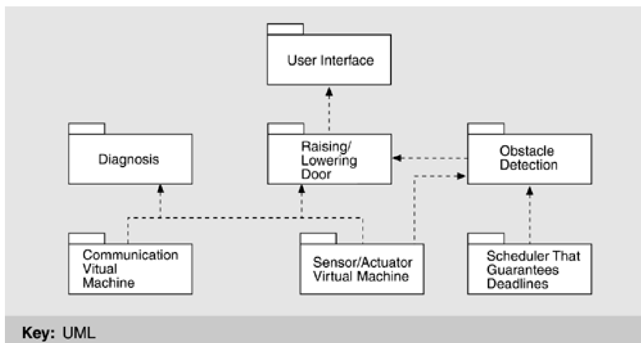
Figure 7.3. First-level decomposition of garage door opener
