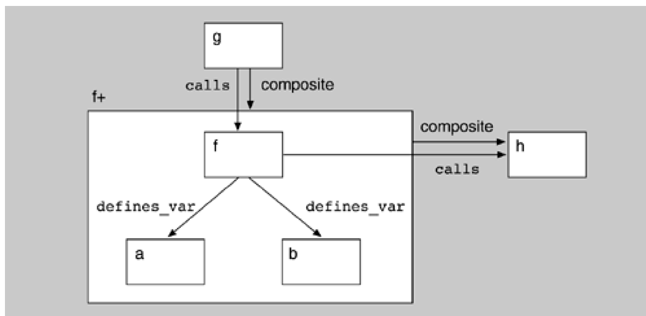
Figure 10.10. Result of applying the code segment in Figure 10.9
