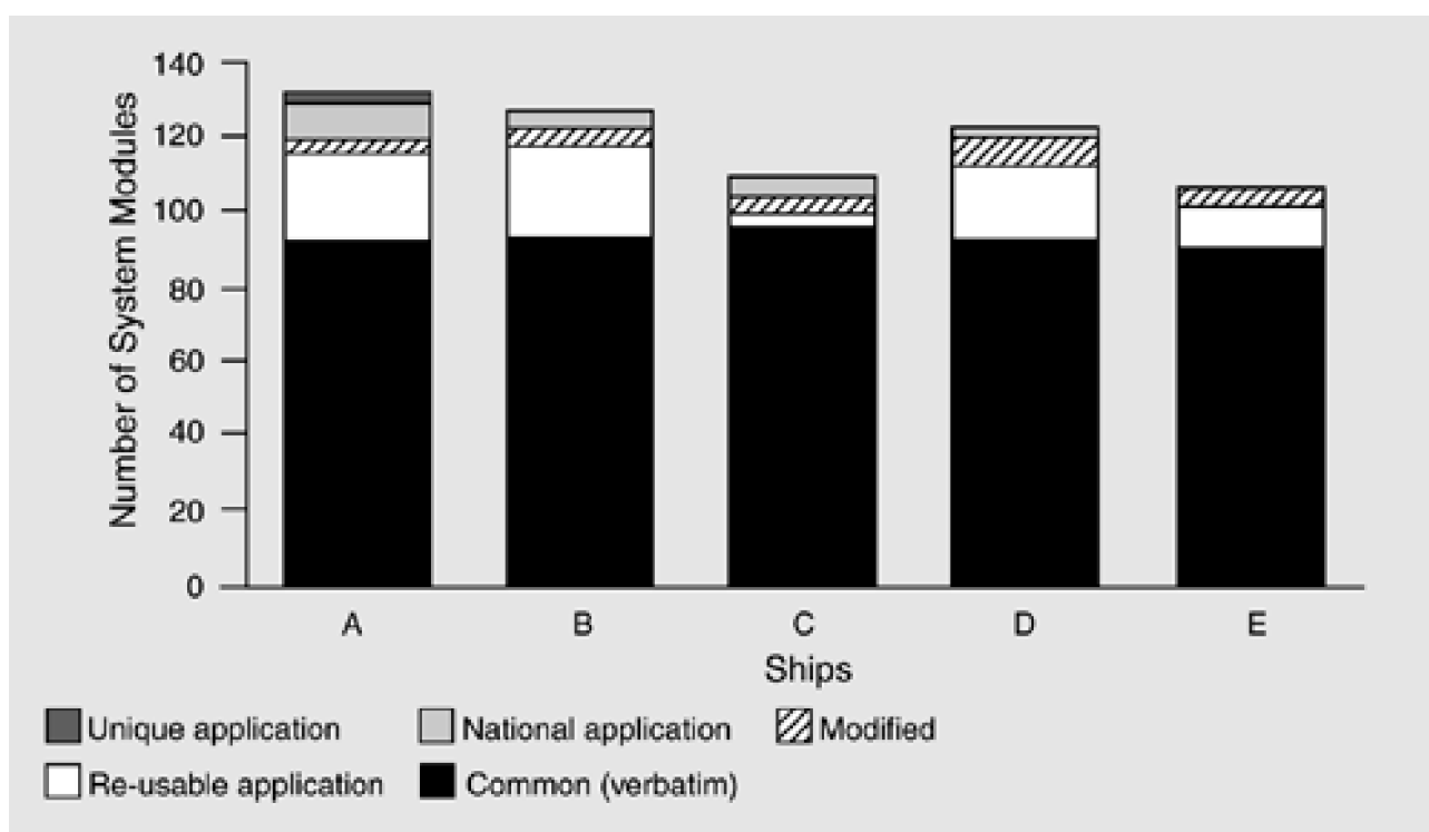
Figure 15.5. Commonality across CelsiusTech naval systems
