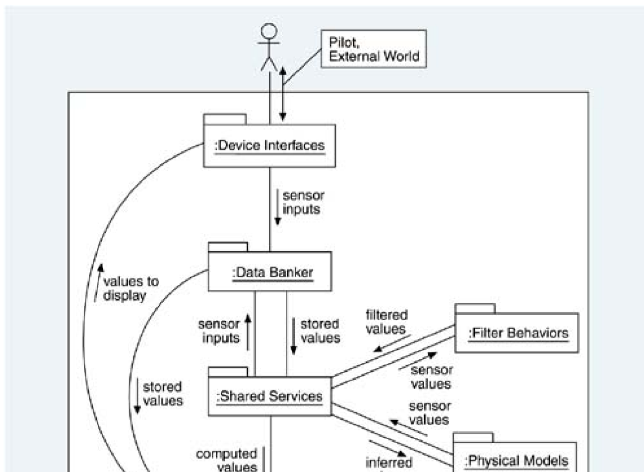
Figure 3.5. Coarse-grained data flow view for the A-7E software
