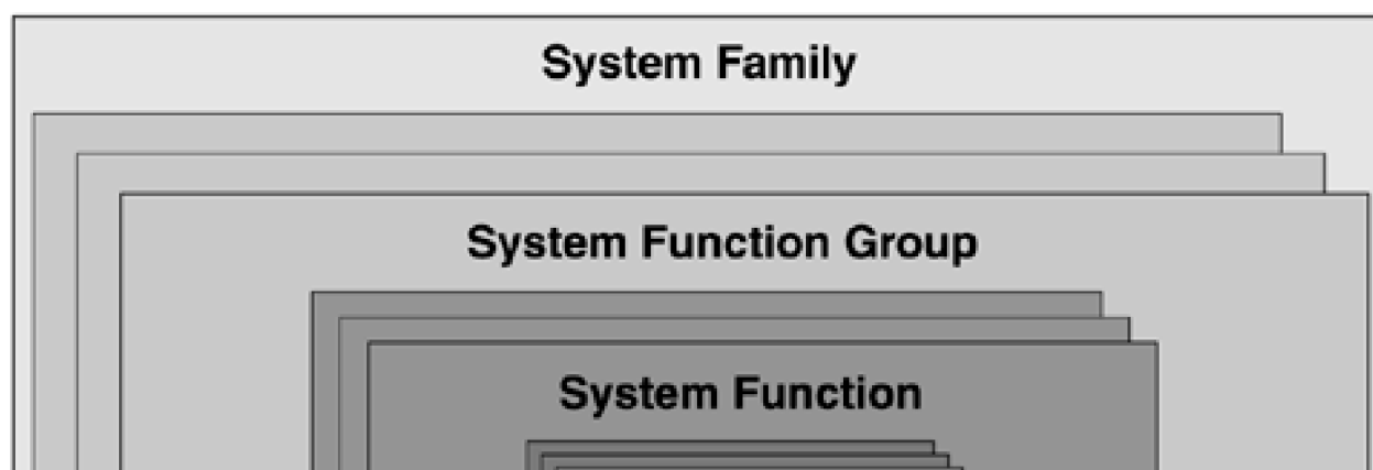
Figure 15.15. Units of software in the module decomposition view
