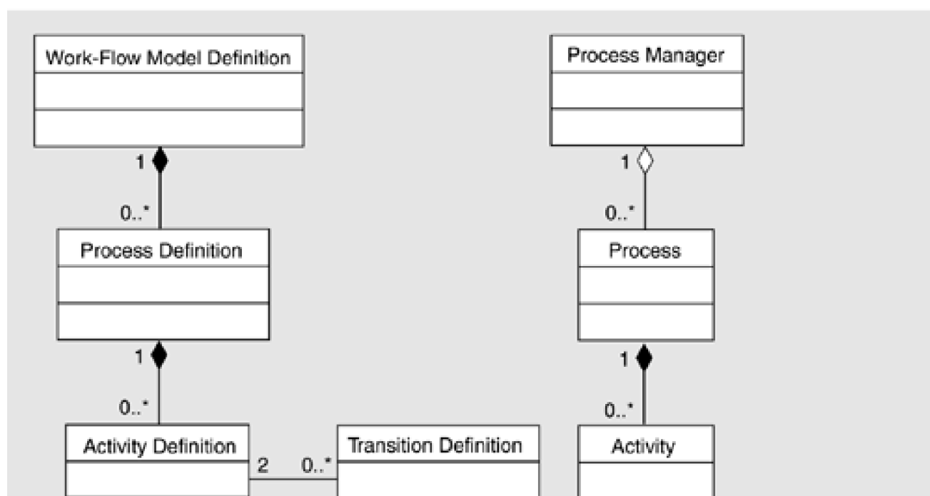
Figure 17.7. Class diagram for the work-flow component
