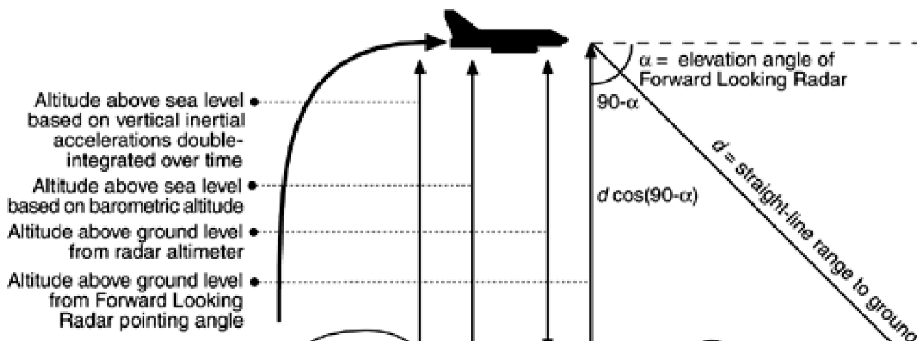
Figure 3.3. Calculation of altitude for the A-7E
