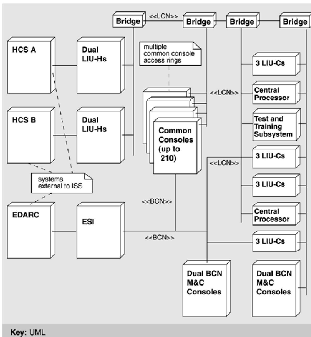
Figure 6.5. ISSS physical view
