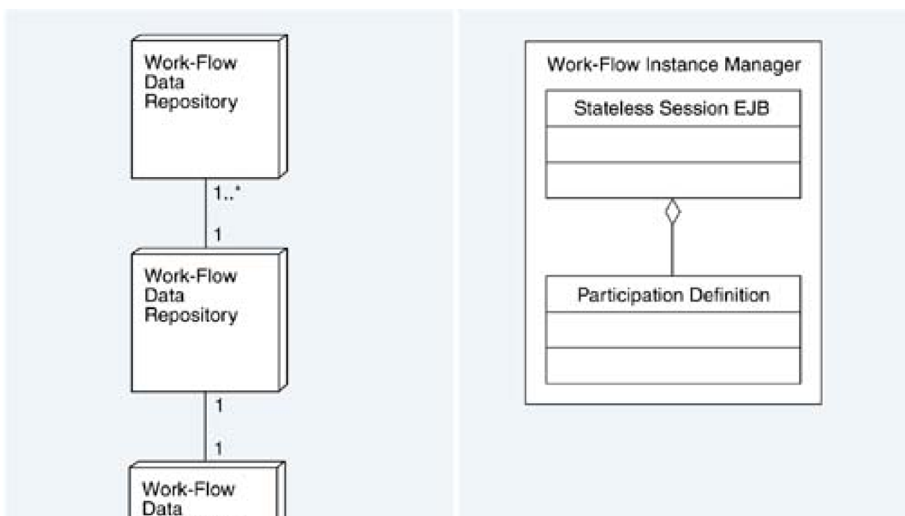
Figure 17.8. Work-flow component packaging diagram
