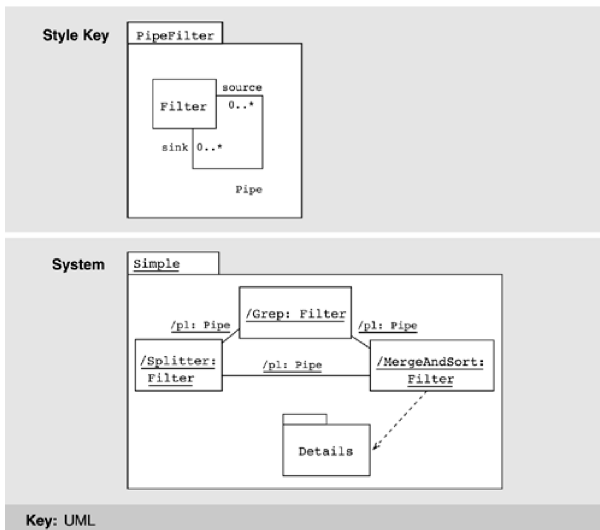
Figure 9.12. Systems as collaborations
