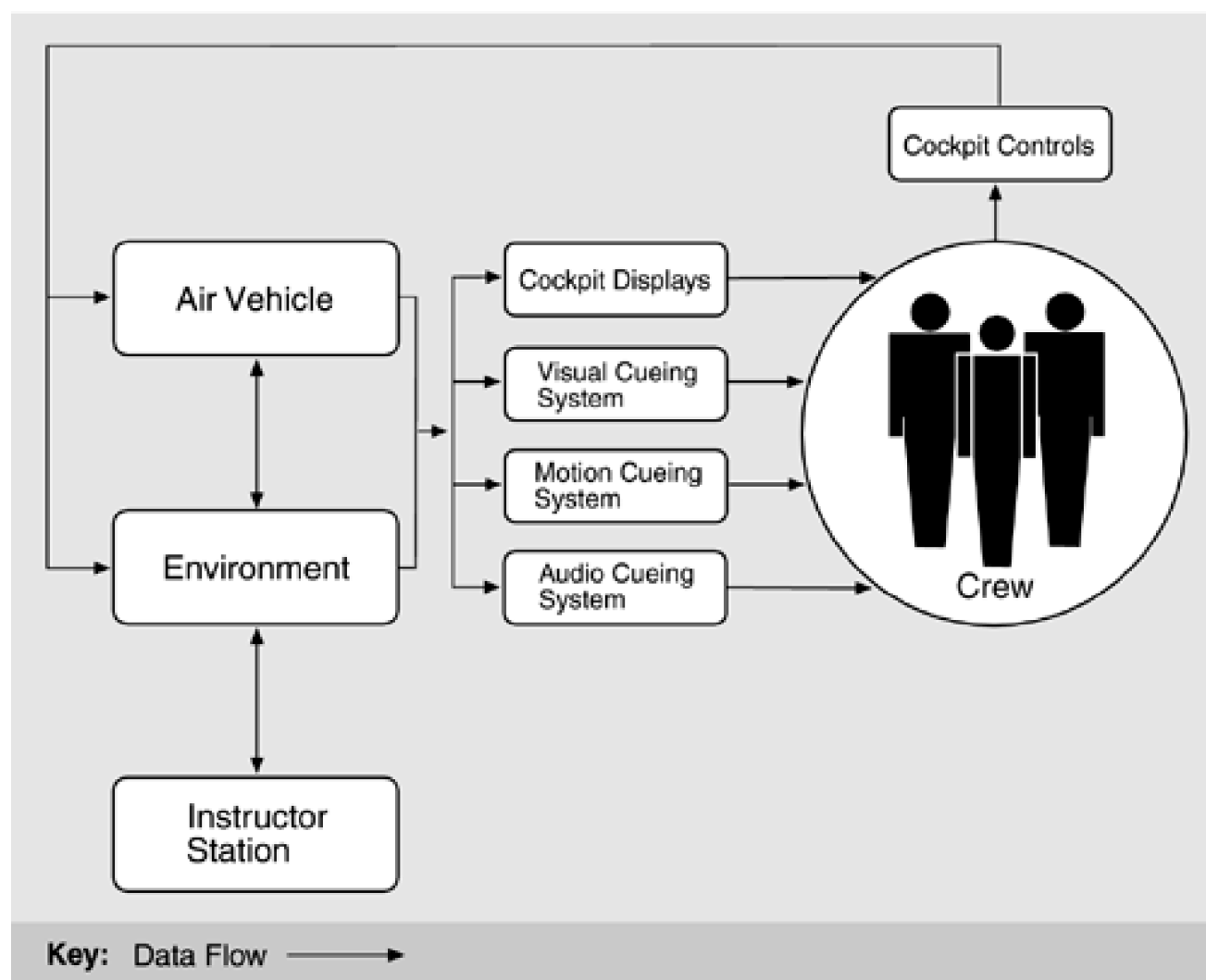
Figure 8.3. Reference model for flight simulator
