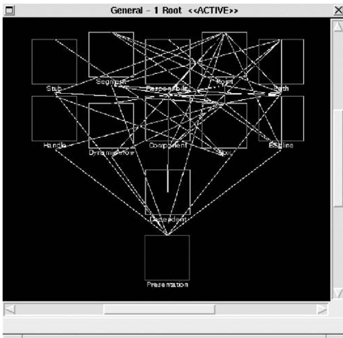
Figure 10.6. An architectural view represented in Dali
