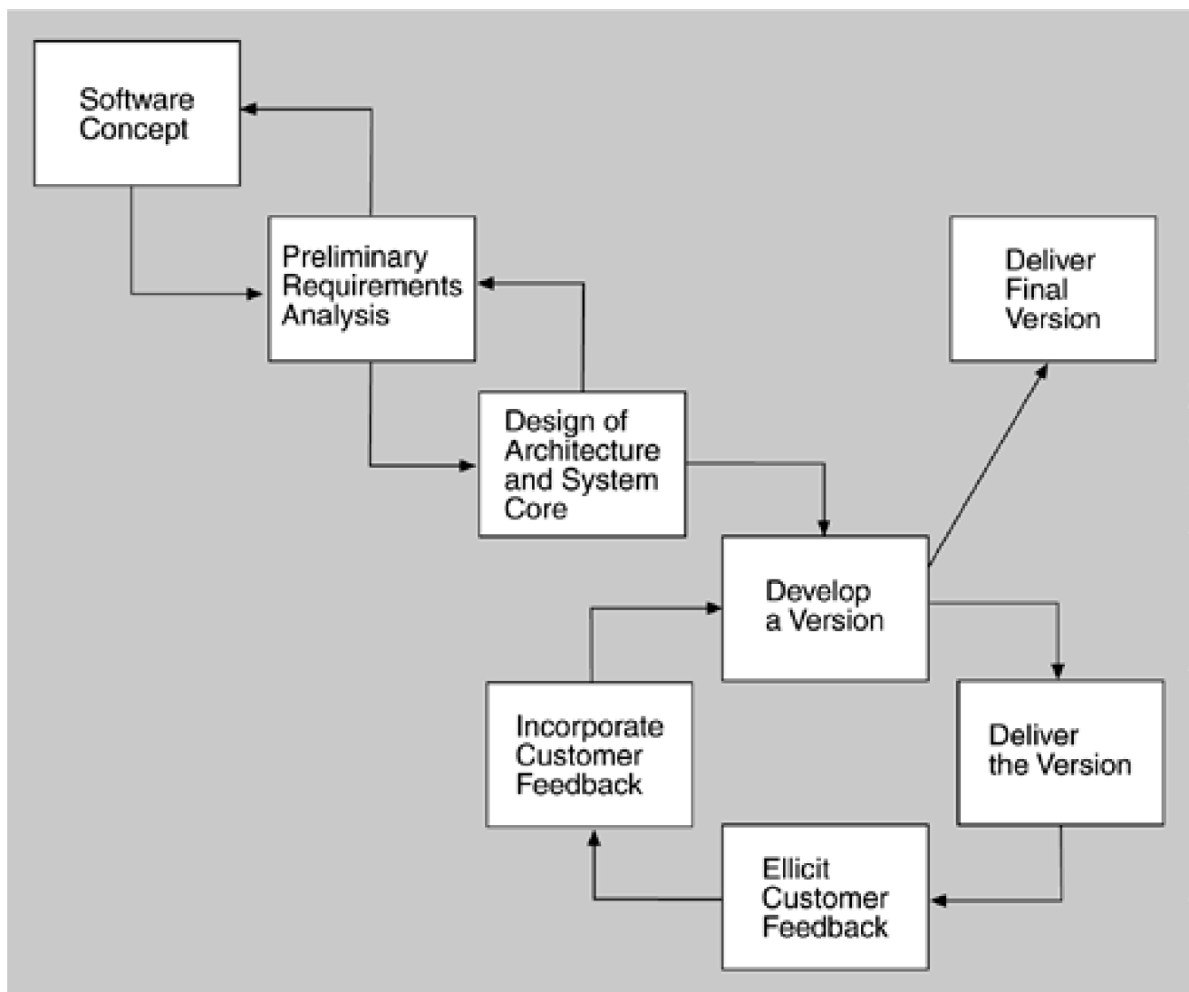
Figure 7.1. Evolutionary Delivery Life Cycle
