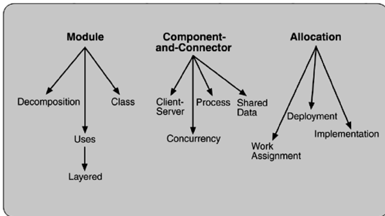
Figure 2-3. Common software architecture structures
