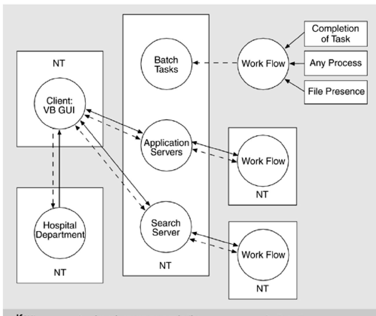
Figure 11.4. A view showing communication, data flow, and processors of the OLTM
