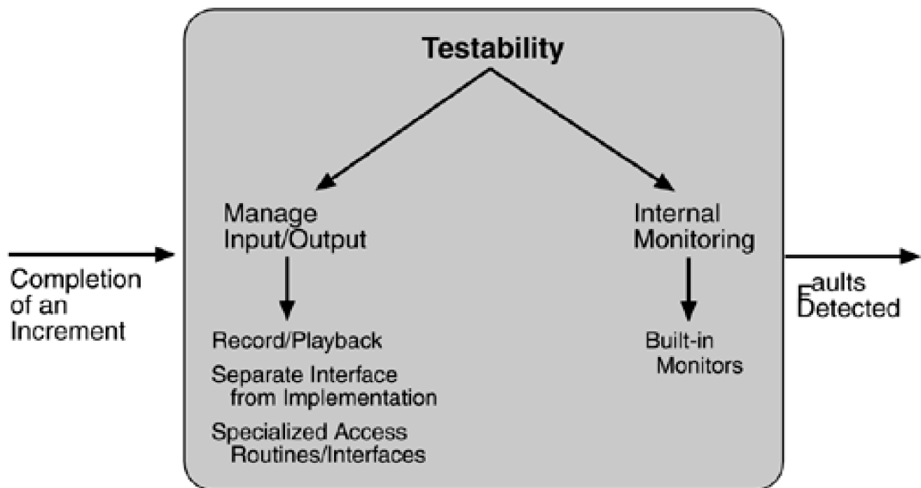
Figure 5.11. Summary of testability tactics
