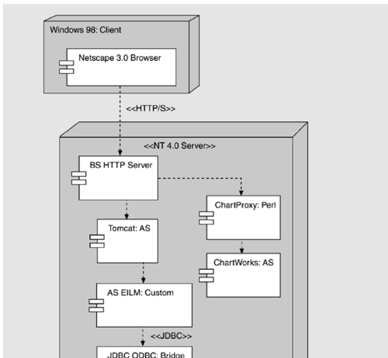
Figure 18.4. JavaServer Pages ensemble
