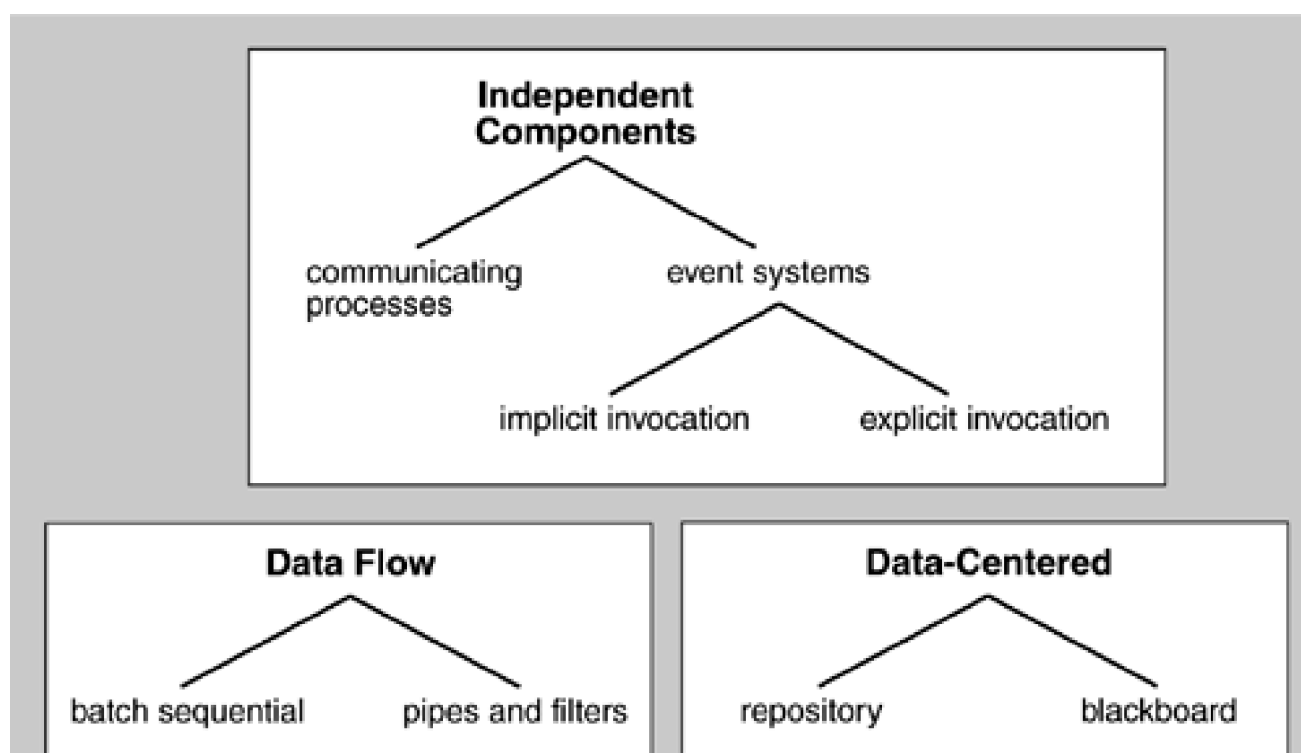
Figure 5.14. A small catalog of architectural patterns, organized by is-a relations
