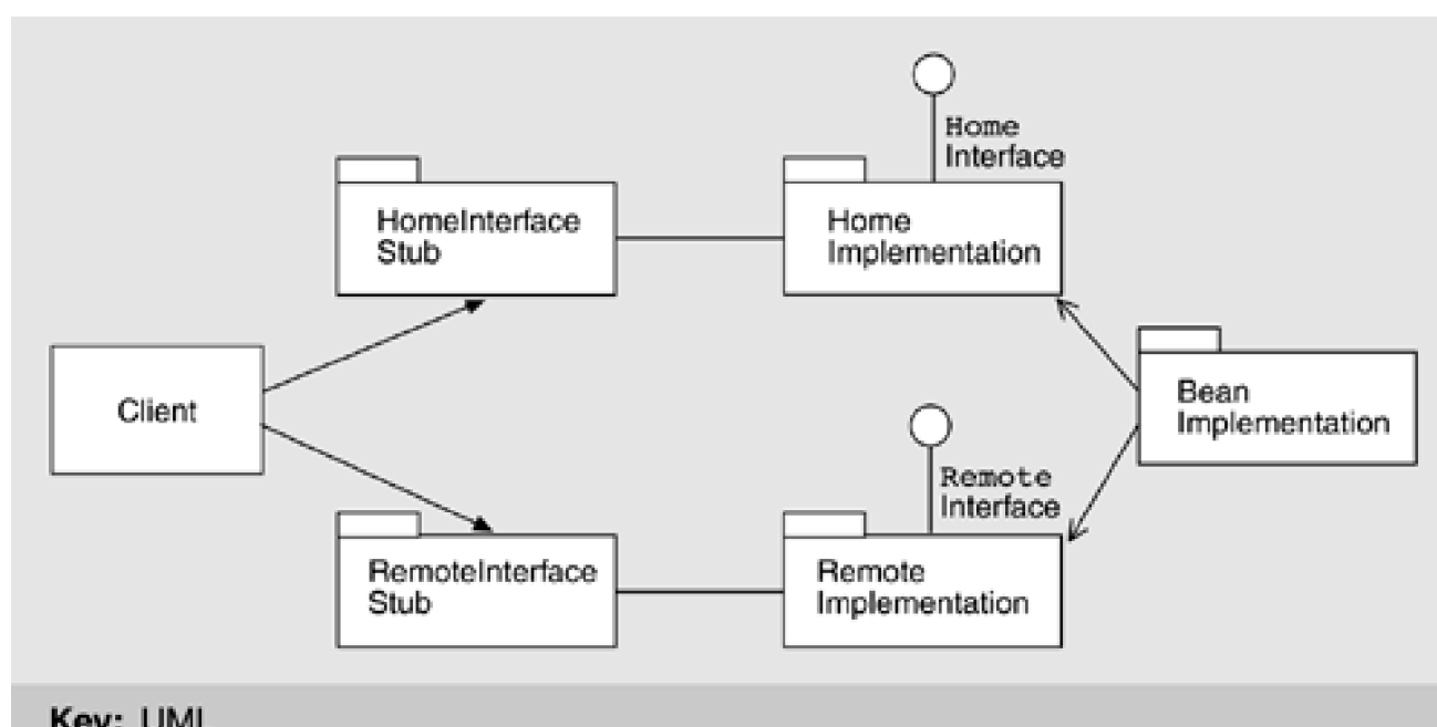
Figure 16.5. EJB package diagram
