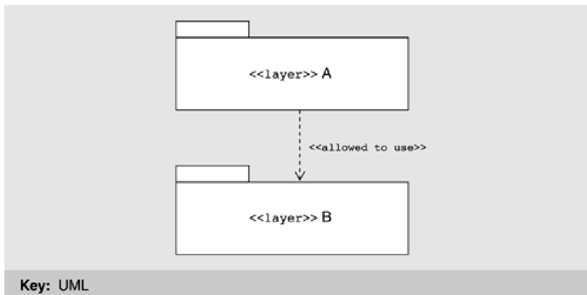
Figure 9.9. A simple representation of layers in UML
