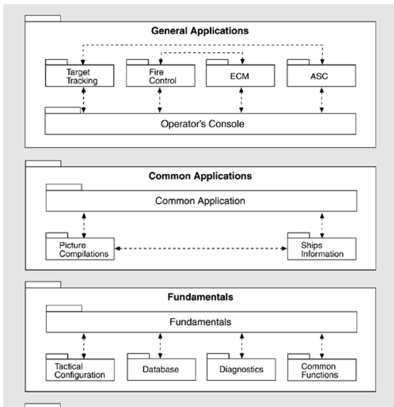
Figure 15.14. SS2000 layered software architecture
