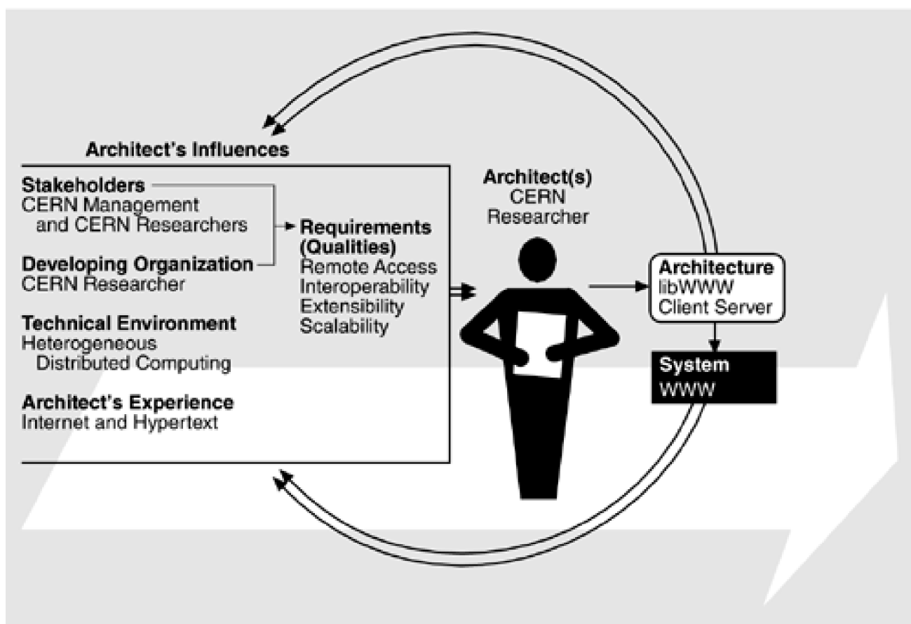
Figure 13.1. The original ABC for the Web
