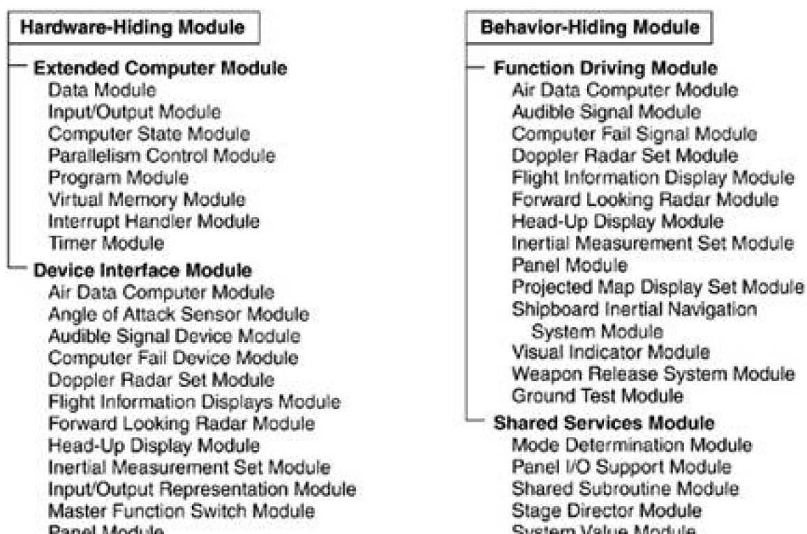
Figure 3.4. The module decomposition view of the A-7E software architecture
