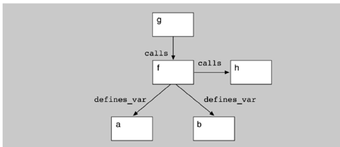
Figure 10.8. Graphical representation of elements and relationships
