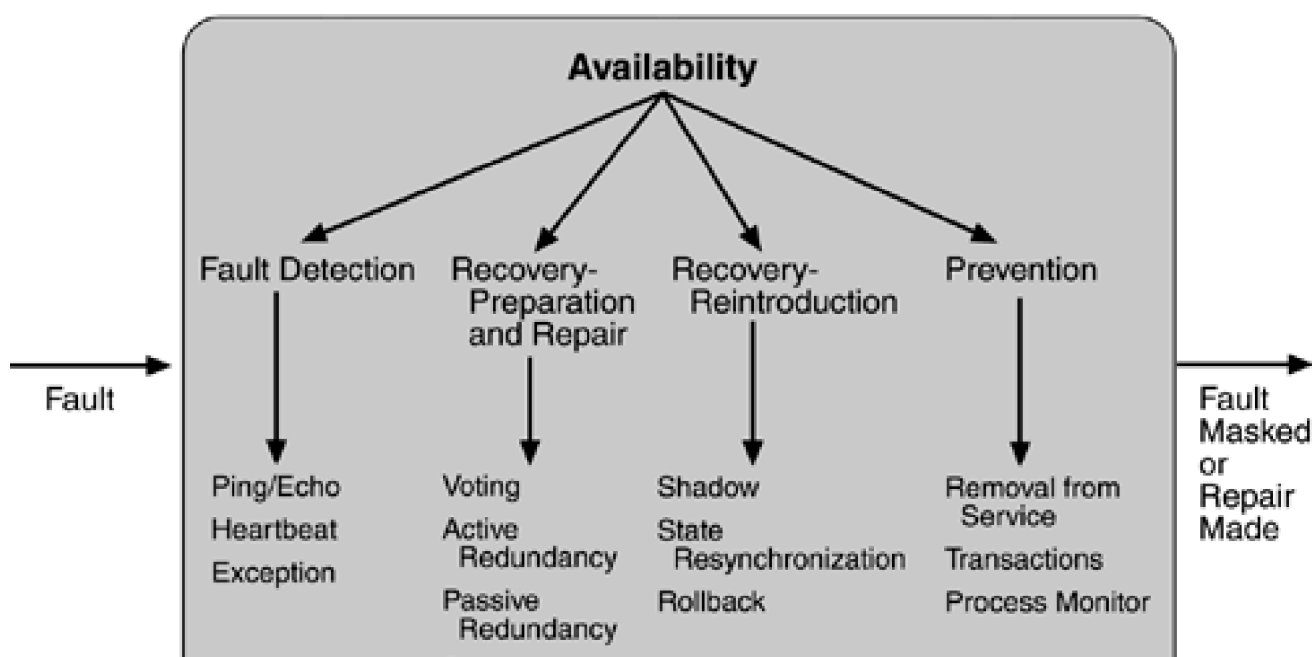
Figure 5.3. Summary of availability tactics
