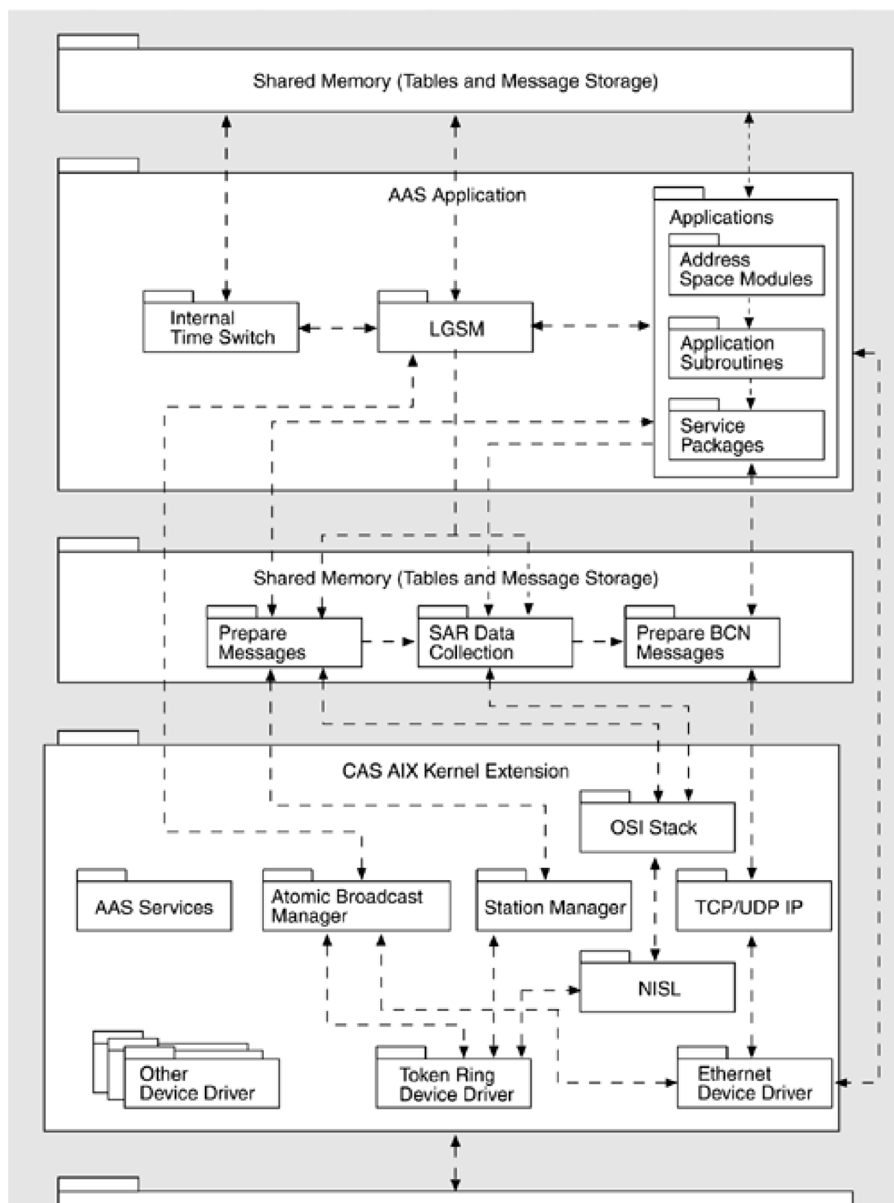
Figure 6.8. ISSS software architecture layers. The associations show data and/or control flow, making this an overlay of layers and a component-and-connector view.
