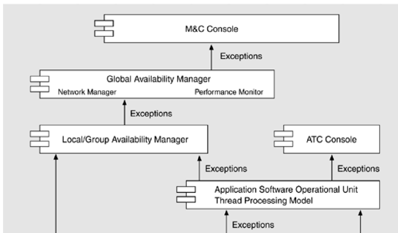
Figure 6.9. ISSS component-and-connector view for fault tolerance
