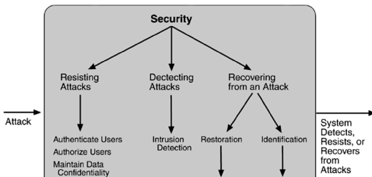
Figure 5.9. Summary of tactics for security
