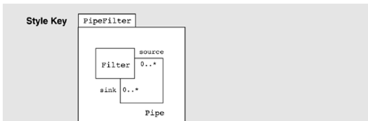
Figure 9.10. Types as classes, and instances as objects, exemplified with a simple pipe and filter
