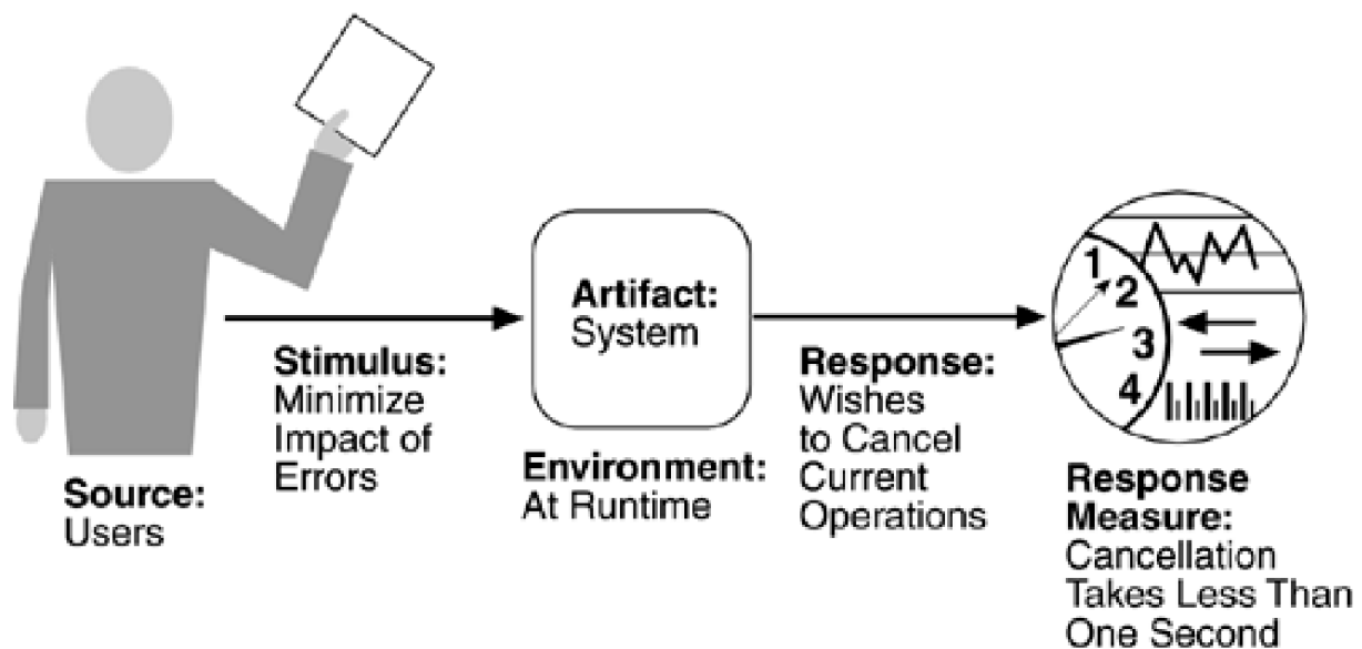
Figure 4.8. Sample usability scenario
