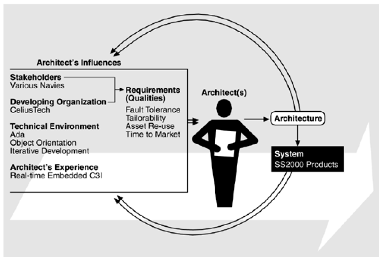
Figure 15.1. The ABC as applied to CelsiusTech
