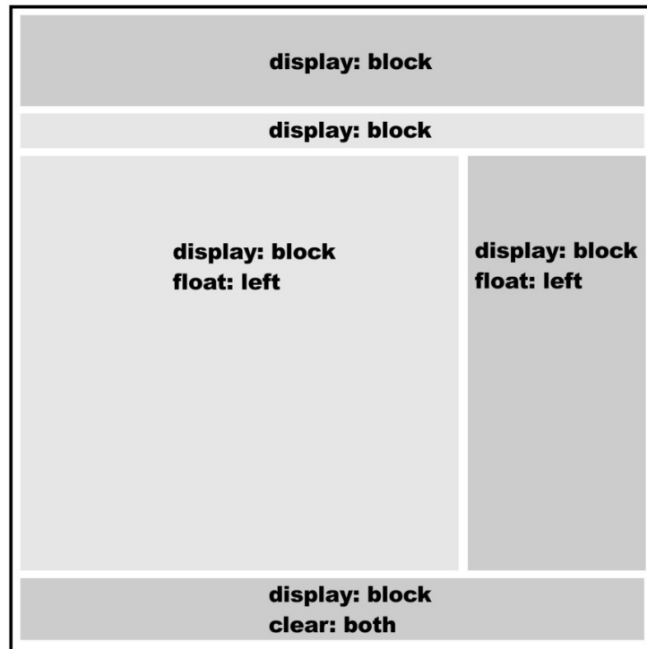
Figure 2-2: visual representation of the Traditional Box Model
