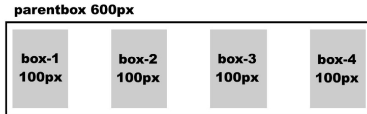
Figure 2-10: free space distributed with box-pack: justify;
