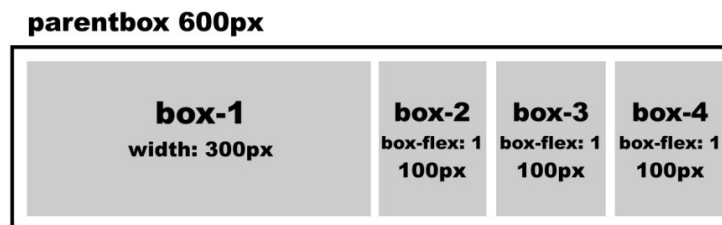
Figure 2-13: only the free space is distributed
