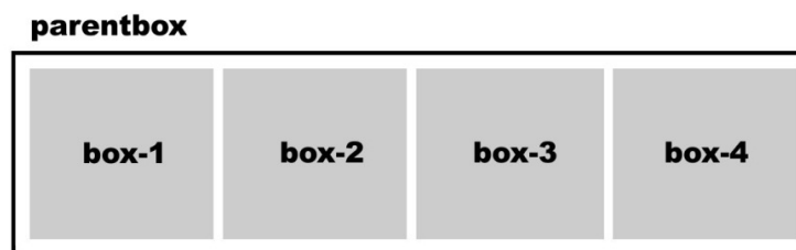
Figure 2-4: a parent box with four children
