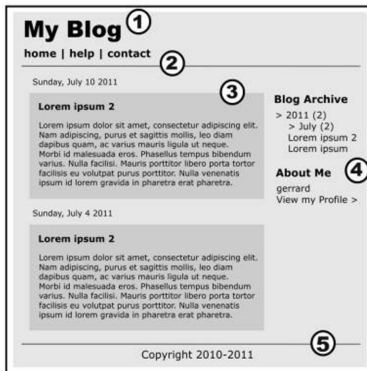
Figure 1-2: visual representation of a typical blog layout
