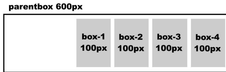
Figure 2-9: free space distributed with box-pack: end;
