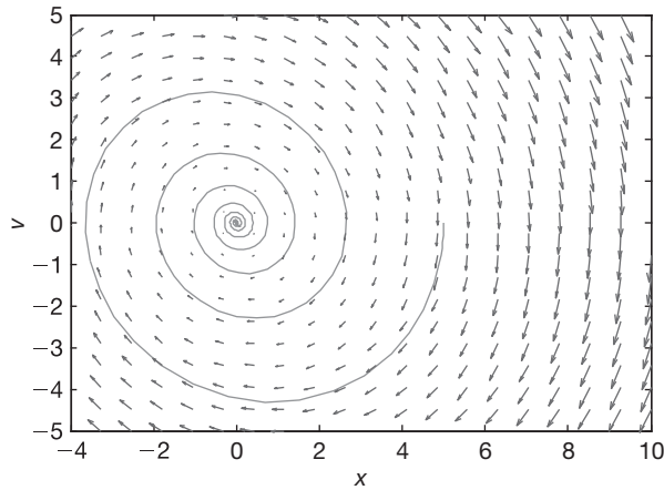
FIGURE 14.15 Slope field for the ODE in equation (14.26) when the square-wave driver is off ( s(t) = 0 ) and the system is relaxing to x = 0 , v = 0 . The vector field is created by the MATLAB quiver command.
