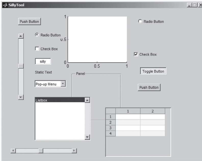
FIGURE 9.5 SillyTool running.
