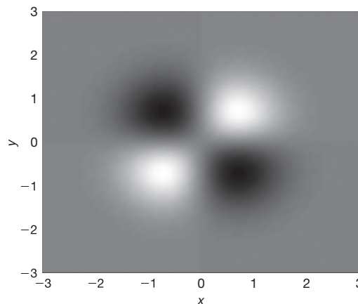
FIGURE 13.7 Four ways to visualize a function of two variables z = f(x, y) .
