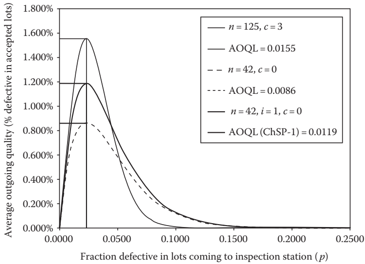
FIGURE 17.14: AOQL curves for the n = 42, c = 0 plan; n = 125, c = 3 plan; and n = 42, i = 1, c = 0 plan.
