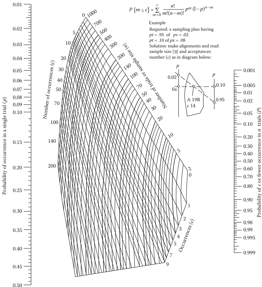
FIGURE 3.5: Larson binomial nomograph. If p is less than .01, set kp on the p -scale and n/k on the n -scale, where k=0.01/9 , rounded upward conveniently. (From Larson, H.R., Ind. Qual. Control , 23(6), 273, 1966. With permission.)
