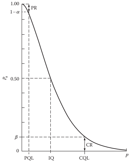
FIGURE 4.6: PQL, CQL, PR, CR ( n = 20 , c = 1 ).
