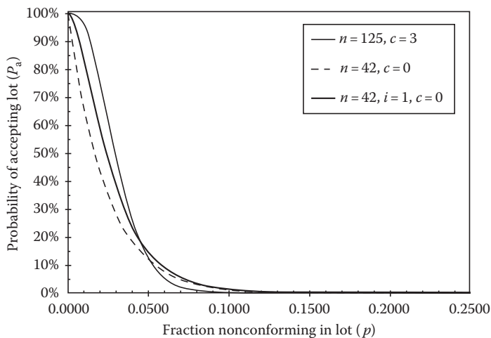
FIGURE 17.13: OC curves for the n = 42 , c = 0 plan; n = 125 , c = 3 plan; and n = 42 , i = 1 , c = 0 plan.
