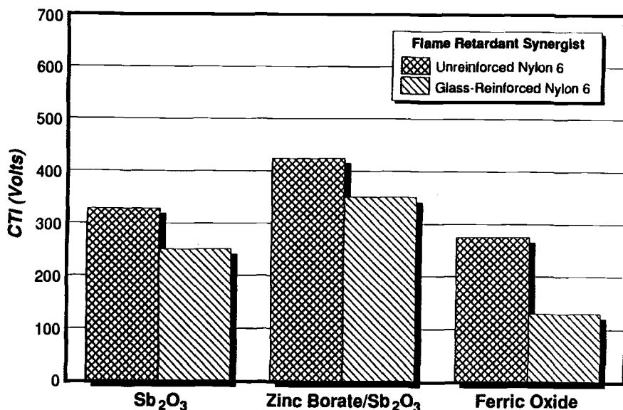
FIG. 5—CTI for FR-Nylon 6, unreinforced vs. glass reinforced.
