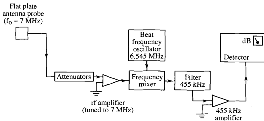
Figure 9 – Schematic circuit diagram of an antenna probe type PD detector for discharge site location in polymeric cables [39]
