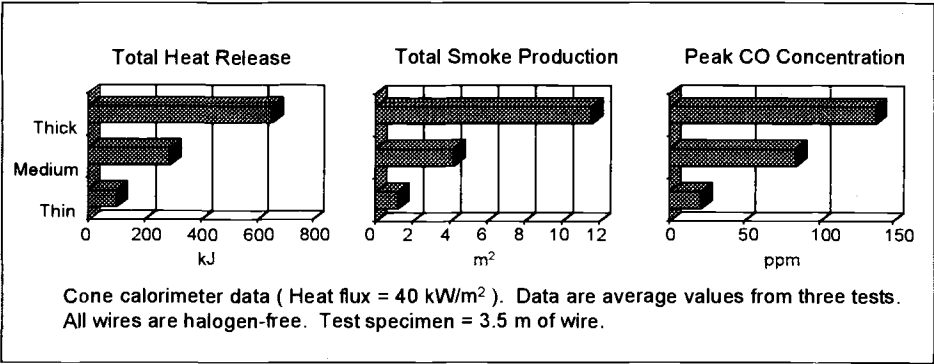
Figure 1 - Cone Calorimeter Data
