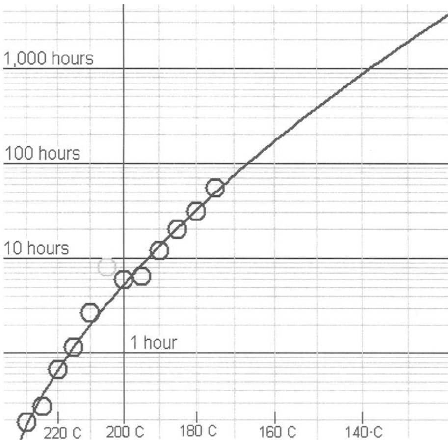
Figure 4 – Asymptotic Kinetic Curve Fit to OMT Data
