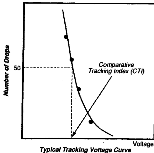
FIG. 2—Tracking resistance.
