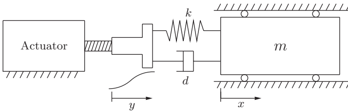
Fig. 7.1. Linear model with one degree of freedom.
