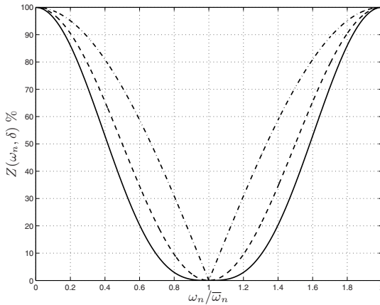
Fig. 7.46. Sensitivity curves of ZV (dashdot) ZVD (dashed) and ZVDD (solid) shapers, obtained for \delta = 0 .
