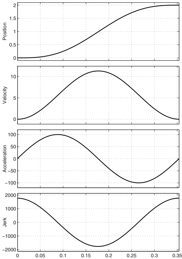
Fig. 3.51. Minimum-time cycloidal trajectory without constant velocity segment.
