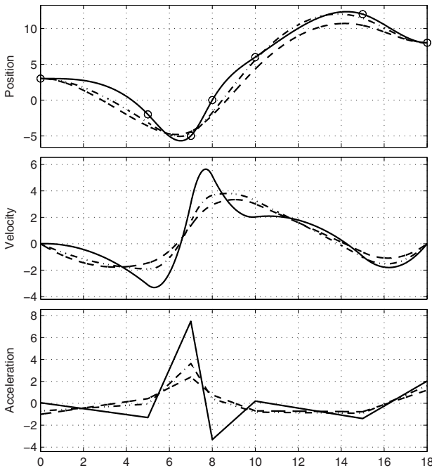
Fig. 4.11. Smoothing splines for different values of \mu and w_k .
