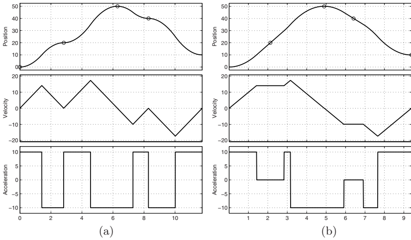
Fig. 3.5. Position, velocity and acceleration of a trapezoidal trajectory through a sequence of points with null (a) and non-null (b) intermediate velocities.
