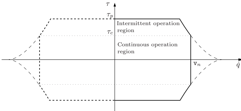
Fig. 6.1. Generic speed-torque diagram for an electric motor.
