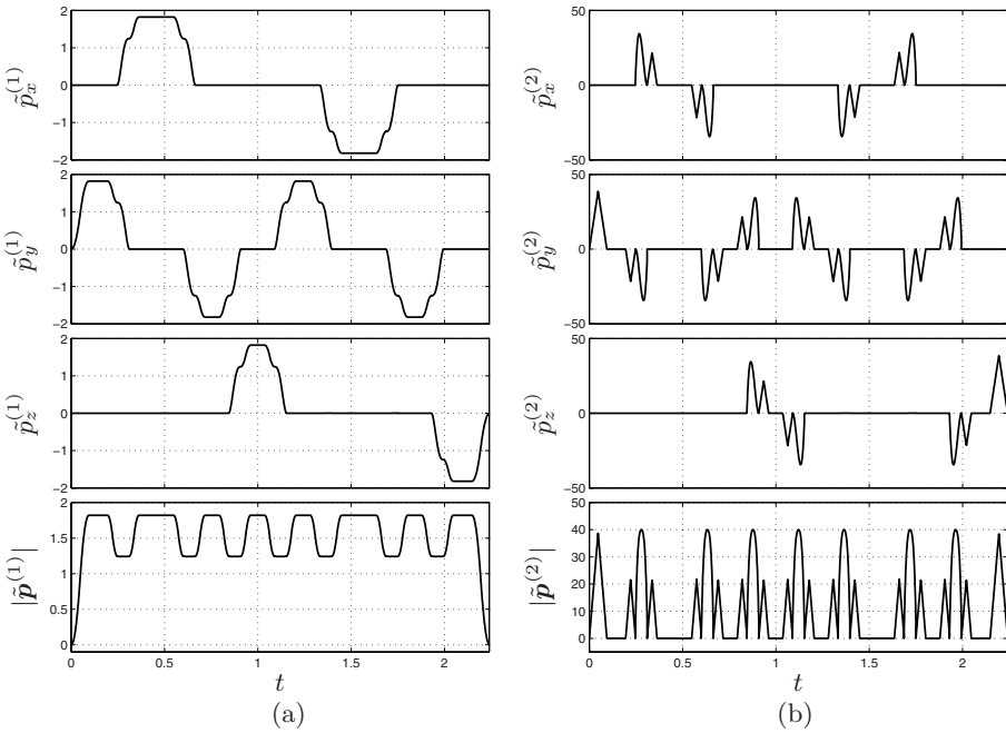
Fig. 9.22. Velocity and acceleration (components and magnitude) of a trajectory composed by linear and 5-th degree Bézier segments, with a motion law optimized in each tract.
