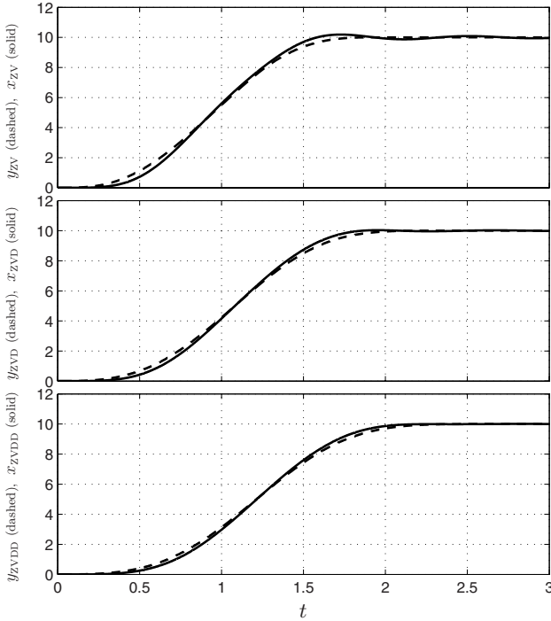
Fig. 7.51. Output x(t) of the system (7.22) (solid) with the parameters values m = 1 \text{ kg} , d = 2 \text{ Ns/m} , k = 64 \text{ N/m} when the input trajectory q(t) is modified with a ZV, a ZVD or a ZVDD shaper.
