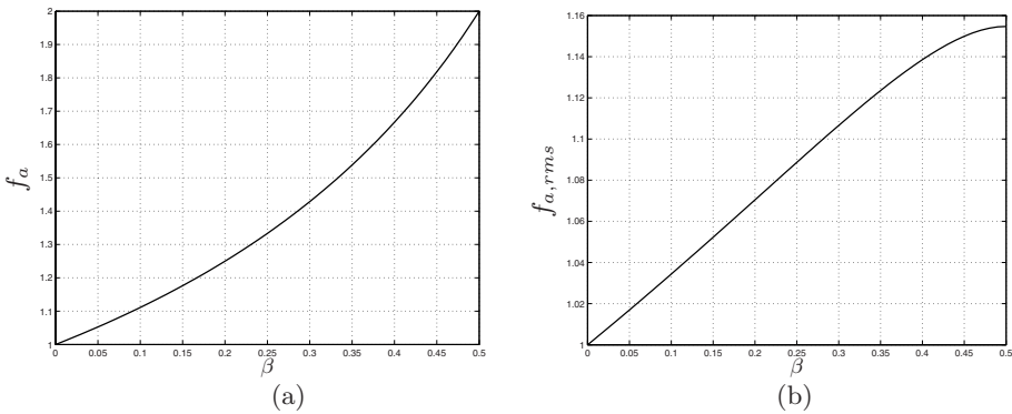
Fig. 6.14. Functions of \beta relating the coefficients C_a (a) and C_{a,rms} (b) of the trapezoidal and double S trajectories.
