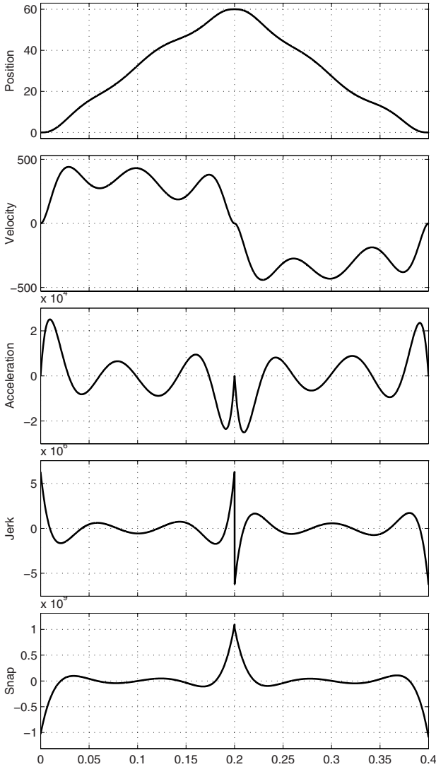
Fig. 7.41. Position, velocity, acceleration, jerk and snap for the Peisekah polydyne trajectory ( T_r = T_d = 0.2 ).
