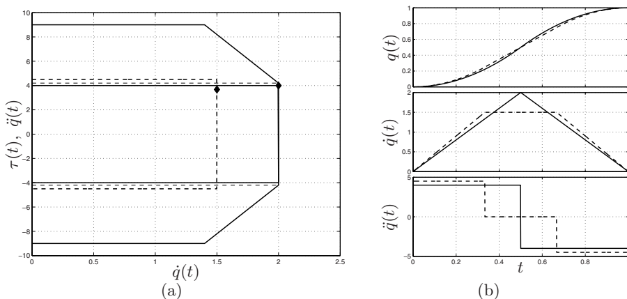
Fig. 6.11. Tasks obtained with a trapezoidal trajectory for different values of \alpha (a) and plots of position, velocity, acceleration (b).
