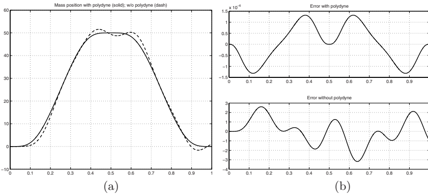
Fig. 7.39. Position of the mass of Fig. 7.34 (a) and tracking errors due to the elasticity (b) with and without using the polydyne; note the different amplitudes of the diagrams in (b).
