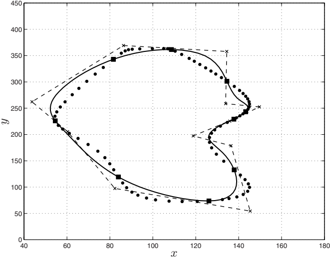
Fig. 8.22. Global interpolation/approximation by means of a B-spline defined by 12 control points (x-marks).
