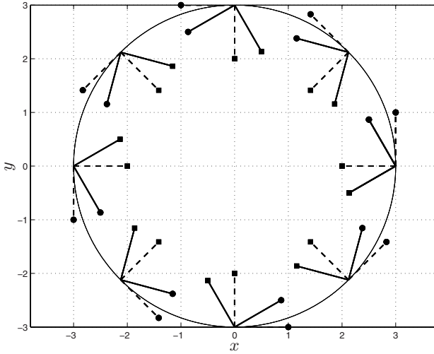
Fig. 8.14. A circular trajectory with the associated Frenet frames (dashed) and the desired tool frames (solid).
