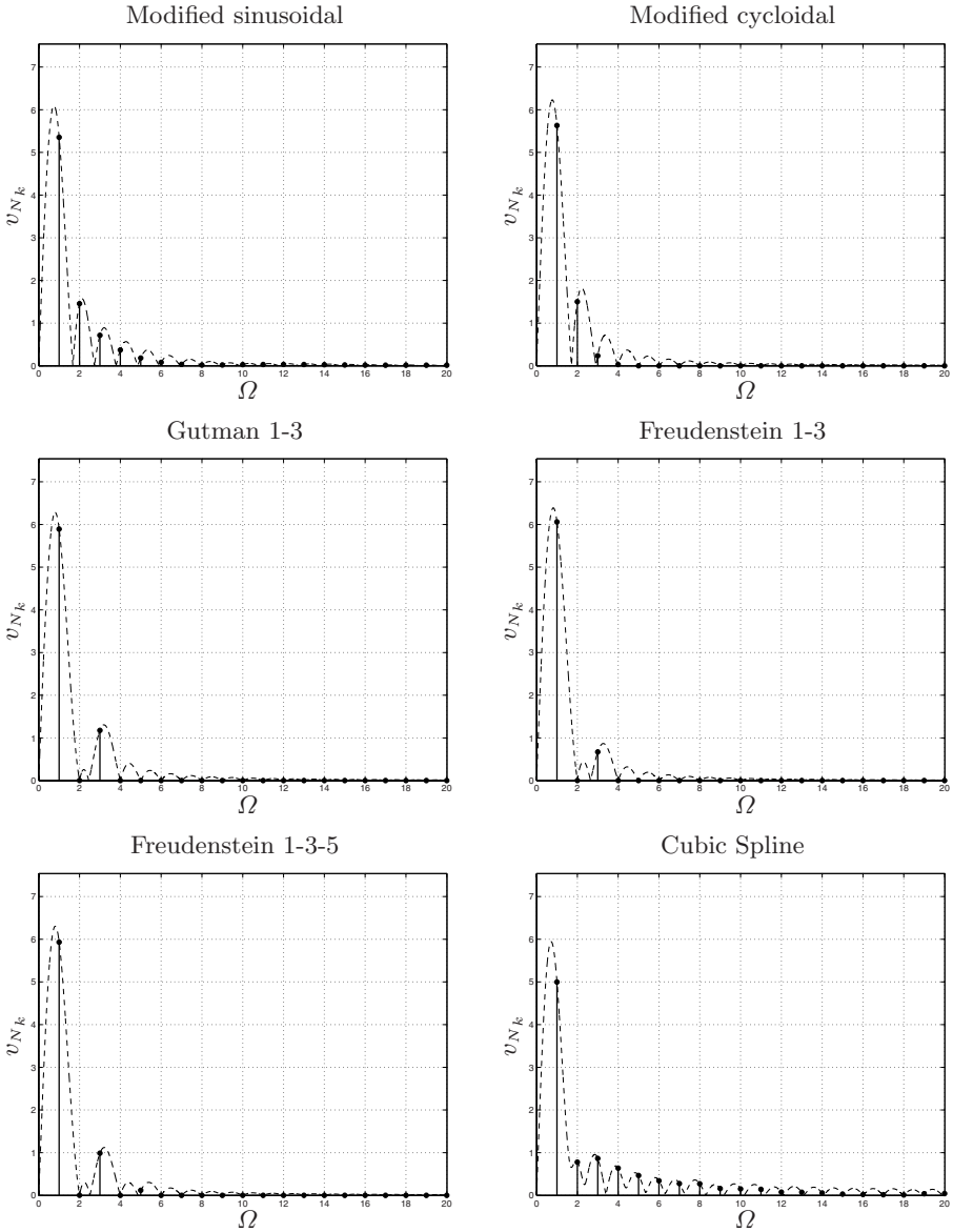
Fig. 7.31. Frequency analysis of the acceleration profiles of the periodic repetition of trajectories: modified sinusoidal, modified cycloidal, Gutman 1-3, Freudenstein 1-3 and 1-3-5, cubic spline.
