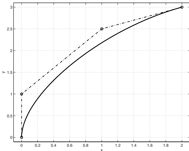
Fig. B.10. 3 – rd degree Bézier curve, in the 2-dimensional space.
