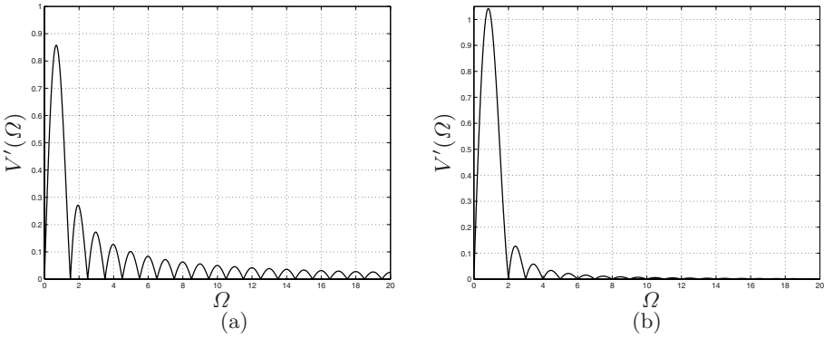
Fig. 7.25. Magnitude spectra of the harmonic (a) and cycloidal (b) trajectories.
