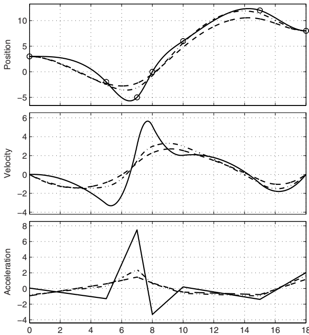
Fig. 4.10. Smoothing splines computed for different values of \mu (0.3, 0.6, 1).
