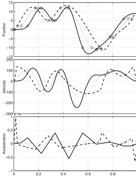
Fig. 4.15. Spline trajectories interpolating a set of data points, with different distributions of time instants: uniformly spaced (solid), cord length (dashed), centripetal (dotted).
