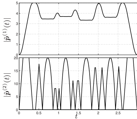
Fig. 9.4. Magnitude of velocity and acceleration of the trajectory composed by straight line segments and 5-th degree Bézier curves.
