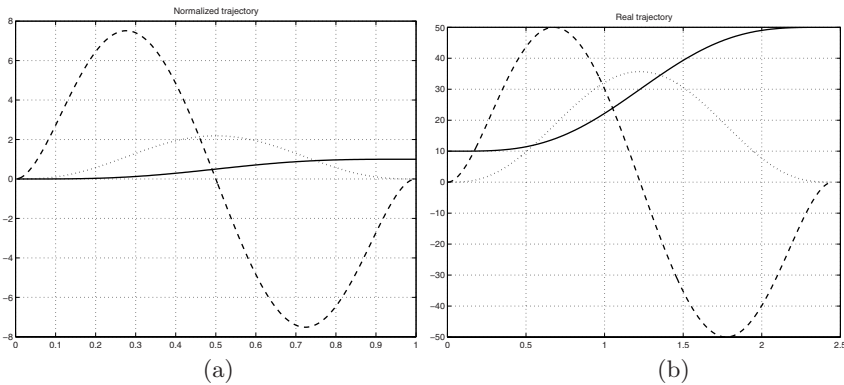
Fig. 5.9. Profiles of acceleration (dashed), velocity (dotted) and position (solid) of a polynomial of degree 7: normalized form (a) and with boundary conditions q_0 = 10 , q_1 = 50 , t_0 = 0 , t_1 = 2.4516 (b).
