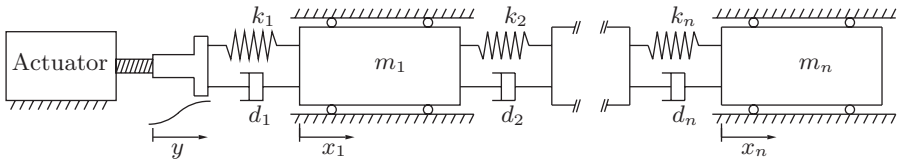
Fig. 7.2. Linear model with n degrees of freedom.
