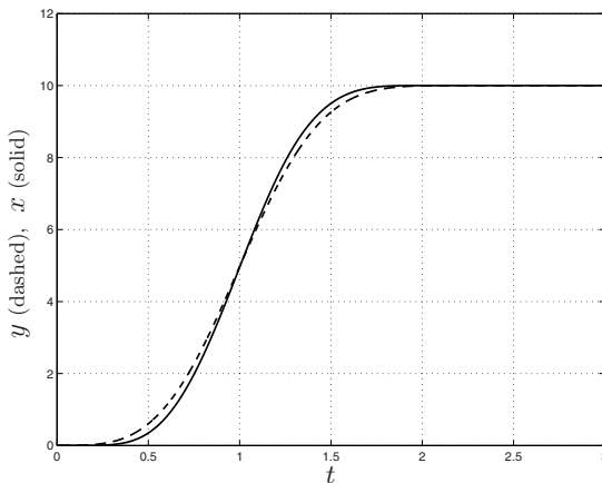
Fig. 7.58. Response of the system G(s) = \frac{800}{(s^2 + 2s + 100)(s^2 + 400)} to a double S trajectory filtered by a cascade of two ZVDD shapers.
