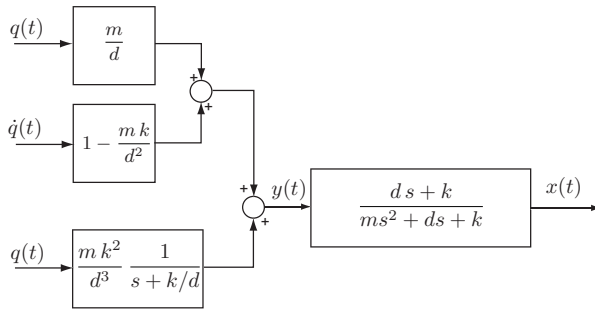
Fig. 7.63. Feedforward action for the tracking of the desired motion profile q(t) , with the mechanical system in Fig. 7.1.
