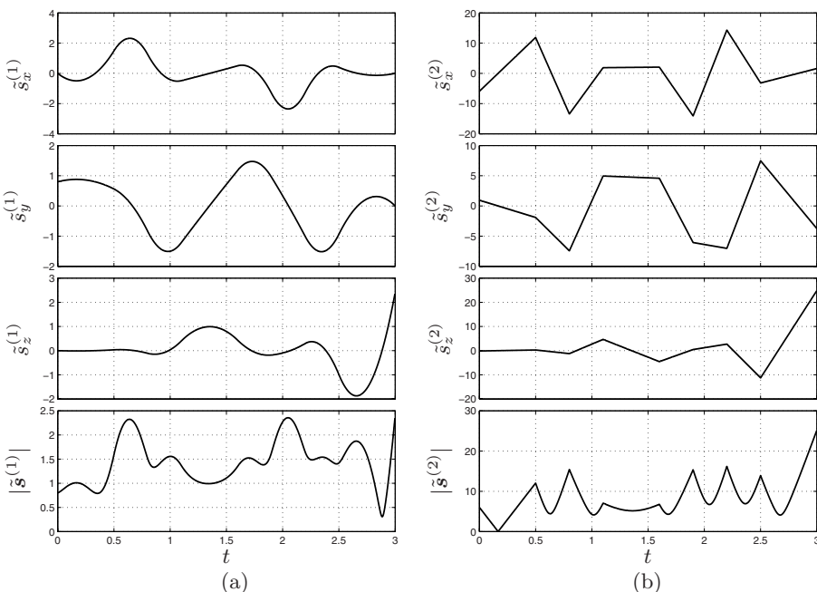
Fig. 9.26. Velocity and acceleration (components and magnitude) of a the position trajectory represented by a B-spline curve, with the parameterization u(t) = t .
