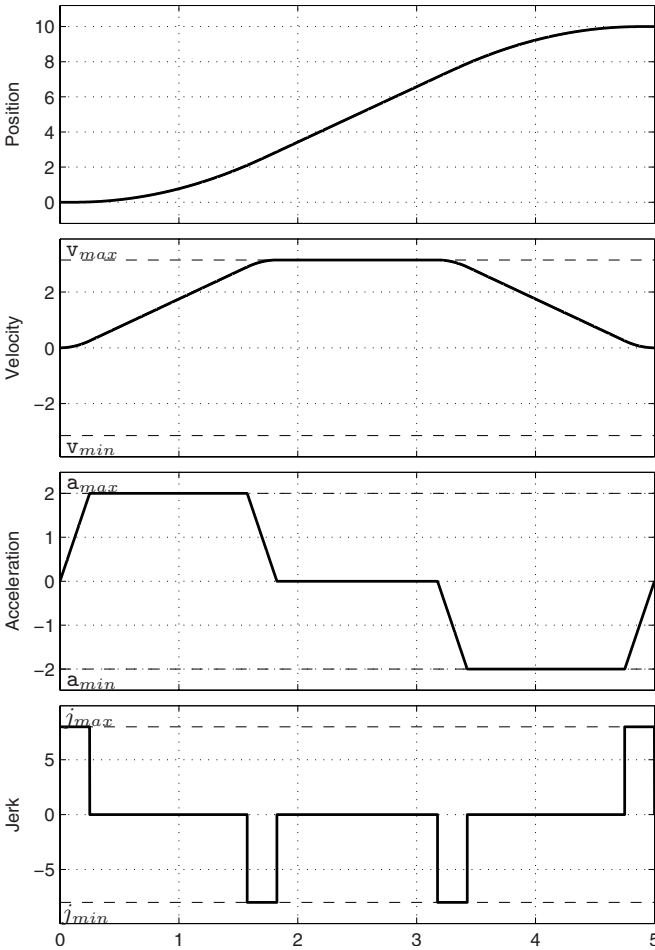
Fig. 3.29. Double S trajectory profiles with prescribed duration T , and with conditions on a_{max} and j_{max} .
