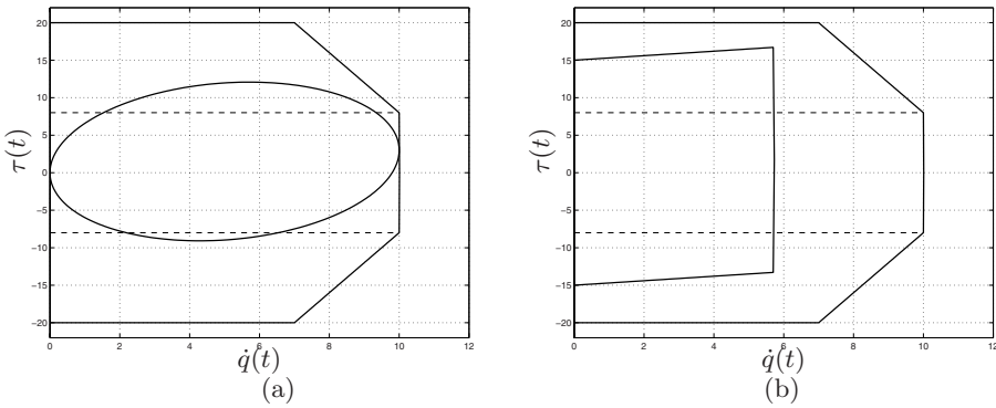
Fig. 6.2. Mechanical tasks obtained with two different motion laws: a cycloidal trajectory (a) and a trapezoidal velocity trajectory (b).
