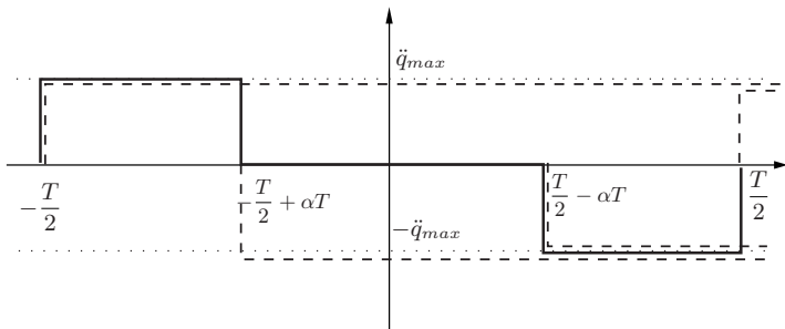
Fig. 7.20. Decomposition of the acceleration profile of the trapezoidal trajectory into elementary functions (step functions).
