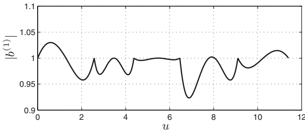
Fig. 8.38. Magnitude of the speed of a trajectory composed by 3-rd degree Bézier curves properly reparameterized.
