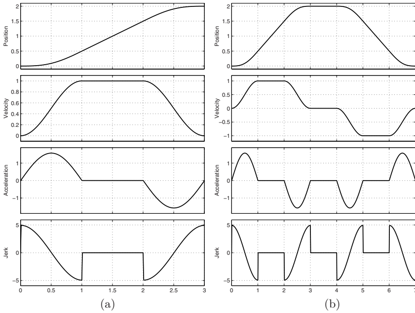
Fig. 3.47. Position, velocity, acceleration and jerk of Example 3.24.b (a), and Example 3.24.c (b).
