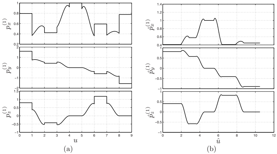
Fig. 8.44. Components of the tangent vectors \mathbf{p}^{(1)}(u) and \hat{\mathbf{p}}^{(1)}(\hat{u}) of the trajectory composed by linear and 4-th degree Bézier segments, without (a) and with (b) “scaling in time”.
