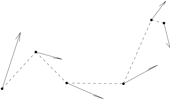
Fig. 8.34. Computation of the tangent vectors for local interpolation.
