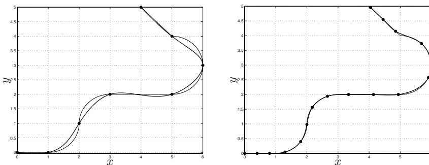
Fig. 8.19. B-spline approximation of motion primitives.
