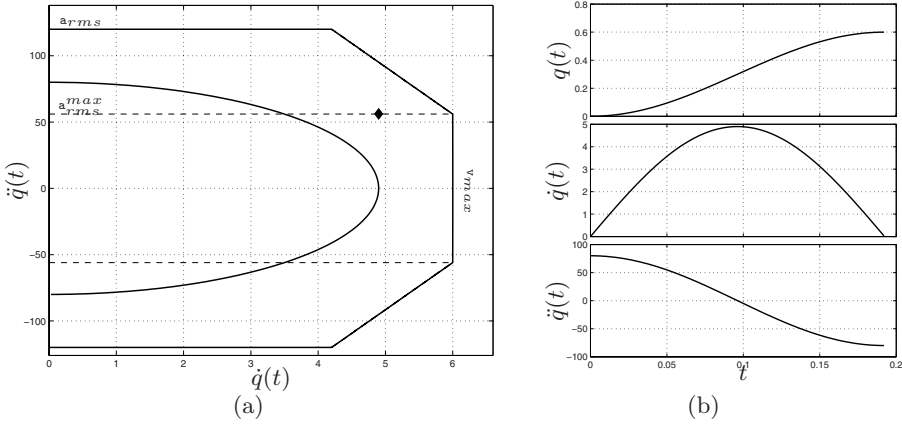
Fig. 6.8. Task obtained with a harmonic trajectory represented in a speed-acceleration diagram (a) and single plots of position, velocity, acceleration (b).
