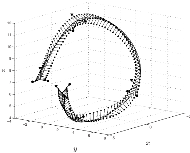
Fig. 8.7. Multipoint trajectory for position and orientation based on Roll-Pitch-Yaw angles representation.
