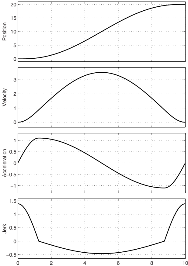
Fig. 3.38. Profiles of position, velocity, acceleration and jerk of a modified sinusoidal trajectory when h = 20 , T = 10 .
