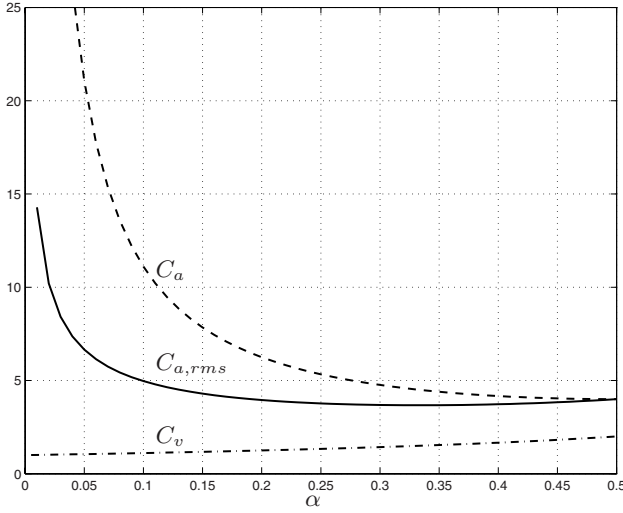
Fig. 6.10. Coefficients C_v , C_a and C_{a,rms} of the trapezoidal trajectory as a function of the parameter \alpha ( T_a = \alpha T ).
