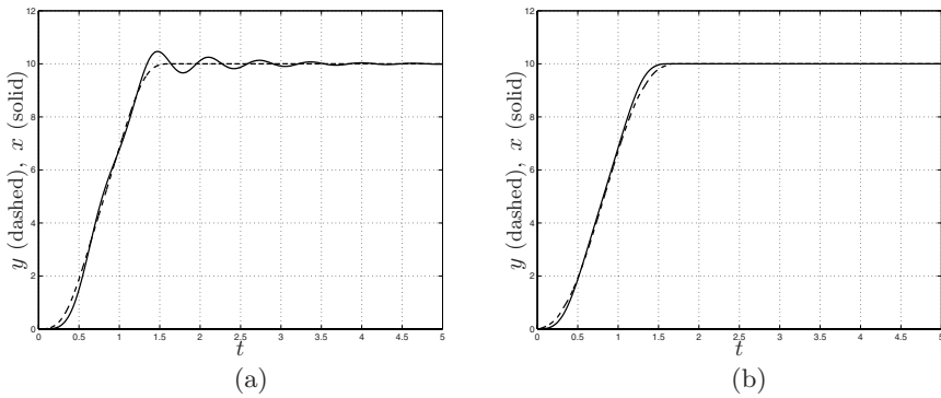
Fig. 7.64. Input and output signals of the system G(s) = \frac{2s+100}{s^2+2s+100} without (a) and with (b) model inversion.
