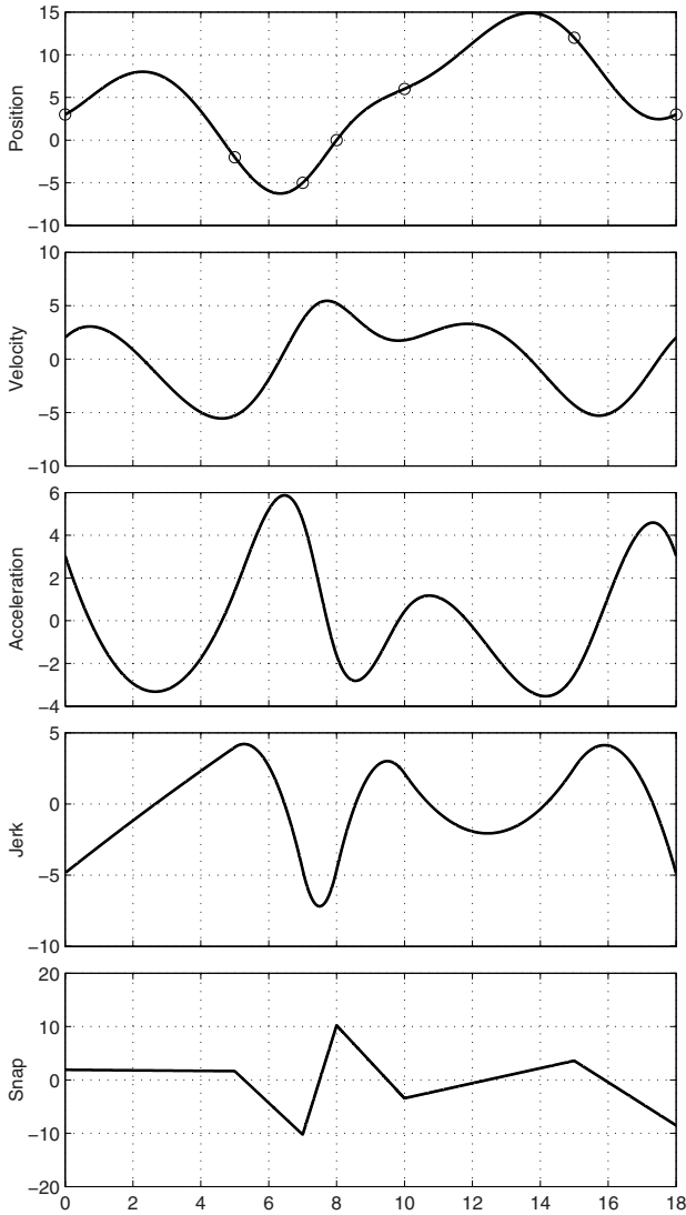
Fig. 4.21. B-spline trajectory of degree 4 with cyclic conditions.
