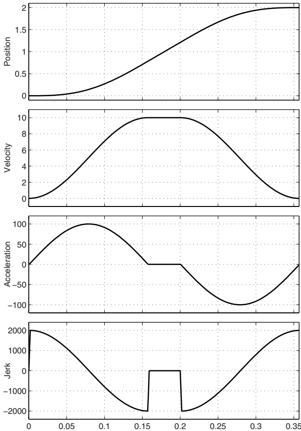
Fig. 3.50. Minimum-time trajectory composed by trigonometric and polynomial segments.
