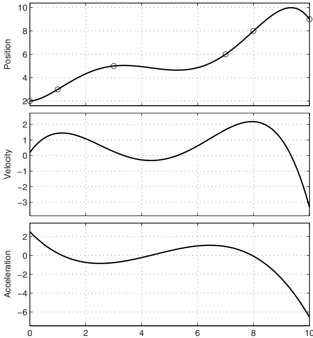
Fig. 4.2. Position, velocity and acceleration of an orthogonal polynomials trajectory ( m = 4 ) with the crossing condition for the initial and final points.
