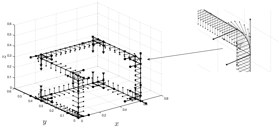
Fig. 9.17. Changes in the orientation superimposed to the position trajectory composed by linear and 5-th degree Bézier segments, with a particular of a Bézier blend.
