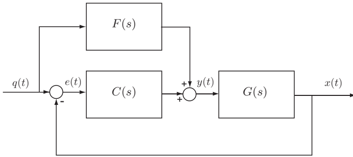
Fig. 7.60. Feedback/feedforward control of a SISO linear system.
