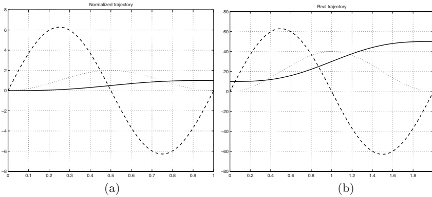
Fig. 5.10. Profiles of acceleration (dashed), velocity (dotted) and position (solid) of a cycloidal motion: normalized form (a) and with boundary conditions q_0 = 10 , q_1 = 50 , t_0 = 0 , t_1 = 2 , (b).
