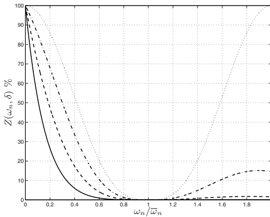
Fig. 7.47. Sensitivity curves of a ZVDD shaper for different value of \delta : \delta = 0 (dot), \delta = 0.2 (dashdot), \delta = 0.4 (dashed), \delta = 0.6 (solid).
