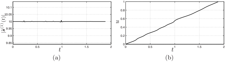
Fig. 9.9. Feed rate of the trajectory defined with a cubic B-spline, with u computed by means of (9.9b) (a), and relation between t and u (b).
