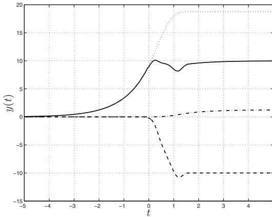
Fig. 7.65. Feedforward signal based on model inversion (solid), decomposed in its components: pre-action (dotted), post-action (dashdot), linear combination of q and \dot{q} (dashed).
