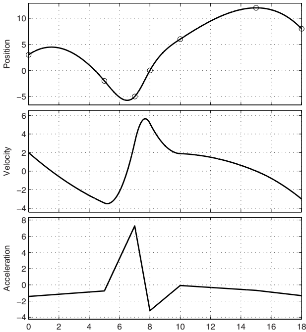
Fig. 4.7. Spline trajectory with constraints on initial and final velocities.
