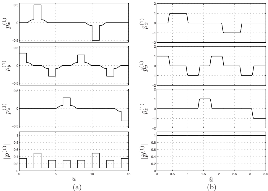
Fig. 9.16. First derivative (components and magnitude) of a trajectory composed by linear and 5-th degree Bézier segments, before (a) and after (b) the reparameterization.
