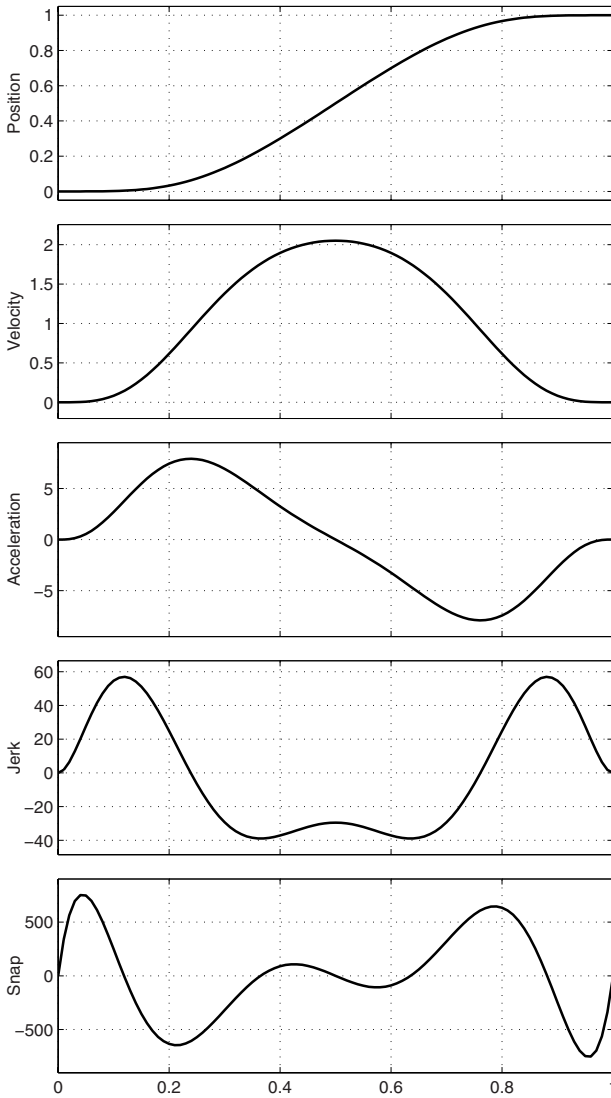
Fig. 7.36. Position, velocity, acceleration, jerk and snap for the Peisekah polynomial function.
