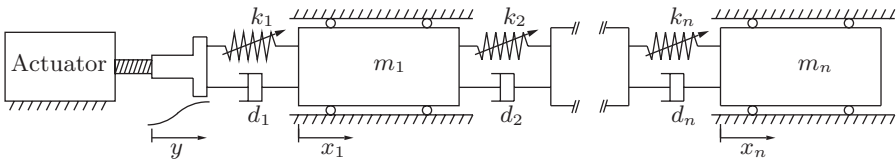
Fig. 7.5. Model with n degrees of freedom with passive nonlinear parameters.
