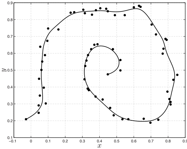
Fig. 9.30. Smoothing B-spline approximating a set of data points, for \lambda = 10^{-6} .
