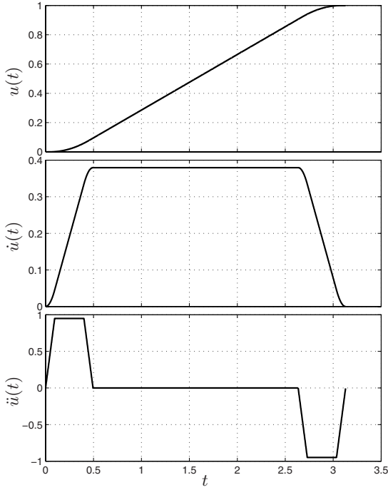
Fig. 9.12. Motion profile of the variable u(t) .
