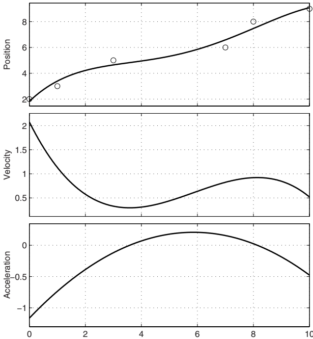
Fig. 4.1. Trajectory approximating 6 points with fourth degree orthogonal polynomials.
