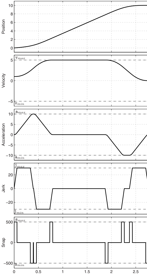
Fig. 3.32. Fifteen segments trajectory (position, velocity, acceleration, jerk and snap).
