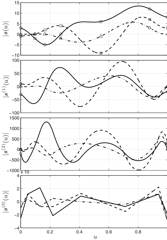
Fig. 8.26. Components of a B-spline trajectory of degree 4 and of its derivatives (component x - solid, component y - dashed, component z - dashdot).
