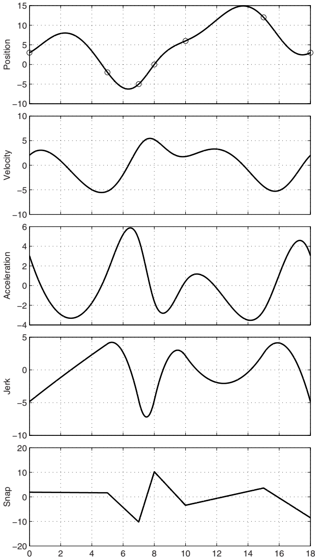
Fig. 4.24. B-spline trajectory with continuity of the snap ( p = 5 ) computed with periodic conditions.
