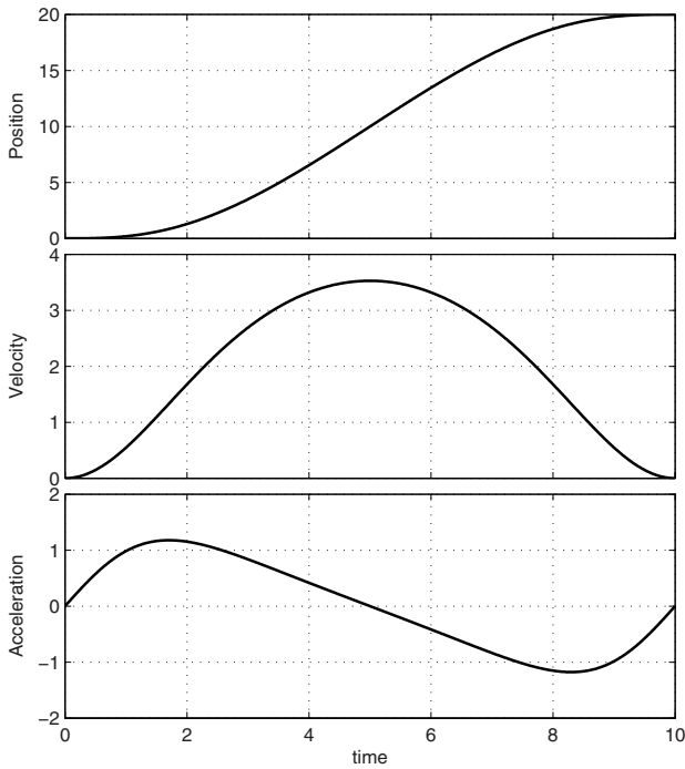
Fig. 3.42. Position, velocity and acceleration profiles for a modified cycloidal trajectory when h = 20 , T = 10 , \kappa = 0.134 .
