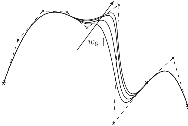
Fig. B.9. Local modification of a Nurbs trajectory by acting on a weight.
