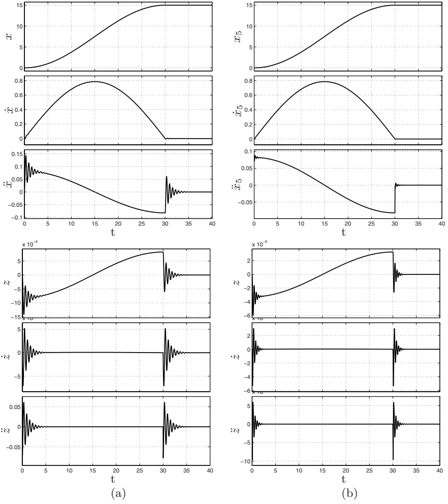
Fig. 7.7. Position, velocity, acceleration and errors ( z = x - q ) of mass m of the one degree of freedom system (a) and of the mass m_5 of the system with five degrees of freedom (b). In this latter case z = x_5 - q . The input q(t) is an harmonic trajectory.
