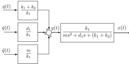
Fig. 7.61. Feedforward action for the tracking of the desired motion profile q(t) , with the mechanical system in Fig. 7.34.
