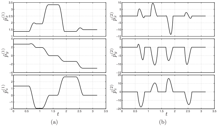
Fig. 9.3. Components of the velocity \tilde{\mathbf{p}}^{(1)}(t) (a) and of the acceleration \tilde{\mathbf{p}}^{(2)}(t) (b) of the trajectory composed by linear and 5-th degree Bézier segments, after a constant scaling.
