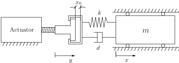
Fig. 7.4. A one degree of freedom model with backlash.
