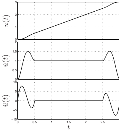
Fig. 9.27. Smooth parameterization u(t) for the computation of B-spline trajectories.
