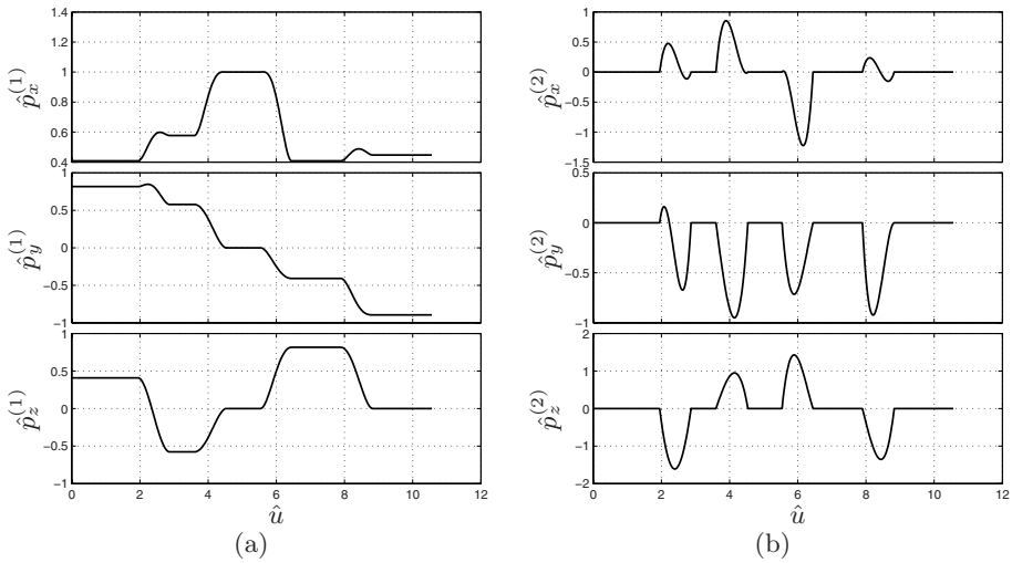
Fig. 8.46. Components of the velocity \hat{\mathbf{p}}^{(1)}(\hat{u}) (a) and of the acceleration \hat{\mathbf{p}}^{(2)}(\hat{u}) (b) of the trajectory composed by linear and 5-th degree Bézier segments.
