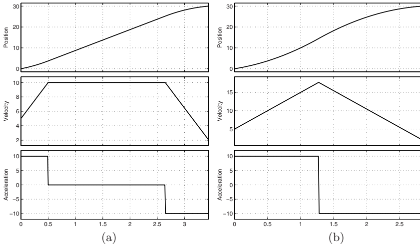
Fig. 3.8. Position, velocity and acceleration of a trapezoidal trajectory with non-null initial and final velocities when the maximum speed v_{max} is reached (a) or not (b).
