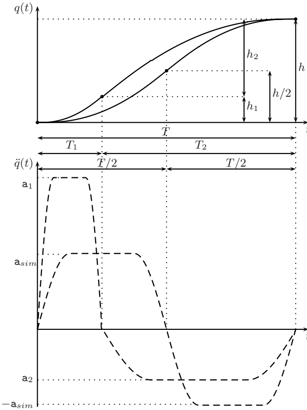
Fig. 3.36. Modified trapezoidal trajectory with different acceleration and deceleration periods.
