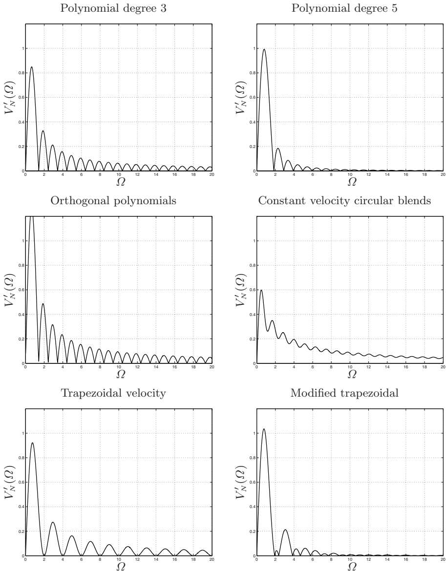
Fig. 7.27. Frequency analysis of the acceleration profiles for the trajectories: polynomials of degree 3 and 5, orthogonal polynomials, constant velocity (linear) with circular blends, trapezoidal, modified trapezoidal.
