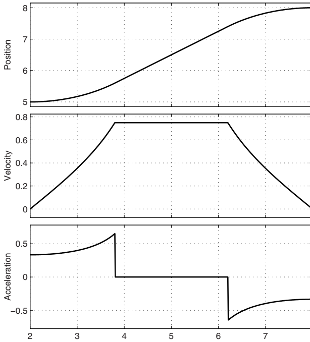
Fig. 3.2. Position, velocity and acceleration of a trajectory with constant velocity and circular connections when t_0 = 2 , t_1 = 8 , q_0 = 5 , q_1 = 8 .
