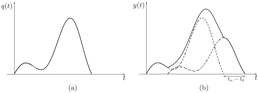
Fig. 7.48. Generic trajectory q(t) (a), and input function y(t) obtained by convoluting q(t) with a ZV shaper (b).
