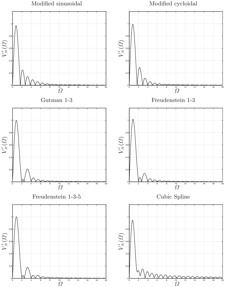
Fig. 7.28. Frequency analysis of the acceleration profiles for the trajectories: modified sinusoidal, modified cycloidal, Gutman 1-3, Freudenstein 1-3 and 1-3-5, cubic spline.
