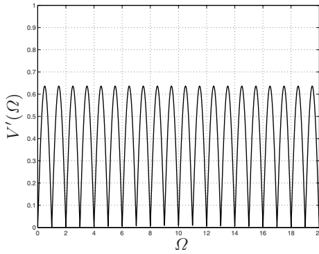
Fig. 7.19. Harmonic content of the constant velocity trajectory.
