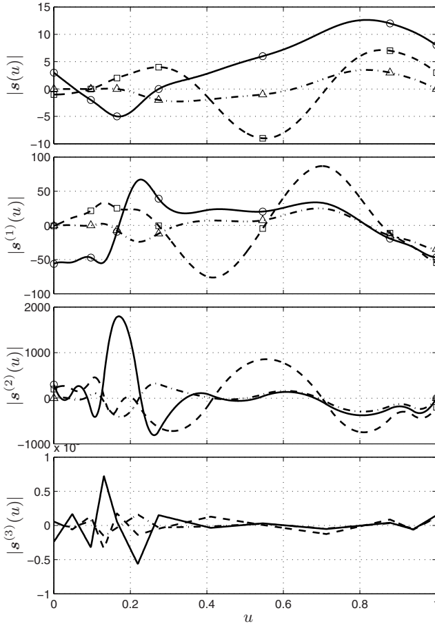
Fig. 8.32. Components of a B-spline trajectory of degree 4 with constraints on positions and tangent vectors (component x - solid, component y - dashed, component z - dashdot).
