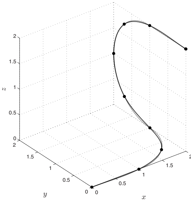
Fig. 9.34. Trajectory based on motion primitives, approximated by a B-spline curve with 12 control points.
