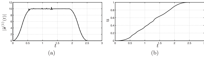
Fig. 9.11. Feed rate of the trajectory defined with a cubic B-spline, with u computed by means of (9.12) (a), and relation between t and u (b).
