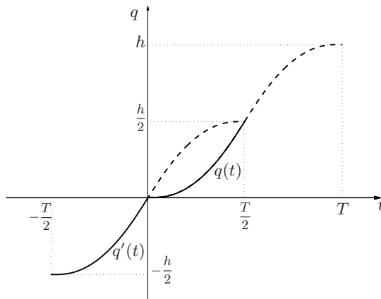
Fig. 5.3. Translation operations on a modified trapezoidal.
