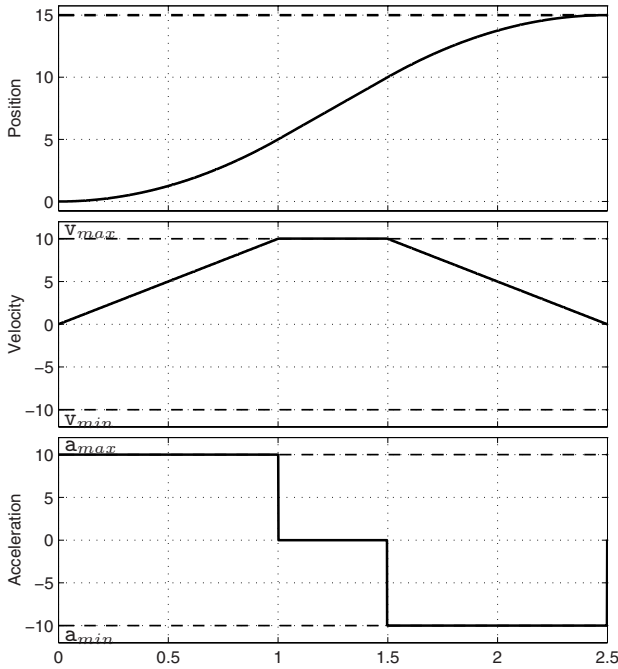
Fig. 4.32. Output (position, velocity and acceleration) of the second order nonlinear filter with a step reference signal.
