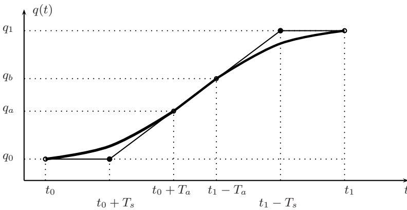
Fig. 3.10. Linear trajectory with polynomial blends.
