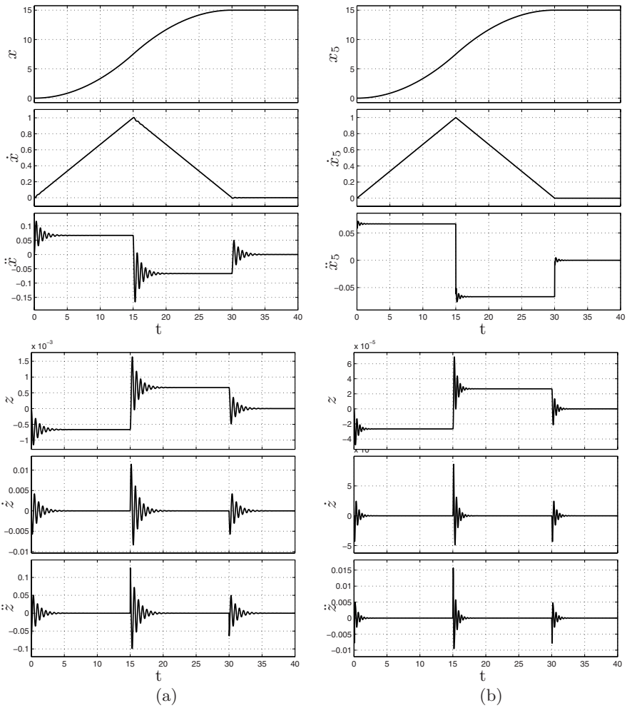
Fig. 7.6. Position, velocity, acceleration and errors ( z = x - q ) of mass m of the one degree of freedom system (a) and of the mass m_5 of the system with five degrees of freedom (b). In this latter case z = x_5 - q . The input q(t) is a constant acceleration trajectory.
