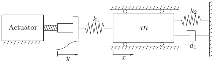
Fig. 7.34. Scheme of the mechanical system considered for the design of a polydyne function.
