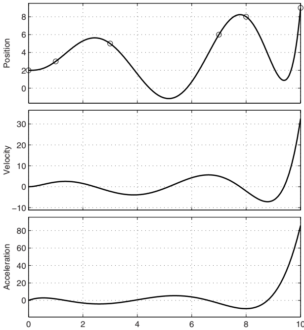
Fig. 4.4. Position, velocity and acceleration of an orthogonal polynomials trajectory ( m = 4 ) with null initial acceleration.
