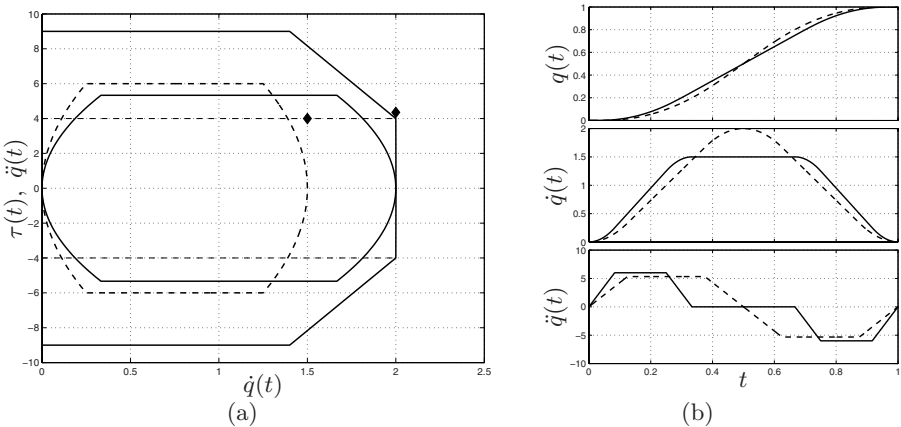
Fig. 6.13. Tasks obtained with a double S trajectory for two different values of \alpha ( \beta = 1/4 in both cases) (a) and plots of position, velocity, acceleration (b).
