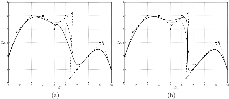
Fig. 8.33. Interpolation by means of smoothing B-spline (dashdot) converted in a Nurbs ( w_j = 1 ), and effects of the modification of some weights.
