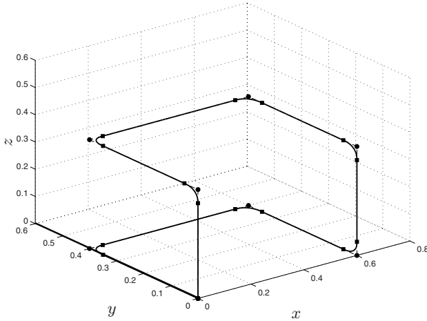
Fig. 9.15. Position trajectory obtained with linear and 5-th degree Bézier segments.
