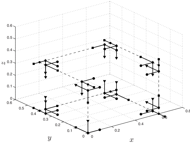
Fig. 9.14. Via-points and related local frames considered for linear interpolation with 5-th degree Bézier blends.
