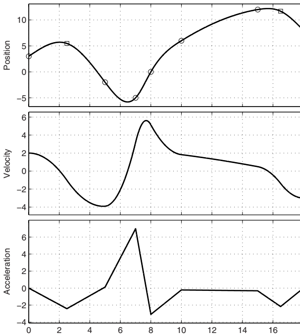
Fig. 4.9. Spline trajectory with constraints on initial and final velocities and accelerations.
