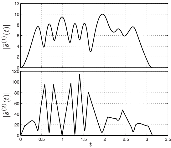
Fig. 9.13. Feed rate induced by a double S trajectory for u(t) .
