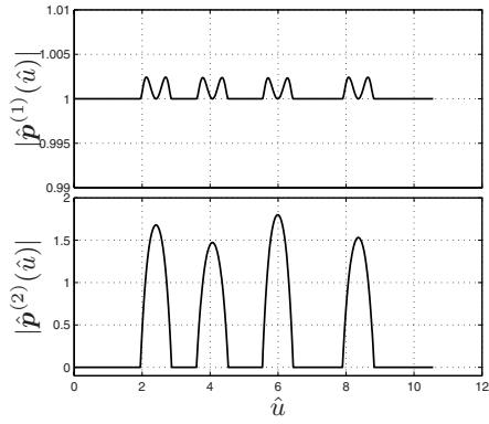
Fig. 8.47. Magnitude of the tangent and curvature vectors of the trajectory composed by straight line segments and 5-th degree Bézier curves.
