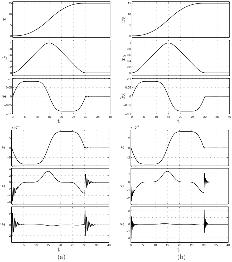
Fig. 7.17. Position, velocity, acceleration and errors ( z = x - q ) of mass m of the one degree of freedom system (a) and of the mass m_5 of the system with five degrees of freedom (b). In this latter case z = x_5 - q . The input q(t) is a Freudenstein 1-3-5 trajectory.
