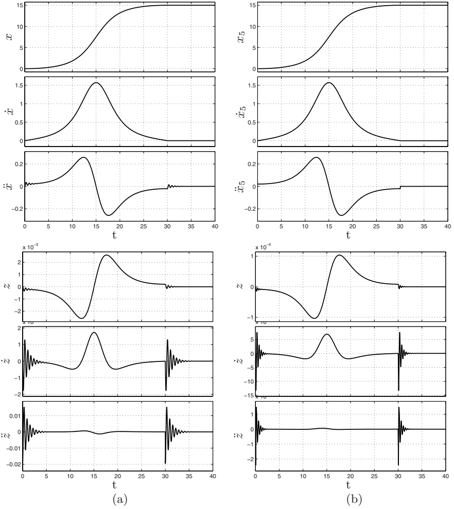
Fig. 7.9. Position, velocity, acceleration and errors ( z = x - q ) of mass m of the one degree of freedom system (a) and of the mass m_5 of the system with five degrees of freedom (b). In this latter case z = x_5 - q . The input q(t) is an elliptic trajectory ( n = 2 ).
