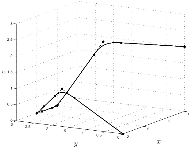
Fig. 8.45. Linear interpolation with polynomial blends obtained as Bézier curves of degree 5.
