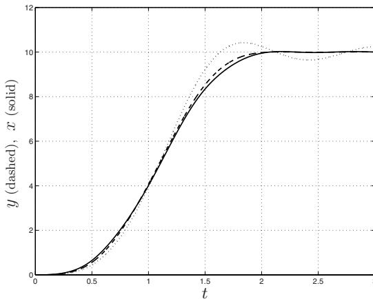
Fig. 7.54. Output of three mechanical systems, which differ from the model G(s) used for the computation of a three-hump EI shaper in the value of the natural frequency. In particular, the values \omega_n = 9 (solid), \omega_n = 7 (dashed), \omega_n = 5 (dotted) are assumed.
