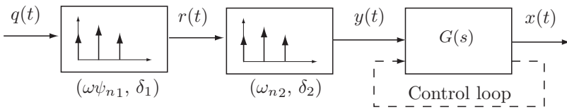
Fig. 7.57. Block diagram of a system with a cascade of two shapers.
