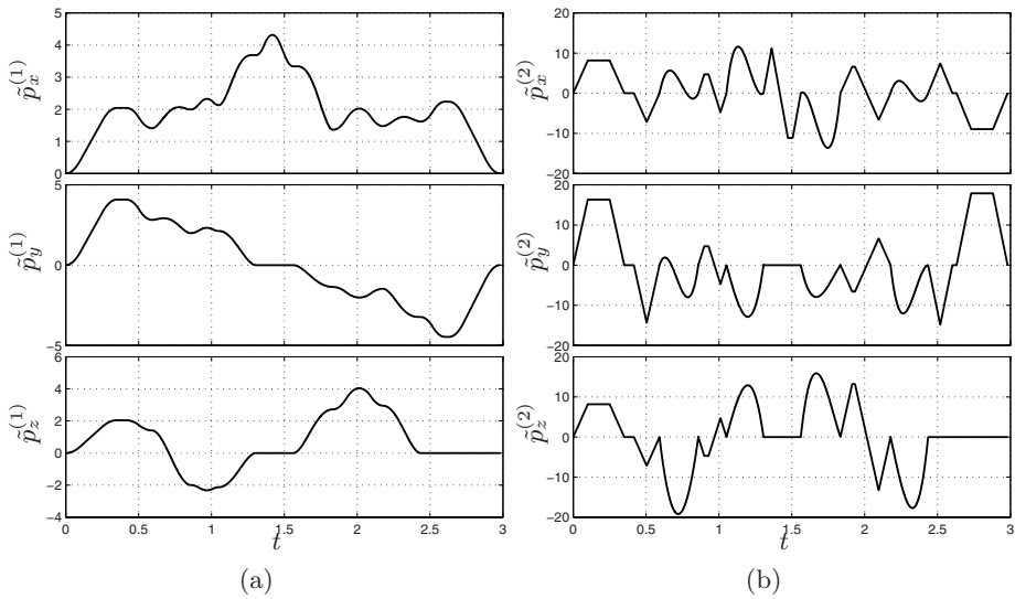
Fig. 9.5. Components of the velocity \tilde{\mathbf{p}}^{(1)}(t) (a) and of the acceleration \tilde{\mathbf{p}}^{(2)}(t) (b) of the trajectory composed by linear and 5-th degree Bézier segments.
