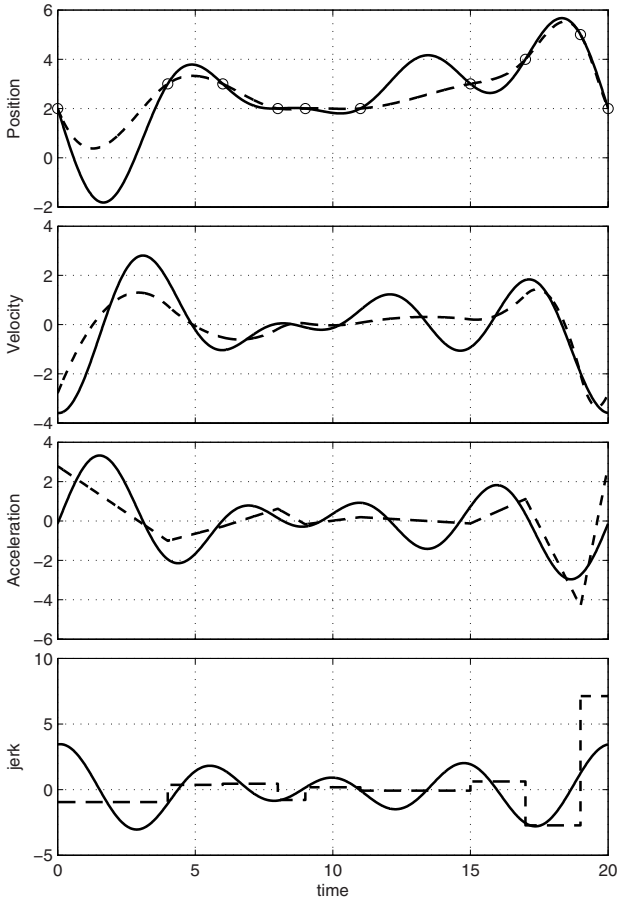
Fig. 4.5. Interpolation of a set of via-points by means of a trigonometric polynomial (solid) compared with a standard cubic spline (dashed).
