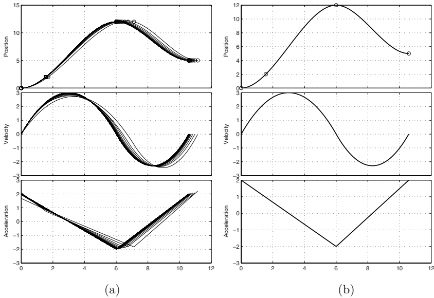
Fig. 4.17. Optimal spline through a set of points: iterative procedure (a) and final trajectory (b).
