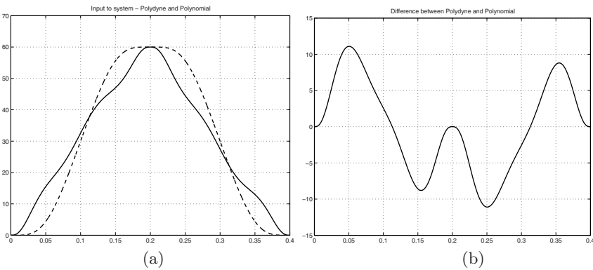
Fig. 7.43. Functions q(t) (solid) and q'(t) (dashed) given as input to the system (a), and their difference (b).
