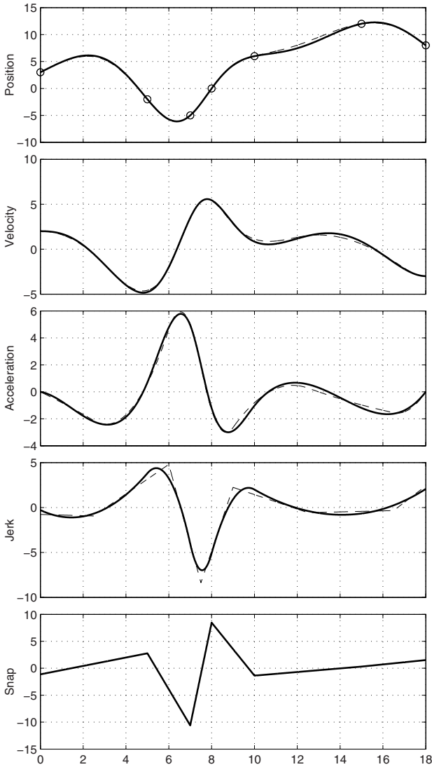
Fig. 4.23. B-spline trajectory with continuity of the snap ( p = 5 ).
