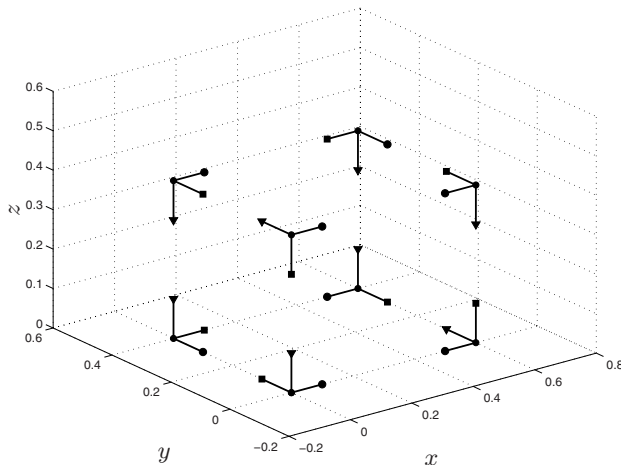
Fig. 9.23. Via-points and related local frames considered for B-spline interpolation.
