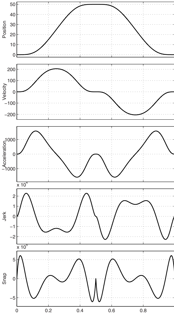
Fig. 7.37. Desired motion profile x(t) for the mass of Fig. 7.34.
