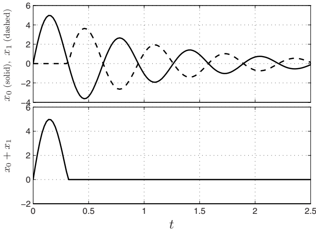
Fig. 7.45. Response to the Dirac impulse of the second order system (7.21) and vibration cancellation using two impulses.
