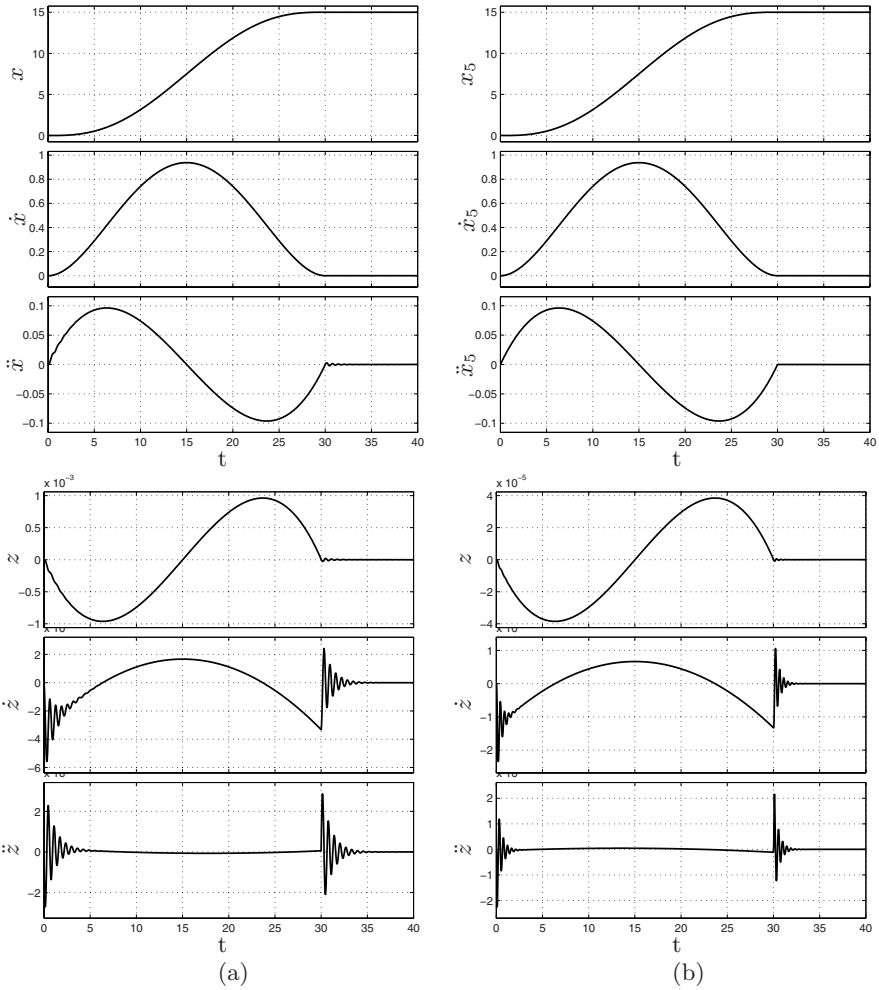
Fig. 7.11. Position, velocity, acceleration and errors ( z = x - q ) of mass m of the one degree of freedom system (a) and of the mass m_5 of the system with five degrees of freedom (b). In this latter case z = x_5 - q . The input q(t) is a polynomial trajectory of degree five.
