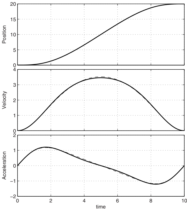
Fig. 3.44. Position, velocity and acceleration profiles for a modified cycloidal trajectory with h = 20 , T = 10 , \kappa = 0.134 (solid), and same trajectory computed with a polynomial function of degree five approximating t_m(t) (dashed).
