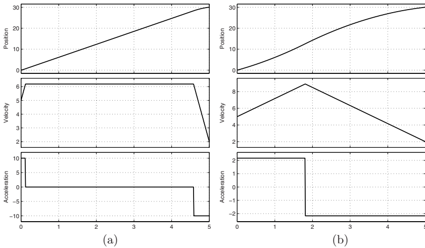
Fig. 3.7. Position, velocity and acceleration of a trapezoidal trajectory with non-null initial and final velocities computed for a given duration T and a maximum acceleration \mathbf{a}_{max} , when the constant speed tract is present (a) or not (b).
