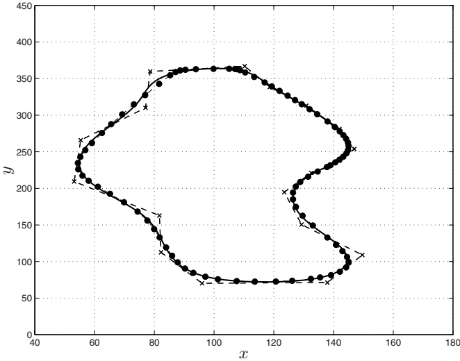
Fig. 8.21. Global approximation by means of a B-spline (solid) defined by 20 control points, represented by the x-marks on the control polygon (dashed).
