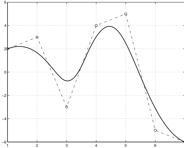
Fig. B.4. Cubic B-spline and its control polygon.
