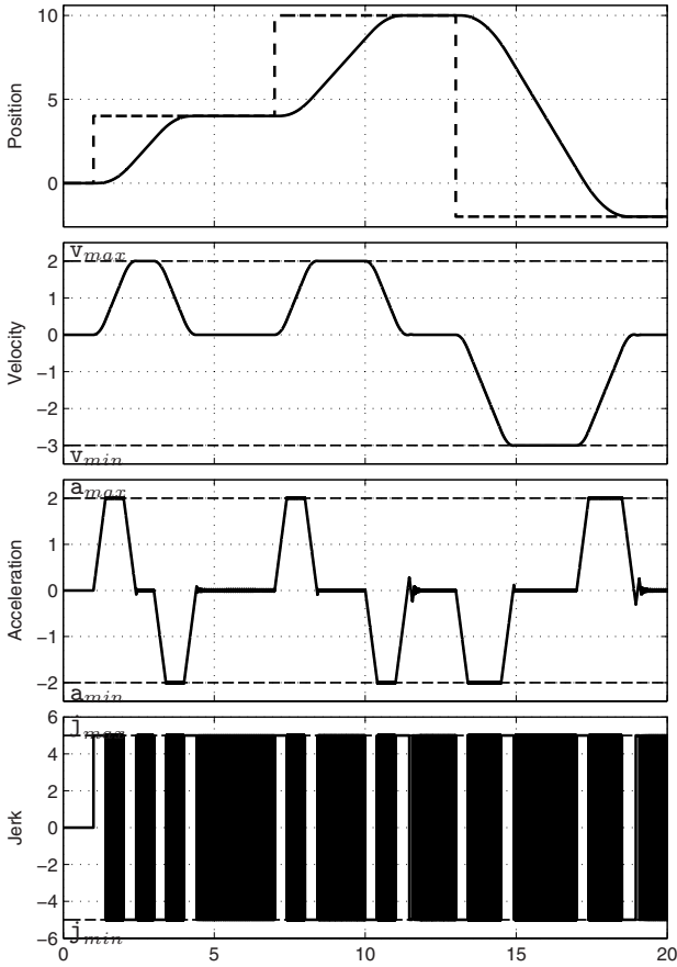
Fig. 4.27. Double S trajectory profiles (position, velocity, acceleration and jerk) computed by means of the third order nonlinear filter, with T_s = 0.001s .
