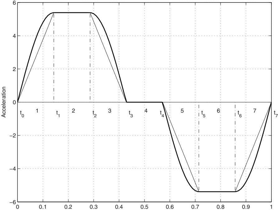
Fig. 3.52. Acceleration of a generic trajectory: the profiles in the odd segments may be defined either by linear or trigonometric functions.
