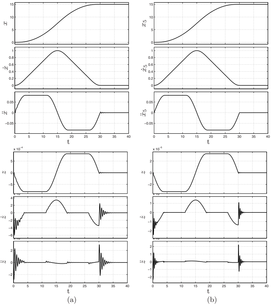
Fig. 7.14. Position, velocity, acceleration and errors ( z = x - q ) of mass m of the one degree of freedom system (a) and of the mass m_5 of the system with five degrees of freedom (b). In this latter case z = x_5 - q . The input q(t) is a modified trapezoidal velocity trajectory.
