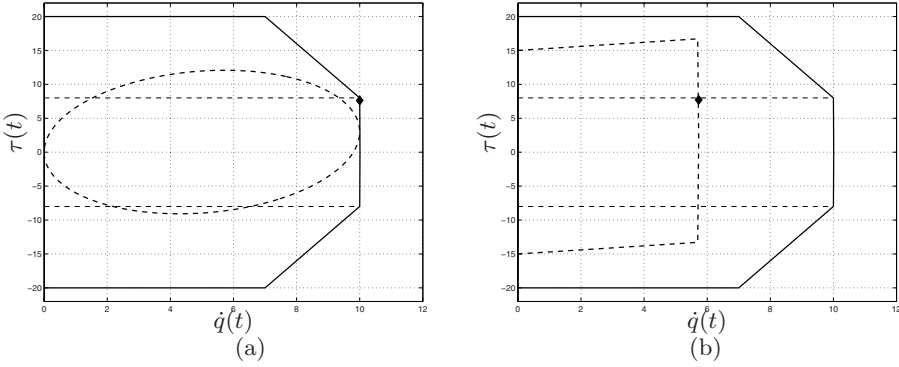
Fig. 6.3. Location of the point (\dot{q}_{max}, \tau_{rms},) for two different motion laws: a cycloidal trajectory (a) and a trapezoidal velocity trajectory (b).
