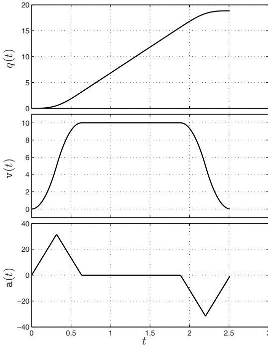
Fig. 9.10. Trajectory of the desired feed rate.
