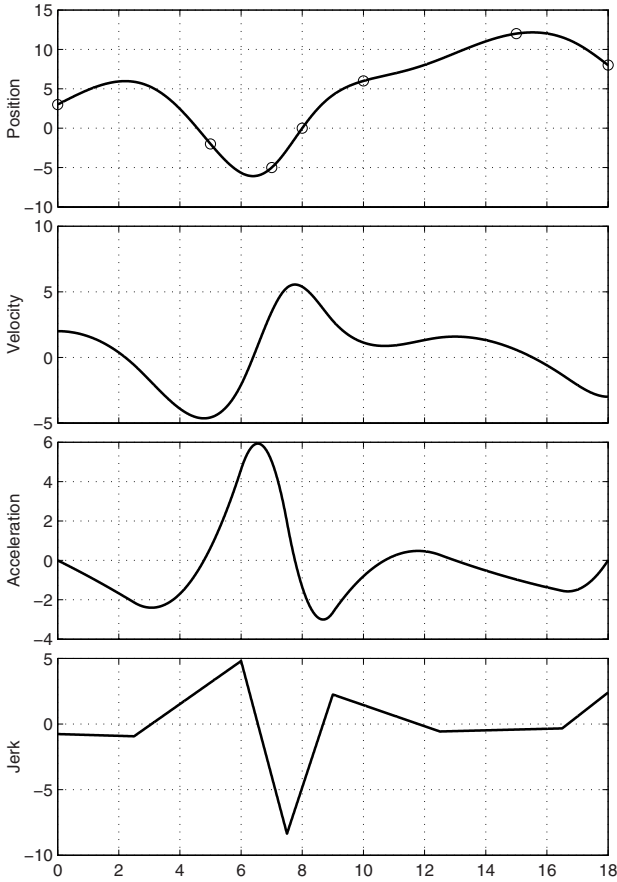
Fig. 4.18. B-spline trajectory with continuity of the jerk ( p = 4 ), obtained by computing the knot vector as in (4.43).
