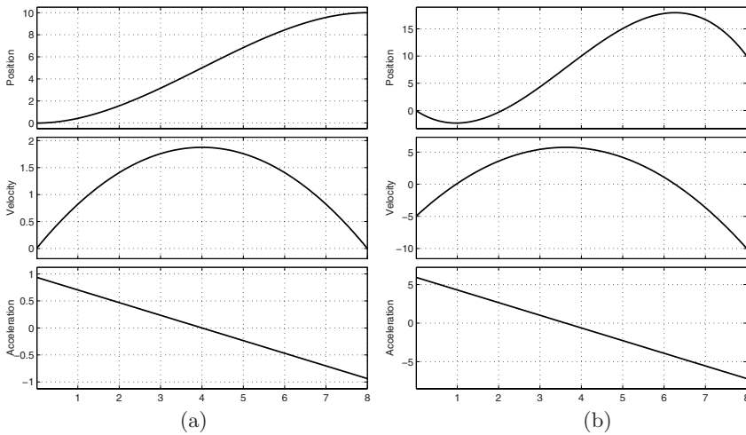
Fig. 2.7. Position, velocity and acceleration of a third degree polynomial trajectory with the conditions q_0 = 0, q_1 = 10, t_0 = 0, t_1 = 8 . In (a) the initial and final velocities are null ( v_0 = v_1 = 0 ), while in (b) the values v_0 = -5, v_1 = -10 have been assigned.
