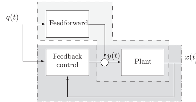
Fig. 7.33. Standard two dof controller.
