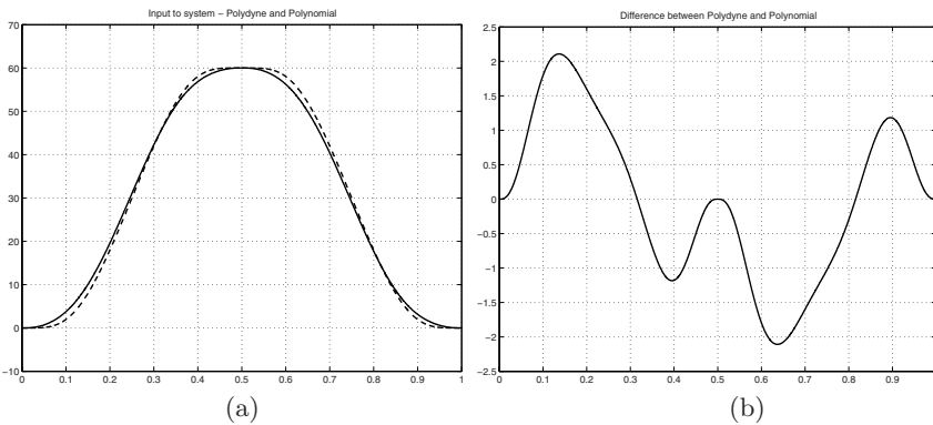
Fig. 7.40. Functions q(t) (solid) and q'(t) (dashed) given as input to the system (a), and their difference (b).
