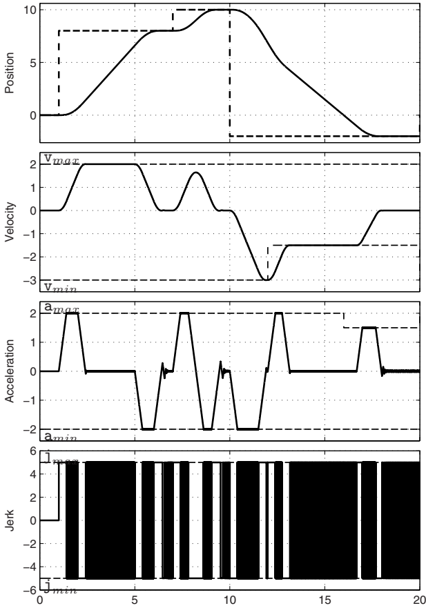
Fig. 4.29. Double S trajectory profiles computed by means of the third order nonlinear filter with variable constraints.
