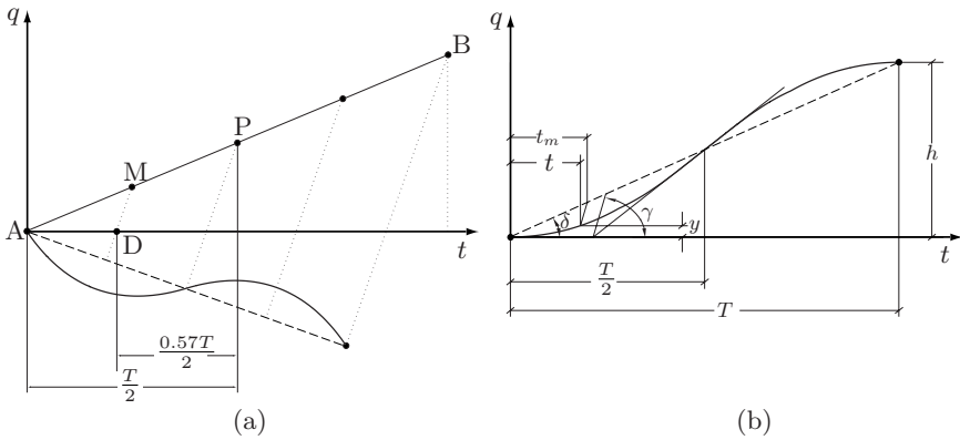
Fig. 3.40. Geometrical construction of the modified cycloidal trajectory with the Wildt method.
