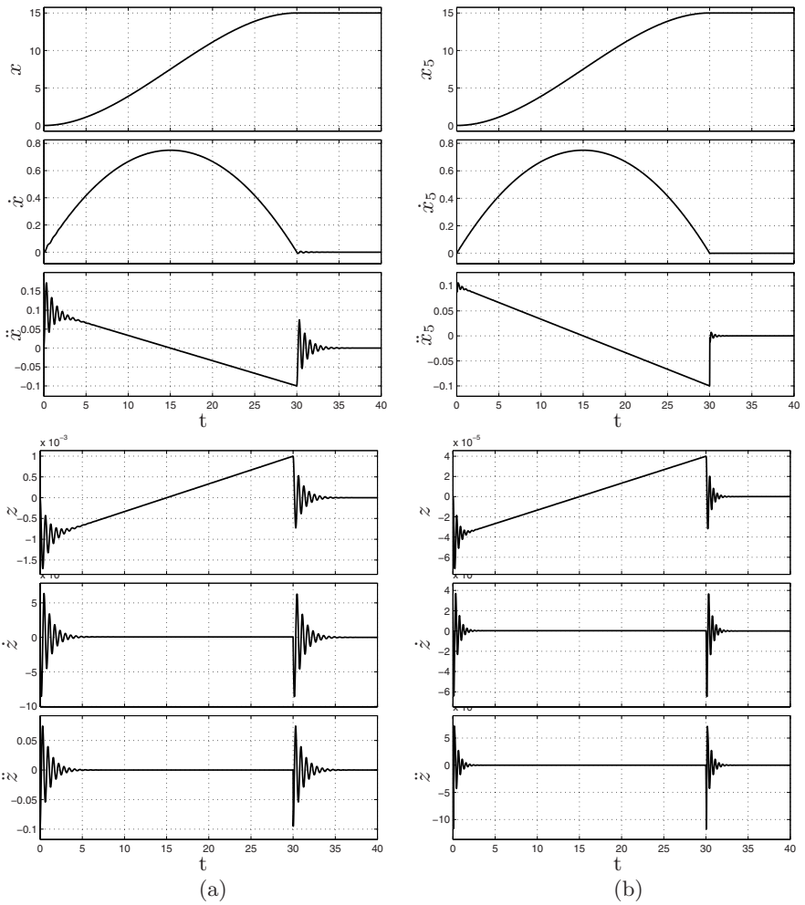
Fig. 7.10. Position, velocity, acceleration and errors ( z = x - q ) of mass m of the one degree of freedom system (a) and of the mass m_5 of the system with five degrees of freedom (b). In this latter case z = x_5 - q . The input q(t) is a polynomial trajectory of degree three.
