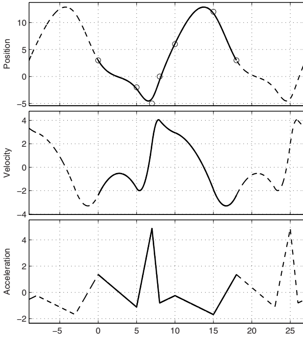
Fig. 4.13. Smoothing splines with periodic conditions.
