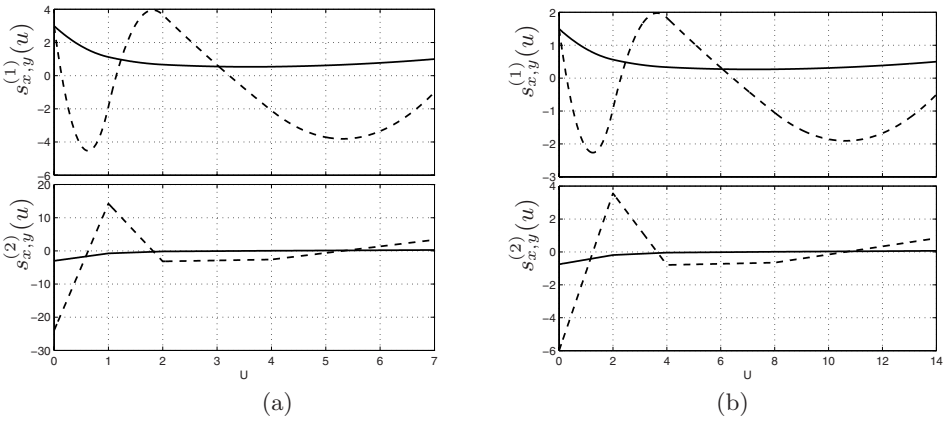
Fig. B.6. Components of the first and second derivatives ( x solid, y dashed) of the B-spline curves computed for u (a) and u' = 2u (b).
