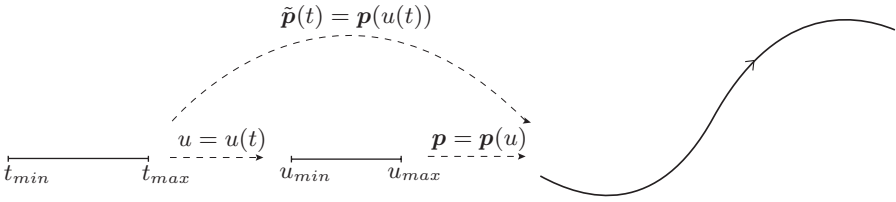
Fig. 9.1. Composition of a generic 3D path \mathbf{p}(u) and of a motion law u(t) .
