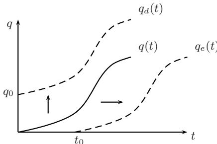
Fig. 5.2. Geometric construction of trajectories by translation.
