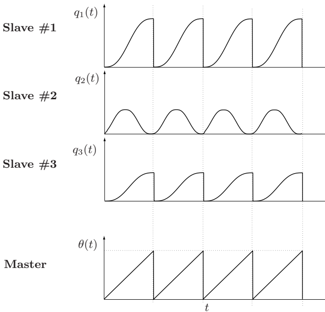
Fig. 5.15. Position profiles of master and slaves as a function of time in a multi-slave system.
