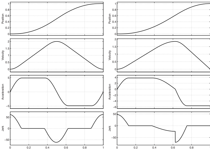
Fig. 3.49. Trajectories obtained with different choices of the parameters T_k : position, velocity, acceleration, and jerk.
