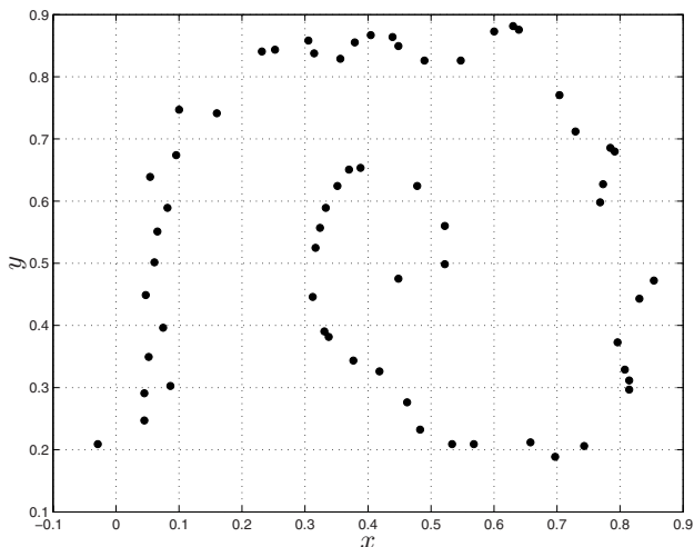
Fig. 9.29. Via-points used for the approximation with a smoothing B-spline.
