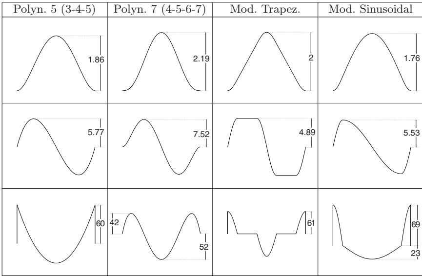
Fig. 6.5. From the top, velocity, acceleration and jerk profiles for the trajectories: 5-th, 7-th degree polynomial, modified trapezoidal, modified sinusoidal.
