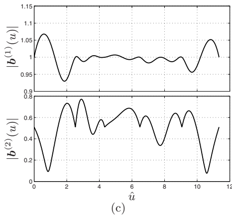
Fig. 8.41. Velocity and acceleration of the trajectory composed by quintic Bézier curves for different values of \bar{\beta} : a) \bar{\beta} = 1 , b) \bar{\beta} = 0.75 , c) \bar{\beta} = 0.51 .
