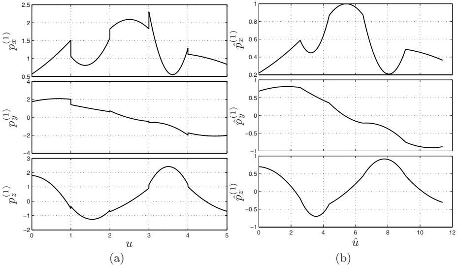
Fig. 8.37. Components of the tangent vector \mathbf{p}^{(1)}(u) of the trajectory composed by Bézier segments, without (a) and with (b) “scaling in time”.
