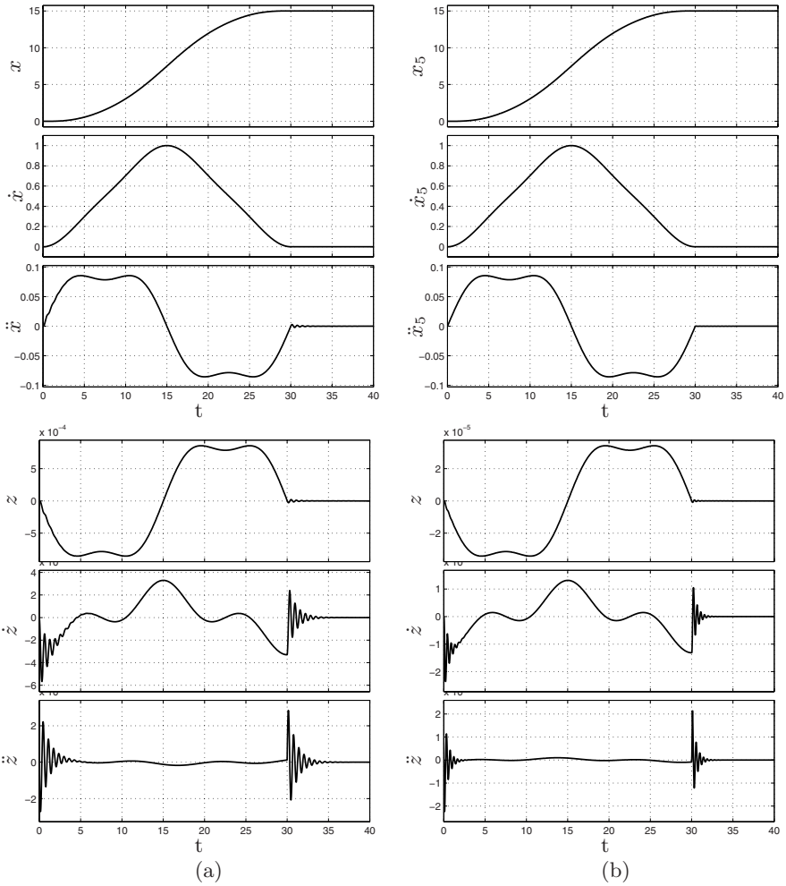
Fig. 7.15. Position, velocity, acceleration and errors ( z = x - q ) of mass m of the one degree of freedom system (a) and of the mass m_5 of the system with five degrees of freedom (b). In this latter case z = x_5 - q . The input q(t) is a Gutman 1-3 trajectory.
