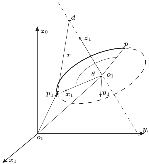
Fig. 8.15. Example of motion primitive: circular arc.
