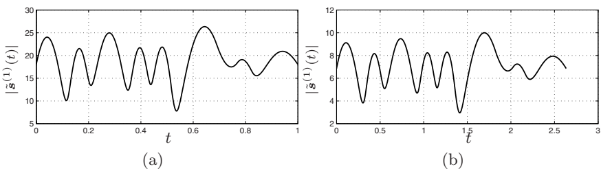
Fig. 9.7. Feed rate of the trajectory defined with a cubic B-spline, with u = t (a), and with u = \lambda t (b).
