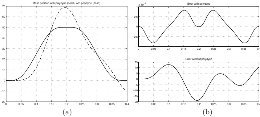
Fig. 7.42. Position of the mass of Fig. 7.34 (a) and tracking errors due to the elasticity (b) with and without using the polydyne; note the different amplitudes of the diagrams in (b).
