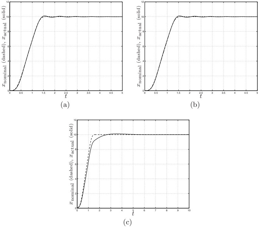
Fig. 7.67. Response of the systems considered in the Examples 7.7, 7.8 and 7.9, when the actual system is different from the nominal model used to compute the feedforward action y(t) .
