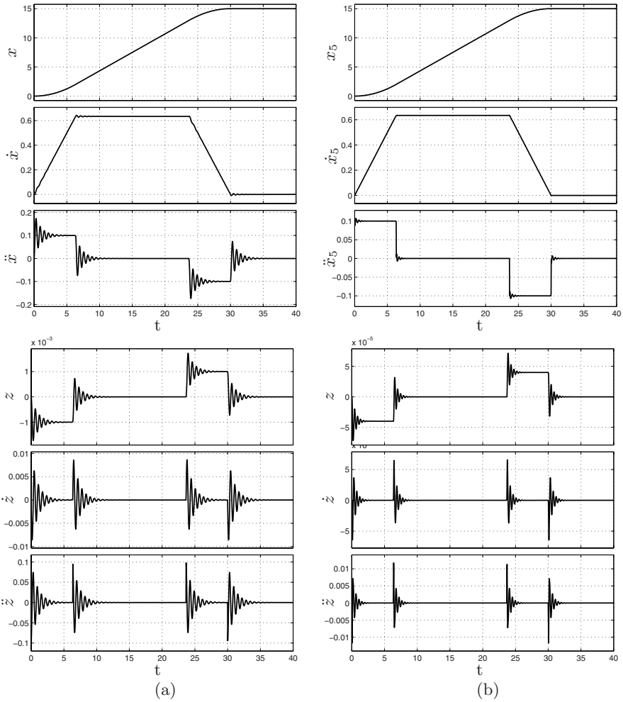
Fig. 7.13. Position, velocity, acceleration and errors ( z = x - q ) of mass m of the one degree of freedom system (a) and of the mass m_5 of the system with five degrees of freedom (b). In this latter case z = x_5 - q . The input q(t) is a trapezoidal velocity trajectory.
