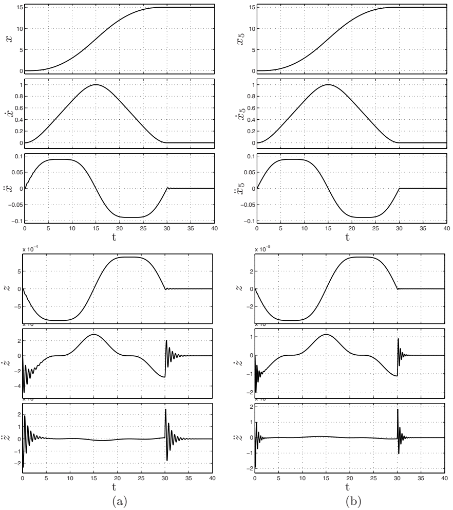
Fig. 7.16. Position, velocity, acceleration and errors ( z = x - q ) of mass m of the one degree of freedom system (a) and of the mass m_5 of the system with five degrees of freedom (b). In this latter case z = x_5 - q . The input q(t) is a Freudenstein 1-3 trajectory.
