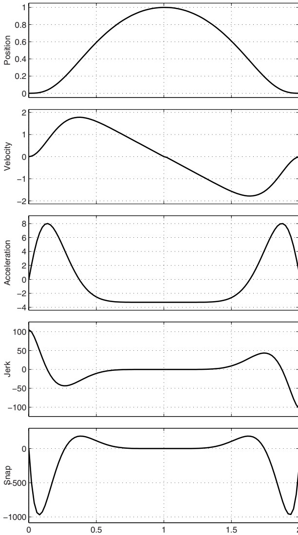
Fig. 7.35. Position, velocity, acceleration, jerk and snap for the Dudley polynomial function.
