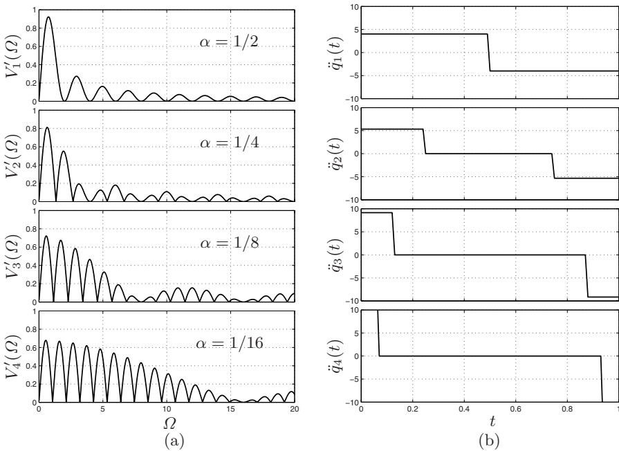
Fig. 7.21. Harmonic content (a) and related acceleration profiles (b) of trapezoidal trajectories for different values of the parameter \alpha .
