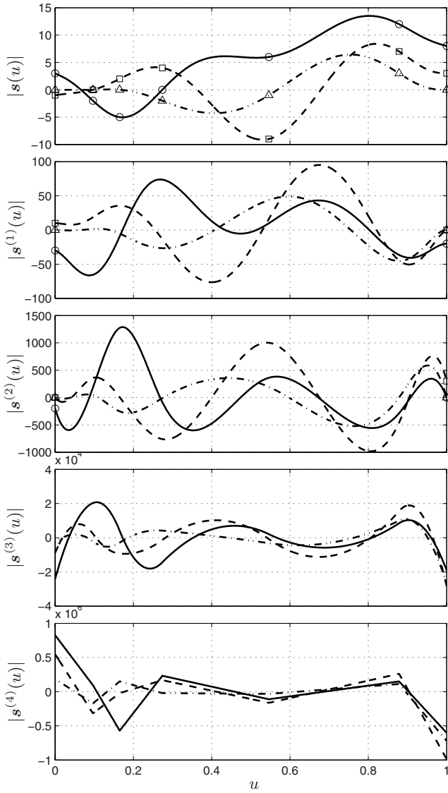
Fig. 8.30. Components of a B-spline trajectory of degree 5 (component x - solid, component y - dashed, component z - dashdot).
