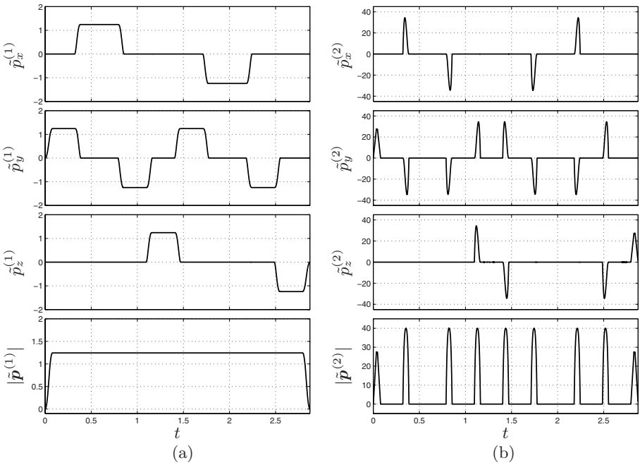
Fig. 9.21. Velocity and acceleration (components and magnitude) of a trajectory composed by linear and 5-th degree Bézier segments, with a motion law which limits the maximum acceleration.
