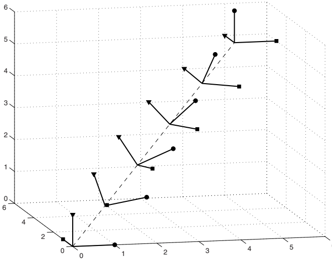
Fig. 8.9. Frame change obtained with an axis-angle representation.
