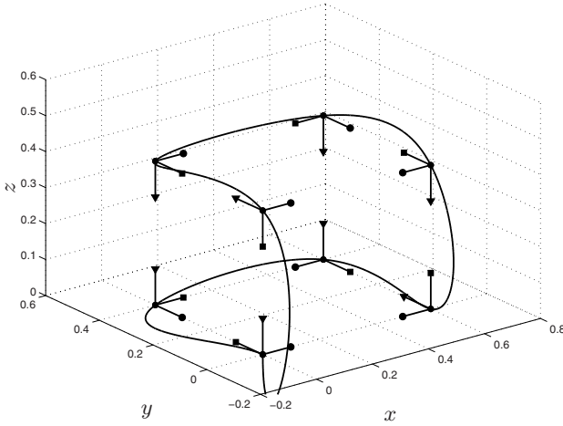
Fig. 9.24. Position trajectory obtained with a B-spline curve.
