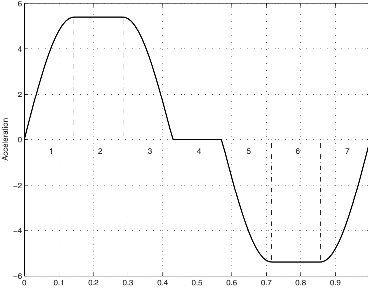
Fig. 3.48. Generic acceleration profile with sinusoidal blends.
