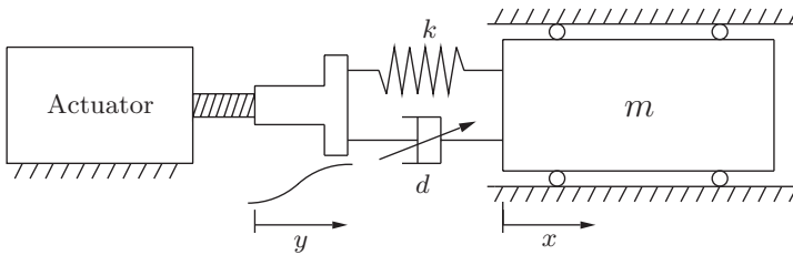
Fig. 7.3. One degree of freedom model with passive nonlinear parameters.
