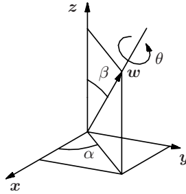
Fig. C.2. Angle-Axis representation.
