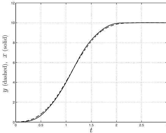
Fig. 7.53. Response of the system G(s) = \frac{2s+1}{s^2+2s+100} to a double S trajectory with a three-hump EI input shaper.
