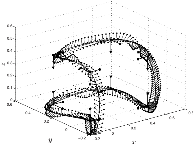
Fig. 9.25. Trajectory for the orientation superimposed to the B-spline position trajectory.
