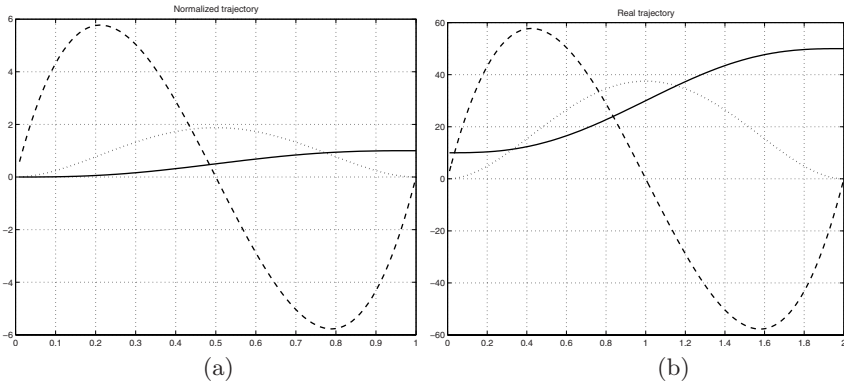
Fig. 5.8. Profiles of acceleration (dashed), velocity (dotted) and position (solid) of a polynomial of degree 5: normalized form (a) and with boundary conditions q_0 = 10 , q_1 = 50 , t_0 = 0 , t_1 = 2 (b).
