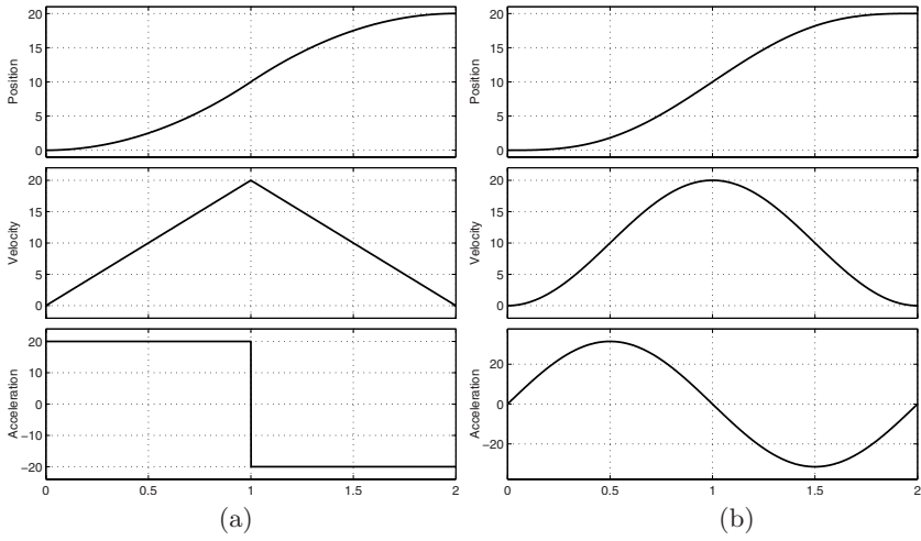
Fig. 3.53. Trajectory with constant (a) and cycloidal (b) acceleration.
