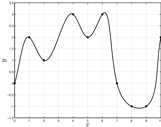
Fig. 9.6. Geometric path defined with a cubic B-spline \mathbf{s}(u) ( 0 \leq u \leq 1 ).
