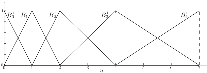
Fig. B.1. B-spline basis functions of degree 1 defined on \mathbf{u} = [0, 0, 1, 2, 4, 7, 7] .
