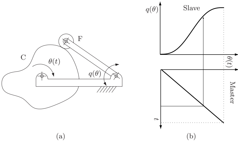
Fig. 5.14. (a) Mechanical cam (C) with a follower (F); (b) function defining an electronic cam.
