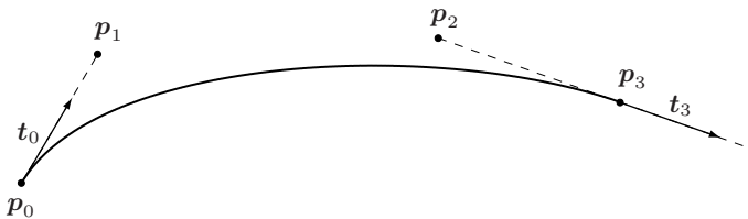
Fig. 8.35. Bézier curve of degree 3 and its control points.
