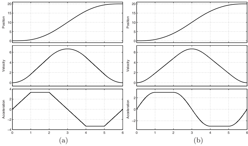
Fig. 3.54. Trajectory with a trapezoidal (a) and modified trapezoidal (b) acceleration profile.
