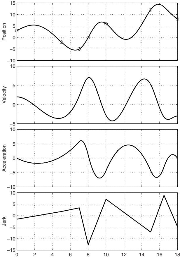
Fig. 4.19. B-spline trajectory of degree 4, obtained by computing the knot vector as in (4.42).
