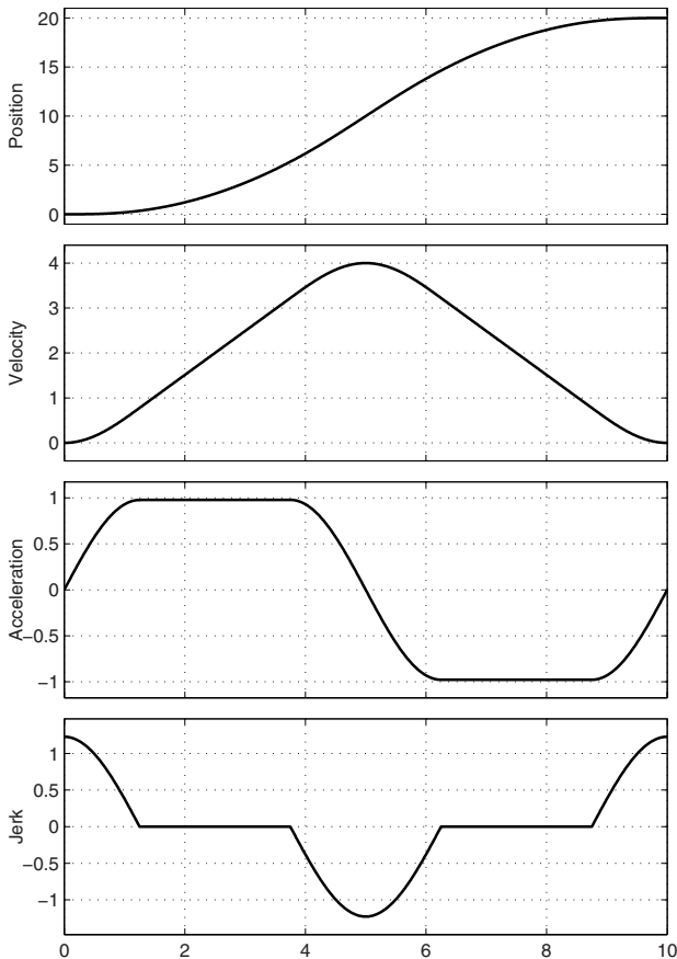
Fig. 3.35. Position, velocity, acceleration and jerk of a modified trapezoidal trajectory with h = 20 , T = 10 .
