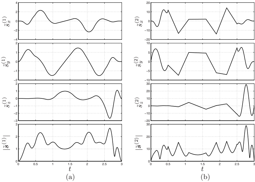
Fig. 9.28. Velocity and acceleration (components and magnitude) of the position trajectory represented by a B-spline curve, with the parameterization of Fig. 9.27.
