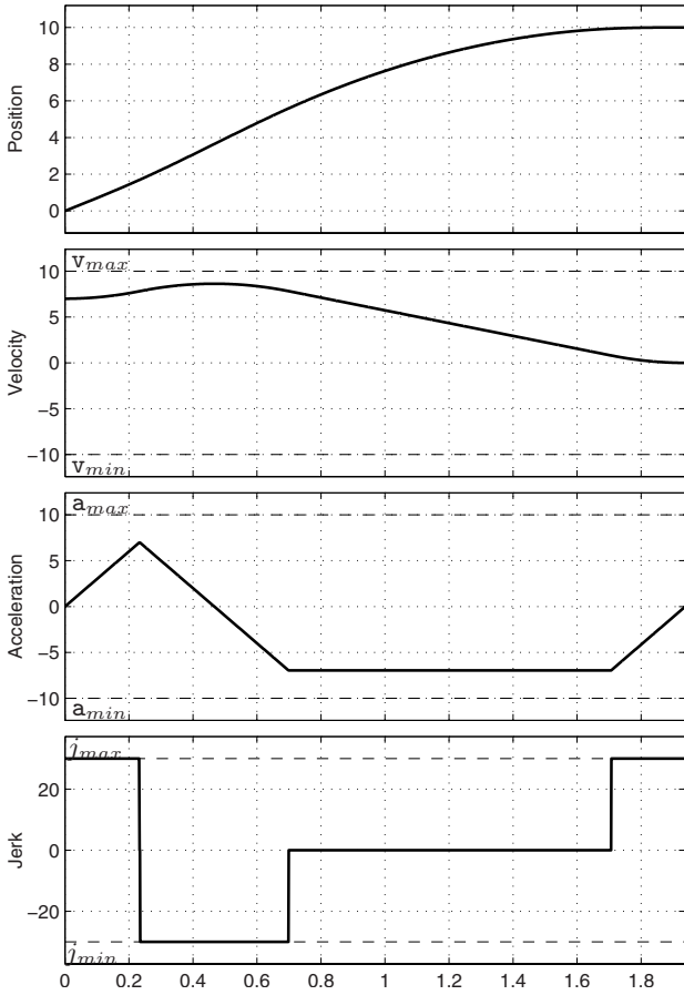
Fig. 3.16. Double S trajectory profiles (position, velocity, acceleration and jerk) without the constant velocity phase and with limit acceleration lower than the maximum value.
