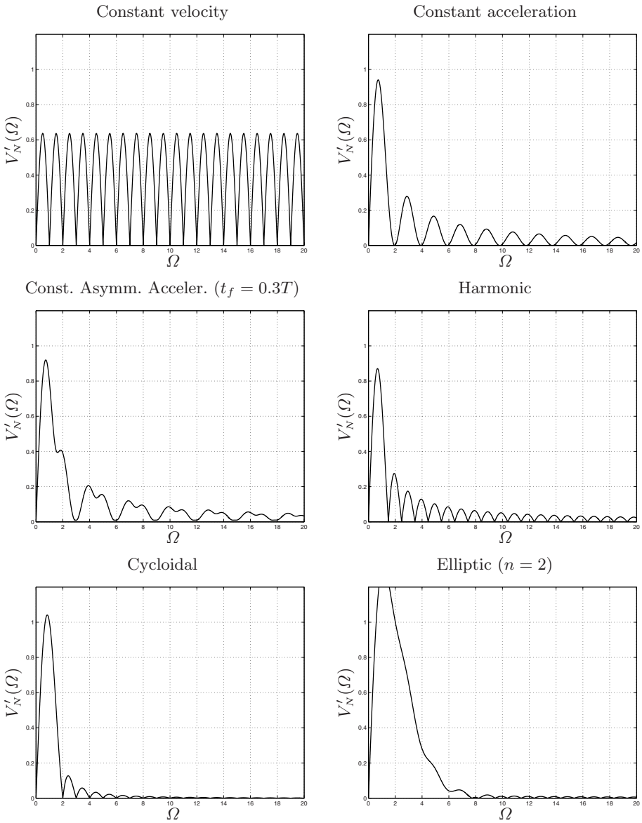
Fig. 7.26. Frequency analysis of the acceleration profiles for the trajectories: constant velocity, constant acceleration, asymmetric constant acceleration, harmonic, cycloidal and elliptic.
