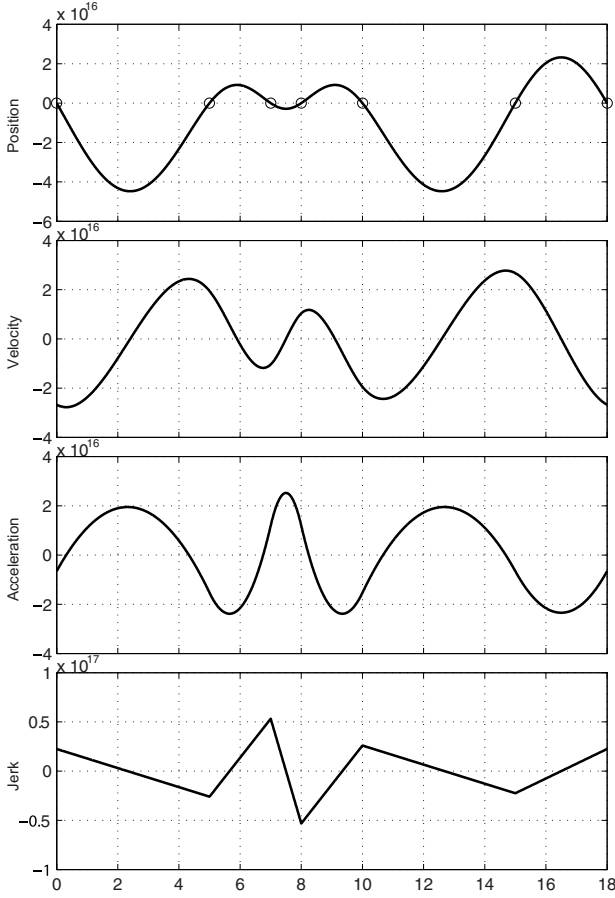
Fig. 4.22. B-spline trajectory of degree 4 with cyclic conditions and with the knot vector \mathbf{u} = [0, 0, 0, 0, 0, 5, 7, 8, 10, 15, 18, 18, 18, 18, 18] .
