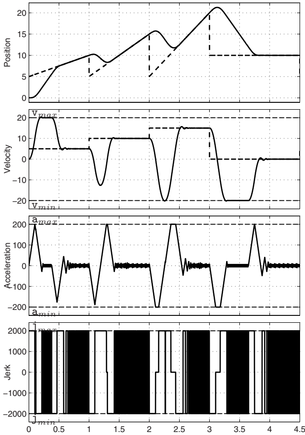
Fig. 4.30. Output (position, velocity, acceleration and jerk) of the third order nonlinear filter with a “sawtooth” reference signal.
