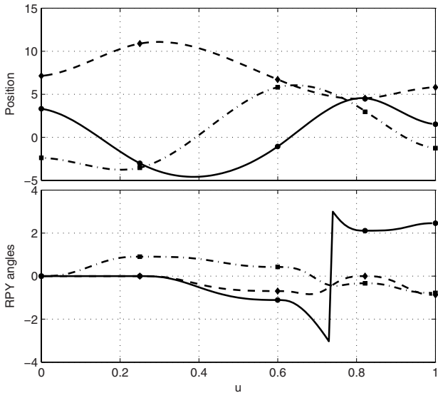
Fig. 8.11. Trajectory for position and orientation in 3D space based on axis-angle representation: profiles of the different components.
