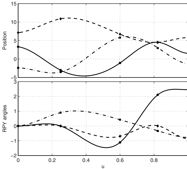
Fig. 8.8. Trajectory for position and orientation in 3D space based on RPY angles representation: profiles of the different components (see Fig. 8.7).
