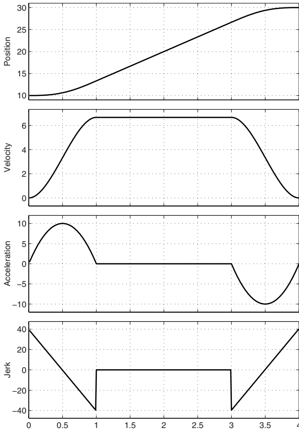
Fig. 3.11. Linear trajectory with fifth degree polynomial blends.
