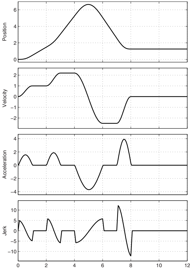
Fig. 3.46. Position, velocity, acceleration and jerk of Example 3.24.a.
