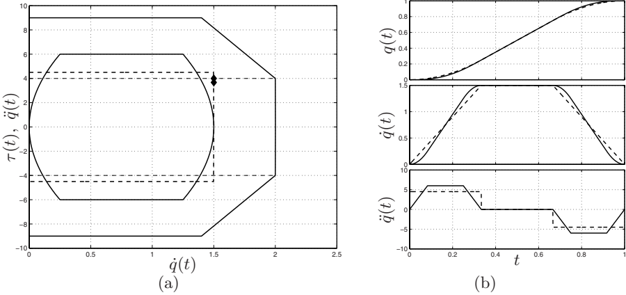
Fig. 6.15. Comparison between trapezoidal (dashed) and double S (solid) trajectories for \alpha = 1/3 : speed-acceleration diagram (a) and plots of position, velocity, acceleration (b).
