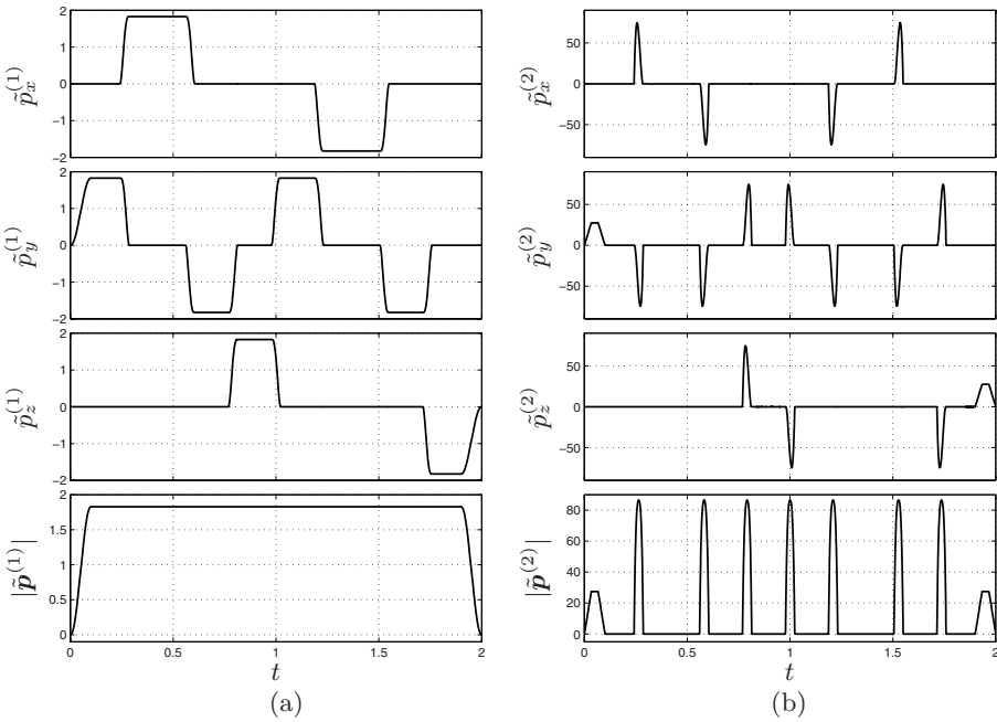
Fig. 9.19. Velocity and acceleration (components and magnitude) of a trajectory composed by linear and 5-th degree Bézier segments, with a double S feed rate.
