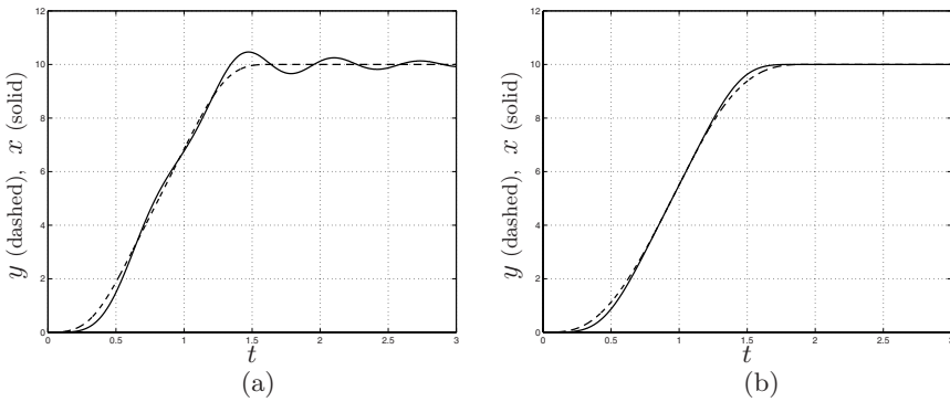
Fig. 7.49. Input (dashed) and output (solid) of G(s) without (a) and with (b) ZV shaper.
