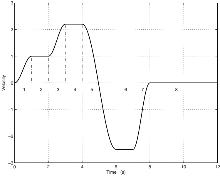
Fig. 3.45. Subdivision of a velocity profile.
