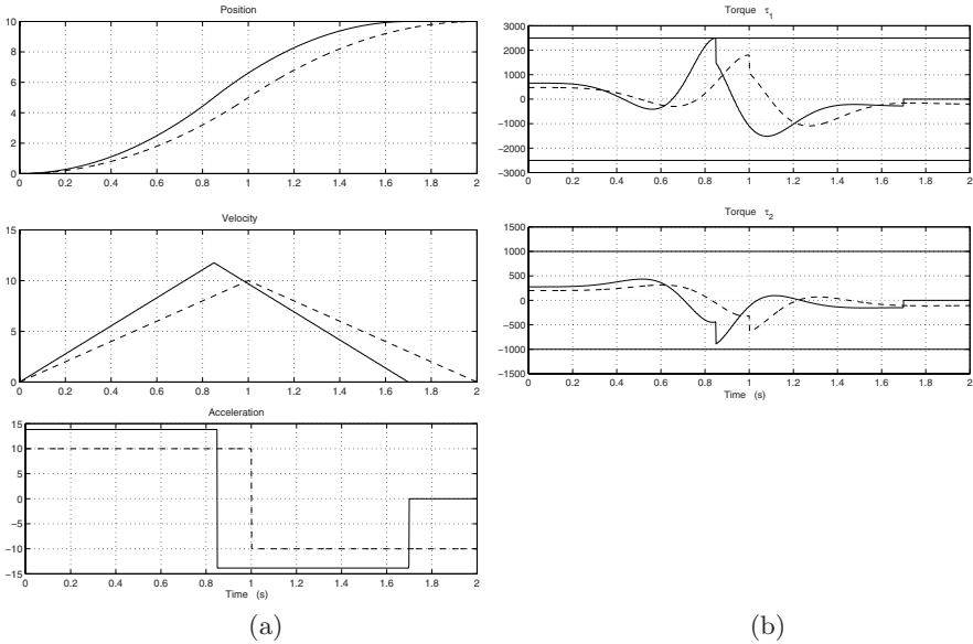
Fig. 5.13. Position, velocity, acceleration (a) and torque (b) profiles before (dashed) and after (solid) a dynamic scaling operation (Example 5.6).
