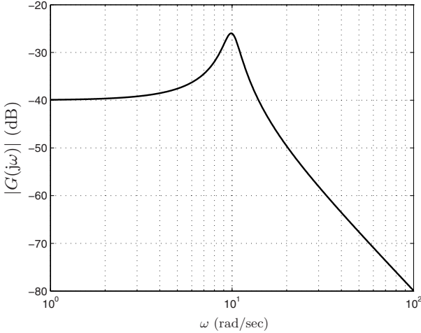
Fig. 7.18. Magnitude of the frequency response of the system (7.2).
