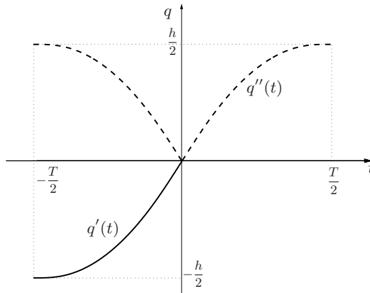
Fig. 5.4. Reflection operations on a segment of the modified trapezoidal profile.
