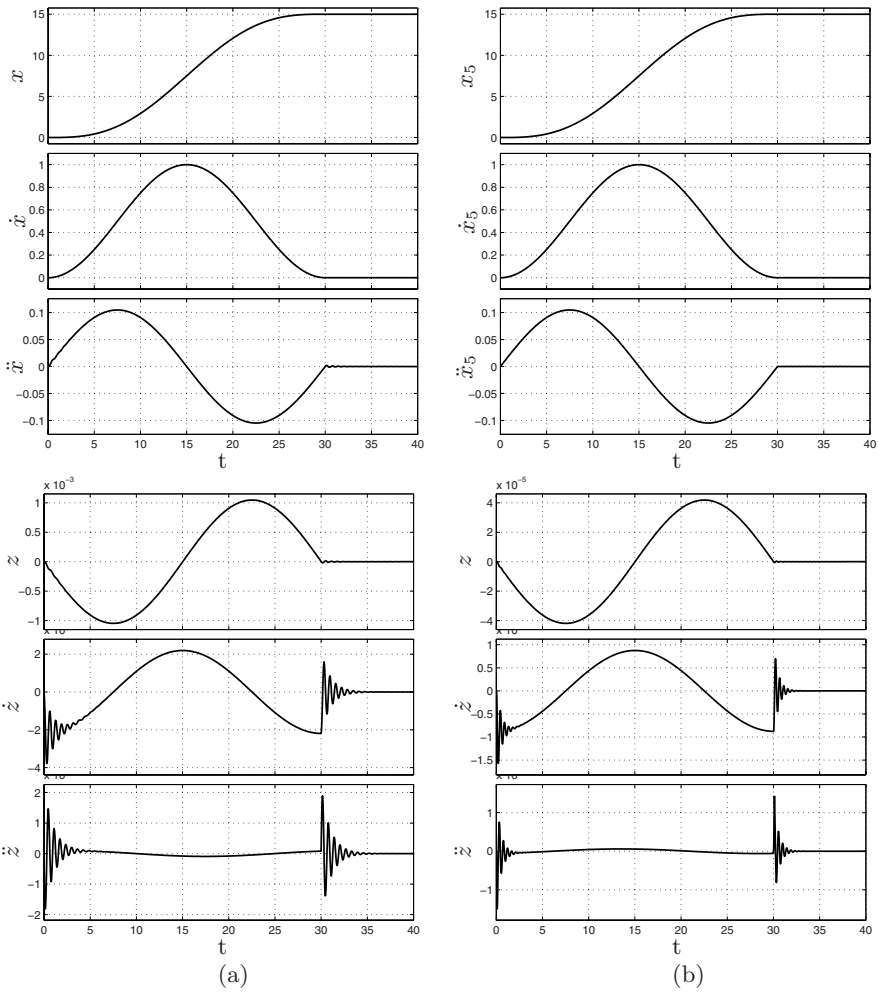
Fig. 7.8. Position, velocity, acceleration and errors ( z = x - q ) of mass m of the one degree of freedom system (a) and of the mass m_5 of the system with five degrees of freedom (b). In this latter case z = x_5 - q . The input q(t) is a cycloidal trajectory.
