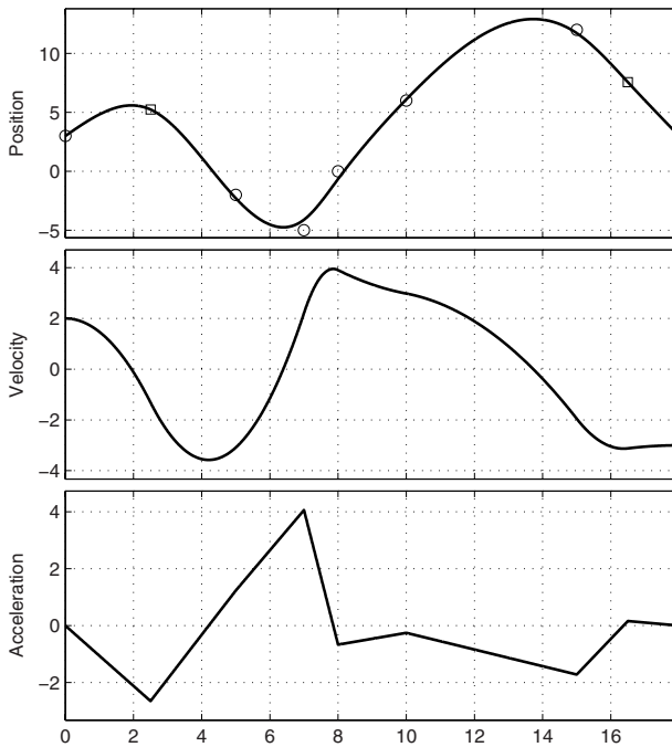
Fig. 4.12. Smoothing splines with assigned initial and final velocity/acceleration.
