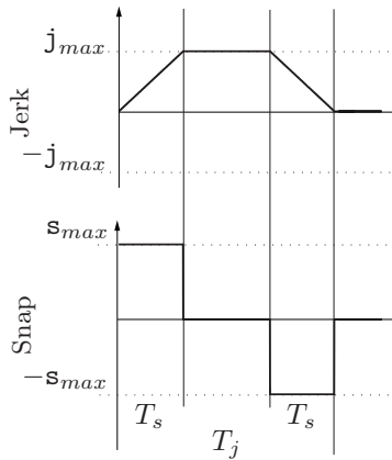
Fig. 3.30. Continuous jerk profile in a 15-segments “double S” trajectory.
