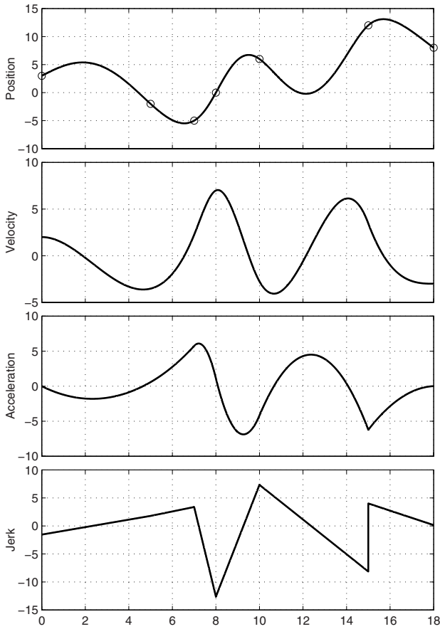
Fig. 4.20. B-spline trajectory of degree 4, with a double knot at 15.
