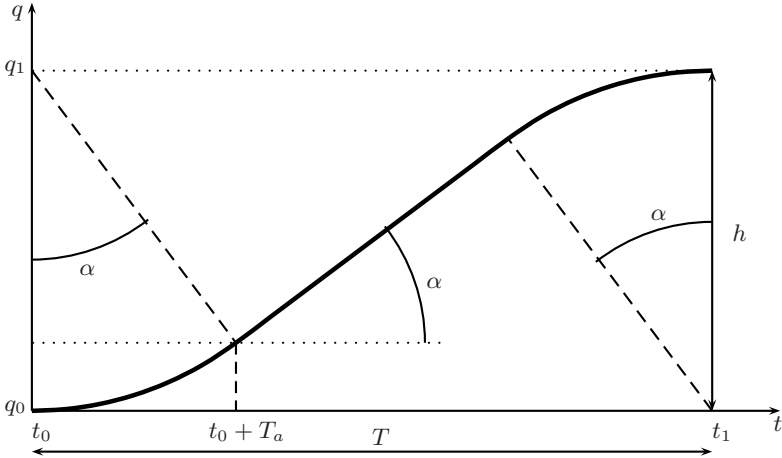
Fig. 3.1. Trajectory with constant velocity and circular blends.
