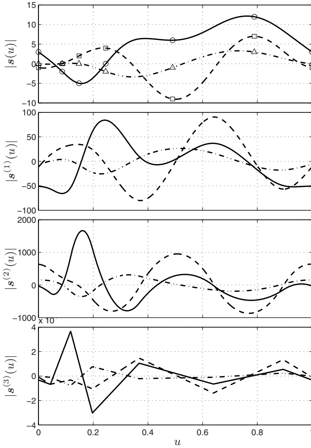
Fig. 8.28. Components of a B-spline trajectory of degree 4 computed with periodic conditions (component x - solid, component y - dashed, component z - dashdot).
