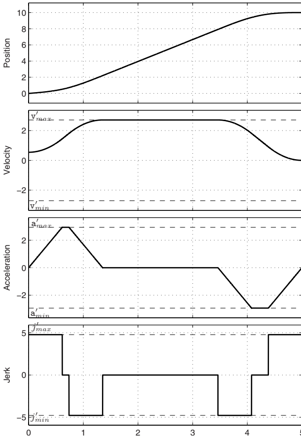
Fig. 3.26. Double S trajectory profiles (position, velocity, acceleration and jerk) properly scaled to impose a desired duration ( T_D = 5 s).
