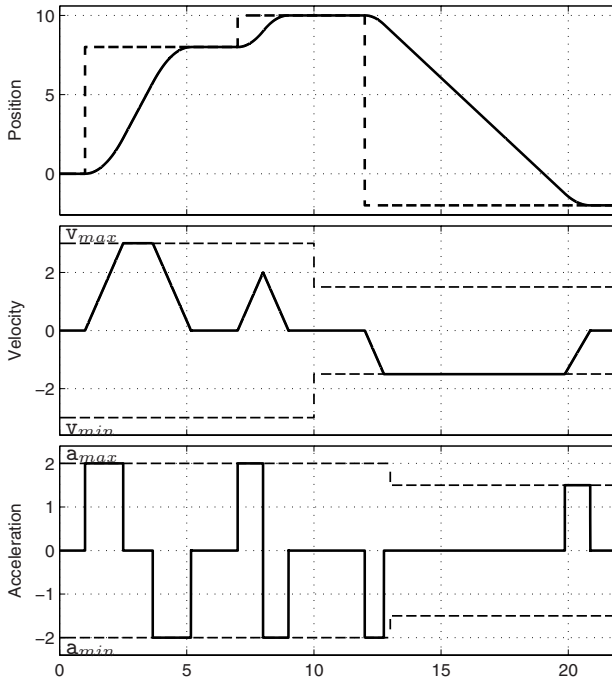
Fig. 4.34. Trajectory computed by means of the second order nonlinear filter when the constraints on velocity and acceleration are changed at runtime.
