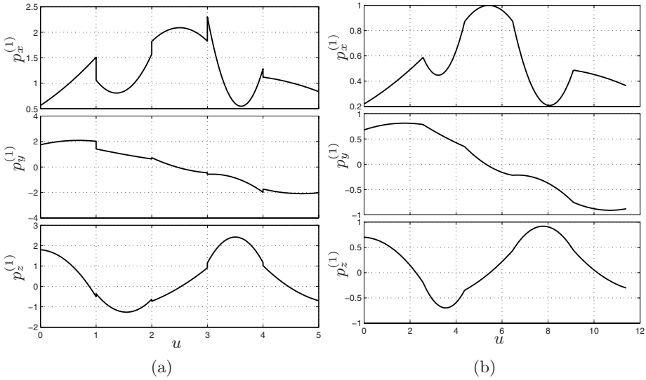
Fig. 8.4. Components along the x, y and z directions of the tangent vector \mathbf{p}^{(1)} of the 3D trajectory shown in Fig. 8.1, with two different parameterizations.
