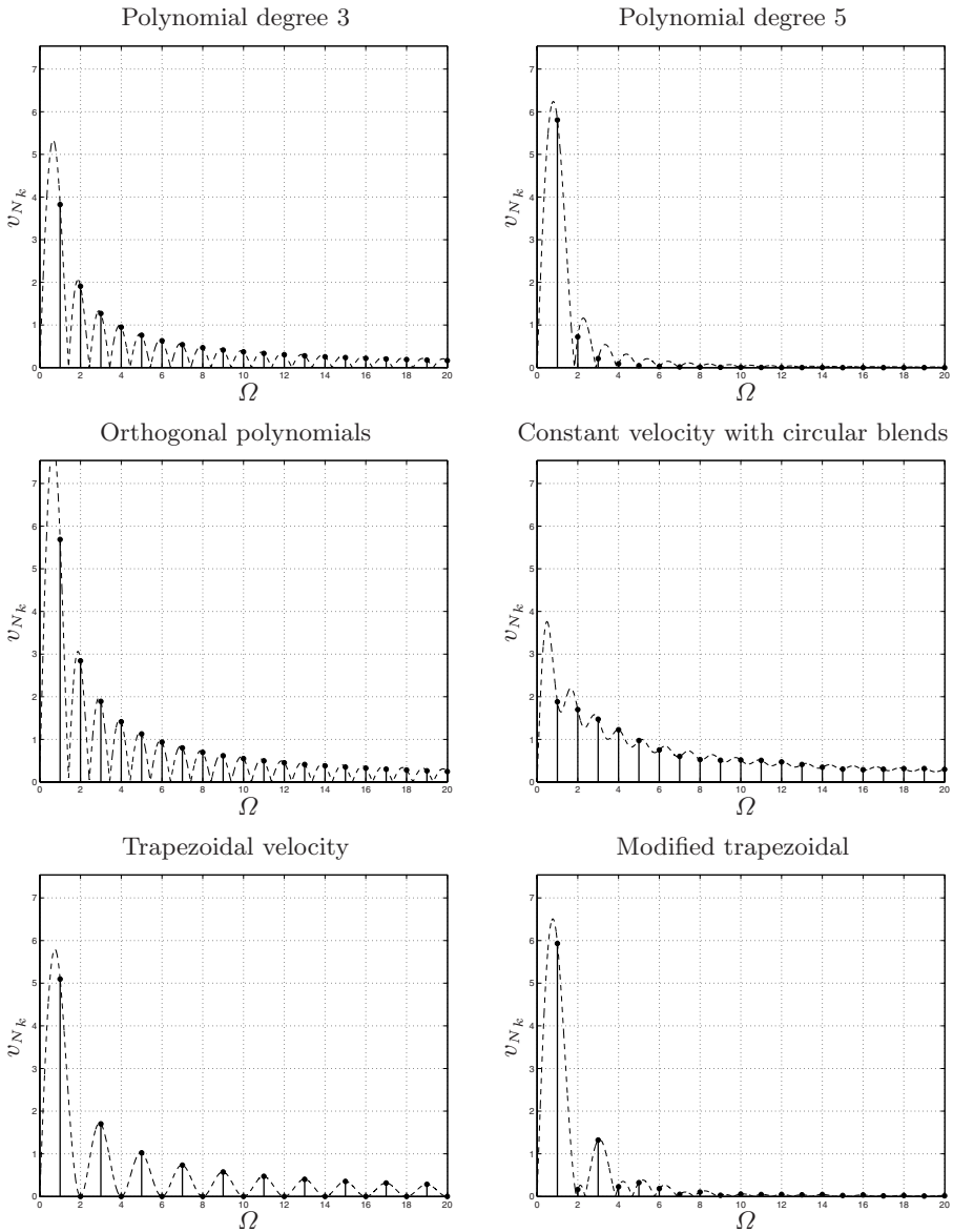
Fig. 7.30. Frequency analysis of the acceleration profiles of the periodic repetition of trajectories: polynomials with degree 3 and 5, orthogonal polynomials, constant velocity with circular blends, trapezoidal, modified trapezoidal.
