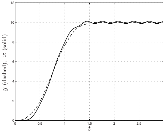
Fig. 7.56. Response of the system G(s) = 800 \frac{s+50}{(s^2+2s+100)(s^2+400)} to a double S trajectory with a ZVDD input shaper based on the first mode of the system.
