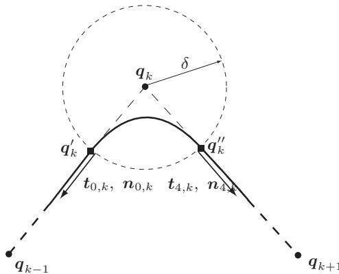
Fig. 8.42. Particular of a linear trajectory with a polynomial blend.
