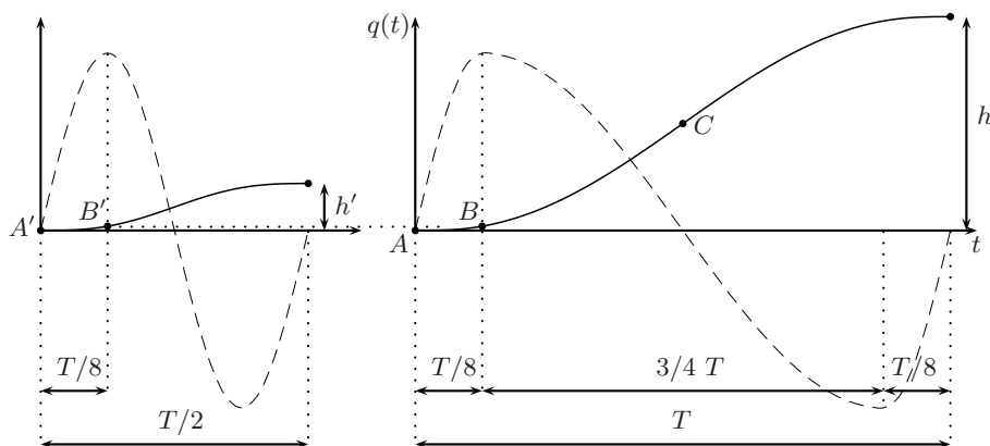
Fig. 3.37. Modified sinusoidal trajectory.
