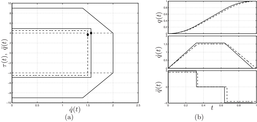
Fig. 6.12. Tasks obtained with a trapezoidal trajectory with \alpha = 1/3 for different values of the duration T (a) and plots of position, velocity, acceleration (b).
