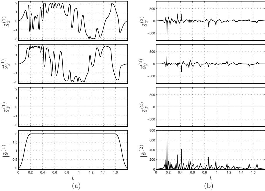
Fig. 9.33. Velocity and acceleration (components and magnitude) of the position trajectory represented by a smoothing B-spline approximating a set of data points, for \lambda = 10^{-8} .
