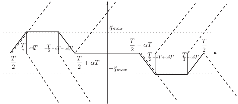
Fig. 7.22. Decomposition of the acceleration profile of the double S trajectory into elementary functions (ramp functions).
