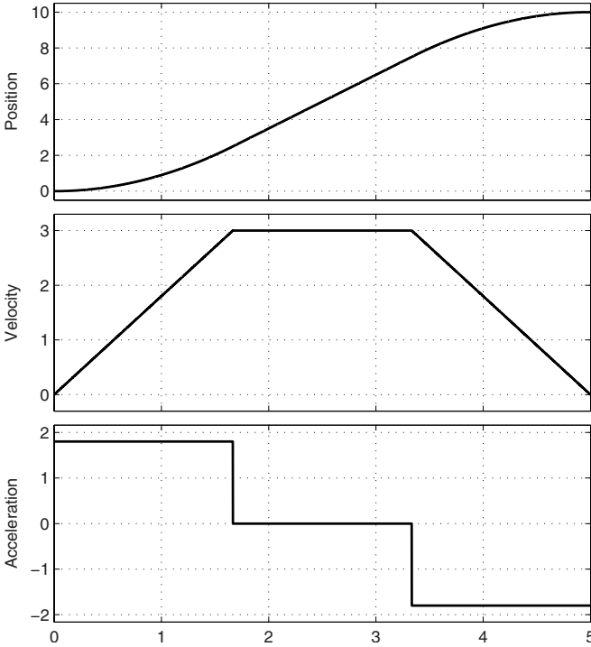
Fig. 3.6. Trapezoidal trajectory with prescribed duration T , and with T_a = T/3 .
