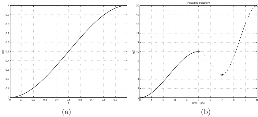
Fig. 5.6. Composition of 3-rd degree polynomial trajectories; normalized function q_N(\tau) (a), and overall trajectory obtained as union of the three segments (b).
