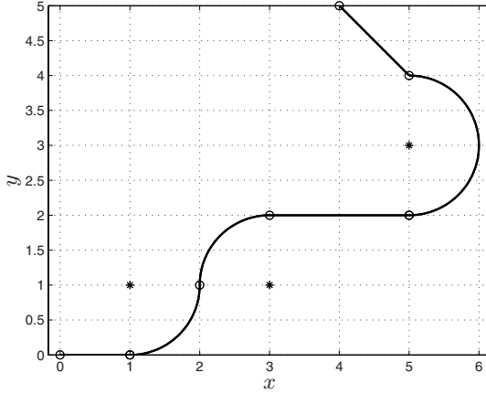
Fig. 8.16. Complex trajectory in the two-dimensional space obtained by composing linear and circular motion primitives.
