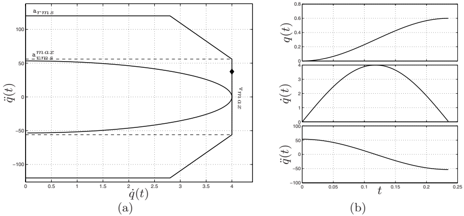
Fig. 6.9. Task obtained with a harmonic trajectory represented in a speed-acceleration diagram (a) and single plots of position, velocity, acceleration (b).
