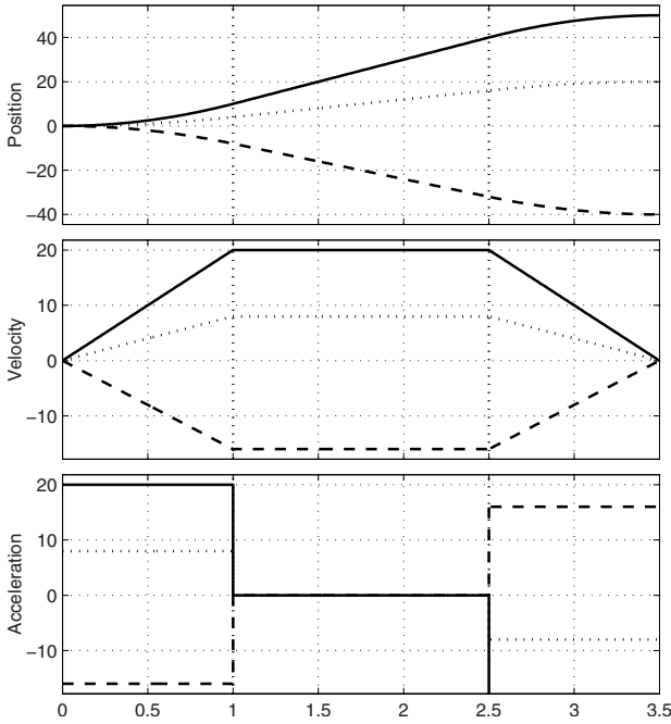
Fig. 3.4. Three synchronized trapezoidal trajectories.
