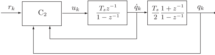
Fig. 4.31. Second order filter for online optimal trajectory generation.
