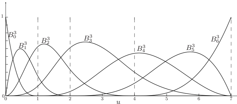
Fig. B.2. Cubic basis functions defined on \mathbf{u} = [0, 0, 0, 0, 1, 2, 4, 7, 7, 7, 7] .
