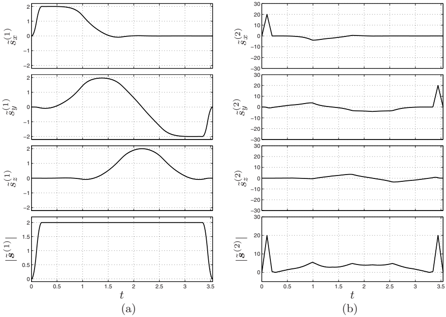
Fig. 9.35. Velocity and acceleration (components and magnitude) of a B-spline curve approximating a trajectory based on motion primitives, with a double S feed rate profile.
