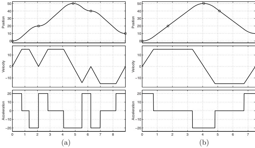
Fig. 3.9. Position, velocity and acceleration of a trapezoidal trajectory through a sequence of points with null (a) and non-null (b) intermediate velocities.
