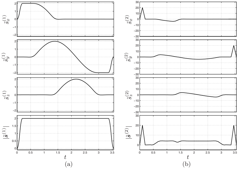
Fig. 9.37. Velocity and acceleration (components and magnitude) of a B-spline curve approximating a trajectory based on motion primitives, with a double S feed rate profile.
