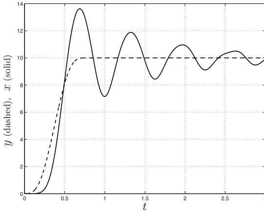
Fig. 7.55. Output of the system G(s) = 800 \frac{s+50}{(s^2+2s+100)(s^2+400)} when a double S trajectory is applied, without input shaper.
