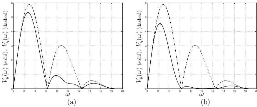
Fig. 7.50. Spectrum of \ddot{y}(t) (solid) obtained by shaping the trajectory q(t) , compared with the spectrum of \ddot{q}(t) (dashed): ZV shaper (a), ZVDD shaper (b).
