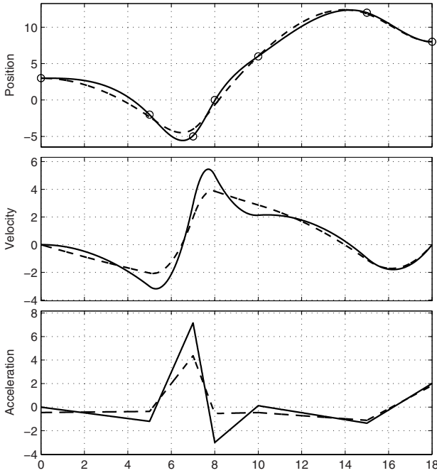
Fig. 4.14. Smoothing splines computed with a approximation error of 0.1 (solid) and 1 (dashed).
