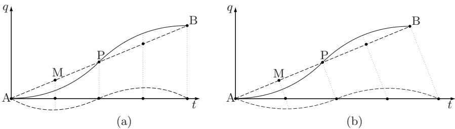
Fig. 3.39. Geometrical construction of the cycloidal (a) and modified cycloidal trajectory with the Alt method (b).
