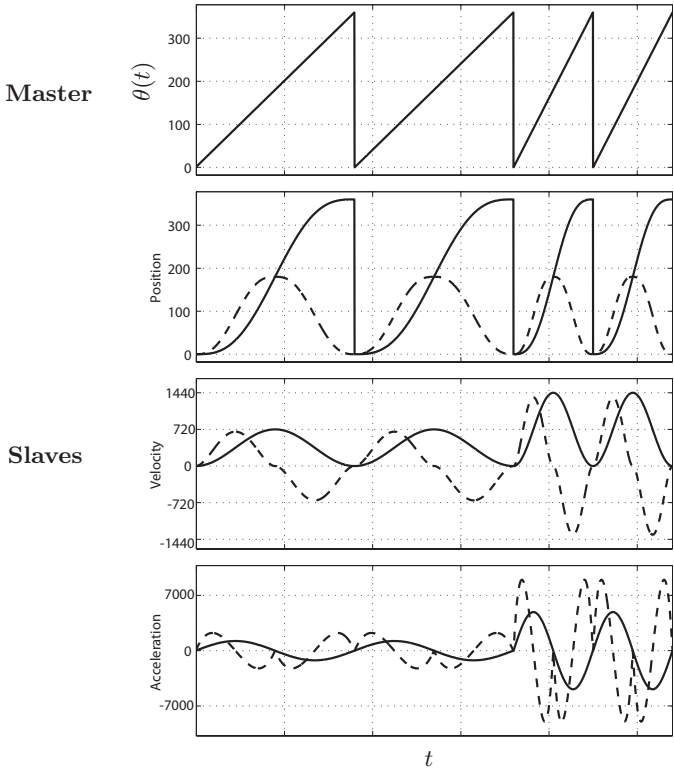
Fig. 5.16. Synchronization of two electronic cams with different profiles: cycloidal (solid) and polynomial of degree 5 (dashed).
