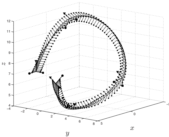
Fig. 8.10. Trajectory for position and orientation based on axis-angle representation.
