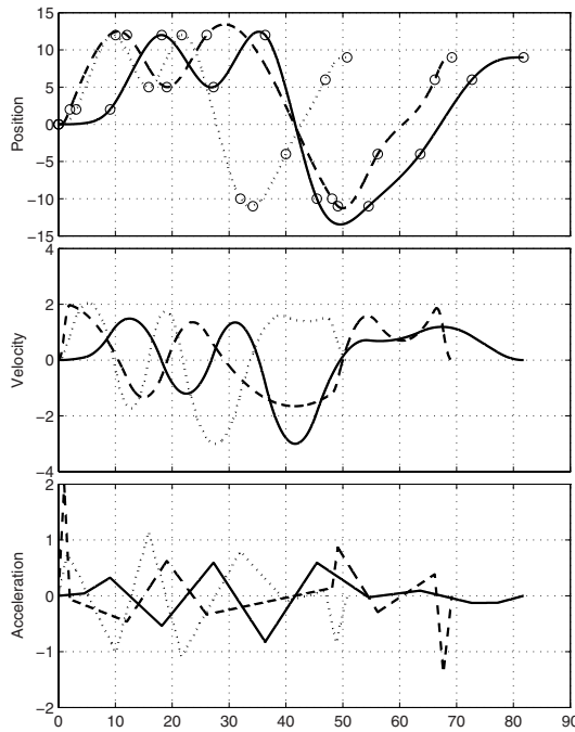
Fig. 4.16. Spline trajectories interpolating a set of data points, with different distributions of time instants, and properly scaled to be compliant with the constraints on the velocity and acceleration: uniformly spaced (solid), cord length (dashed), centripetal (dotted).
