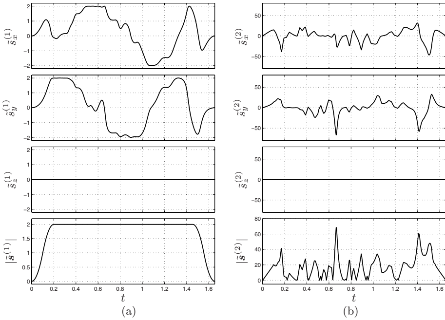
Fig. 9.31. Velocity and acceleration (components and magnitude) of the position trajectory represented by a smoothing B-spline approximating a set of data points, for \lambda = 10^{-6} .
