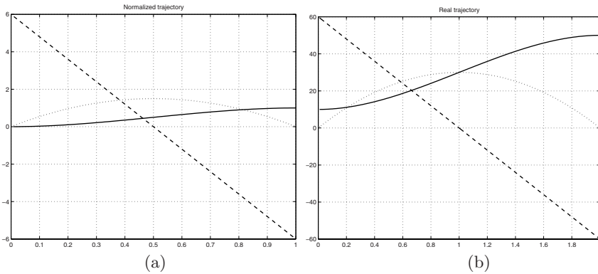
Fig. 5.7. Profiles of acceleration (dashed), velocity (dotted) and position (solid) a polynomial trajectory of degree 3: normalized form (a) and with conditions q_0 = 10 , q_1 = 50 , t_0 = 0 , t_1 = 2 (b).
