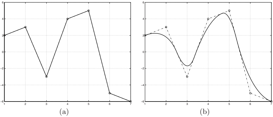
Fig. B.7. B-spline curves of degree 1 (a) and 2 (b) computed with the same control points.
