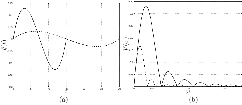
Fig. 7.32. (a) Acceleration profiles of a polynomial trajectory of degree 5 (solid) and of the same function scaled in time, with \lambda = 0.5 (dashed). (b) Frequency content of the same signals.
