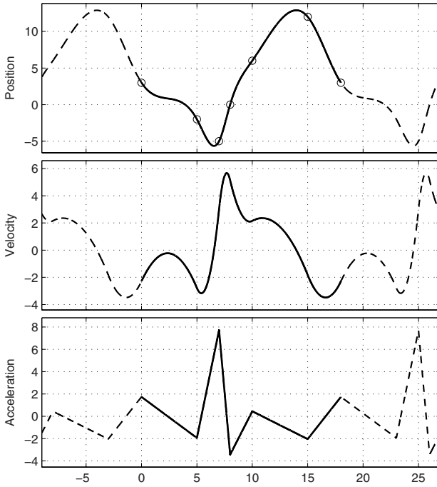
Fig. 4.8. Spline trajectory for periodic motions.
