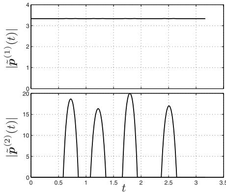
Fig. 9.2. Magnitude of velocity and acceleration of the trajectory composed by straight line segments and 5-th degree Bézier curves.
