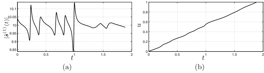
Fig. 9.8. Feed rate of the trajectory defined with a cubic B-spline, with u computed by means of (9.9a) (a), and relation between t and u (b).
