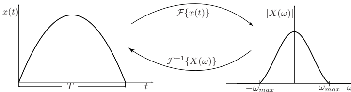
Fig. D.1. Fourier transform of a bandlimited (and finite length) signal x(t) .
