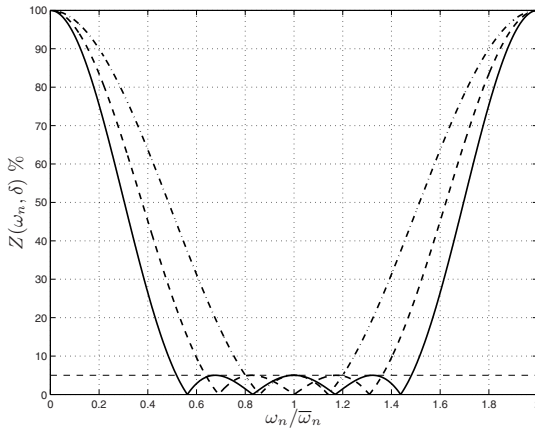
Fig. 7.52. Sensitivity curves of one-hump (dashdot), two-hump (dashed) and three-hump (solid) EI shapers, obtained for \delta = 0 .
