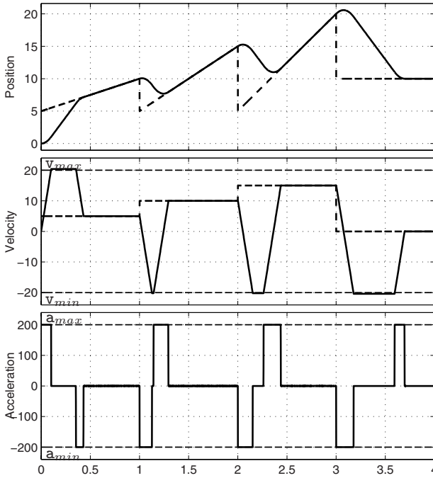
Fig. 4.33. Output (position, velocity and acceleration) of the second order nonlinear filter with a “sawtooth” reference signal.
