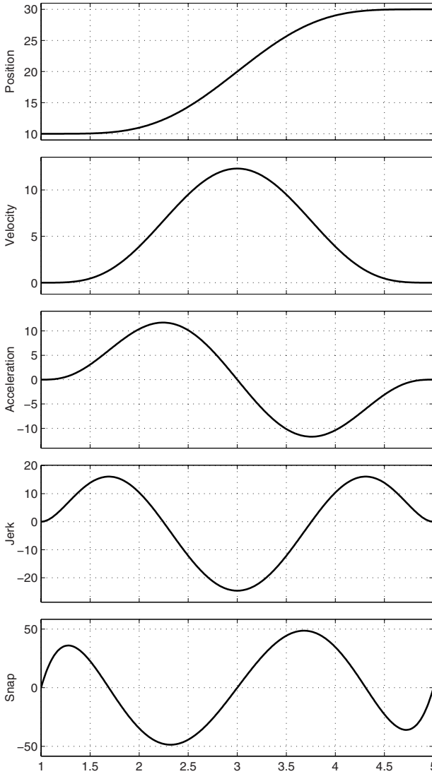
Fig. 2.15. Polynomial function of degree 9 of Example 2.13.
