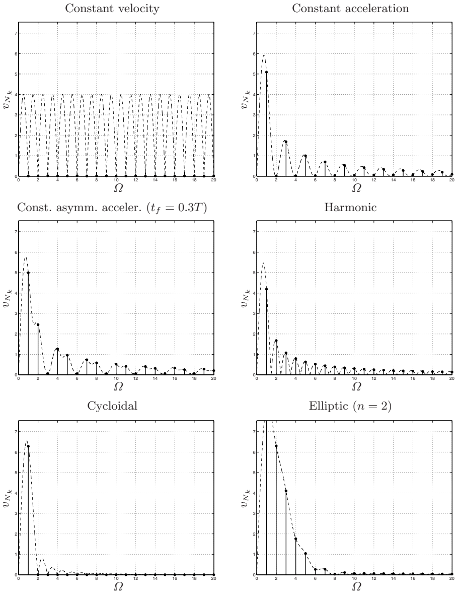
Fig. 7.29. Frequency analysis of the acceleration profiles of the periodic repetition of trajectories: constant velocity, constant acceleration, asymmetric constant acceleration, harmonic, cycloidal and elliptic.
