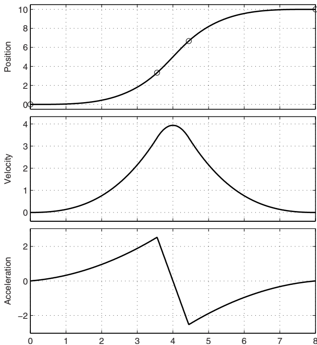
Fig. 3.33. Position, velocity and acceleration profiles for a ‘4-3-4’ trajectory; the circles in the position diagram refer to the inner points (t_a, q_a) , (t_b, q_b) .
