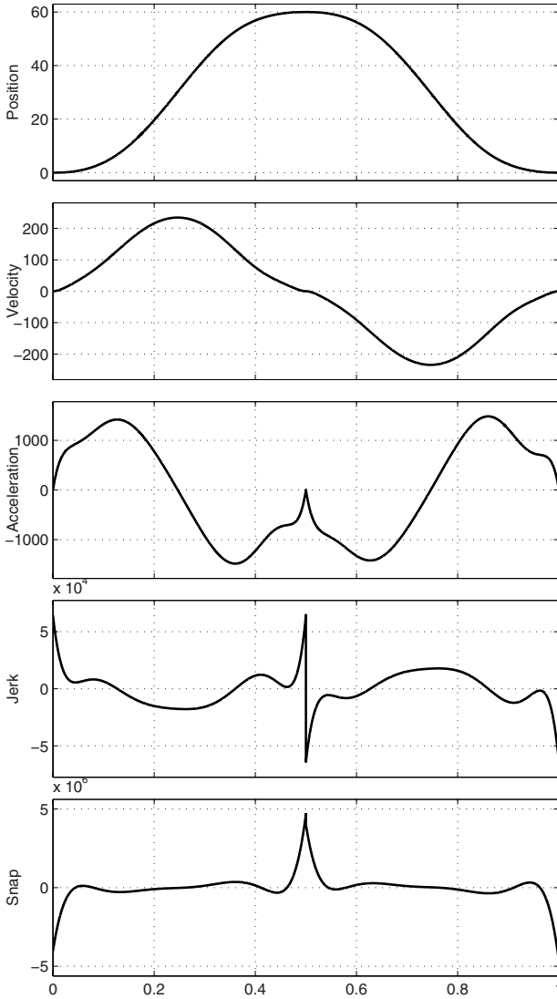
Fig. 7.38. Position, velocity, acceleration, jerk and snap for the Peisekah polydyne trajectory q(t) .
