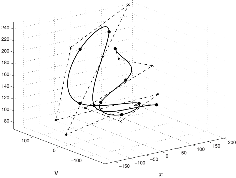
Fig. 8.18. Three dimensional global interpolation by a cubic B-spline (solid) and related control polygon (dashed).
