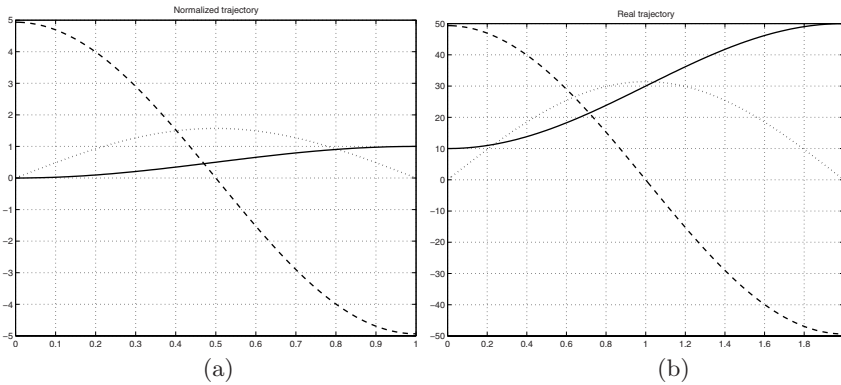
Fig. 5.11. Profiles of acceleration (dashed), velocity (dotted) and position (solid) of an harmonic motion: normalized form (a) and with boundary conditions q_0 = 10 , q_1 = 50 , t_0 = 0 , t_1 = 2 , (b).
