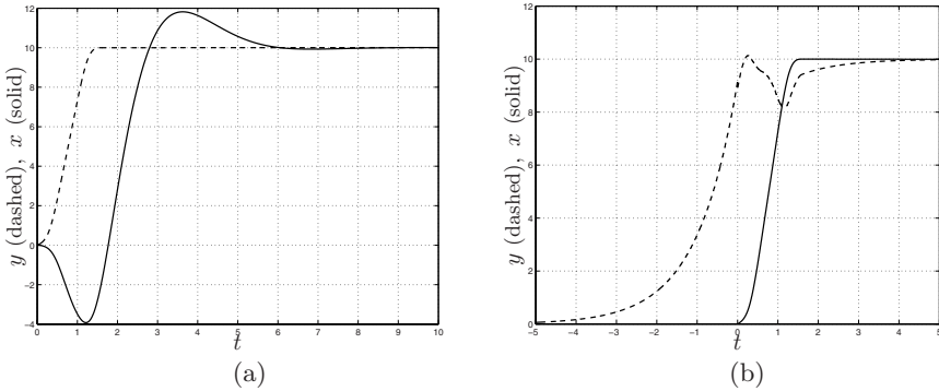
Fig. 7.66. Input and output signals of the system G(s) = 4 \frac{(1-s)(s+1)}{(s+2)(s^2+2s+2)} without (a) and with (b) model inversion.
