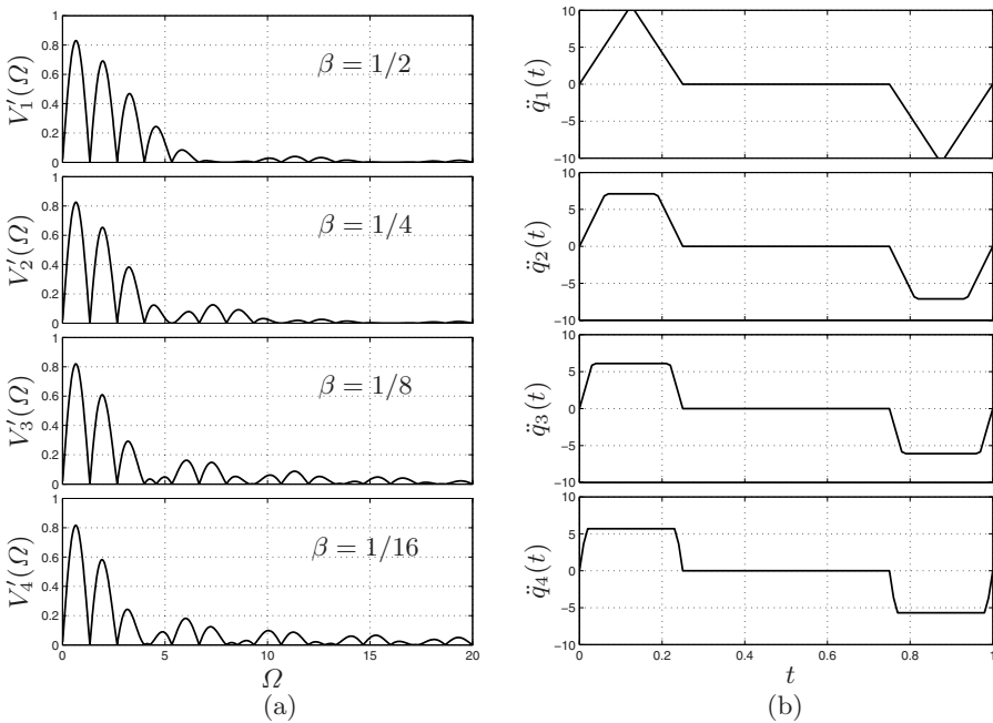
Fig. 7.23. Harmonic content (a) and related acceleration profiles (b) of double S trajectories for different values of the parameter \beta ( \alpha is constant and equal to 1/4 ).
