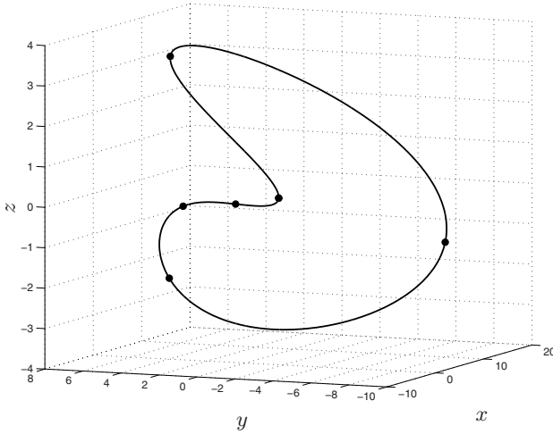
Fig. 8.27. B-spline curve of degree 4 computed with periodic conditions.
