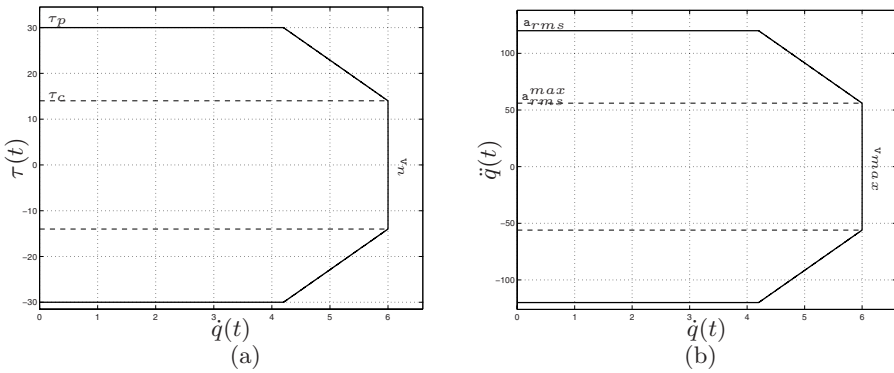
Fig. 6.7. Speed-torque and speed-acceleration diagrams for a given mechanical/actuation system.
