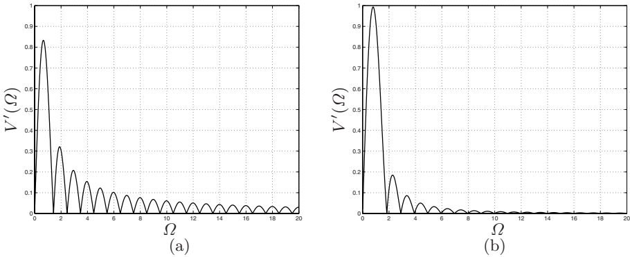
Fig. 7.24. Harmonic content of the 3-rd degree (a) and 5-th degree (b) polynomial trajectories.
