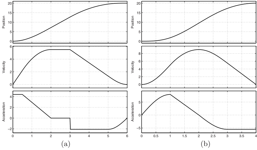
Fig. 3.55. Composition of elementary trajectories: parabolic-cubic-constant-cycloidal (a); cycloidal-cubic-cycloidal-parabolic (b).
