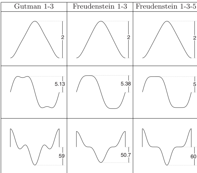
Fig. 6.6. From the top, velocity, acceleration and jerk profiles for the trajectories: Gutman 1-3, Freudenstein 1-3, Freudenstein 1-3-5.
