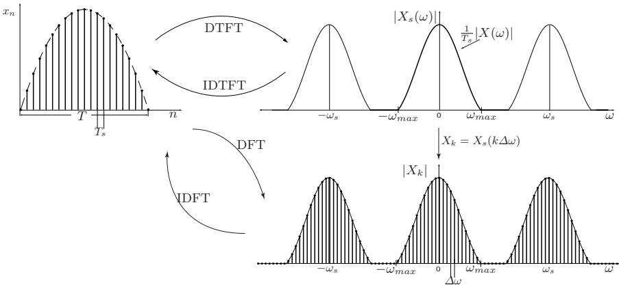
Fig. D.3. Discrete time Fourier transform and discrete Fourier transform of a sequence x_n .
