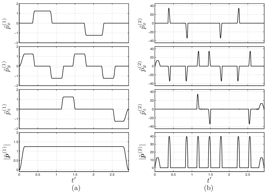
Fig. 9.20. Velocity and acceleration (components and magnitude) of a trajectory composed by linear and 5-th degree Bézier segments, properly scaled in time in order to have a maximum acceleration of 40.
