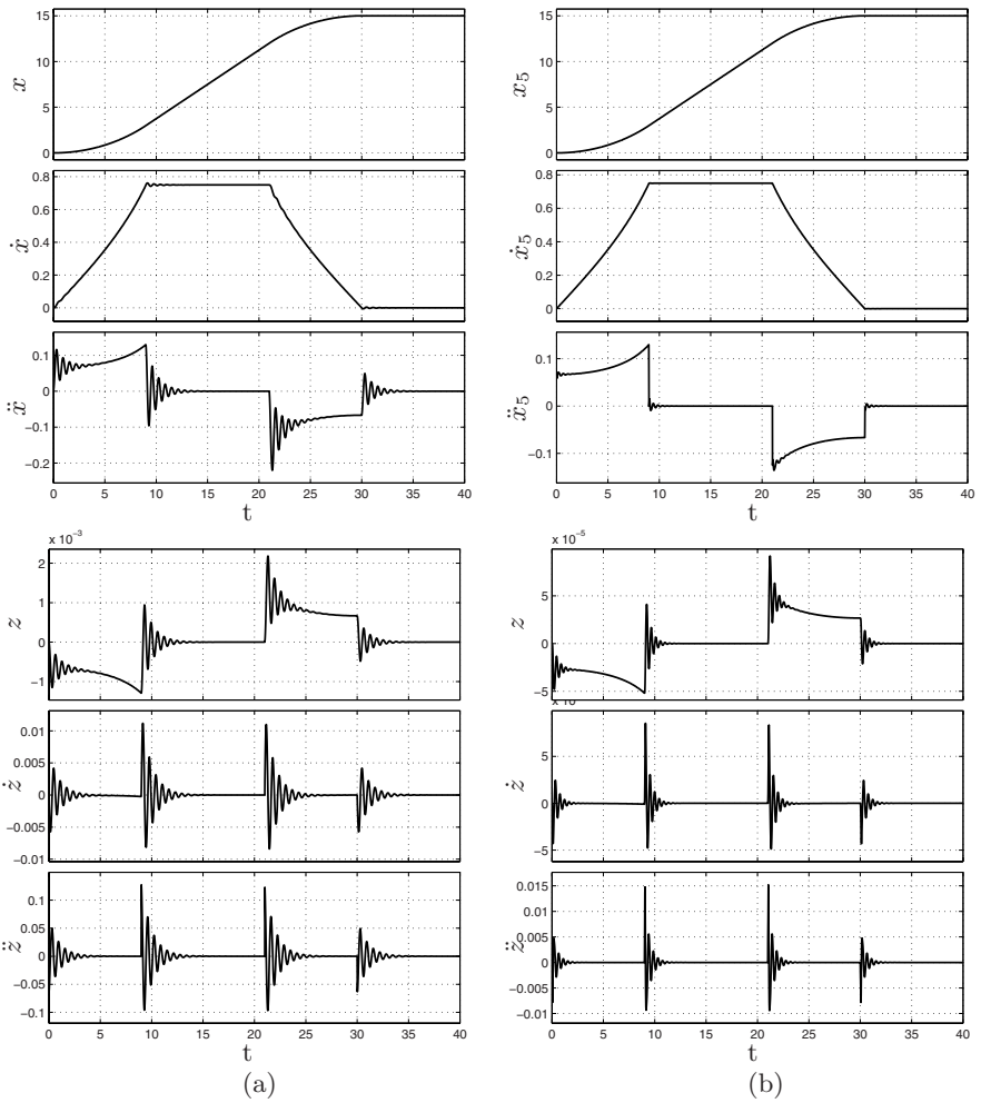
Fig. 7.12. Position, velocity, acceleration and errors ( z = x - q ) of mass m of the one degree of freedom system (a) and of the mass m_5 of the system with five degrees of freedom (b). In this latter case z = x_5 - q . The input q(t) is a linear trajectory with circular blends.
