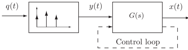
Fig. 7.44. Block diagram of a system with a shaper.
