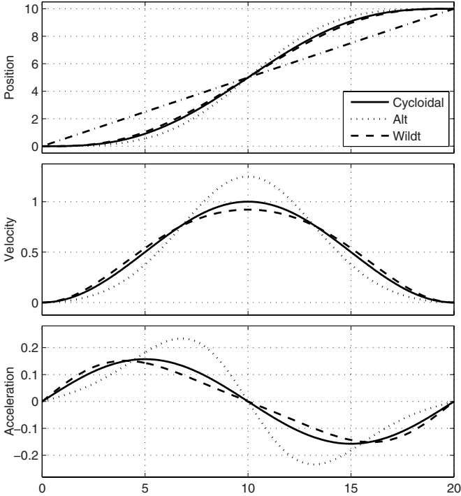
Fig. 3.41. Cycloidal and modified cycloidal trajectories (position, velocity, acceleration).
