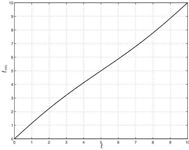
Fig. 3.43. Relation between t and t_m for the modified cycloidal trajectory of Fig. 3.42.
