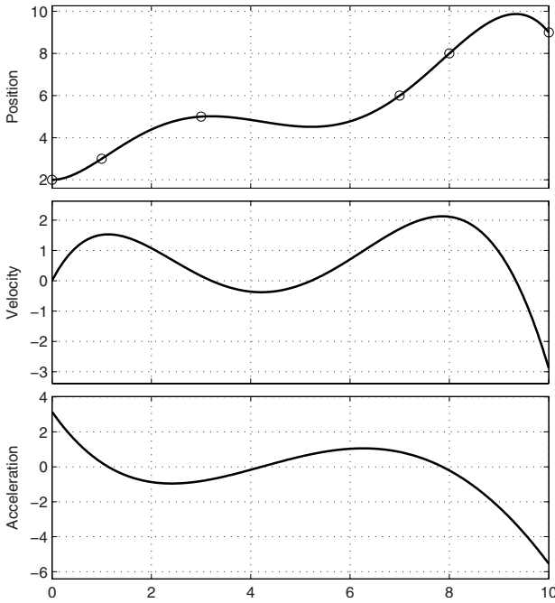
Fig. 4.3. Position, velocity and acceleration of an orthogonal polynomials trajectory ( m = 4 ) with null initial velocity.
