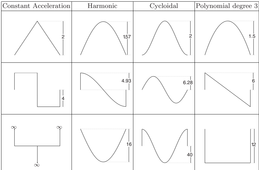
Fig. 6.4. From the top, velocity, acceleration and jerk profiles for the trajectories: with constant acceleration, harmonic, cycloidal, 3-rd degree polynomial.
