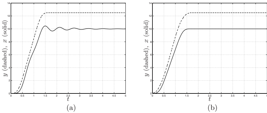
Fig. 7.62. Input and output signals of the system G(s) = \frac{80}{s^2+2s+100} without (a) and with (b) model inversion; q(t) is a double S trajectory.
