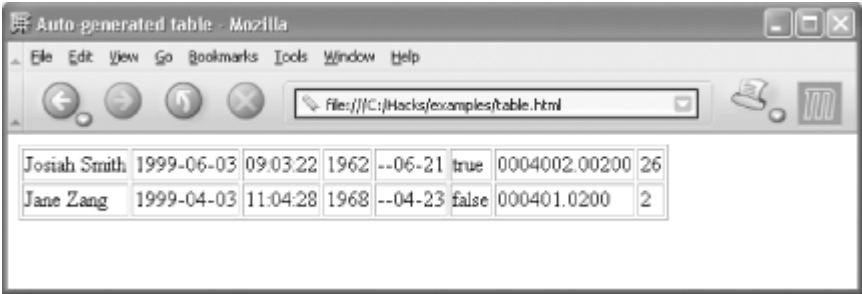
Figure 3-15. A table created with generic XSLT, viewed in Mozilla
