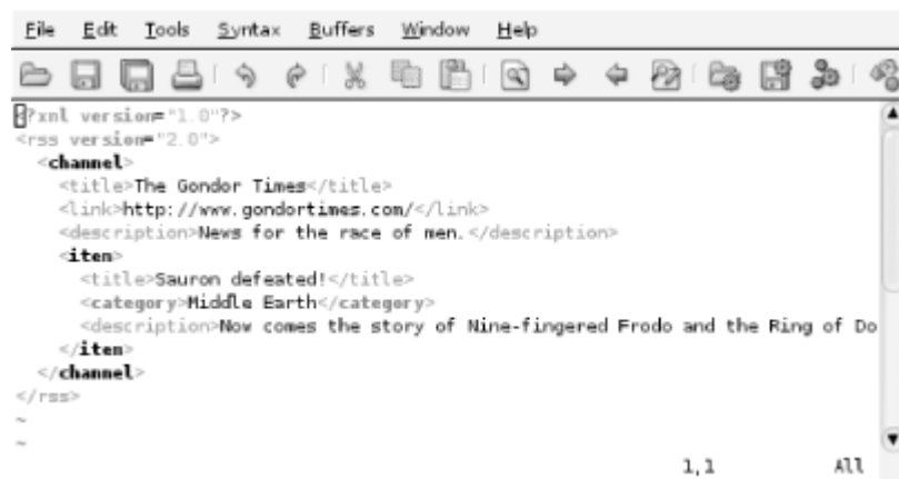
Figure 2-5. frodo.rss in gVim
