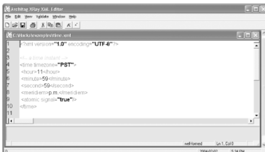
Figure 3-4. time.xml in xRay2
