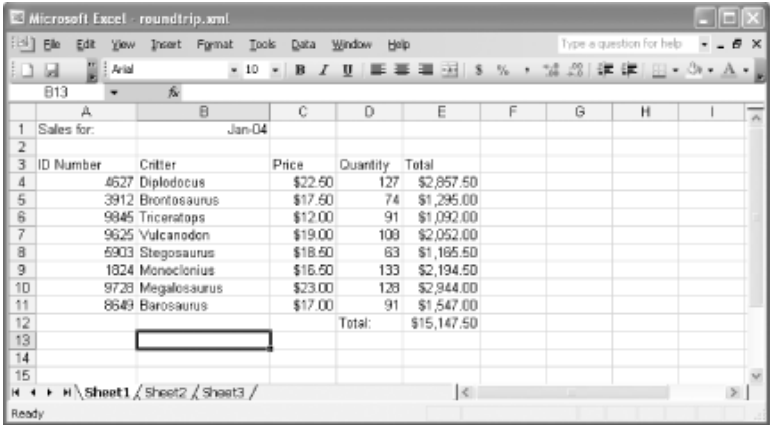
Figure 3-21. The test spreadsheet after its data has gone from SpreadsheetML to another vocabulary and back again
