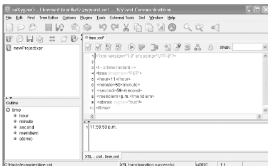
Figure 3-9. Result of transforming time.xml with clock.xsl in <oXygen />
