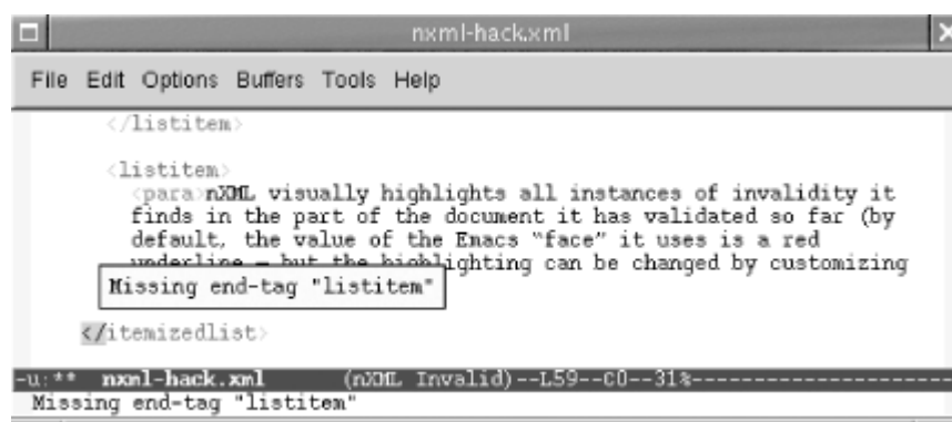
Figure 2-2. nXML validation error message
