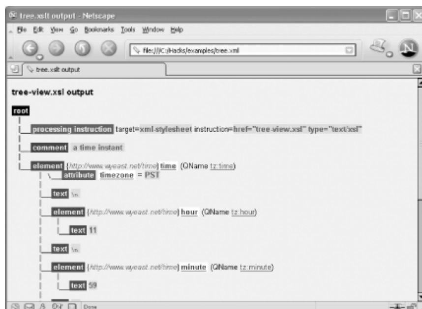
Figure 3-11. tree.xml transformed by tree-view.xsl and styled by tree-view.css
