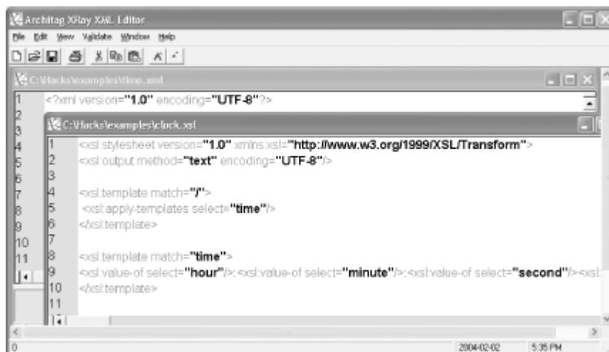
Figure 3-5. clock.xsl in xRay2
