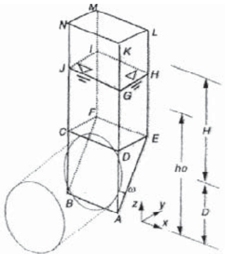
Figure ap.4.10 The tunnel-face stability model of the method of Anagnostou & Kovari.
