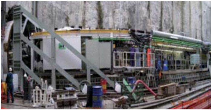
Figure ap.7.11.5 The TBM back-up.
