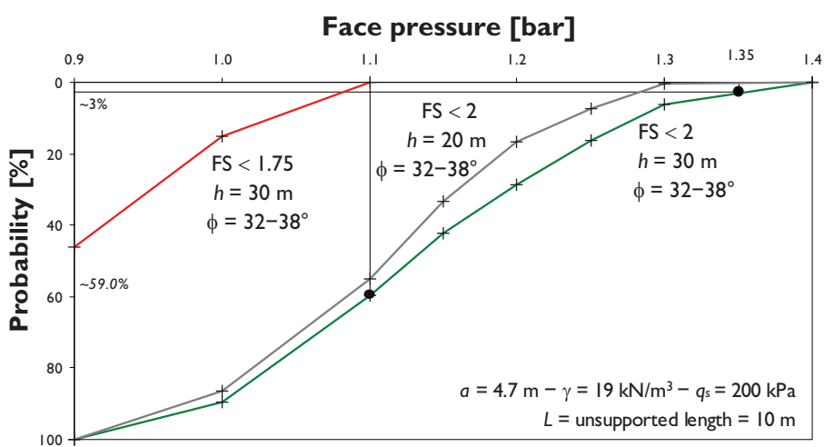
Figure 5.27 Face-support pressure and FS probability.
