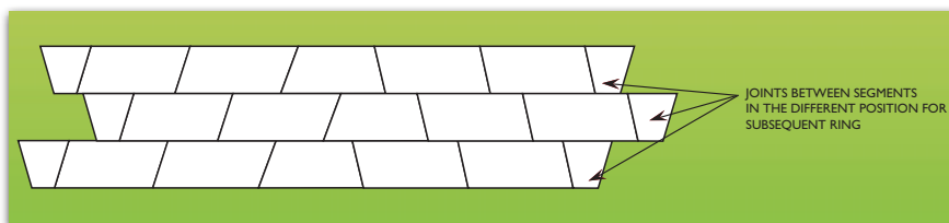
Figure 5.61 Allowed sequence of rings (unfolded view).
