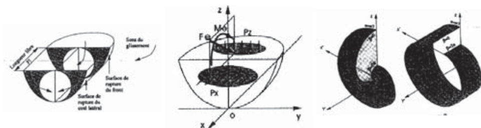
Figure ap.4.7 The failure mechanism assumed for the method of Mohkam et al.
