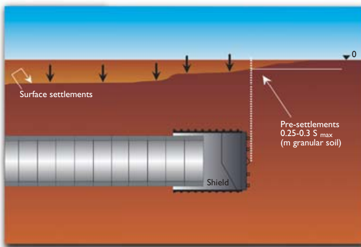
Figure 5.6 Development of longitudinal settlements in mechanized tunneling.
