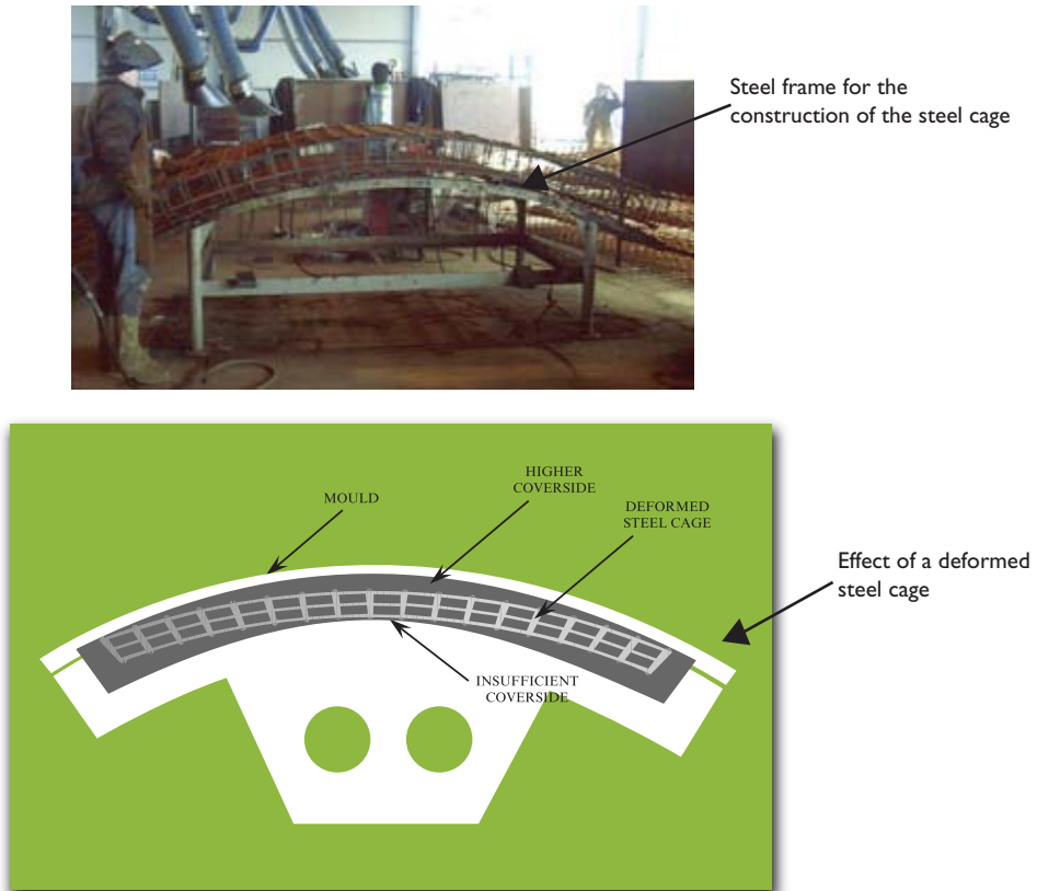
Figure 5.77 Variation in the cover-side due to imperfect geometry of the steel cage.
