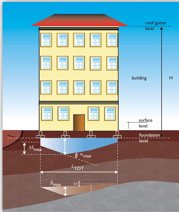
Figure 5.8 “Control parameters” that regulate the behaviour of a building towards settlements. (Burland et al. , 1977). Key: S_{\max} : maximum vertical settlement, \Delta S_{\max} : Maximum differential or relative settlement, \alpha_{\max} : Maximum angular strain (sagging when positive; hogging when negative), \beta_{\max} : maximum angular distortion, \omega : Tilt (rigid body rotation of the whole superstructure or a well-defined part of it), \Delta_{\max} : maximum relative deflection (max. displacement relative to the straight line connecting two reference points with a distance L ).
