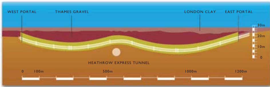
Figure 3.5 The Road Tunnel in Heathrow: elevation variation foreseen to pass over the Heathrow Express Tunnel.
