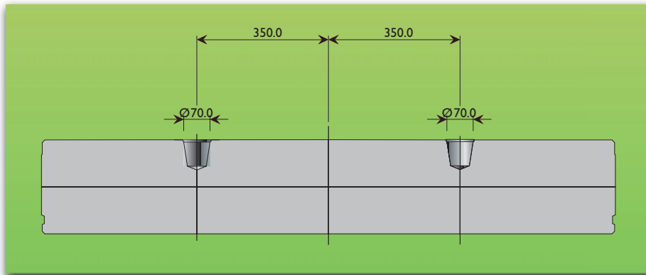
Figure 5.45 Conical insert for the vacuum system.
