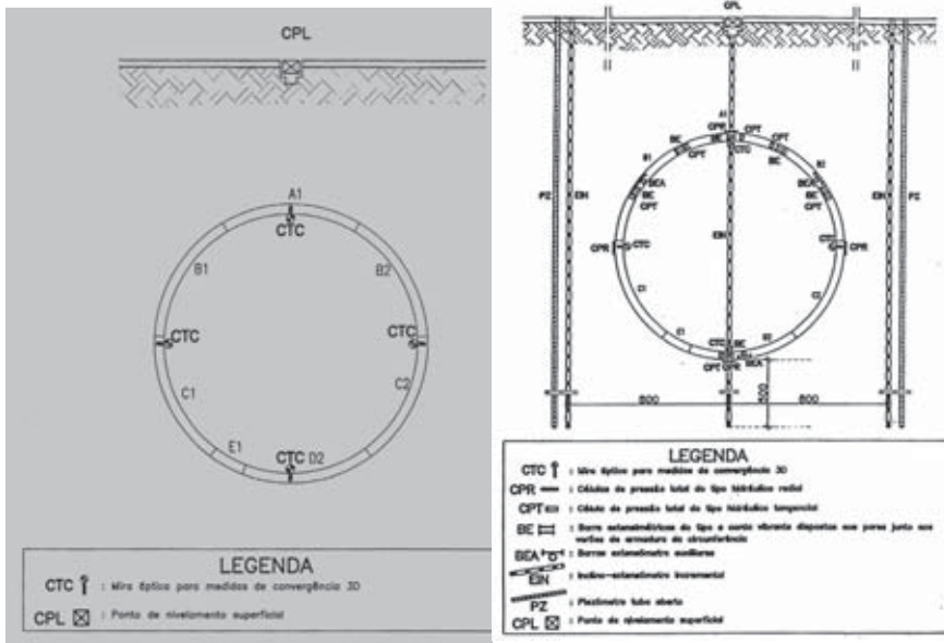
Figure 5.80 Current and special monitoring section.
