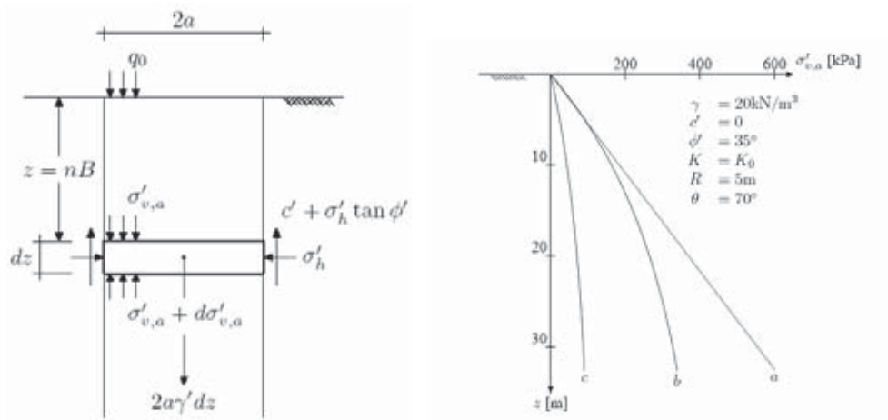
Figure ap.4.13 Definition of forces acting on a strip of soil in an arching soil column according to the Terzaghi theory (Broere, 2001).
