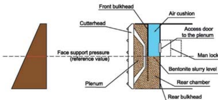
Figure 6.4 Schematic representation of a Hydroschild.
