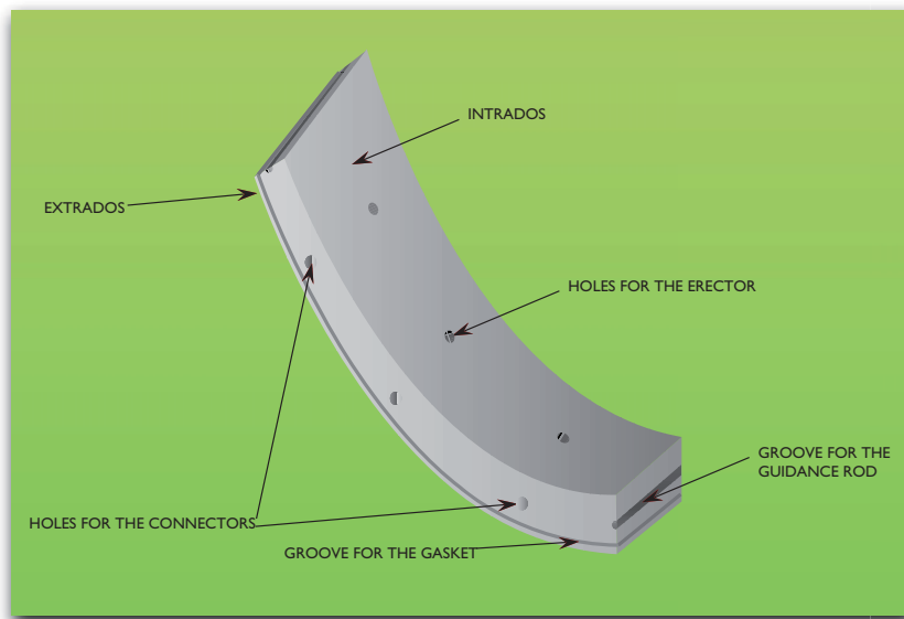
Figure 5.41 3D view of a complete single segment.
