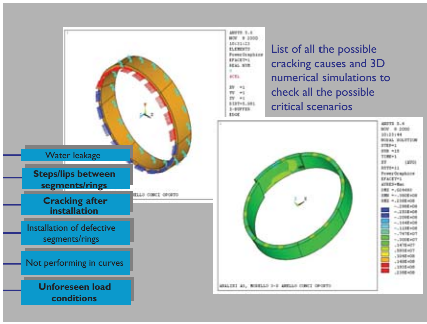
Figure 2.14 Design of tunnel lining in response to risks: measures for reducing the risk of critical scenarios leading to anomalous load conditions, cracking and defects.
