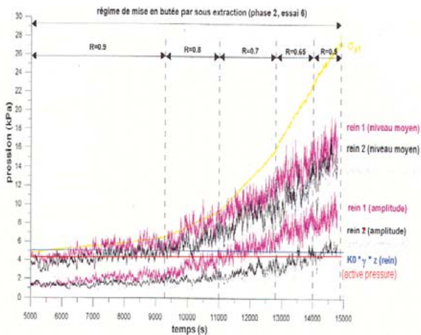
Figure 5.22 Régime of under-extraction ( R < 1 ).
