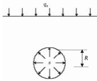
Figure ap.4.4 The tunnel-face stability model of the method of Atkinson & Potts.
