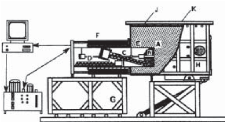
Figure 5.19 EPBS model used in laboratory tests (AFTES, 2001).
