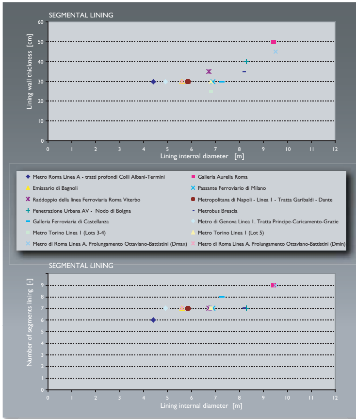
Figure 5.58 Relation between internal diameter and (a) lining thickness, (b) number of segments.
