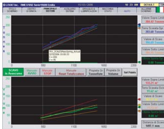
Figure 6.23c Example of the use of screw conveyor for controlling the material extraction.
