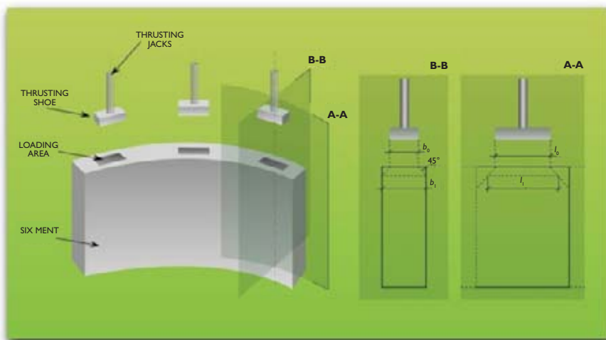
Figure 5.65 Geometrical definition of a single segment under the thrust of the TBM.
