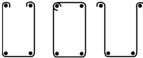
FIGURE 8.49 Typical web steel (stirrups) to resist diagonal tension associated with shear stress in beams
