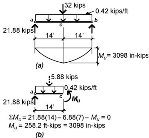
FIGURE 8.37 To find maximum moment for Example 8.8, draw (a) loading and moment diagram and (b) free-body diagram cut at midpoint with equation of moment equilibrium
