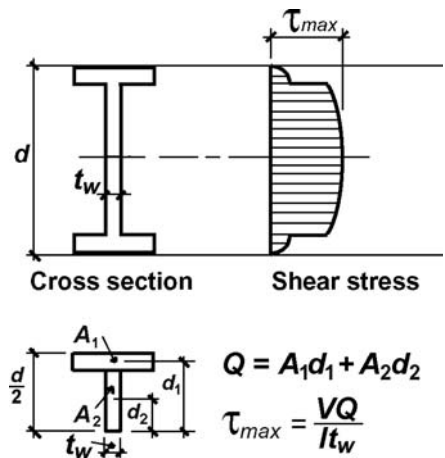
FIGURE 8.12 Distribution of shear stress on a flanged cross section, and calculation of maximum shear stress, \tau_{max}
