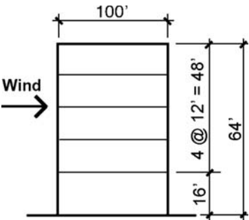
FIGURE 2.14 Schematic section through building for Example 2.4
