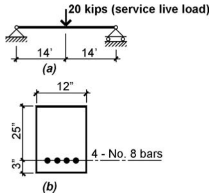
FIGURE 8.36 Reinforced concrete beam showing (a) loading diagram and (b) cross section through beam for Example 8.8
