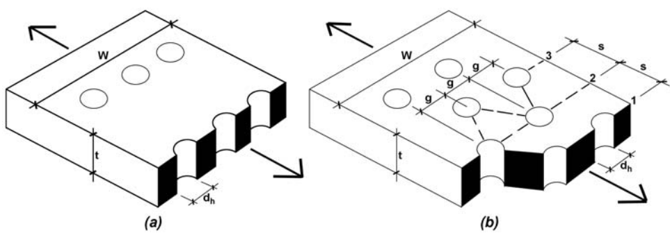
FIGURE 6.2 Net area of a cross section, shown in darker tone, with (a) one possible failure surface when bolt holes are arrayed in orthogonal grid and (b) multiple possible failure surfaces when bolt holes are staggered
