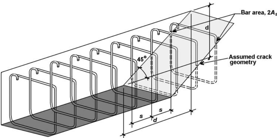
FIGURE 8.50 Assumed crack geometry for calculation of web steel capacity to resist shear forces (at diagonal tension cracks)
