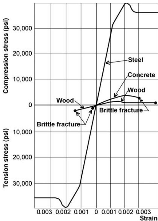
FIGURE 3.1 Stress–strain curves for structural materials
