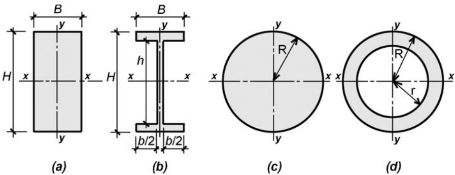
FIGURE 1.48 Cross sections typically encountered as structural elements include (a) rectangles, (b) I-shaped sections, (c) circles, and (d) circular rings
