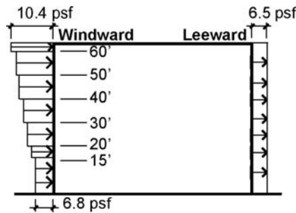
FIGURE 2.15 Distribution of wind pressure on windward and leeward surfaces for Example 2.4
