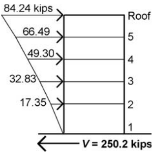
FIGURE 2.18 Distribution of story forces, F_x , for Example 2.5
