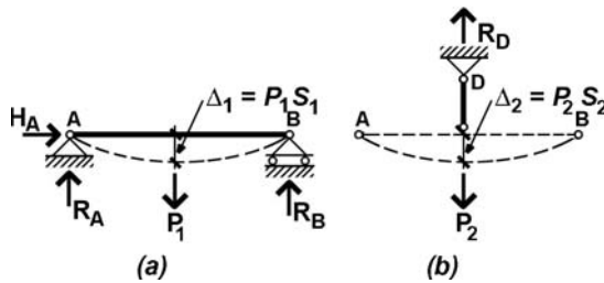
FIGURE 1.47 Deflection diagrams for the two components of the structure shown in Figure 1.46: (a) a simply supported beam with a concentrated load, P_1 , and (b) a tension hanger with load P_2
