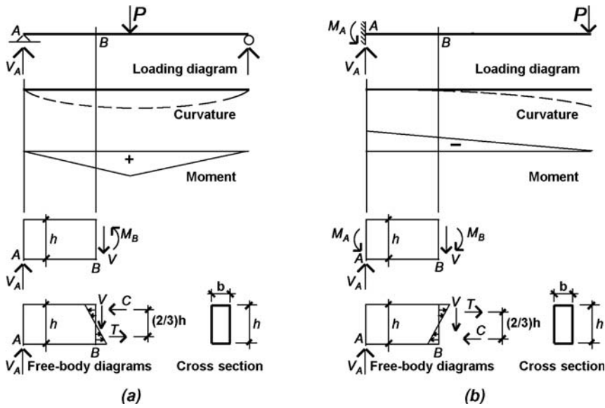
FIGURE 8.4 Comparison of “positive” and “negative” bending in (a) a simply supported beam and (b) a cantilevered beam
