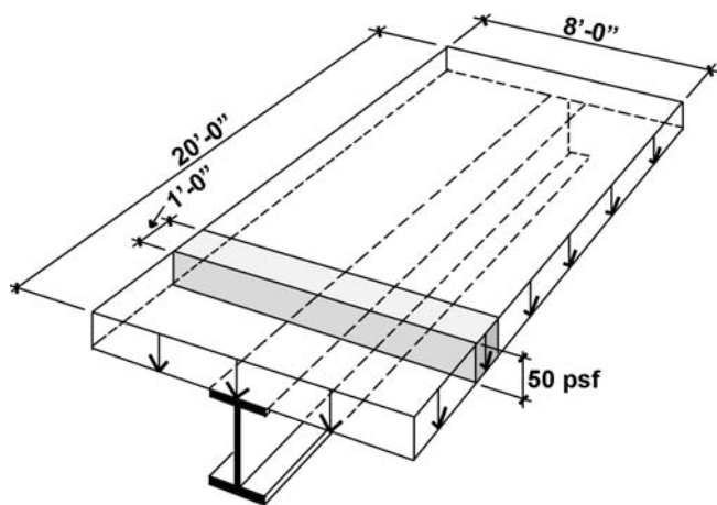
FIGURE 2.7 Tributary area for live load on one linear foot of beam for Example 2.2, with shaded “stress block” volume of 50 \times 8 \times 1 = 400\text{lb/ft} being the unreduced live load on one linear foot of the beam
