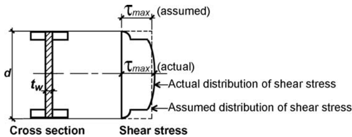
FIGURE 8.13 Comparison of actual and assumed maximum shear stress, \tau_{max} , for a steel wide-flange beam
