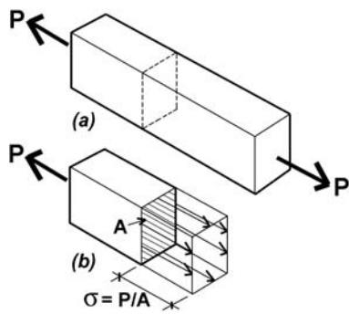
FIGURE 6.1 Illustrations of (a) tension element and (b) free-body diagram cut at any cross section with area, A
