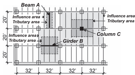
FIGURE 2.6 Framing plan for Example 2.2
