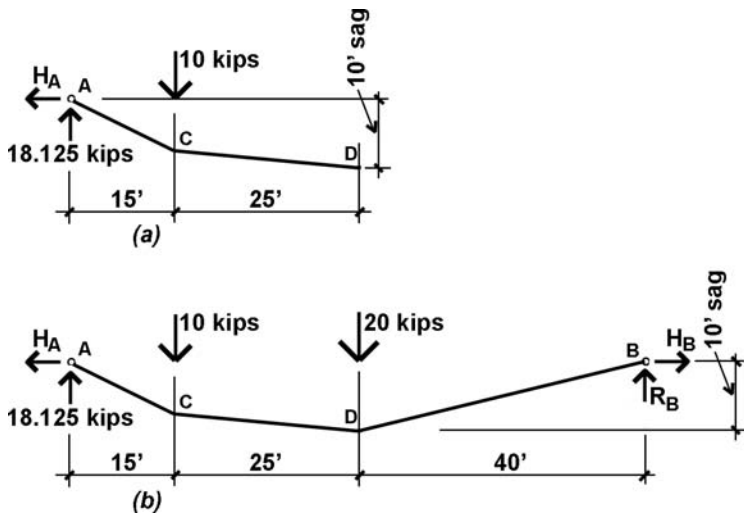
FIGURE 1.25 Free-body diagram cut at the sag point for Example 1.3
