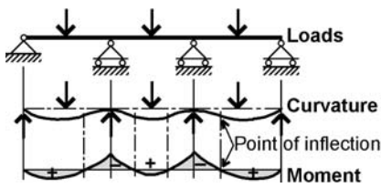
FIGURE 8.5 Continuous beam showing correspondence of points of inflection (change from positive to negative curvature) and points of zero moment
