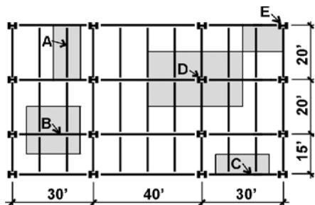
FIGURE 1.5 Framing plan showing tributary areas for beams, girders, and columns
