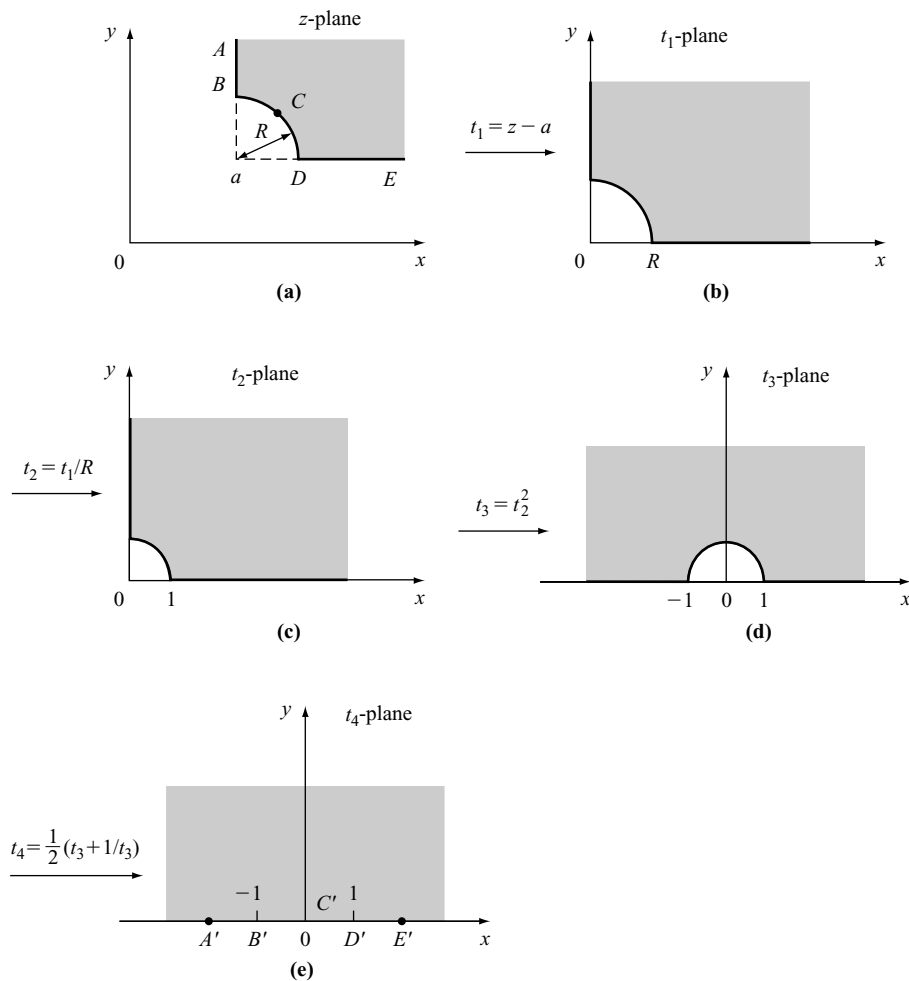
Figure 30.31. The mapping w = \frac{1}{2} \left[ \left( \frac{z-a}{R} \right)^2 + \left( \frac{R}{z-a} \right)^2 \right]
