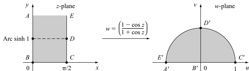
Figure 30.23. The mapping w = \left( \frac{1 - \cos z}{1 + \cos z} \right) .
