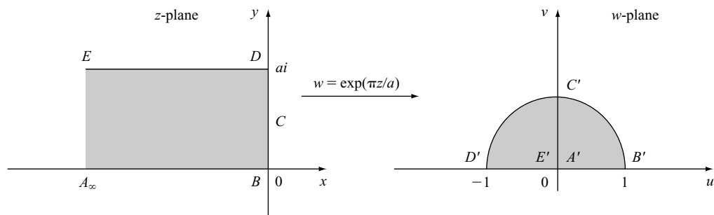
Figure 30.17. The mapping w = \exp(\pi z/a) .
