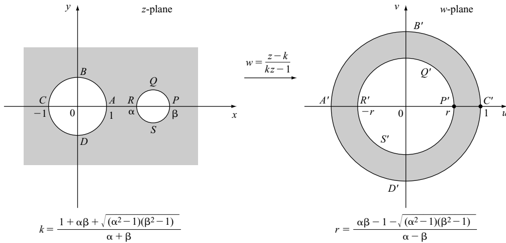
Figure 30.12. The mapping w = f(z) = \frac{z-k}{kz-1} .
