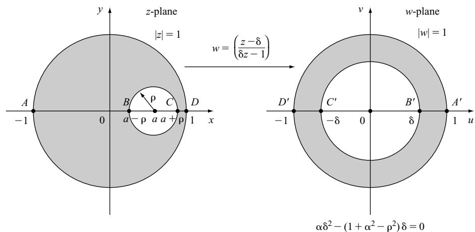
Figure 30.11. The mapping w = \frac{z - \delta}{\delta z - 1} .
