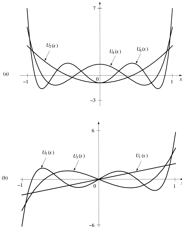
Figure 18.4. Chebyshev polynomials U_n(x) : (a) even polynomials and (b) odd polynomials.
