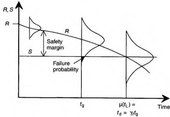
Figure 5.2 The meaning of lifetime safety factor in a performance problem.
