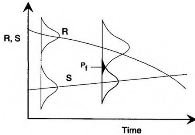
Figure 3.1 The increase of failure probability. Illustrative presentation.
