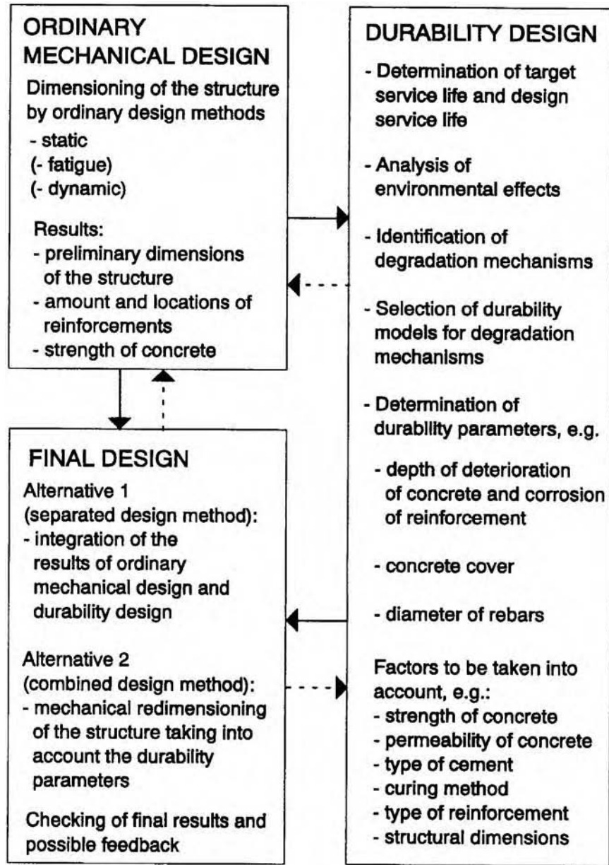
Figure 6.5 Flow chart of the durability design procedure.
