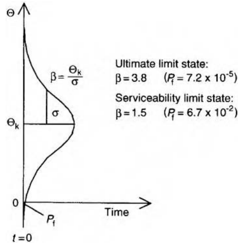
Figure 5.6 Safety requirements for ordinary design according to Eurocode 1.
