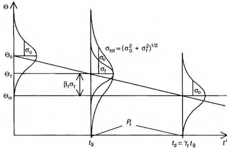
Figure 5.7 Decrease of the safety margin with time.
