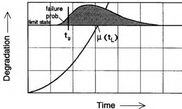
Figure 5.1 Relationship between mean service life and target service life.
