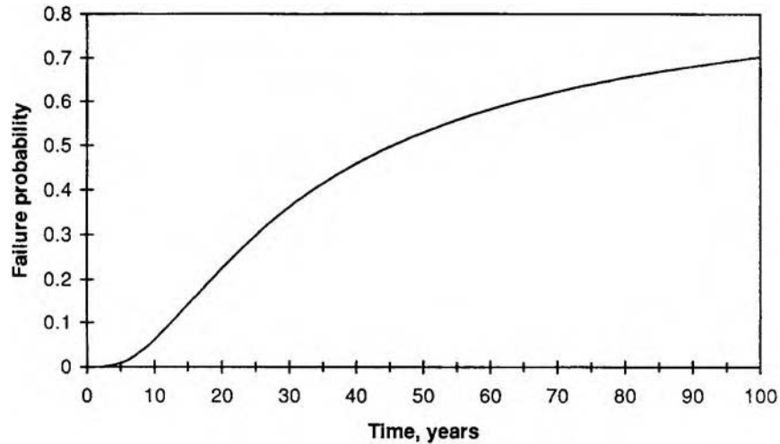
Figure 4.2 Probability distribution function of service life.
