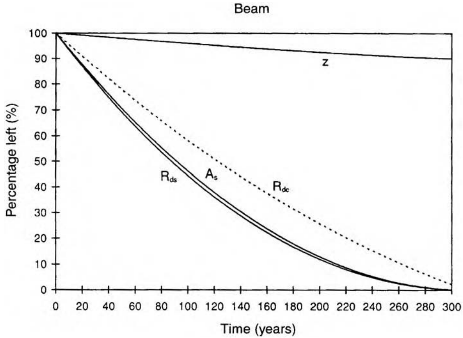
Figure 6.4 Reduction in the bending capacity of a beam.
