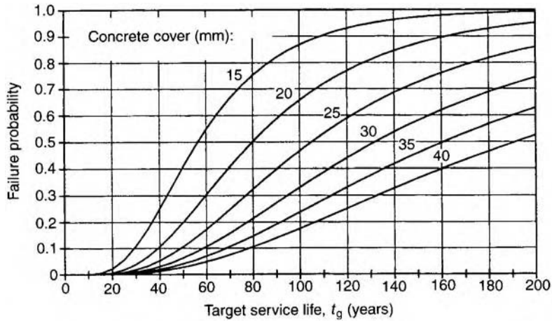
Figure 4.5 Probability of service life being shorter than the target service life when the structures are sheltered from rain. The characteristic cubic strength of concrete is 30 MPa and the diameter of the rebar is 25 mm.
