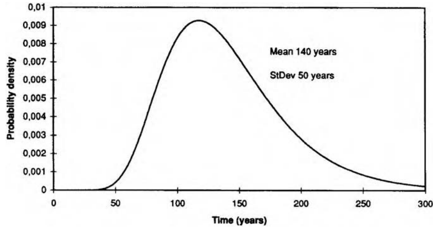
Figure 4.4 Log-normal distribution of service life.
