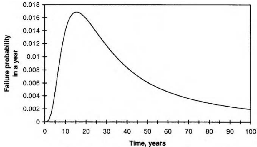
Figure 4.3 Probability density function of service life.
