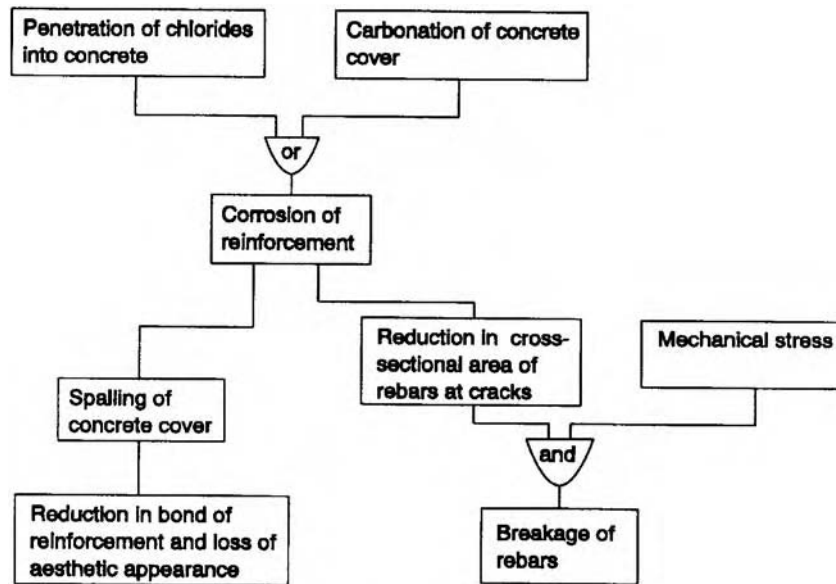
Figure 7.2 Fault tree for the corrosion of reinforcement.
