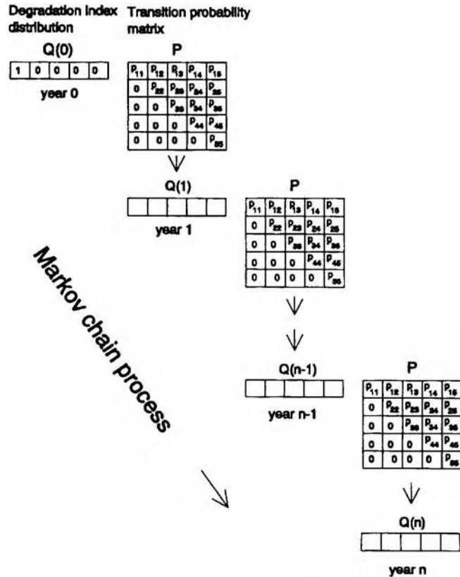
Figure A.1 Principle of the Markov chain method.
