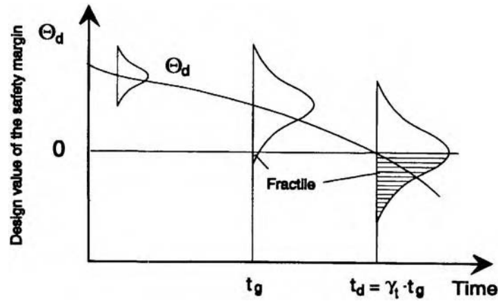
Figure 5.5 Decrease of the design value of the safety margin, and effect of the lifetime safety factor calculated with design values of loads and load-bearing capacities.
