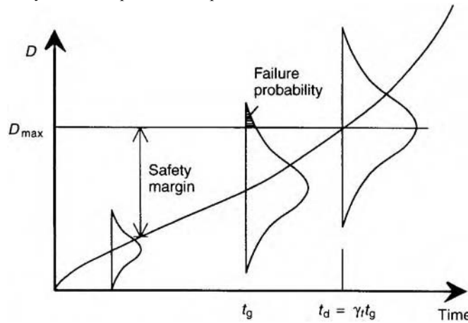
Figure 5.3 The meaning of lifetime safety factor in a degradation problem.
