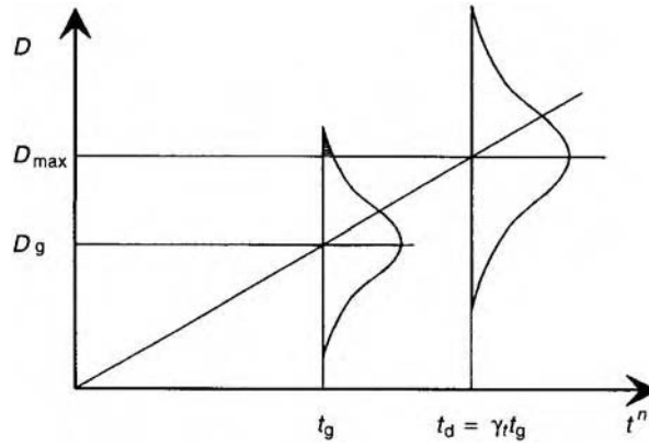
Figure 5.4 Deterioration of lifetime safety factors with normally distributed D .
