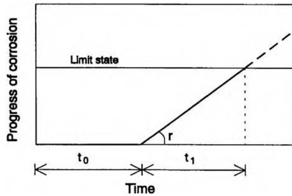
Figure 8.5 Determination of service life with respect to corrosion of reinforcement.
