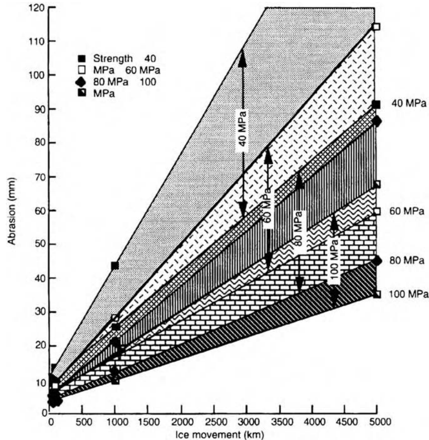
Figure 8.4 Abrasion of concrete for compressive strengths f_{ck}=40, 60, 80 and 100 MPa as a function of ice sheet movement. (Redrawn from S. Huovinen, Publications No. 62 , published by Technical Research Centre of Finland, 1990.)
