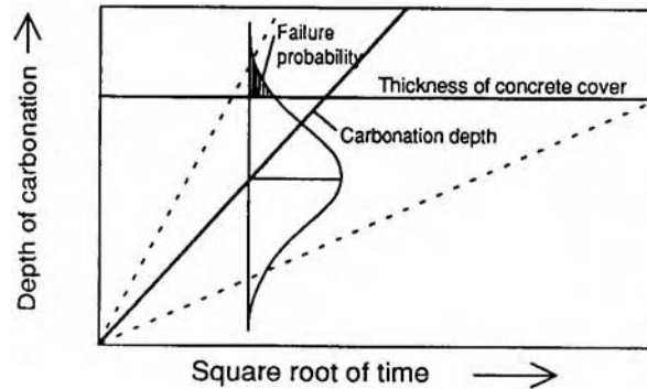
Figure 4.1 Schematic representation of the process of carbonation in a concrete cover.
