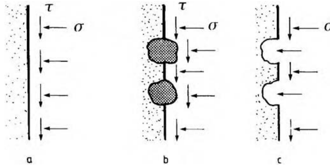
Figure 8.3 Abrasion mechanisms. (Redrawn from S. Huovinen, Publications No. 62 , published by Technical Research Centre of Finland, 1990.)
