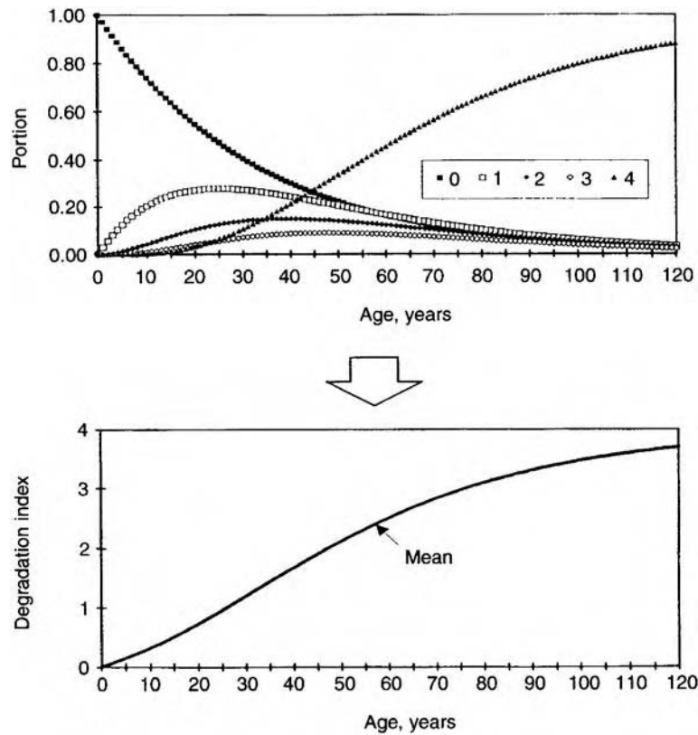
Figure A.2 Degradation index distributions for each year, calculated by the Markov chain method, and curve for the mean degradation index.
