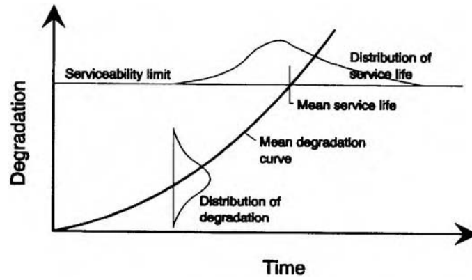
Figure 7.3 Mean degradation and mean service life.
