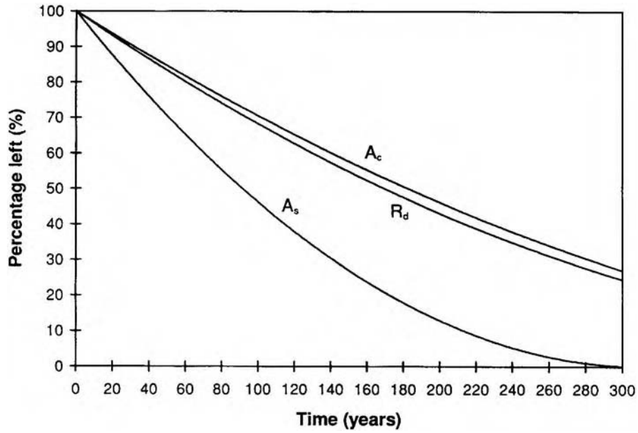
Figure 6.2 Reductions in material cross-sections and compressive capacity of a column.
