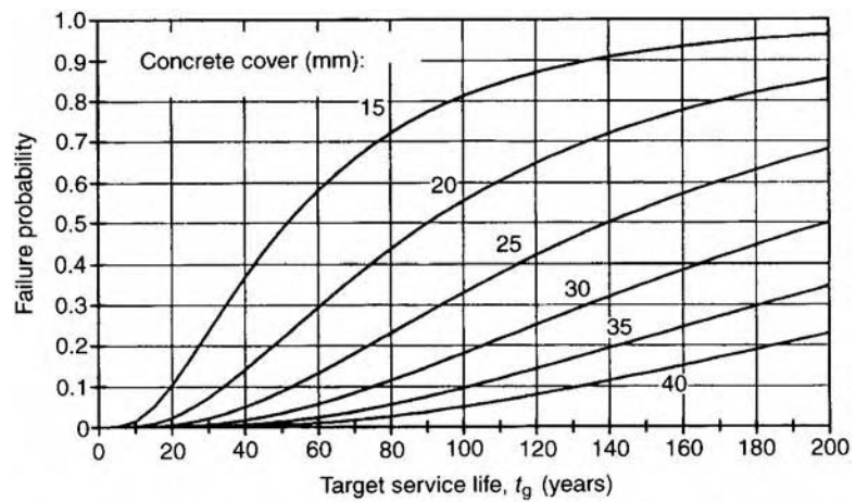
Figure 4.6 Probability of service life being shorter than the target service life when the structures are exposed to rain. The characteristic cubic strength of concrete is 30 MPa and the diameter of the rebar is 25 mm.
