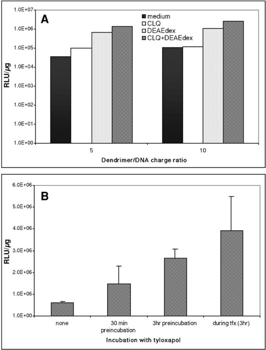
Fig. 4. Augmentation of the dendrimer-mediated transfection by the addition of chloroquine (CLQ) and DEAE-dextran (A) and tyloxapol (B). Rat 2 (A) and Jurkat (B) cells were transfected with 0.5 \mu g of pCF1-Luc DNA complexed with G9 EDA at charge ratios of 5 and 10 (A) and 10 (B). Luciferase activity was measured 36 h after transfection.
