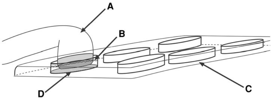
Fig. 1. Application of ultrasound to cells. (A) transducer; (B) culture medium; (C) 6-well plate; (D) cells.
