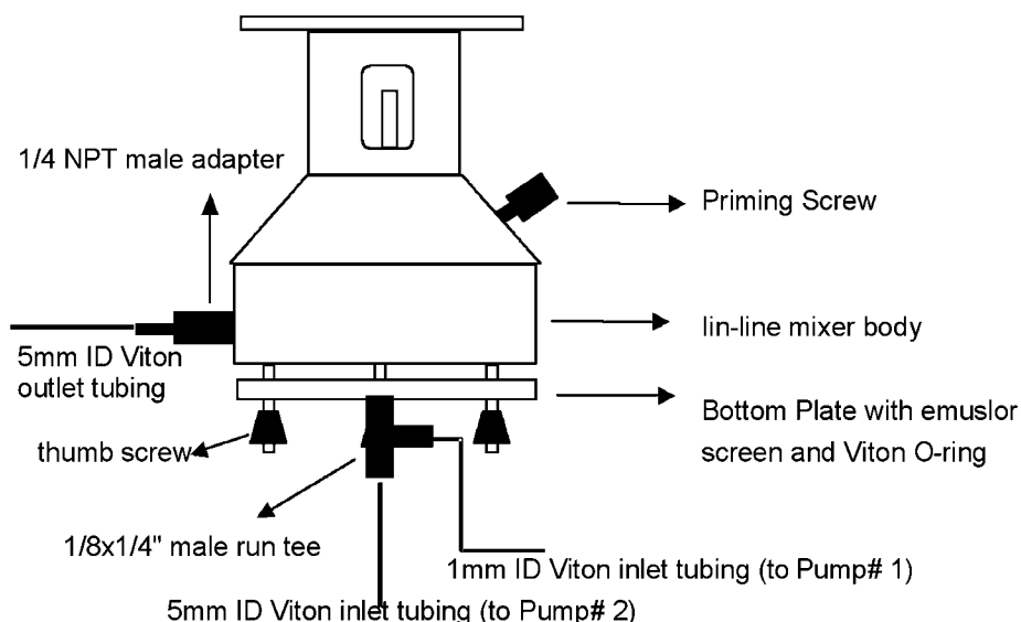
Fig. 1. Set up for production of w/o/w emulsion. A schematic of the in line mixer is depicted. Location of 1-mm and 5-mm viton tubing is indicated.
