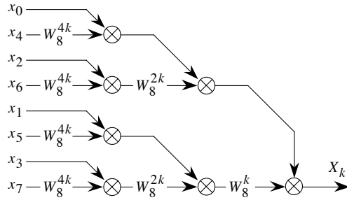
Figure 2.12 – Calculation of one of the FFT's terms
