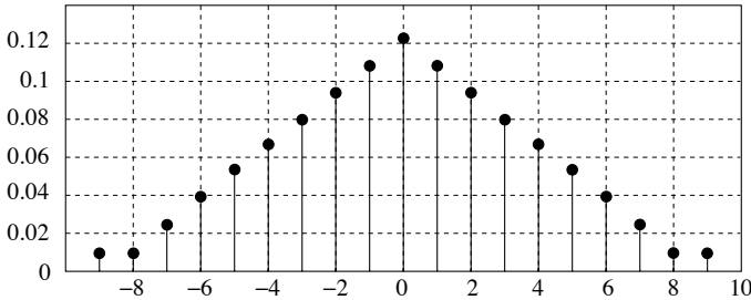
Figure H8.1 – Triangular autocovariance function
