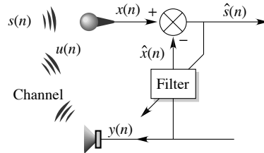
Figure 11.20 – The echo cancellation principle
