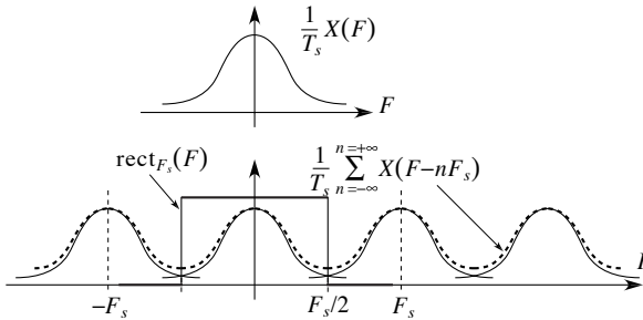
Figure 2.4 – The aliasing phenomenon
