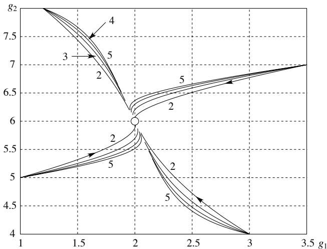
Figure 11.13 – Gradient algorithm: evolution trajectories of the pairs (g_0(n), g_1(n)) as functions of the ratios \rho \in \{2, 3, 4, 5\} of the two eigenvalues of the matrix \mathbf{R} , at a constant power, for four different initialization points. The Wiener filter is \mathbf{g}_w = \{2, 6\}
