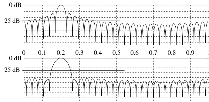
Figure H3.1 – Comparing the rectangular window (above) and the Hamming window (below)
