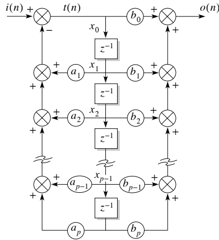
Figure 5.1 – Processing architecture
