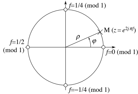
Figure 4.5 – Unit circle
