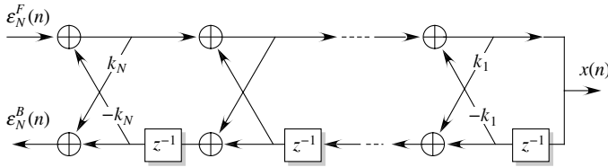
Figure 11.9 – The lattice synthesis filter
