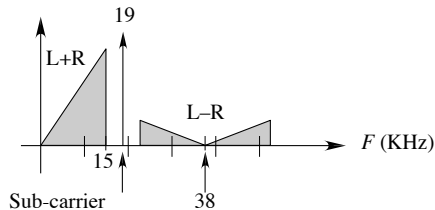
Figure H3.7 – Spectrum of the stereophonic signal used for FM radio broadcasting
