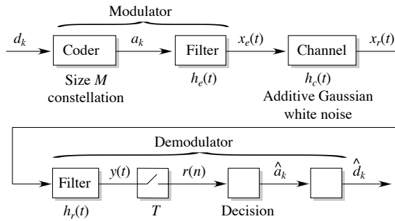
Figure 12.39 – Baseband modulation and demodulation
