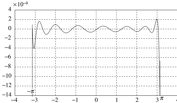
Figure 11.4 – Error resulting from the polynomial approximation
