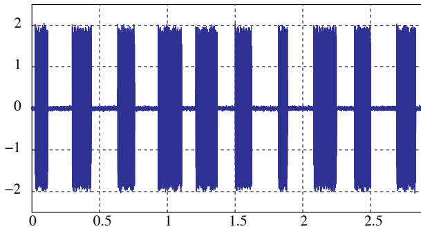
Figure 12.3 – DTMF Signal
