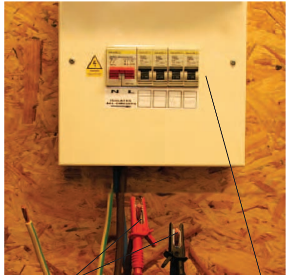
Connected to live conductors
