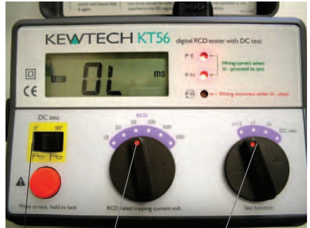
Switch on 180°
