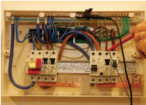
Earthing terminal Between live conductor and earth Phase
