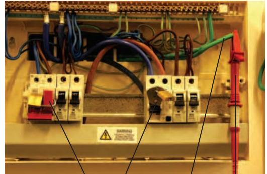
Isolated and locked off Disconnected conductor Test lead conductor
