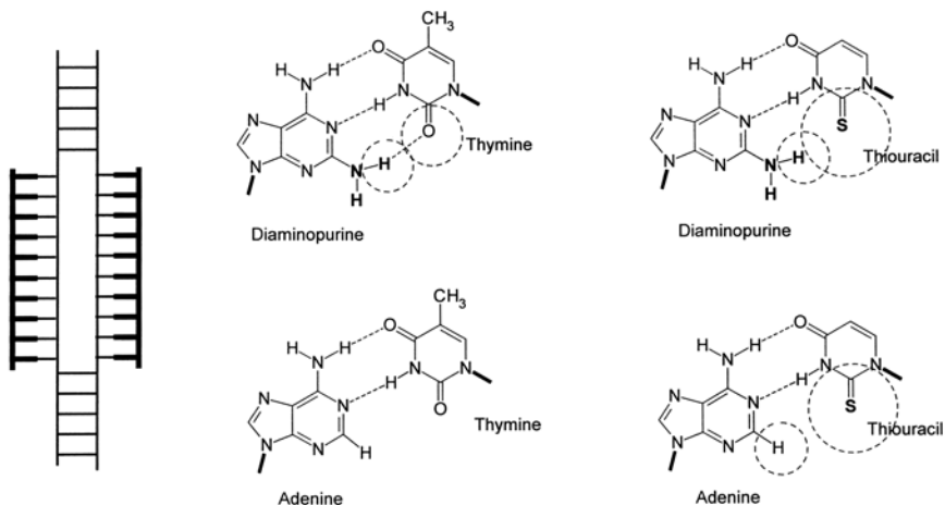
Fig. 3. Interactions in a double duplex invasion complex. Left, double duplex invasion complex. Right: Favorable (diaminopurine-thymine, adenine-thymine, adenine-thiouracil) and unfavorable (diaminopurine-thiouracil) base pairs with the indicated nucleobases and nucleobase analogs.
