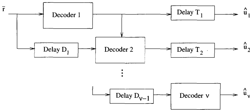
(b) Multistage Decoder
