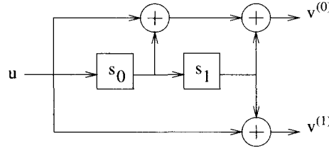
Figure 29 An encoder of a rate-1/2 memory-2 convolutional encoder.
