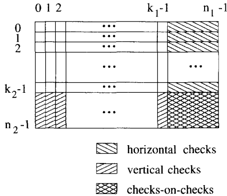
Figure 54 Codeword of a two-dimensional product code.
