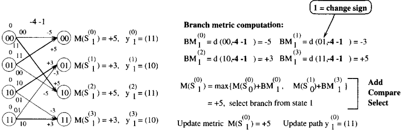
Figure 69 Soft-decision Viterbi decoder operation at i = 1 .
