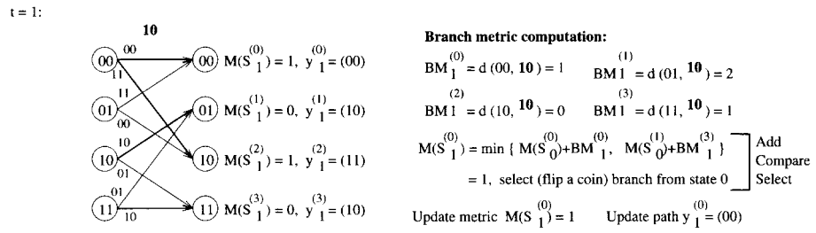
Figure 40 VD operation for Example 62, at i = 0 and i = 1 .
