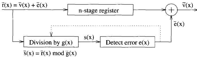
Figure 18 General architecture of a decoder for cyclic codes.
