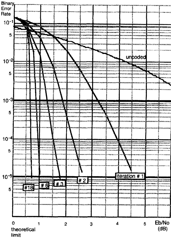
Figure 78 Performance of a rate-1/2 parallel concatenated (turbo) code with memory-4 rate-1/2 RSC codes, \bar{g}_0 = 21 and \bar{g}_1 = 37 . Block interleaver size 256 \times 256 = 65536 . From [BG2]. Reproduced by permission of IEEE. (©1996 IEEE)
