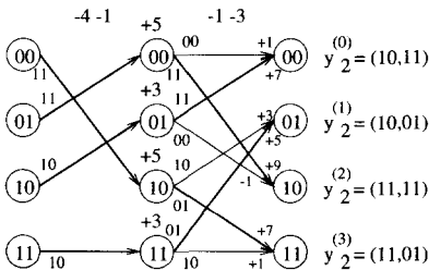
Figure 70 Soft-decision Viterbi decoder operation at i = 2 .
