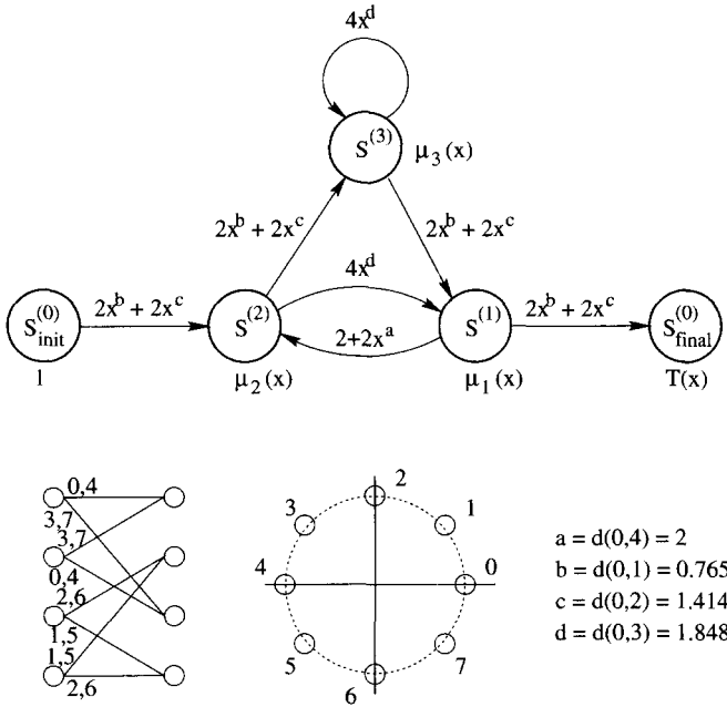
Figure 107 The modified state diagram of a 4-state TC 8-PSK modulation scheme.
