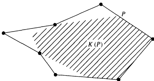
FIGURE 6.21 A polygon and its kernel (shaded region).
