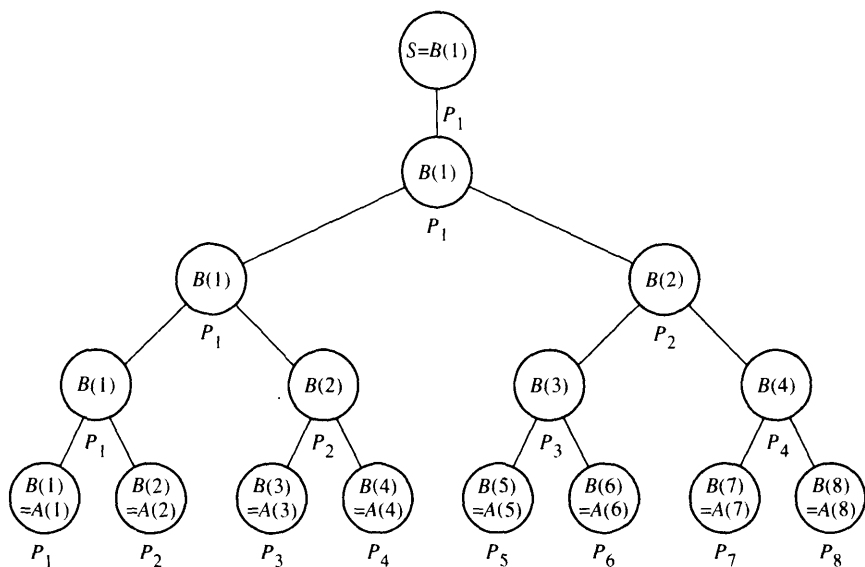
FIGURE 1.4 Computation of the sum of eight elements on a PRAM with eight processors. Each internal node represents a sum operation. The specific processor executing the operation is indicated below each node.
