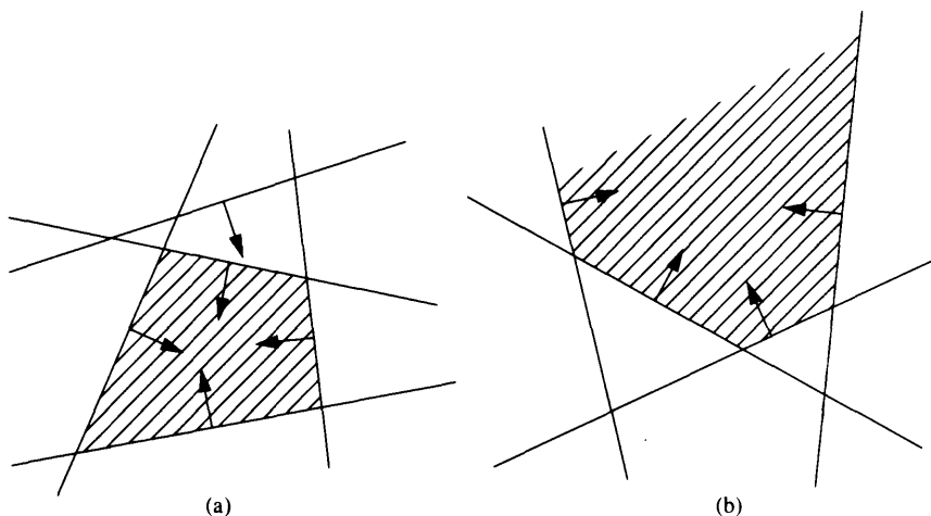
FIGURE 6.6 Intersections of a set of half-planes. (a) Bounded case. (b) Unbounded case.
