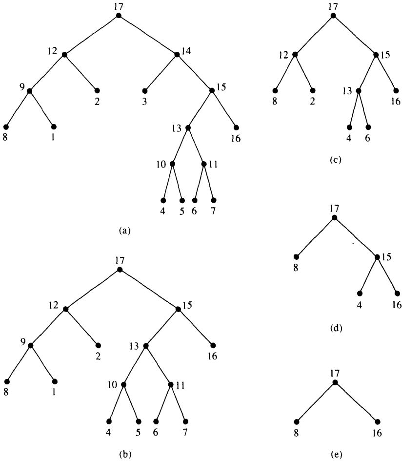
FIGURE 3.14 Tree contraction. (a) Initial tree; (b) tree after raking of node 3; (c) tree after raking of nodes 1, 5, and 7; (d) tree after raking of nodes 2 and 6; (e) the final tree obtained after raking of node 4.
