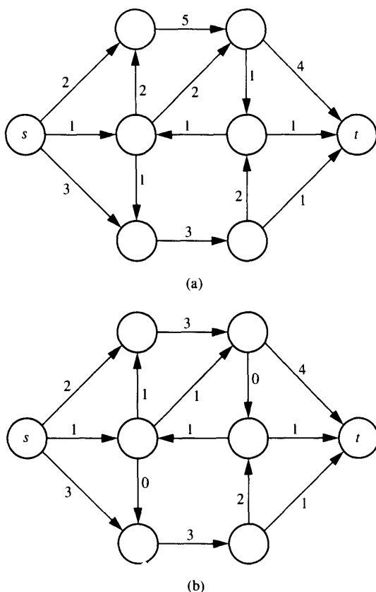
FIGURE 10.7 Network and corresponding maximum flow. (a) A network with the edge capacities. (b) A maximum flow of value 6.
