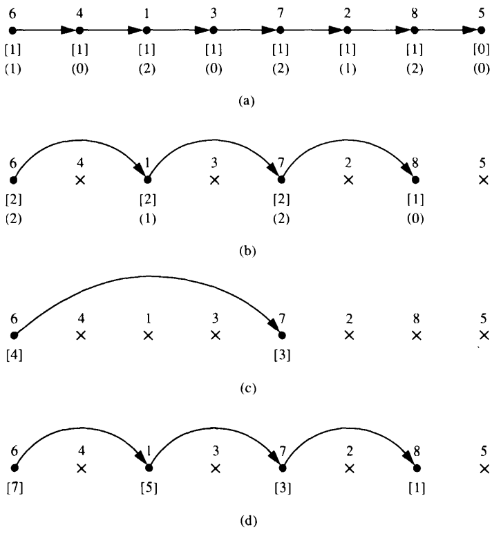
FIGURE 3.2 A linked list and its processing by Algorithm 3.3. (a) The initial list; the initial R values are given in brackets, and a 3-coloring is shown in parentheses. (b), (c) The lists obtained during the contraction process. (d) Restoration of the nodes removed from the list in (c).
