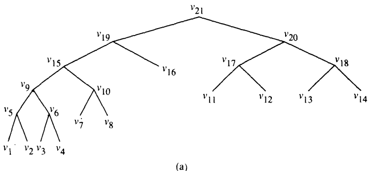
FIGURE 4.7 The tree for Example 4.8. (a) A binary tree.
