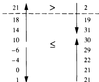
FIGURE 4.13 The horizontal cut for the given bitonic sequence.
