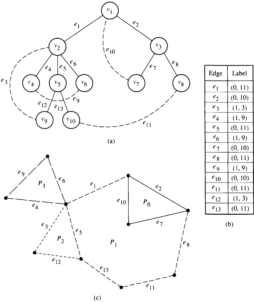
FIGURE 5.17 Ear decomposition for the graph of Example 5.11. (a) A graph G , where the tree edges are shown in solid lines and the remaining edges shown in dashed lines. (b) The labels of all the edges. (c) The decomposition determined by the ear-decomposition algorithm. The edges in each ear are drawn using a different type of lines. The cycle P_0 consists of all the edges with the label (0, 10), P_1 corresponds to the label (0, 11), P_2 corresponds to the label (1, 3), and P_3 corresponds to the label (1, 9).
