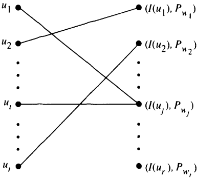
FIGURE 10.1 The bipartite graph for the proof of Lemma 10.4. u_i is connected to (I(u_j), P_{w_j}) if and only if u_i affects P_{w_j} at time t + 1 with input I(u_j) .
