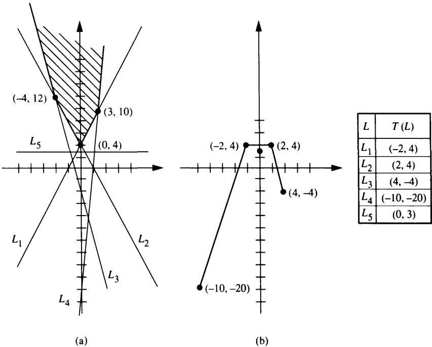
FIGURE 6.8 The five lines for Example 6.5. (a) Intersections of a set of upper half-planes determined by the lines L_1 , L_2 , L_3 , L_4 , and L_5 . (b) The transformation T maps the five lines in (a) into the five points shown in (b), as indicated by the accompanying table; the ordered upper hull of these points uniquely define the polygonal chain of the region formed in (a).
