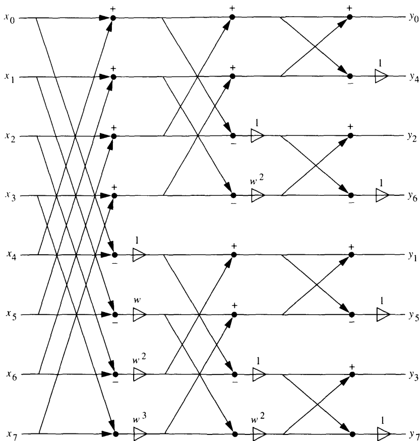
FIGURE 8.2 The FFT algorithm for n = 8 .
