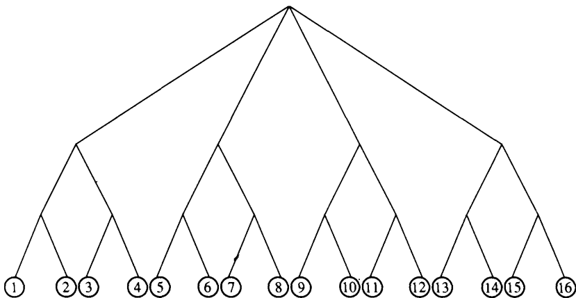
FIGURE 2.12 Doubly logarithmic-depth tree on 16 nodes.
