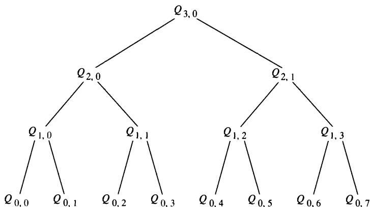
FIGURE 8.3 The binary tree used for polynomial evaluation.
