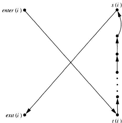
FIGURE 10.13 The path taken on visiting enter(i) , whenever g_i has the value 0.
