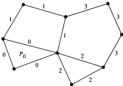
FIGURE 5.16 An ear decomposition of G consisting of four ears, such that the edges in ear P_i are all marked with the index i .
