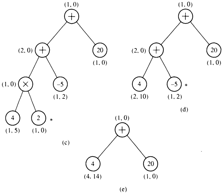
FIGURE 3.16 (continued) (c) The tree generated at the end of the first iteration of the tree-contraction algorithm. (d, e) The trees obtained during the last two iterations.
