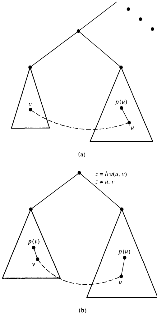
FIGURE 5.13 Pairs of edges defining the relation R'_C . (a) (u, v) is a nontree edge such that v < u ; hence, the pair of edges (u, v) and (u, p(u)) belong to R'_C . (b) (u, v) is a nontree edge such that u and v are not related; hence, (u, p(u)) and (v, p(v)) belong to R'_C .
