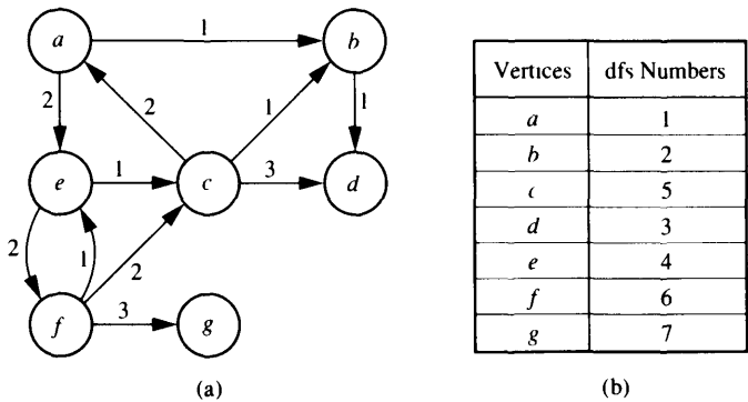
FIGURE 10.6 Graph for ordered depth-first search. (a) A directed graph with the arcs numbered according to their order of appearance on the adjacency lists. (b) The depth-first search numbers of the vertices, with a as the starting vertex.
