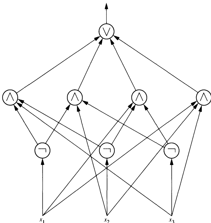
FIGURE 10.2 A circuit for the parity function of three variables.
