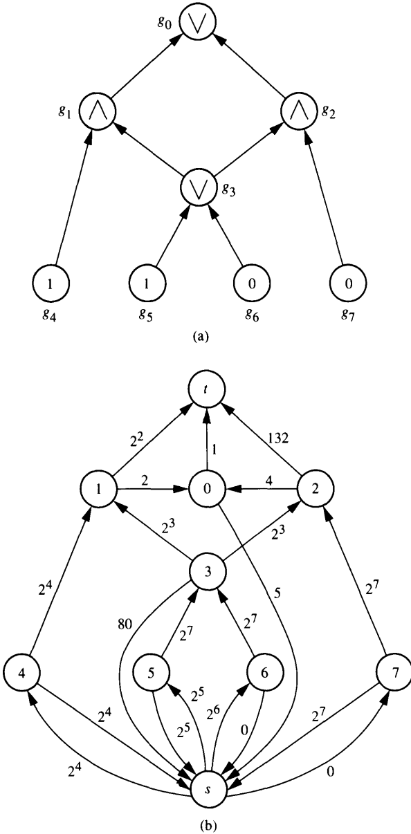
FIGURE 10.16 A circuit and its corresponding network. (a) A Boolean circuit describing an instance of MCVP2. (b) The network corresponding to the circuit shown in (a).
