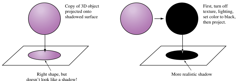
Figure 17.26 Projective shadow technique.
