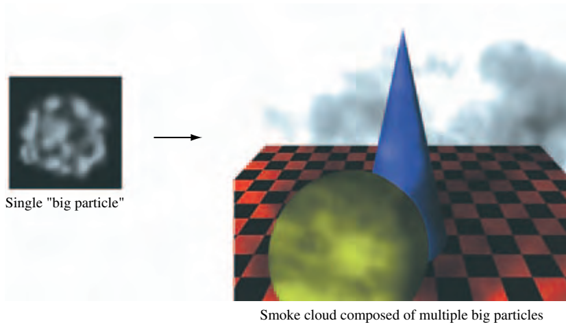
Figure 18.1 Big particles.
