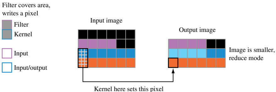
Figure 4.5 Convolution.
