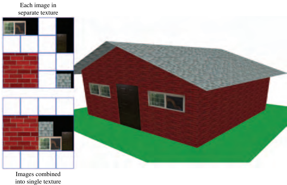
Figure 14.3 Texture mosaicing.
