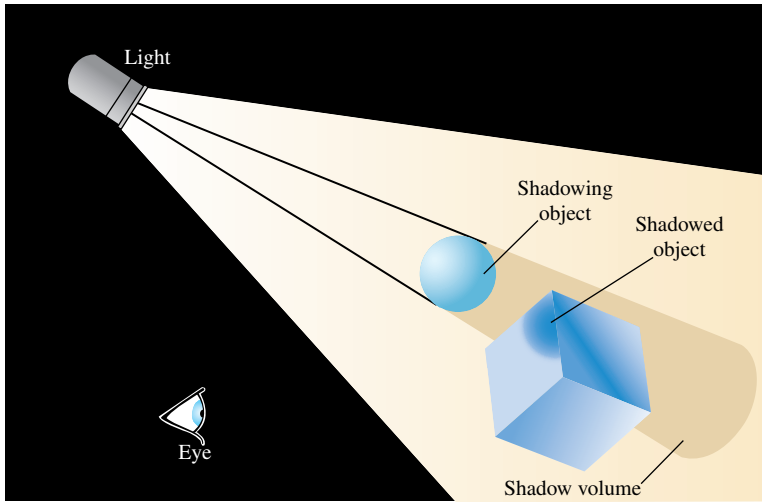
Figure 17.27 Shadow volume.
