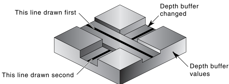
Figure 16.7 Haloed line.
