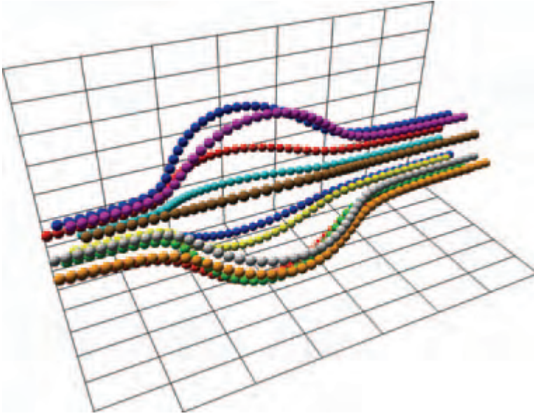
Figure 20.19 Particle tracing.
