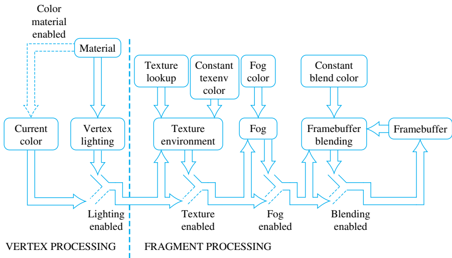
Figure 3.3 Color-processing path.
