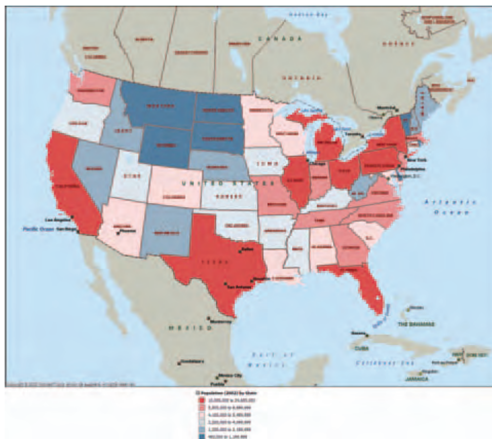
Figure 20.8 Census choropleth.
