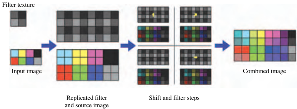
Figure 18.12 Output image.
