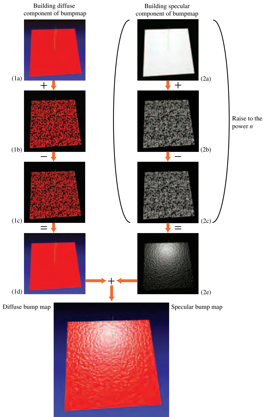
Figure 15.13 Bump mapping: shift and subtract image.
