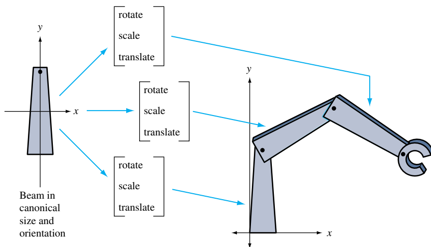
Figure 2.6 Modeling transform as part of model description.
