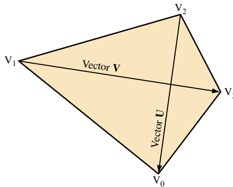
Figure 1.7 Computing quadrilateral surface normal from vertex cross-product.
